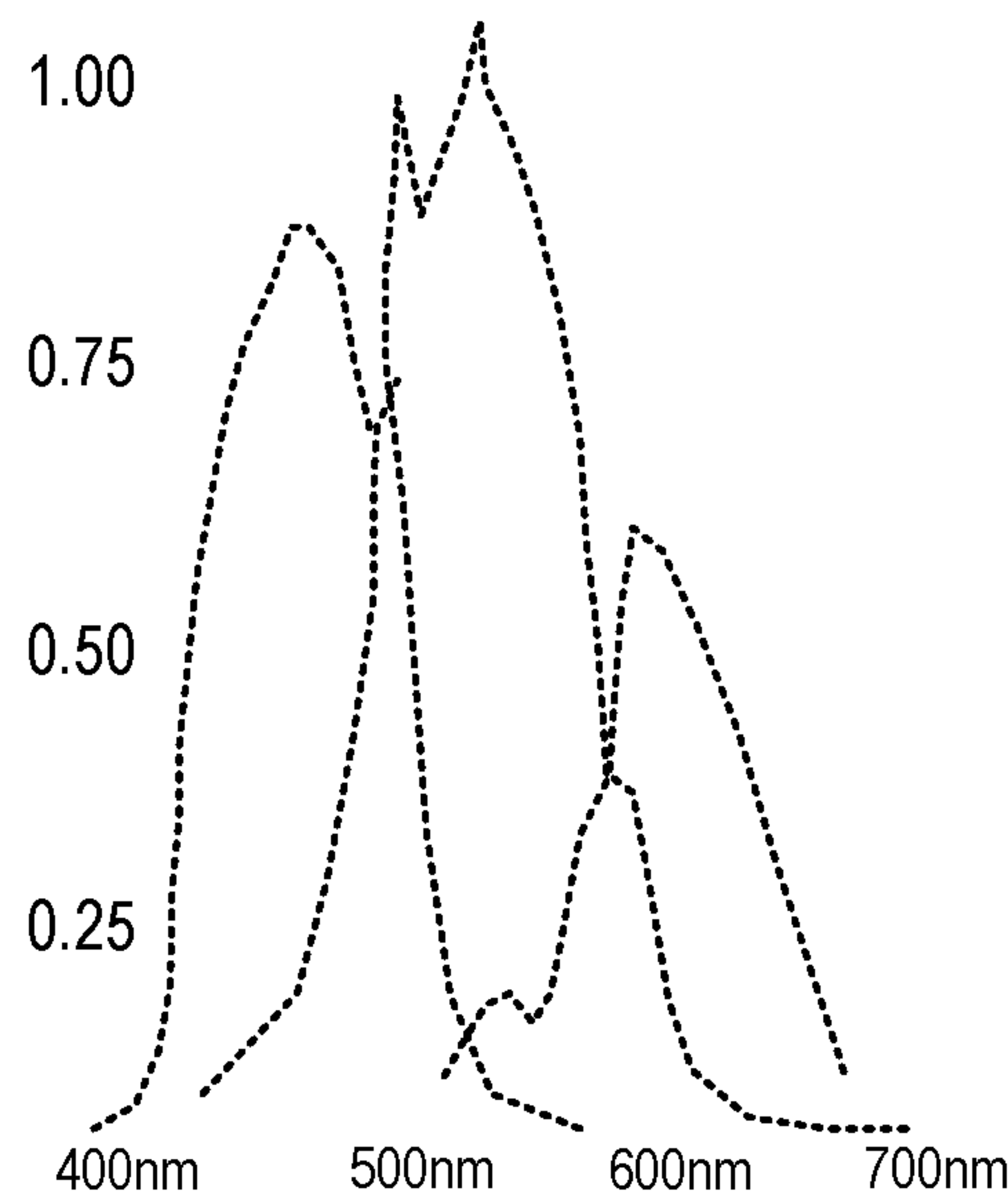
Known Sensor Response Curves. Here we show the three channels of a typical camera (RGB)
