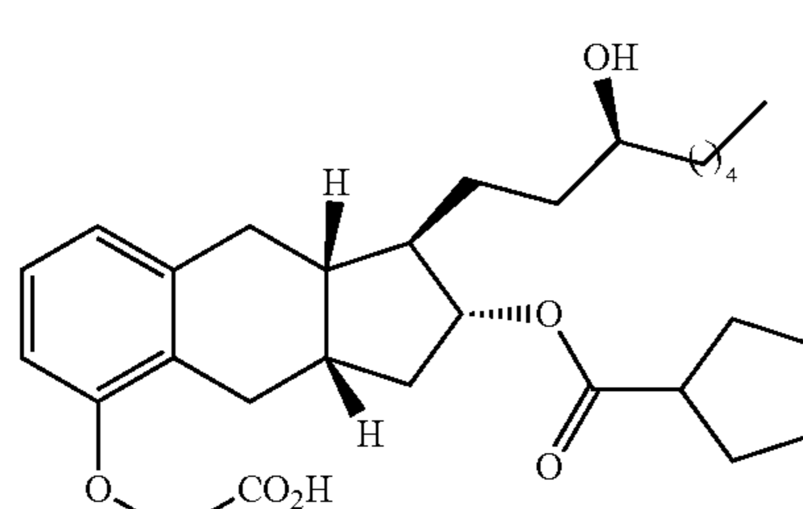
Compound Ia-30
