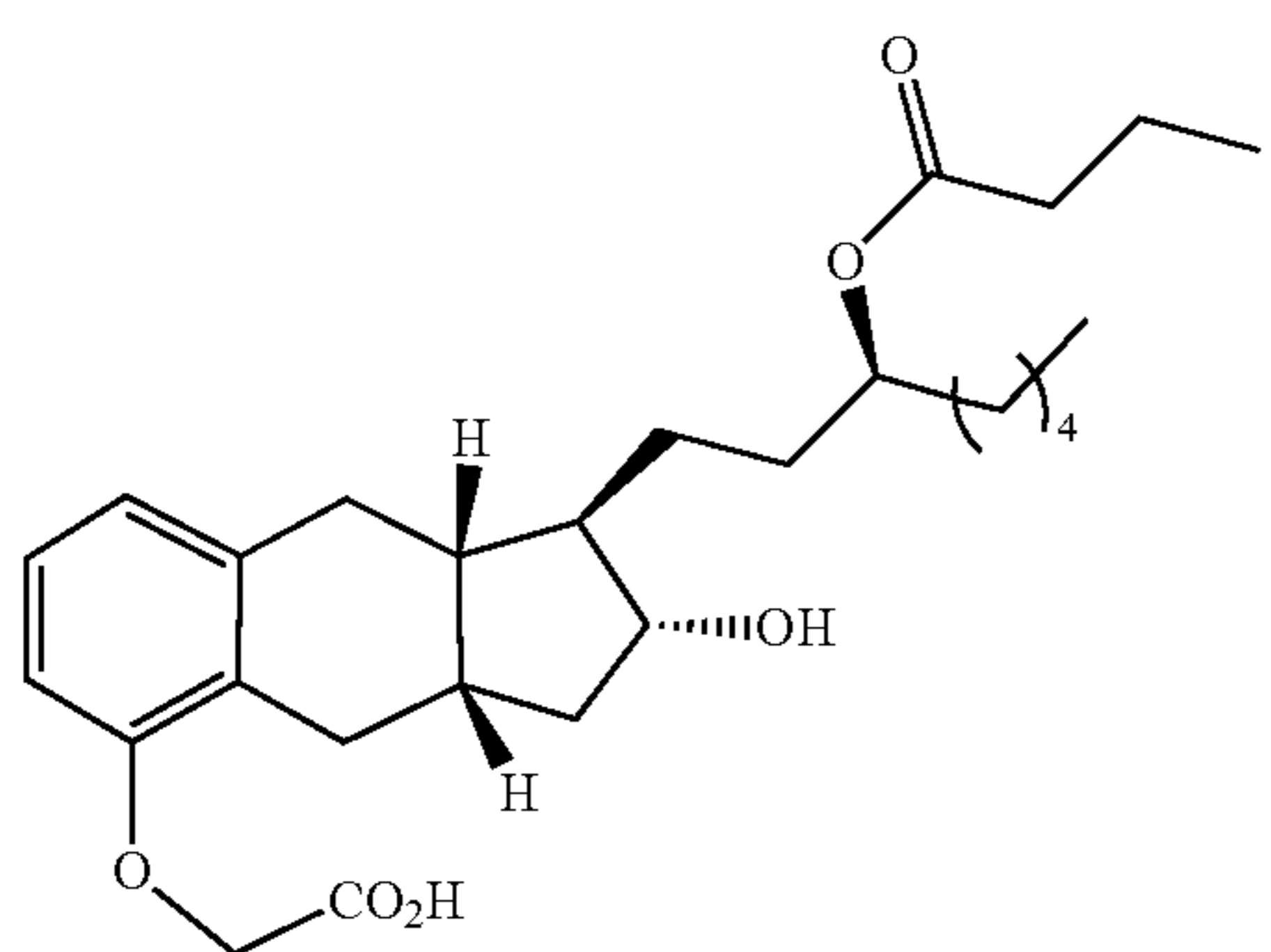
Compound Ib-2
