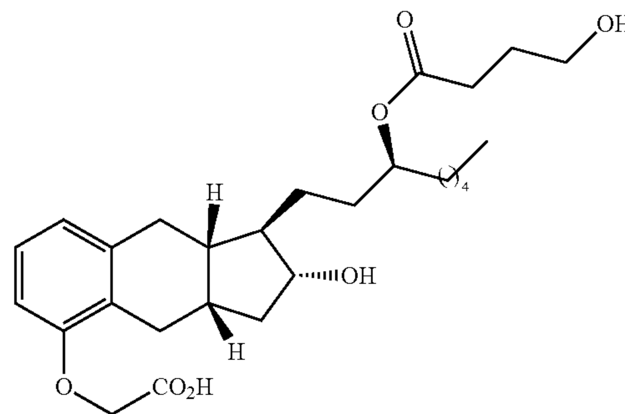
Compound Ib-18
