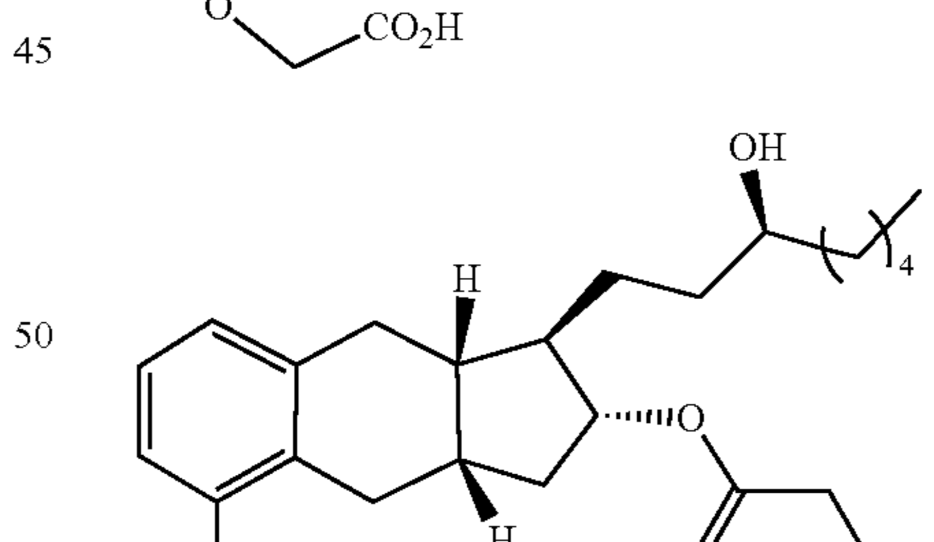
Compound Ia-6
