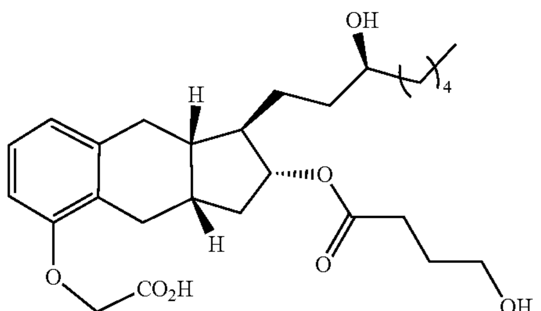
Compound Ia-19
