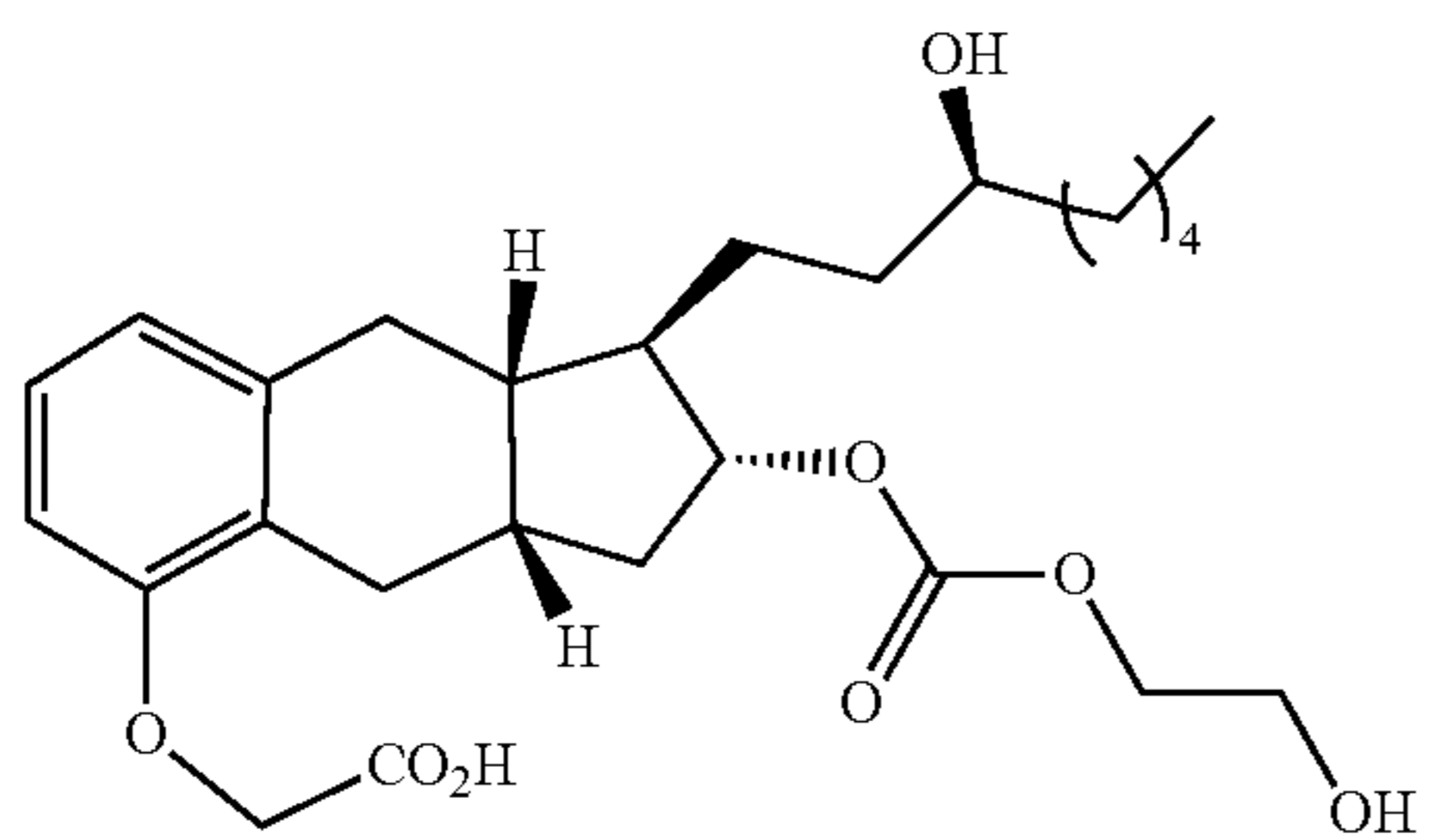
Compound Ia-15
