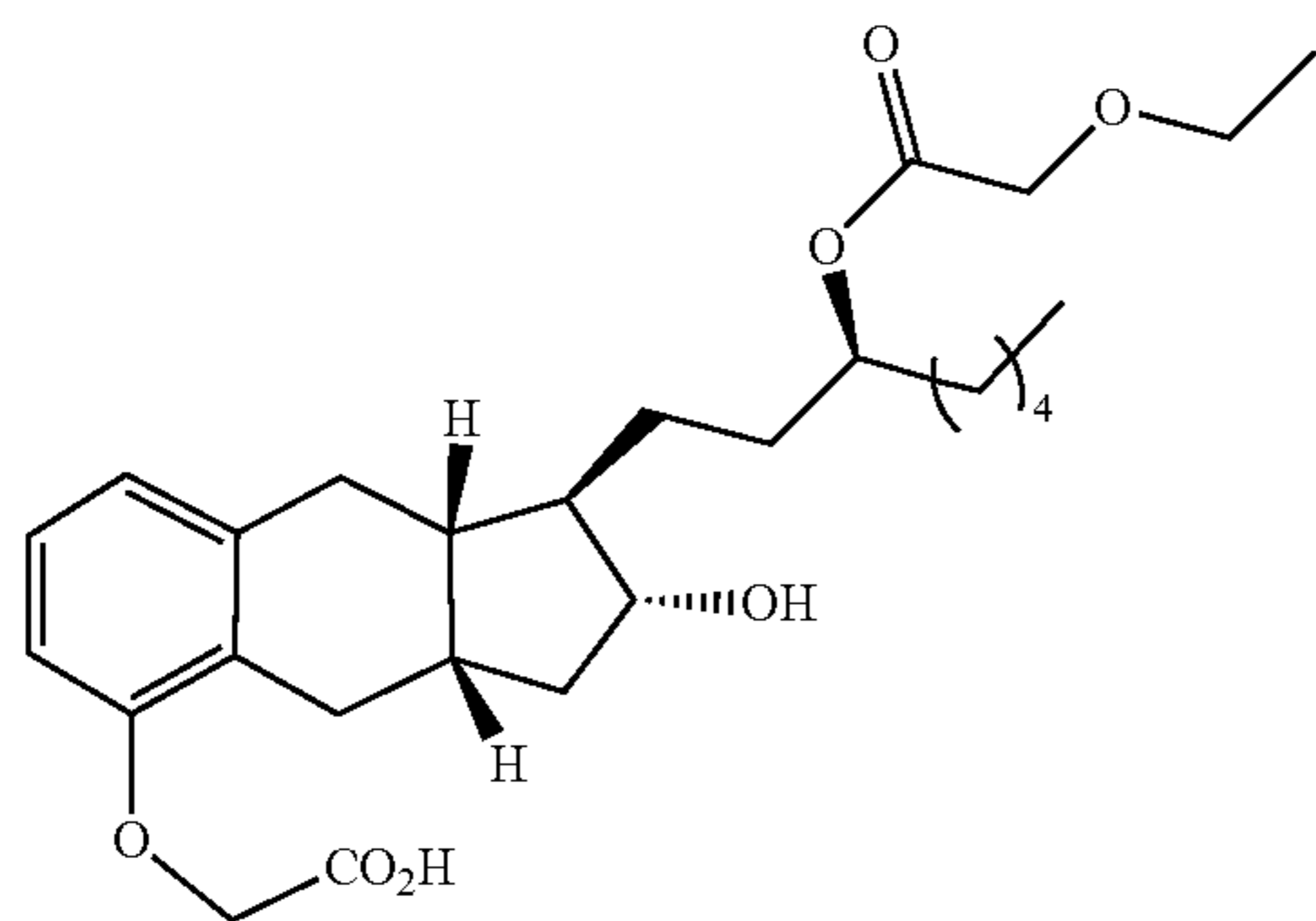
Compound Ib-9
