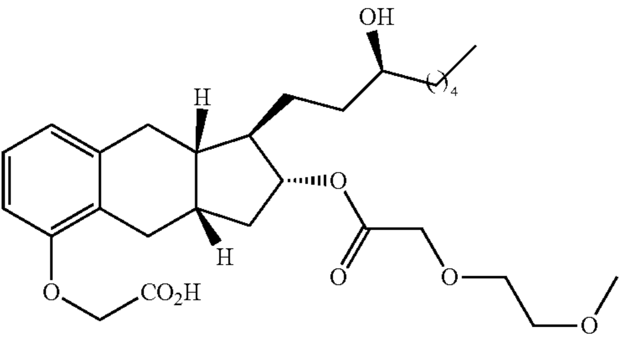
Compound Ia-21
