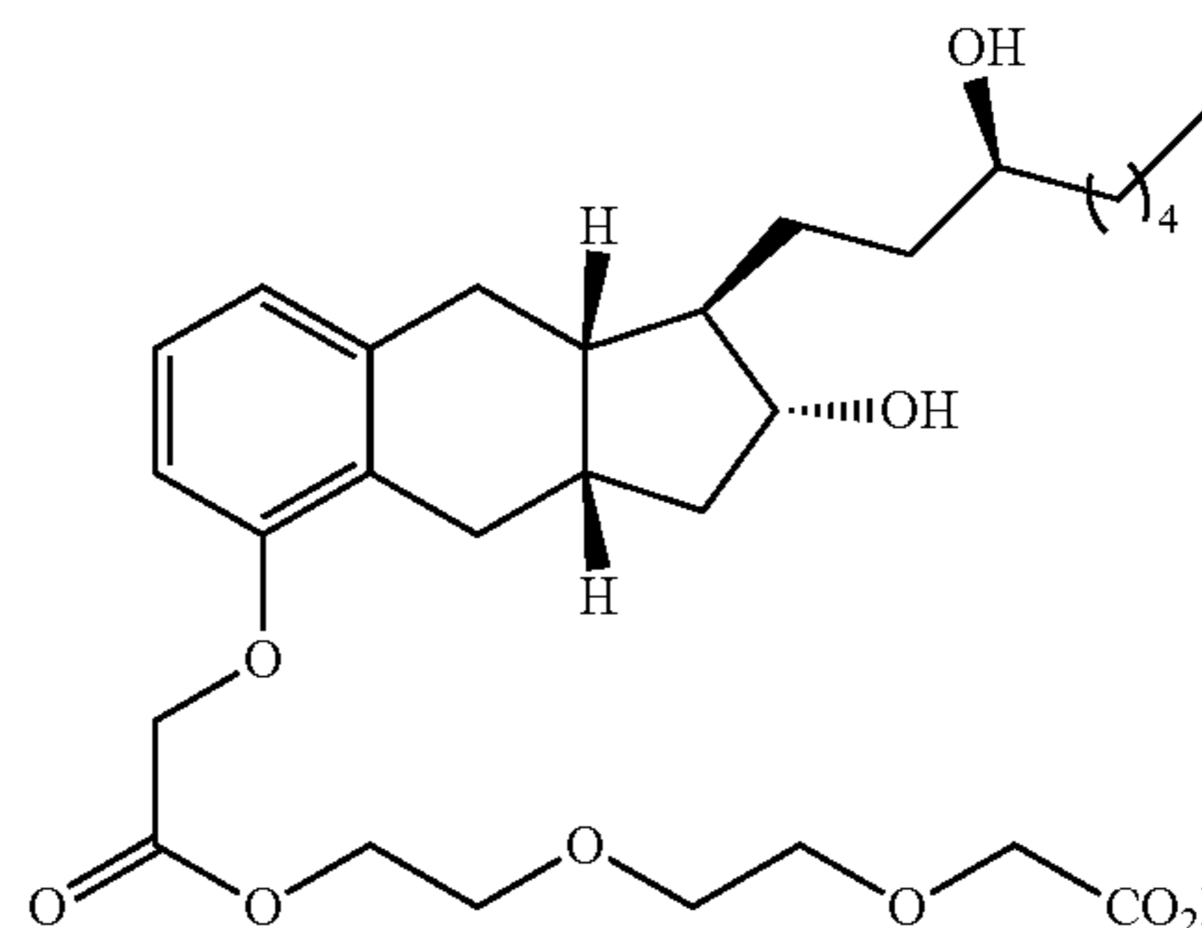
Compound II-17
