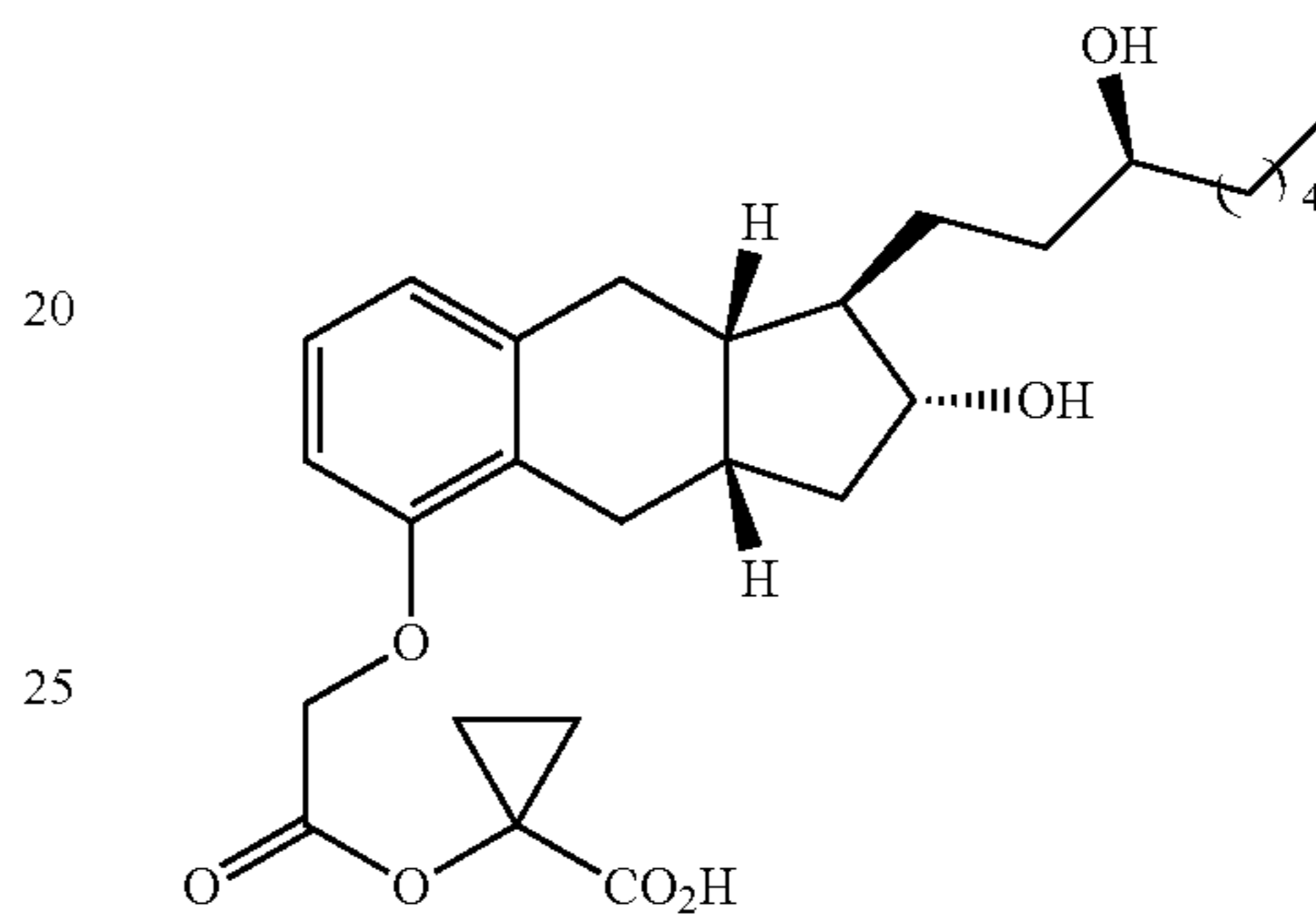
Compound II-23
