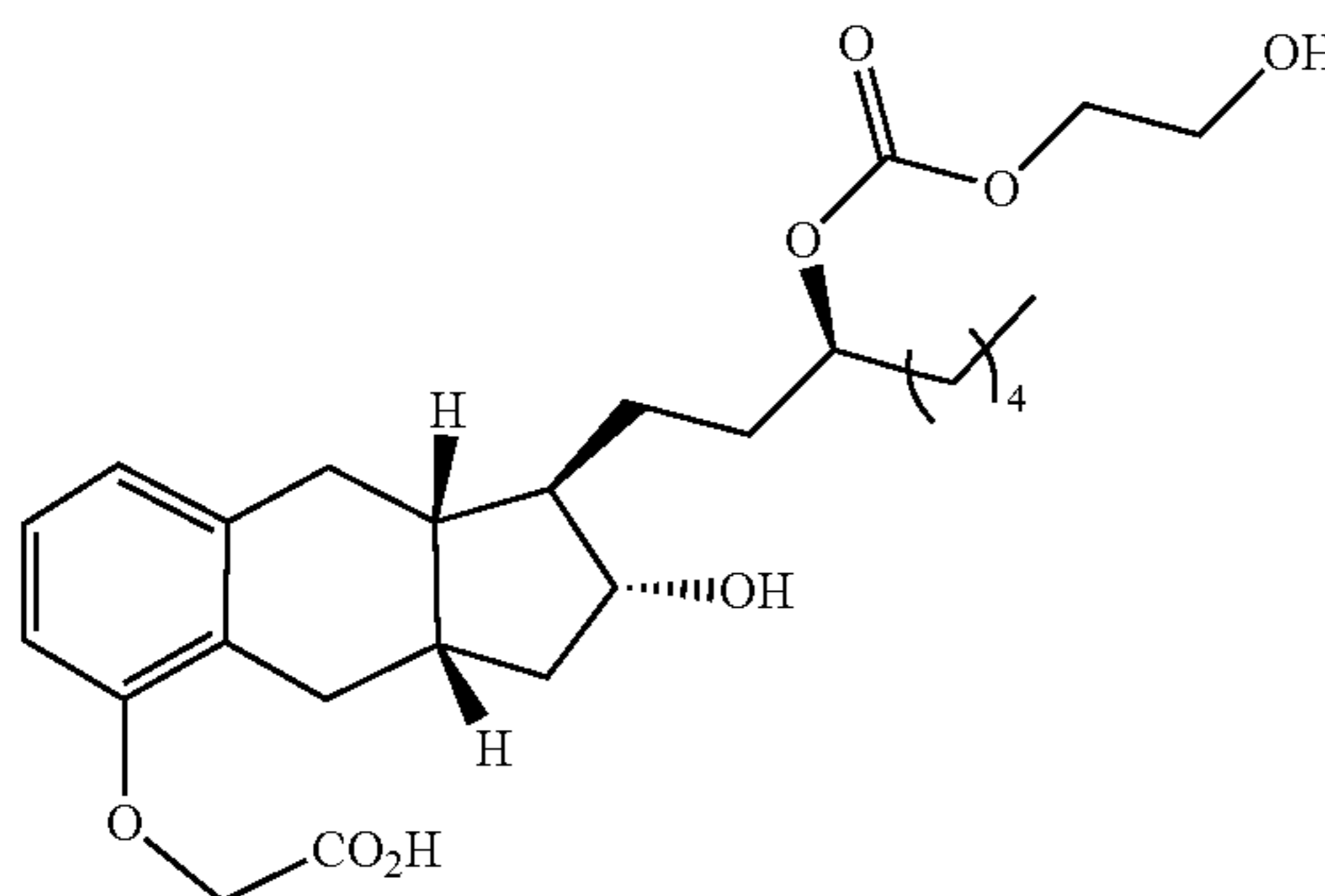
Compound Ib-14
