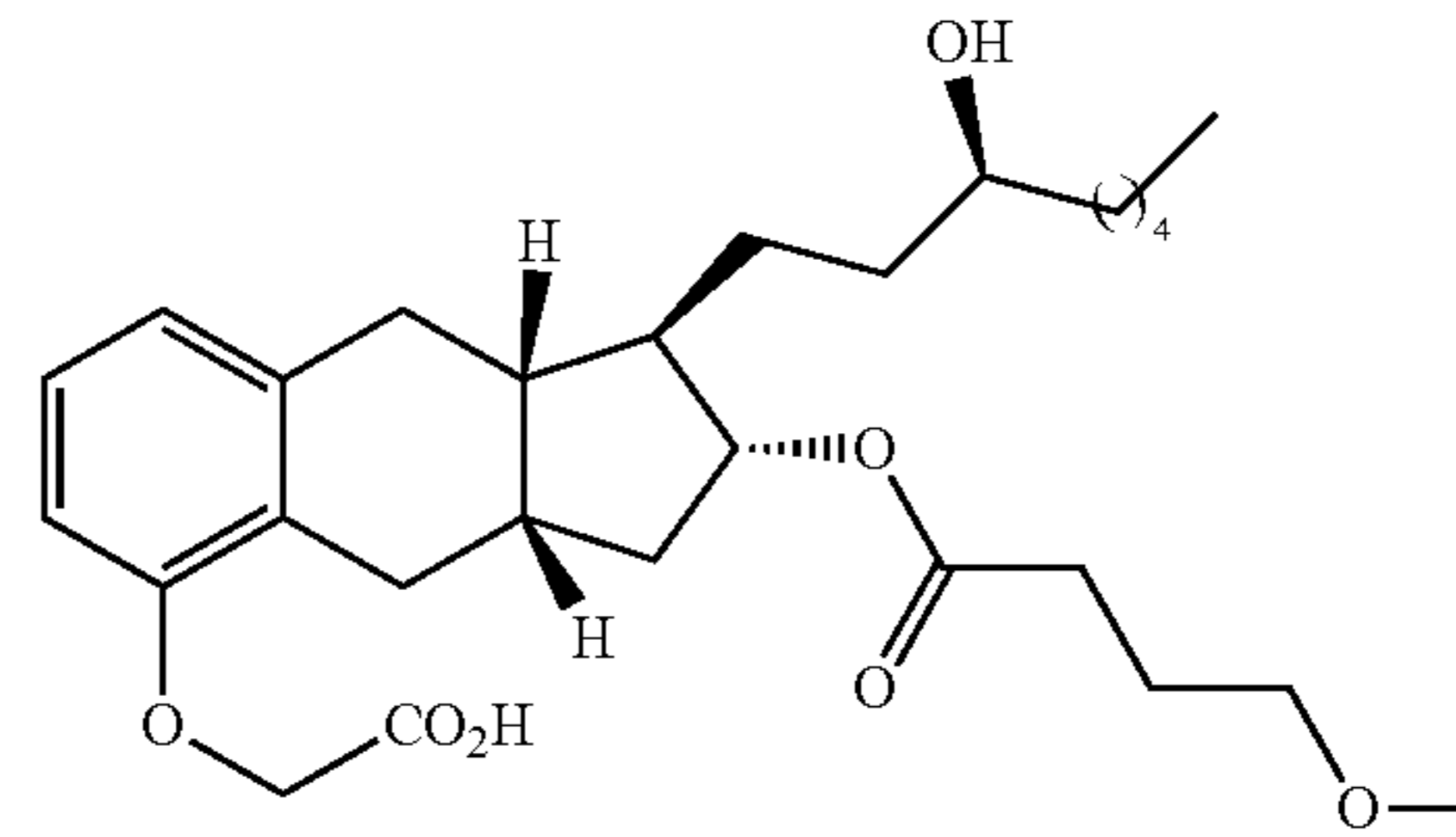
Compound Ia-19
