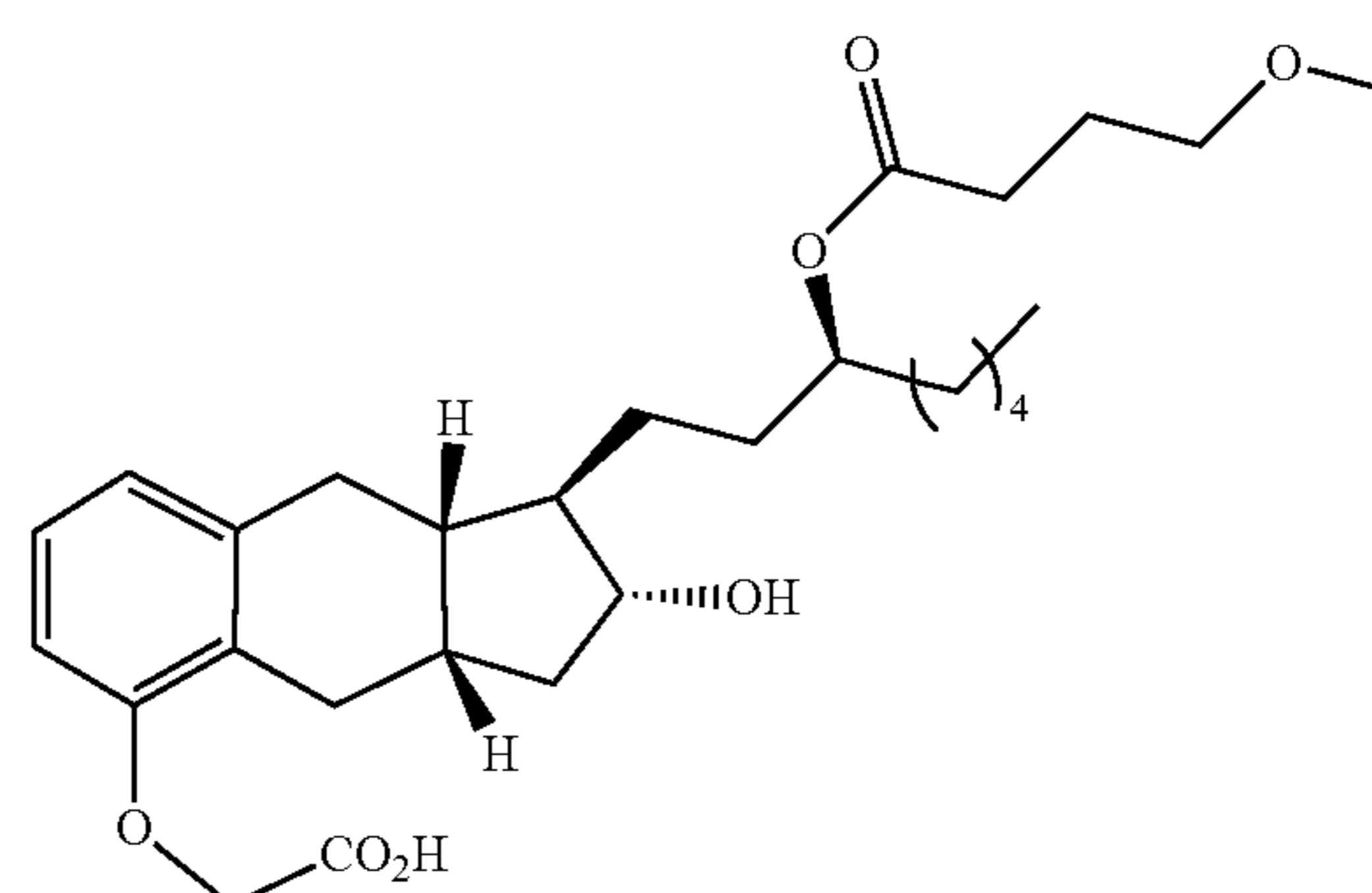
Compound Ib-20
