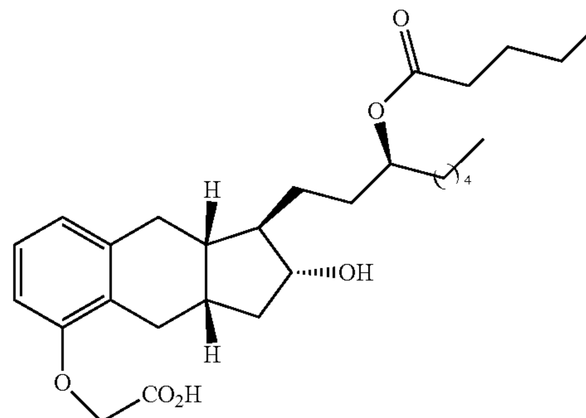
Compound Ib-3
