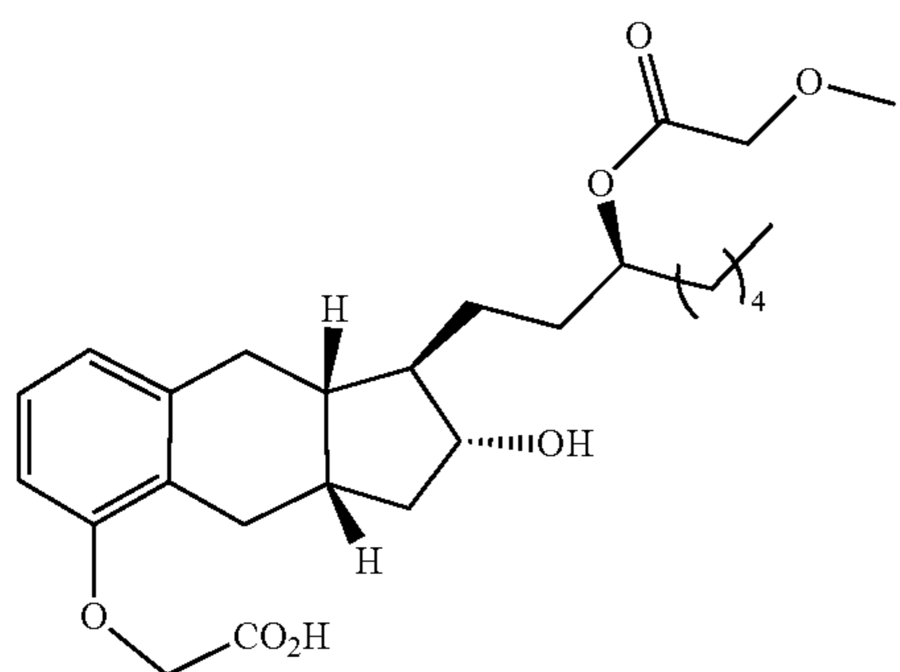
Compound Ib-8
