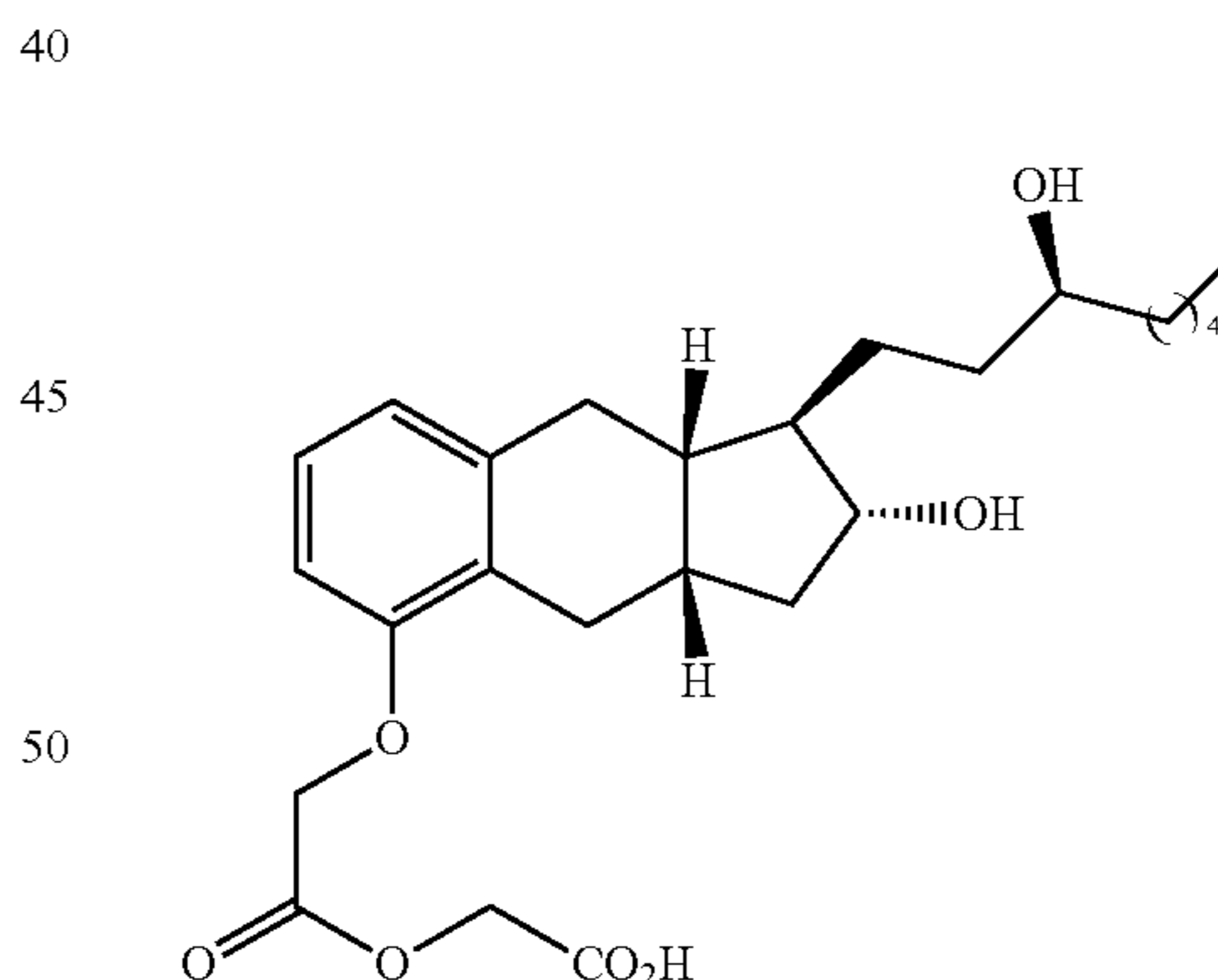
Compound II-1
