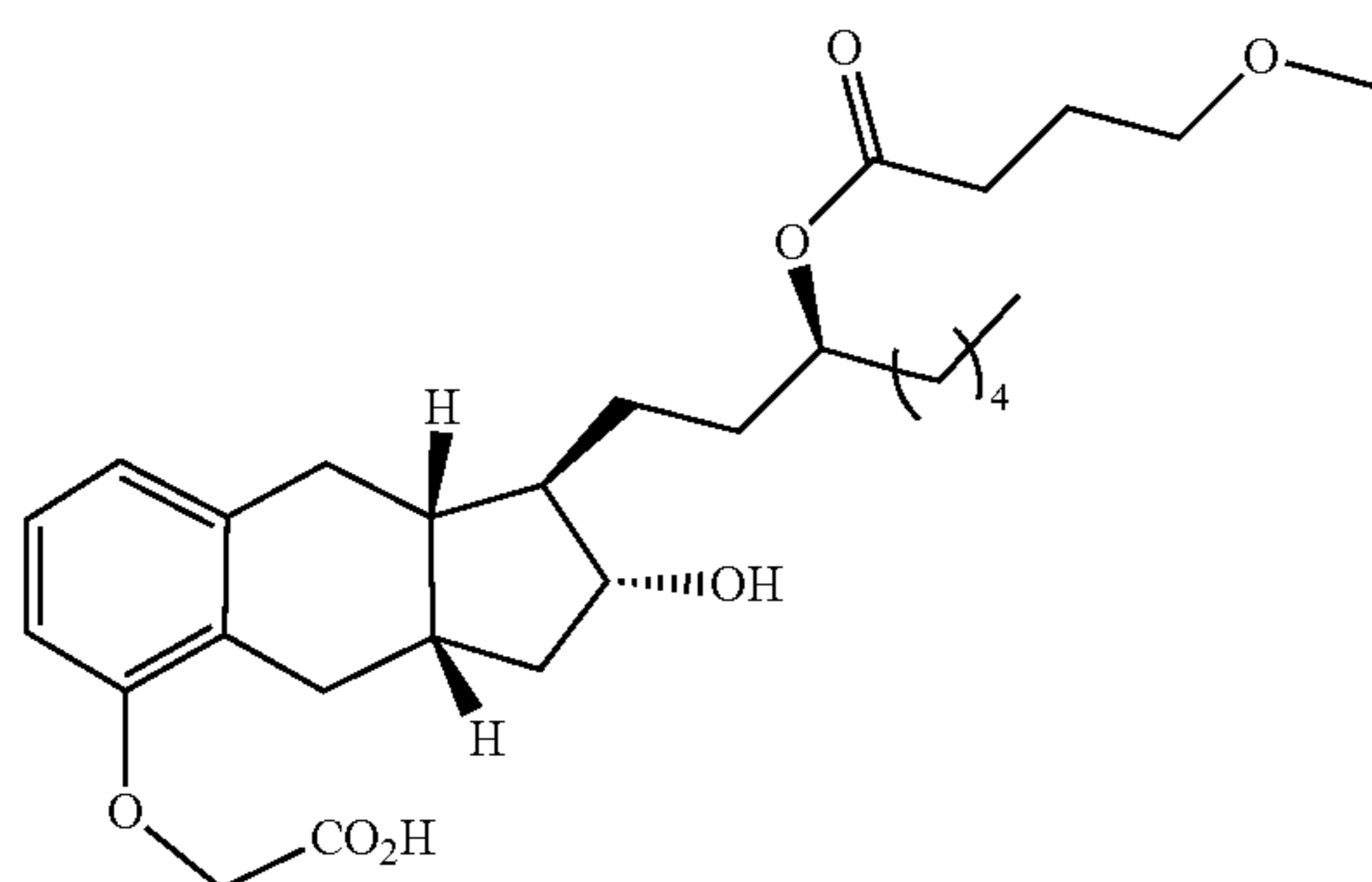
Compound Ib-20
