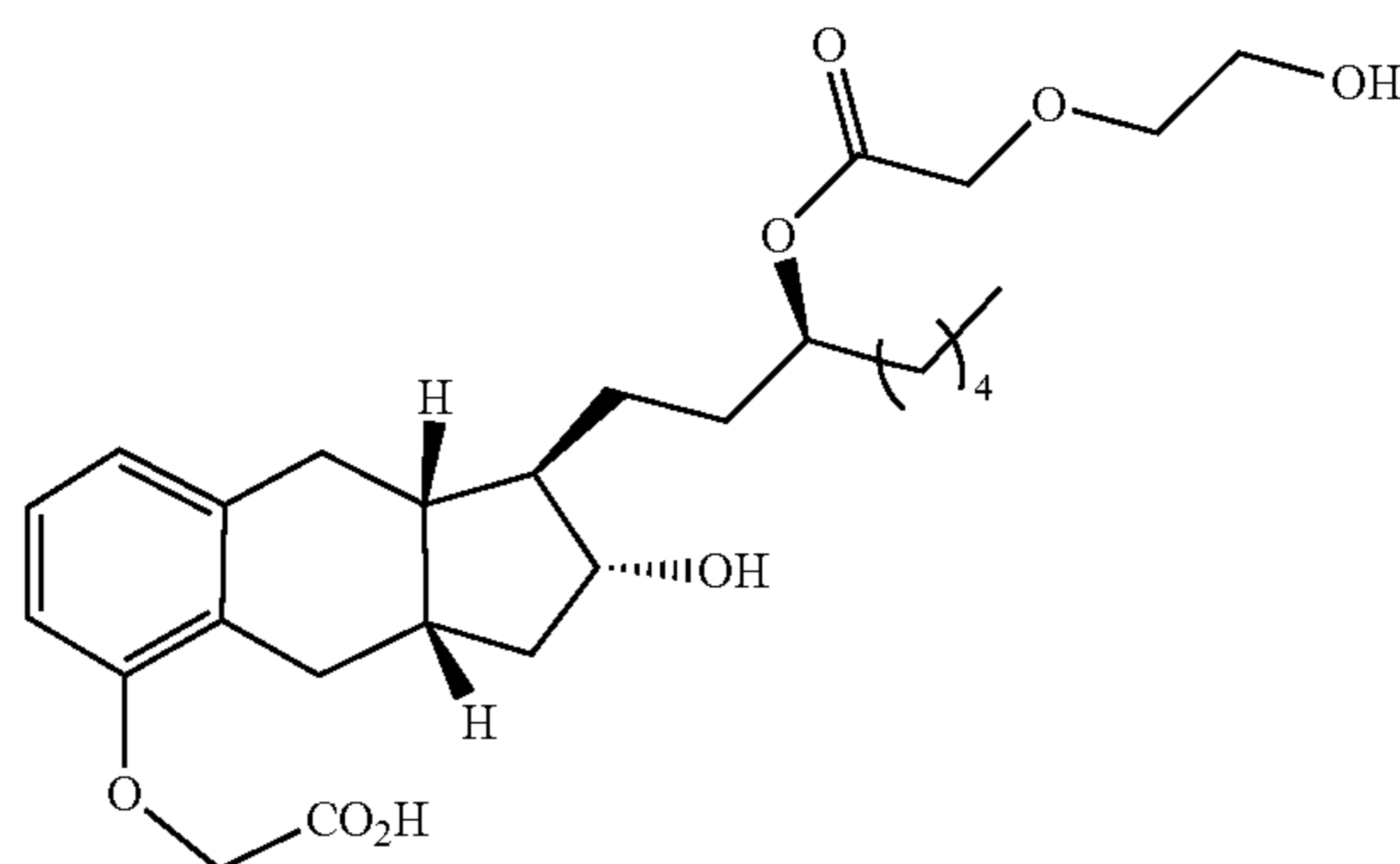
Compound Ib-20
