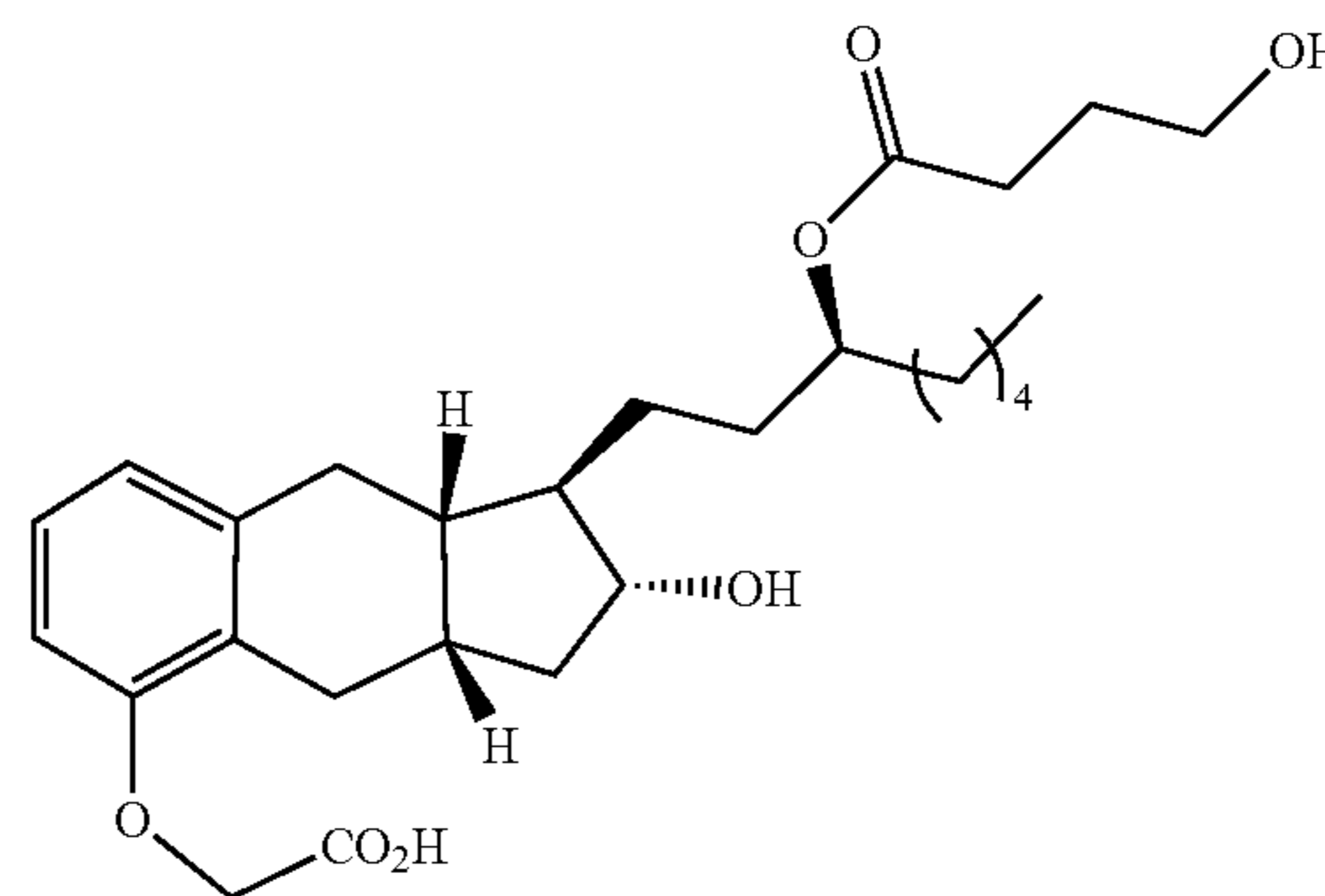
Compound Ib-18
