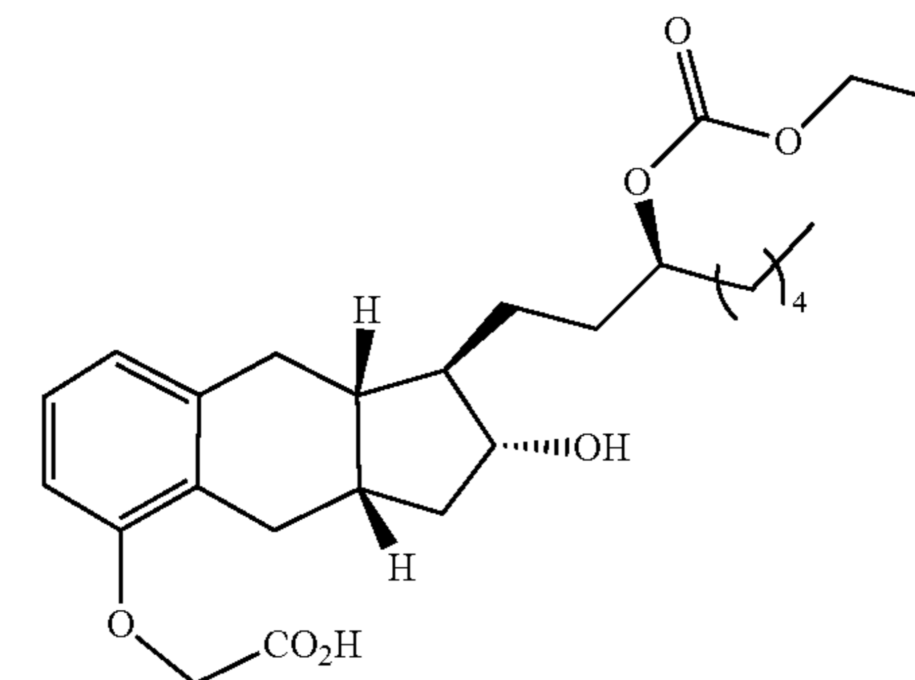
Compound Ib-12
