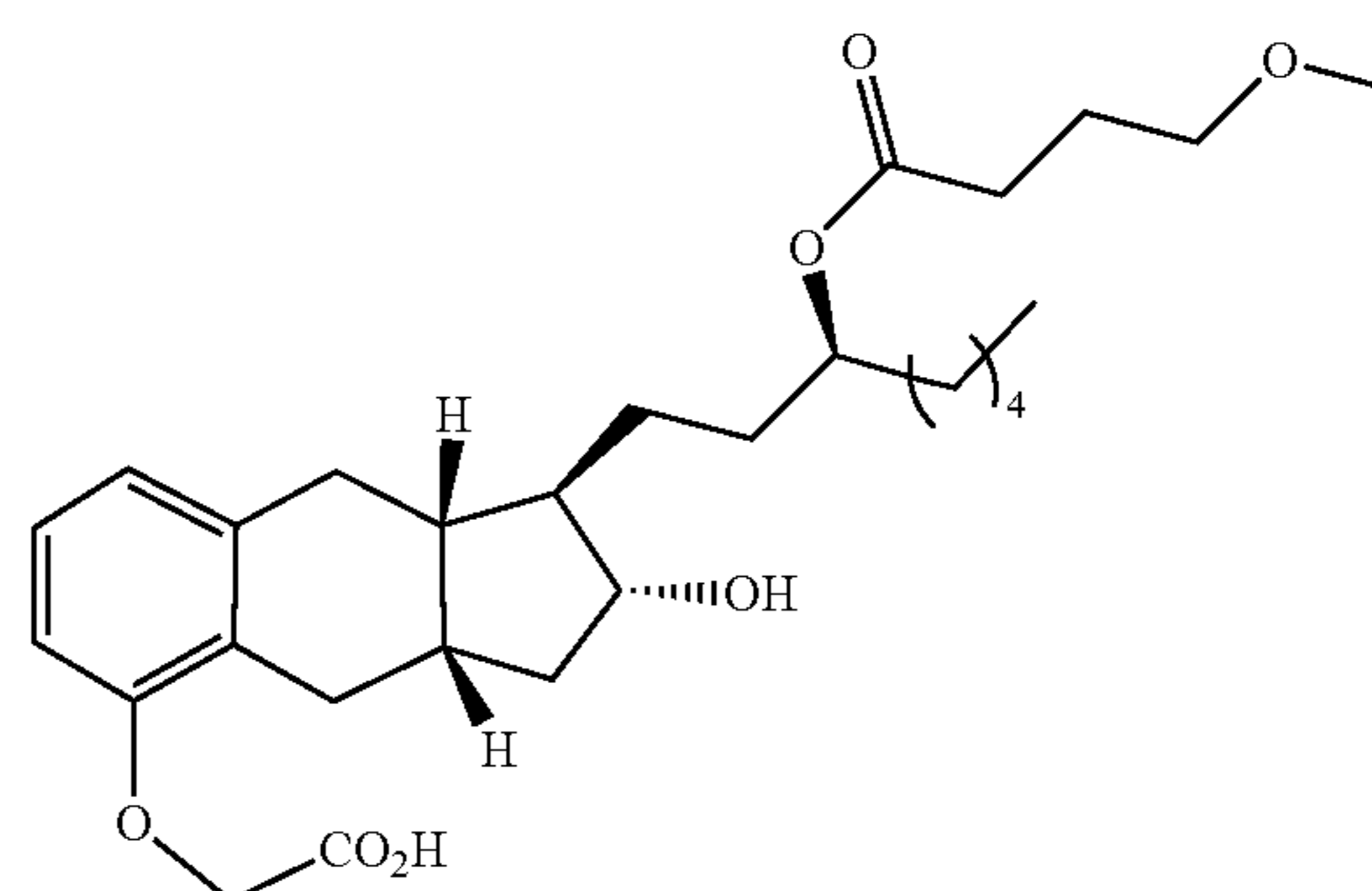
Compound Ib-19
