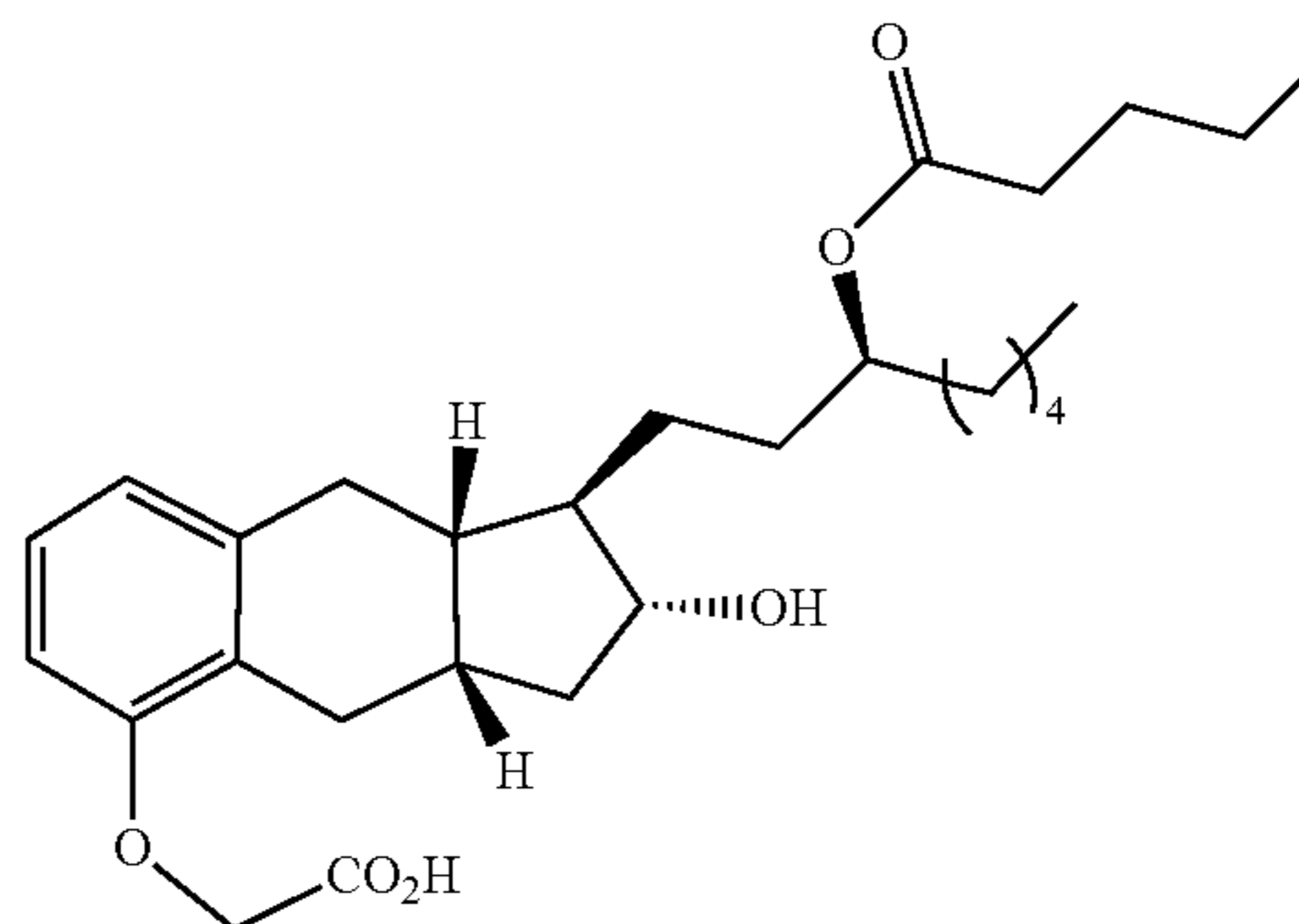
Compound Ib-3
