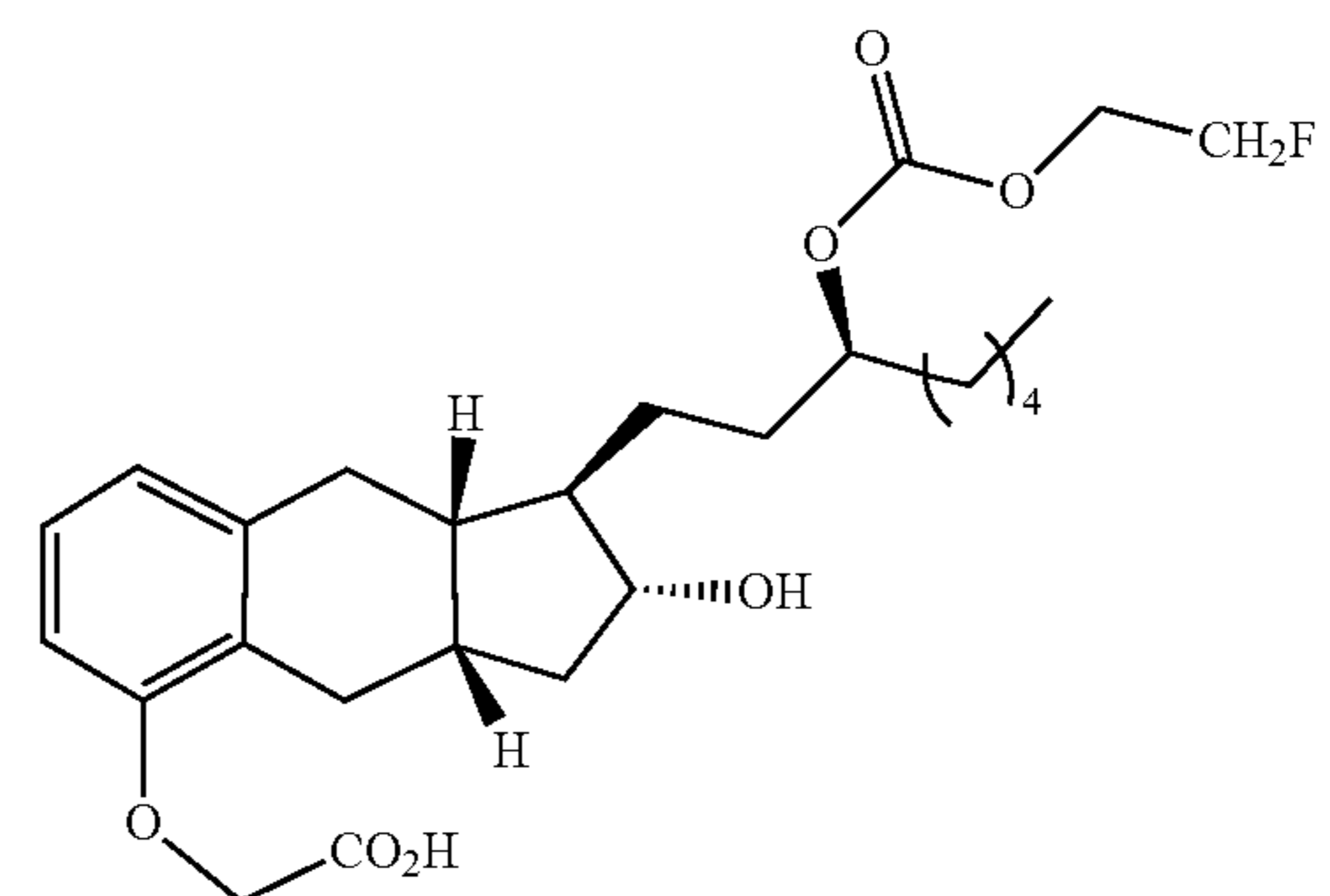
Compound Ib-12
