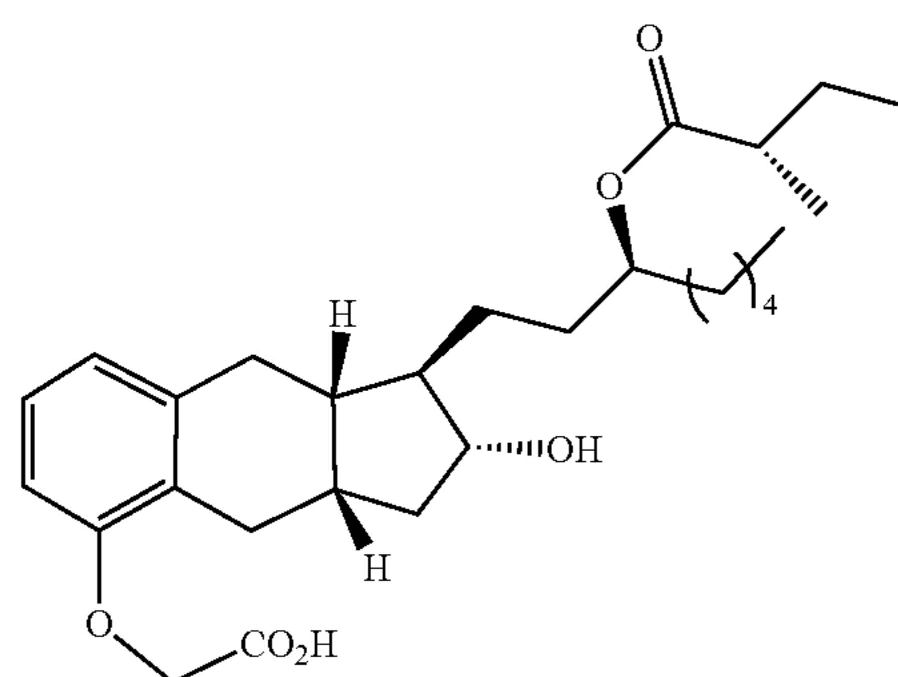
Compound Ib-27
