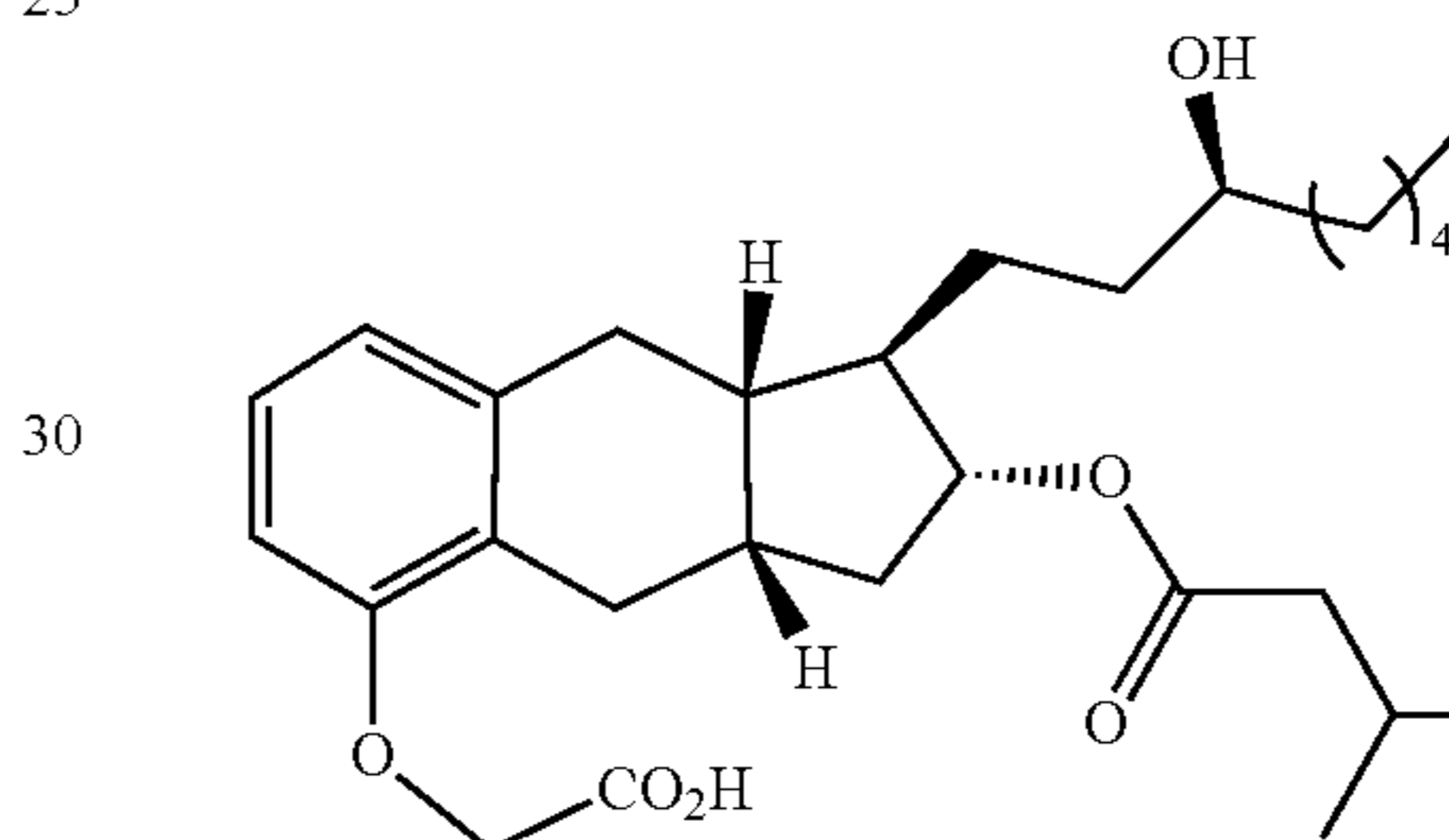
Compound Ia-1
