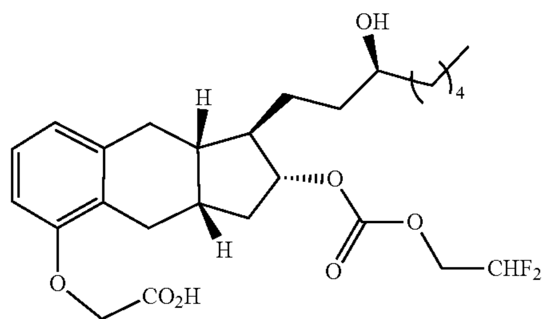
Compound Ia-13
