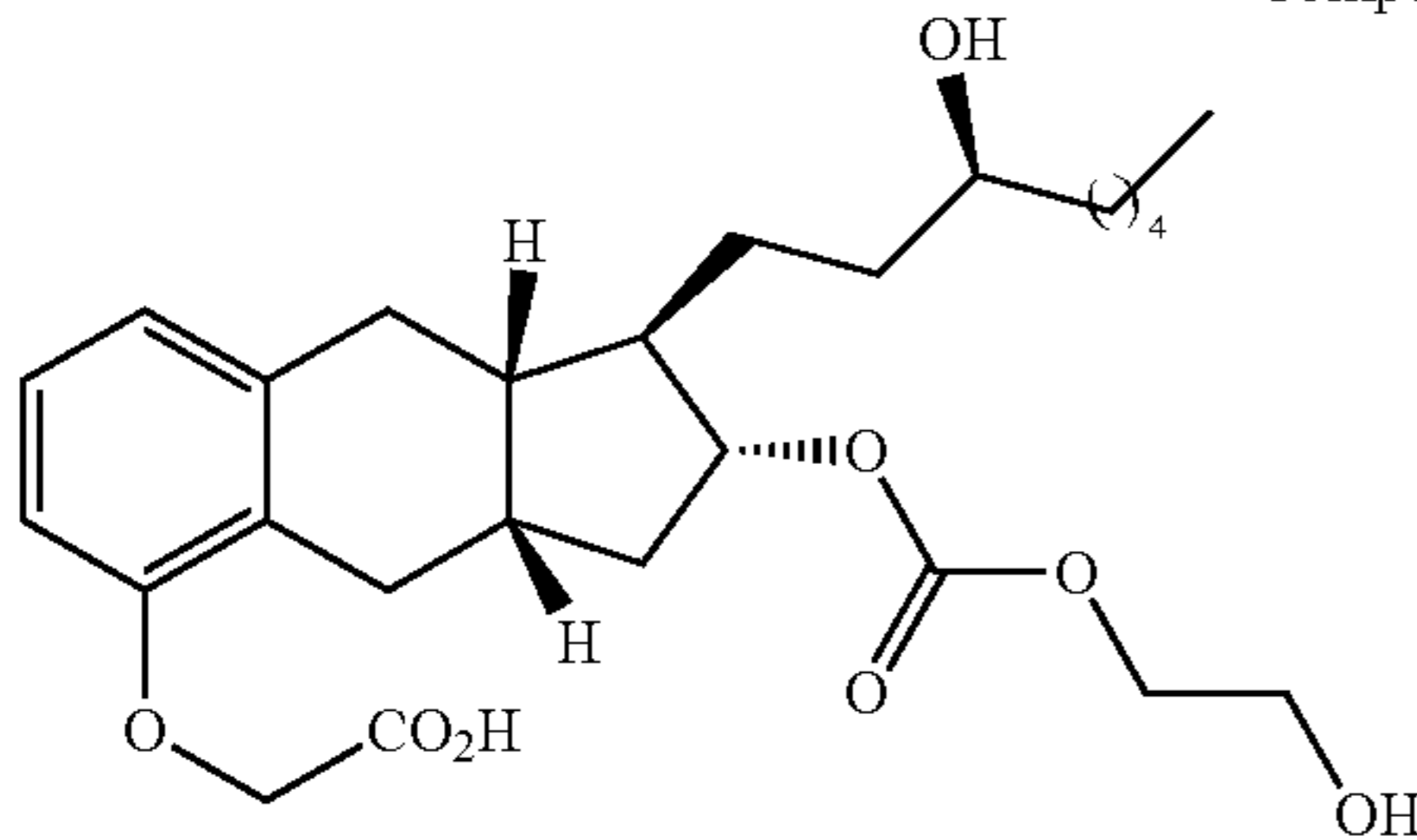
Compound Ia-14
