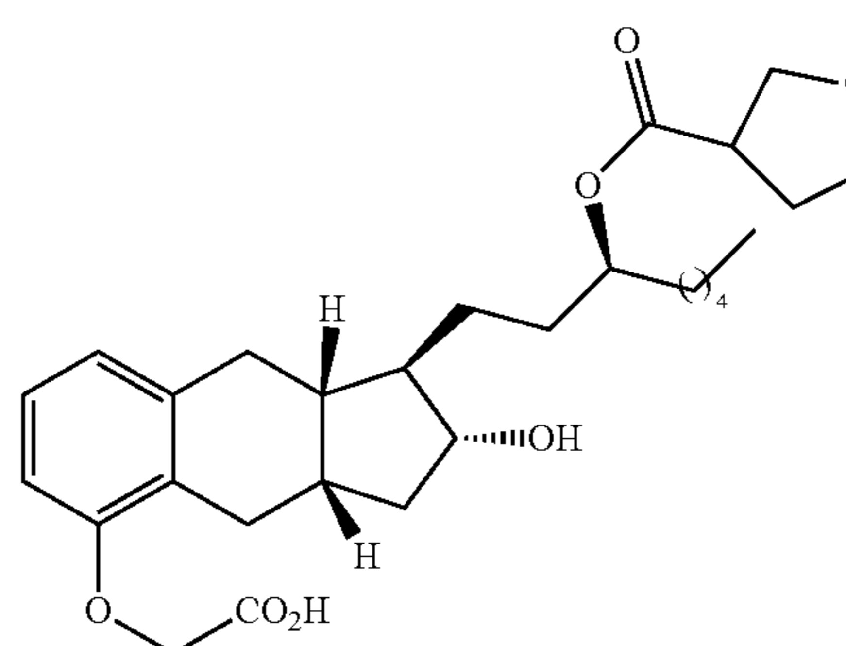
Compound Ib-33
