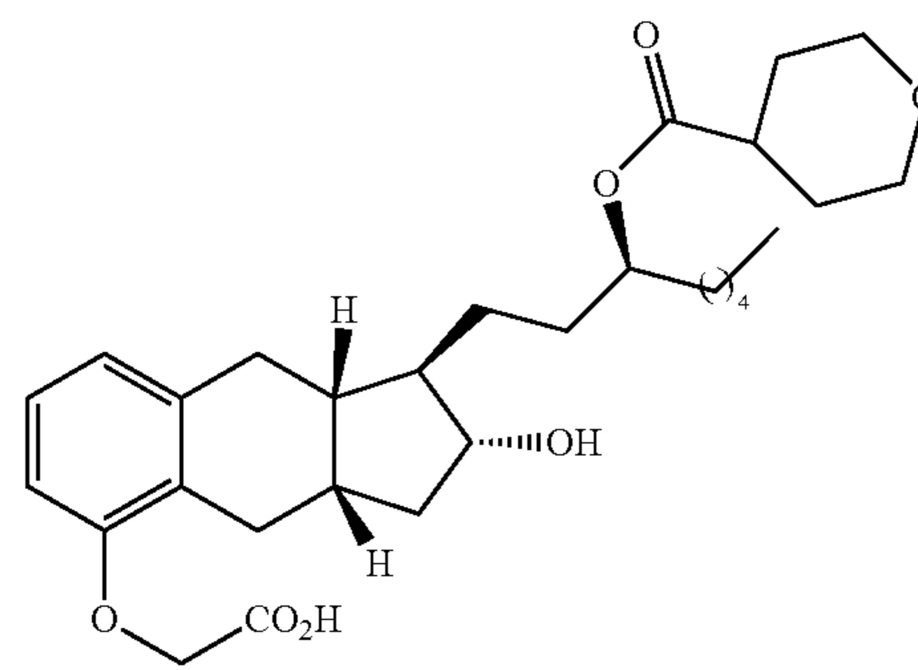
Compound Ib-34
