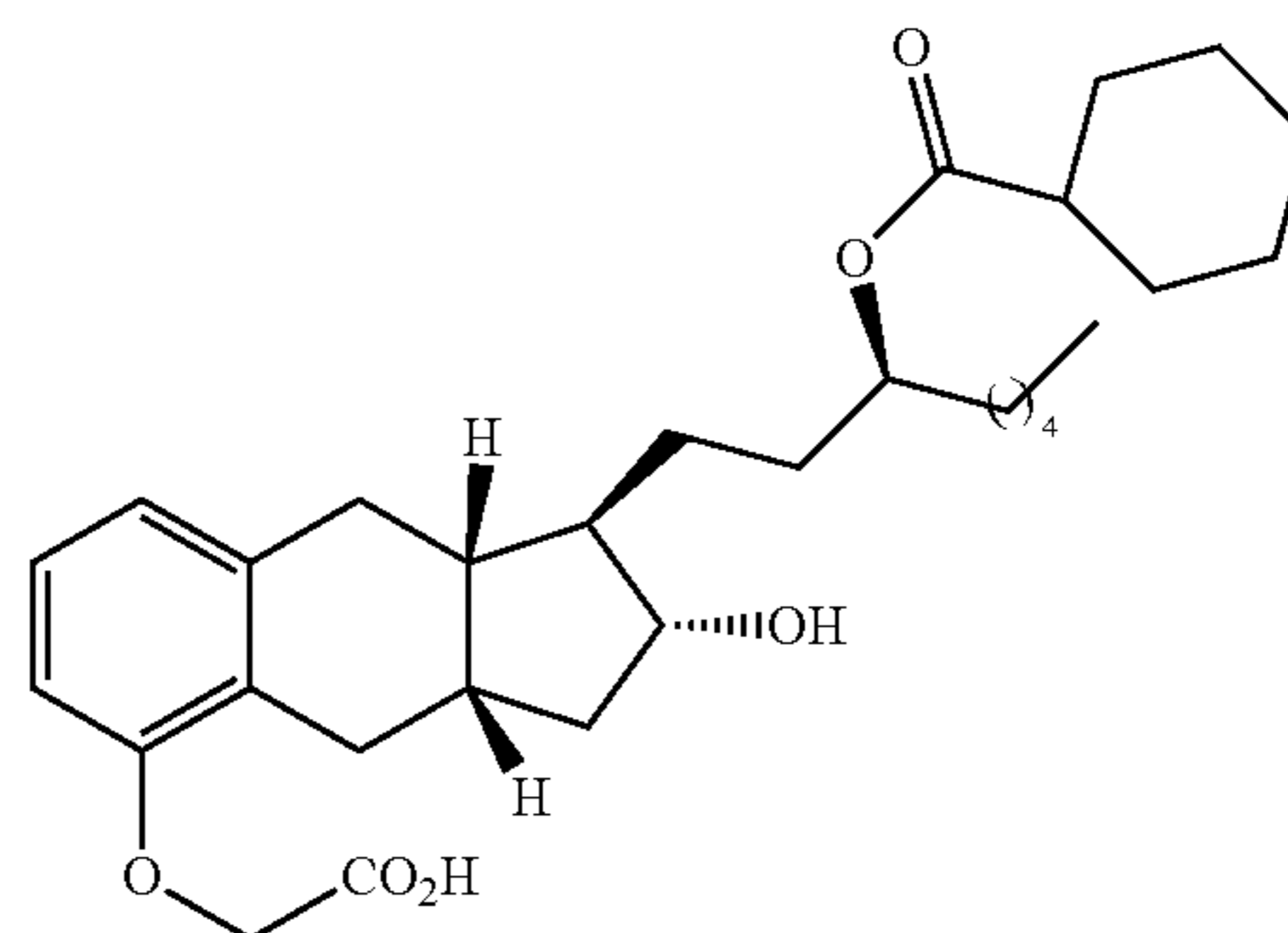
Compound Ib-31
