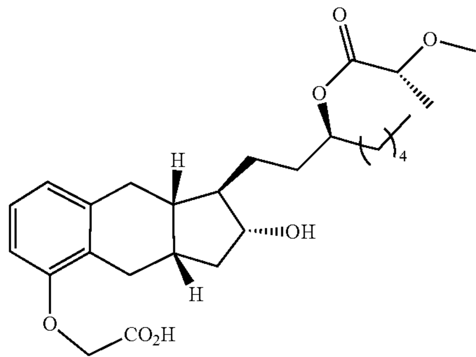
Compound Ib-25
