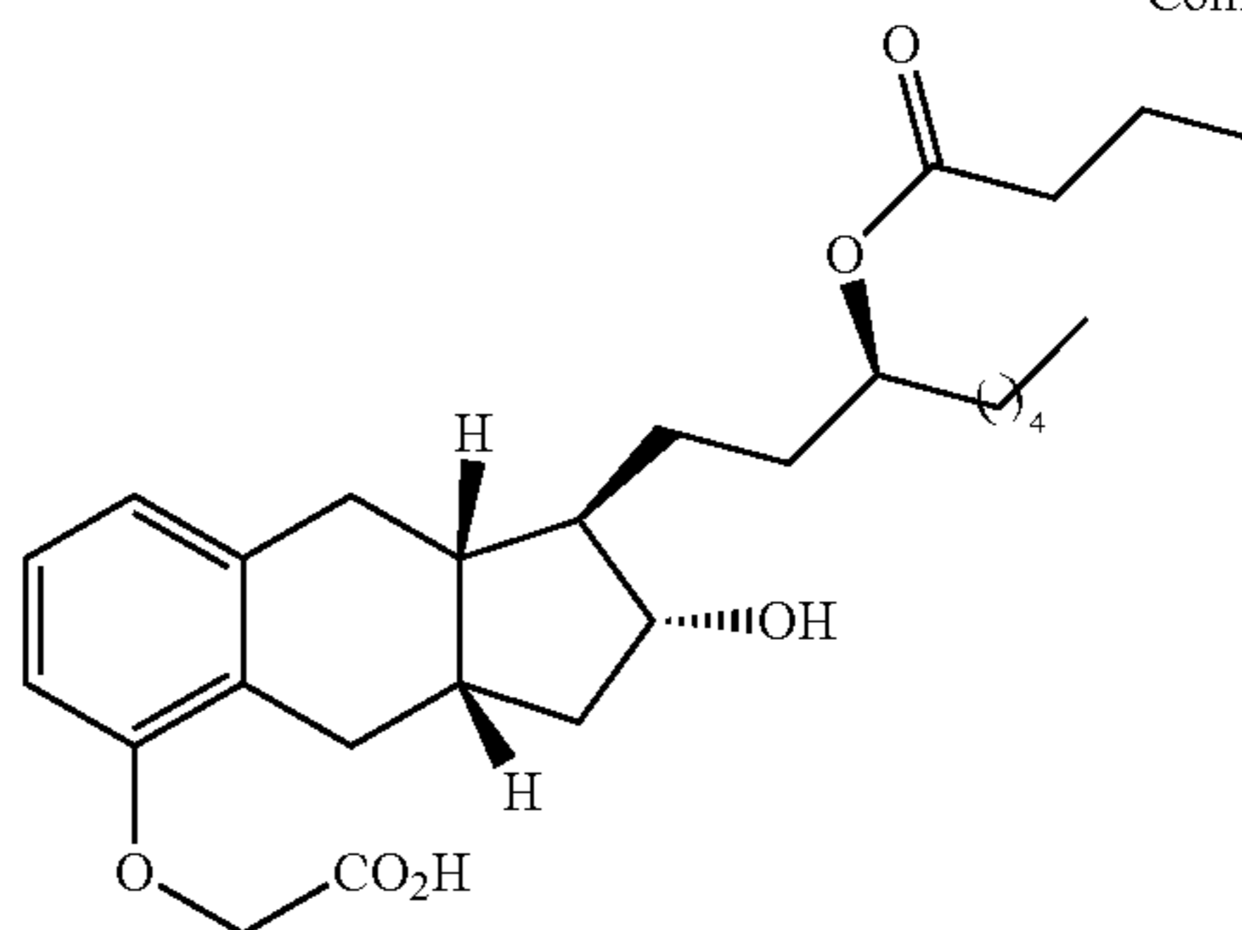
Compound Ib-3
