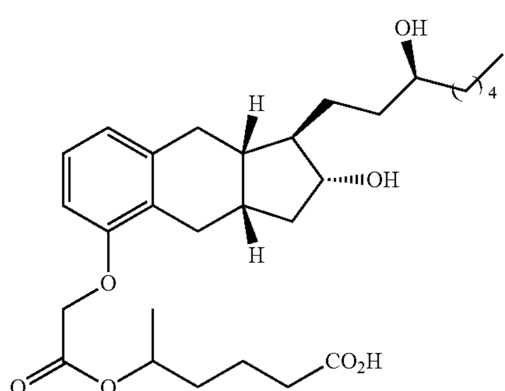
Compound II-8
