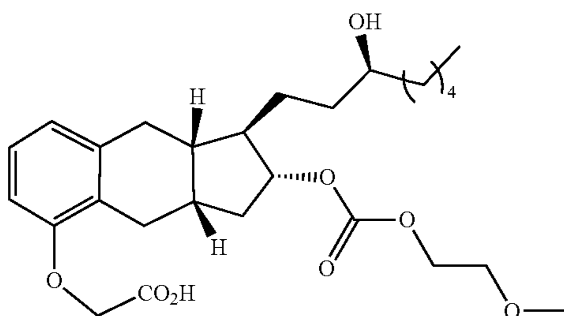
Compound Ib-1
