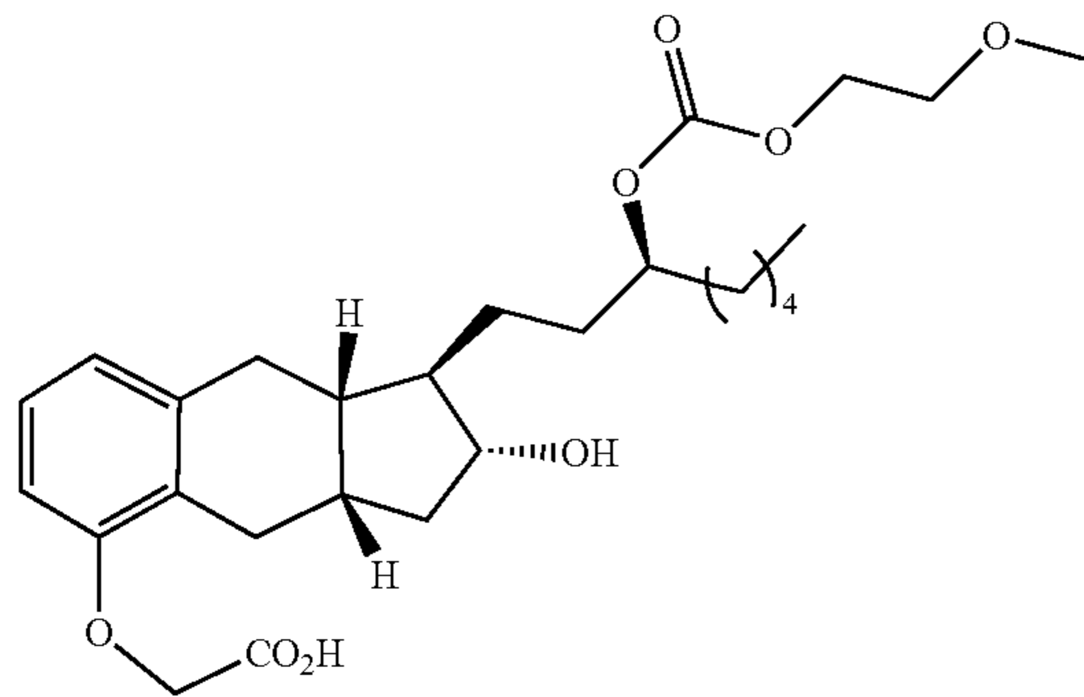
Compound Ib-15
