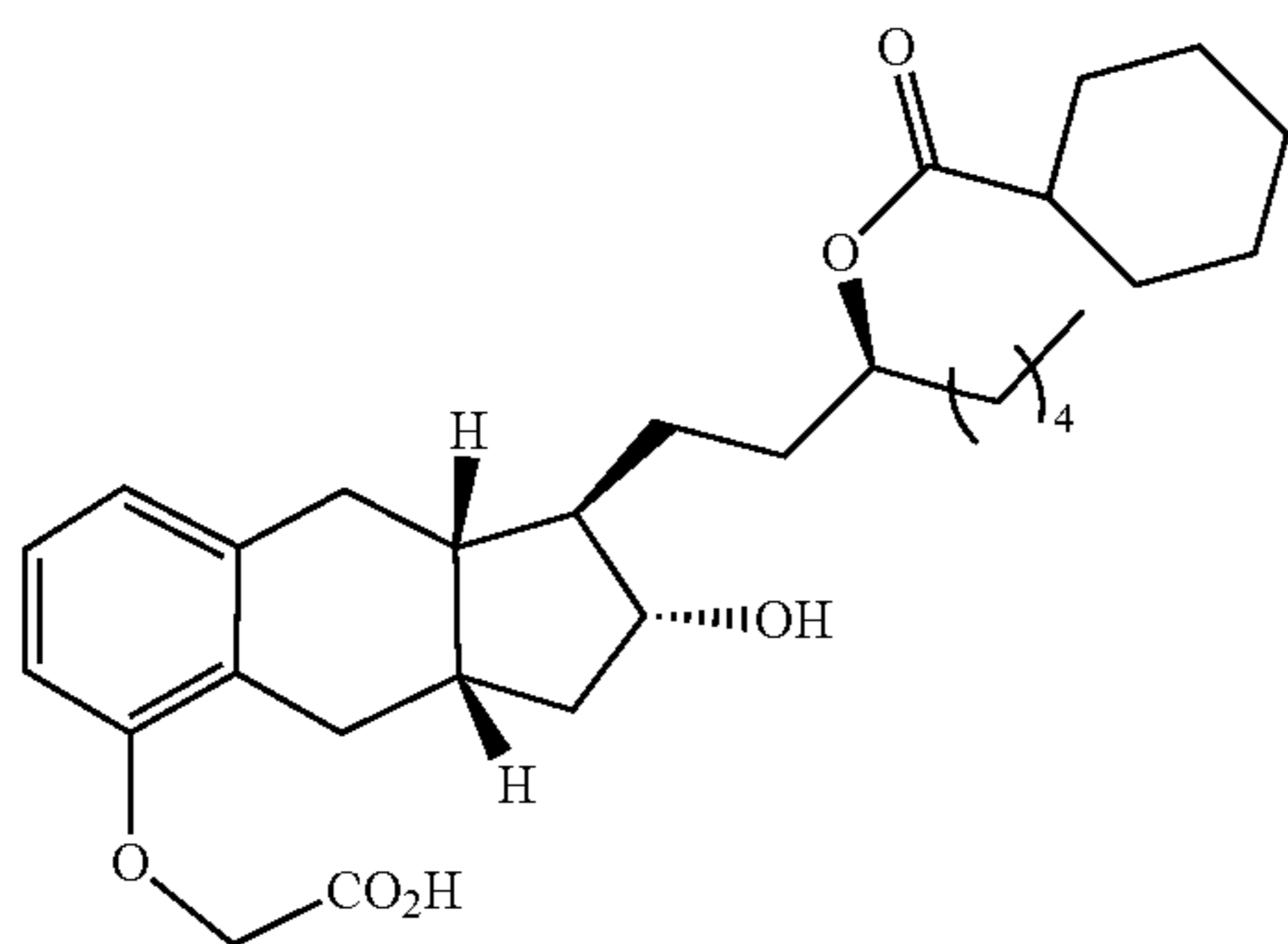
Compound Ib-31
