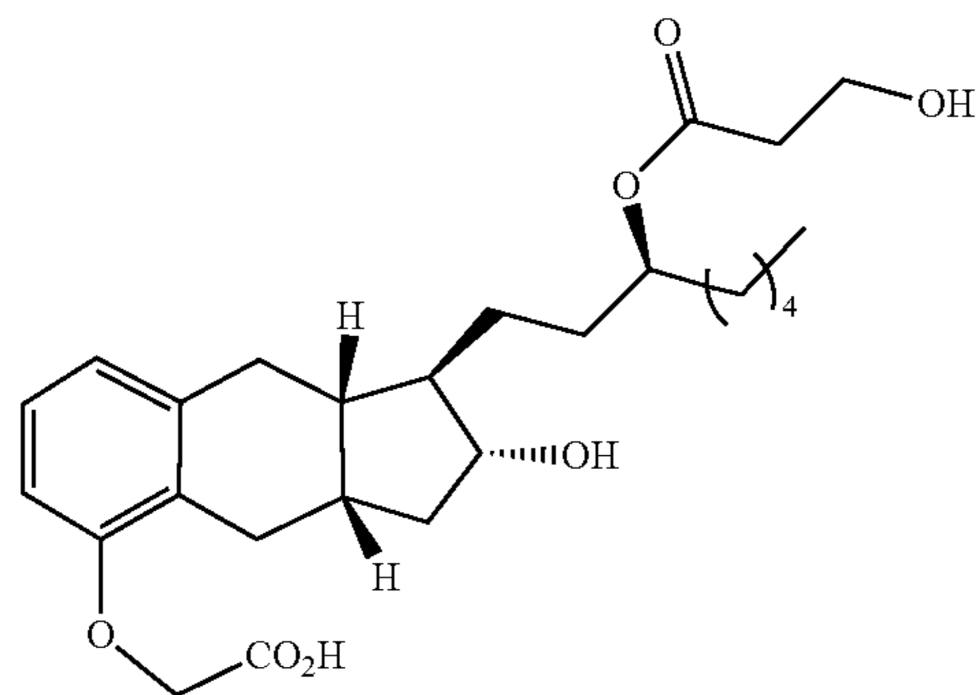
Compound Ib-5
