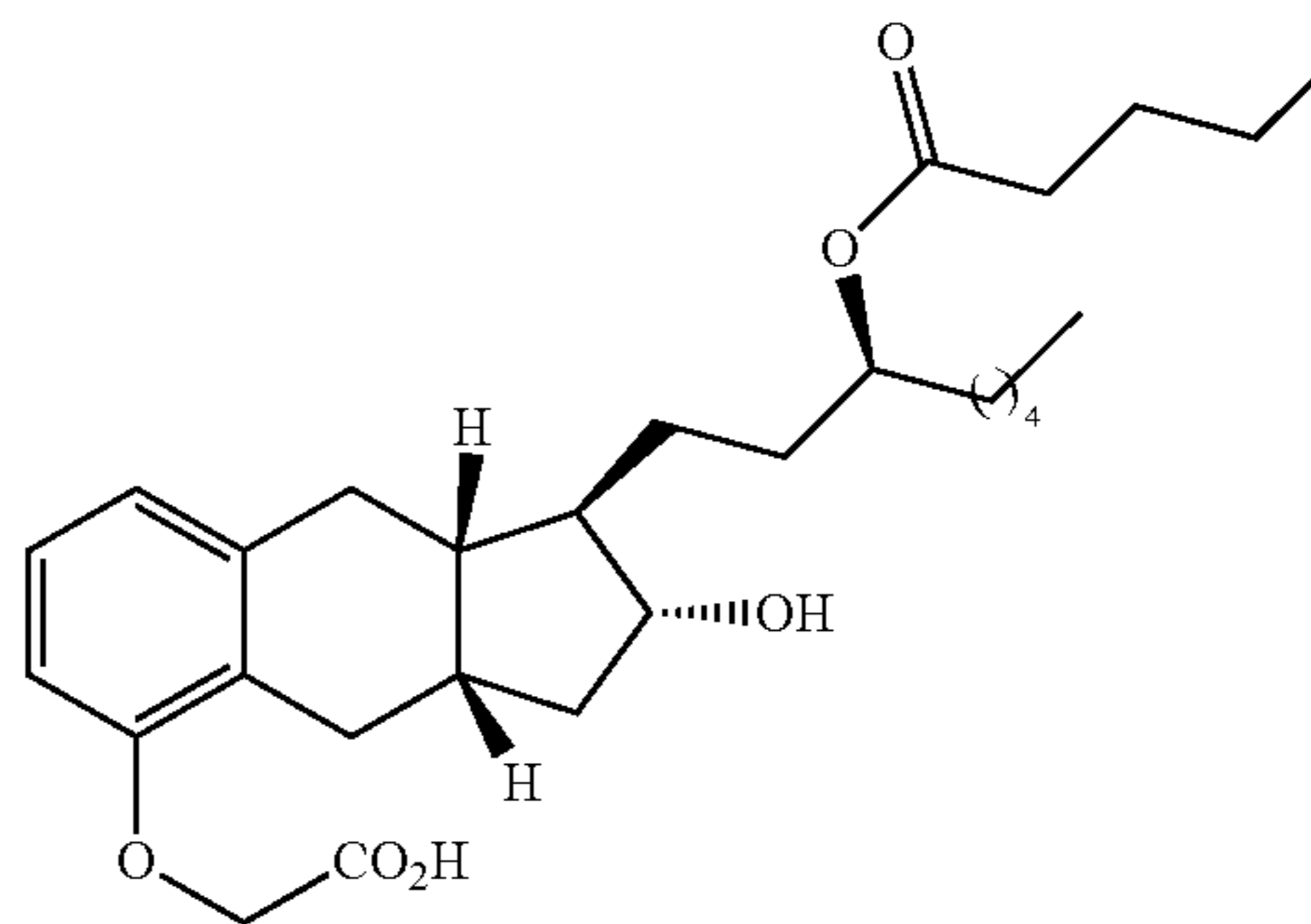
Compound Ib-16
