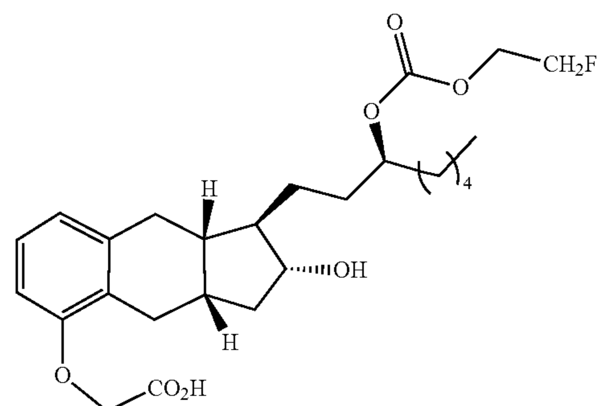
Compound Ib-12
