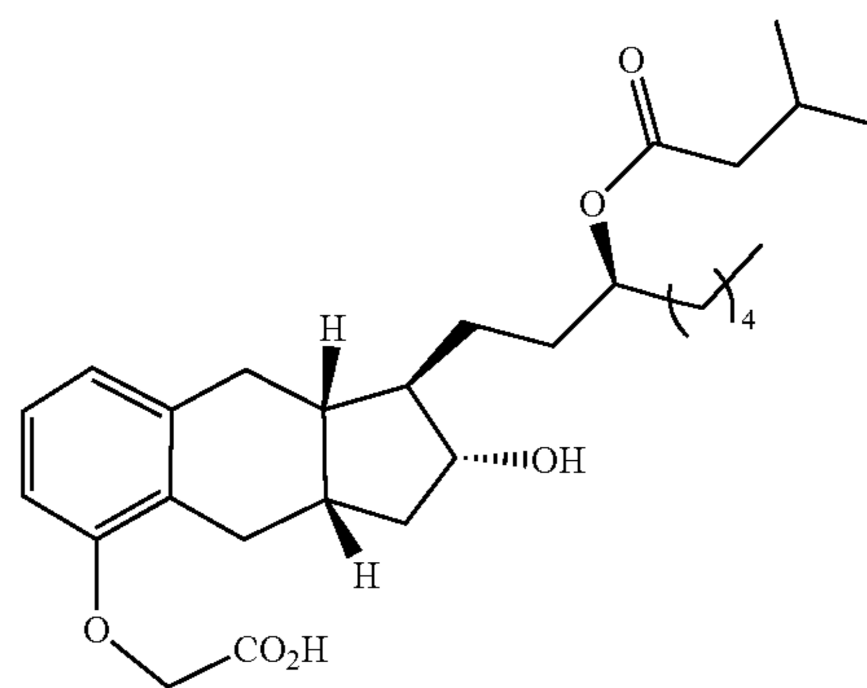
Compound Ib-4
