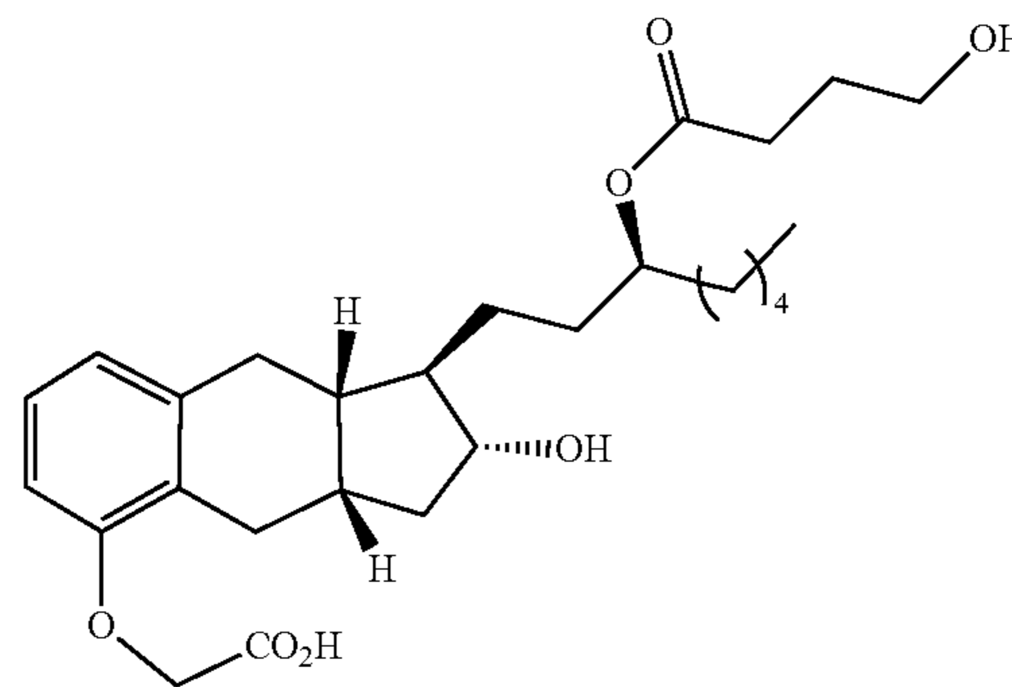
Compound Ib-18
