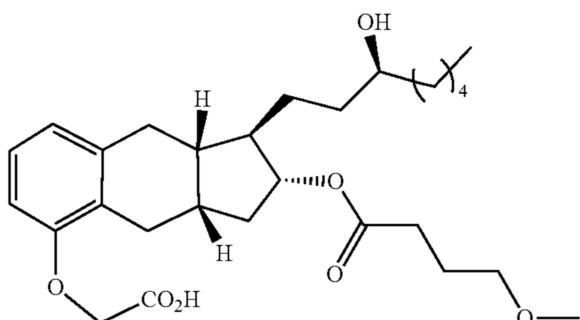
Compound Ia-19
