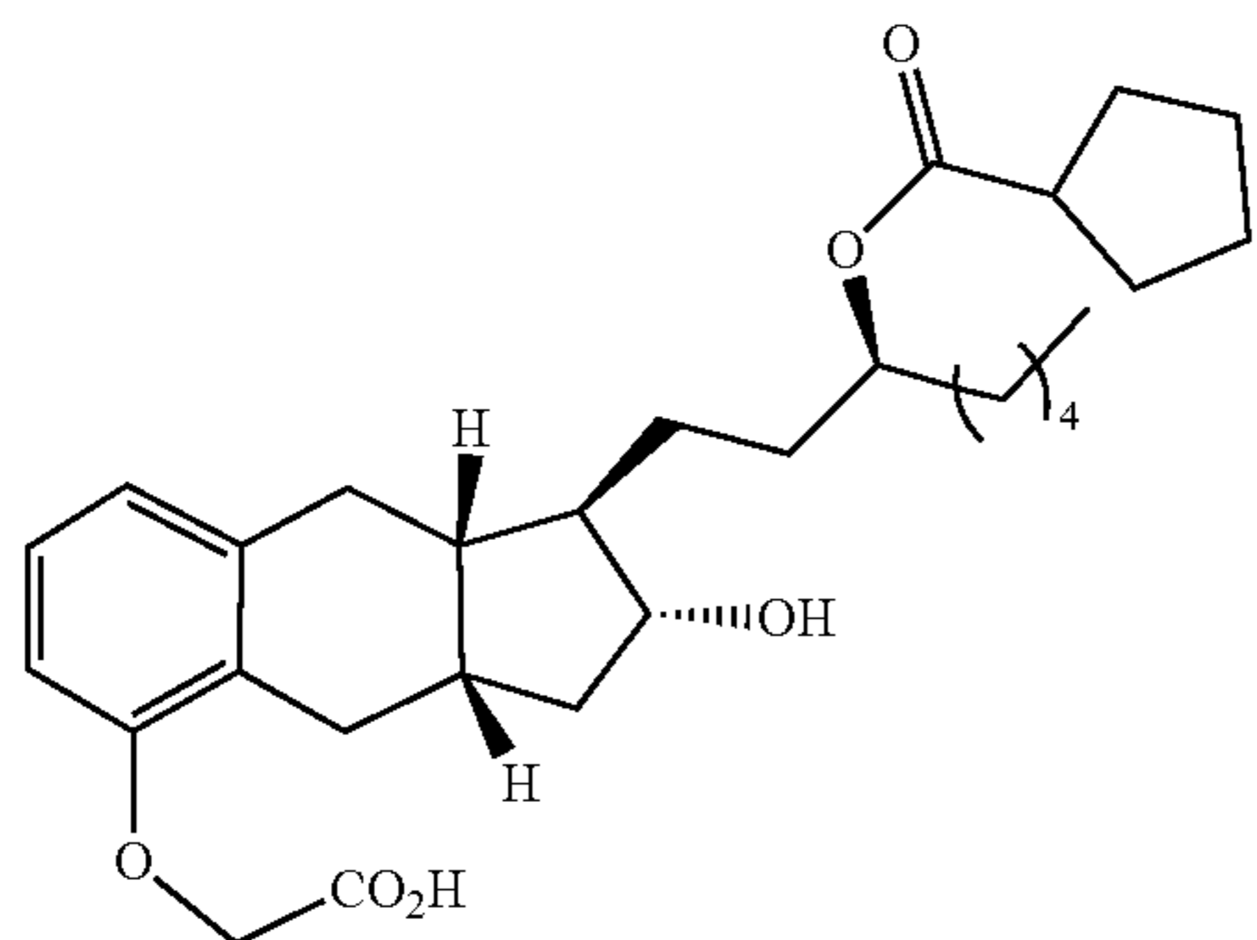
Compound Ib-30
