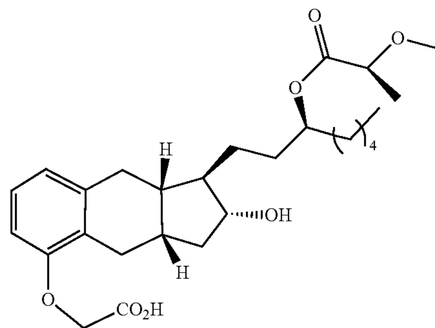
Compound Ib-26
