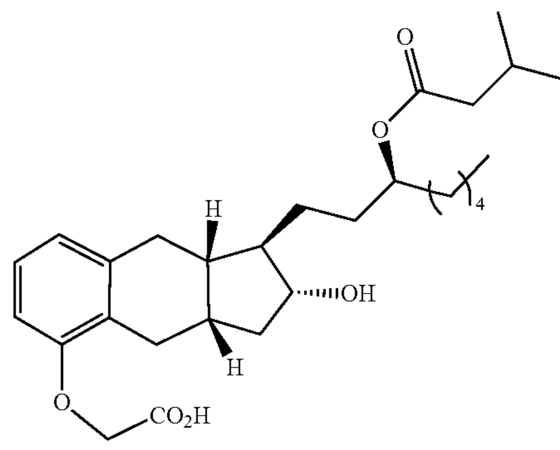
Compound Ib-4
