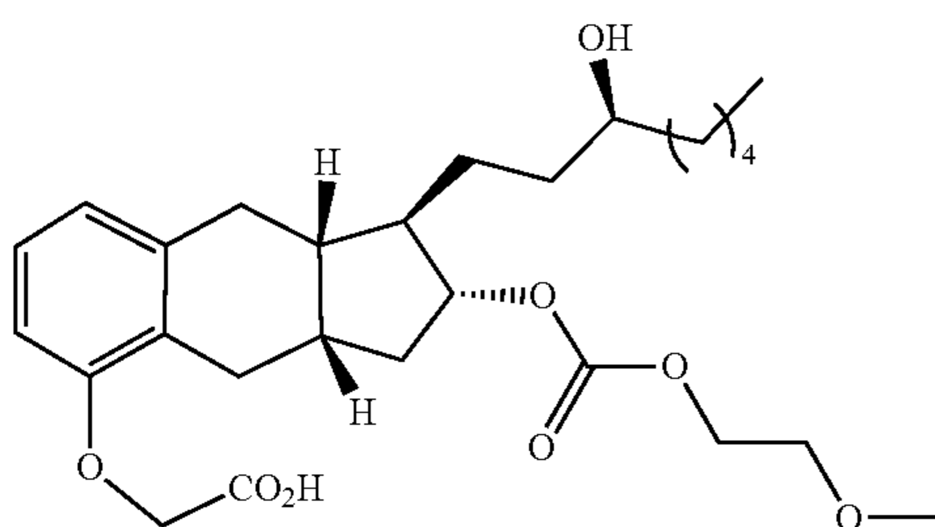
Compound Ib-1
