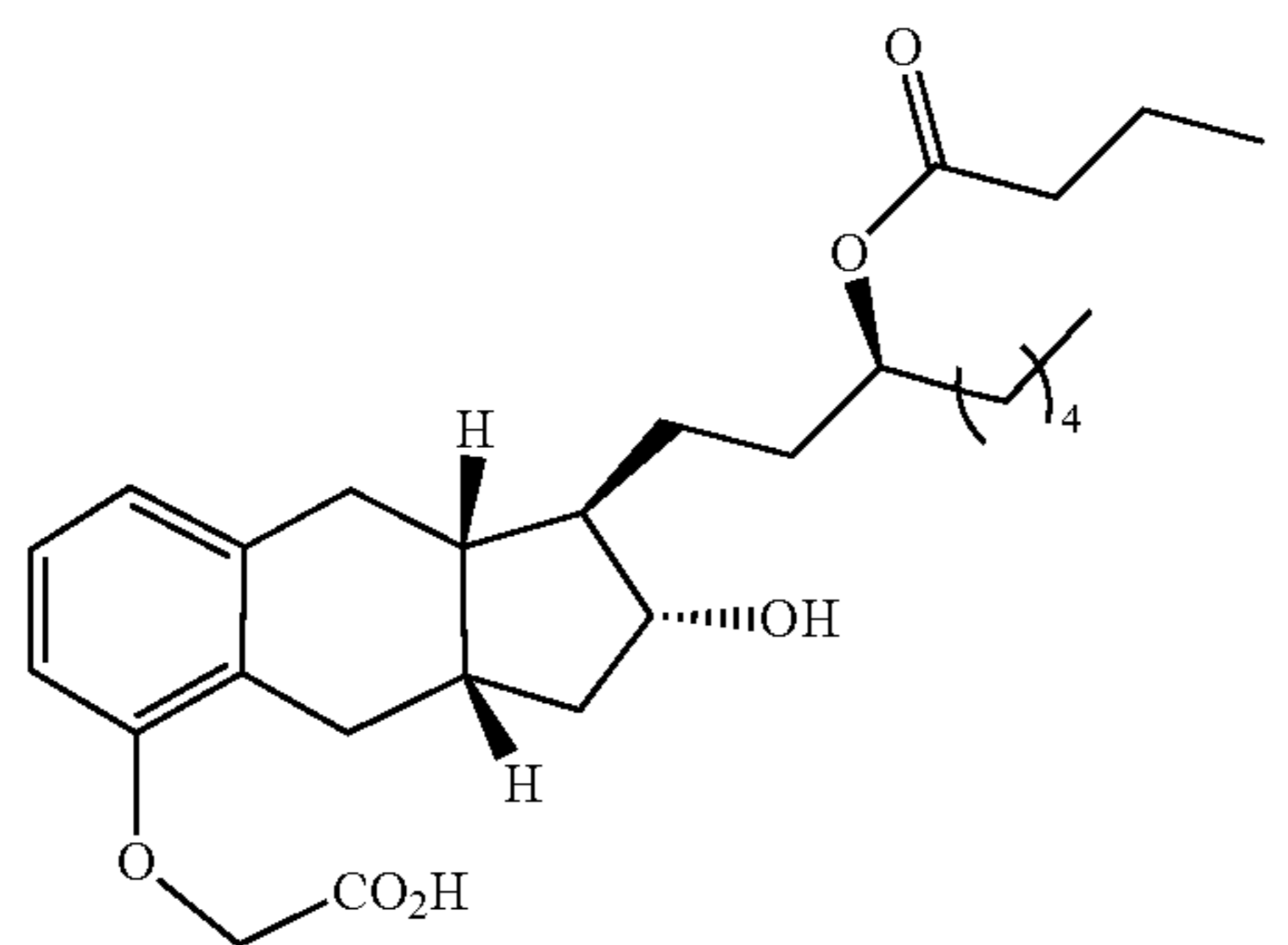
Compound Ib-3
