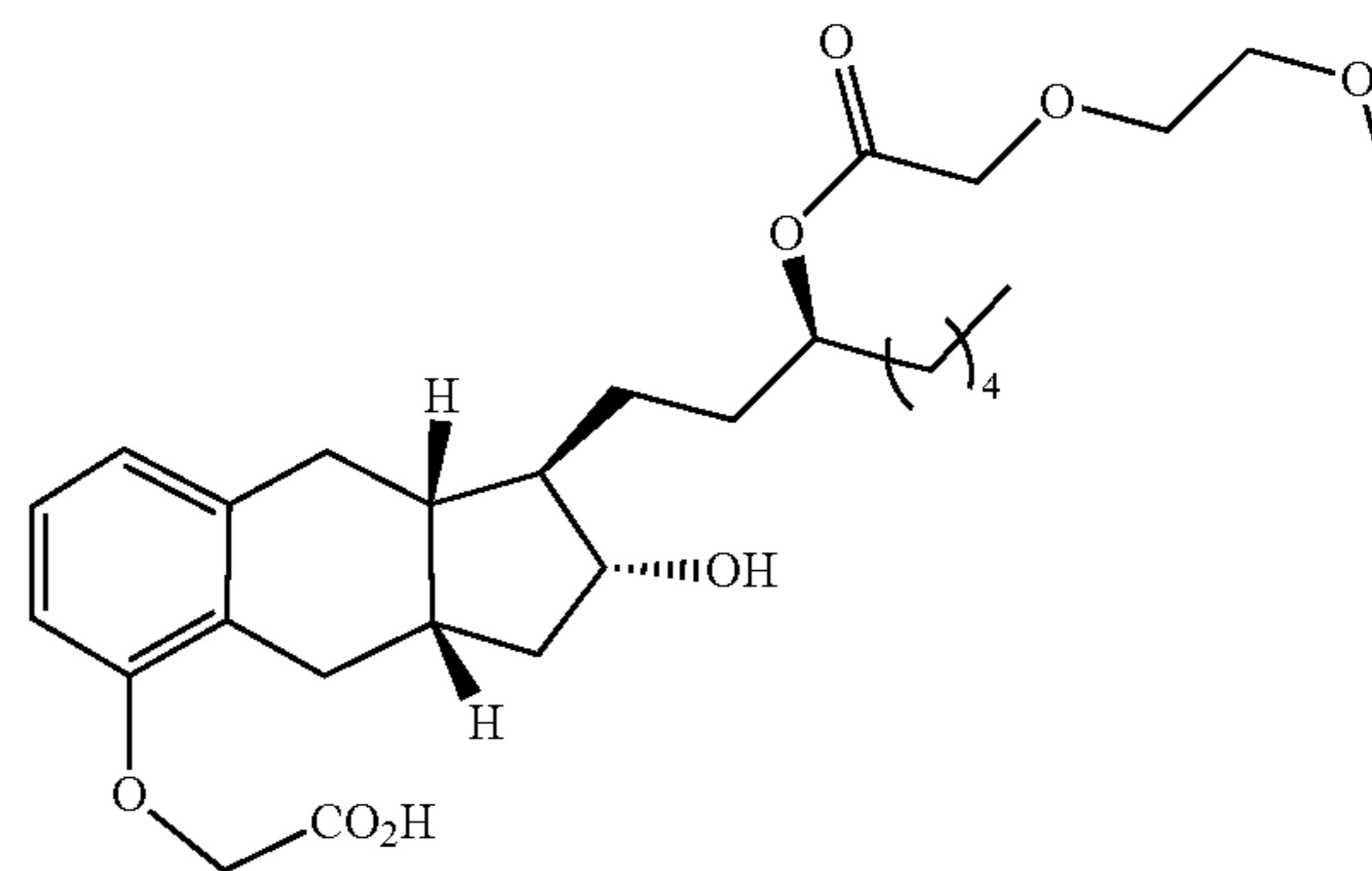
Compound Ib-21
