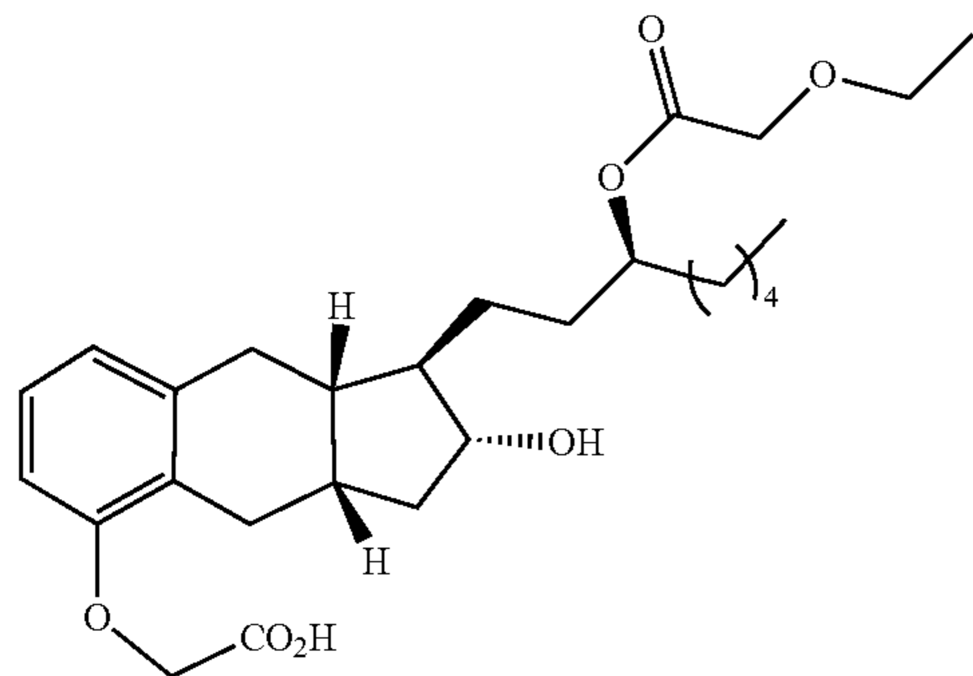
Compound Ib-9
