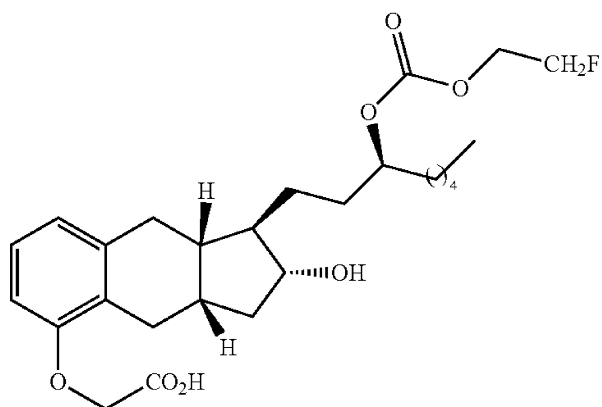
Compound Ib-12
