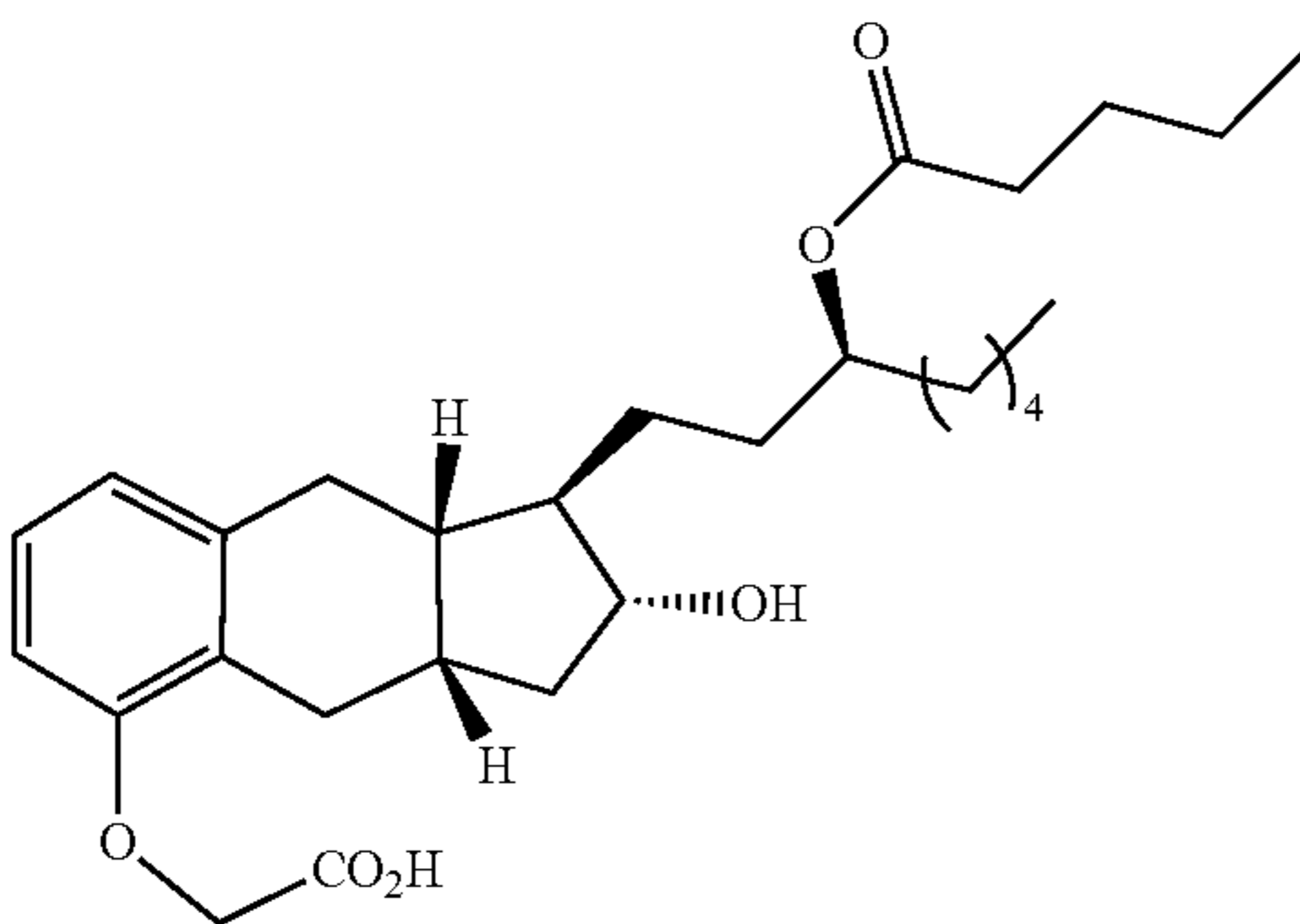
Compound Ib-3
