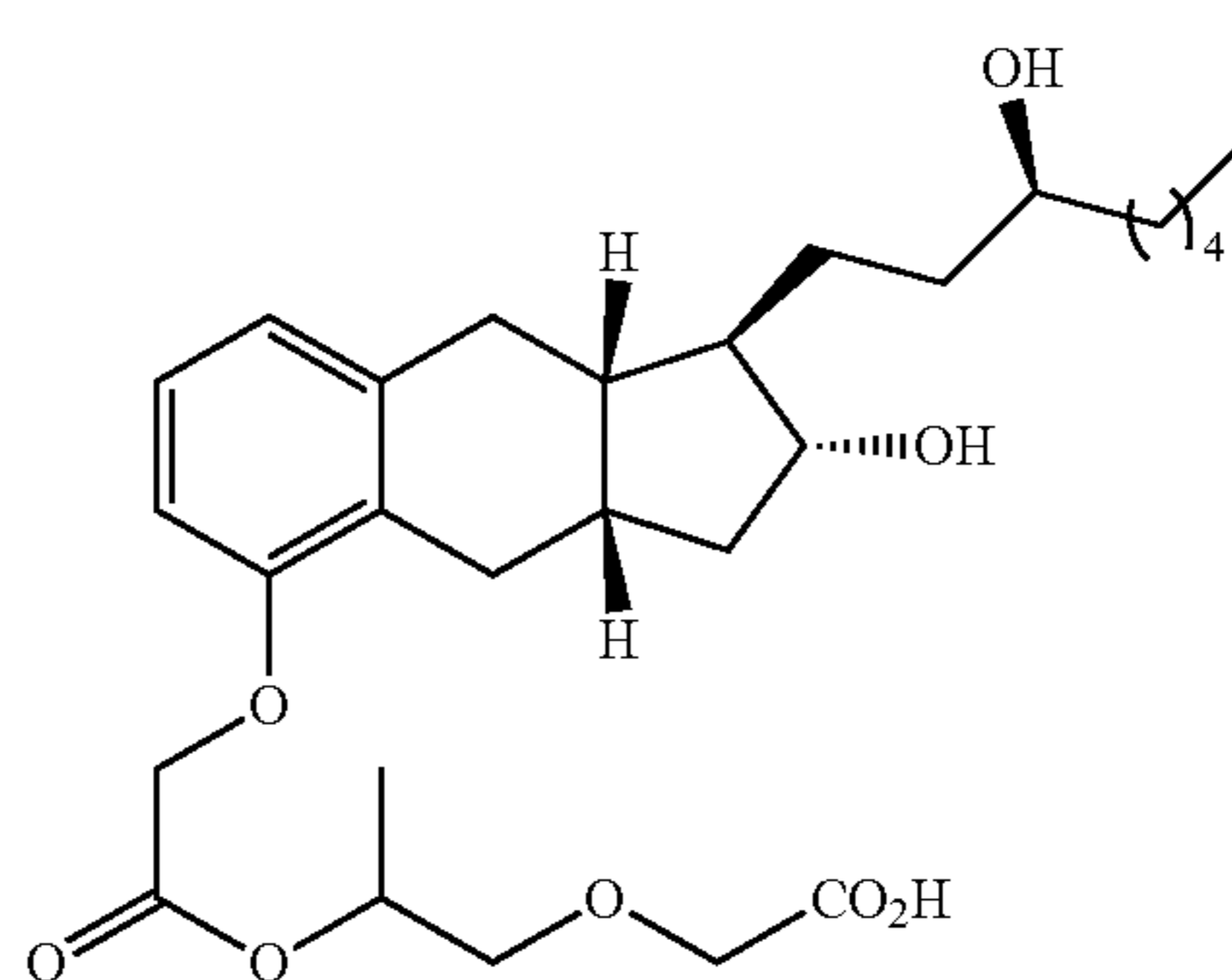
Compound II-14
