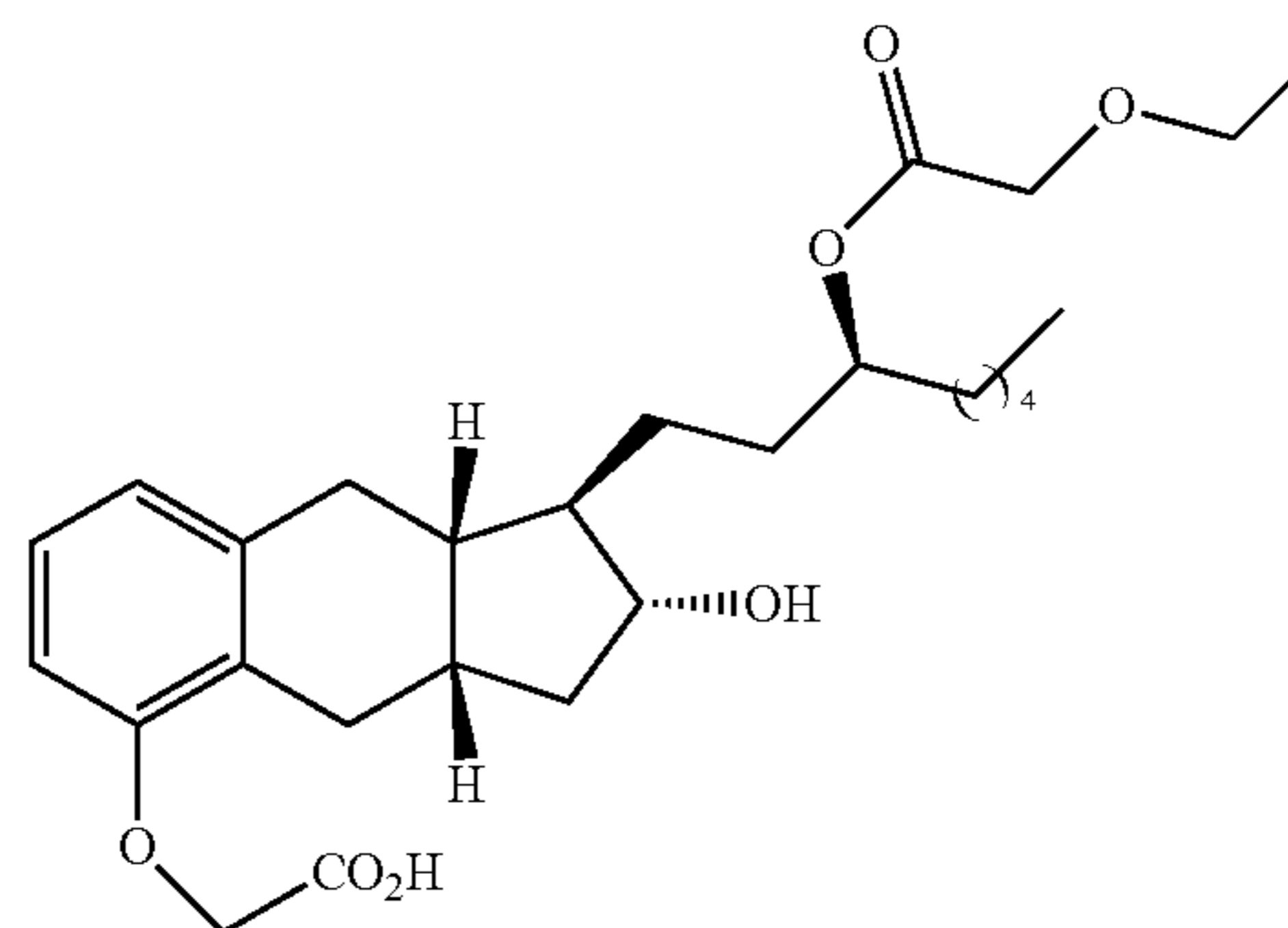
Compound Ib-9
