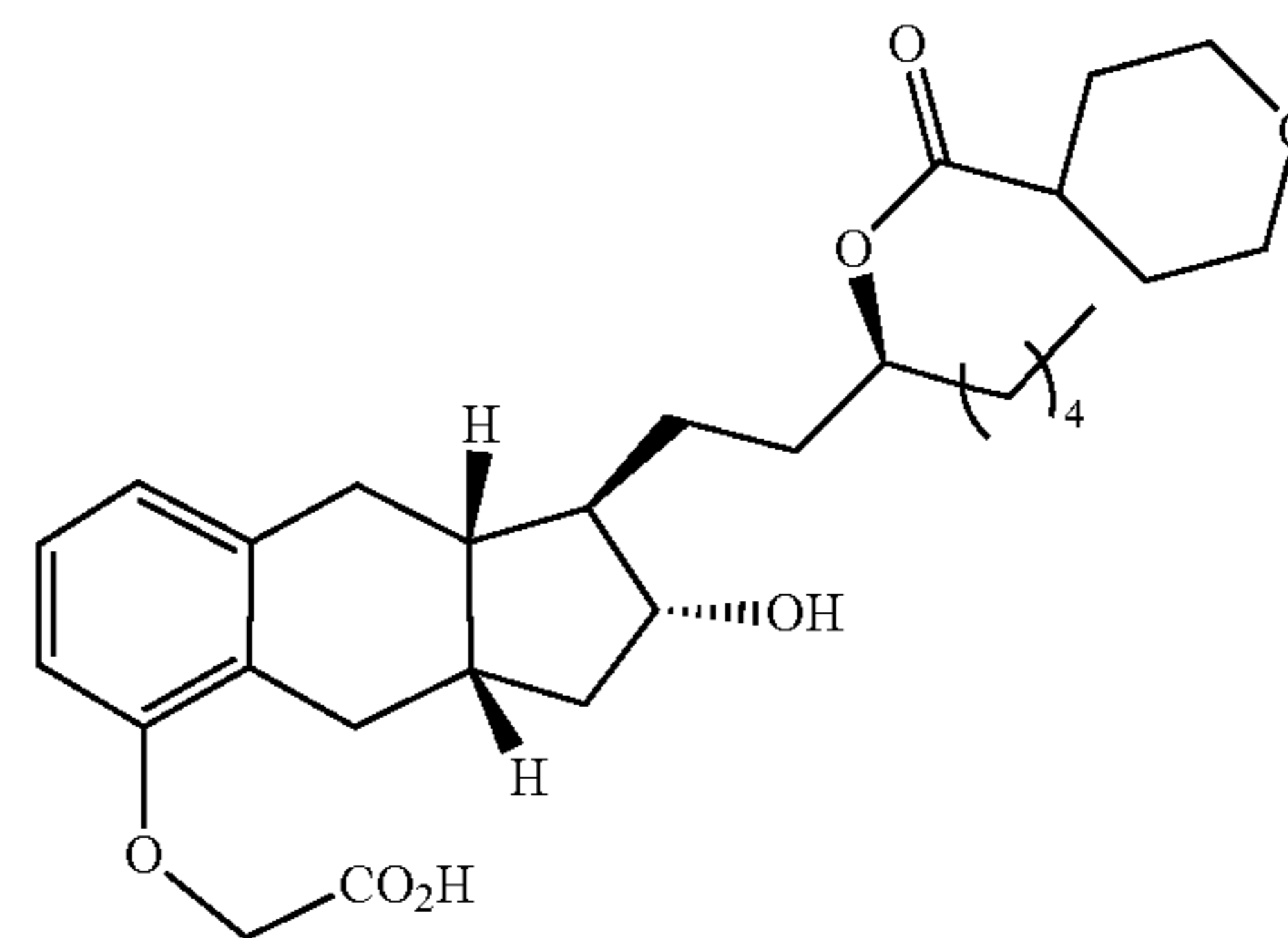
Compound Ib-34
