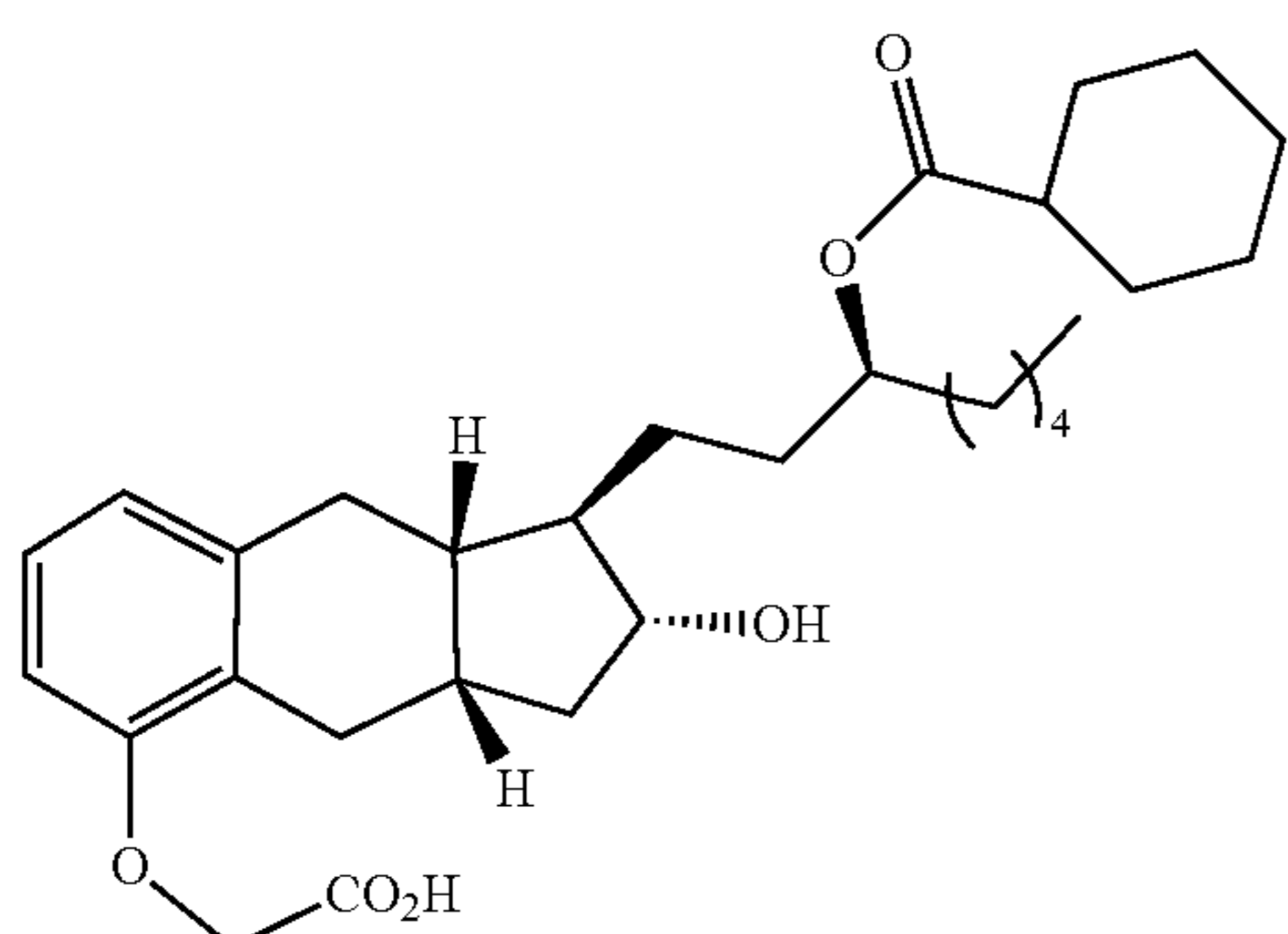
Compound Ib-31
