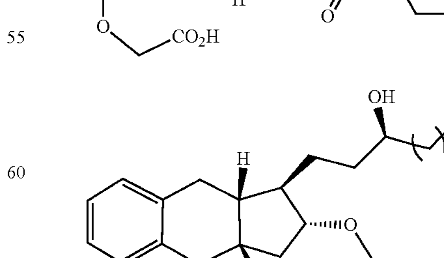
Compound Ia-3
