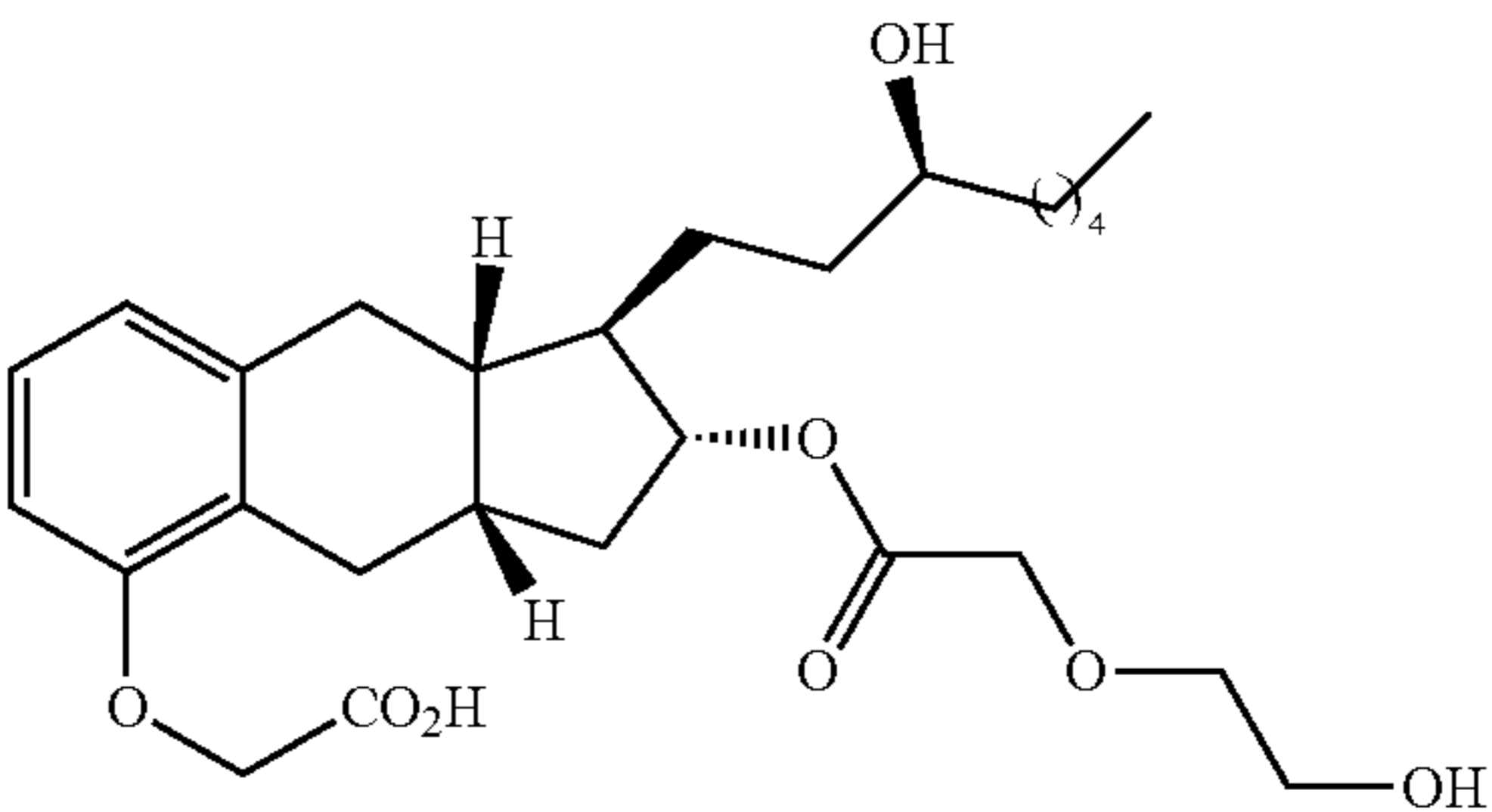
Compound Ia-20
