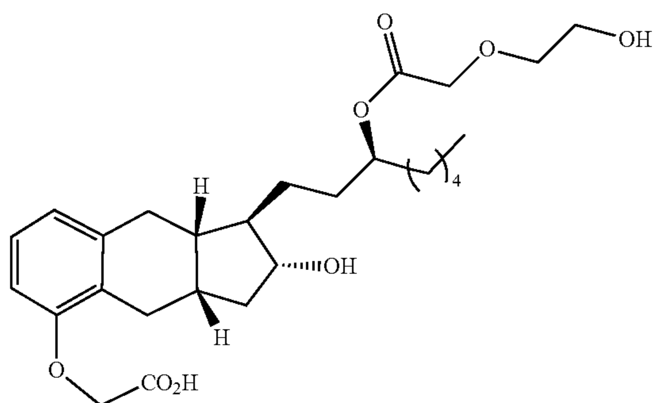
Compound Ib-20
