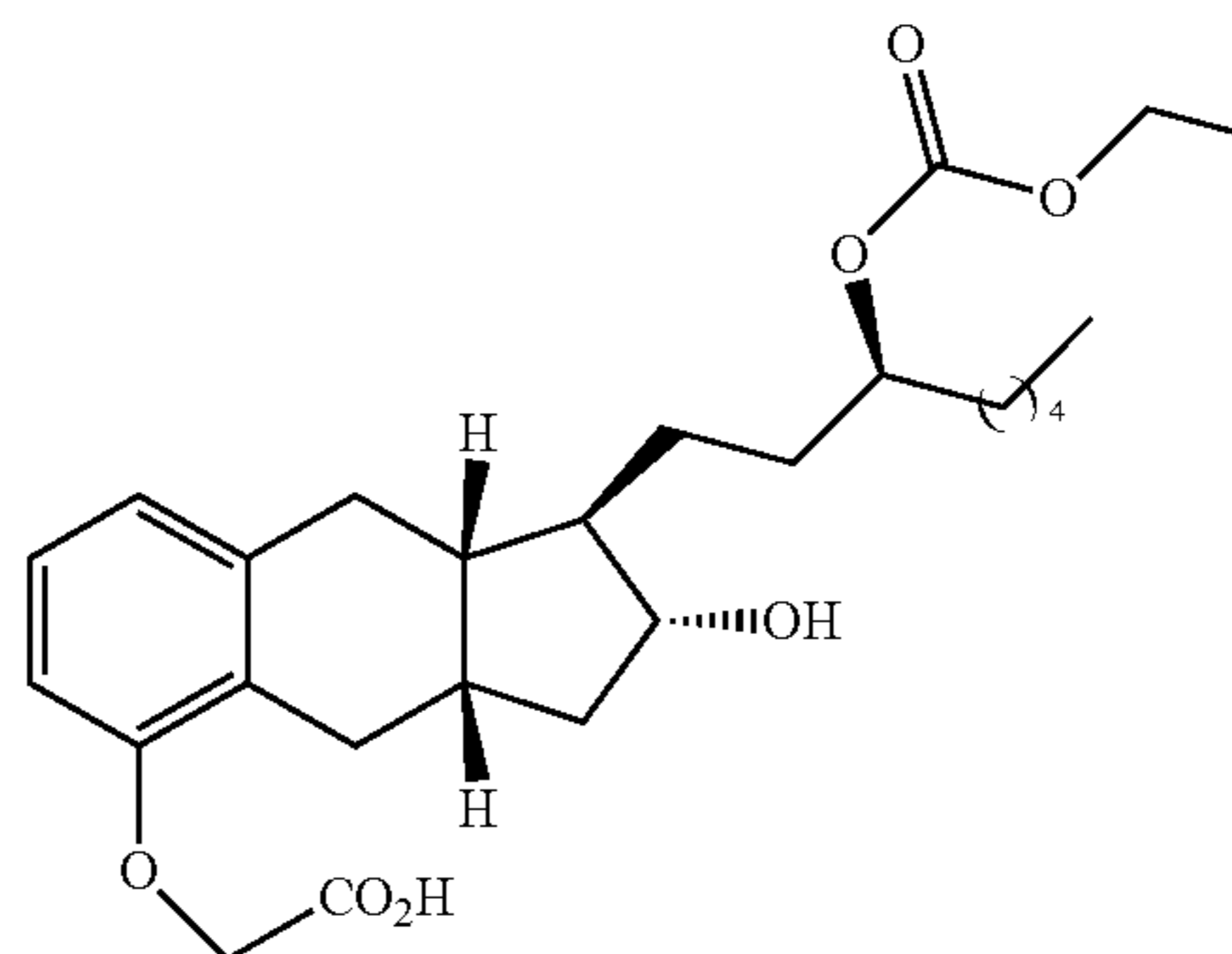
Compound Ib-11
