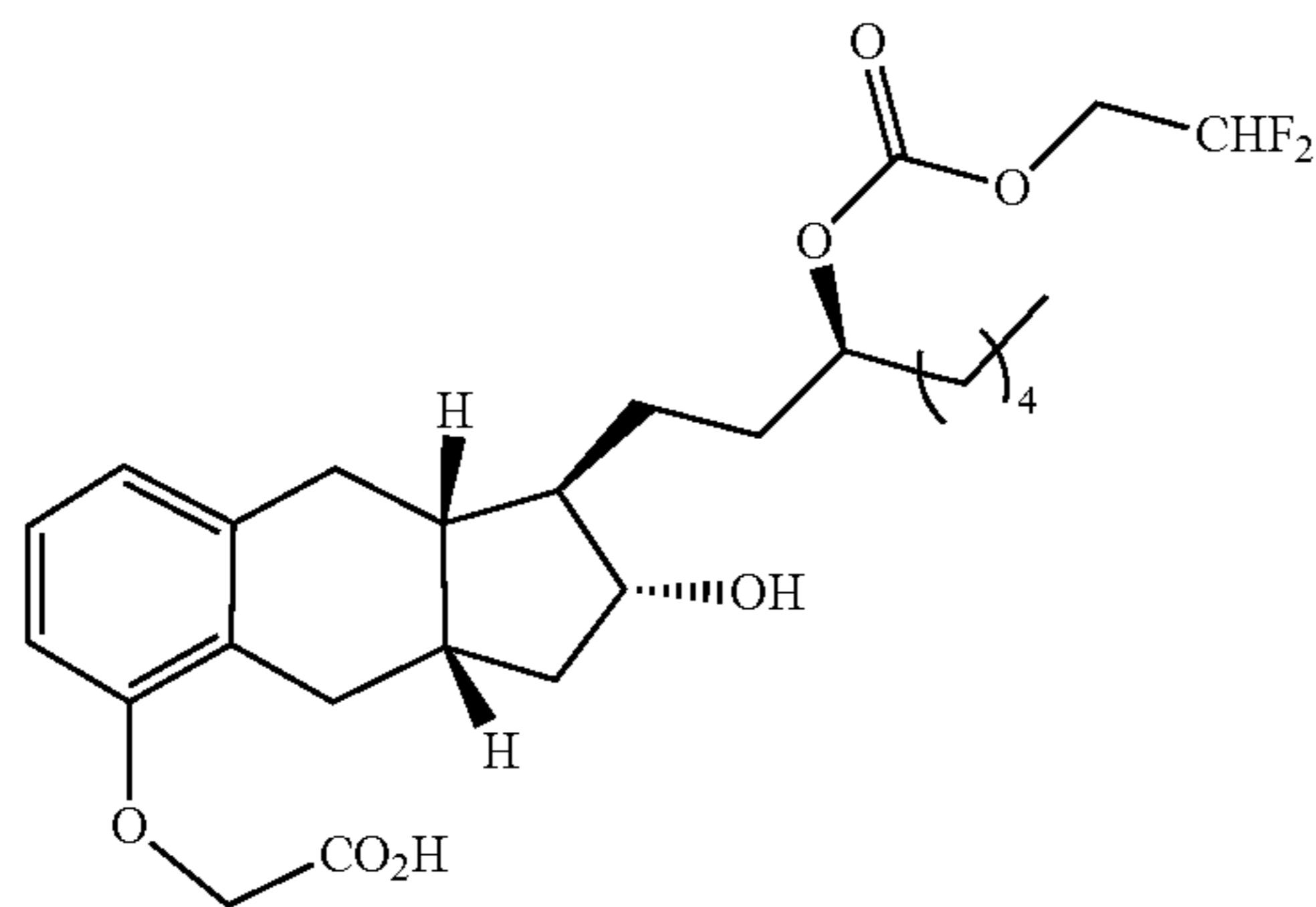
Compound Ib-13
