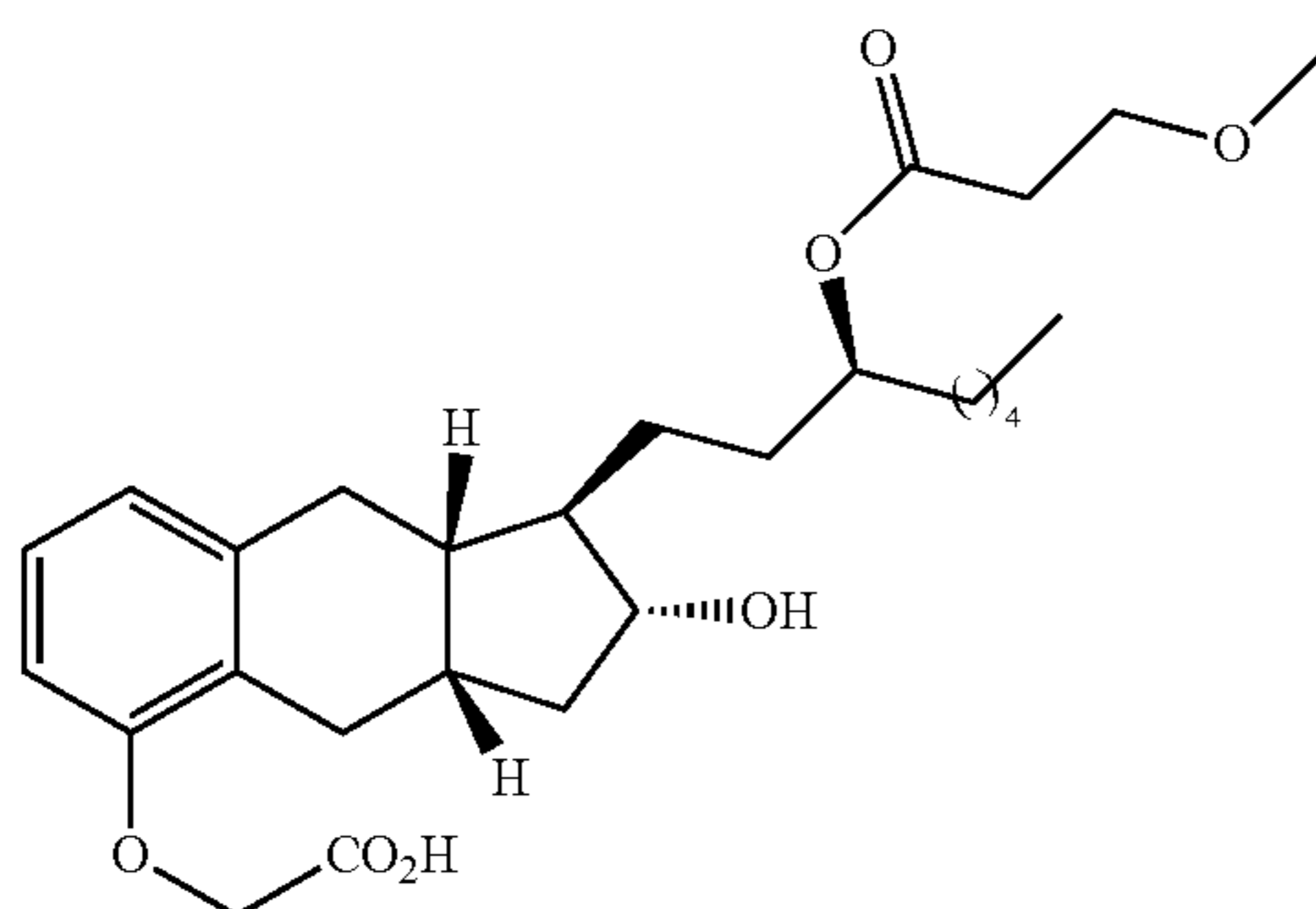
Compound Ib-6
