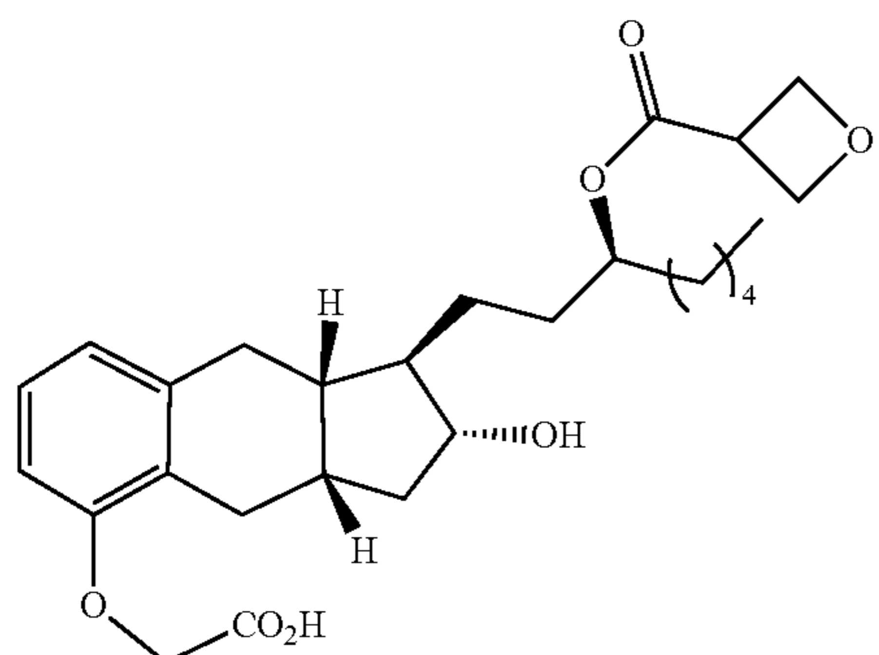
Compound Ib-33
