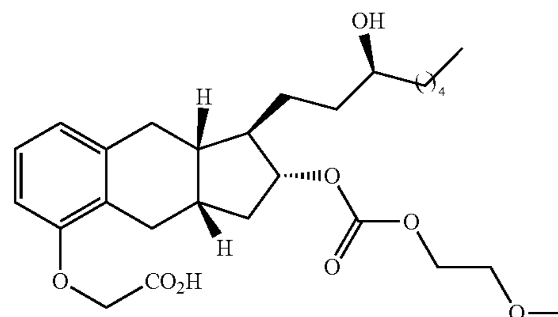
Compound Ib-1
