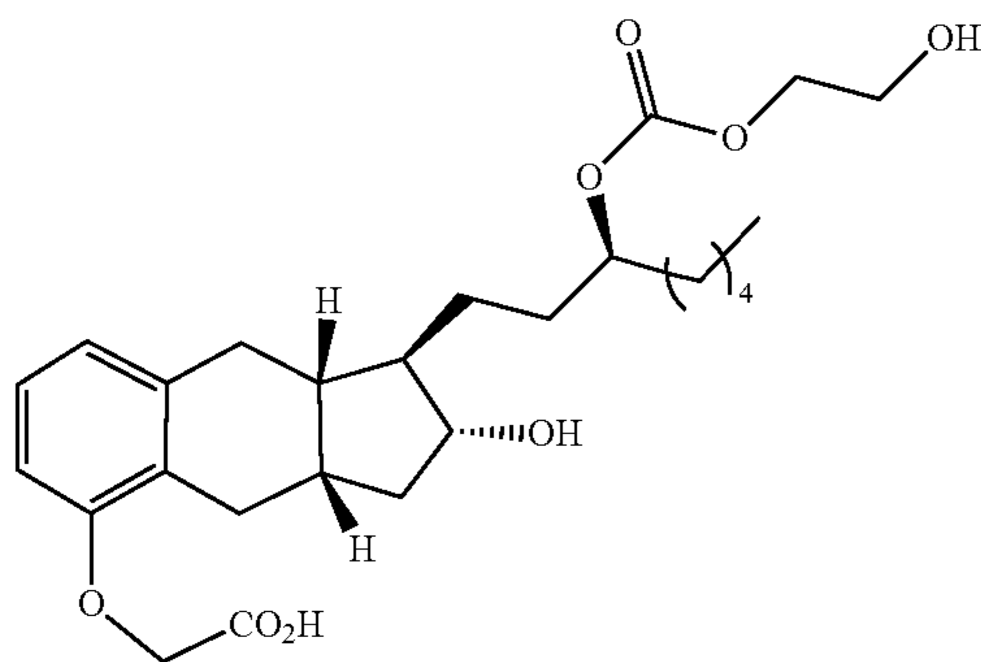
Compound Ib-15
