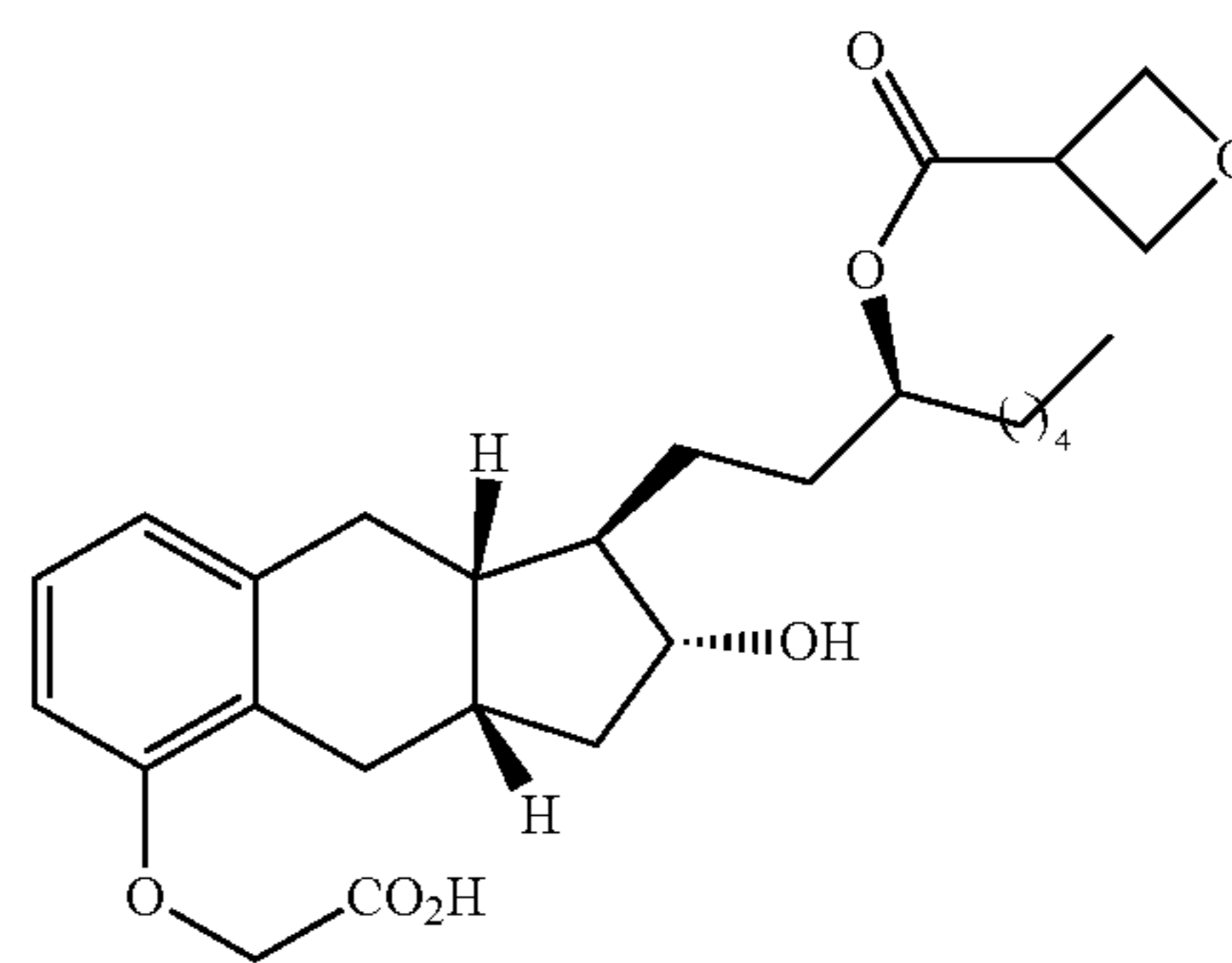
Compound Ib-32
