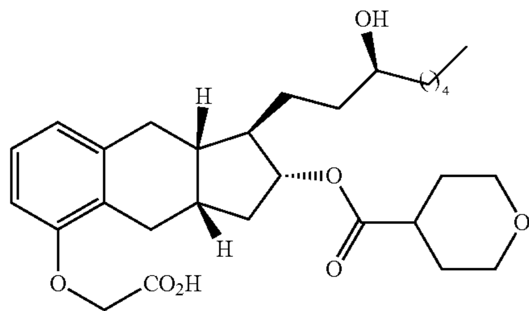
Compound Ia-10
