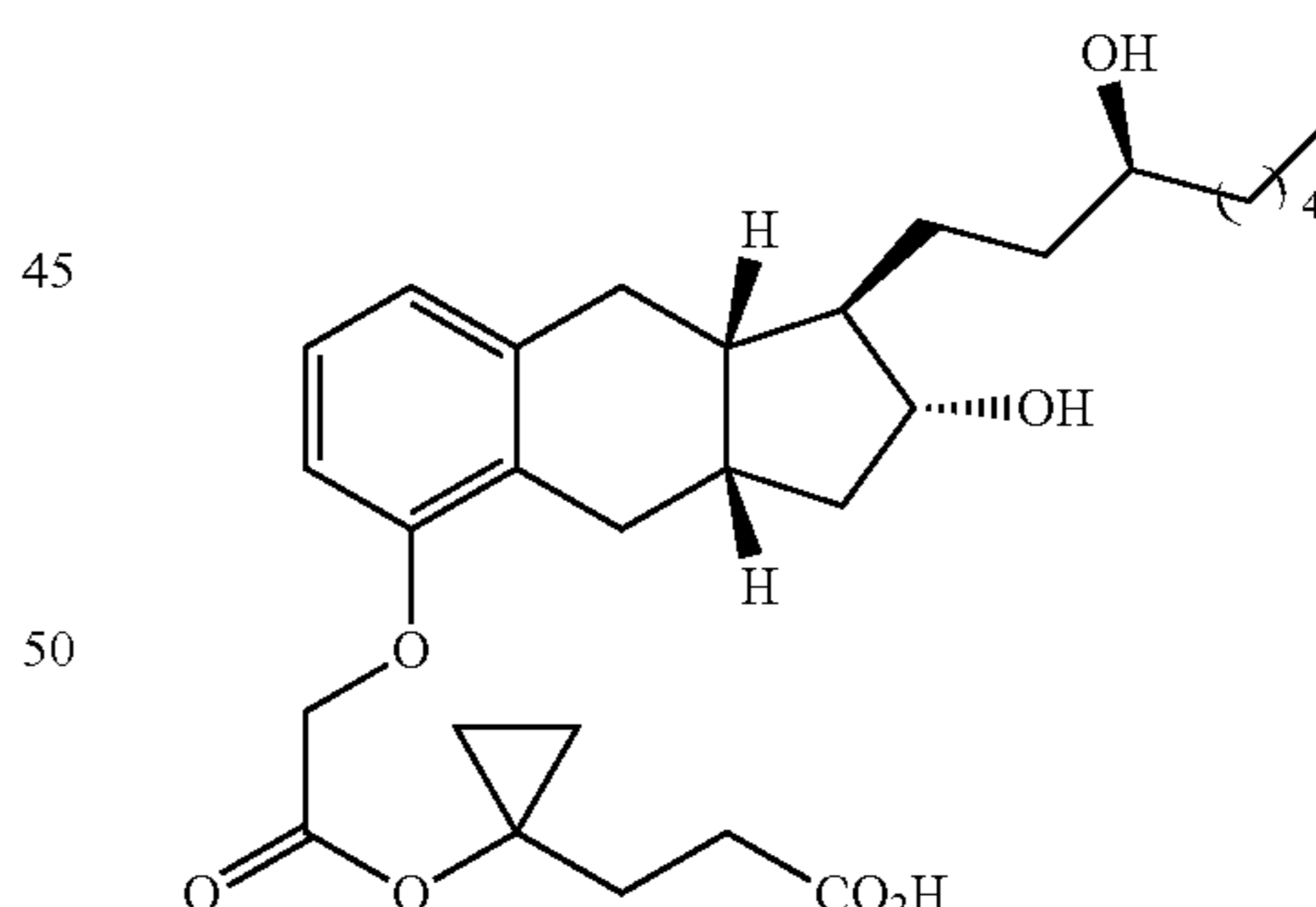
Compound II-25
