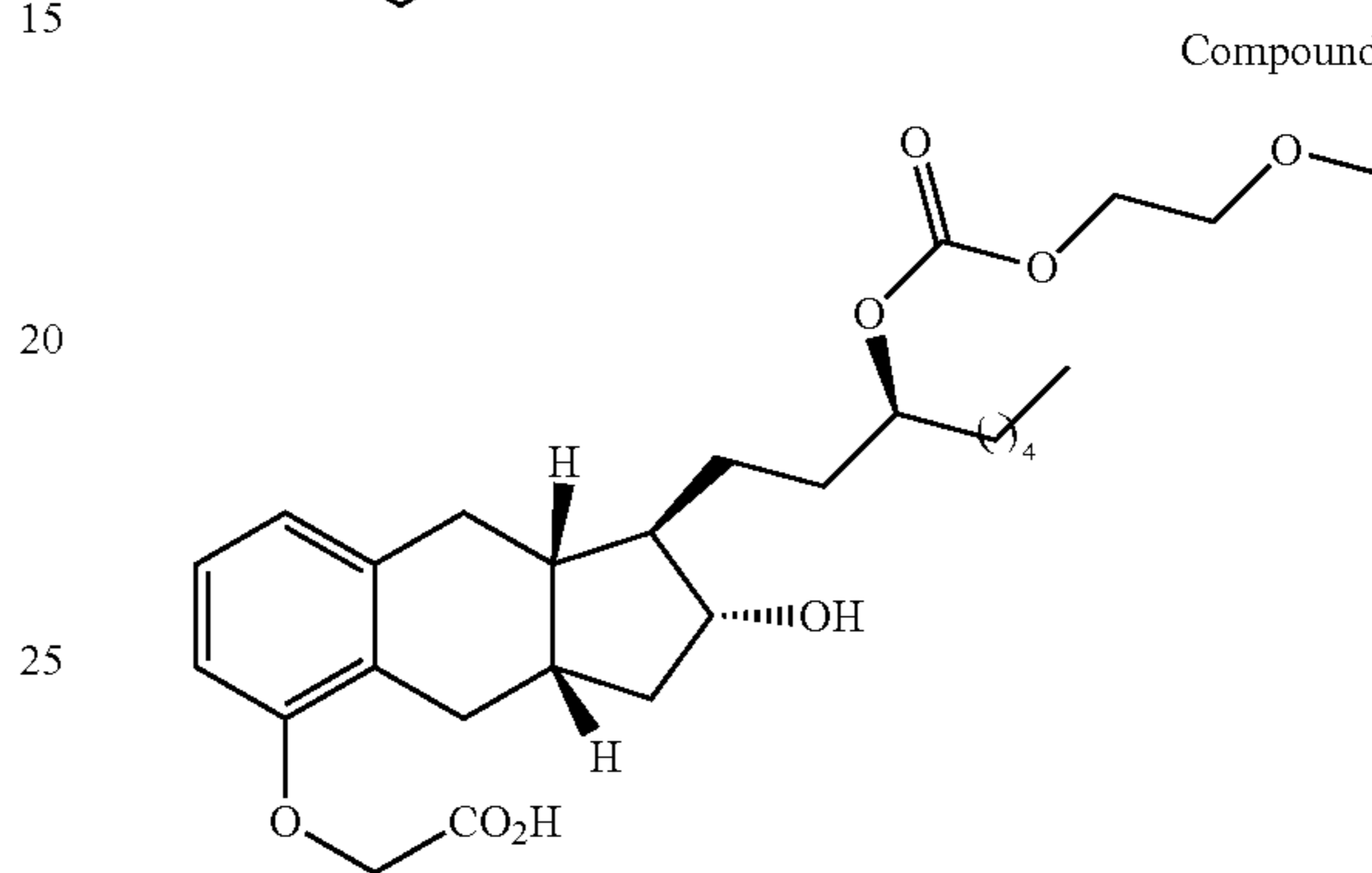
Compound Ib-11
