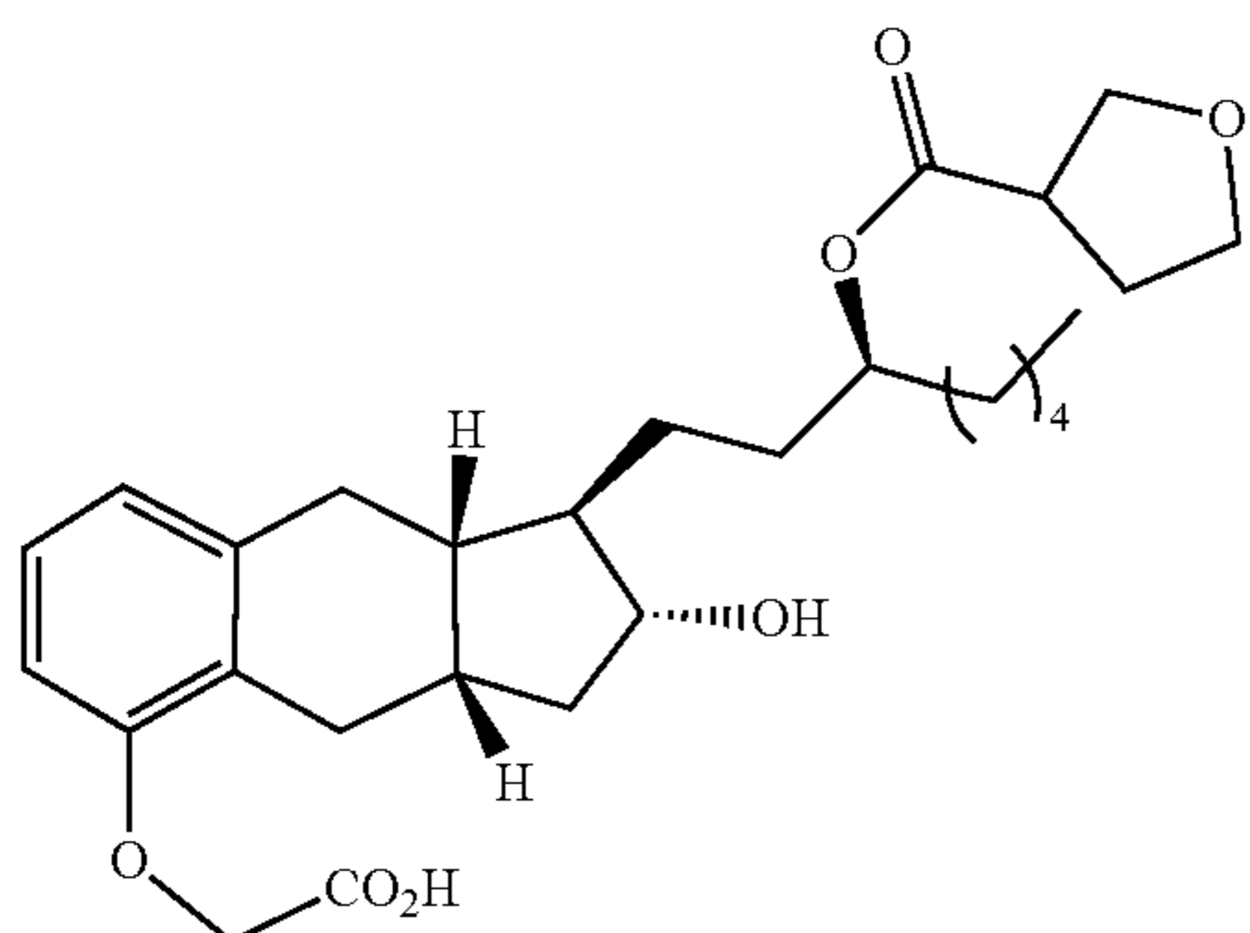
Compound Ib-33
