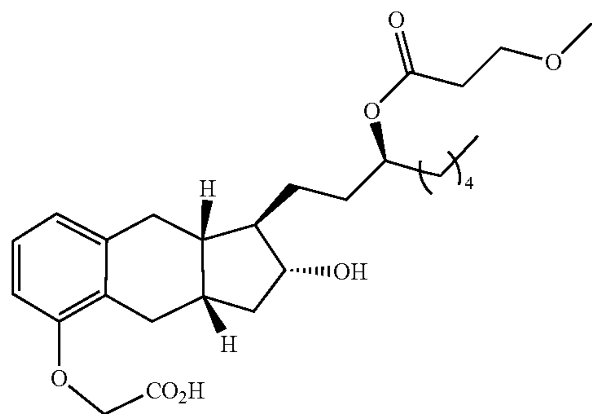
Compound Ib-6
