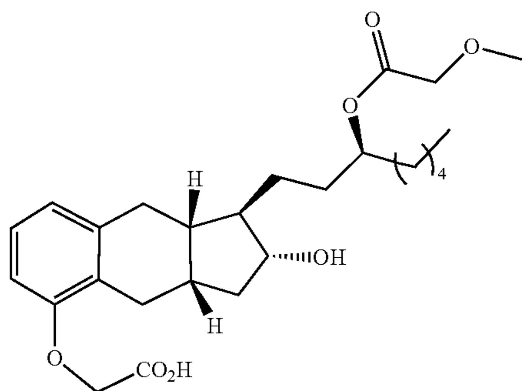
Compound Ib-8
