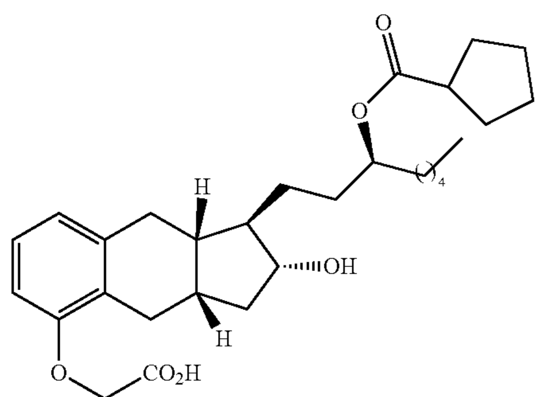
Compound Ib-30
