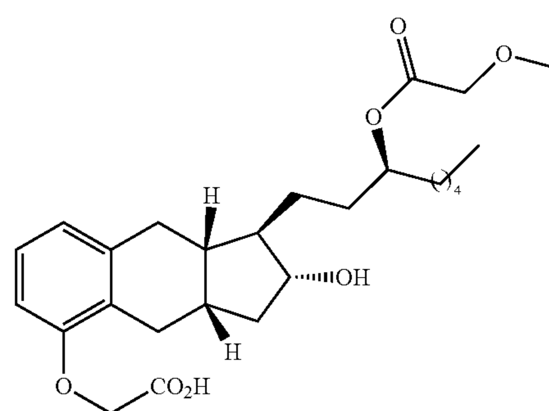
Compound Ib-8
