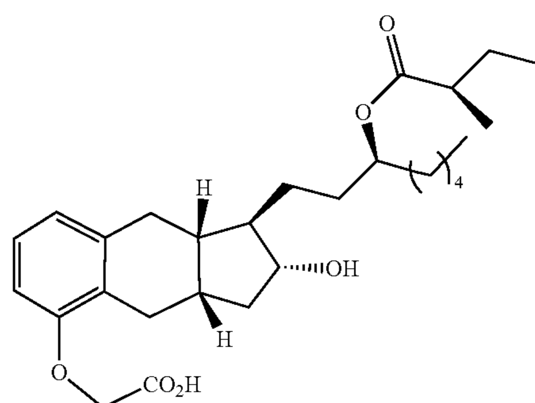
Compound Ib-29
