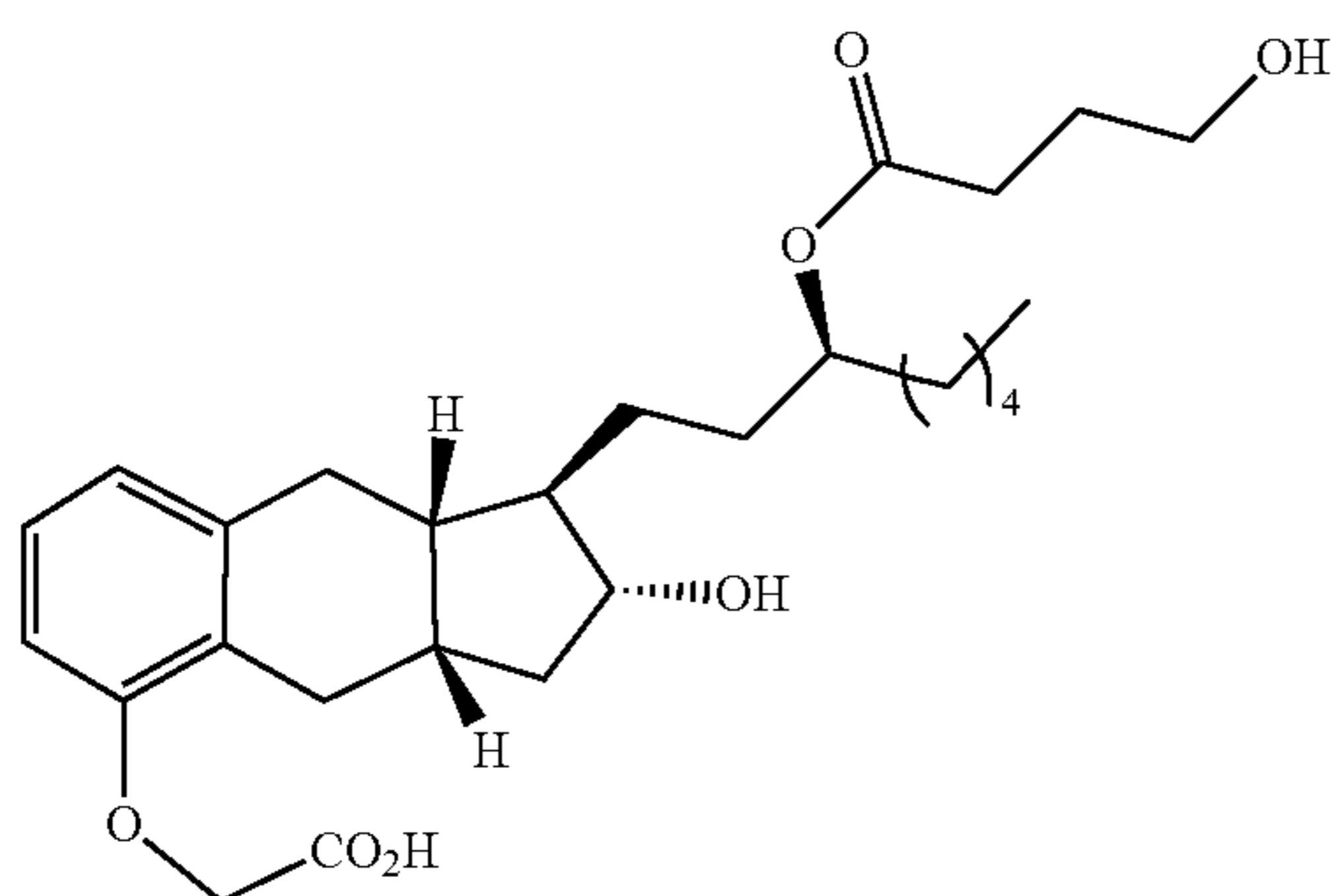
Compound Ib-18
