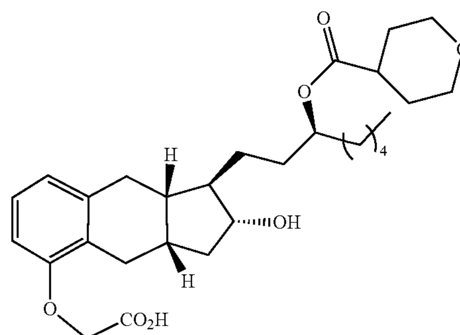
Compound Ib-34
