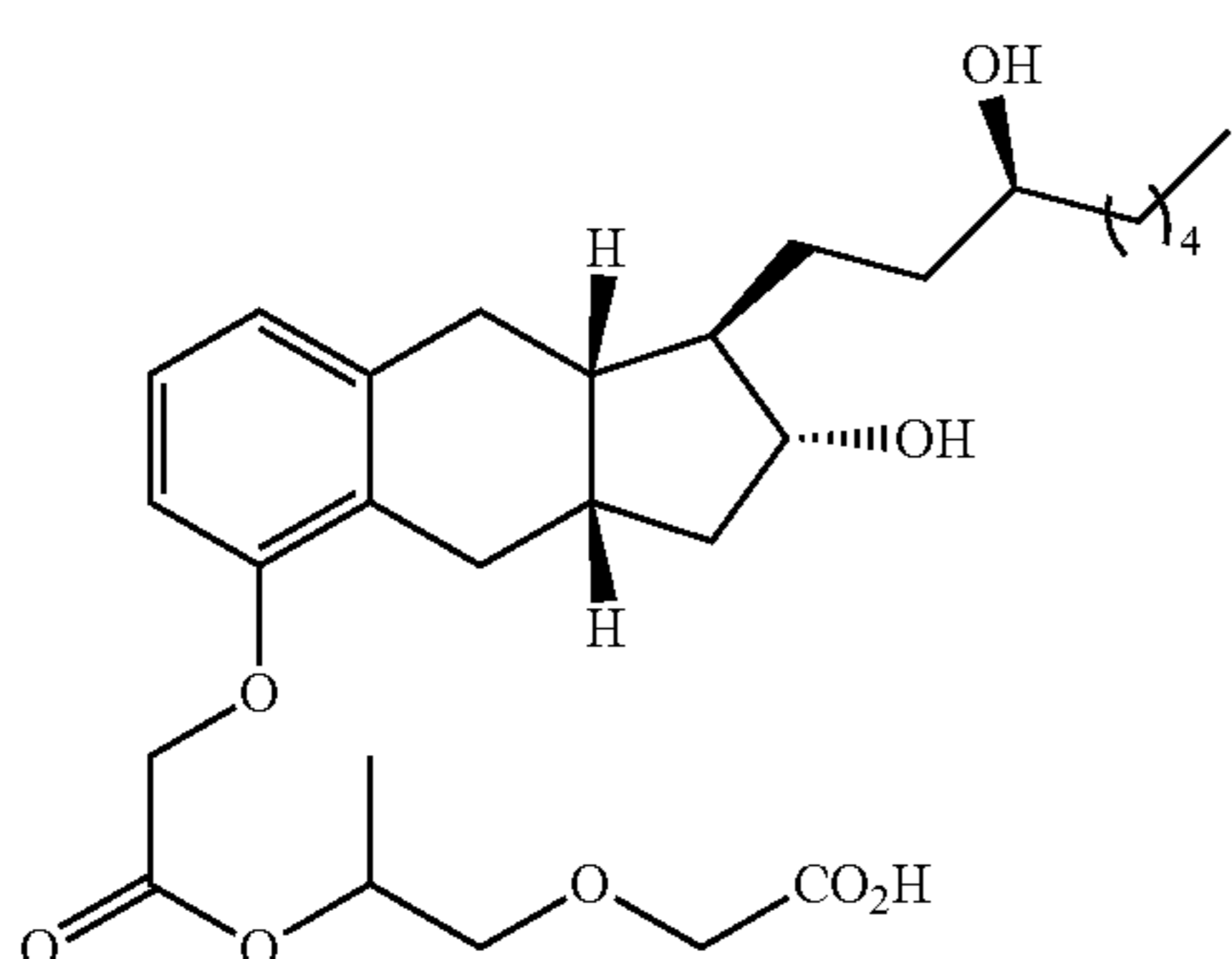
Compound II-14
