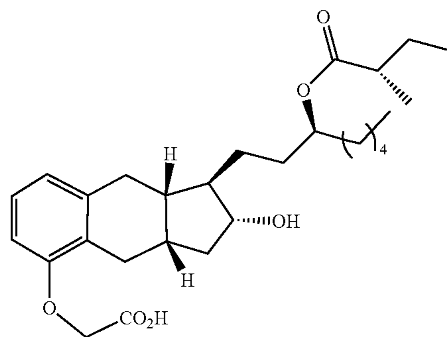
Compound Ib-27
