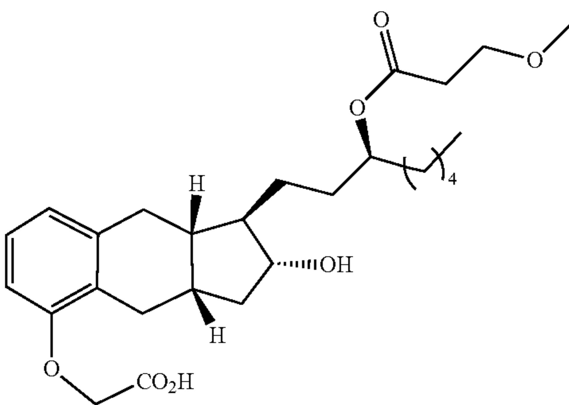
Compound Ib-6
