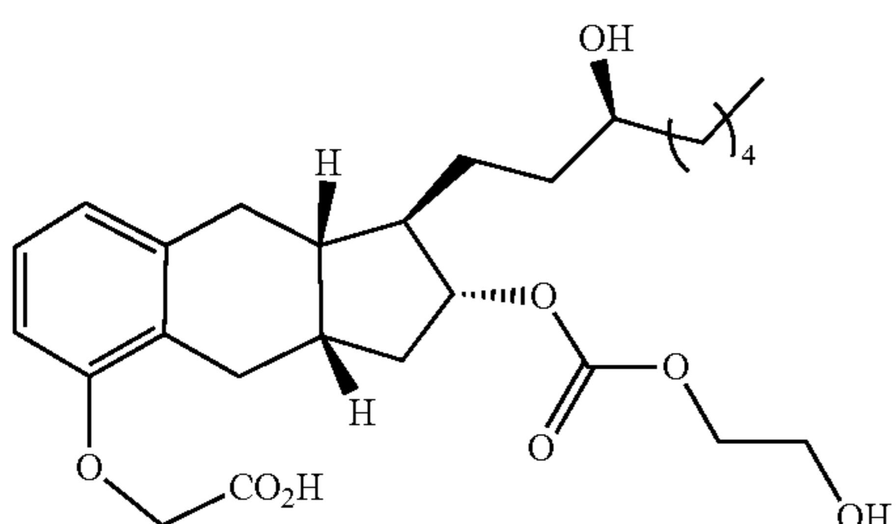
Compound Ia-15
