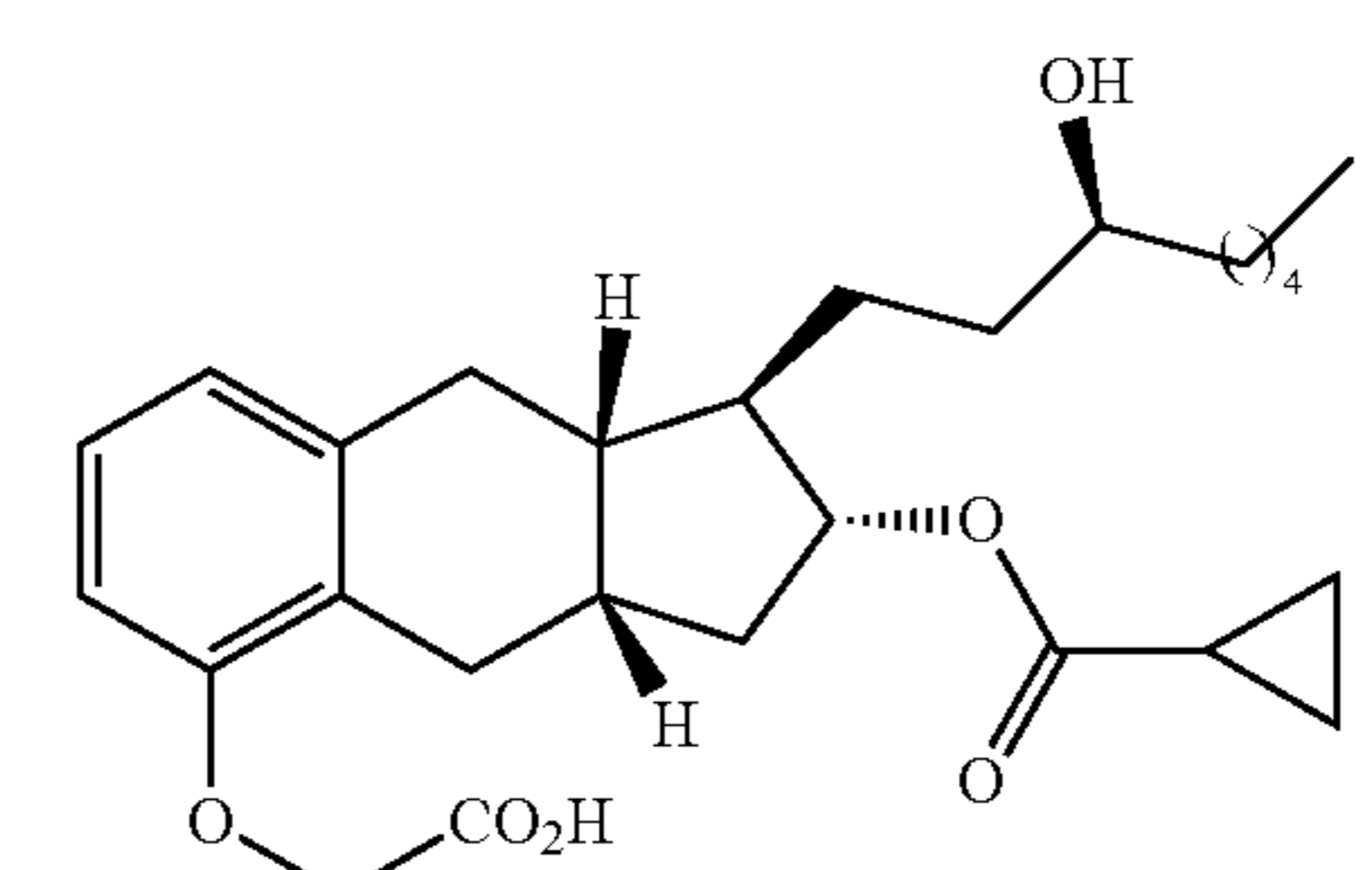
Compound Ia-29
