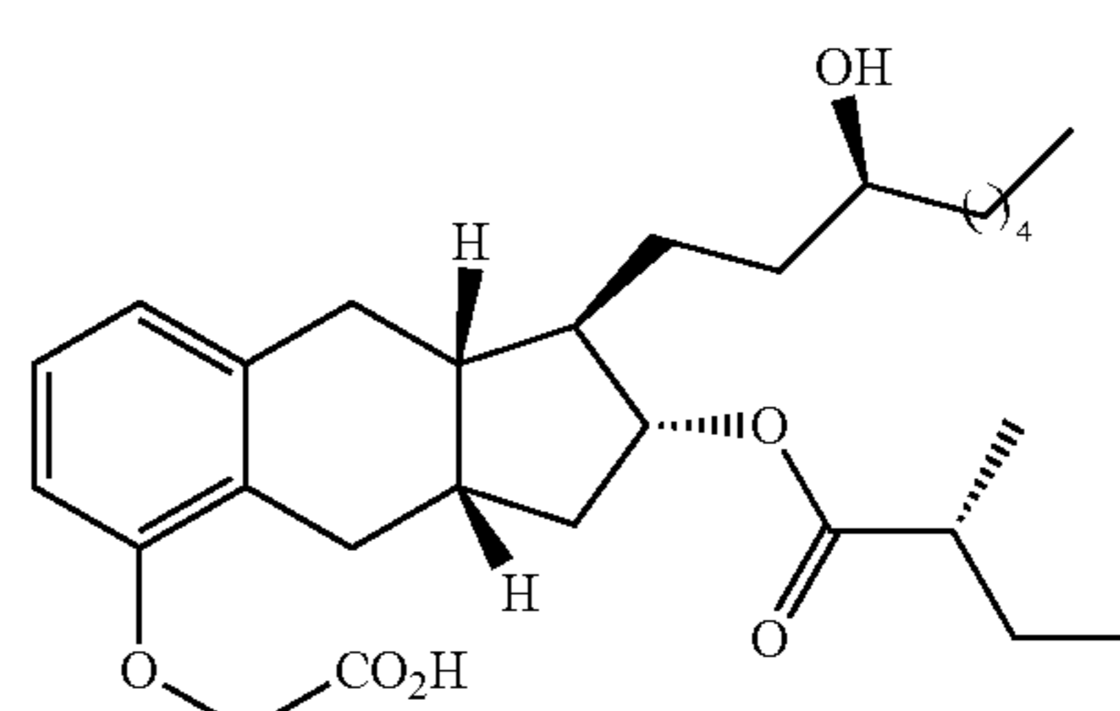
Compound Ia-28
