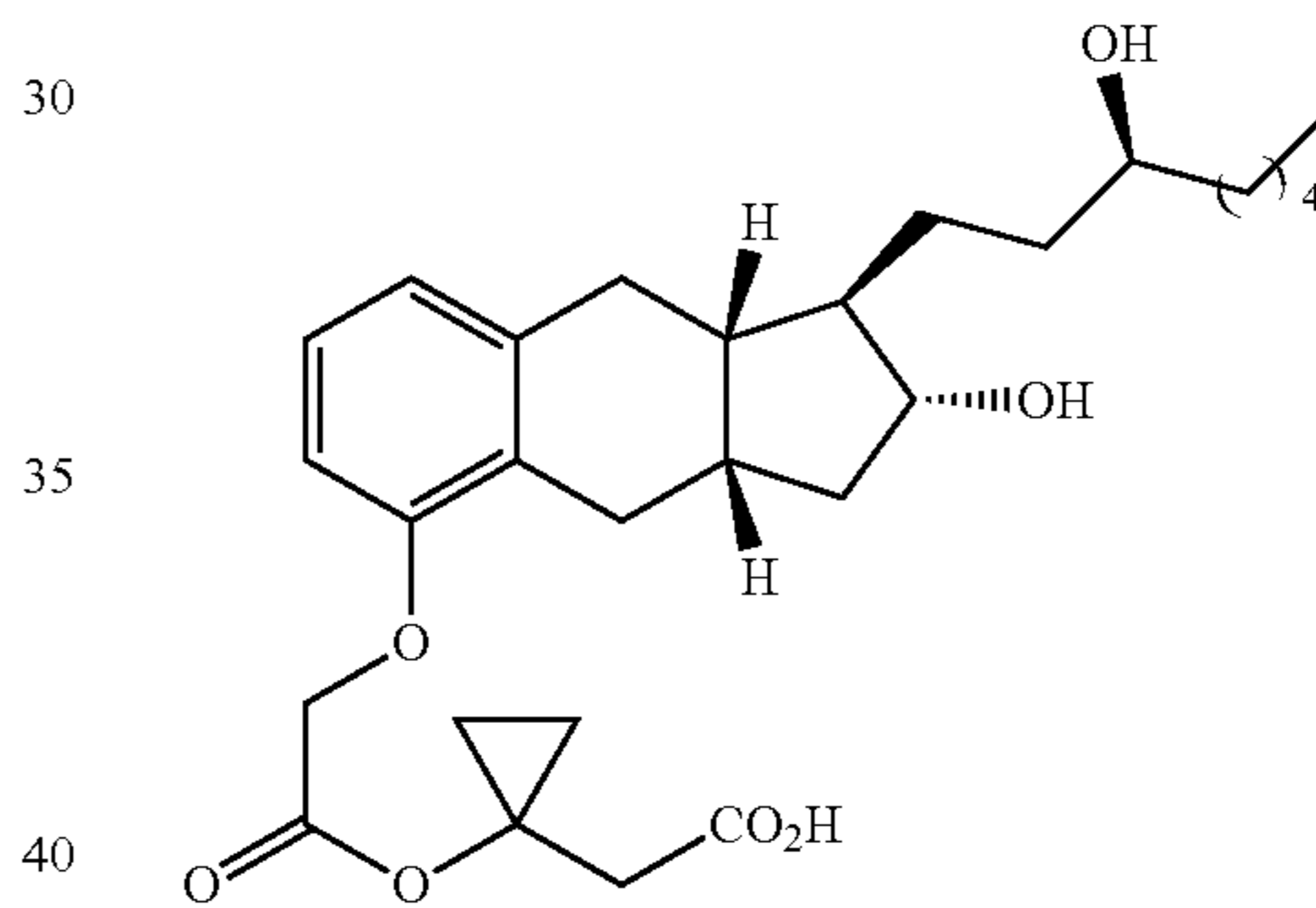
Compound II-24
