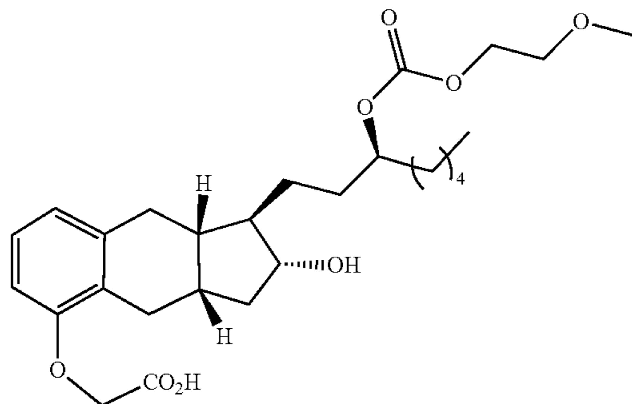
Compound Ib-15
