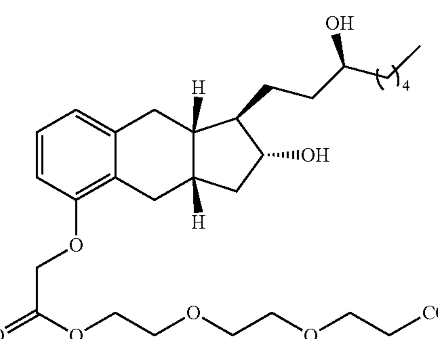
Compound II-19
