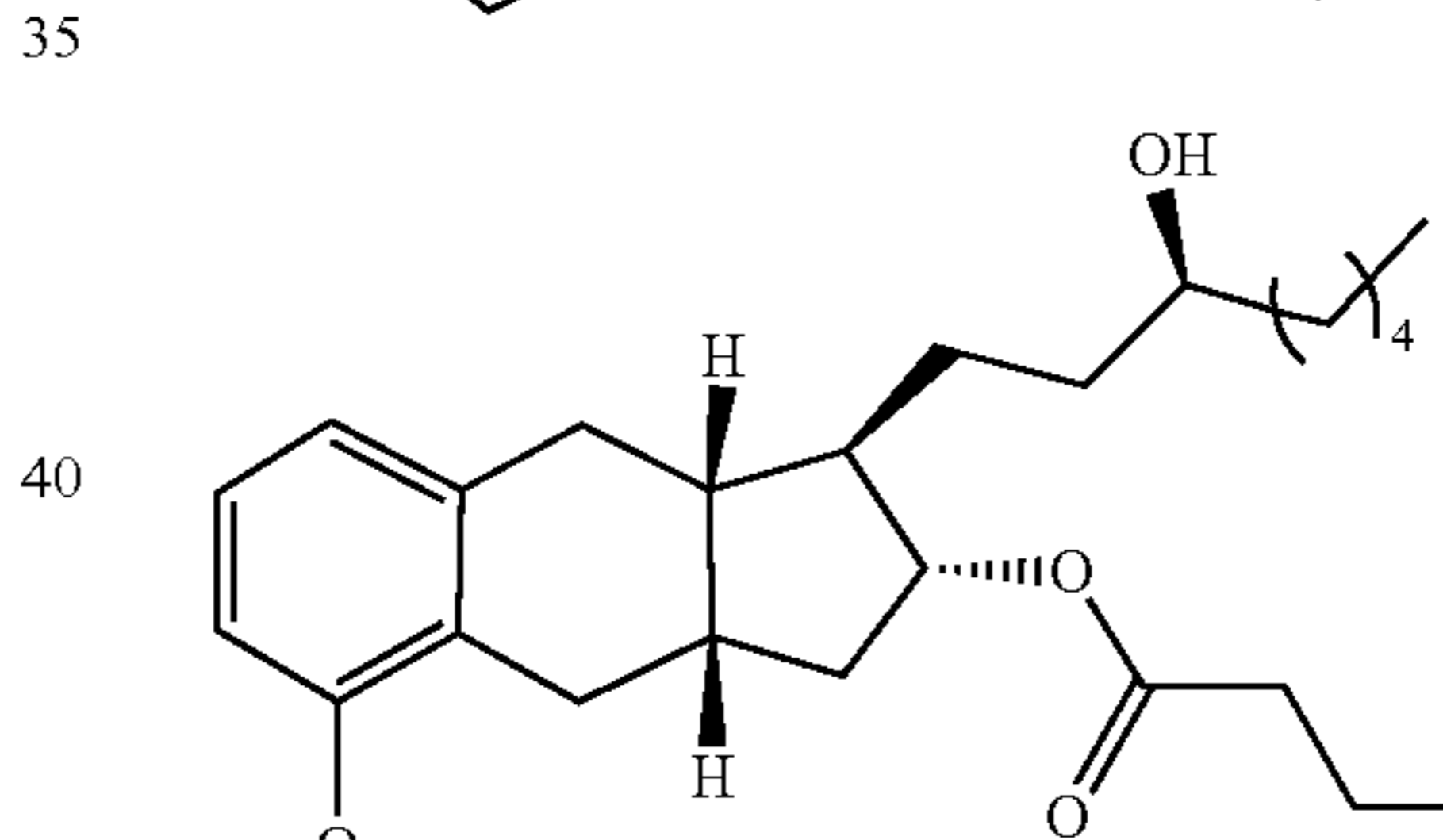
Compound Ia-2
