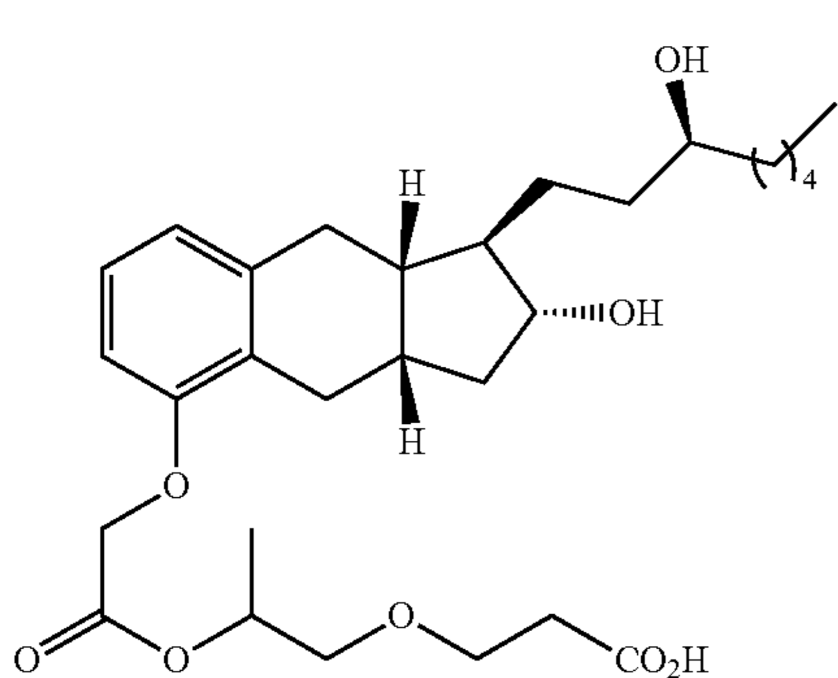
Compound II-16
