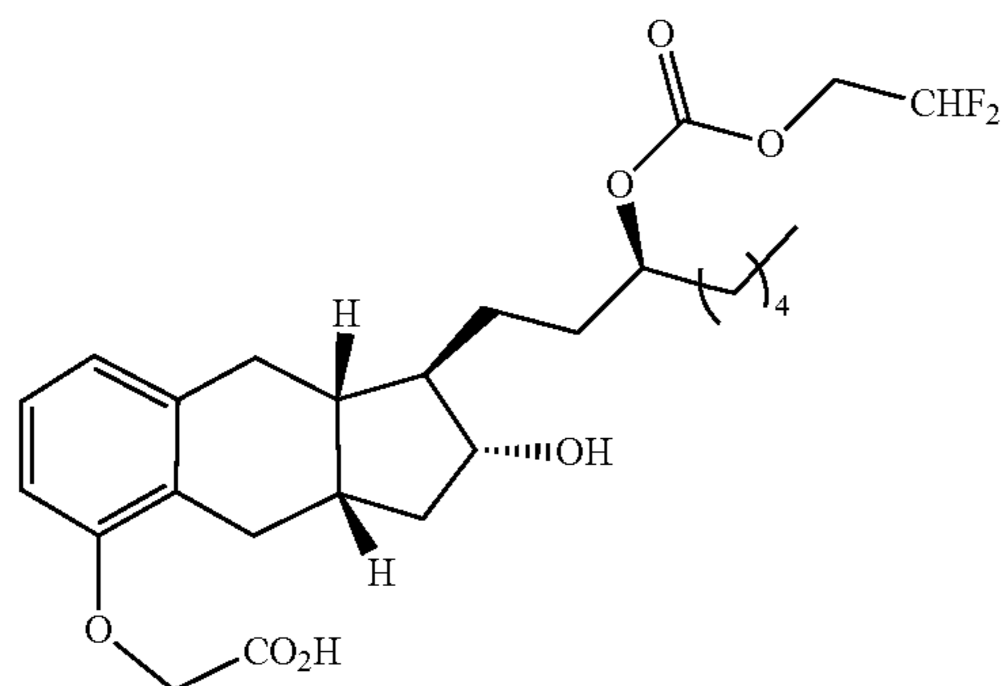
Compound Ib-13
