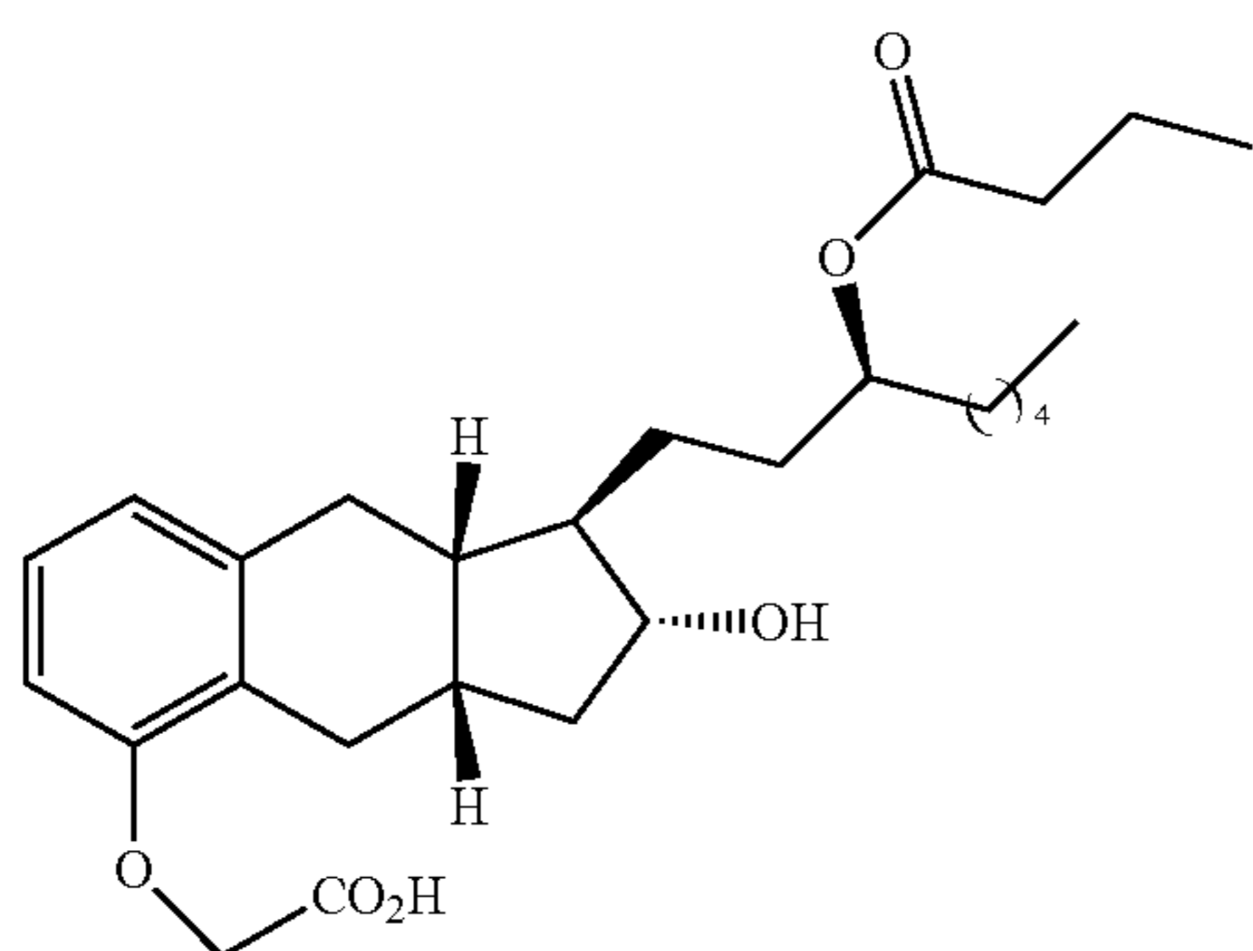
Compound Ib-2
