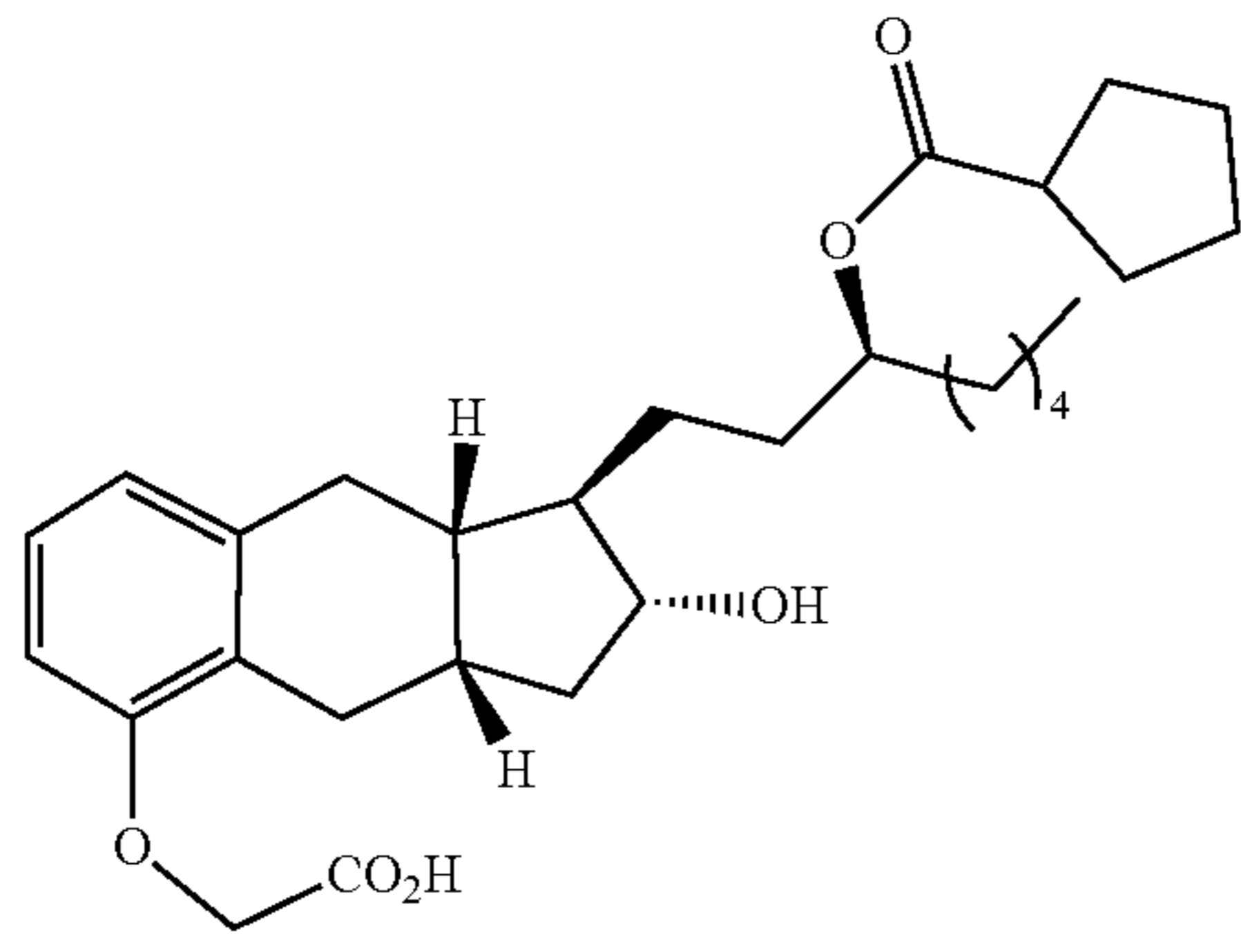
Compound Ib-30
