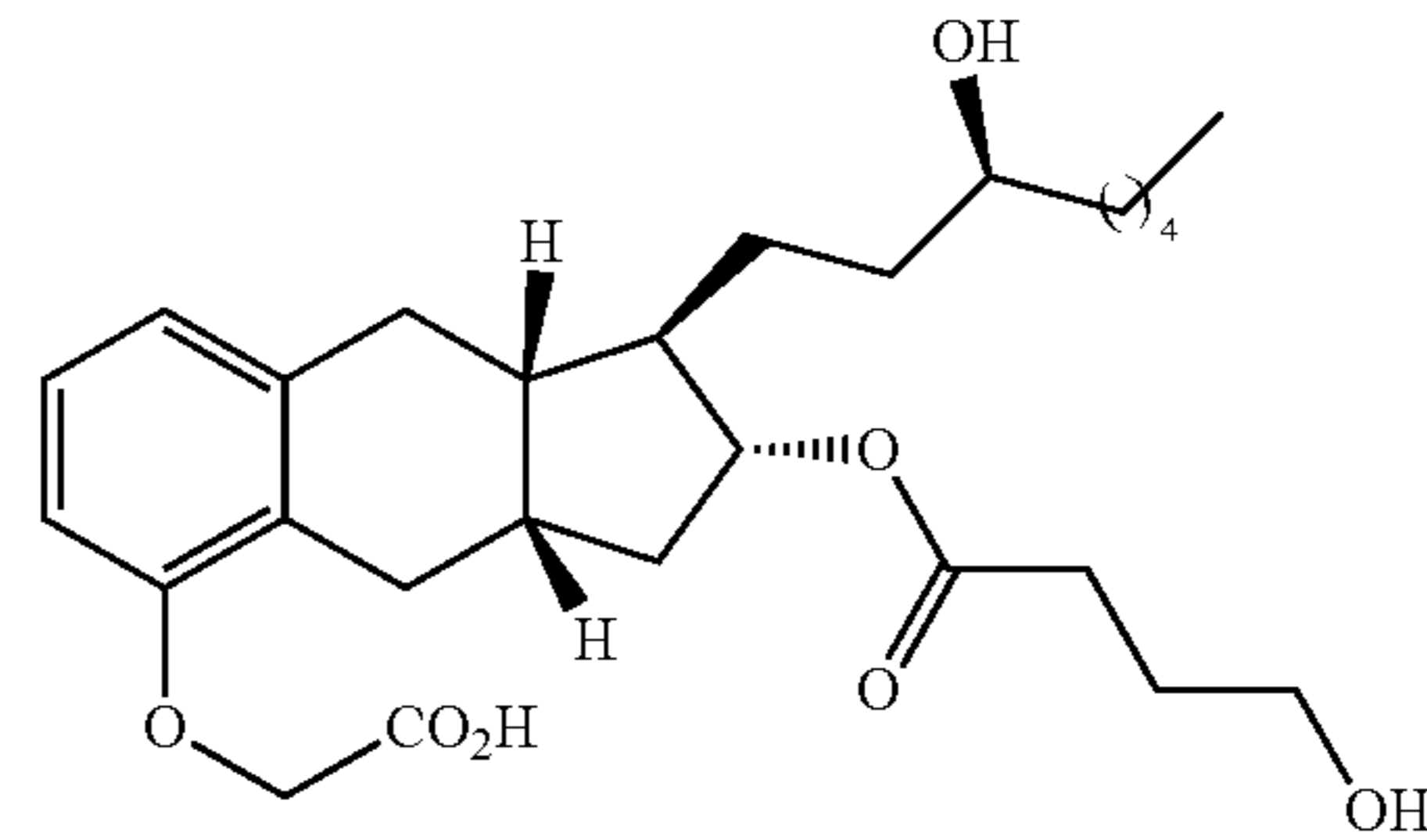
Compound Ia-18
