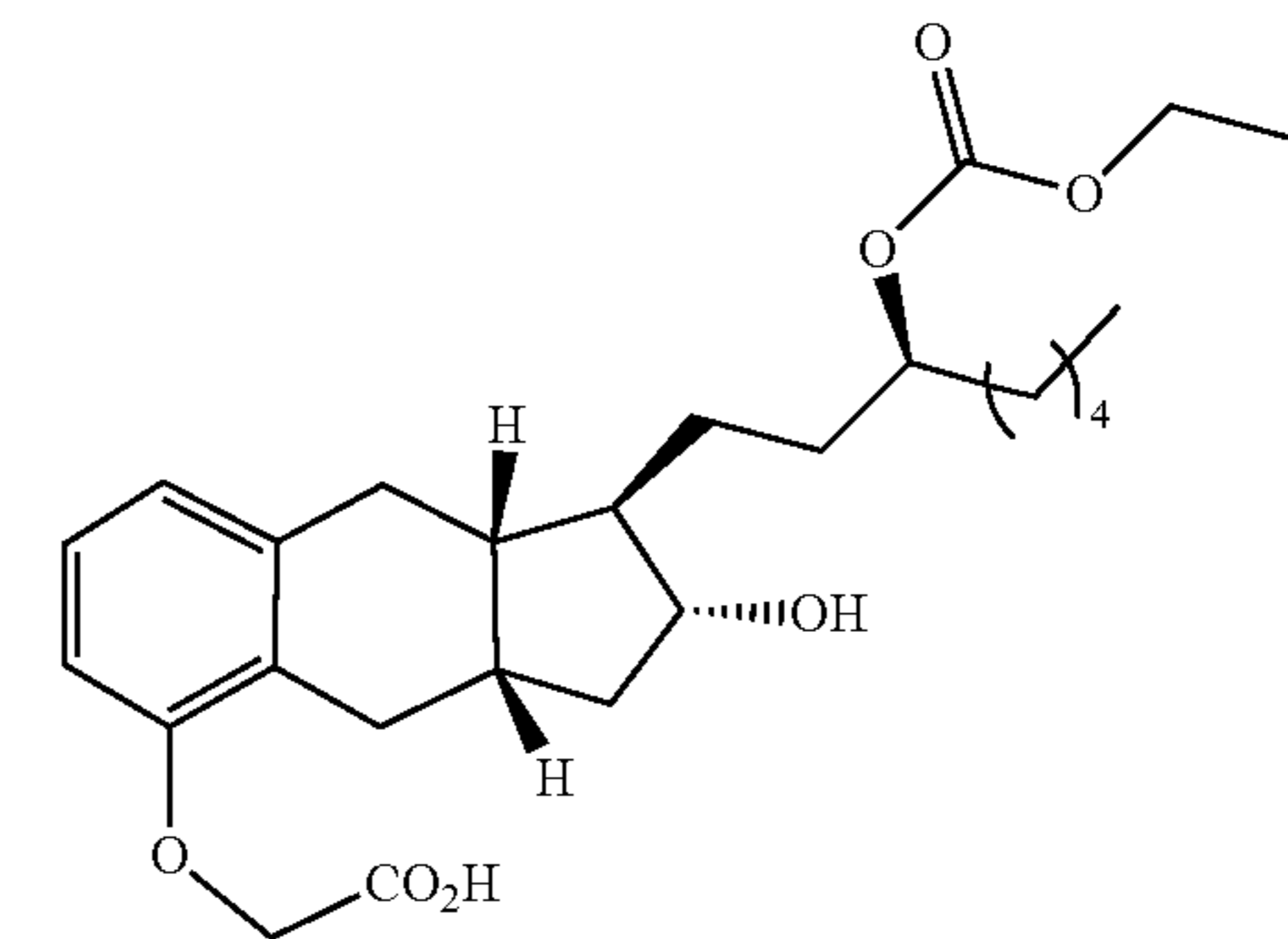
Compound Ib-12
