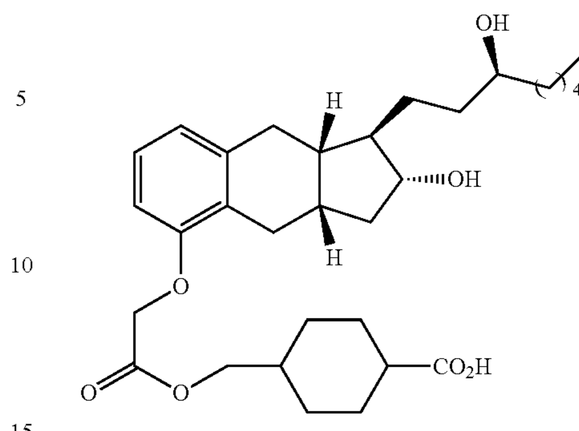
Compound II-27
