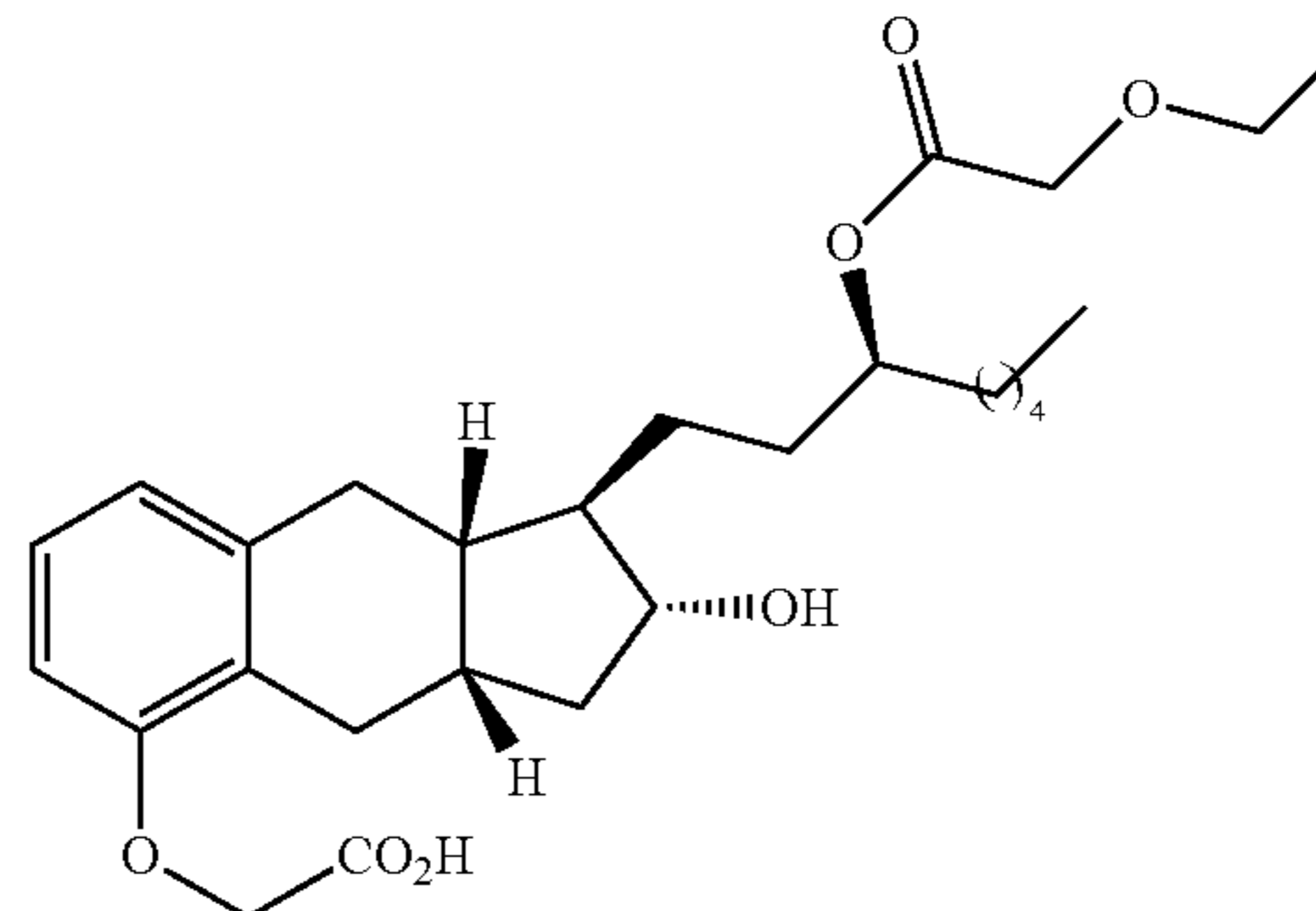
Compound Ib-9
