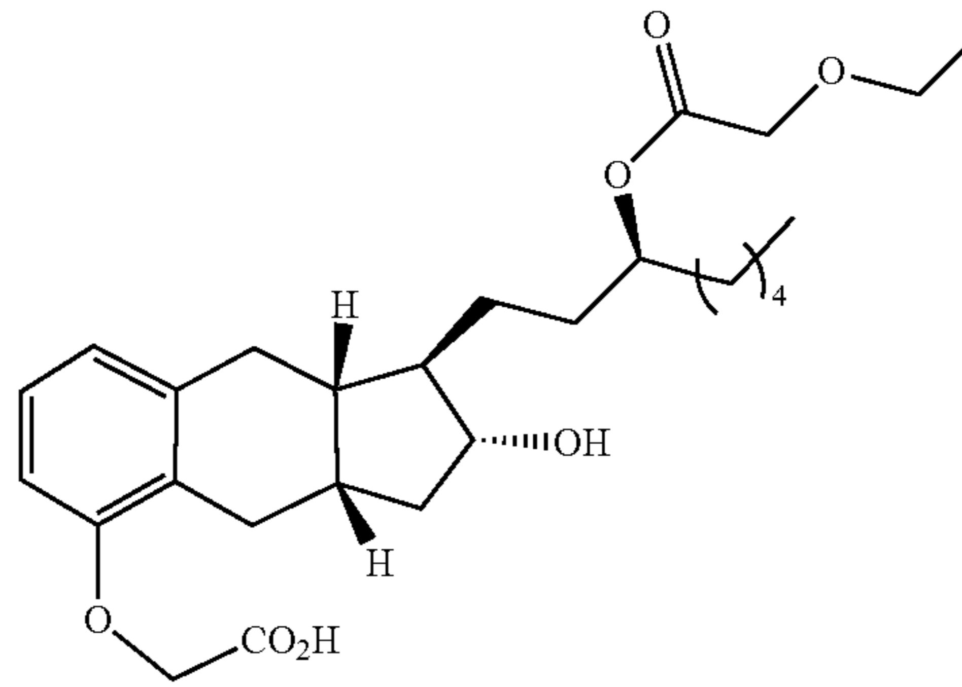
Compound Ib-9
