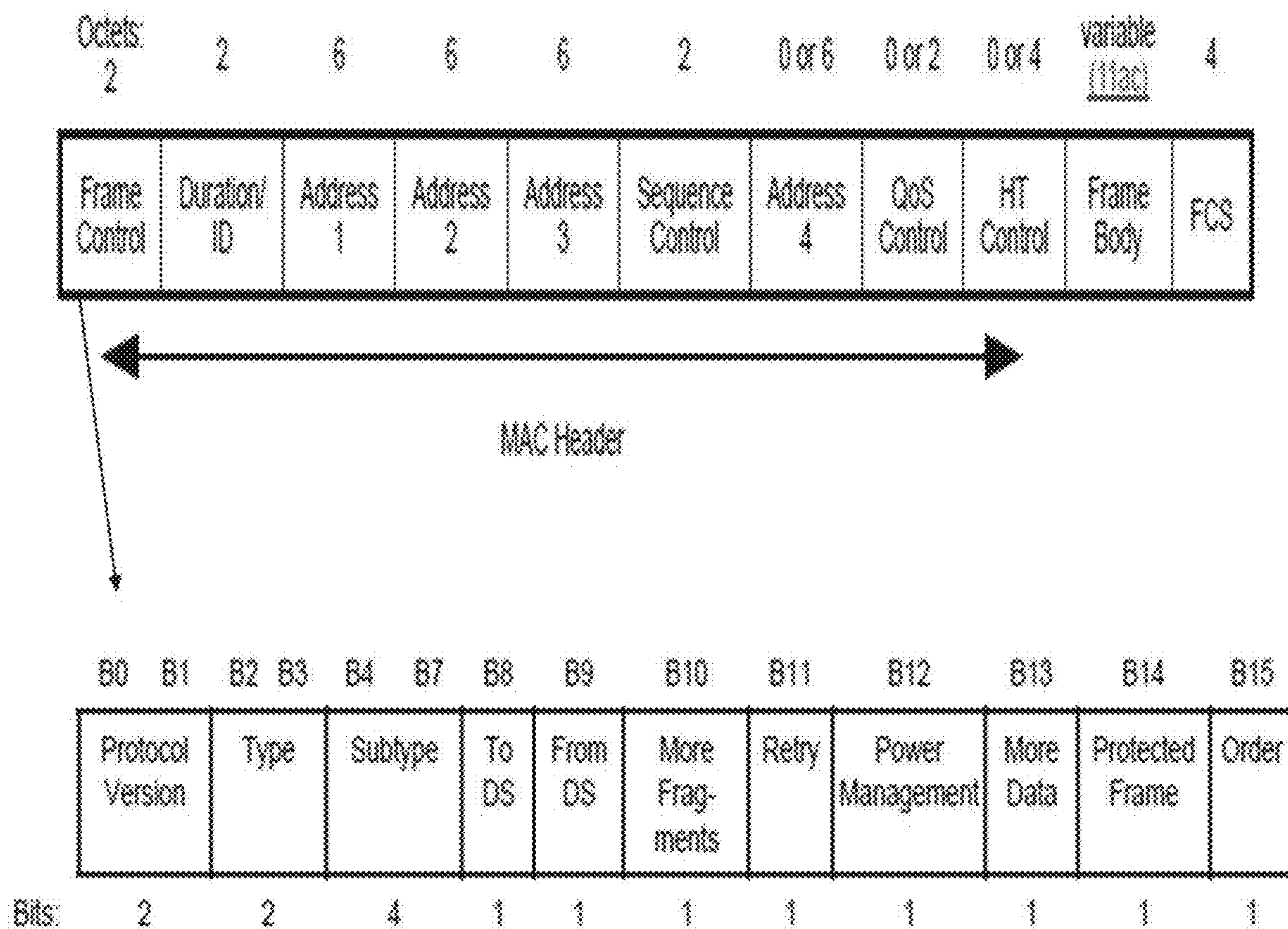
FIG. 5 (PRIOR ART)
