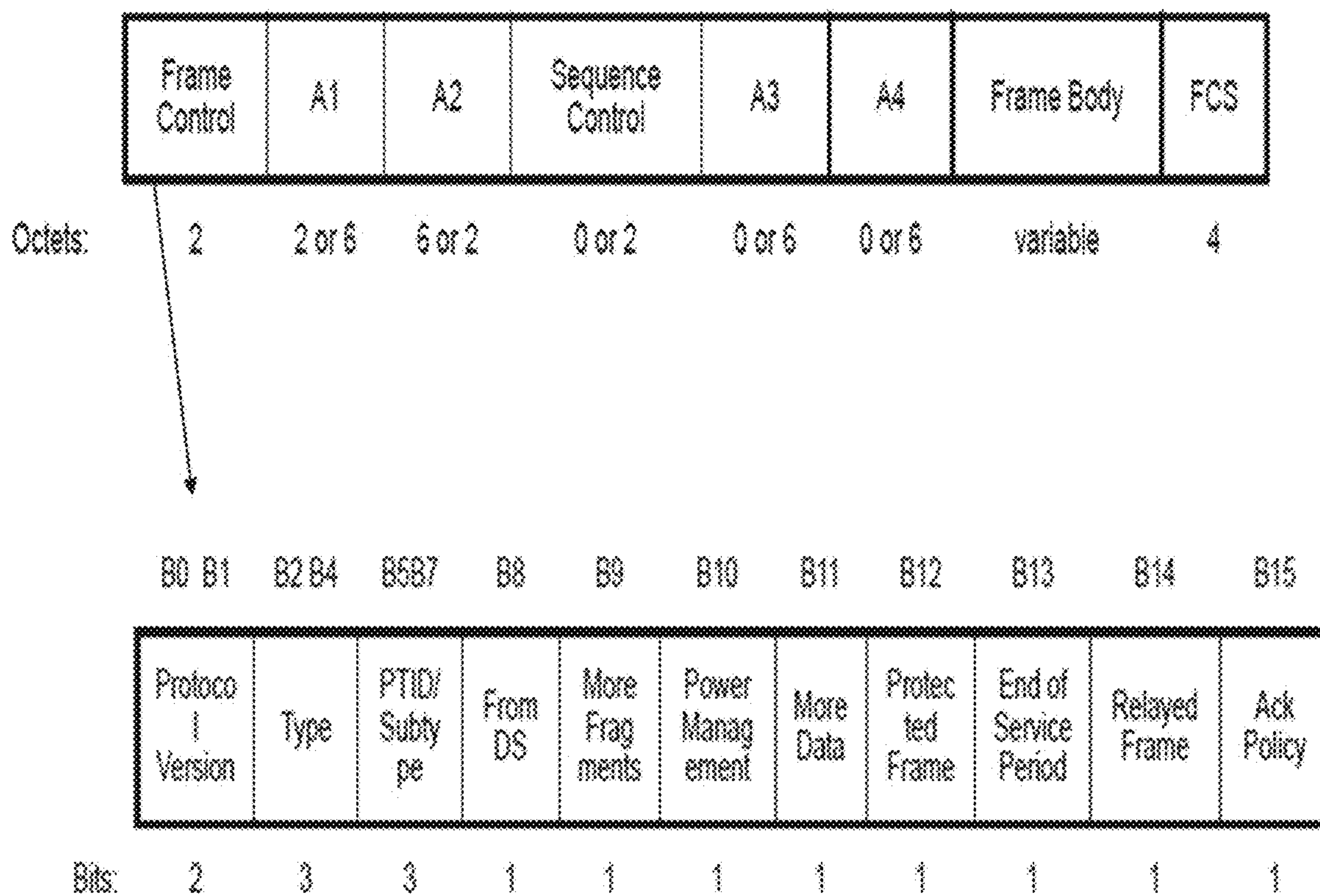
FIG. 6 (PRIOR ART)
