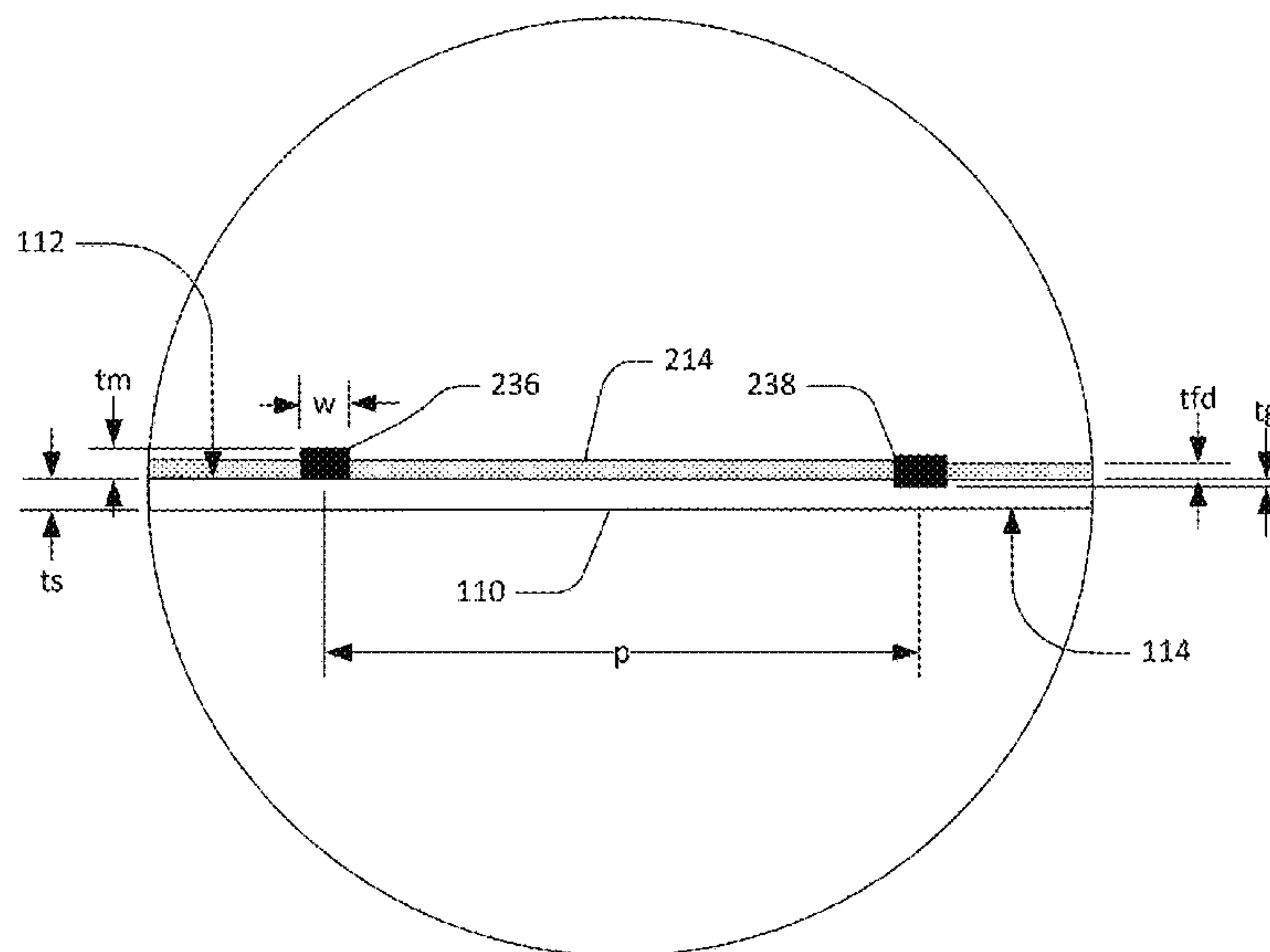
DETAIL C
