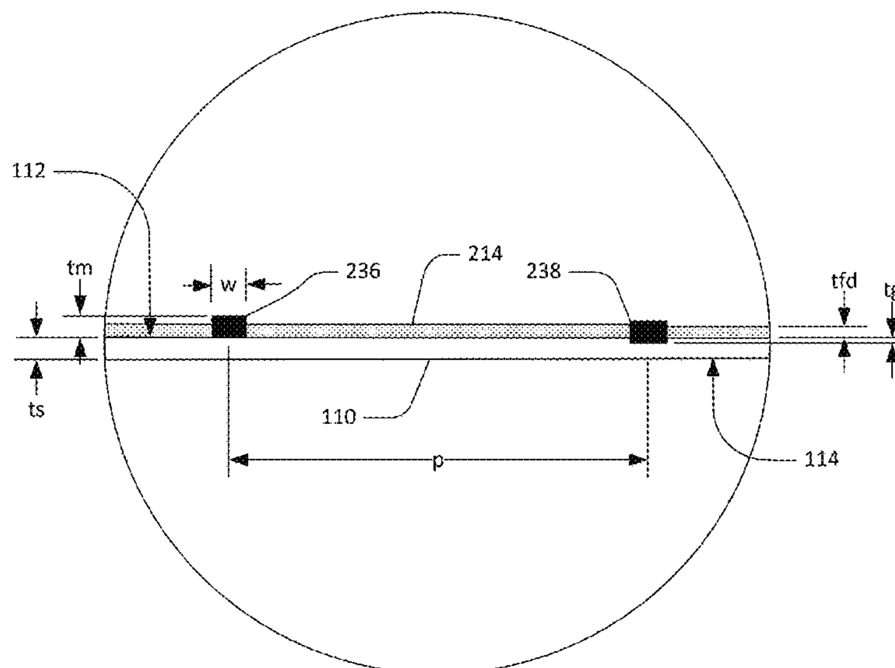
DETAIL C
