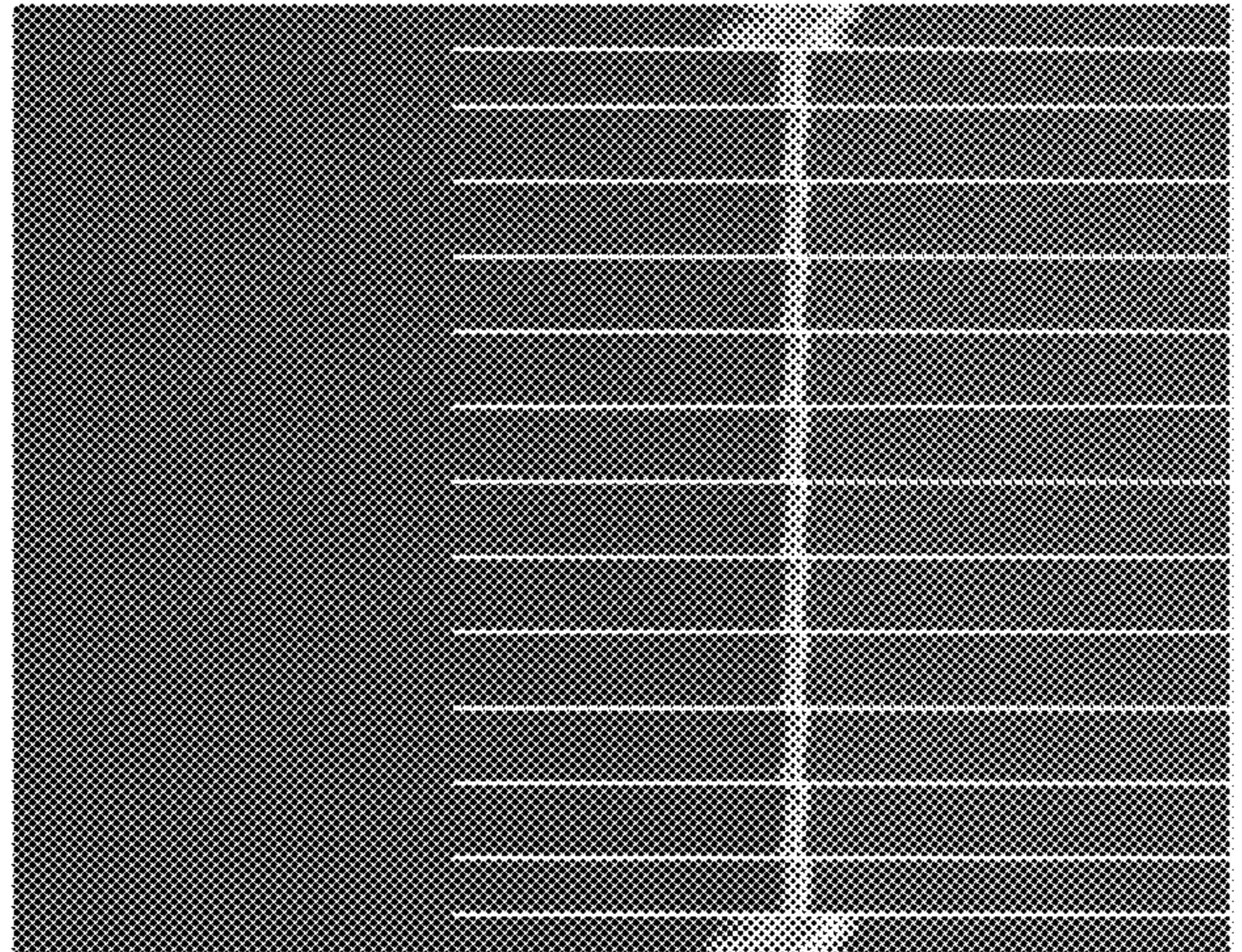
Solid Sub-model results @ 60 s
