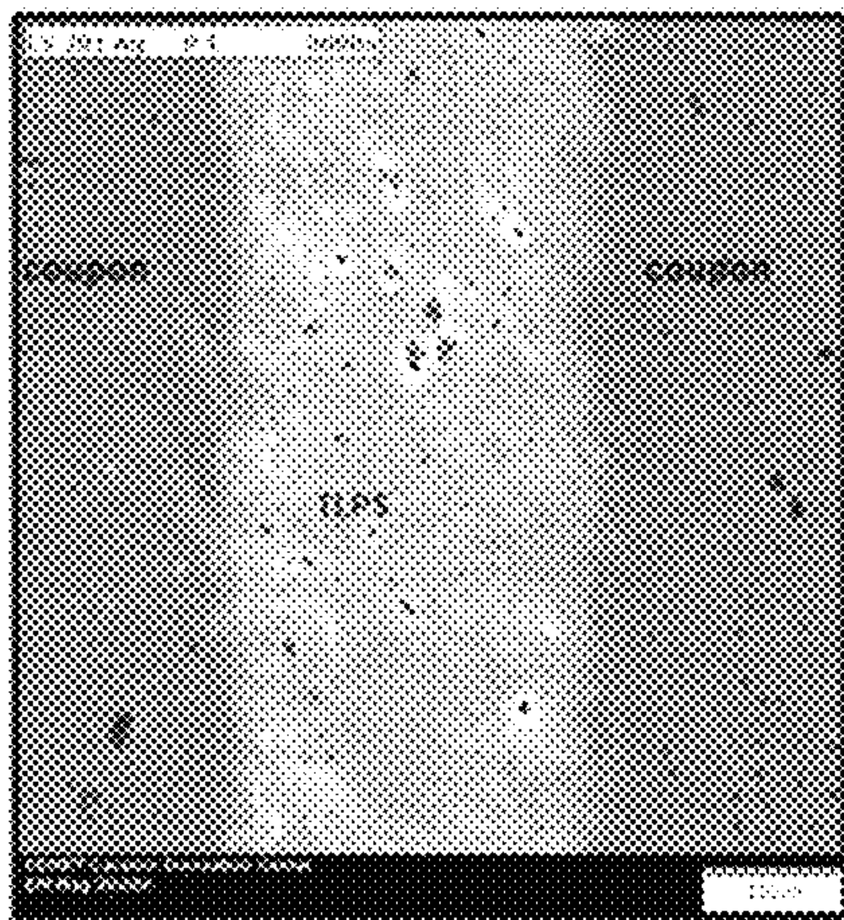
Ag/SnBi THERMO-COMPRESSSION BOND NO POST CURE
