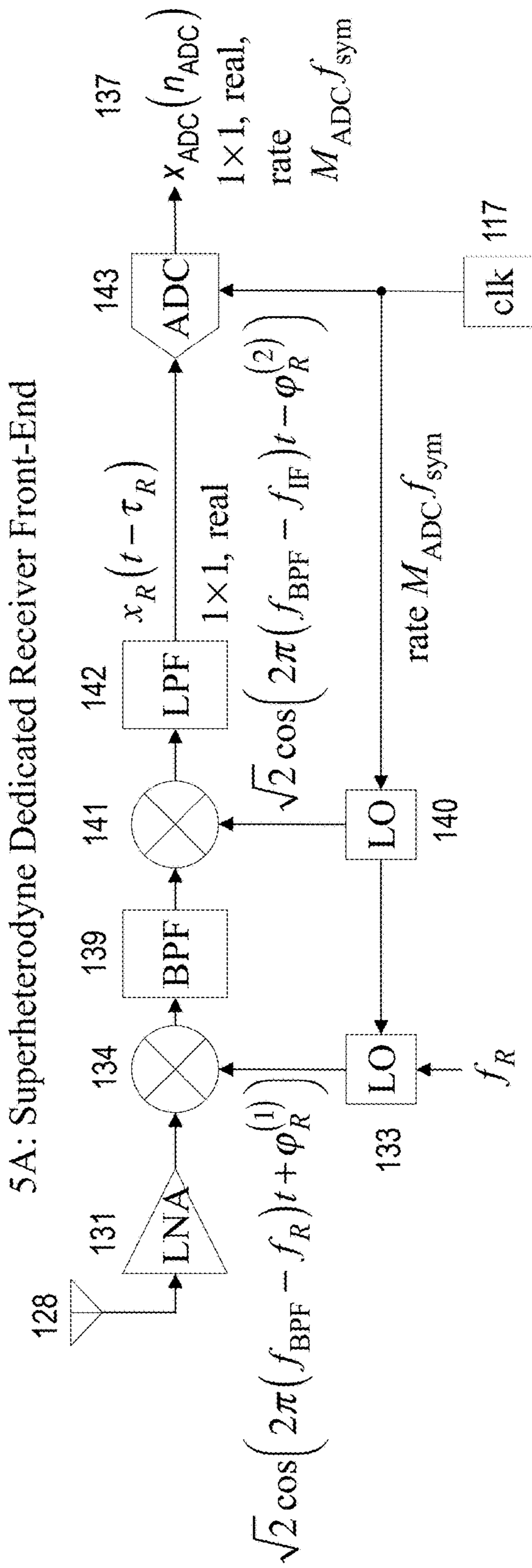
Figure 5 (Prior Art) 5A: Superheterodyne Dedicated Receiver Front-End 5B: Superheterodyne SDR Receiver Front-End
