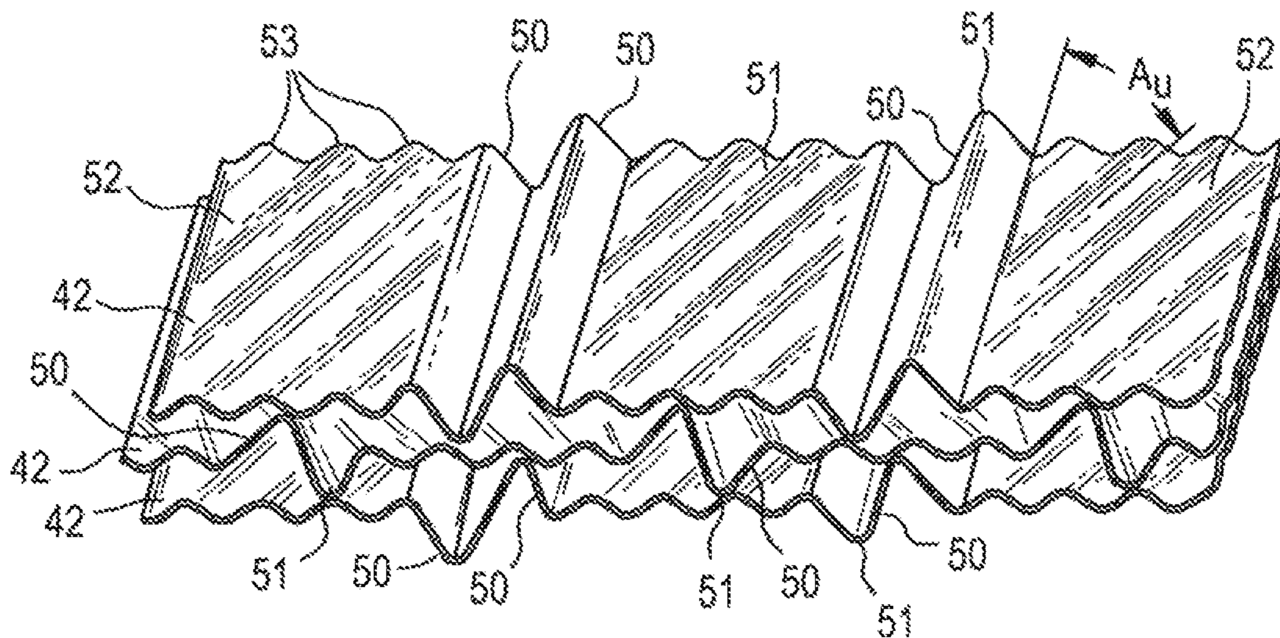
FIG. 3 PRIOR ART
