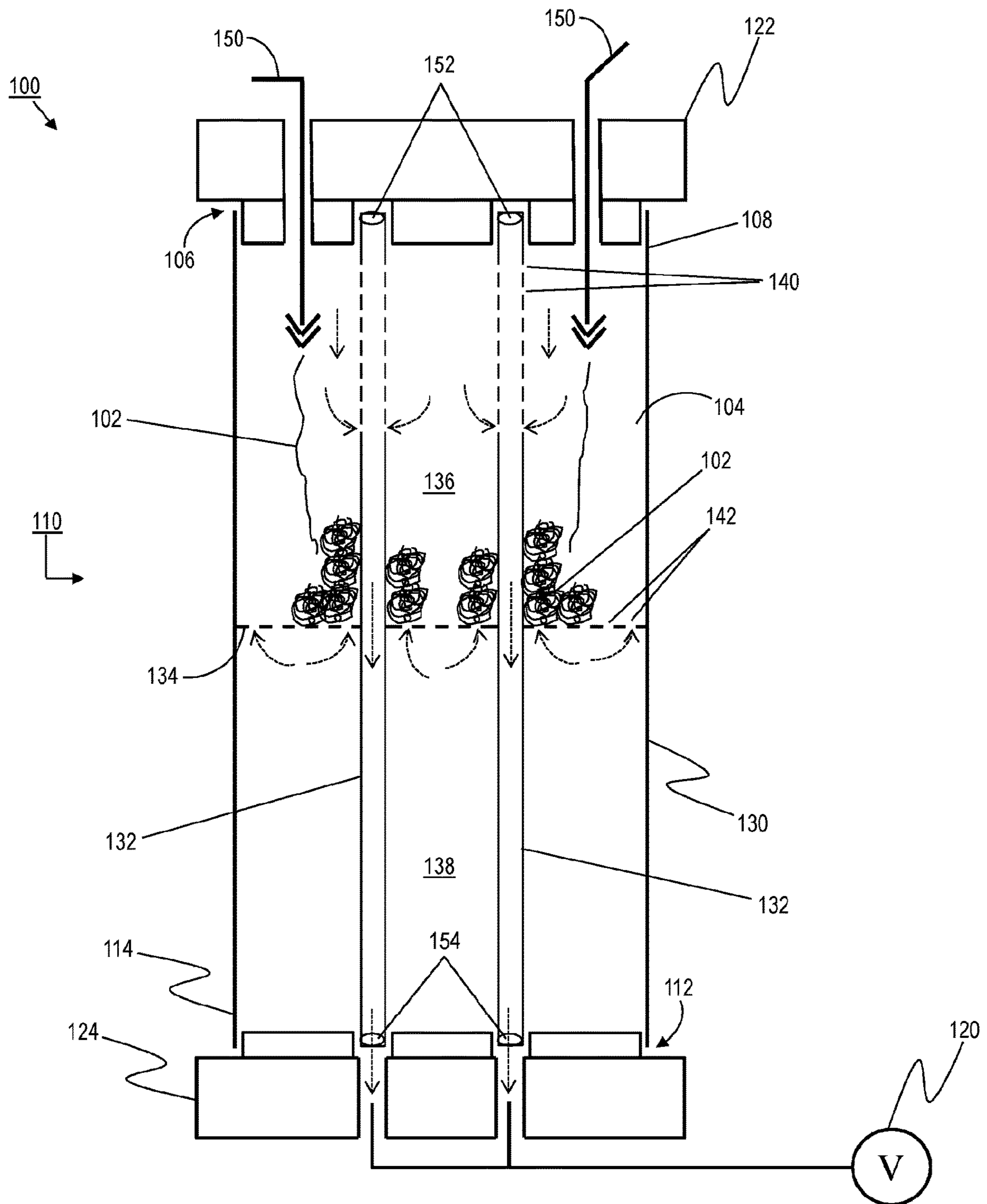
FIG. 1 PRIOR ART
