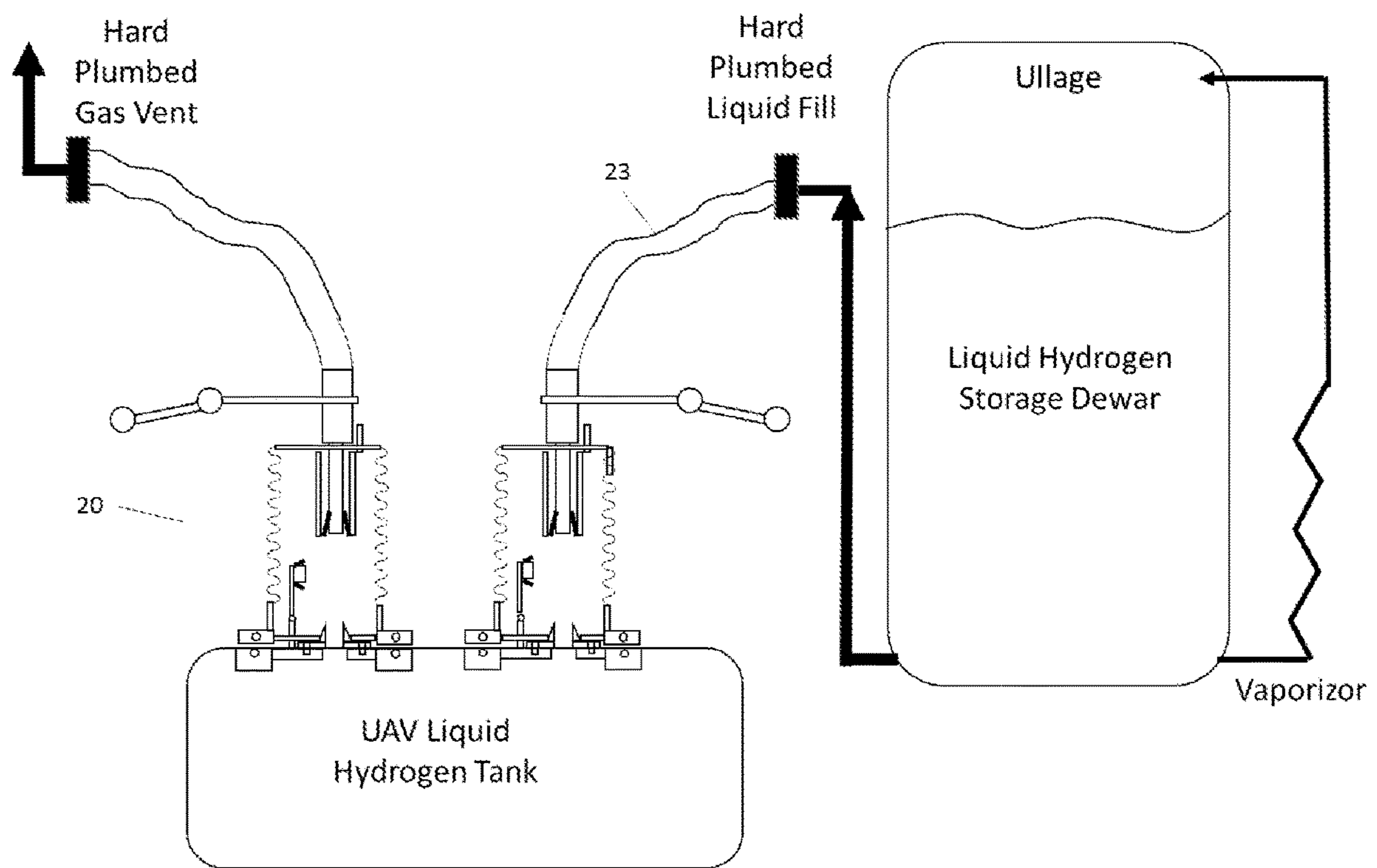
Cap Lifted Figure 11C
