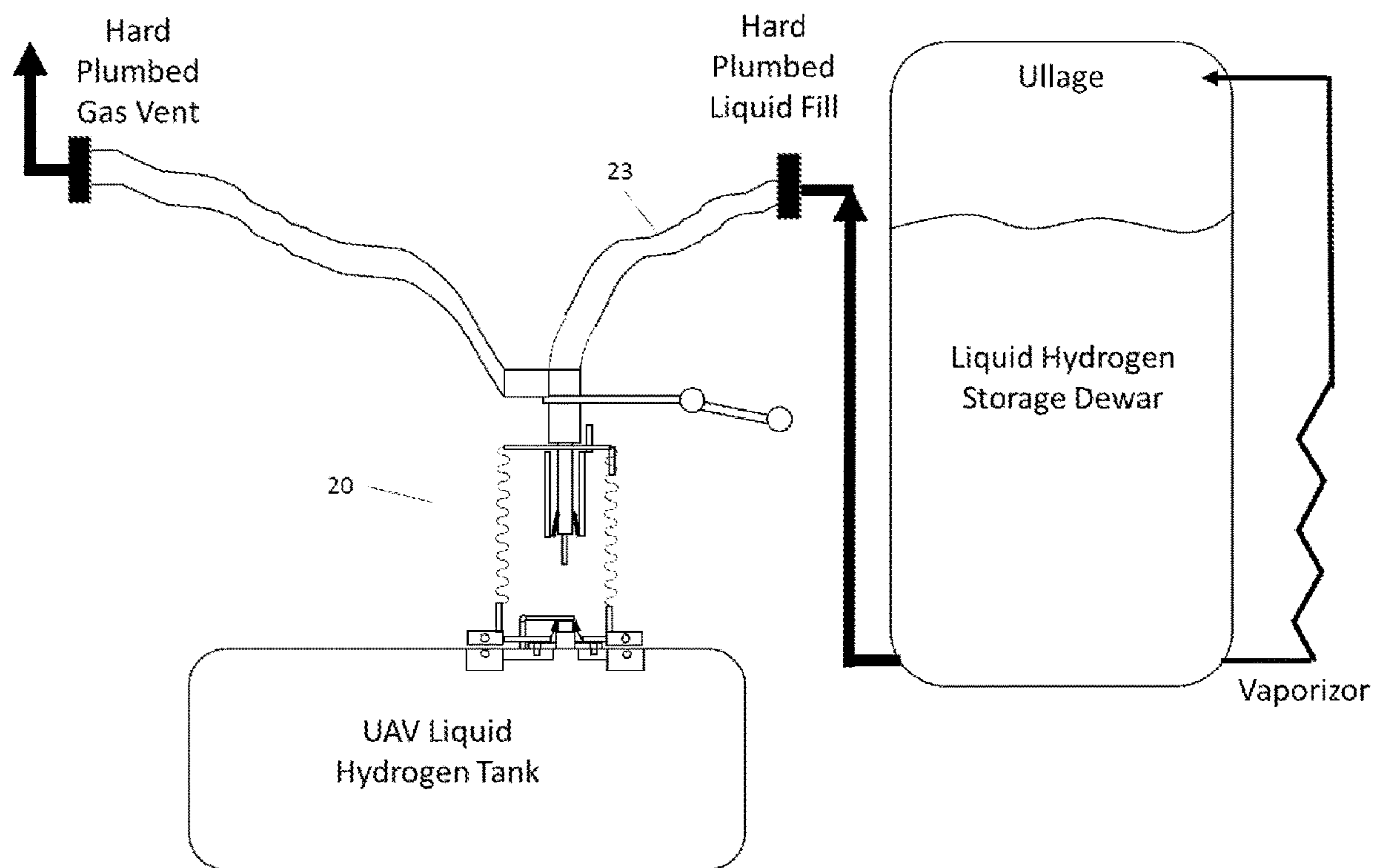
Nozzle Assembly Connected to Tank Flange
