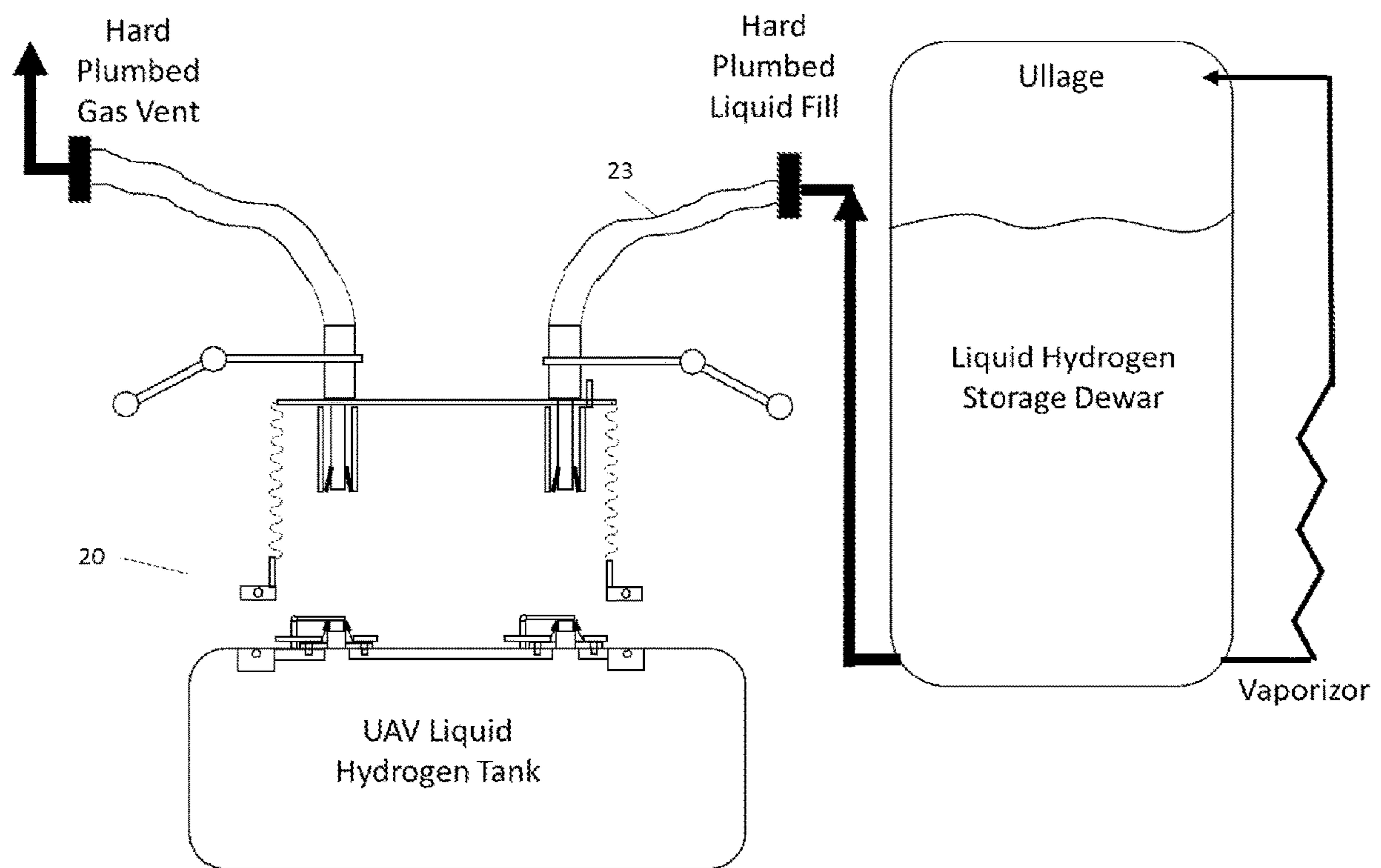
Nozzel Assembly Disconnected from Tank Flange Figure 12A
