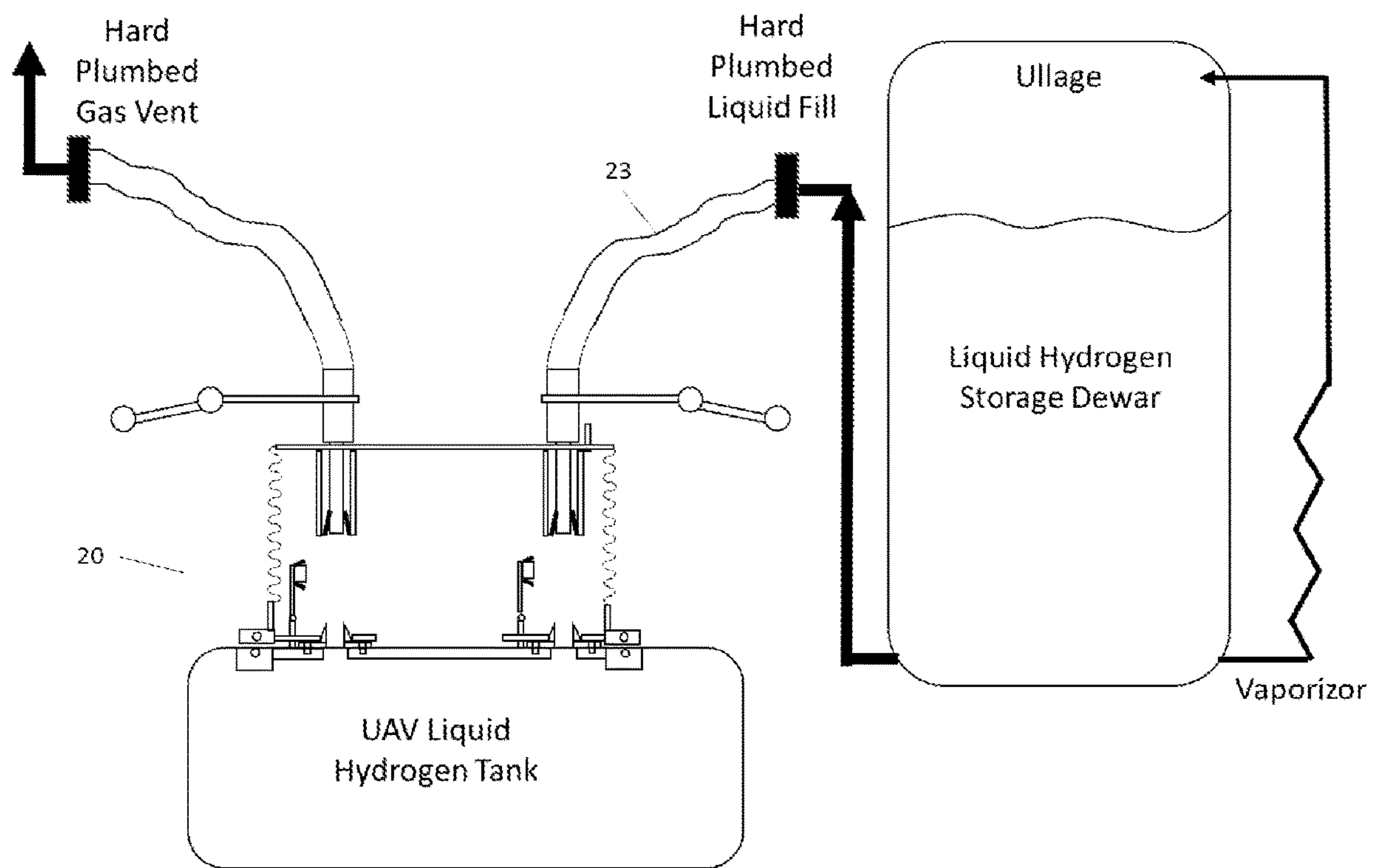
Cap Lifted Figure 12C
