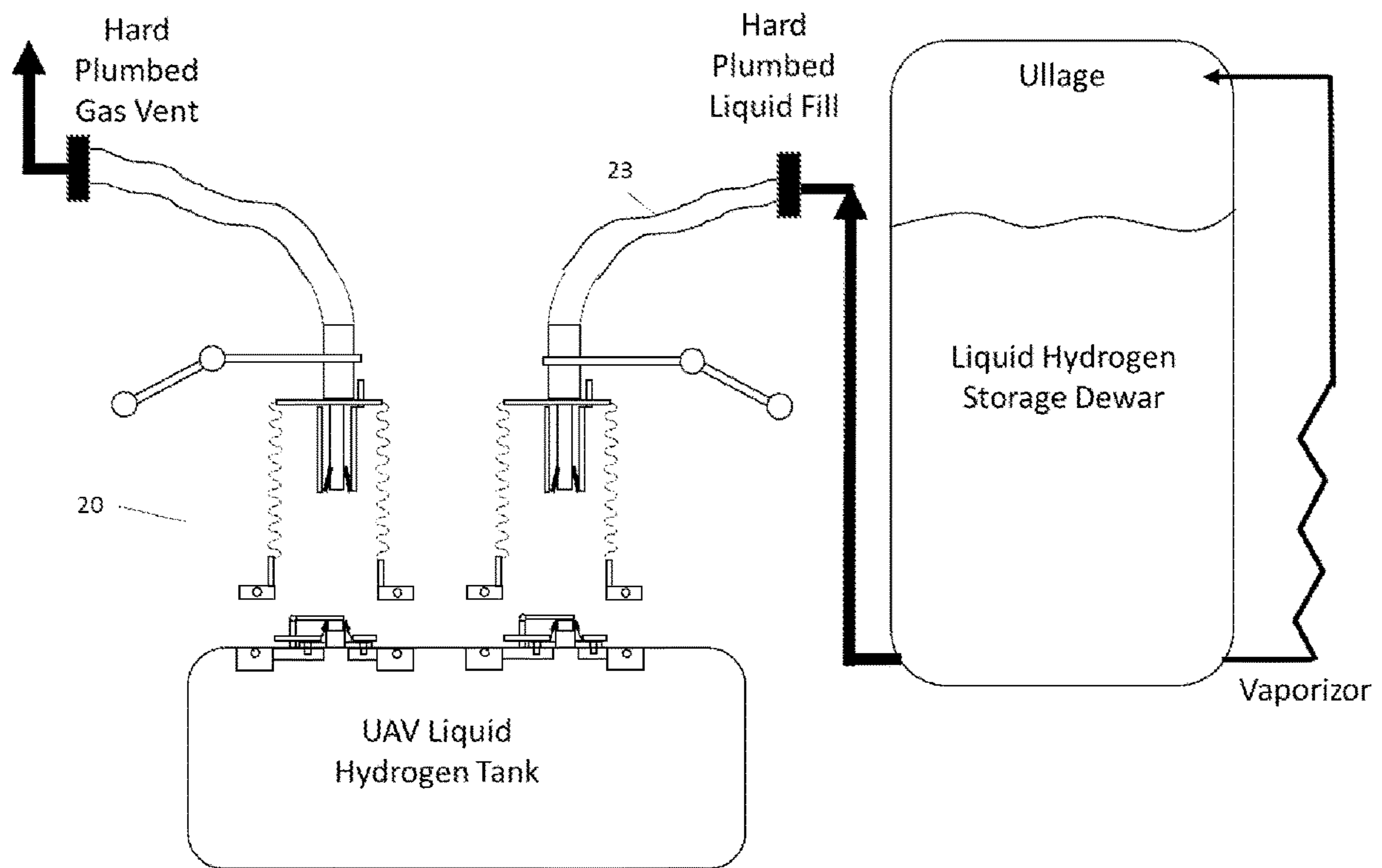
Nozzel Assemby Disconnected from Tank Flange Figure 11A
