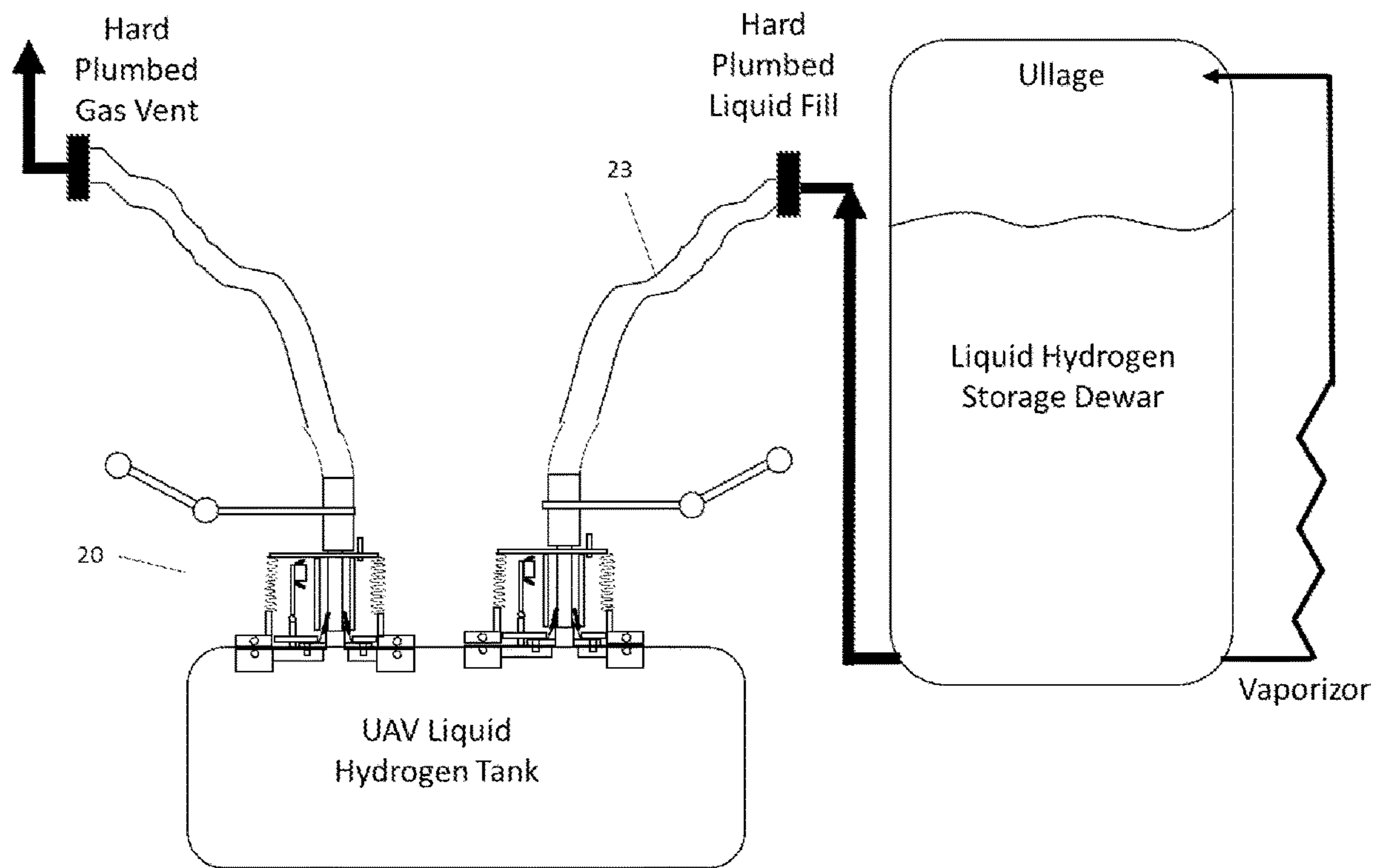
Nozzles Inserted into Tank Figure 11D
