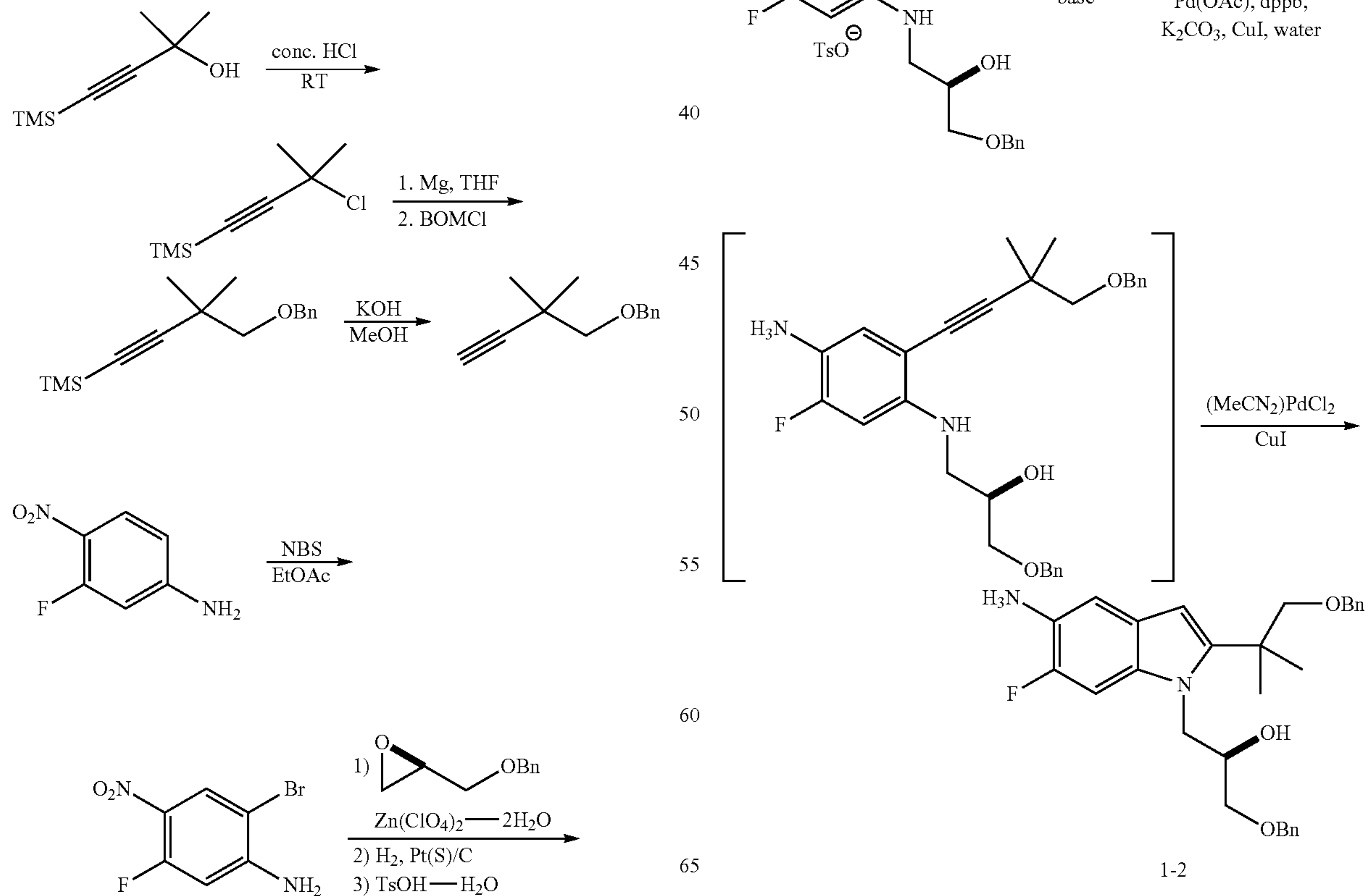
Scheme 3: Preparation of Compound 1-2.
