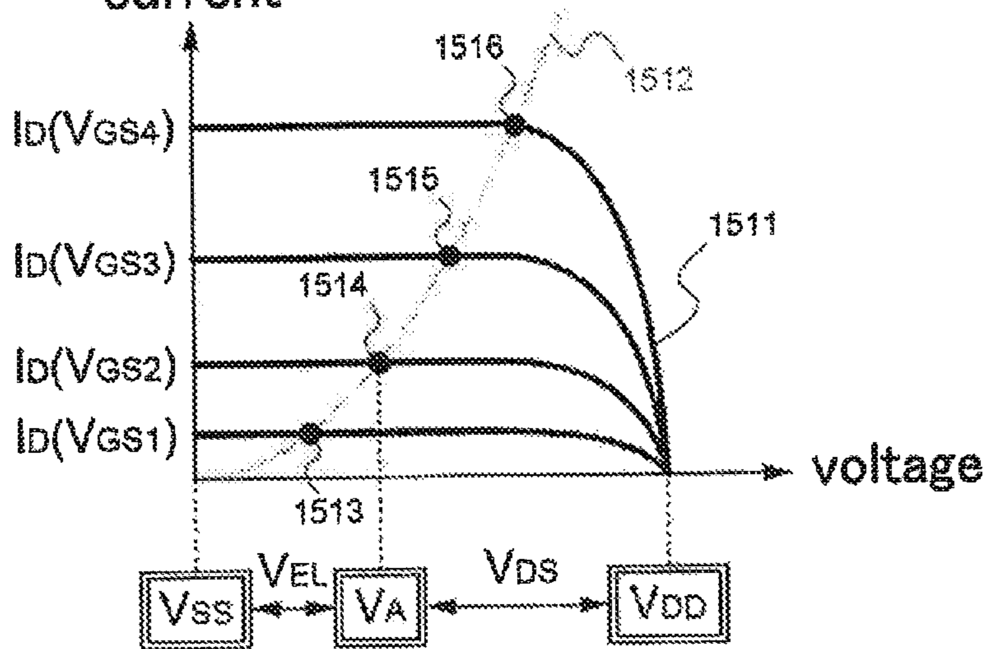
Fig. 15B Prior Art current
