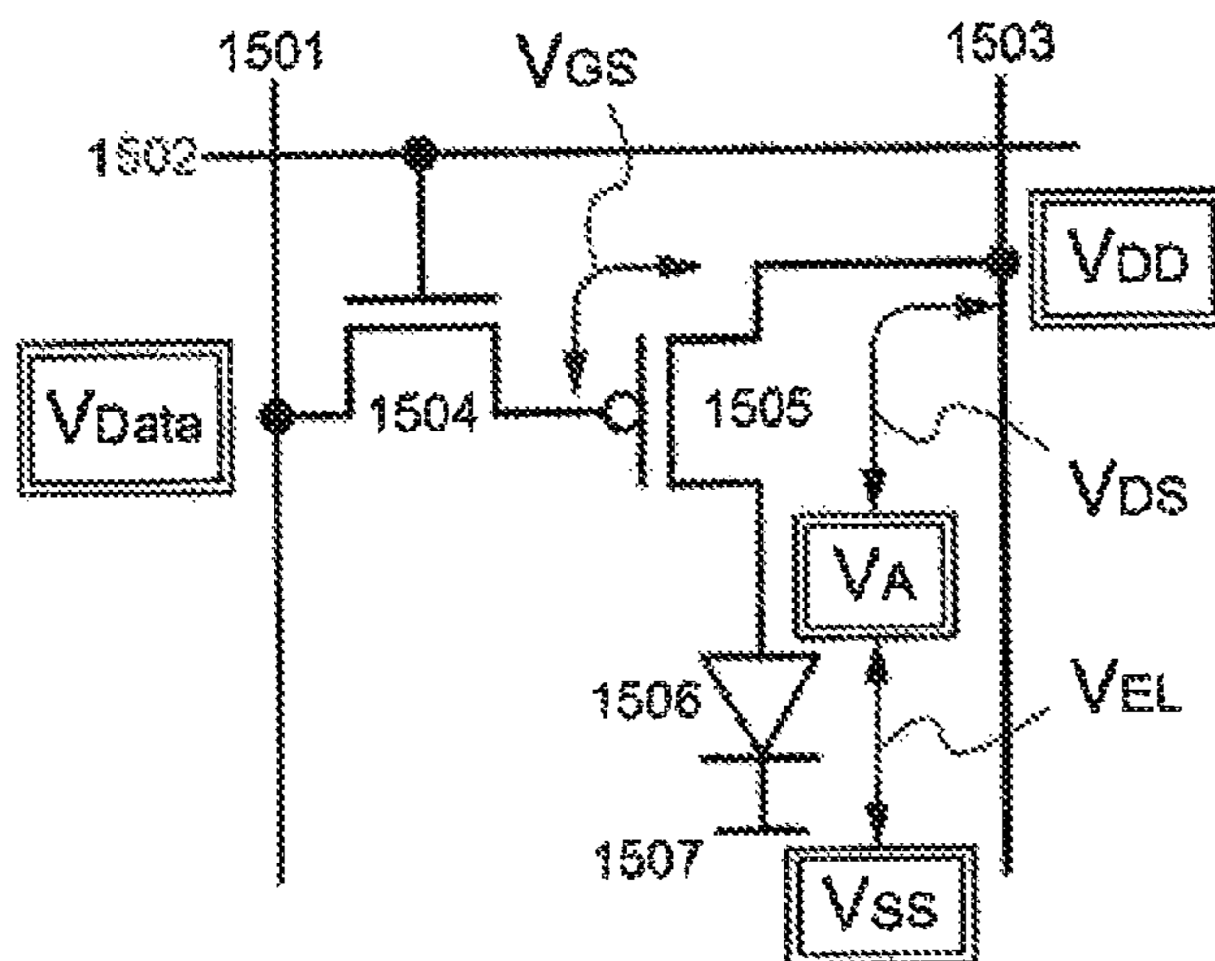
Fig. 15B Prior Art current
