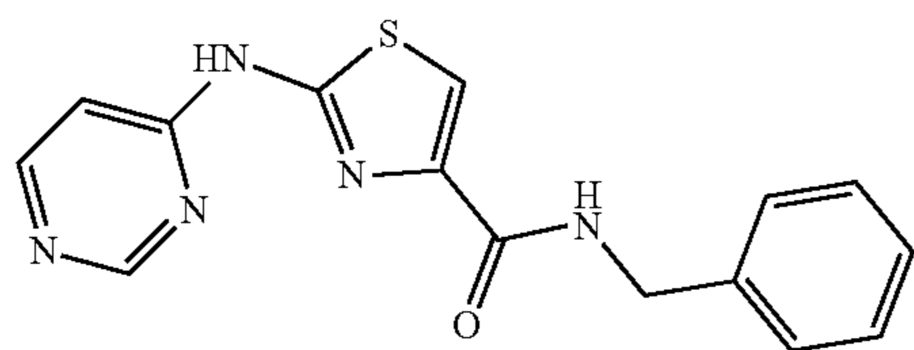
N-Benzyl-2-(pyrimidin-4-ylamino)thiazole-4-carboxamide
