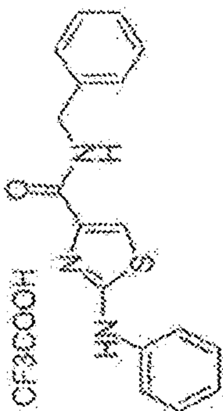
HHS-378-2
