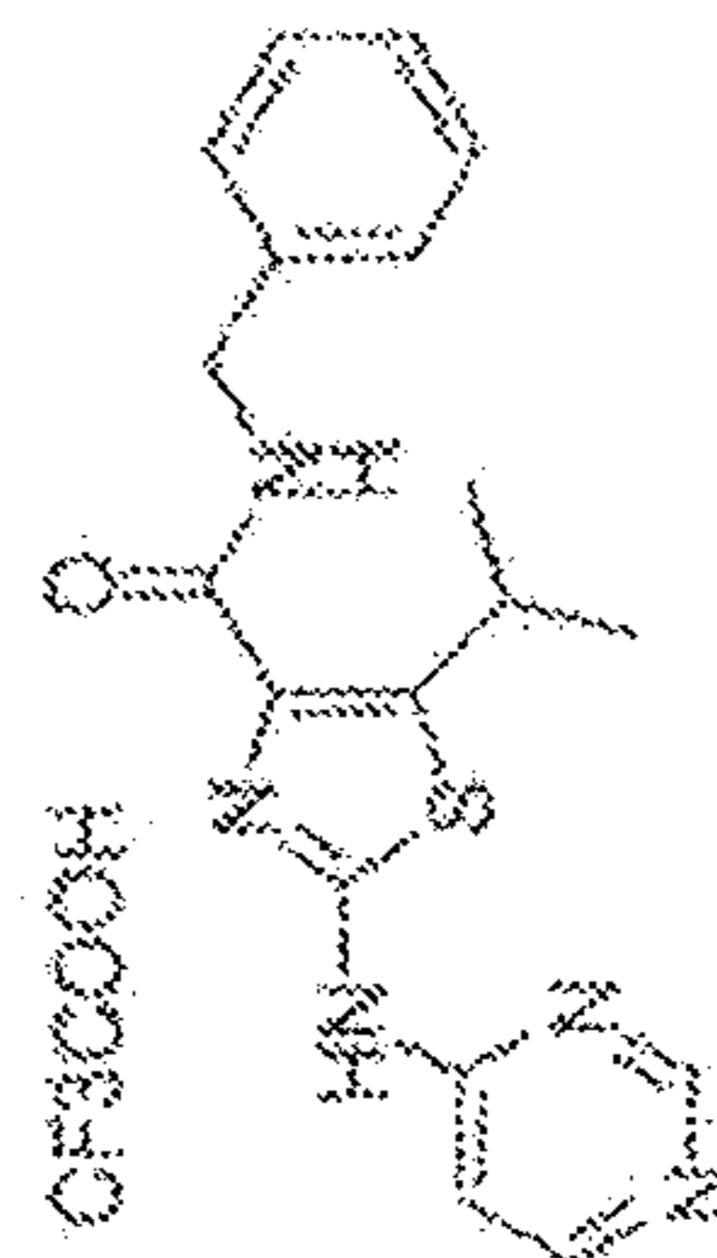
HHS-378-6
