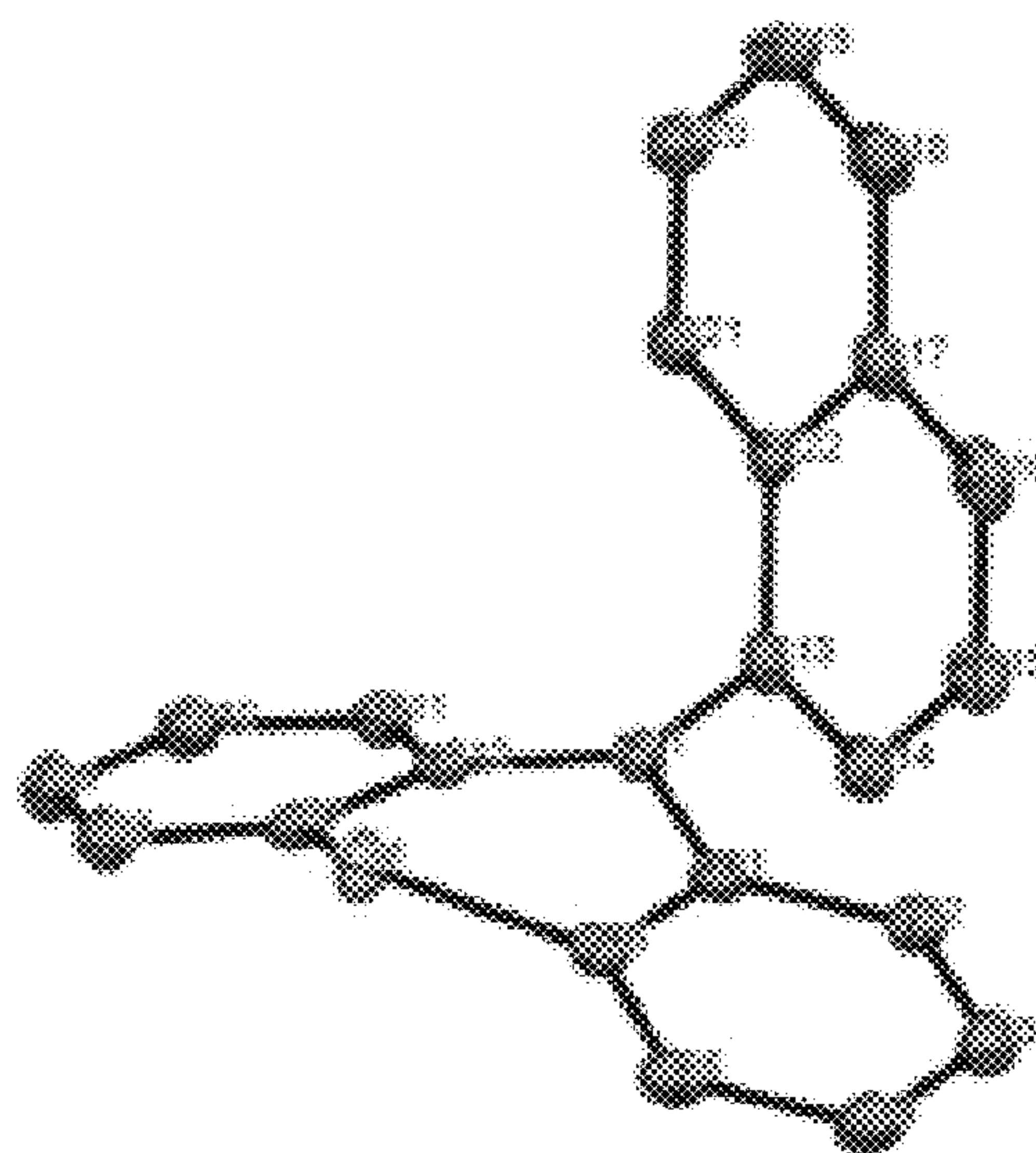
1-naphthalene-10-phenothiazine
