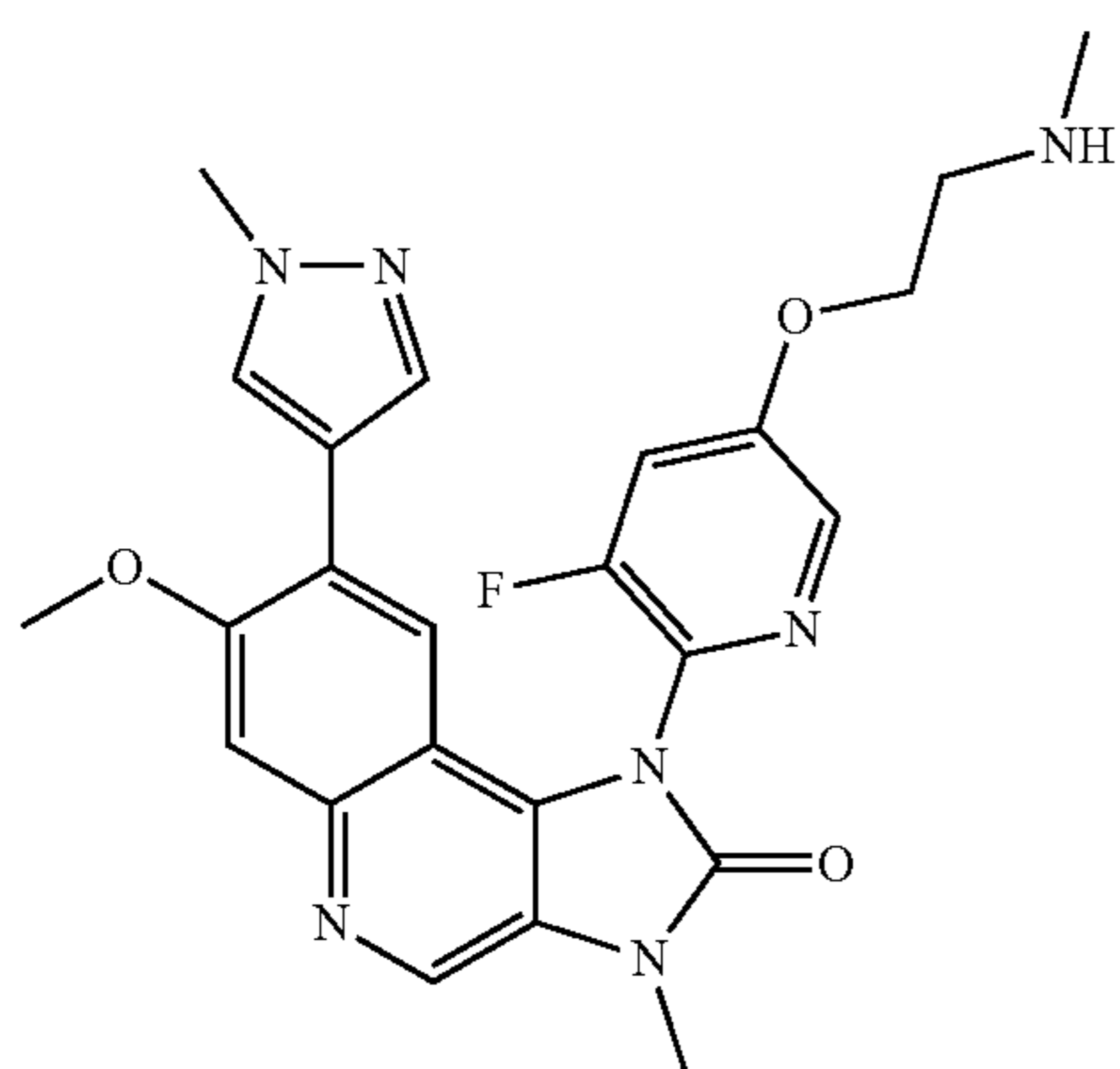
1-[3-Fluoro-5-(2-methylaminoethoxy)-pyridin-2-yl]-7-methoxy-3-methyl-8-(1-methyl-1H-pyrazol-4-yl)-1,3-dihydroimidazo[4,5-c]quinolin-2-one
