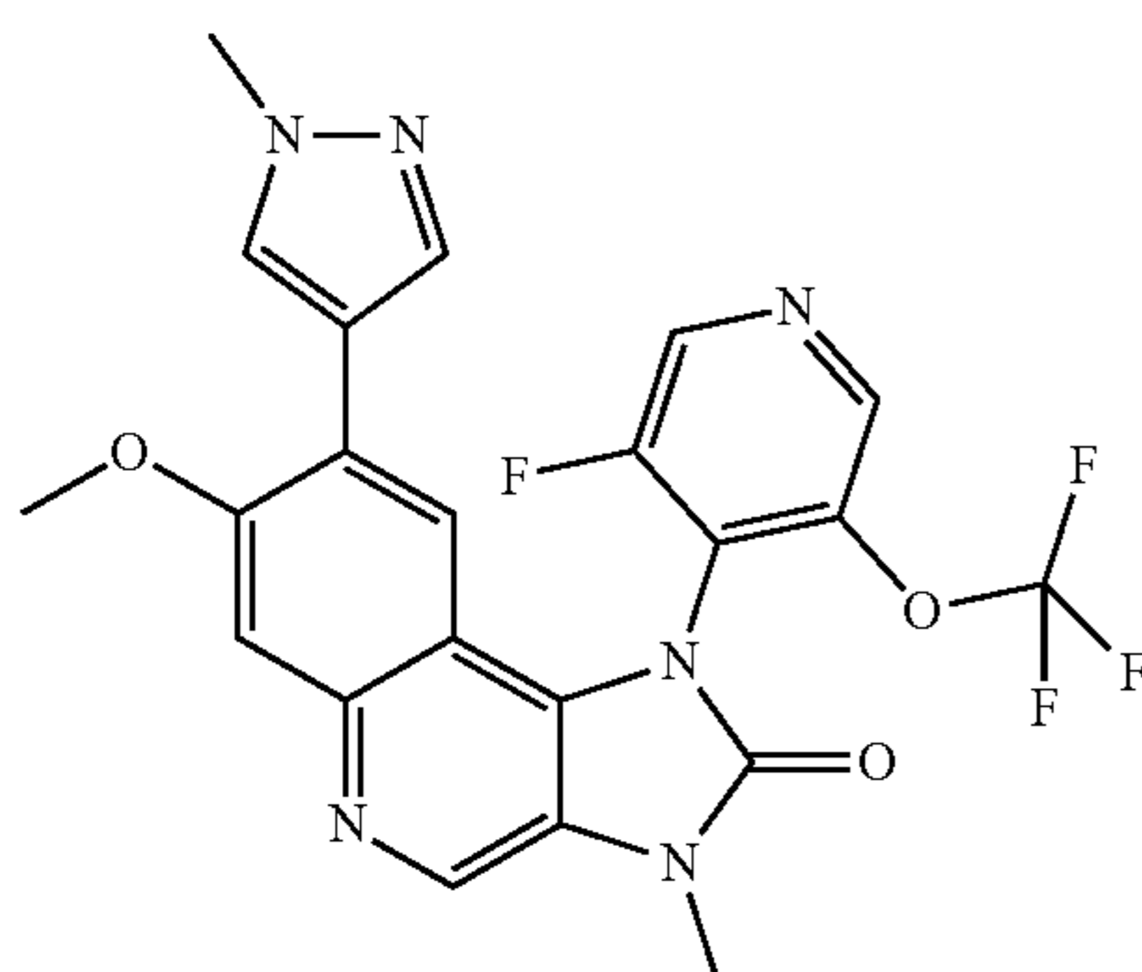
1-[3-Fluoro-5-(trifluoromethoxy)-4-pyridyl]-7-methoxy-3-methyl-8-(1-methyl-1H-pyrazol-4-yl)-1,3-dihydroimidazo[4,5-c]quinolin-2-one
