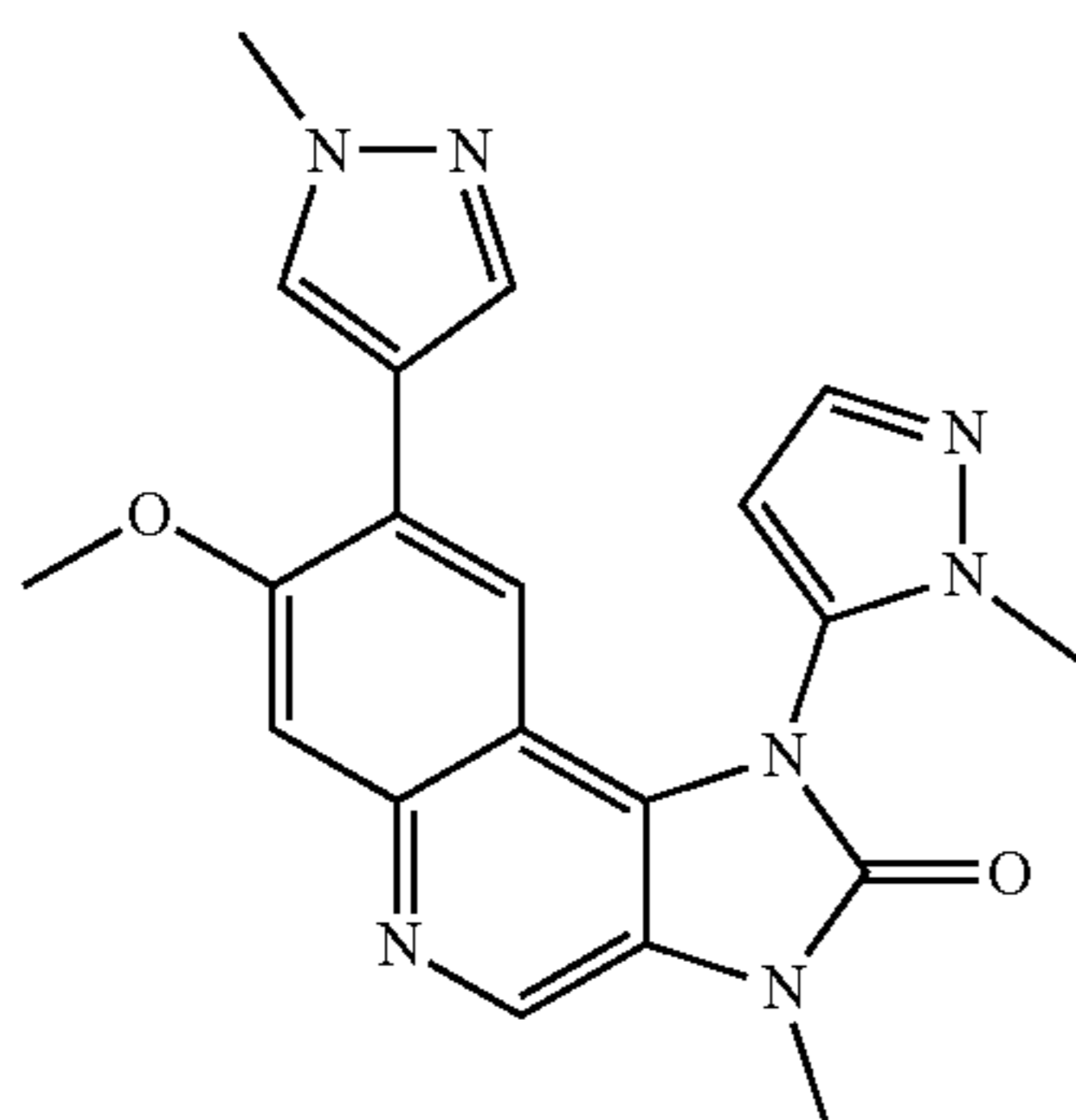
7-Methoxy-3-methyl-1-(2-methyl-2H-pyrazol-3-yl)-8-(1-methyl-1H-pyrazol-4-yl)-1,3-dihydroimidazo[4,5-c]quinolin-2-one
