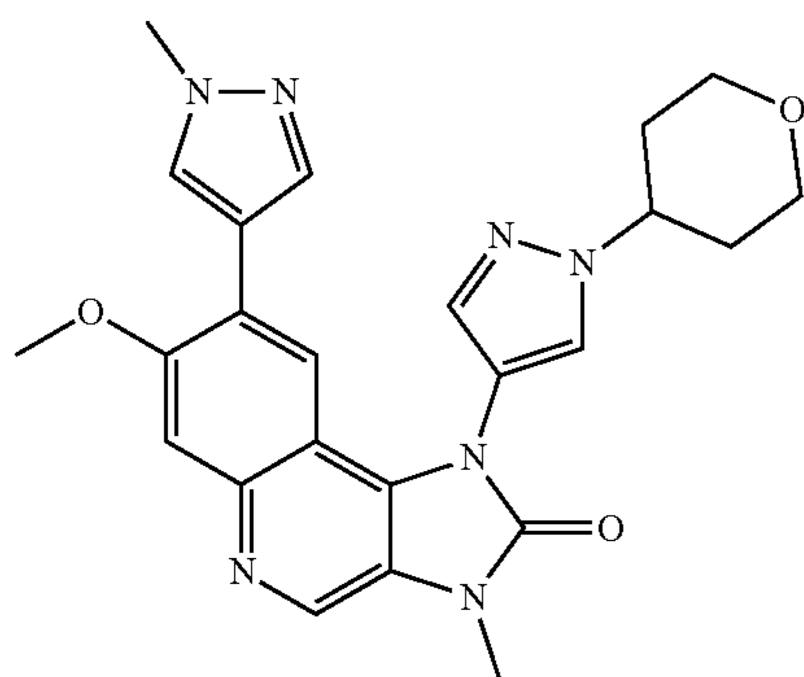
7-Methoxy-3-methyl-8-(1-methyl-1H-pyrazol-4-yl)-1-[1-(tetrahydropyran-4-yl)-1H-pyrazol-4-yl]-1,3-dihydroimidazo[4,5-c]quinolin-2-one
