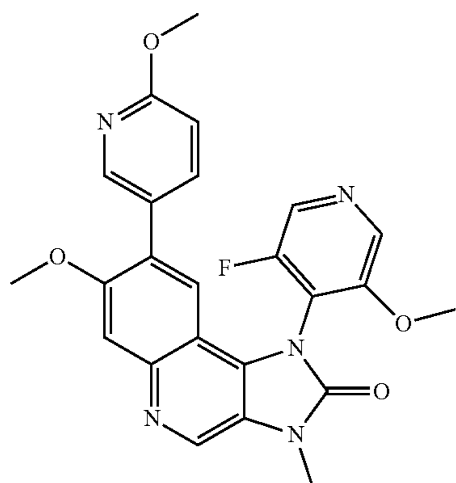
1-(3-Fluoro-5-methoxypyridin-4-yl)-7-methoxy-8-(6-methoxypyridin-3-yl)-3-methyl-1,3-dihydroimidazo[4,5-c]quinolin-2-one
