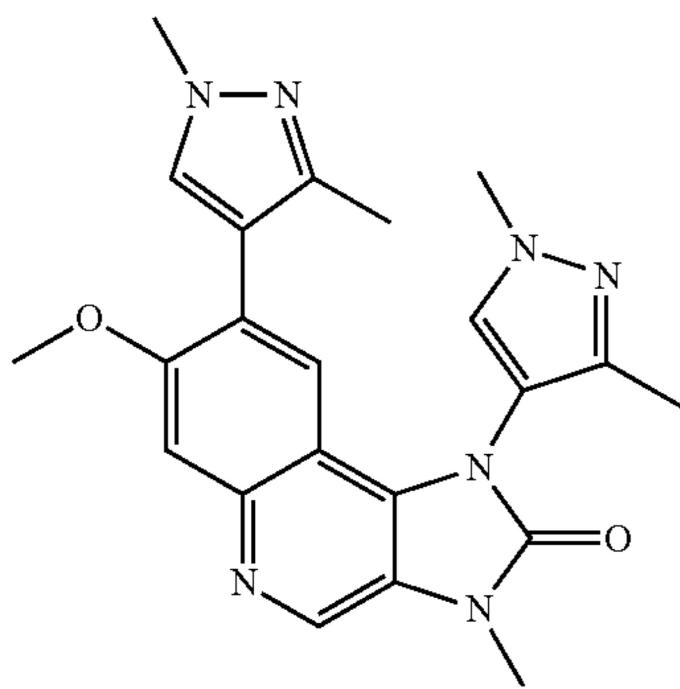
1,8-Bis-(1,3-dimethyl-1H-pyrazol-4-yl)-7-methoxy-3-methyl-1,3-dihydroimidazo[4,5-c]-quinolin-2-one
