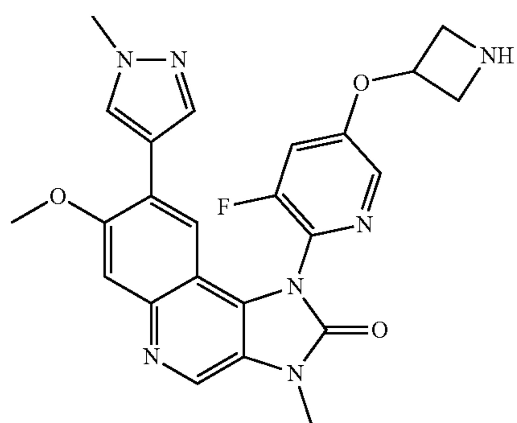
1-[5-(Azetidin-3-yloxy)-3-fluoropyridin-2-yl]-7-methoxy-3-methyl-8-(1-methyl-1H-pyrazol-4-yl)-1,3-dihydroimidazo[4,5-c]quinolin-2-one
