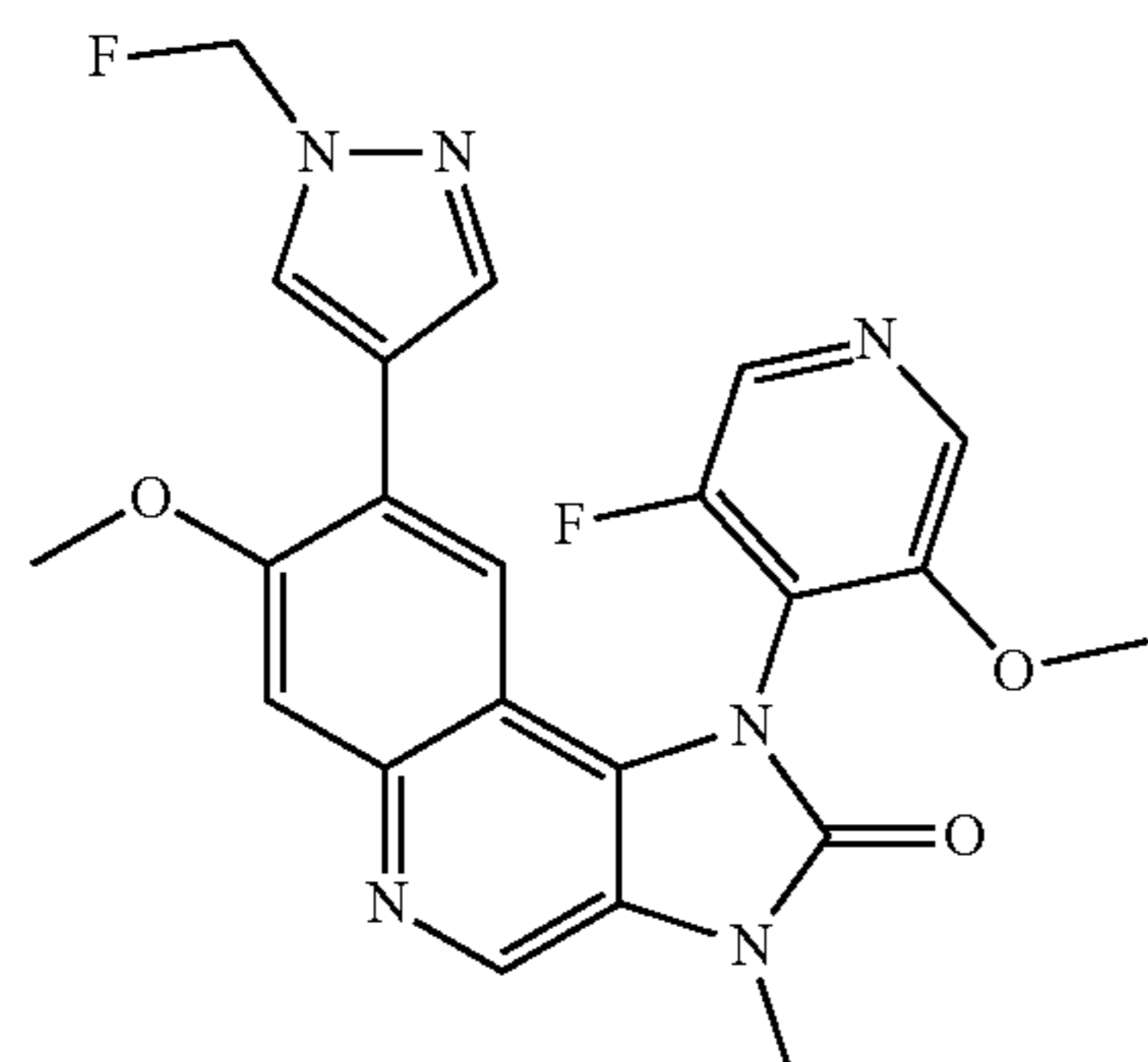
1-(3-Fluoro-5-methoxypyridin-4-yl)-8-(1-fluoromethyl-1H-pyrazol-4-yl)-7-methoxy-3-methyl-1,3-dihydroimidazo[4,5-c]quinolin-2-one
