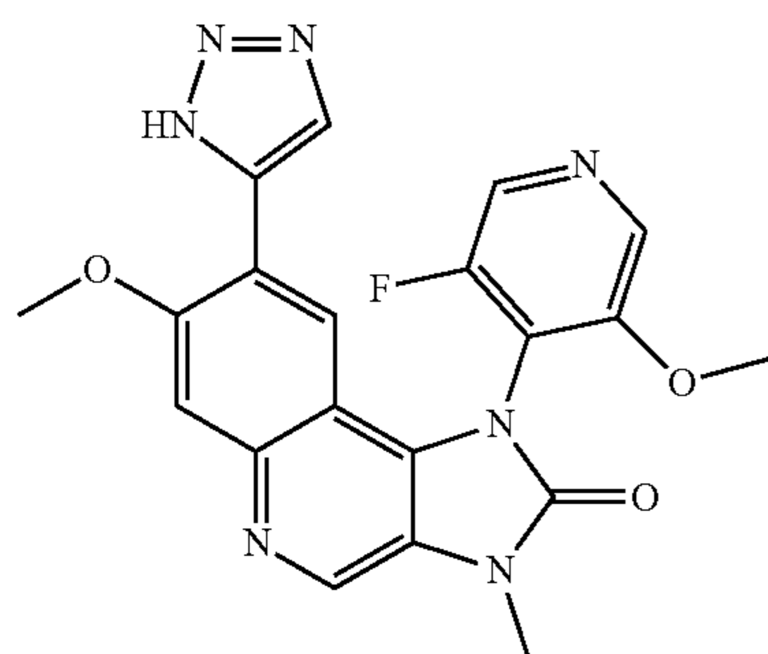
1-(3-Fluoro-5-methoxypyridin-4-yl)-7-methoxy-3-methyl-8-(3H-1,2,3-triazol-4-yl)-1,3-dihydroimidazo[4,5-c]quinolin-2-one
