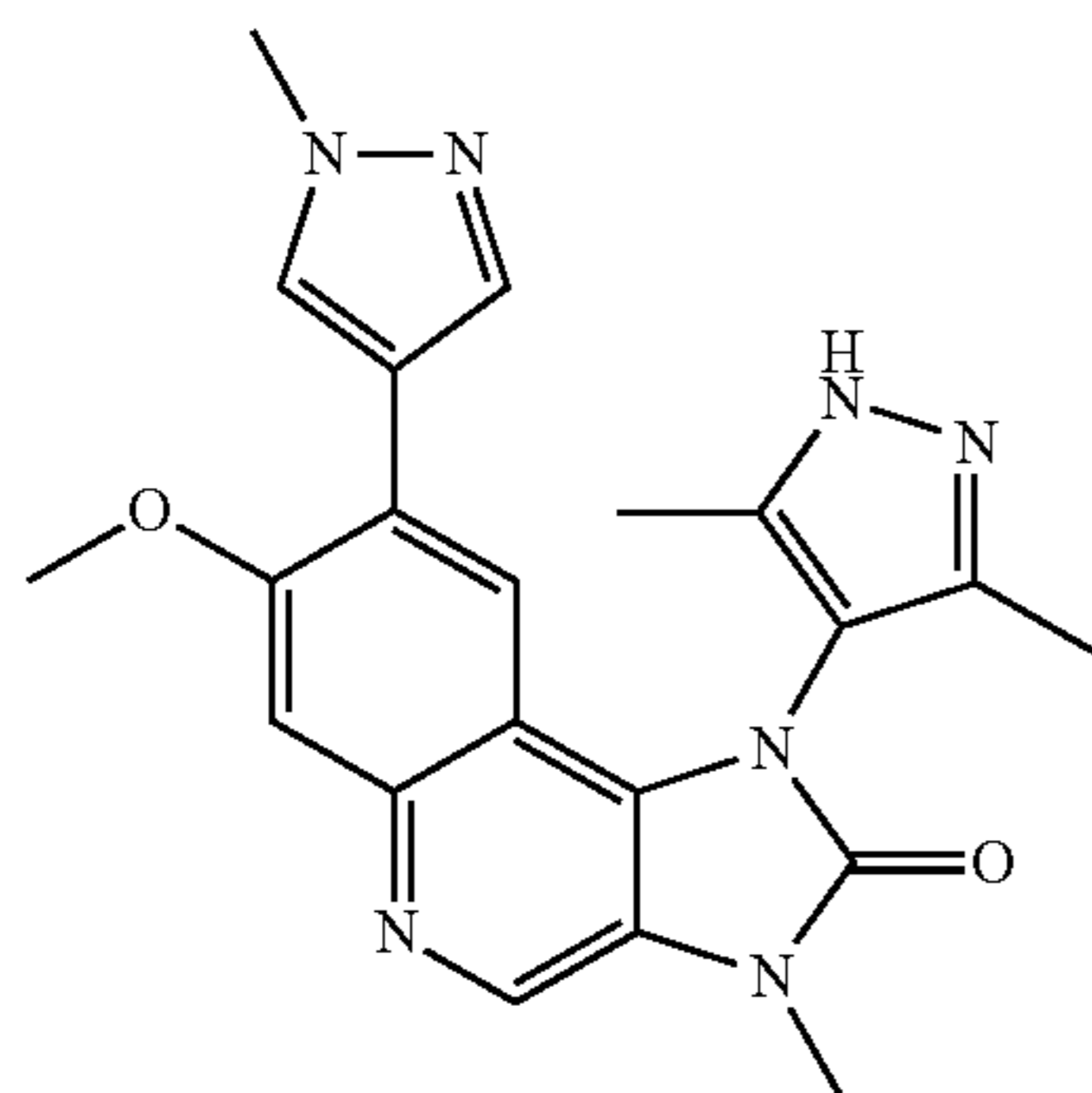
1-(3,5-Dimethyl-1H-pyrazol-4-yl)-7-methoxy-3-methyl-8-(1-methyl-1H-pyrazol-4-yl)-1,3-dihydroimidazo[4,5-c]quinolin-2-one
