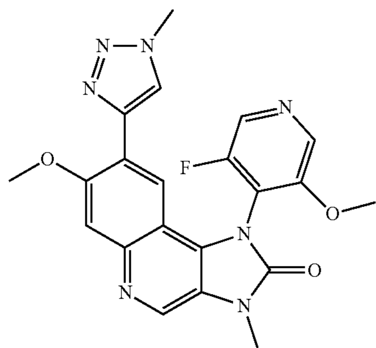
1-(3-Fluoro-5-methoxypyridin-4-yl)-7-methoxy-3-methyl-8-(1-methyl-1H-1,2,3-triazol-4-yl)-1,3-dihydroimidazo[4,5-c]quinolin-2-one
