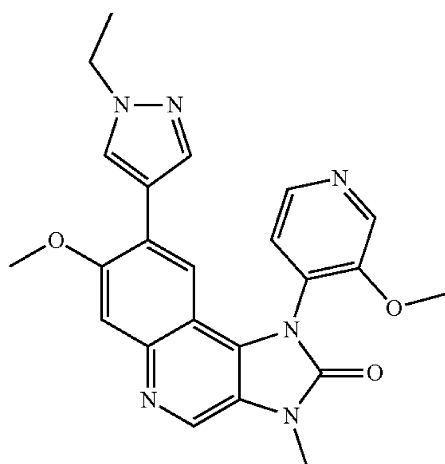
8-(1-Ethyl-1H-pyrazol-4-yl)-7-methoxy-1-(3-methoxypyridin-4-yl)-3-methyl-1,3-dihydroimidazo[4,5-c]quinolin-2-one
