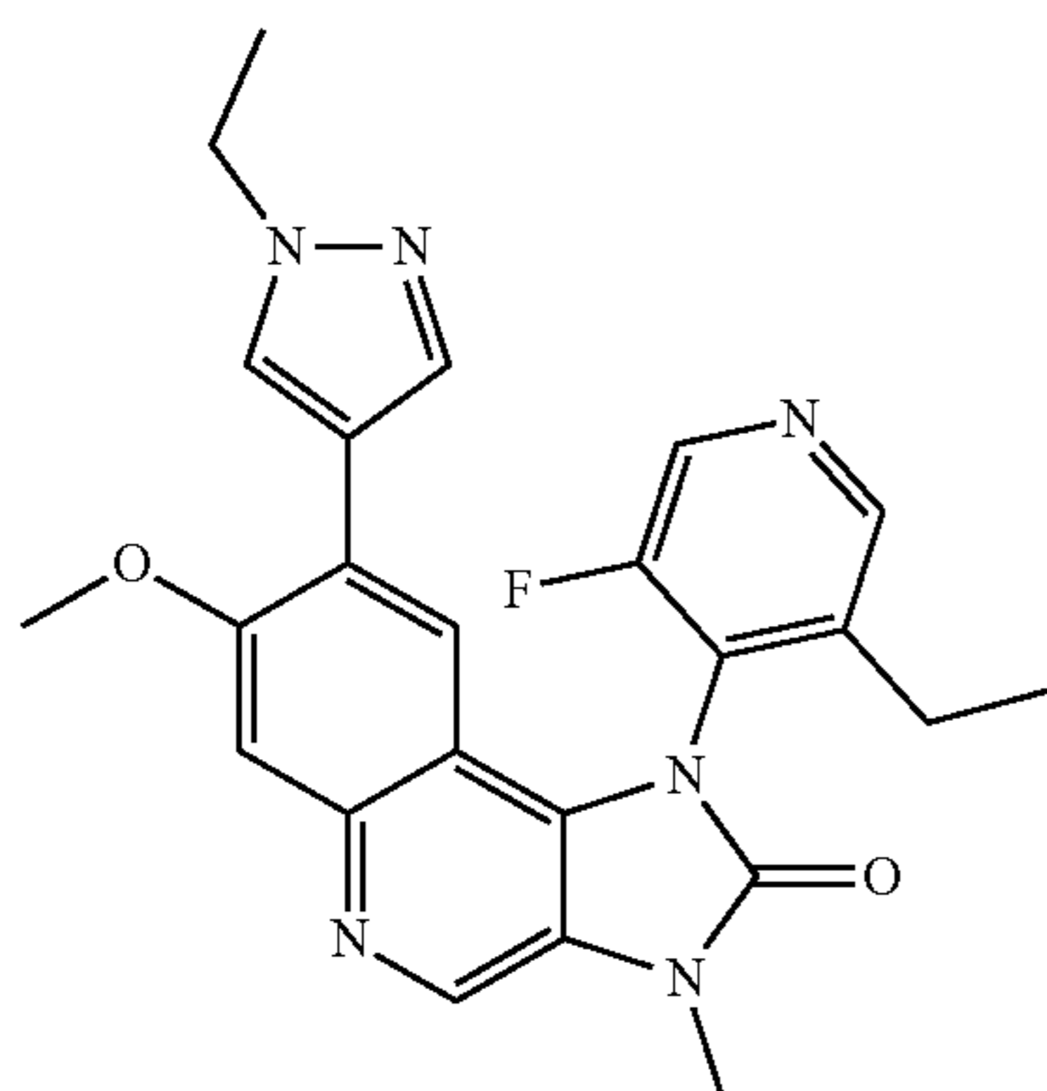
1-(3-Ethyl-5-fluoropyridin-4-yl)-8-(1-ethyl-1H-pyrazol-4-yl)-7-methoxy-3-methyl-1,3-dihydroimidazo[4,5-c]quinolin-2-one
