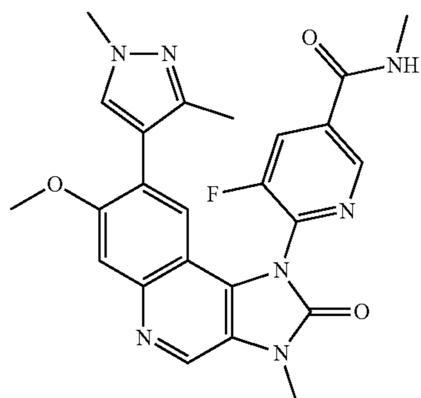
6-[8-(1,3-Dimethyl-1H-pyrazol-4-yl)-7-methoxy-3-methyl-2-oxo-2,3-dihydroimidazo[4,5-c]quinolin-1-yl]-5-fluoro-N-methylnicotinamide
