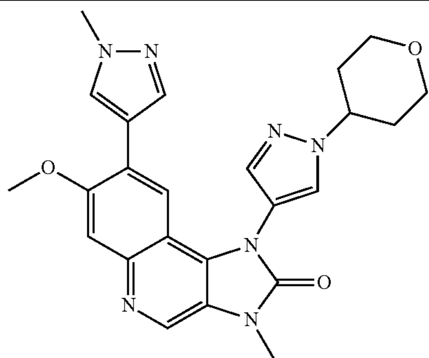
7-Methoxy-3-methyl-8-(1-methyl-1H-pyrazol-4-yl)-1-[1-(tetrahydropyran-4-yl)-1H-pyrazol-4-yl]-1,3-dihydroimidazo[4,5-c]quinolin-2-one
