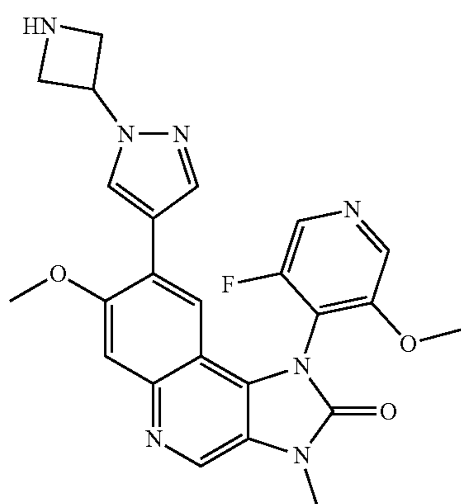
8-[1-(Azetidin-3-yl)-1H-pyrazol-4-yl]-1-(3-fluoro-5-methoxy-pyridin-4-yl)-7-methoxy-3-methyl-1H,2H,3H-imidazo[4,5-c]quinolin-2-one
