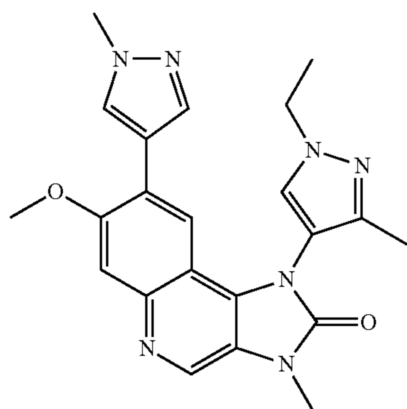
1-(1-Ethyl-3-methyl-1H-pyrazol-4-yl)-7-methoxy-3-methyl-8-(1-methyl-1H-pyrazol-4-yl)-1,3-dihydroimidazo[4,5-c]quinolin-2-one
