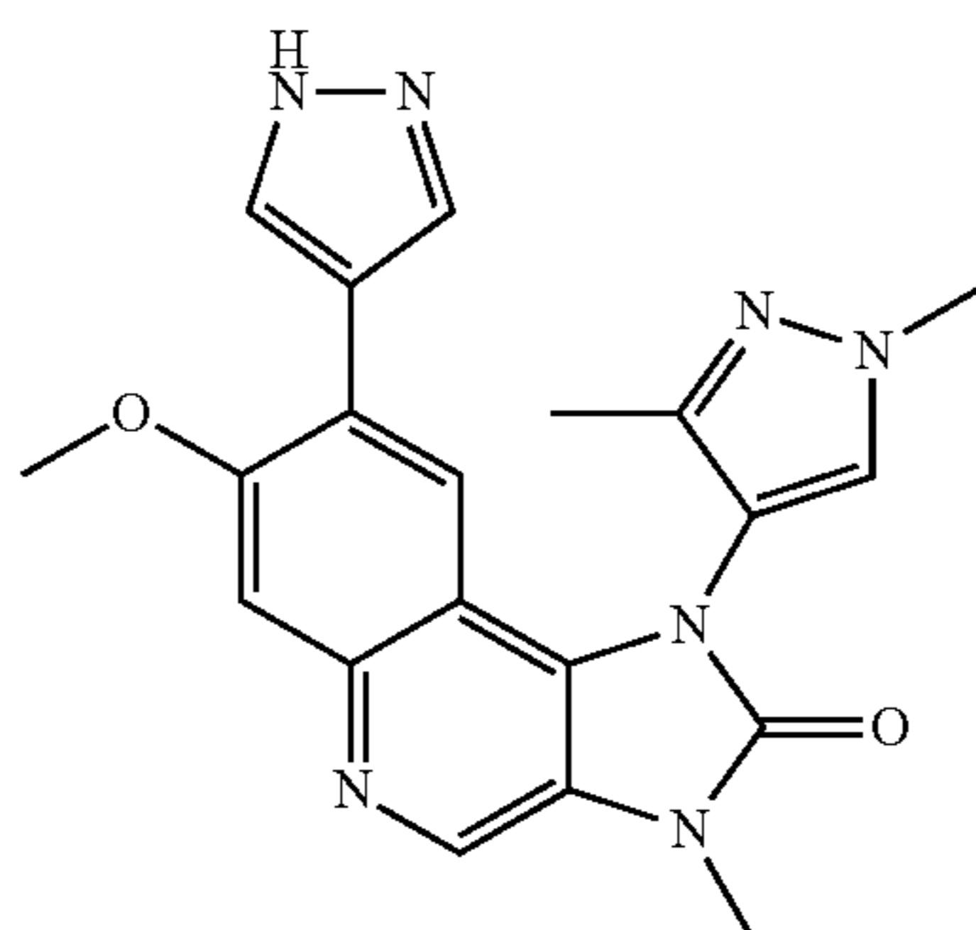
1-(1,3-Dimethyl-1H-pyrazol-4-yl)-7-methoxy-3-methyl-8-(1H-pyrazol-4-yl)-1,3-dihydroimidazo[4,5-c]quinolin-2-one
