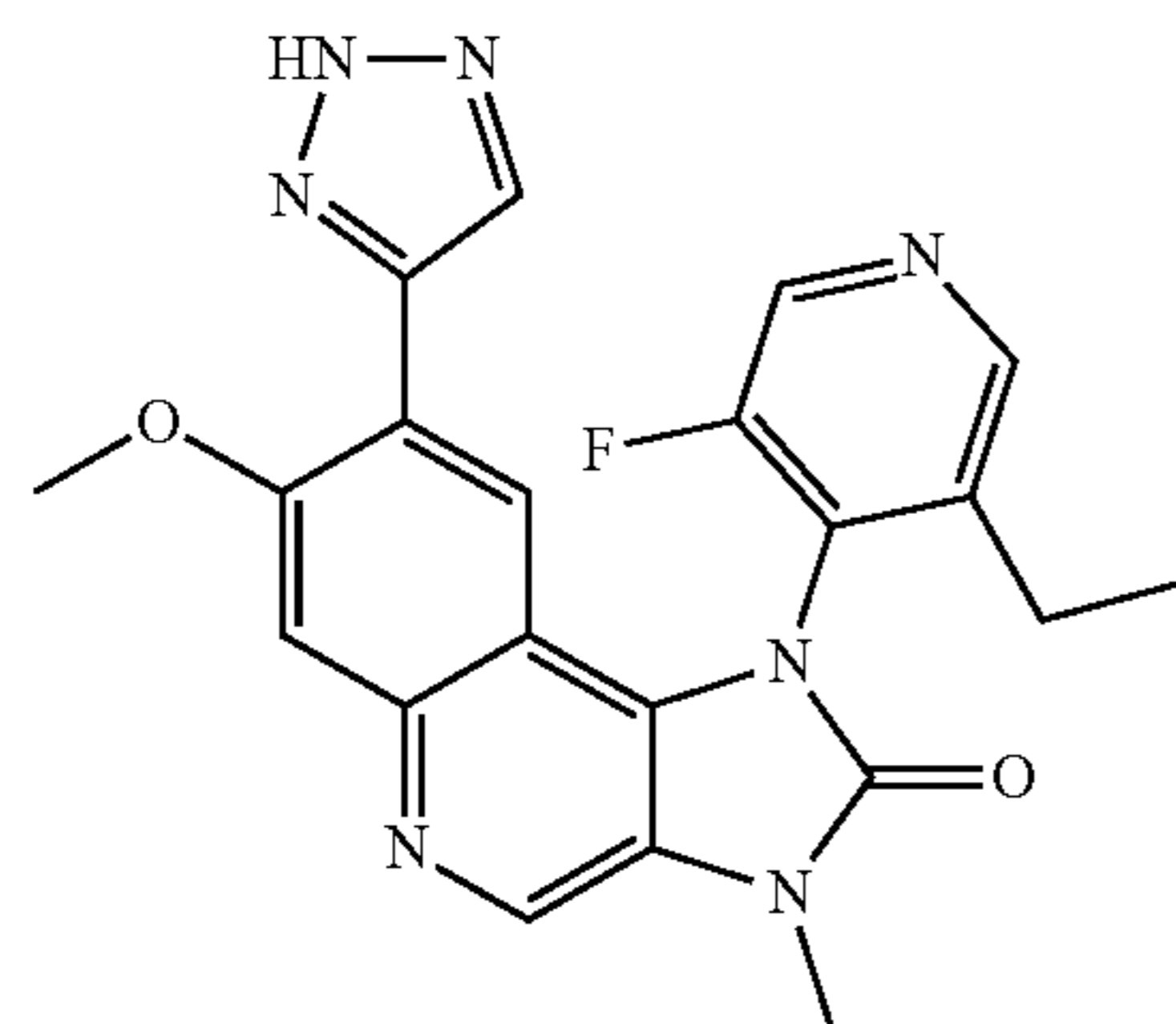
1-(3-Ethyl-5-fluoropyridin-4-yl)-7-methoxy-3-methyl-8-(2H-1,2,3-triazol-4-yl)-1,3-dihydroimidazo[4,5-c] quinolin-2-one
