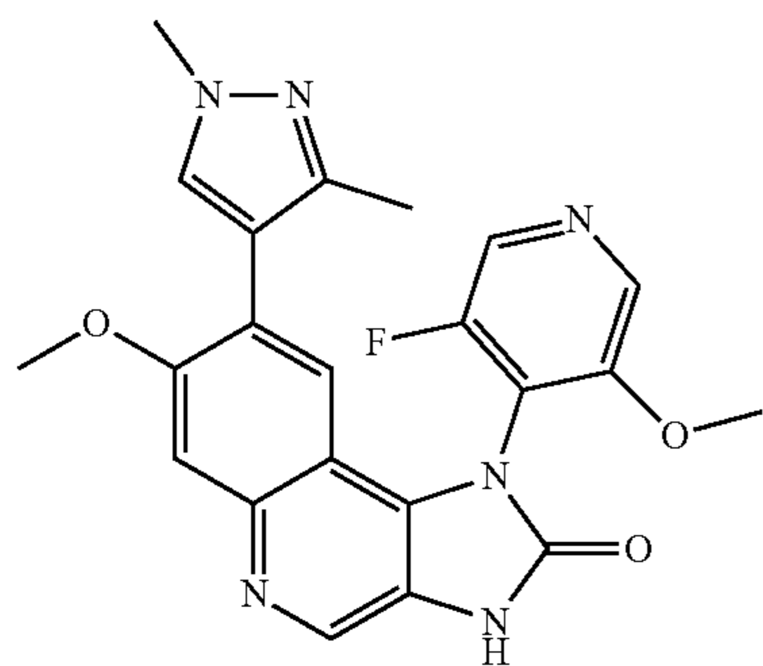
8-(1,3-Dimethyl-1H-pyrazol-4-yl)-1-(3-fluoro-5-methoxy-pyridin-4-yl)-7-methoxy-1,3-dihydroimidazo[4,5-c]quinolin-2-one
