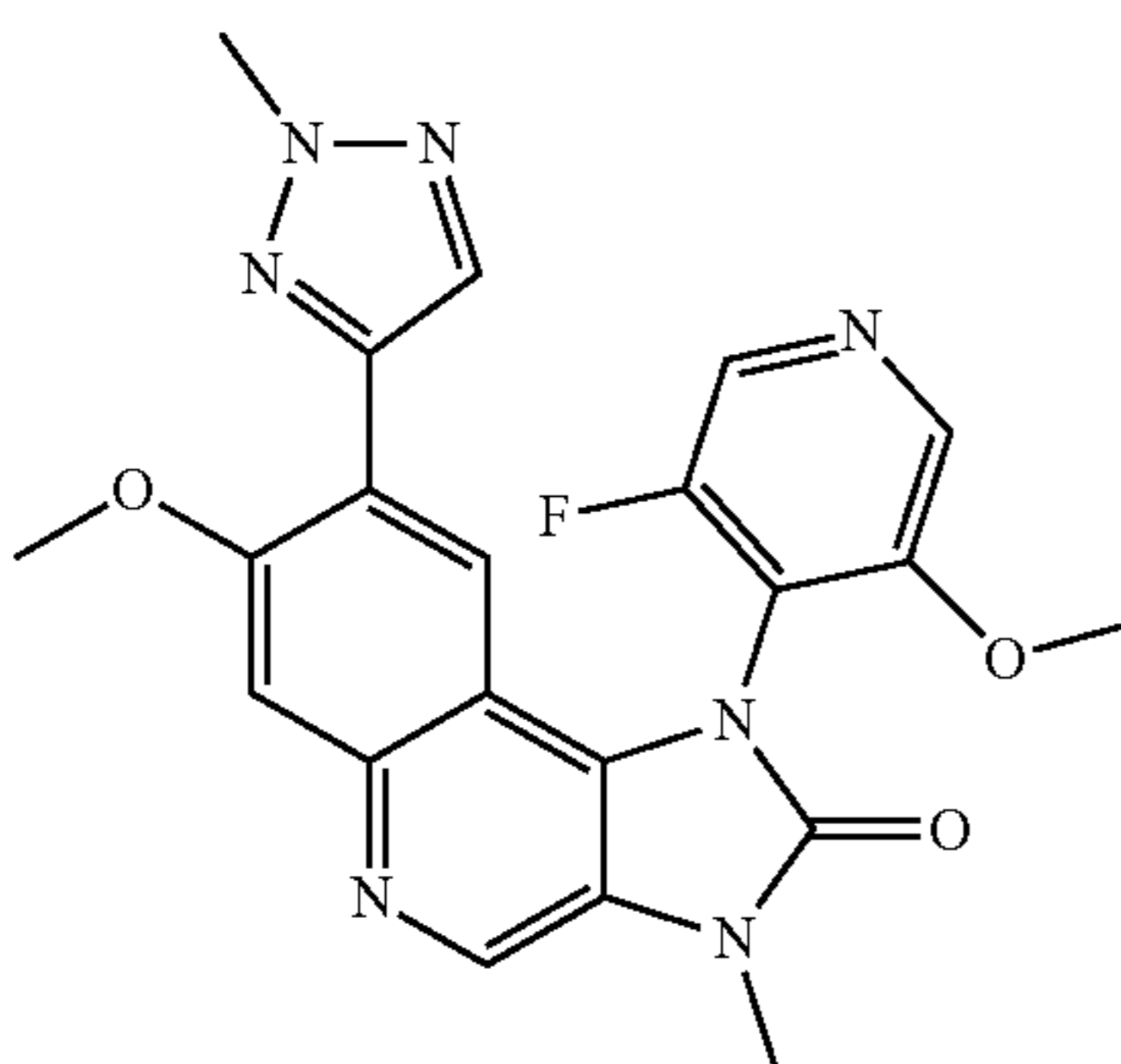
1-(3-Fluoro-5-methoxypyridin-4-yl)-7-methoxy-3-methyl-8-(2-methyl-2H-1,2,3-triazol-4-yl)-1,3-dihydroimidazo[4,5-c] quinolin-2-one
