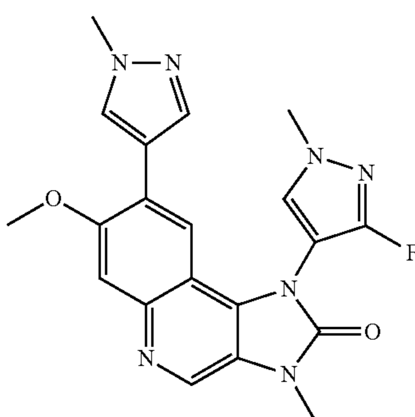
1-(3-Fluoro-1-methyl-1H-pyrazol-4-yl)-7-methoxy-3-methyl-8-(1-methyl-1H-pyrazol-4-yl)-1,3-dihydroimidazo[4,5-c]quinolin-2-one
