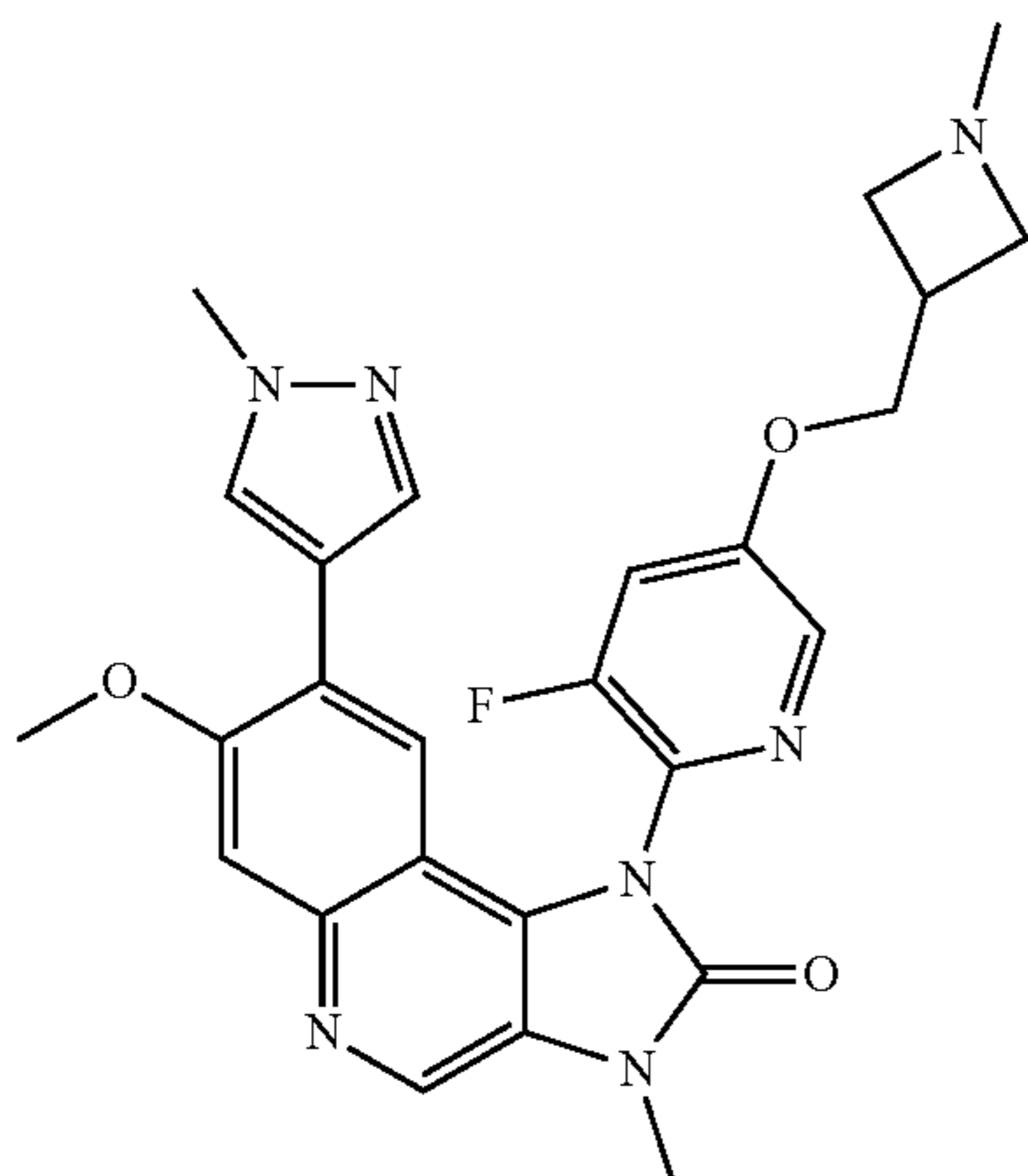
1-[3-Fluoro-5-(1-methylazetidin-3-ylmethoxy)pyridin-2-yl]-7-methoxy-3-methyl-8-(1-methyl-1H-pyrazol-4-yl)-1,3-dihydroimidazo[4,5-c]quinolin-2-one
