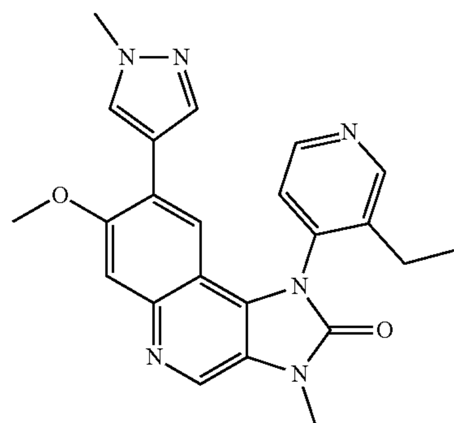
1-(3-Ethylpyridin-4-yl)-7-methoxy-3-methyl-8-(1-methyl-1H-pyrazol-4-yl)-1,3-dihydroimidazo[4,5-c]quinolin-2-one
