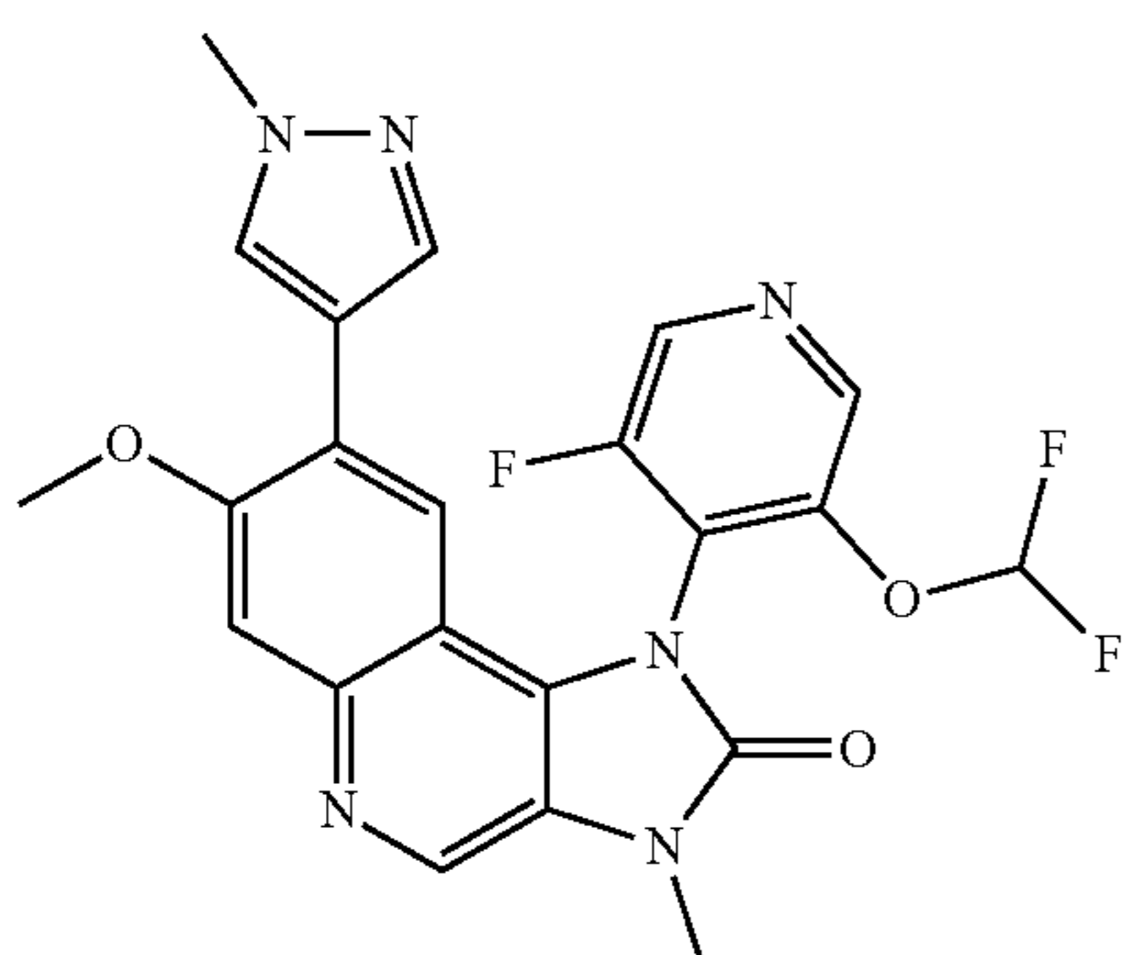
1-(3-Difluoromethoxy-5-fluoropyridin-4-yl)-7-methoxy-3-methyl-8-(1-methyl-1H-pyrazol-4-yl)-1,3-dihydroimidazo[4,5-c]quinolin-2-one
