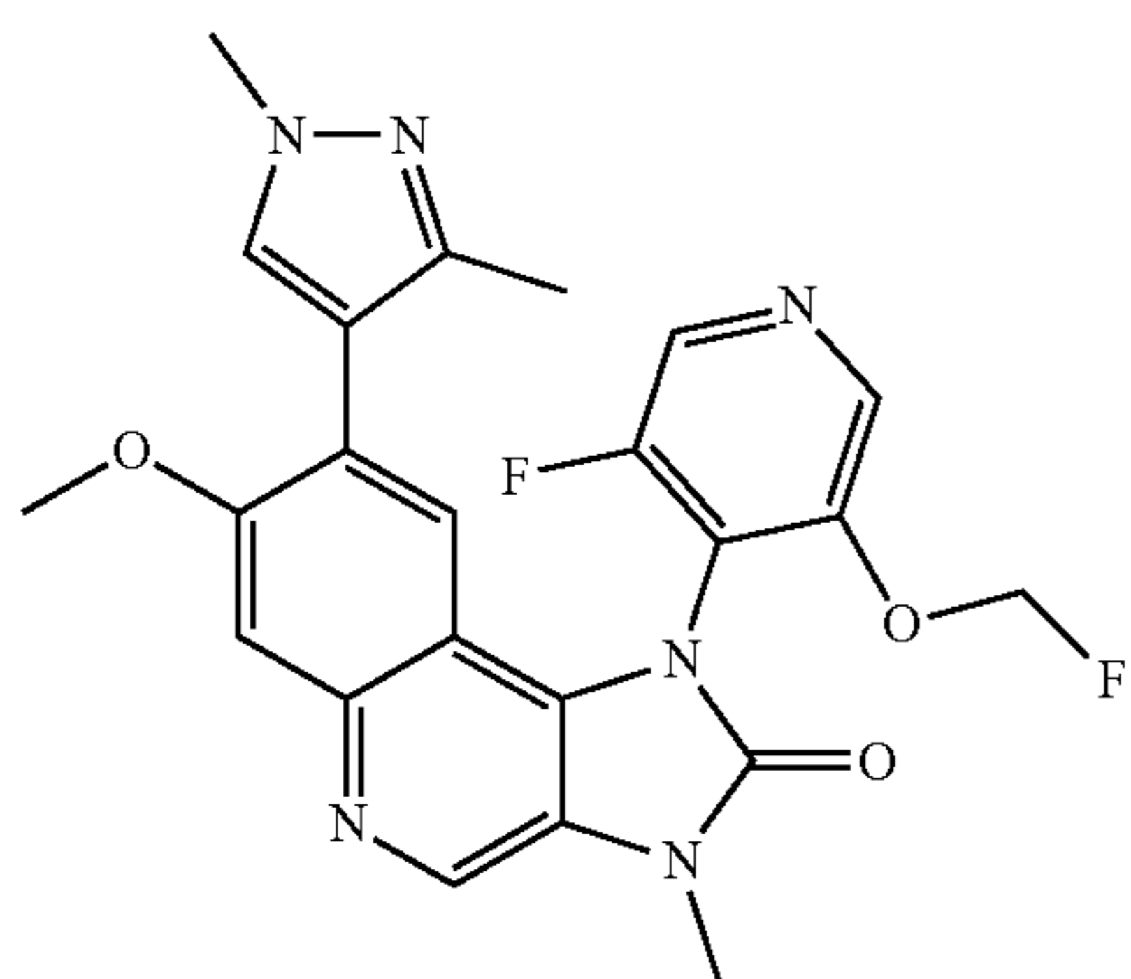
8-(1,3-Dimethyl-1H-pyrazol-4-yl)-1-(3-fluoro-5-fluoromethoxy)pyridin-4-yl)-7-methoxy-3-methyl-1,3-dihydroimidazo[4,5-c]quinolin-2-one
