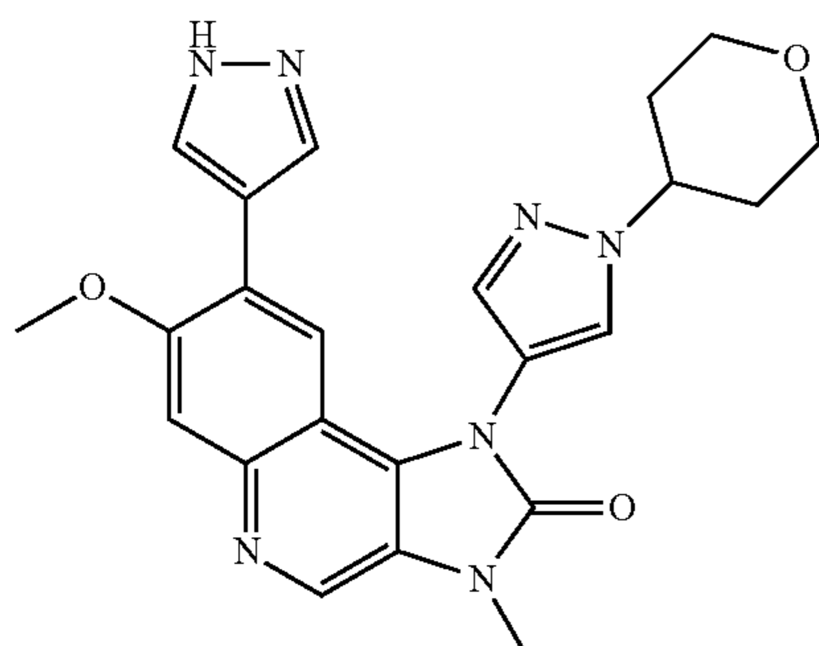
7-Methoxy-3-methyl-8-(1H-pyrazol-4-yl)-1-[1-(tetrahydropyran-4-yl)-1H-pyrazol-4-yl]-1,3-dihydroimidazo[4,5-c]quinolin-2-one
