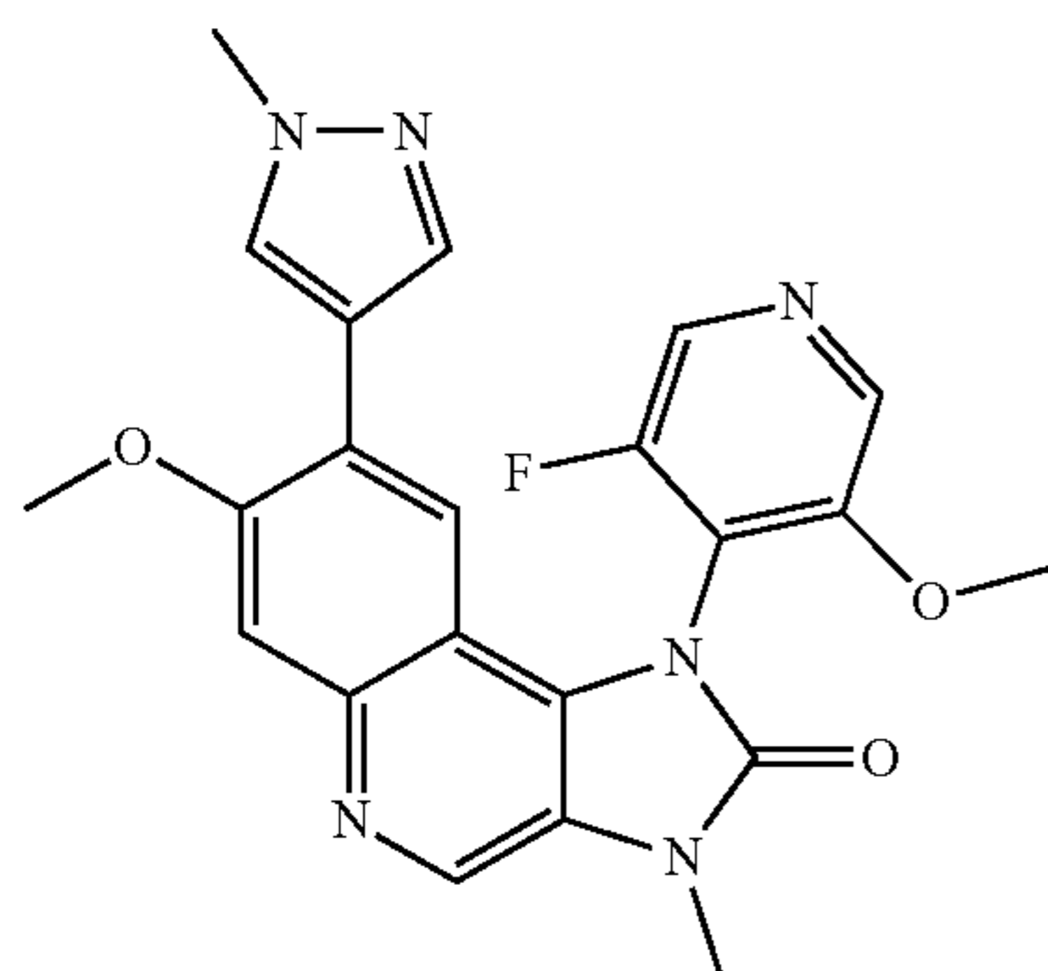
1-(3-Fluoro-5-methoxypyridin-4-yl)-7-methoxy-3-methyl-8-(1-methyl-1H-pyrazol-4-yl)-1,3-dihydroimidazo[4,5-c]quinolin-2-one
