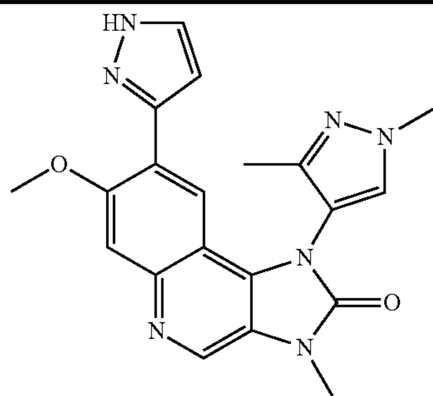
1-(1,3-Dimethyl-1H-pyrazol-4-yl)-7-methoxy-3-methyl-8-(1H-pyrazol-3-yl)-1,3-dihydro-imidazo[4,5-c]quinolin-2-one
