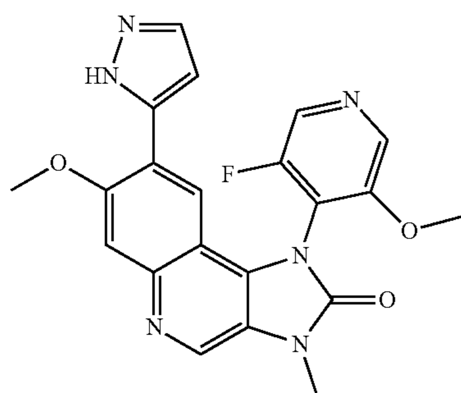
1-(3-Fluoro-5-methoxypyridin-4-yl)-7-methoxy-3-methyl-8-(2H-pyrazol-3-yl)-1,3-dihydroimidazo[4,5-c]quinolin-2-one
