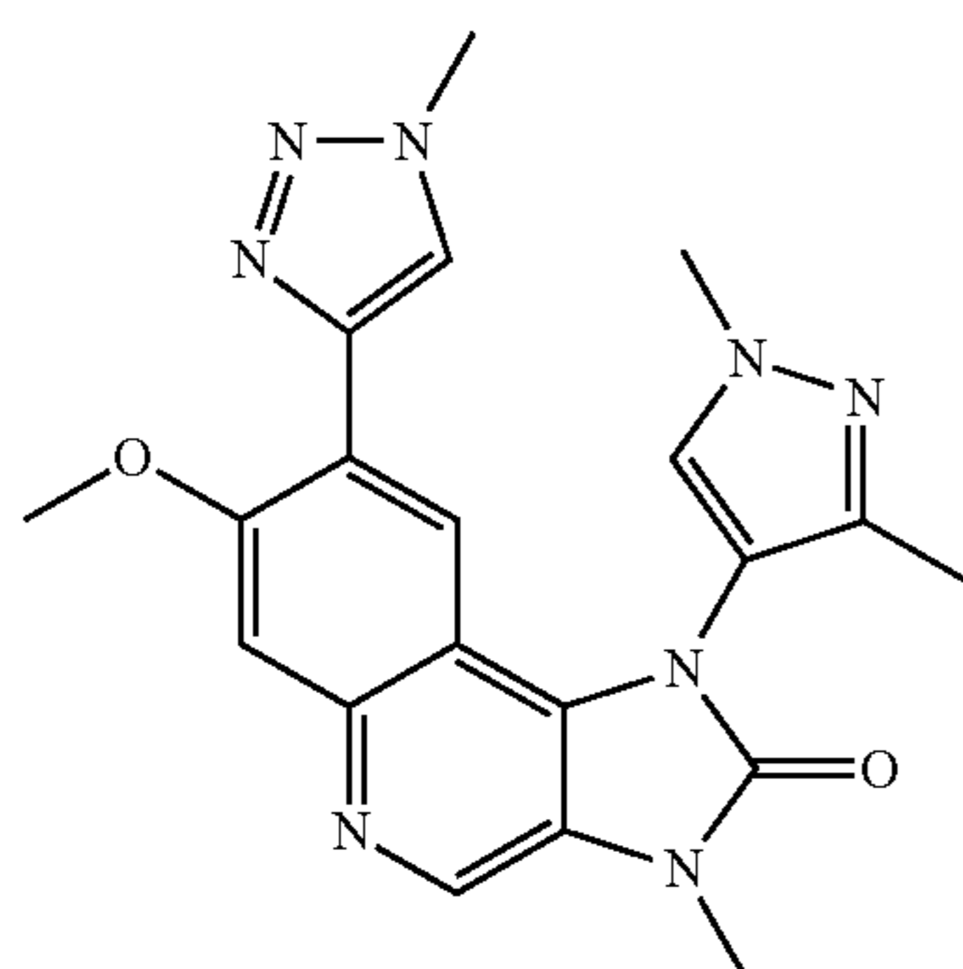
1-(1,3-Dimethyl-1H-pyrazol-4-yl)-7-methoxy-3-methyl-8-(1-methyl-1H-1,2,3-triazol-4-yl)-1,3-dihydroimidazo[4,5-c]quinolin-2-one
