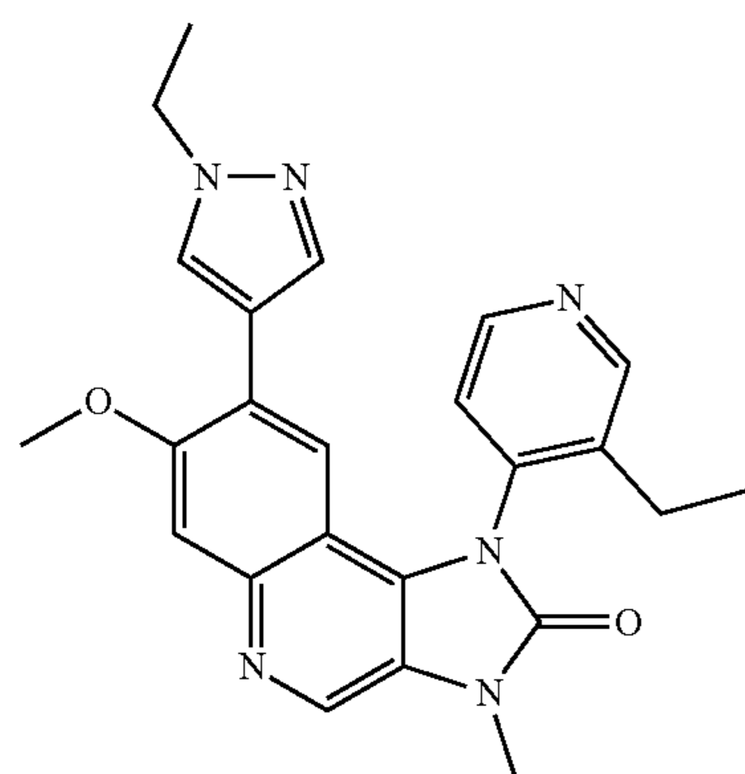
8-(1-Ethyl-1H-pyrazol-4-yl)-1-(3-ethylpyridin-4-yl)-7-methoxy-3-methyl-1,3-dihydroimidazo[4,5-c]quinolin-2-one
