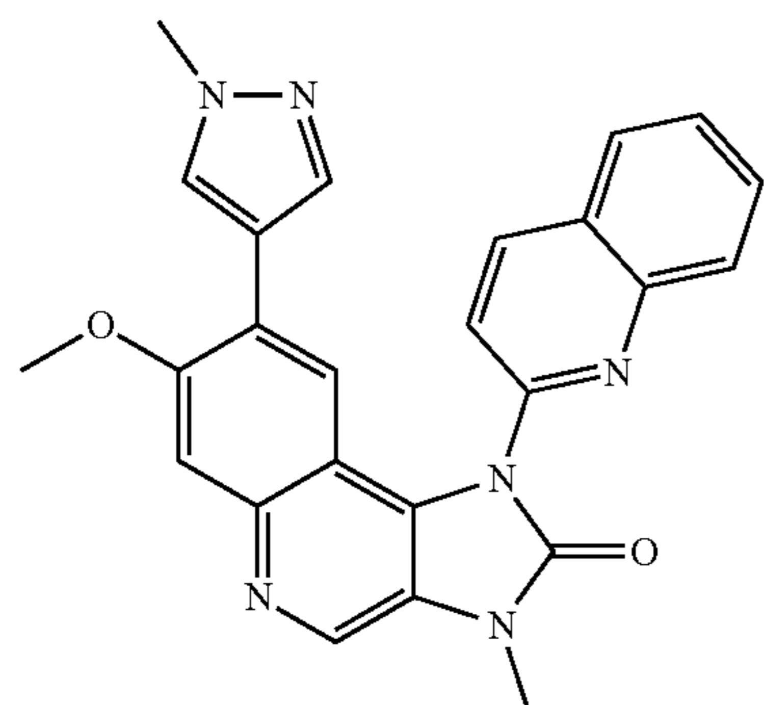
7-Methoxy-3-methyl-8-(1-methyl-1H-pyrazol-4-yl)-1-quinolin-2-yl-1,3-dihydroimidazo[4,5-c]quinolin-2-one
