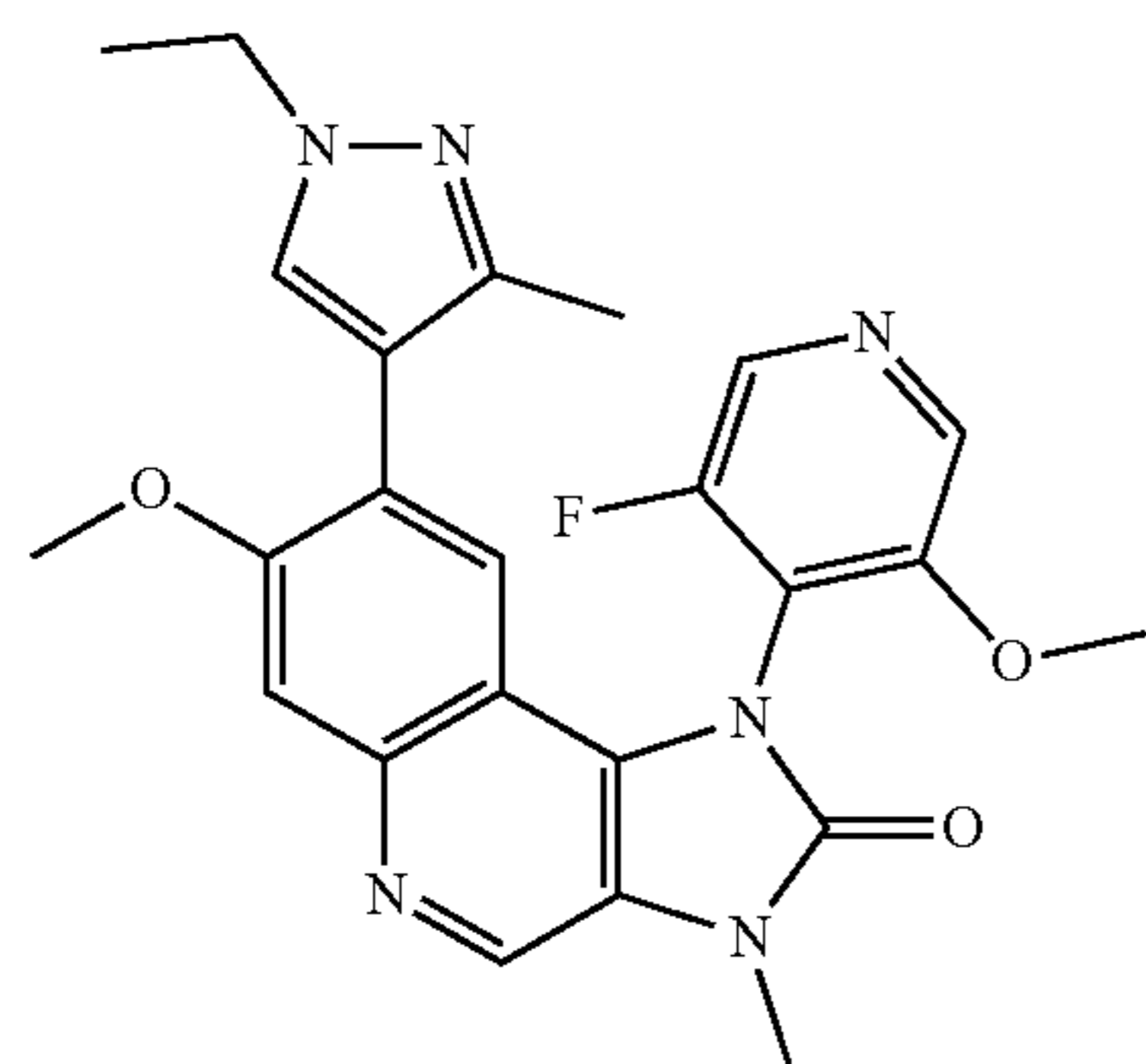
8-(1-Ethyl-3-methyl-1H-pyrazol-4-yl)-1-(3-fluoro-5-methoxypyridin-4-yl)-7-methoxy-3-methyl-1,3-dihydroimidazo[4,5-c]quinolin-2-one
