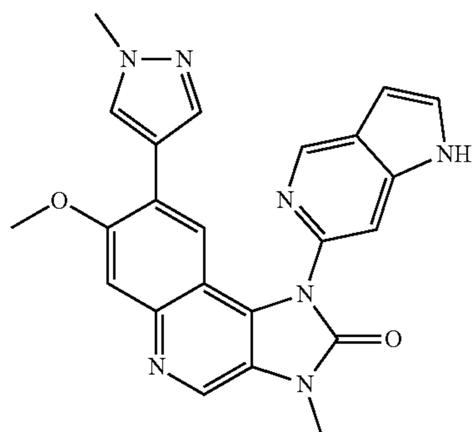
7-Methoxy-3-methyl-8-(1-methyl-1H-pyrazol-4-yl)-1-(1H-pyrrolo[3,2-c]pyridin-6-yl)-1,3-dihydroimidazo[4,5-c]quinolin-2-one
