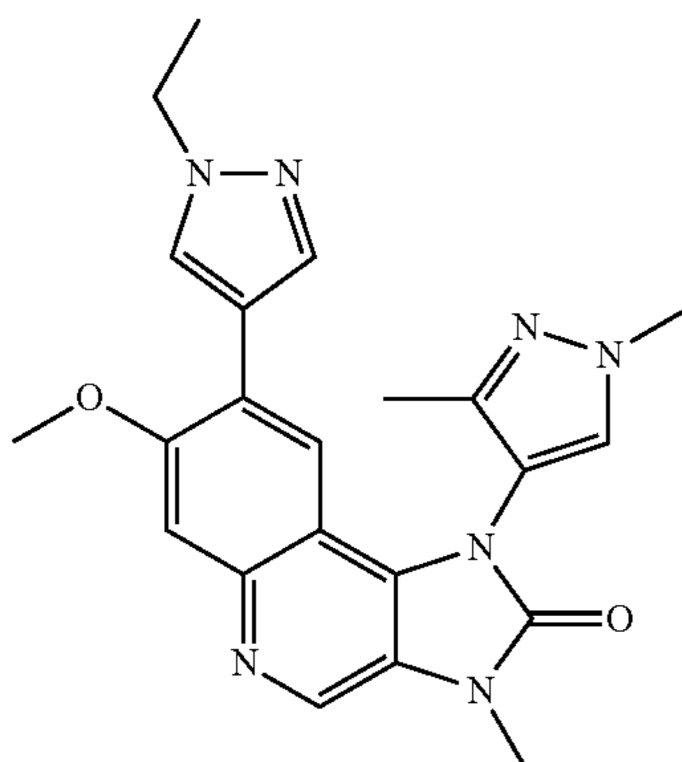
1-(1,3-Dimethyl-1H-pyrazol-4-yl)-8-(1-ethyl-1H-pyrazol-4-yl)-7-methoxy-3-methyl-1,3-dihydroimidazo[4,5-c]quinolin-2-one
