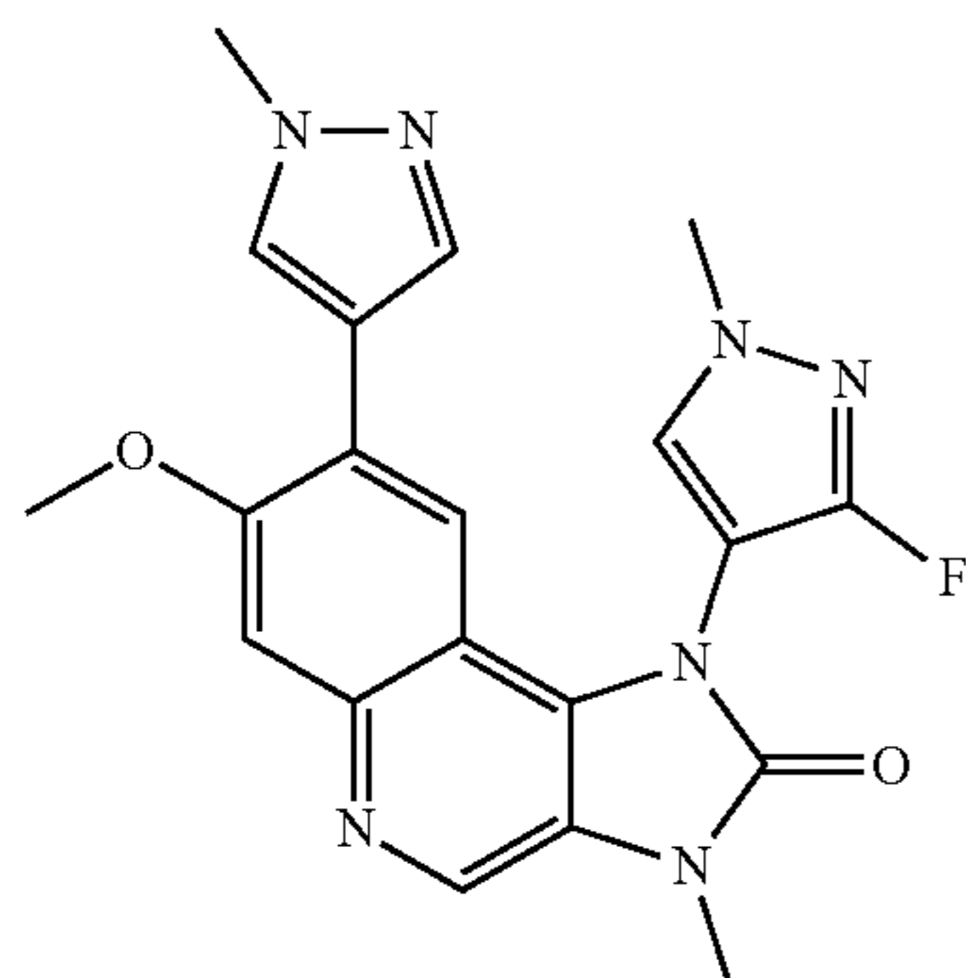
1-(3-Fluoro-1-methyl-1H-pyrazol-4-yl)-7-methoxy-3-methyl-8-(1-methyl-1H-pyrazol-4-yl)-1,3-dihydroimidazo[4,5-c]quinolin-2-one
