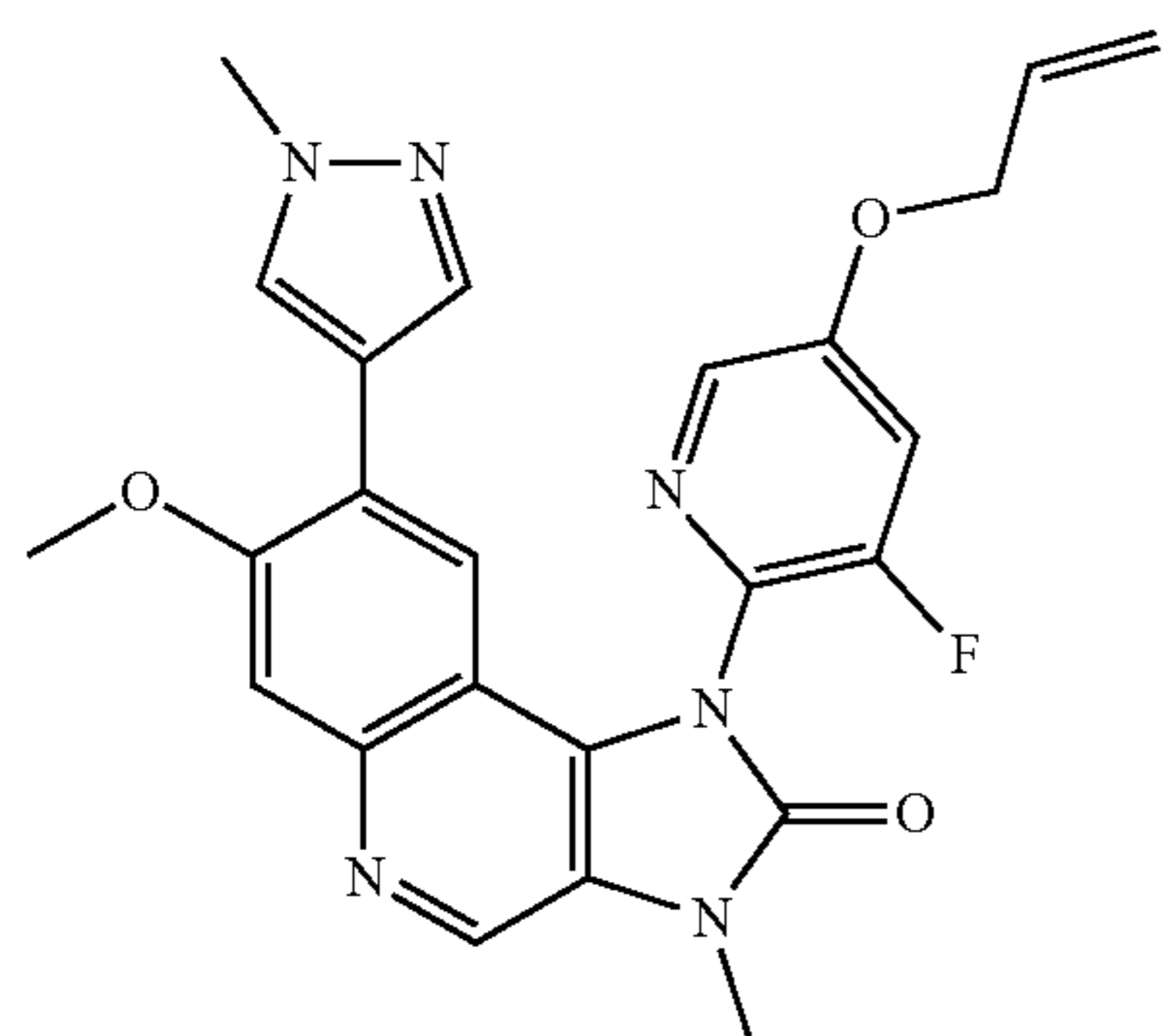
1-(5-Allyloxy-3-fluoropyridin-2-yl)-7-methoxy-3-methyl-8-(1-methyl-1H-pyrazol-4-yl)-1,3-dihydroimidazo[4,5-c]quinolin-2-one
