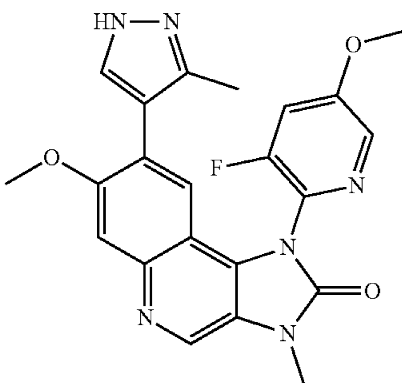
1-(3-Fluoro-5-methoxypyridin-2-yl)-7-methoxy-3-methyl-8-(3-methyl-1H-pyrazol-4-yl)-1,3-dihydroimidazo[4,5-c]quinolin-2-one
