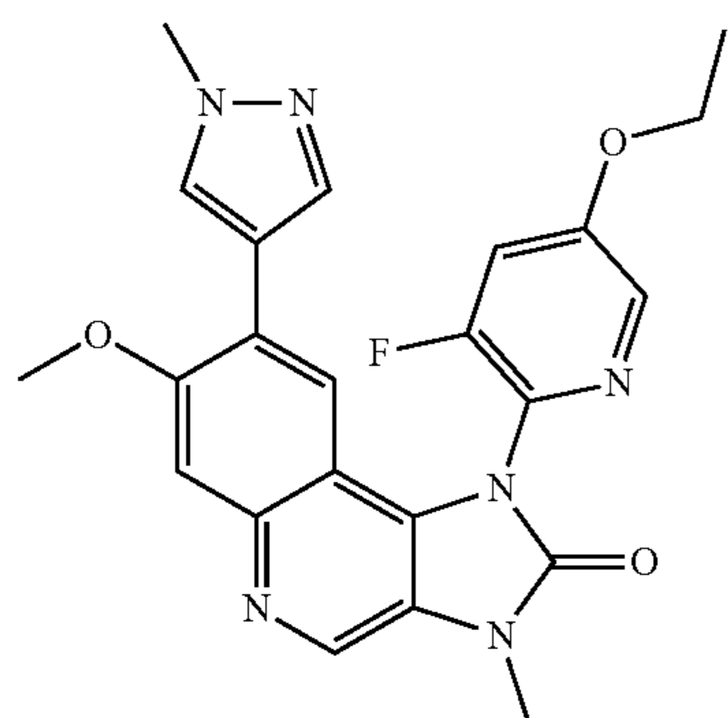
1-(5-Ethoxy-3-fluoropyridin-2-yl)-7-methoxy-3-methyl-8-(1-methyl-1H-pyrazol-4-yl)-1,3-dihydroimidazo[4,5-c]quinolin-2-one
