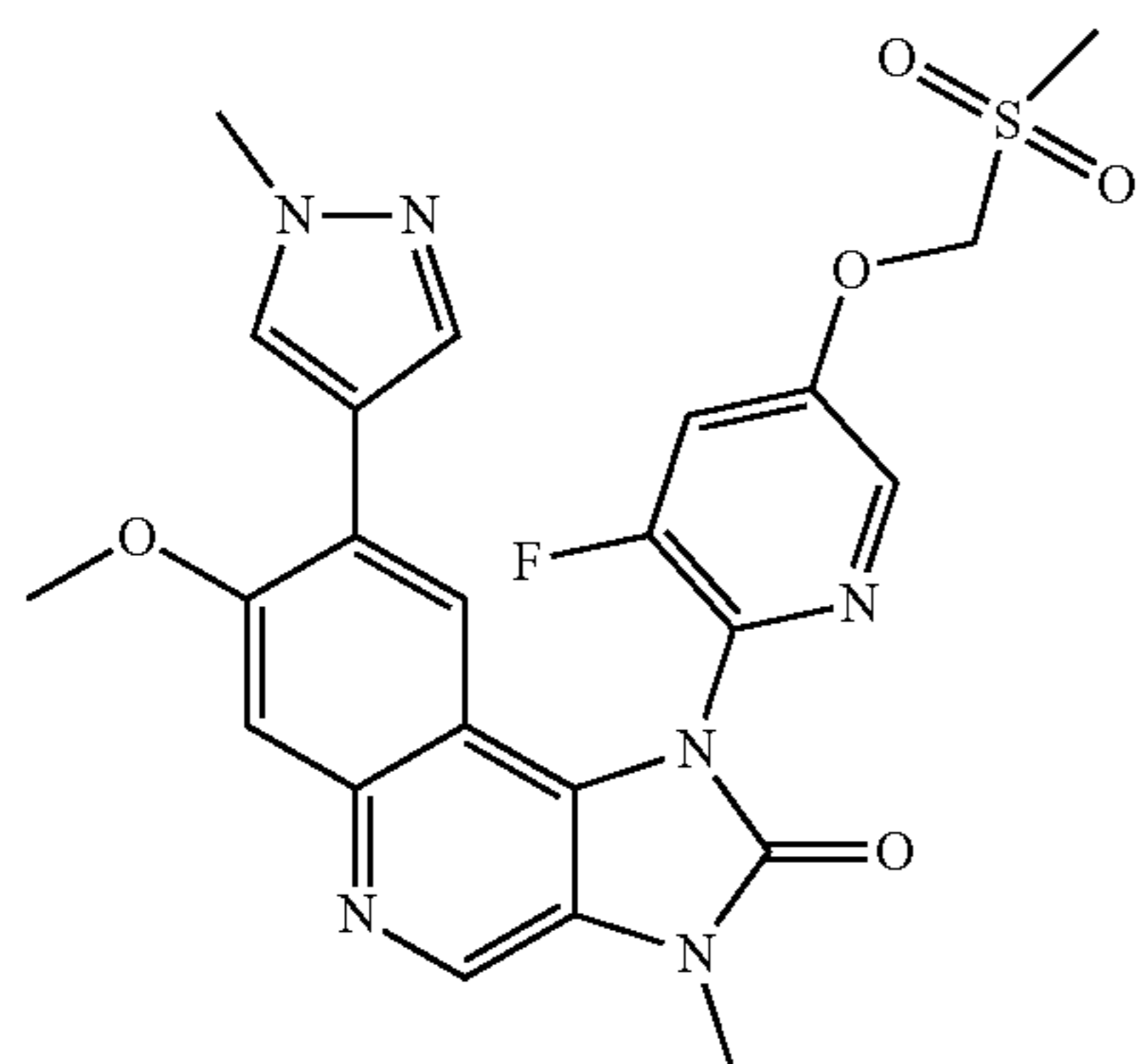
1-(3-Fluoro-5-methylsulfonylmethoxypyridin-2-yl)-7-methoxy-3-methyl-8-(1-methyl-1H-pyrazol-4-yl)-1,3-dihydroimidazo[4,5-c]quinolin-2-one
