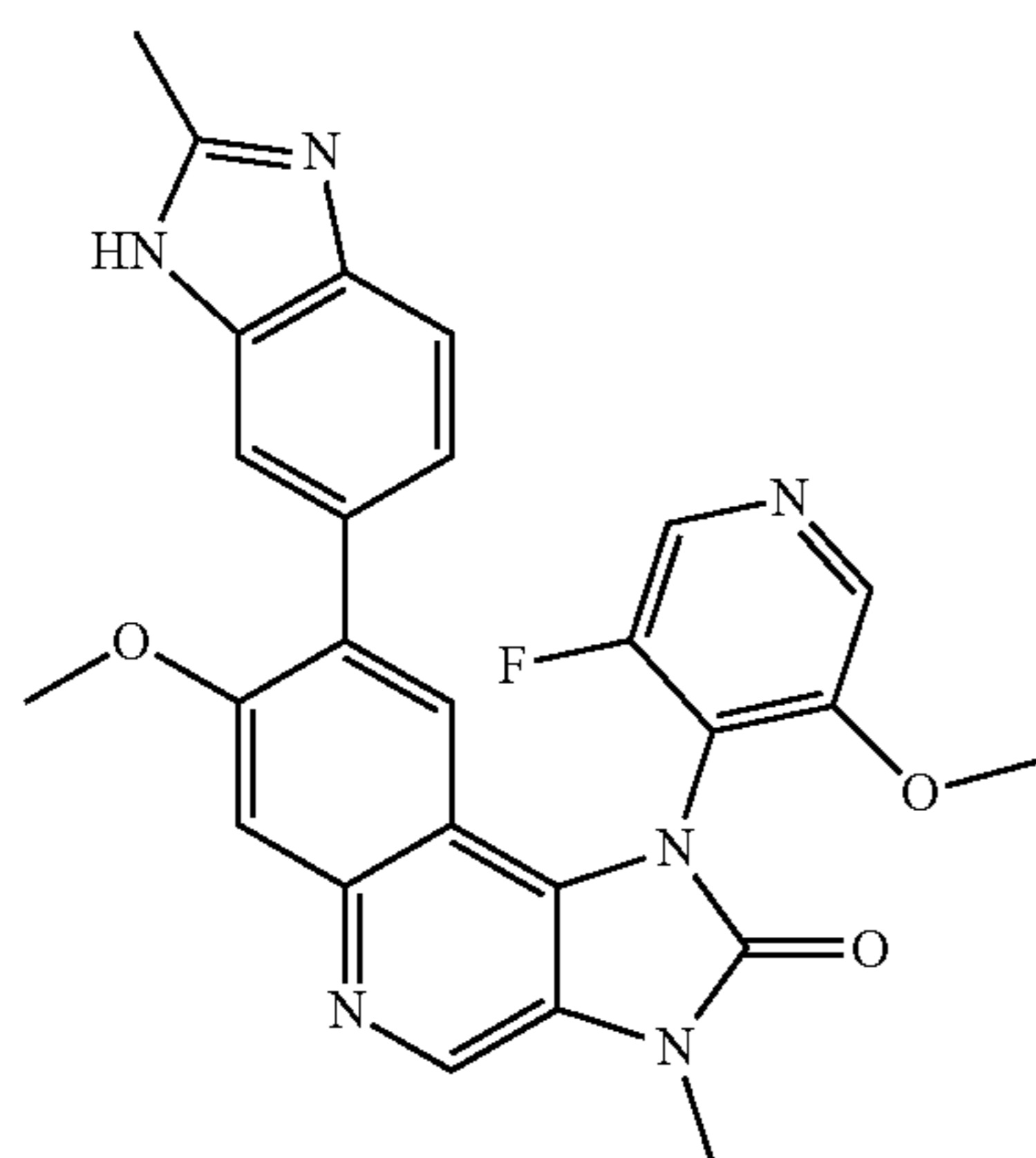
1-(3-Fluoro-5-methoxypyridin-4-yl)-7-methoxy-3-methyl-8-(2-methyl-3H-benzimidazol-5-yl)-1,3-dihydroimidazo[4,5-c]quinolin-2-one
