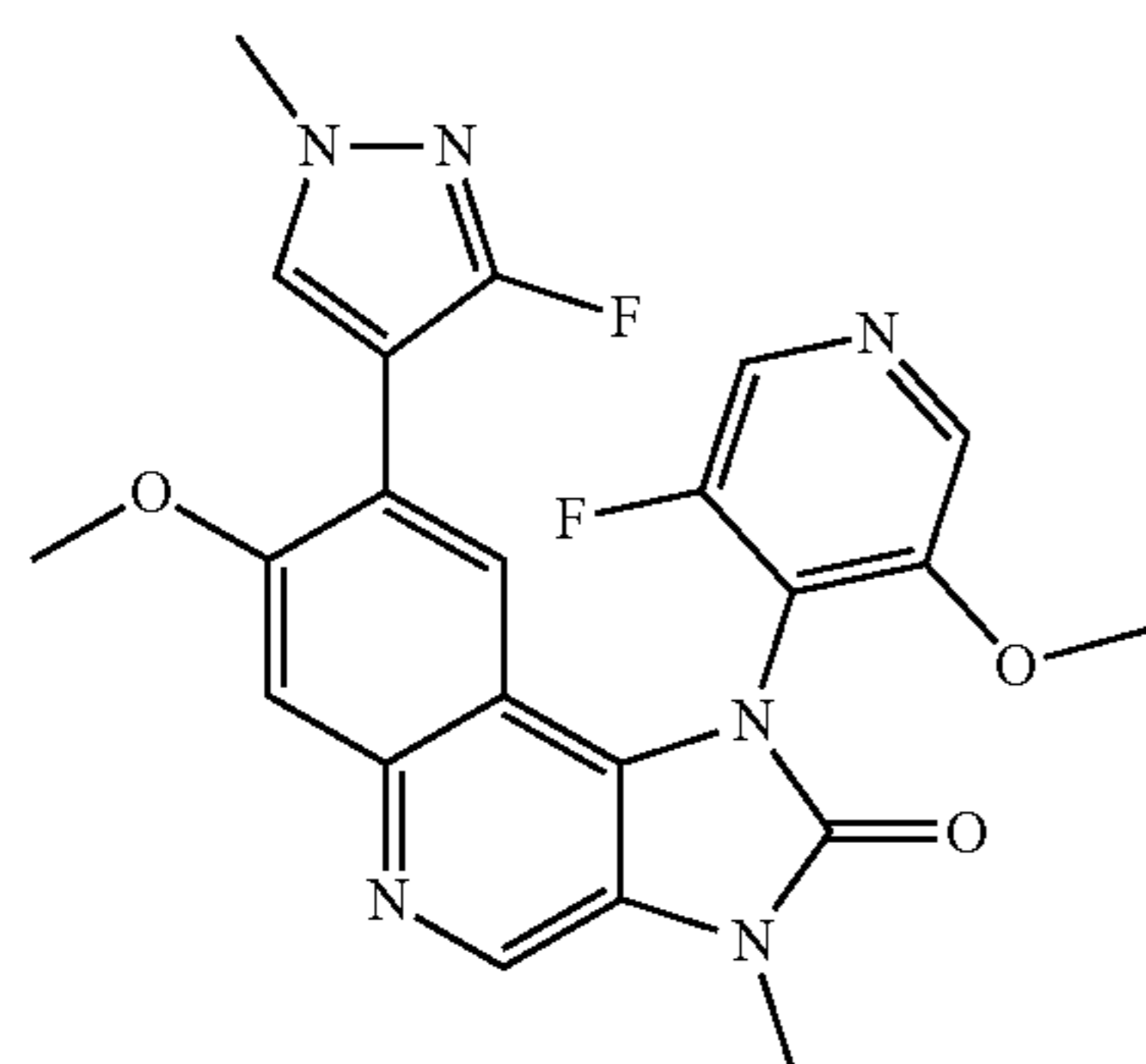
1-(3-Fluoro-5-methoxypyridin-4-yl)-7-methoxy-3-methyl-8-(3-fluoro-1-methyl-1H-pyrazol-4-yl)-1,3-dihydroimidazo[4,5-c]quinolin-2-one
