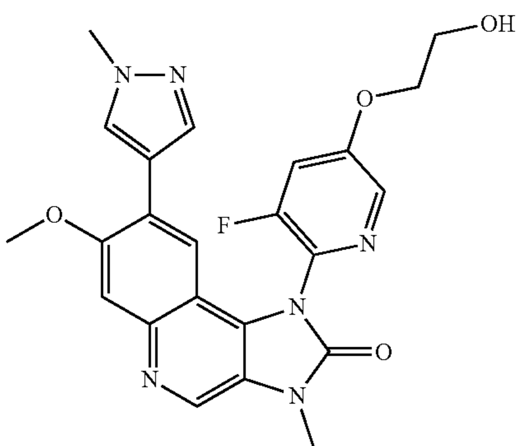
1-[3-Fluoro-5-(2-hydroxyethoxy)-2-pyridyl]-7-methoxy-3-methyl-8-(1-methylpyrazol-4-yl)imidazo[4,5-c]quinolin-2-one
