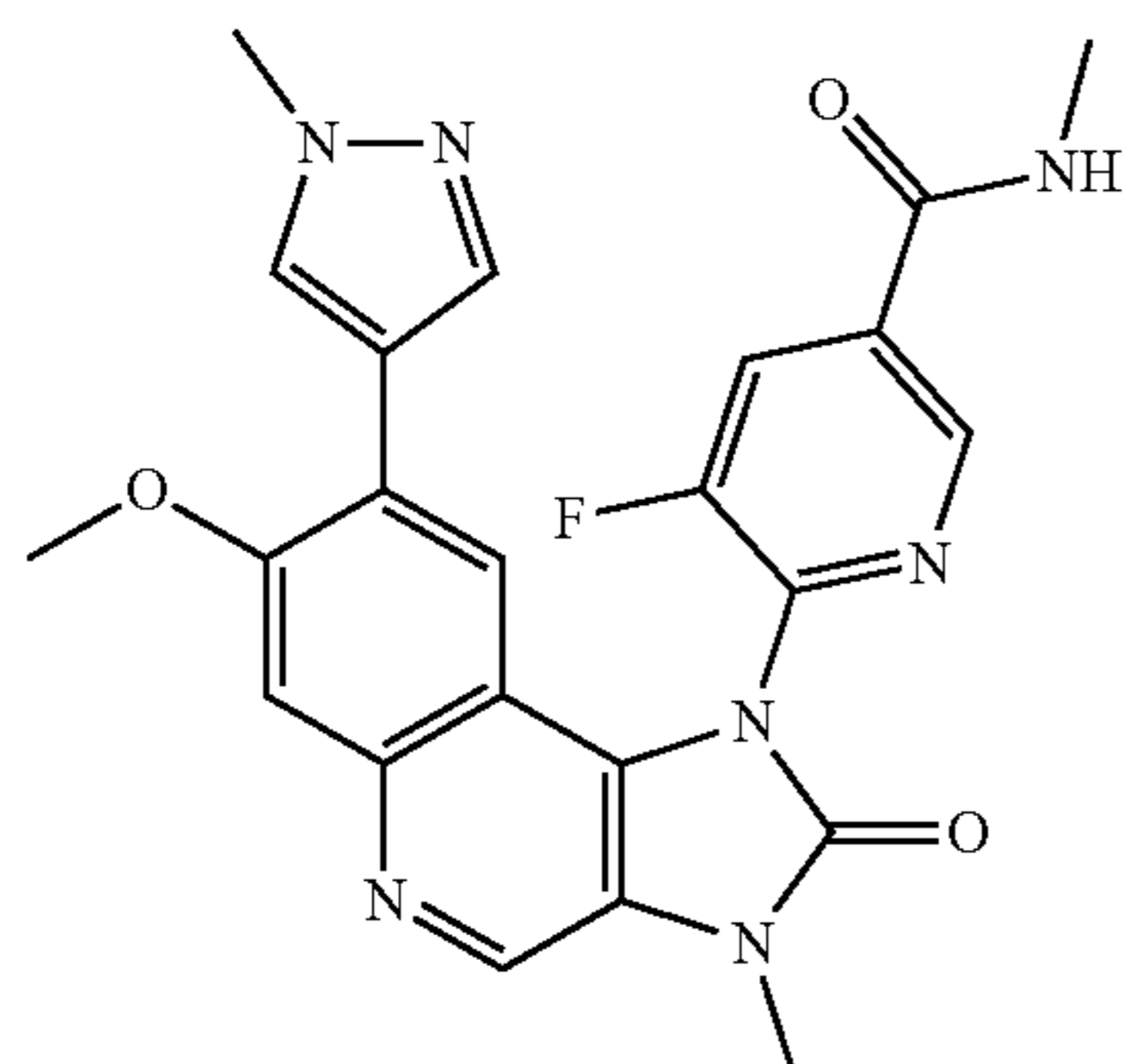
5-Fluoro-6-[7-methoxy-3-methyl-8-(1-methyl-1H-pyrazol-4-yl)-2-oxo-2,3-dihydroimidazo[4,5-c]quinolin-1-yl]-N-methylnicotinamide
