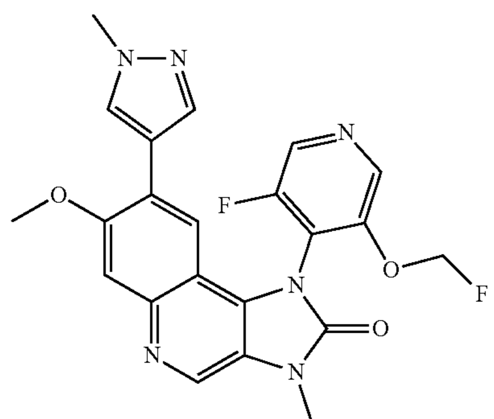
1-(3-Fluoro-5-fluoromethoxypyridin-4-yl)-7-methoxy-3-methyl-8-(1-methyl-1H-pyrazol-4-yl)-1,3-dihydroimidazo[4,5-c]quinolin-2-one
