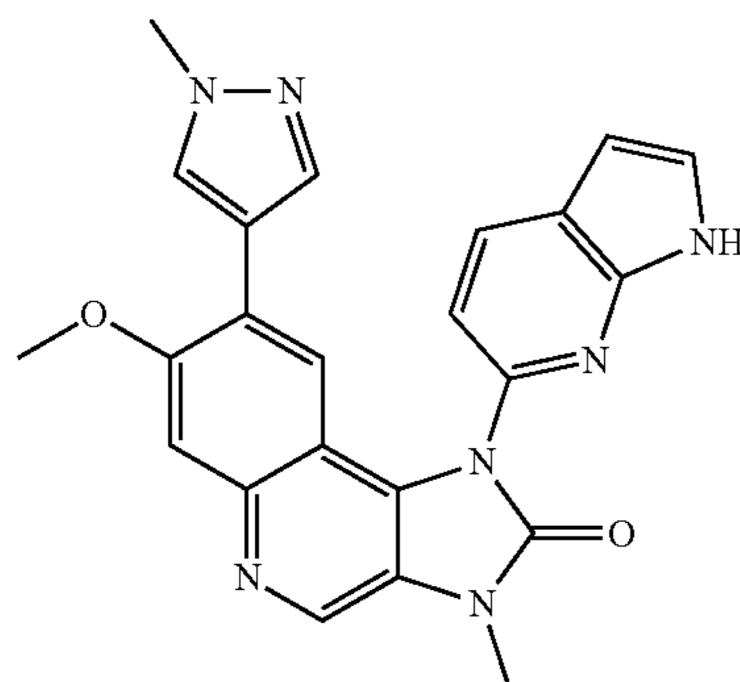
7-Methoxy-3-methyl-8-(1-methyl-1H-pyrazol-4-yl)-1-(1H-pyrrolo[2,3-b]pyridin-6-yl)-1,3-dihydroimidazo[4,5-c]quinolin-2-one
