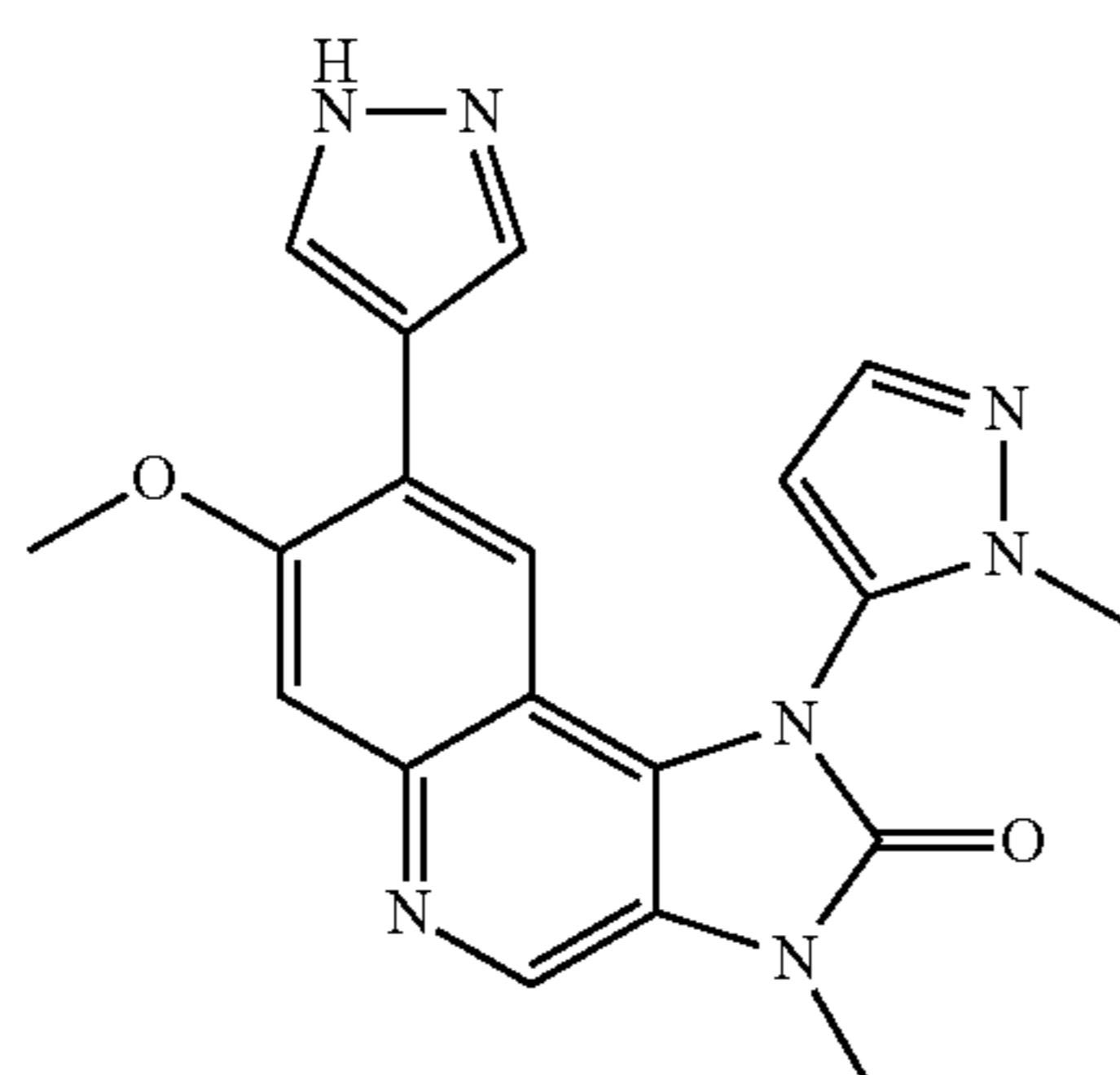
7-Methoxy-3-methyl-1-(2-methyl-2H-pyrazol-3-yl)-8-(1H-pyrazol-4-yl)-1,3-dihydroimidazo[4,5-c]quinolin-2-one
