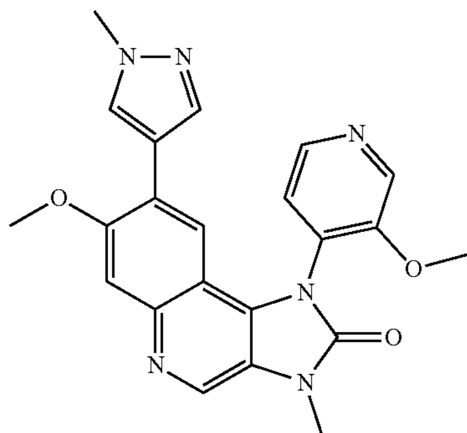
7-Methoxy-1-(3-methoxypyridin-4-yl)-3-methyl-8-(1-methyl-1H-pyrazol-4-yl)-1,3-dihydroimidazo[4,5-c]quinolin-2-one
