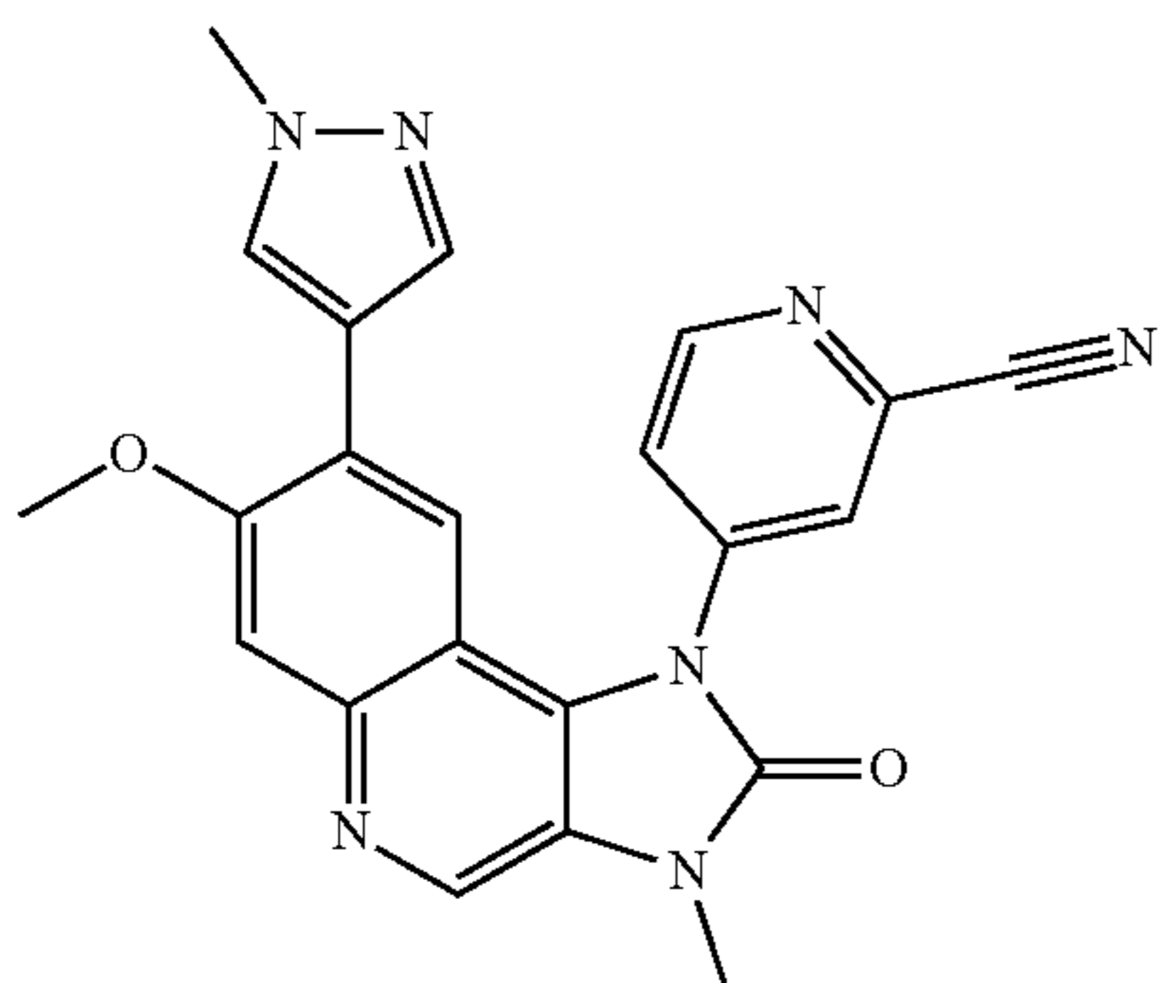
4-[7-Methoxy-3-methyl-8-(1-methyl-1H-pyrazol-4-yl)-2-oxo-2,3-dihydroimidazo[4,5-c]quinolin-1-yl]pyridine-2-carbonitrile
