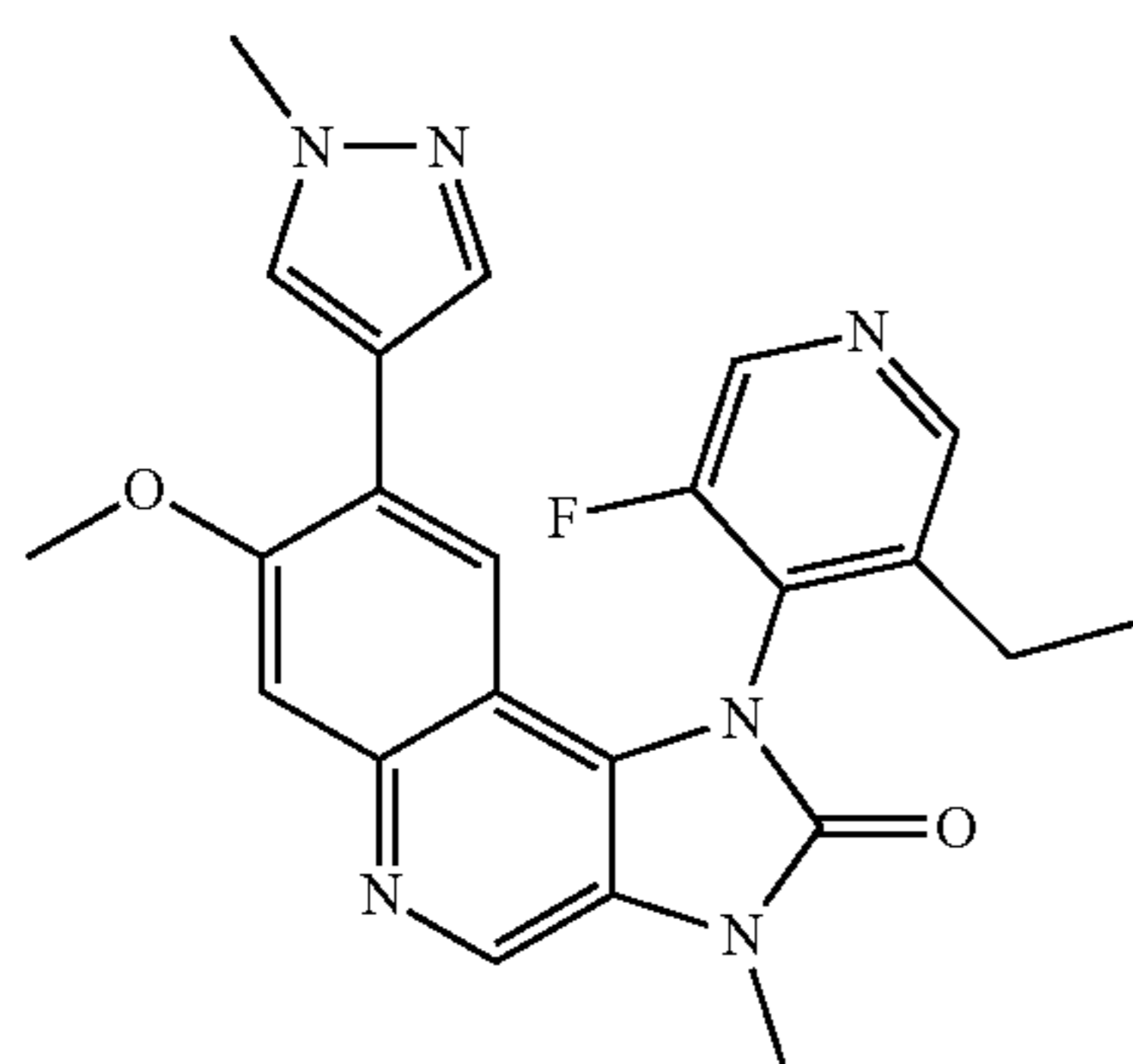
1-(3-Ethyl-5-fluoropyridin-4-yl)-7-methoxy-3-methyl-8-(1-methyl-1H-pyrazol-4-yl)-1,3-dihydroimidazo[4,5-c]quinolin-2-one
