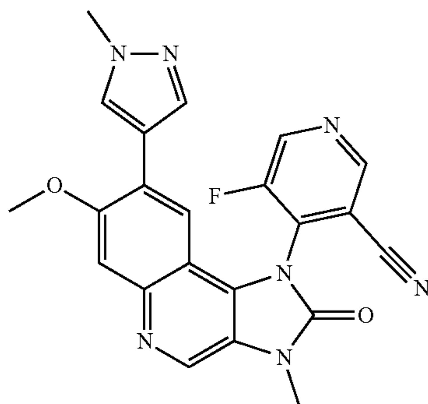
5-Fluoro-4-[7-methoxy-3-methyl-8-(1-methyl-1H-pyrazol-4-yl)-2-oxo-2,3-dihydroimidazo[4,5-c]quinolin-1-yl]nicotinonitrile
