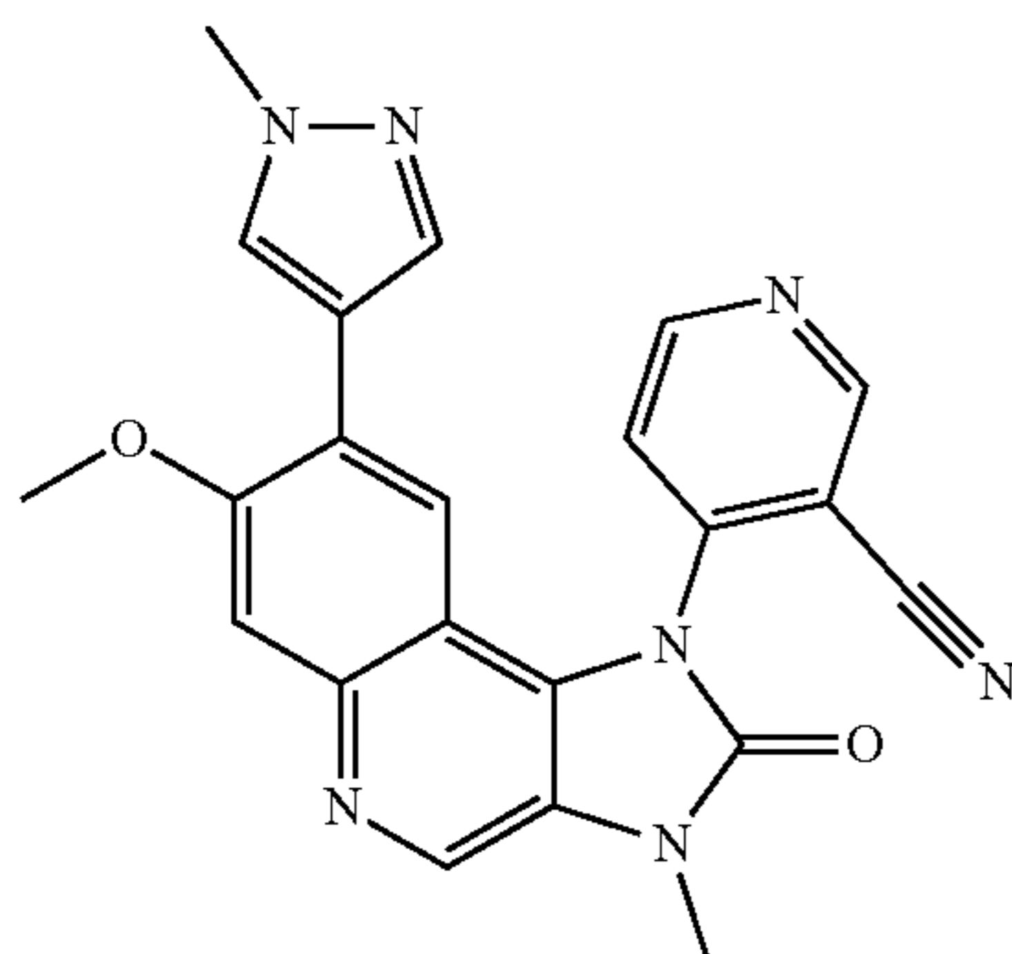
4-[7-Methoxy-3-methyl-8-(1-methyl-1H-pyrazol-4-yl)-2-oxo-2,3-dihydroimidazo[4,5-c]quinolin-1-yl]nicotinonitrile
