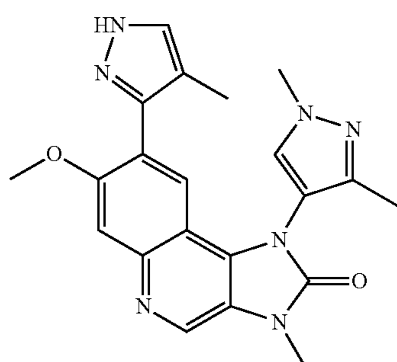
1-(1,3-Dimethyl-1H-pyrazol-4-yl)-7-methoxy-3-methyl-8-(4-methyl-1H-pyrazol-3-yl)-1,3-dihydroimidazo[4,5-c]quinolin-2-one
