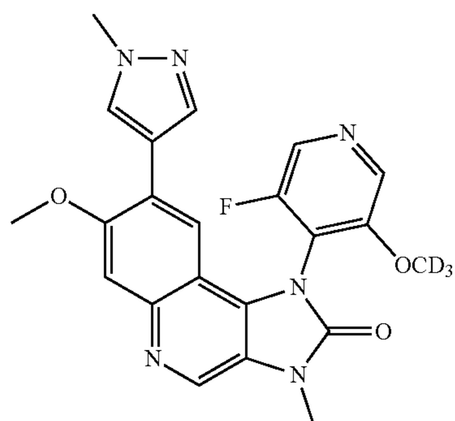
1-[3-Fluoro-5-(trideuteriomethoxy)-4-pyridyl]-7-methoxy-3-methyl-8-(1-methylpyrazol-4-yl)imidazo[4,5-c]quinolin-2-one
