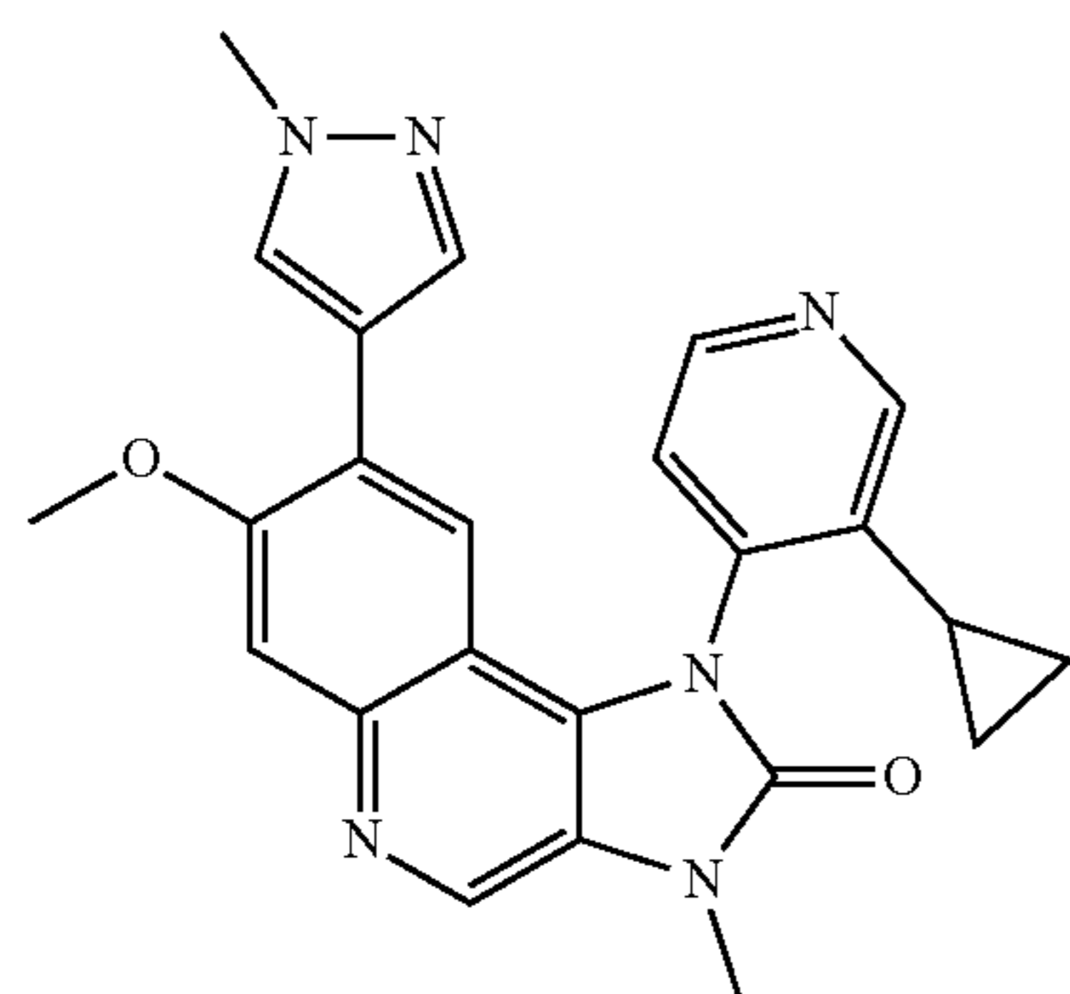
1-(3-Cyclopropylpyridin-4-yl)-7-methoxy-3-methyl-8-(1-methyl-1H-pyrazol-4-yl)-1,3-dihydroimidazo[4,5-c]quinolin-2-one
