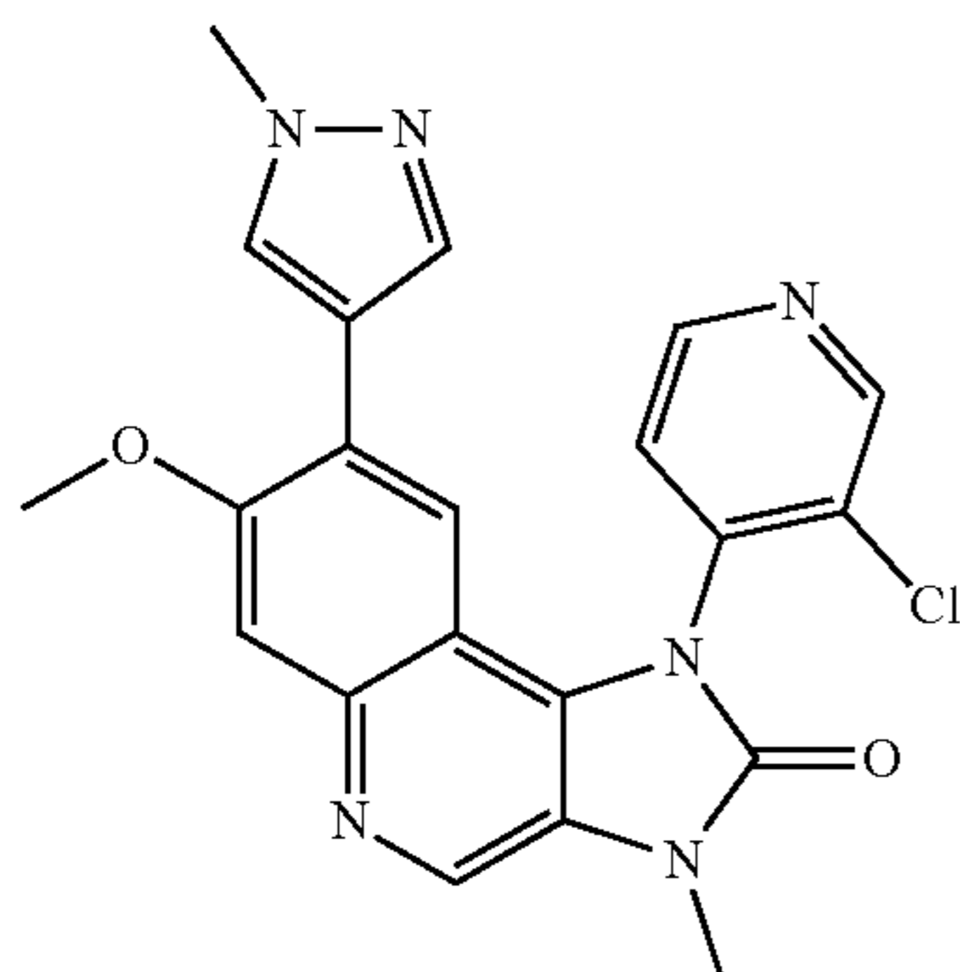
1-(3-Chloropyridin-4-yl)-7-methoxy-3-methyl-8-(1-methyl-1H-pyrazol-4-yl)-1,3-dihydroimidazo[4,5-c]quinolin-2-one
