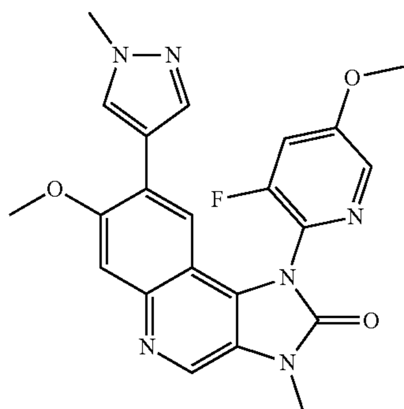
1-(3-Fluoro-5-methoxypyridin-2-yl)-7-methoxy-3-methyl-8-(1-methyl-1H-pyrazol-4-yl)-1,3-dihydroimidazo[4,5-c]quinolin-2-one
