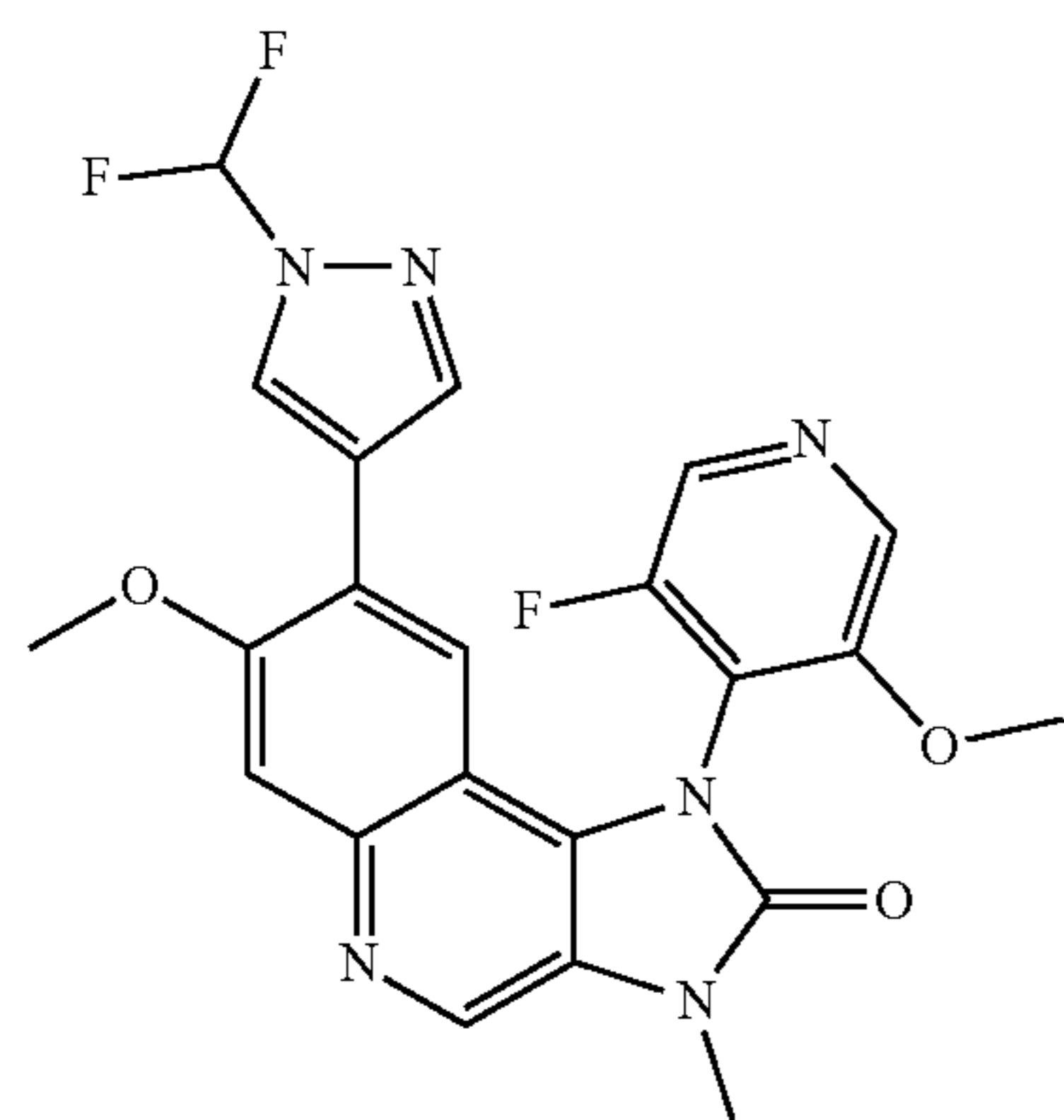
8-(1-Difluoromethyl-1H-pyrazol-4-yl)-1-(3-fluoro-5-methoxypyridin-4-yl)-7-methoxy-3-methyl-1,3-dihydroimidazo[4,5-c]quinolin-2-one
