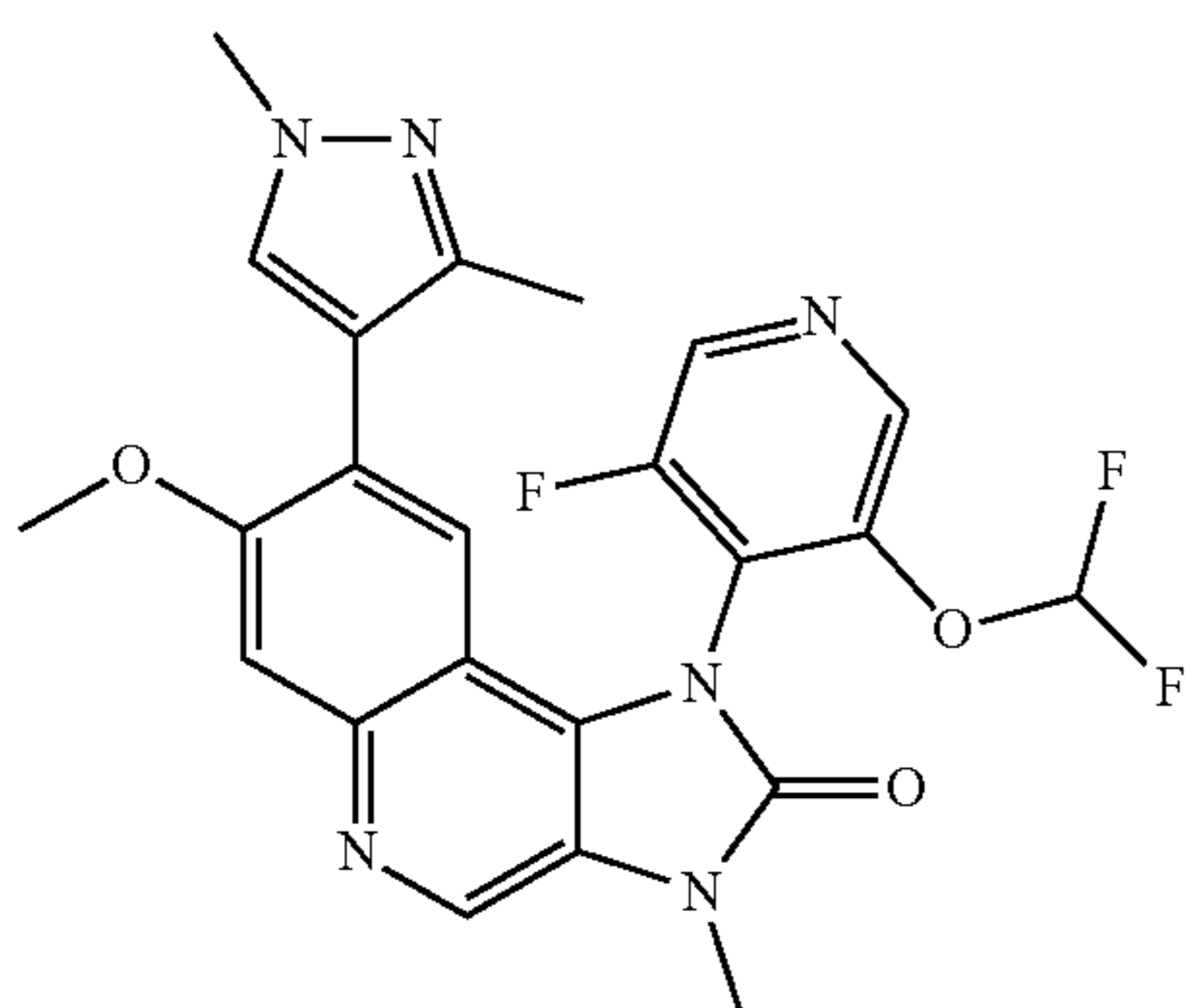
1-(3-Difluoromethoxy-5-fluoropyridin-4-yl)-8-(1,3-dimethyl-1H-pyrazol-4-yl)-7-methoxy-3-methyl-1,3-dihydroimidazo[4,5-c]quinolin-2-one
