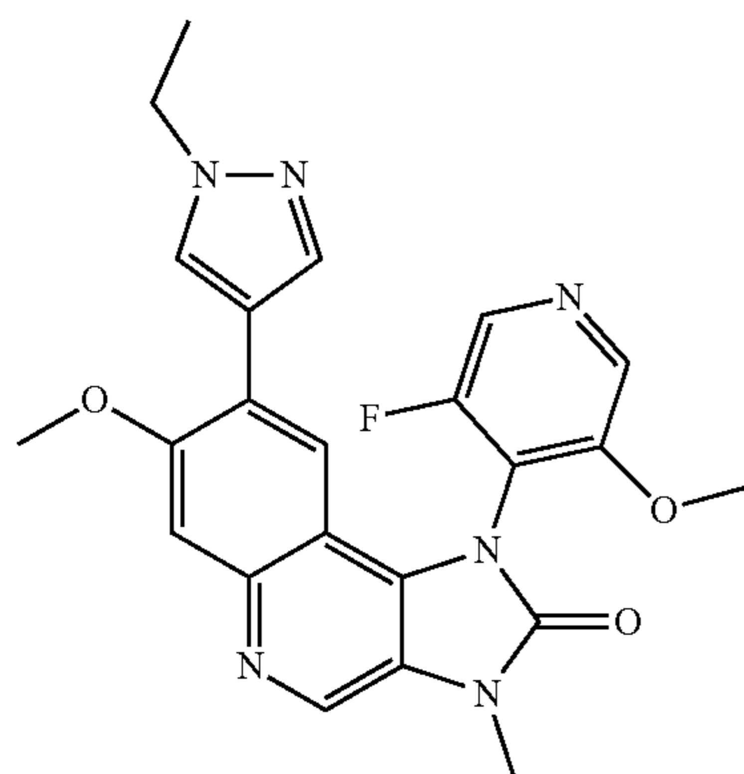
8-(1-Ethyl-1H-pyrazol-4-yl)-1-(3-fluoro-5-methoxypyridin-4-yl)-7-methoxy-3-methyl-1,3-dihydroimidazo[4,5-c]quinolin-2-one
