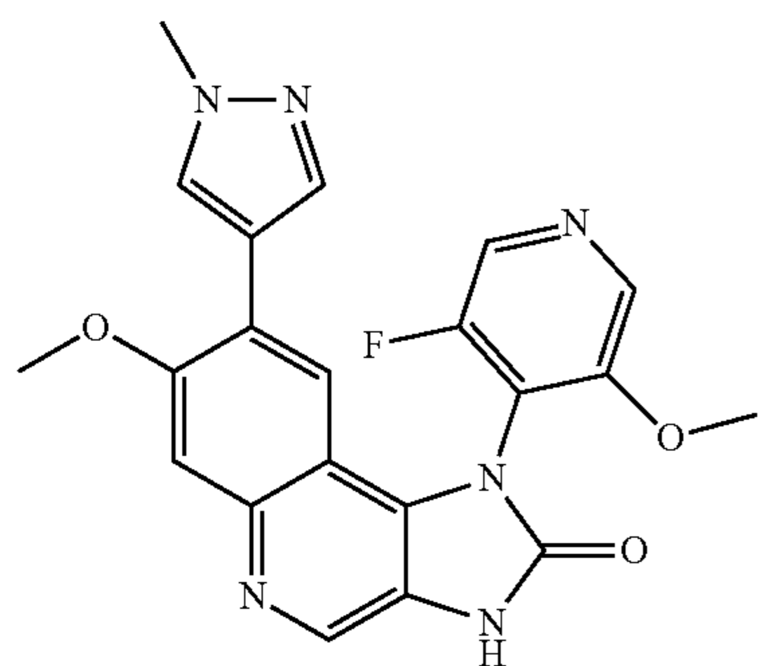
1-(3-Fluoro-5-methoxypyridin-4-yl)-7-methoxy-8-(1-methyl-1H-pyrazol-4-yl)-1,3-dihydroimidazo[4,5-c]quinolin-2-one
