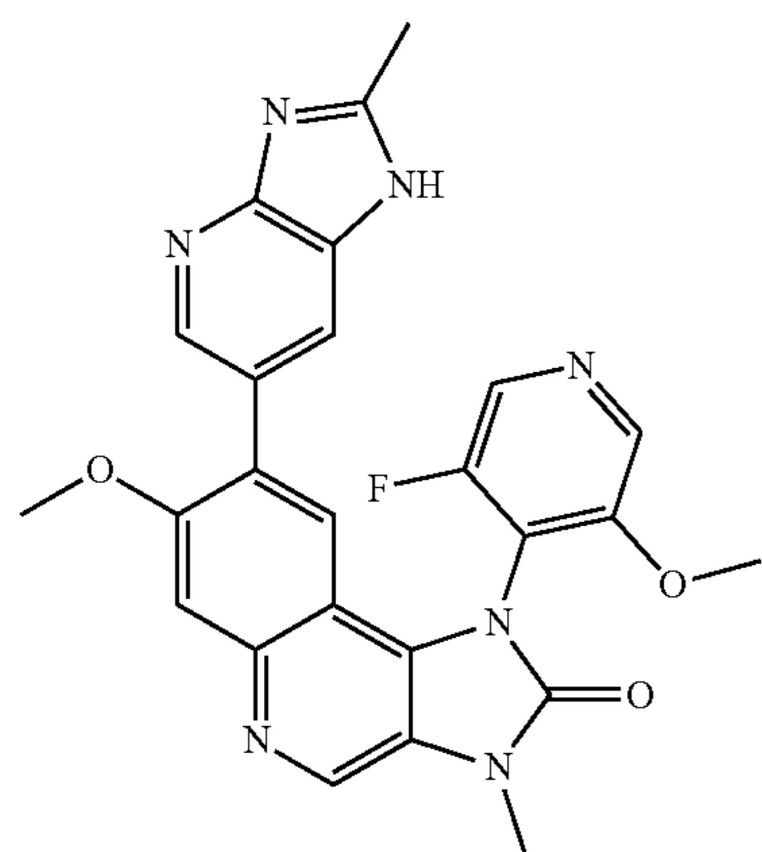
1-(3-Fluoro-5-methoxypyridin-4-yl)-7-methoxy-3-methyl-8-(2-methyl-1H-imidazo[4,5-b]pyridin-6-yl)-1,3-dihydroimidazo[4,5-c]quinolin-2-one
