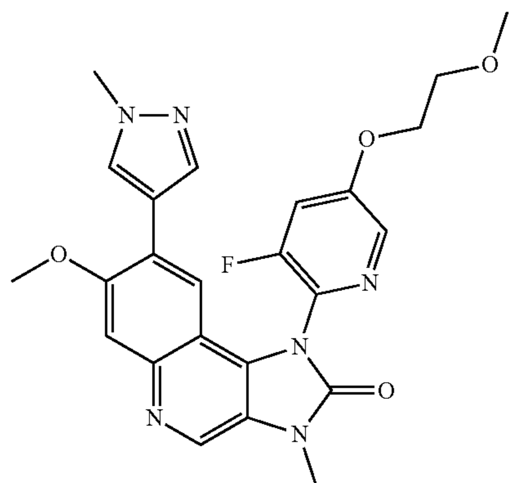
1-[3-Fluoro-5-(2-methoxyethoxy)-2-pyridyl]-7-methoxy-3-methyl-8-(1-methylpyrazol-4-yl)imidazo[4,5-c]quinolin-2-one
