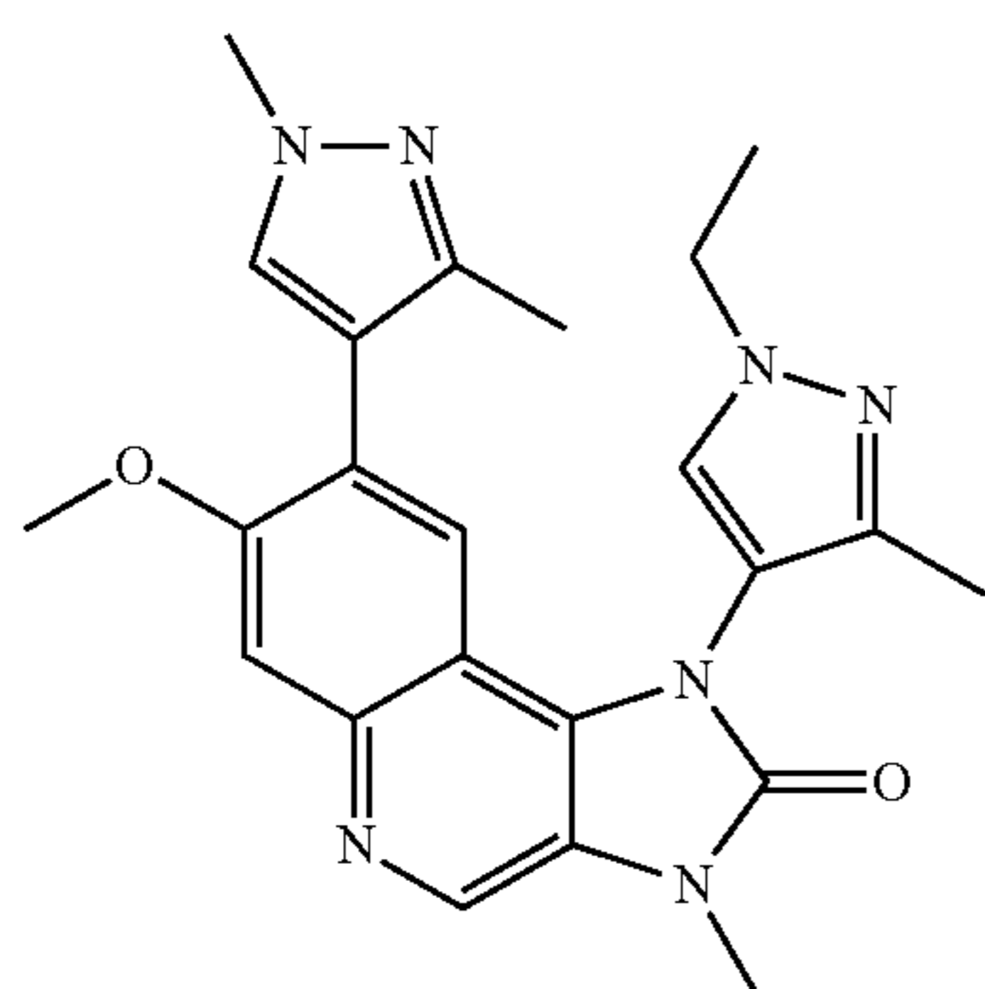
8-(1,3-Dimethyl-1H-pyrazol-4-yl)-1-(1-ethyl-3-methyl-1H-pyrazol-4-yl)-7-methoxy-3-methyl-1,3-dihydroimidazo[4,5-c]quinolin-2-one
