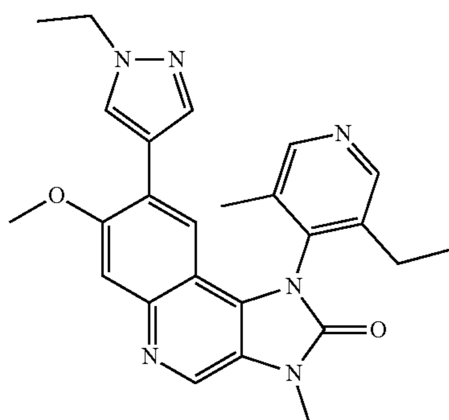
1-(3-Ethyl-5-methylpyridin-4-yl)-8-(1-ethyl-1H-pyrazol-4-yl)-7-methoxy-3-methyl-1,3-dihydroimidazo[4,5-c]quinolin-2-one
