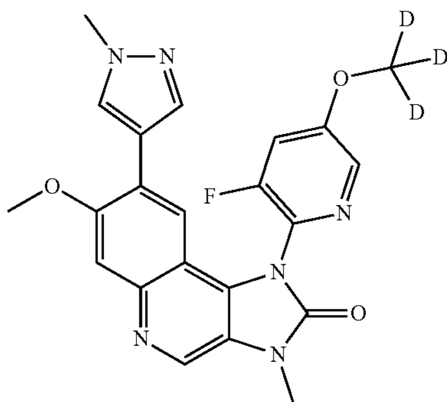
1-[3-Fluoro-5-(trideuteriomethoxy)-2-pyridyl]-7-methoxy-3-methyl-8-(1-methylpyrazol-4-yl)imidazo[4,5-c]quinolin-2-one
