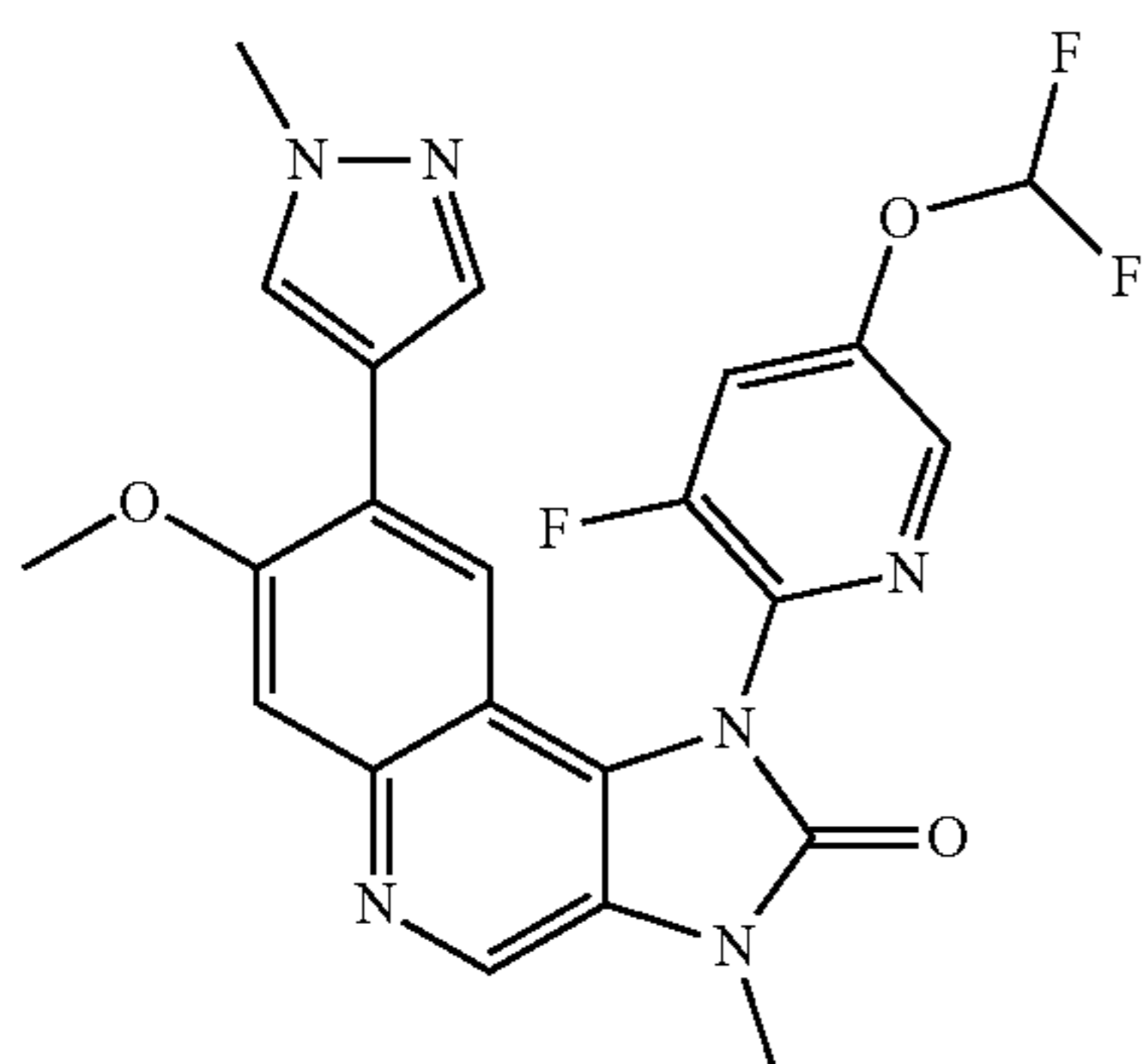
1-(5-Difluoromethoxy-3-fluoropyridin-2-yl)-7-methoxy-3-methyl-8-(1-methyl-1H-pyrazol-4-yl)-1,3-dihydroimidazo[4,5-c]quinolin-2-one
