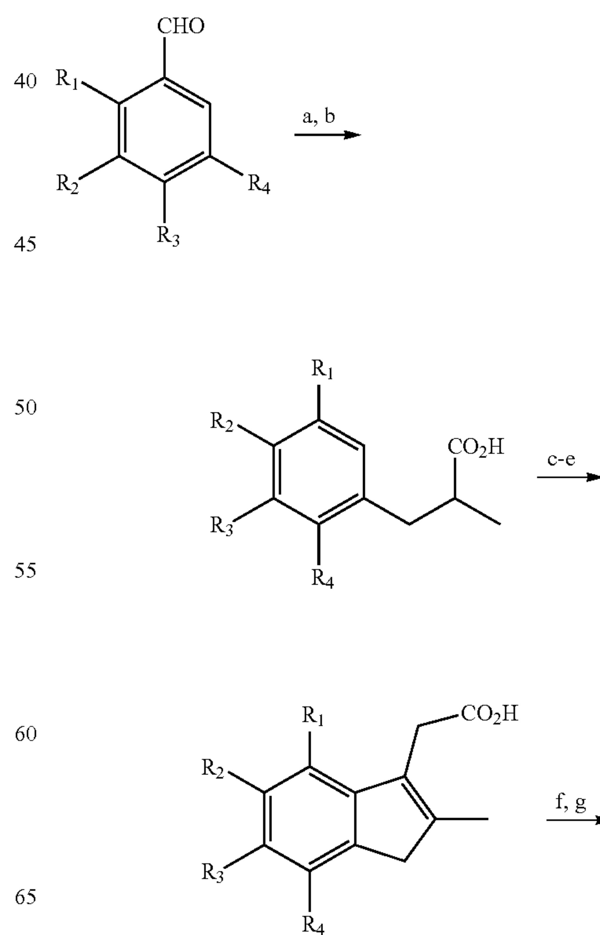
Scheme V
