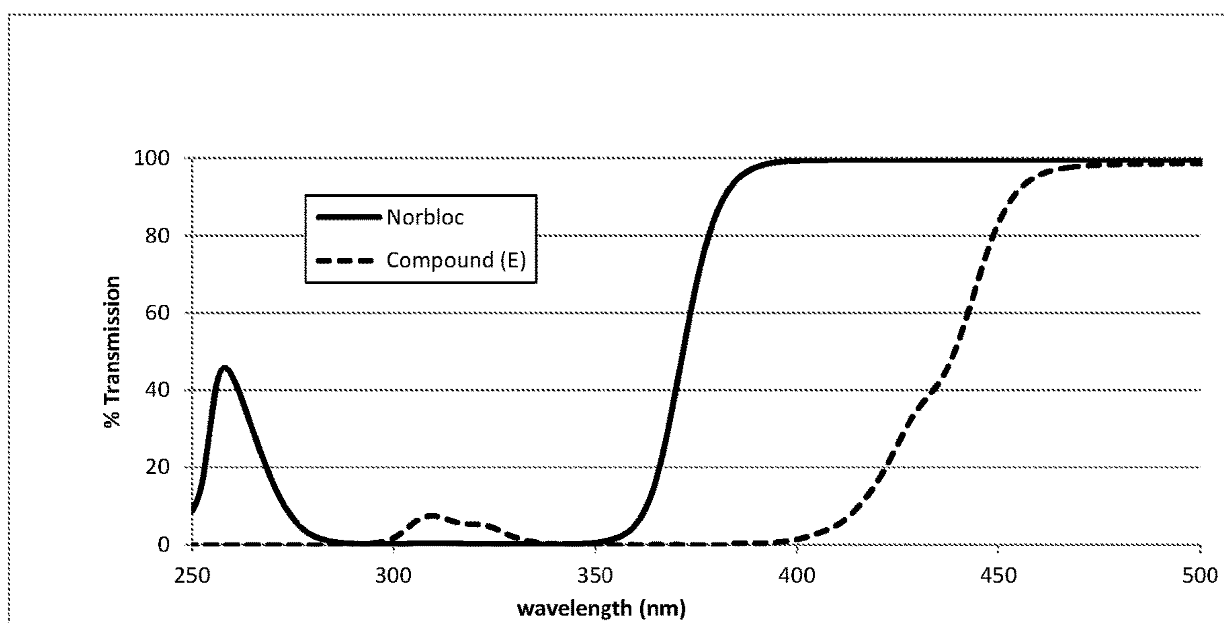
FIG. 1 – Transmission Spectra of Norbloc® and Compound (E) in 0.2 mM methanol solutions
