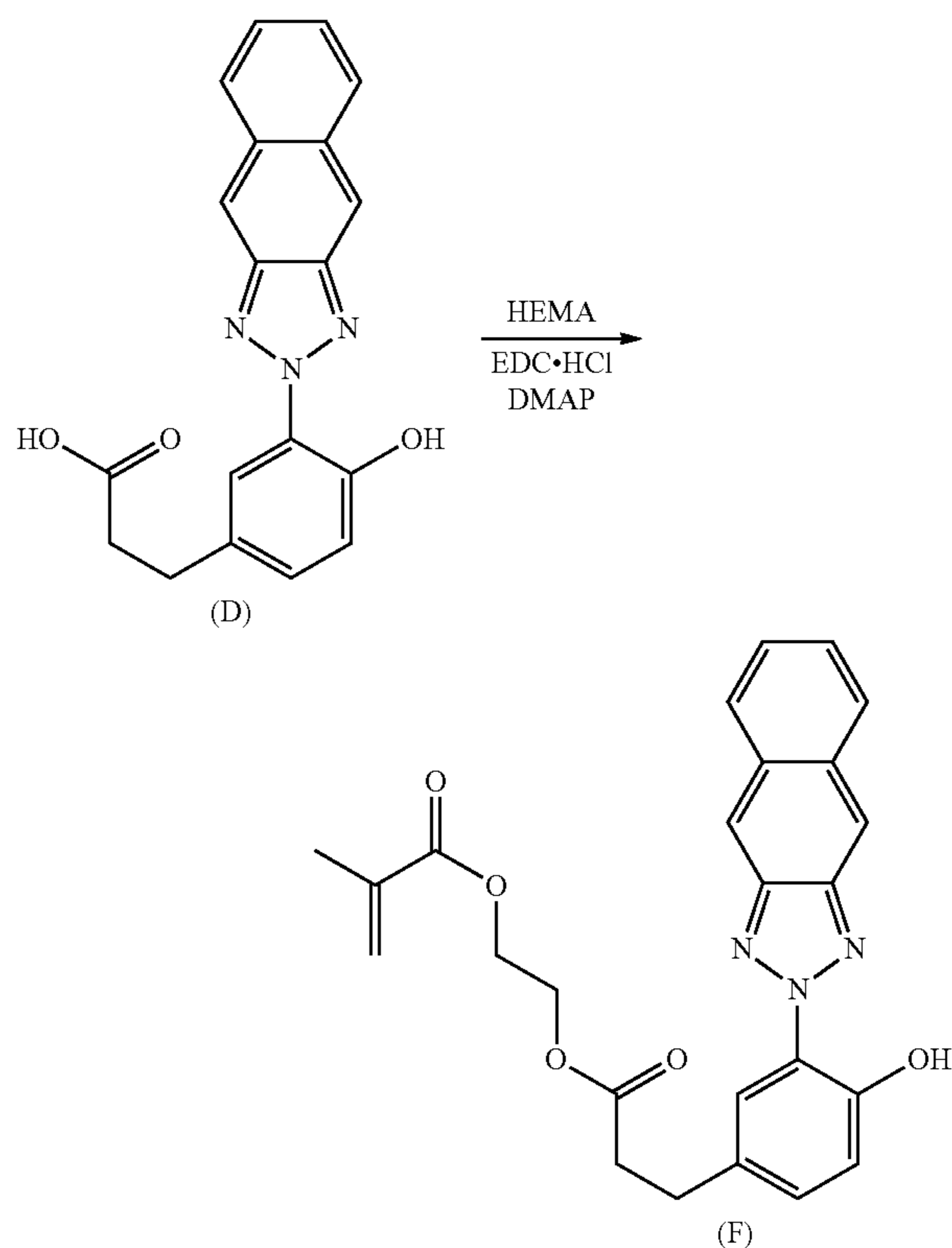
Scheme 2
