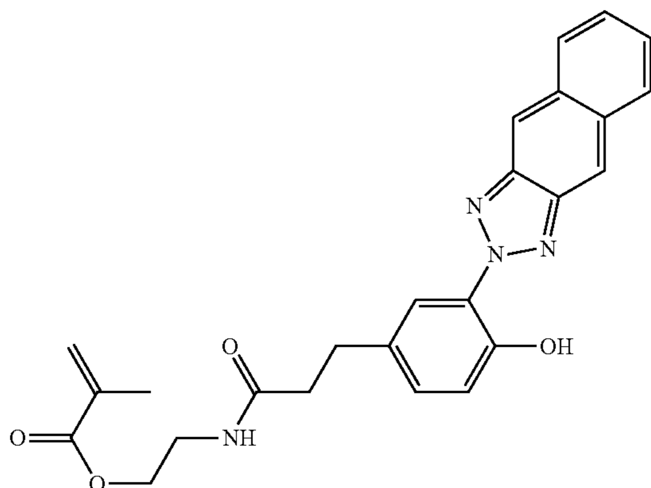
2-(3-(4-hydroxy-3-(2H-naphtho[2,3-d][1,2,3]triazol-2-yl)phenyl)propanamido)ethyl methacrylate
