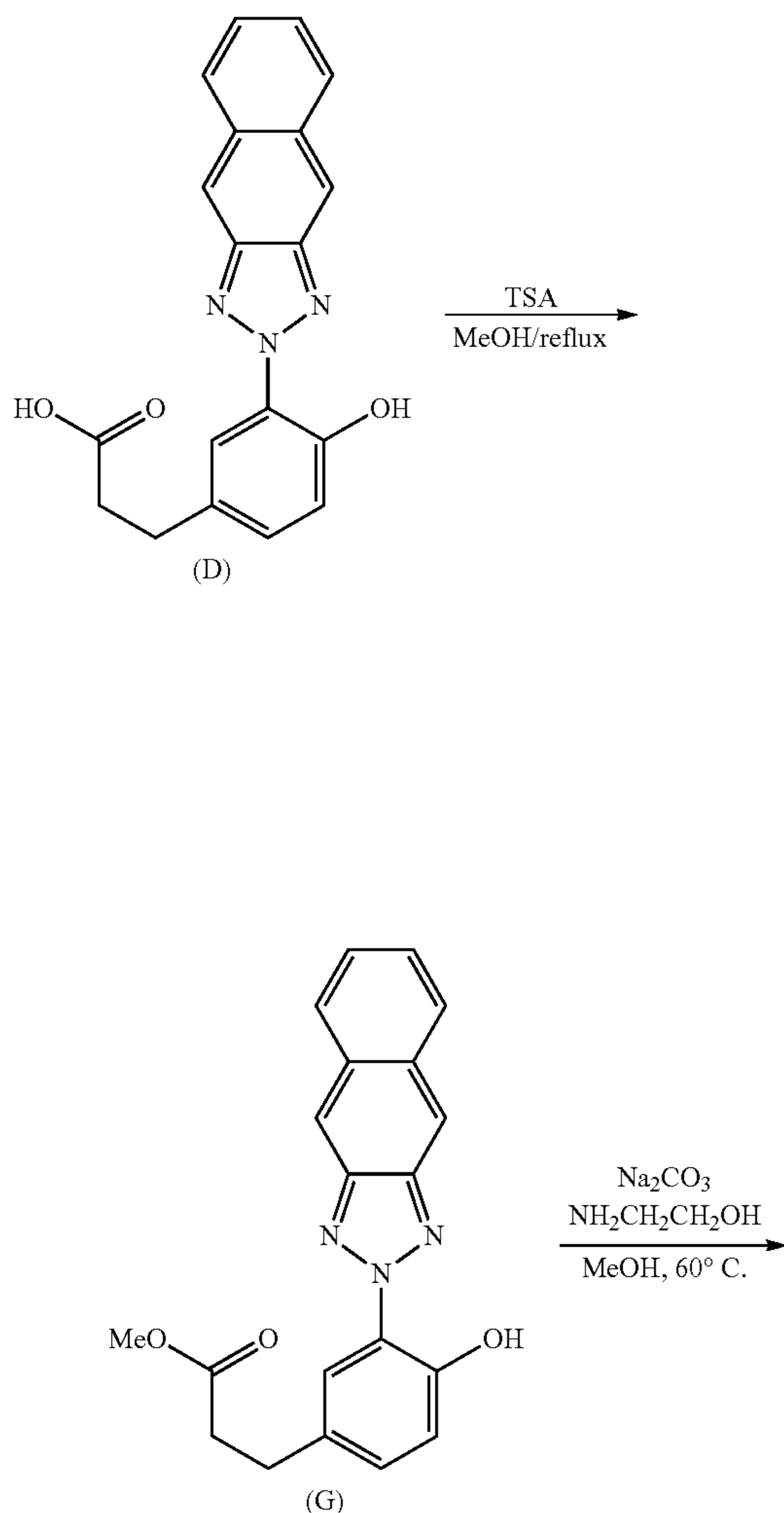
Scheme 3
