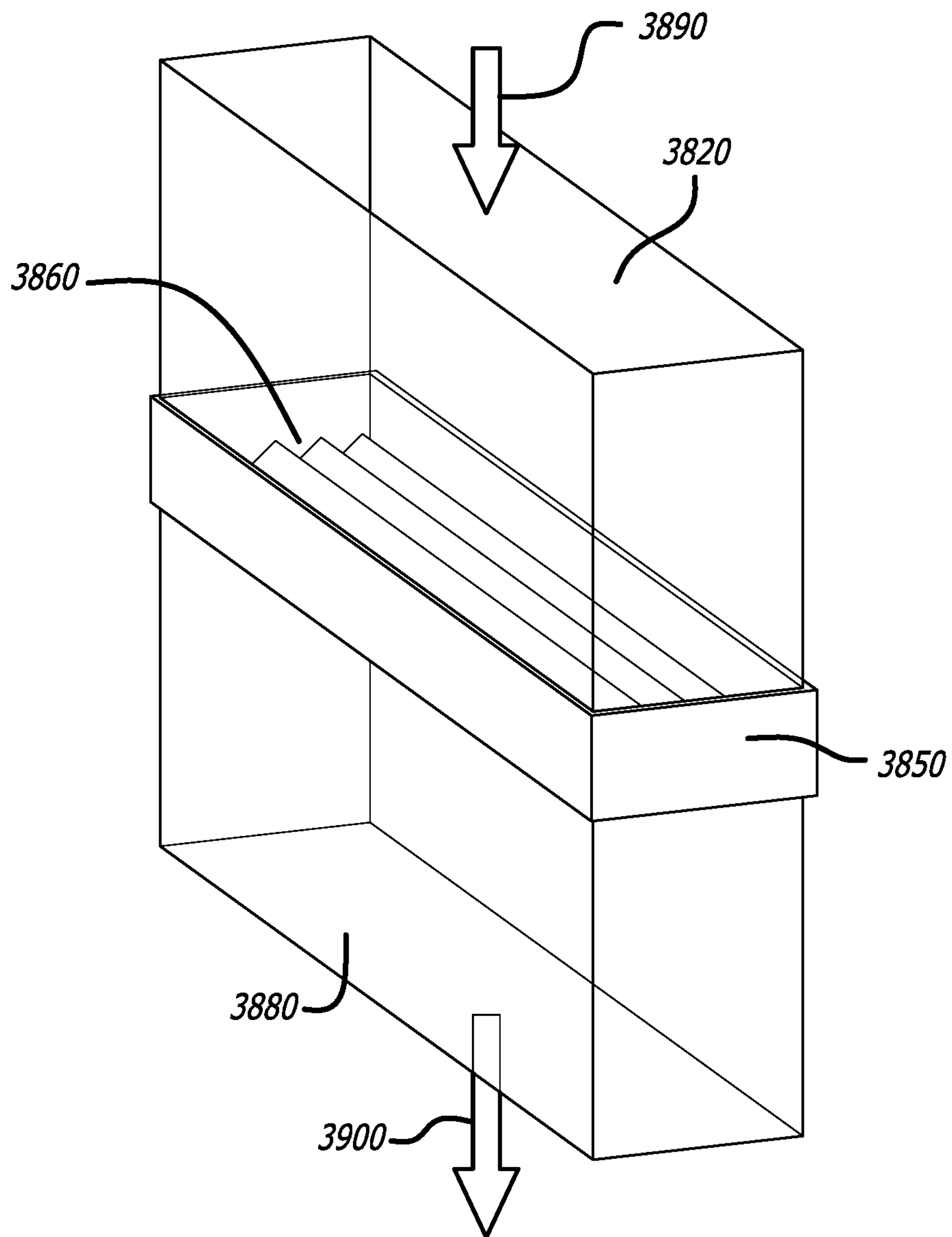
FIG. 55 (Prior Art)
