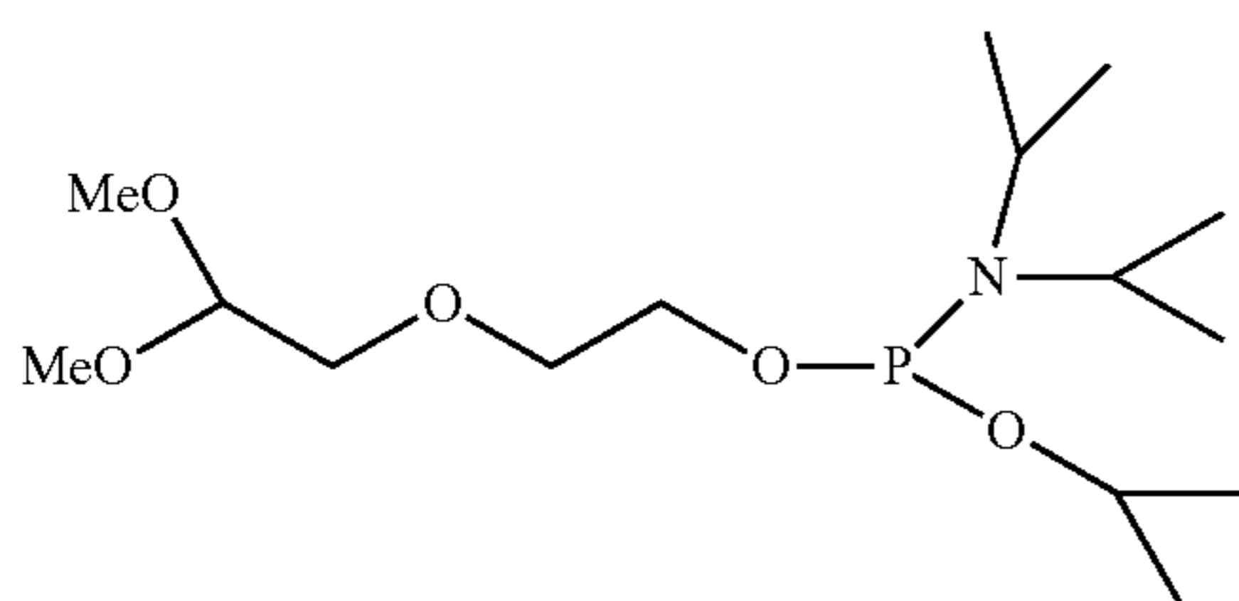
2-(2,2-Dimethoxy-ethoxy)-ethanol
