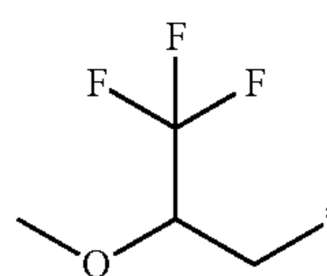
3,3,3-trifluoro-2-methoxypropyl
