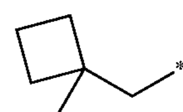
1-methylcyclobutylmethyl
