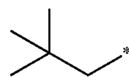
2,2-dimethylpropyl
