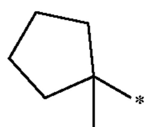
1-methylcyclopentyl
