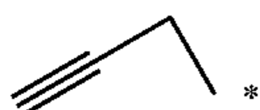
prop-2-yn-1-yl
