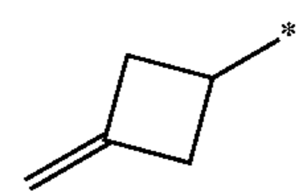
3-methylidenecyclobutyl
