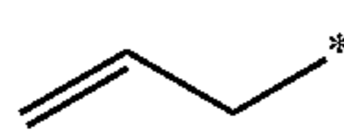
allyl
