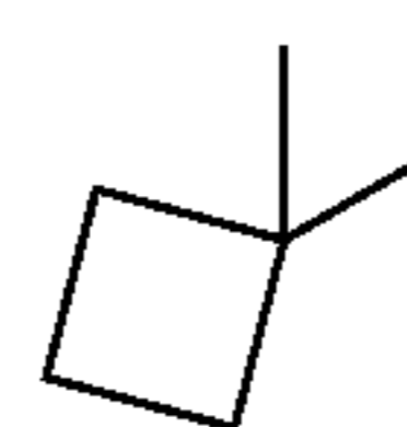
1-methylcyclobutyl
