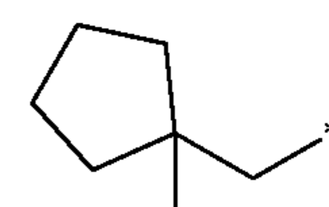
1-methylcyclopentylmethyl
