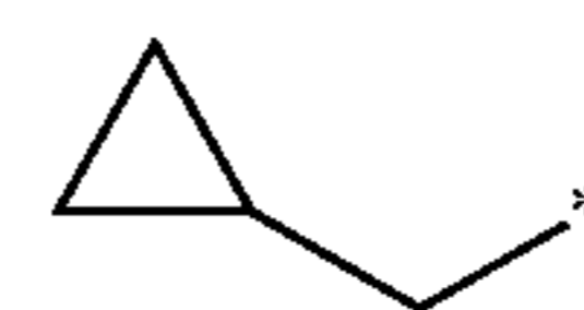
cyclopropylmethyl
