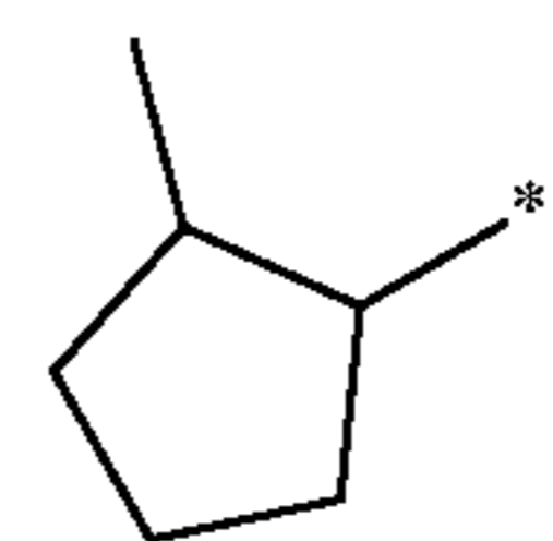
2-methylcyclopentyl
