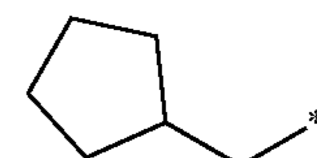
cyclopentylmethyl
