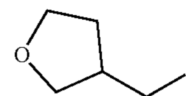
Tetrahydrofuran-3-ylmethyl
