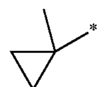
1-methylcyclopropyl
