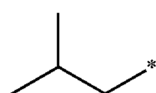
2-methylpropyl
