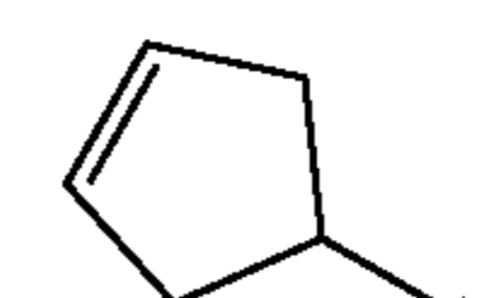
cyclopent-3-en-1-yl
