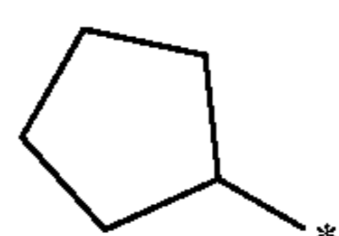
cyclopentyl
