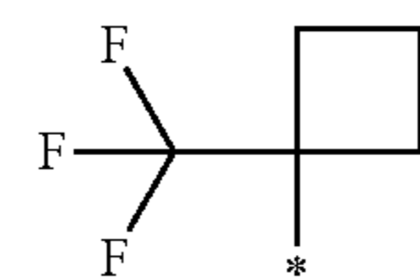
1-trifluoromethylcyclobutyl
