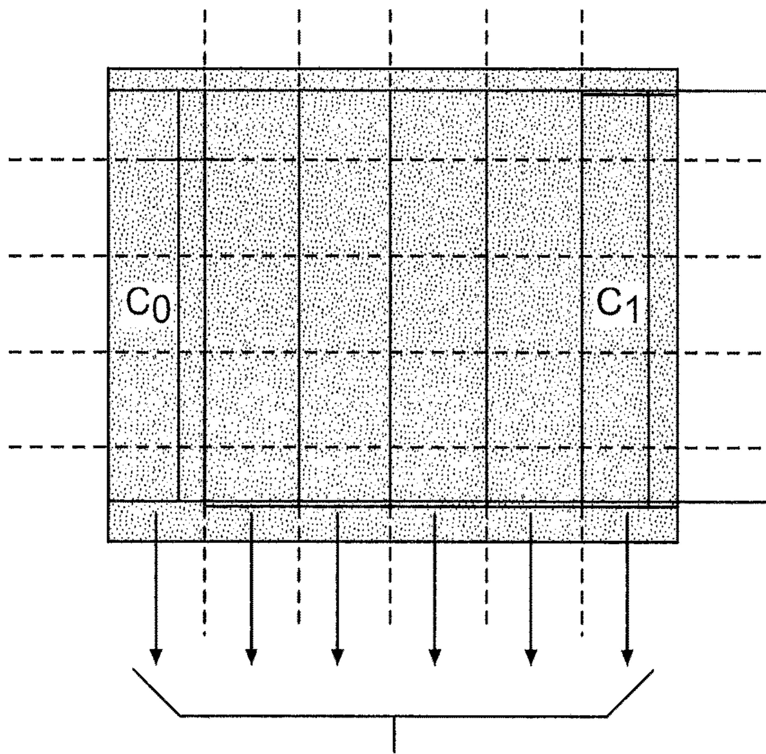
ASYNCHRONOUS (PARALLEL) READ OPERATIONS, ONE FOR EACH COLUMN STRIP
