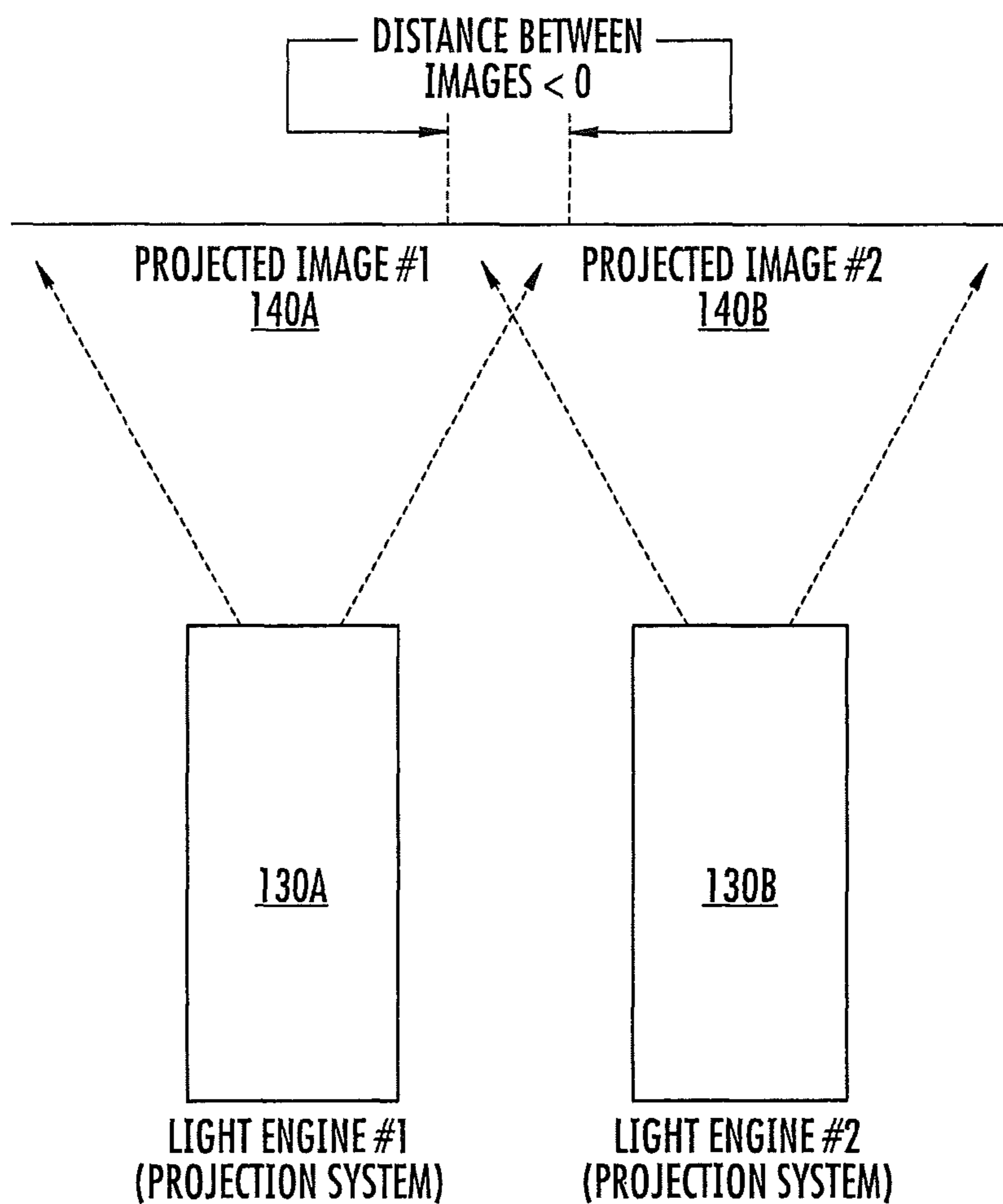
SIDE VIEW TWO LIGHT ENGINES
