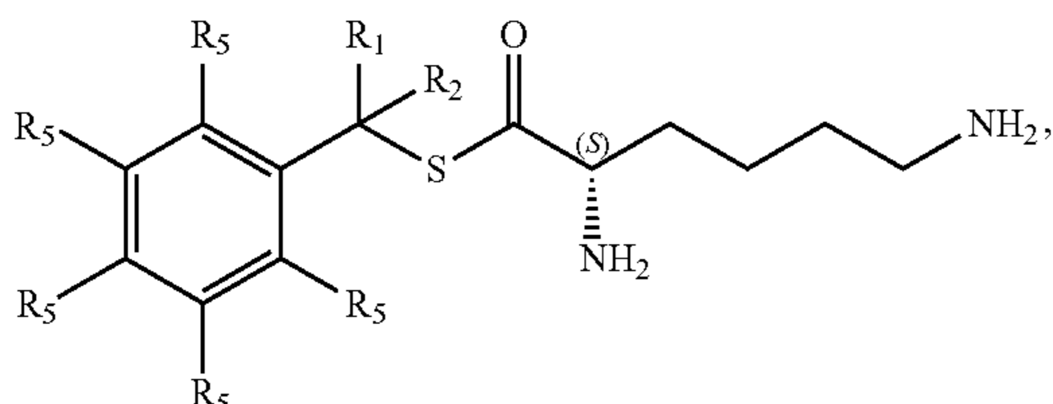
R_6 = Amino Acyl of lysine
