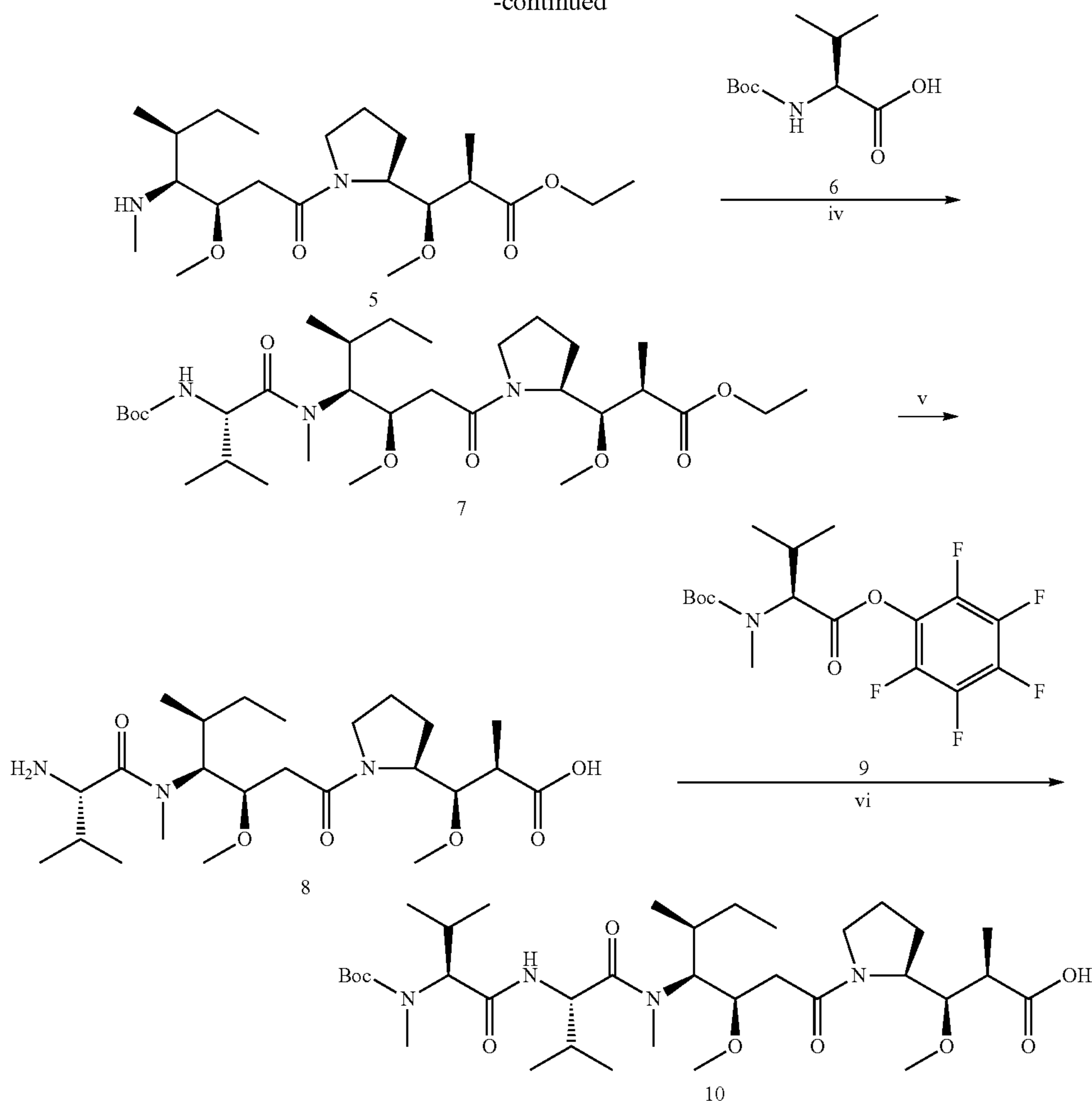
Scheme I. Reagents and conditions: i. \text{SOCl}_2 , EtOH; ii. DEPC, TFA, DCM; iii. TFA, DCM; iv. BrOP, DCM, DIEA; v. TFA, DCM; iv. DIEA, DCM, HOBt.
