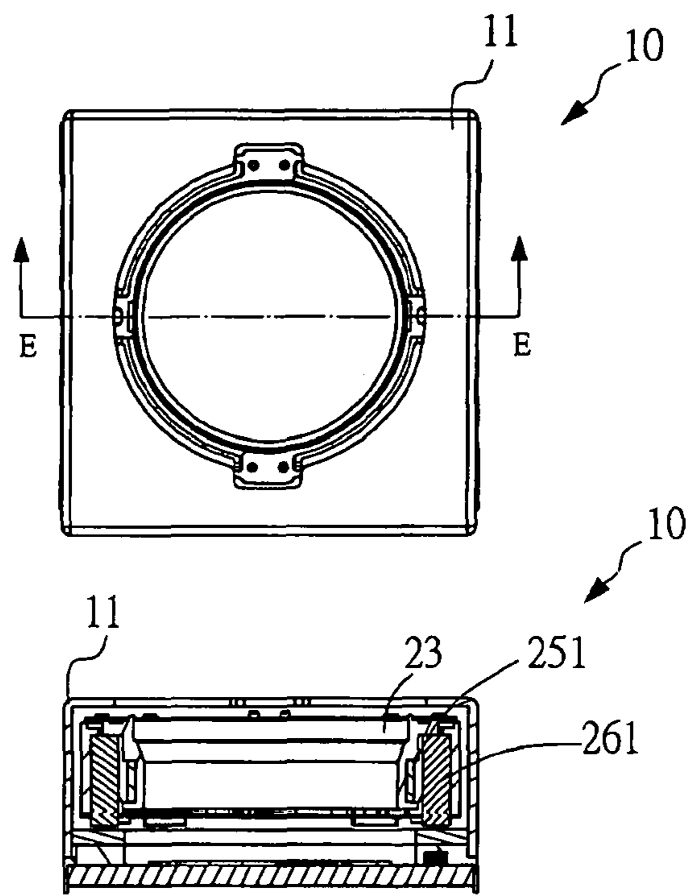
E-E Section
