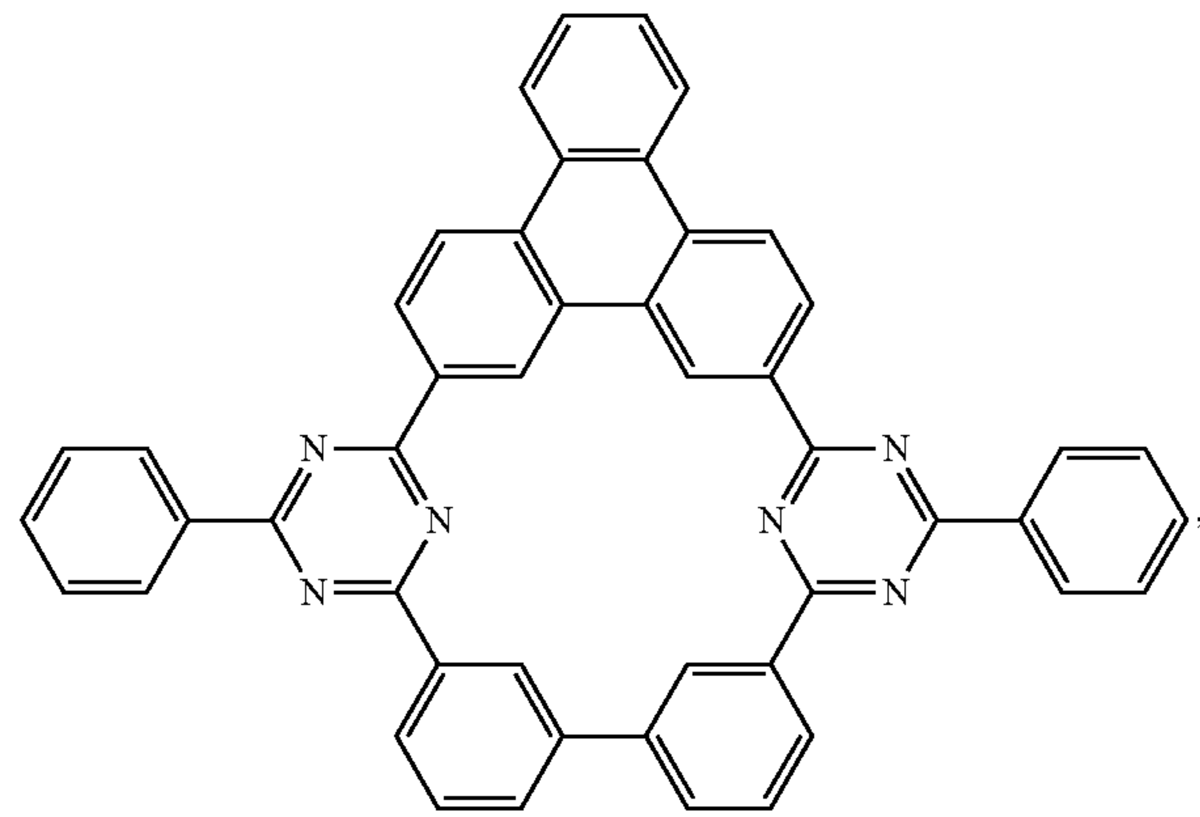
Compound 15
