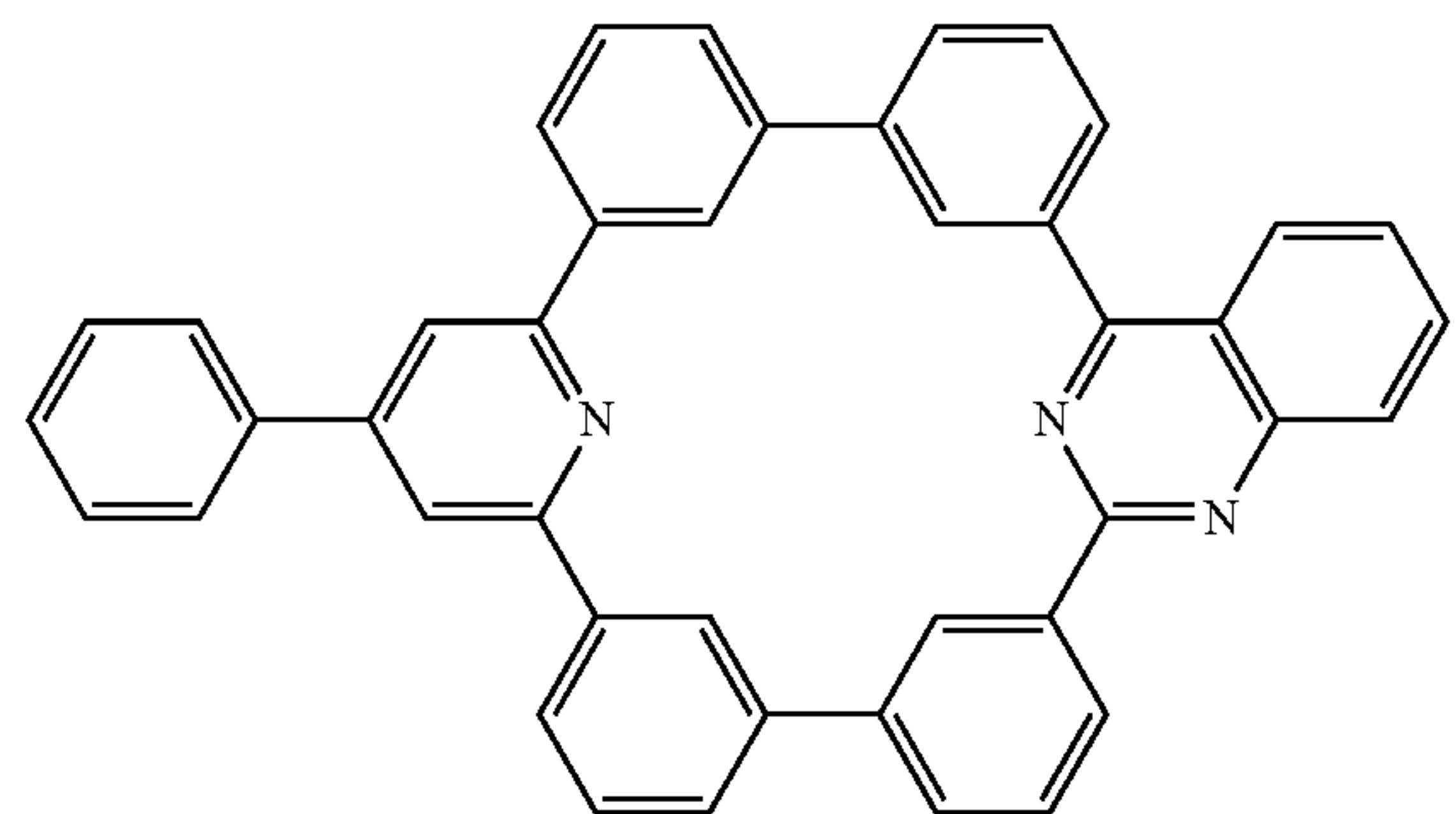
Compound 50
