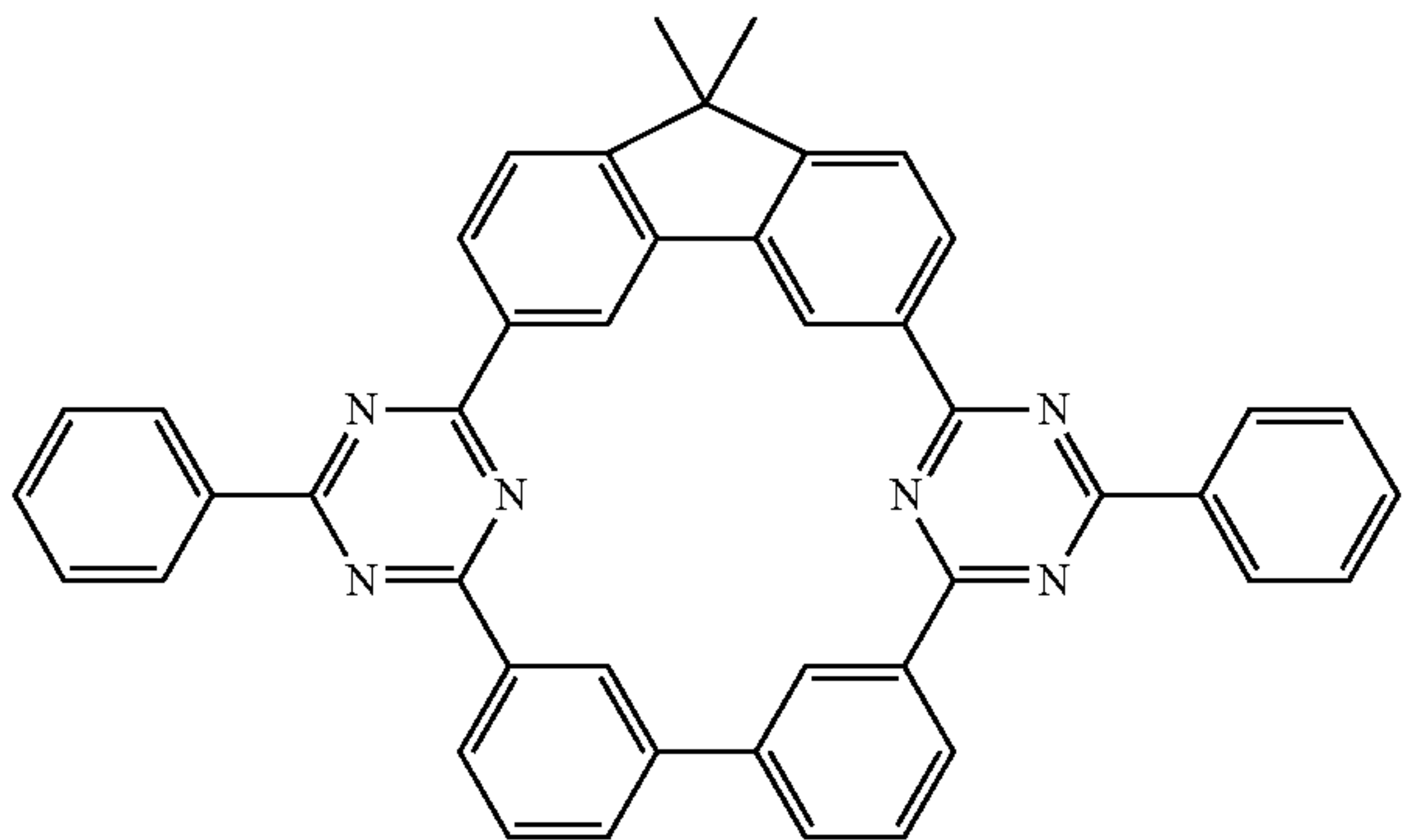
Compound 12
