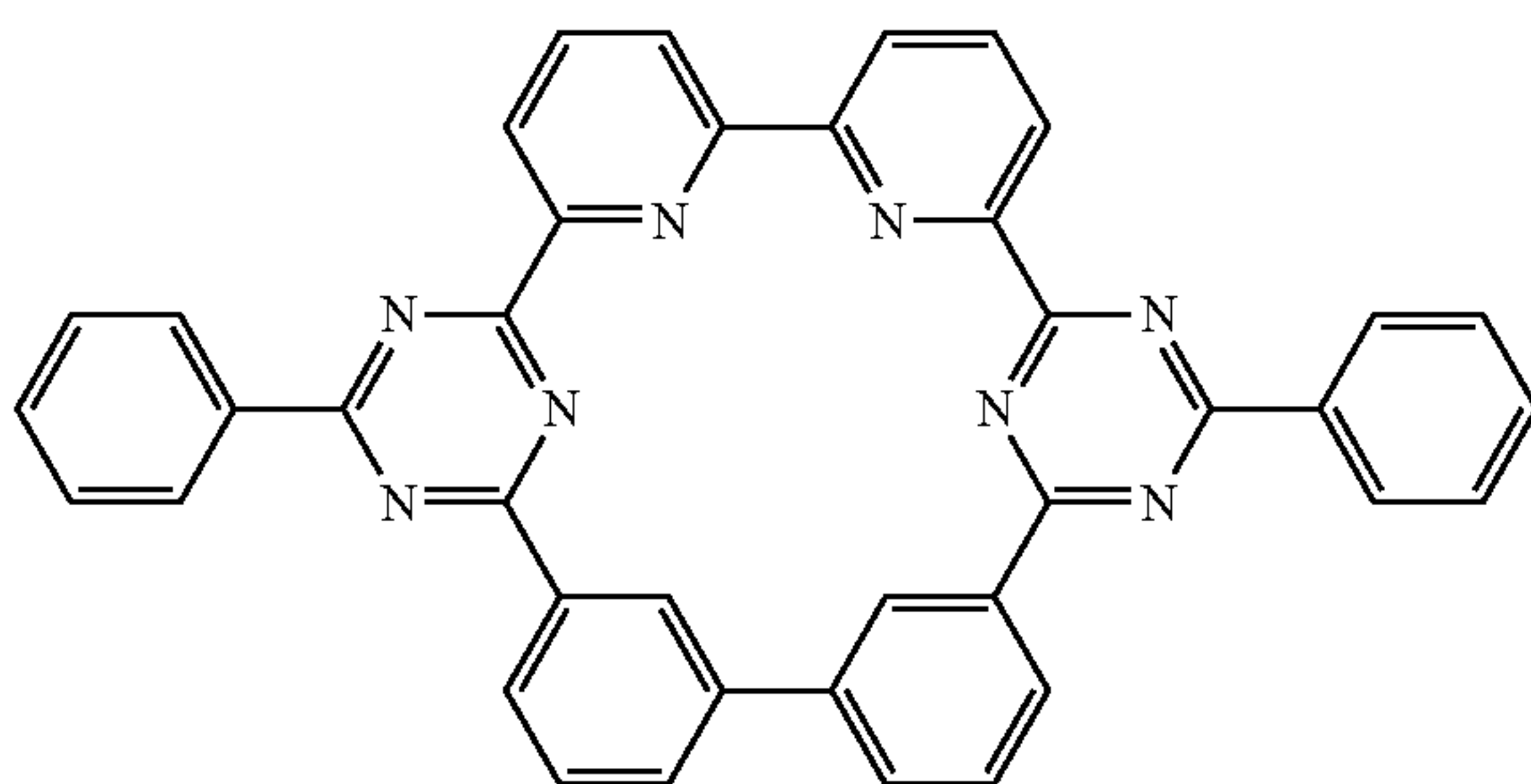
Compound 12
