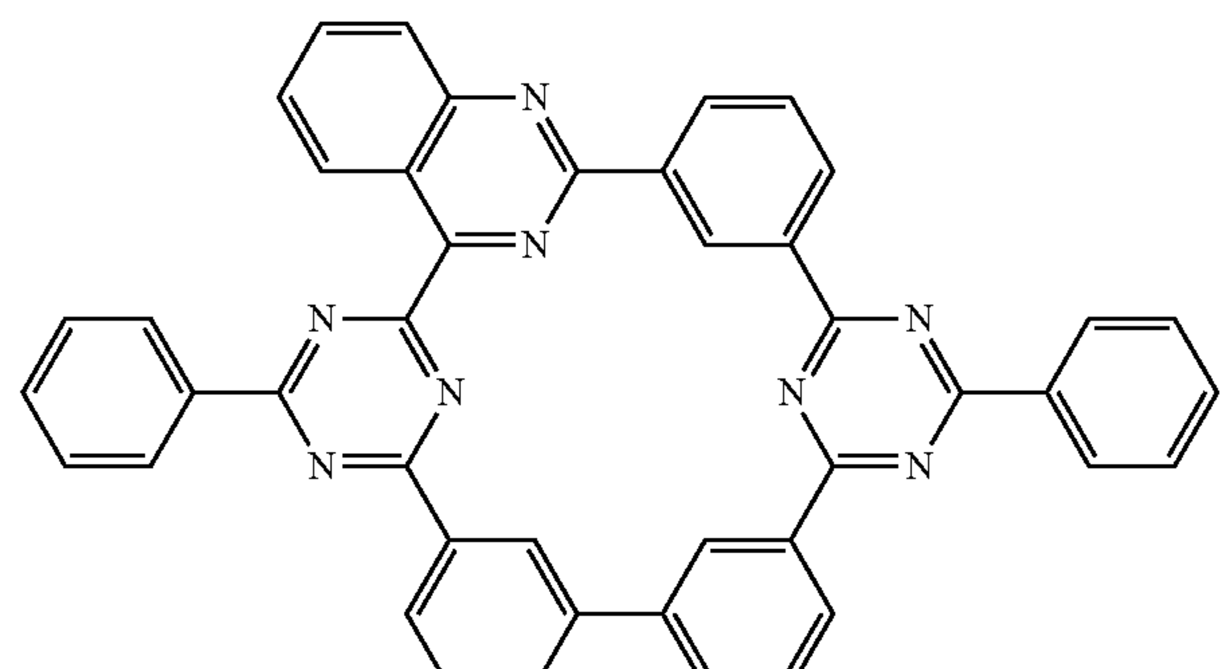
Compound 62
