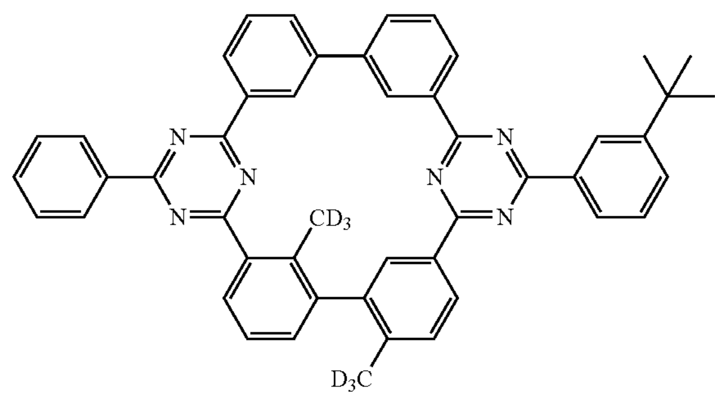
Compound 29
