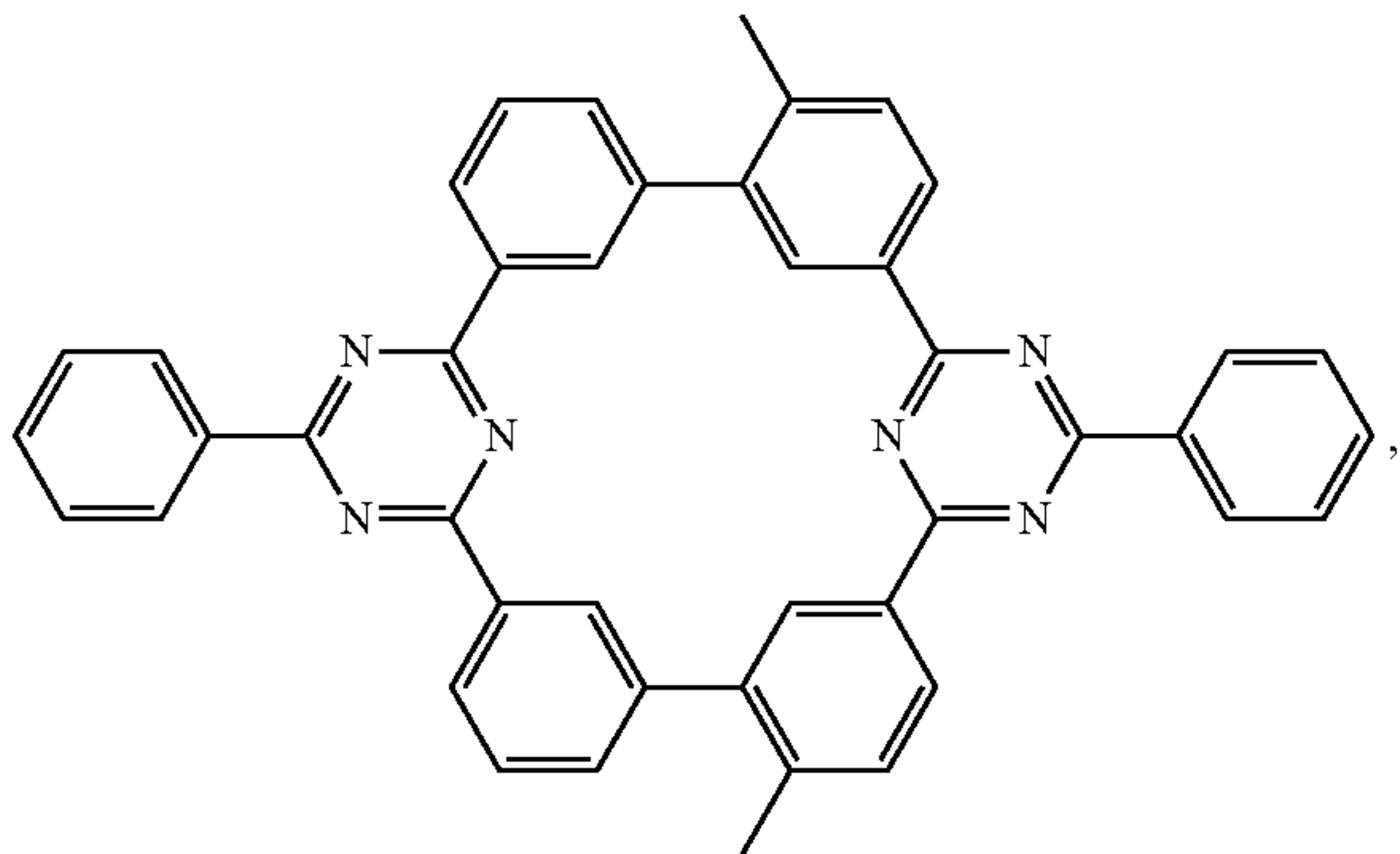
Compound 37
