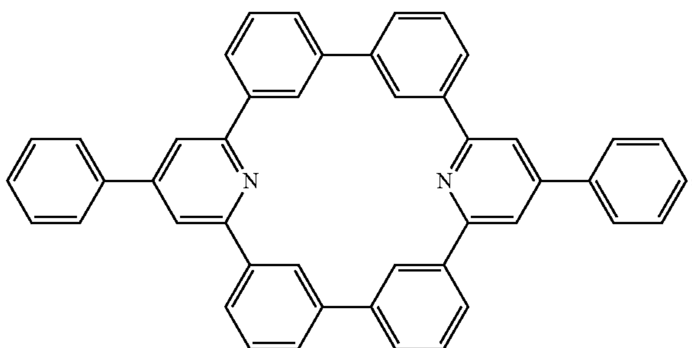
Compound 51
