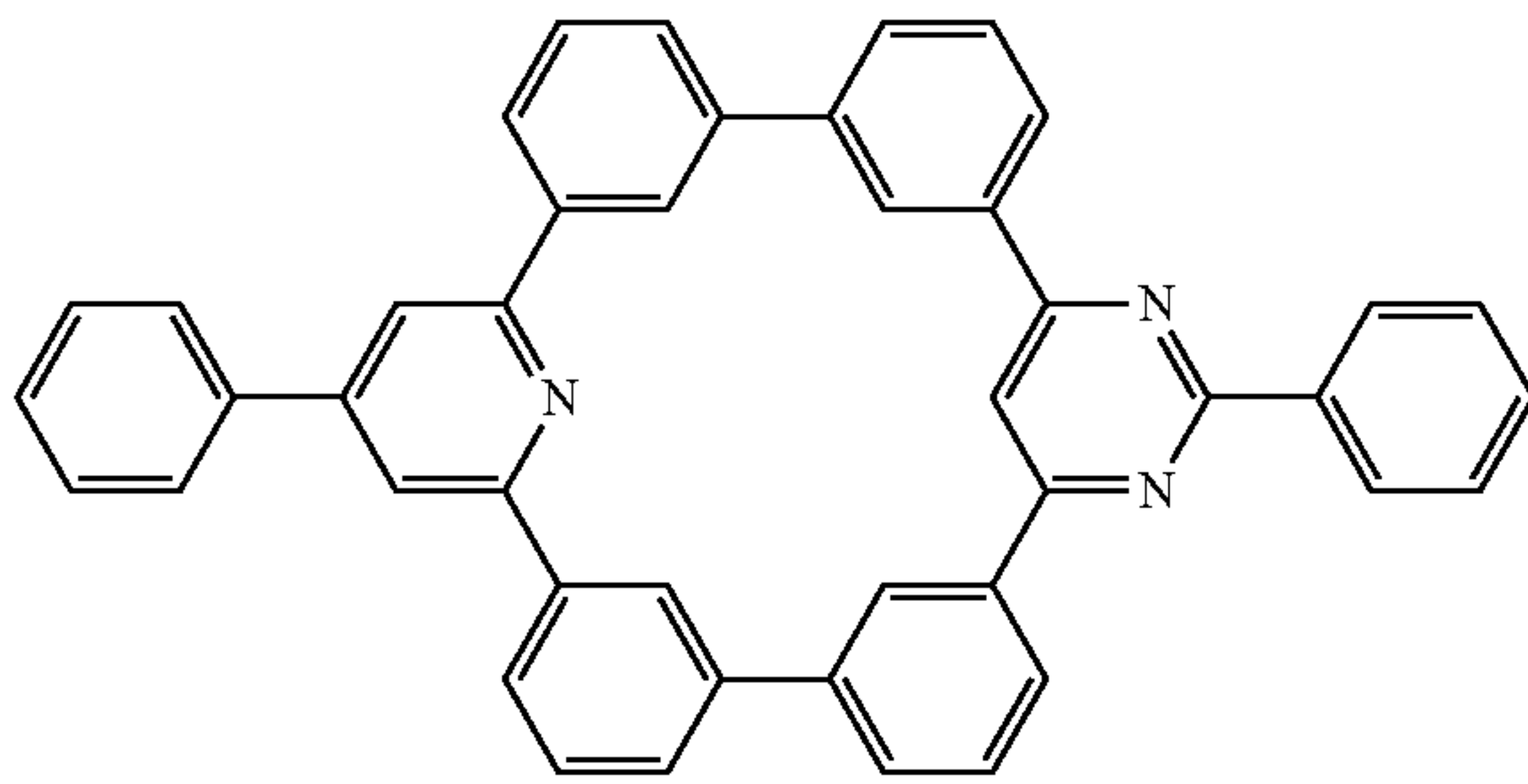
Compound 47
