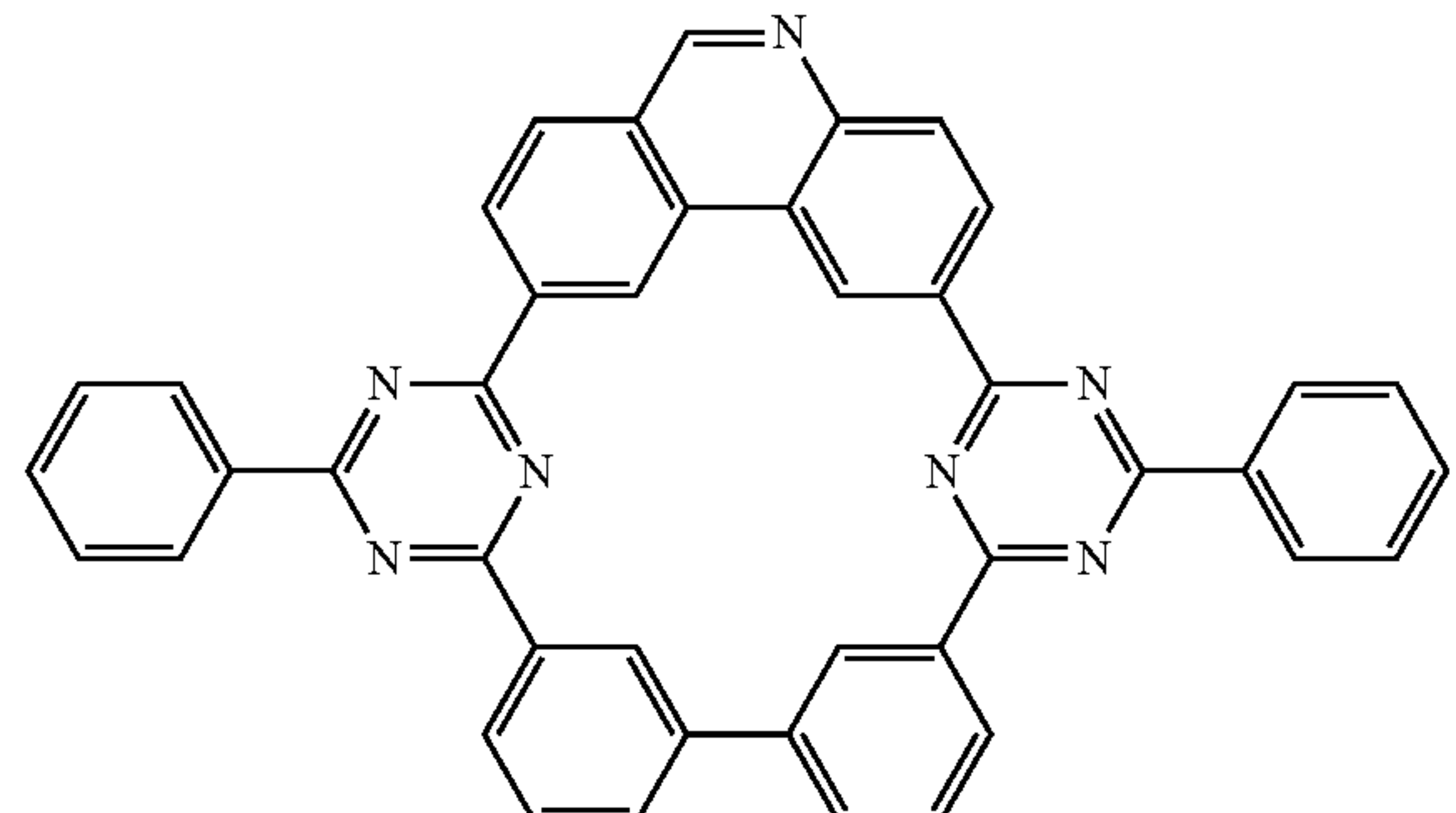
Compound 15
