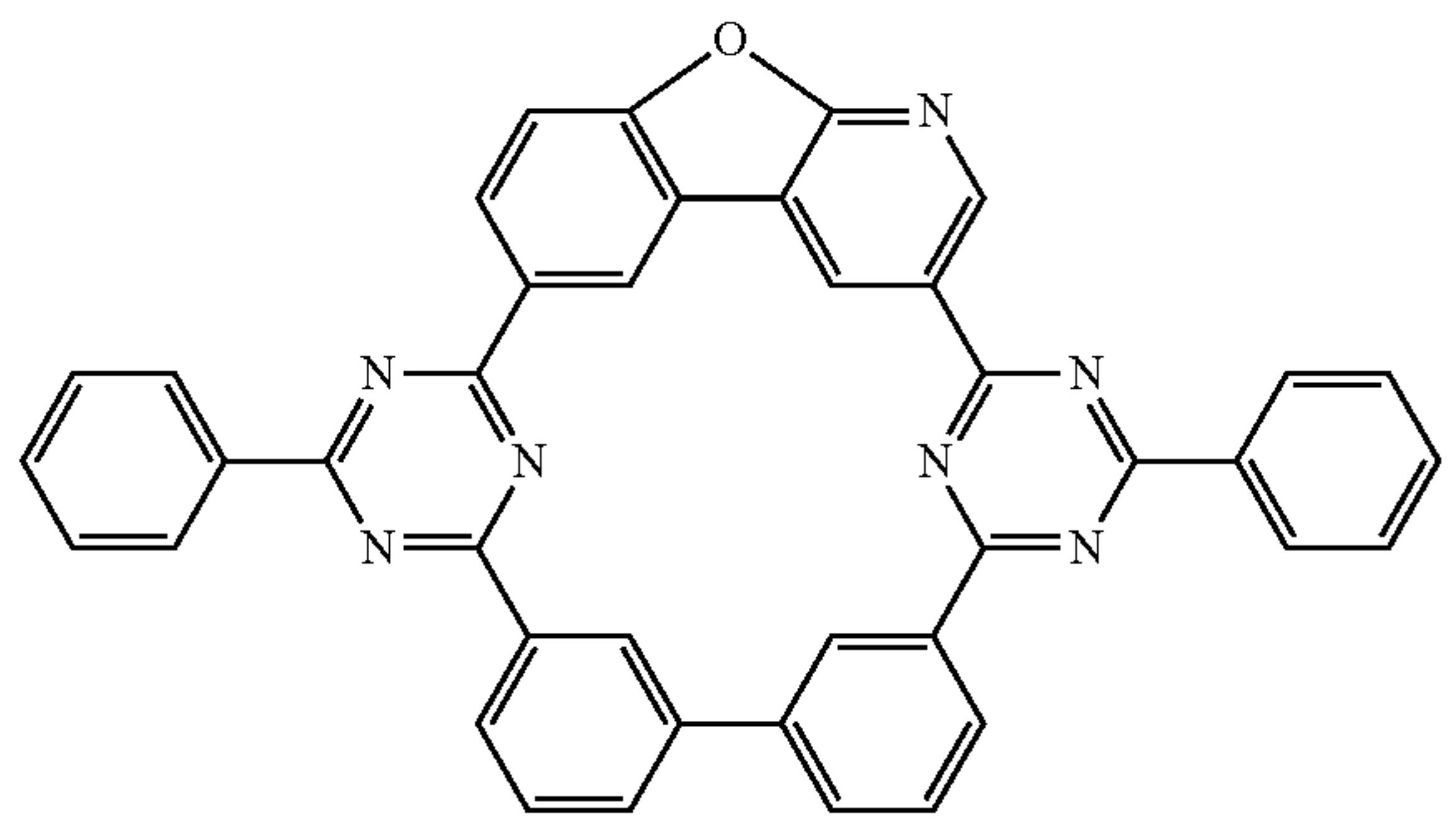
Compound 58
