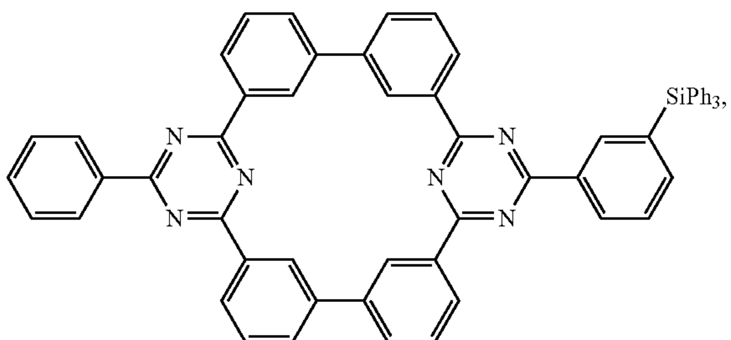
Compound 20
