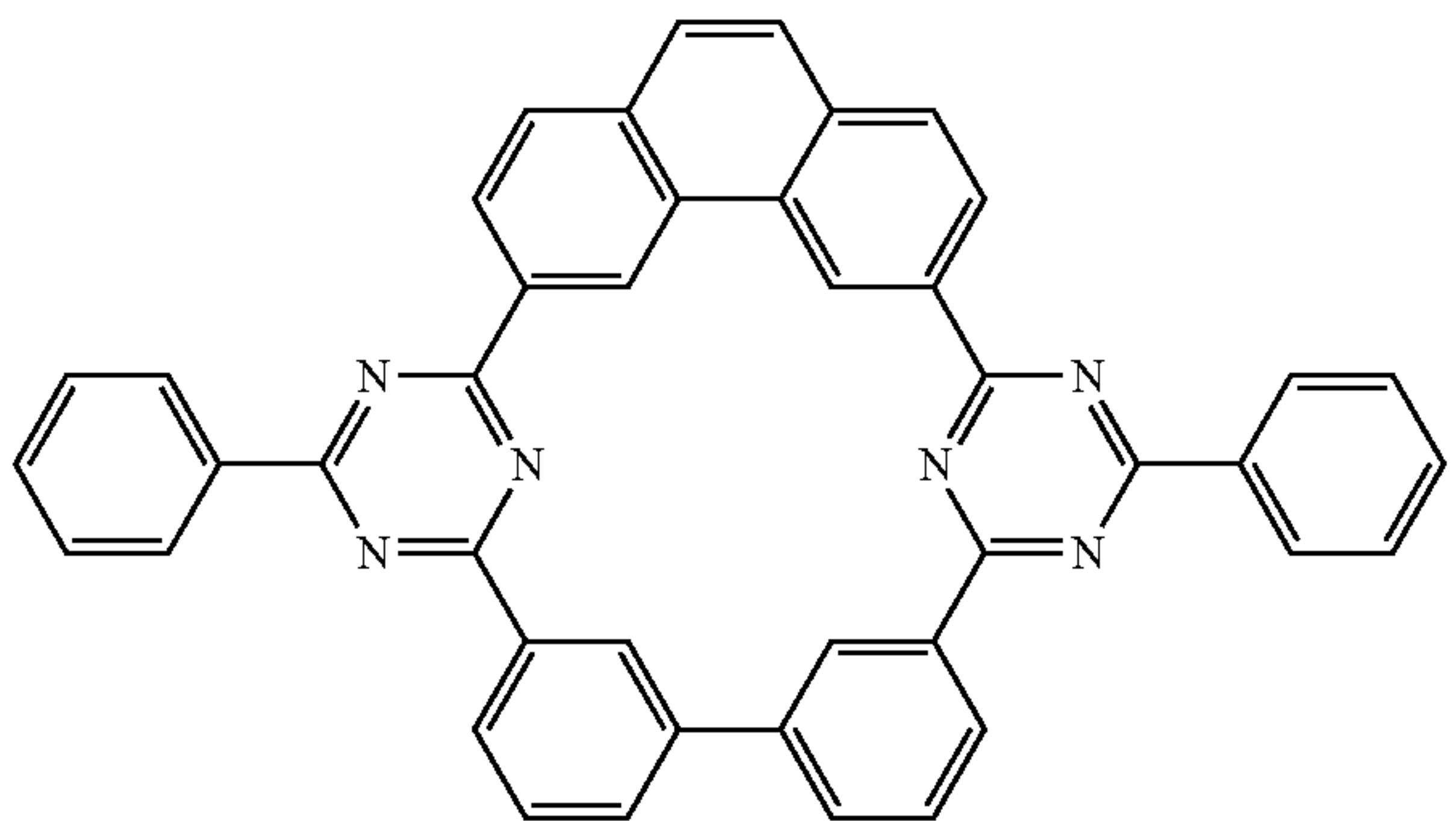
Compound 14
