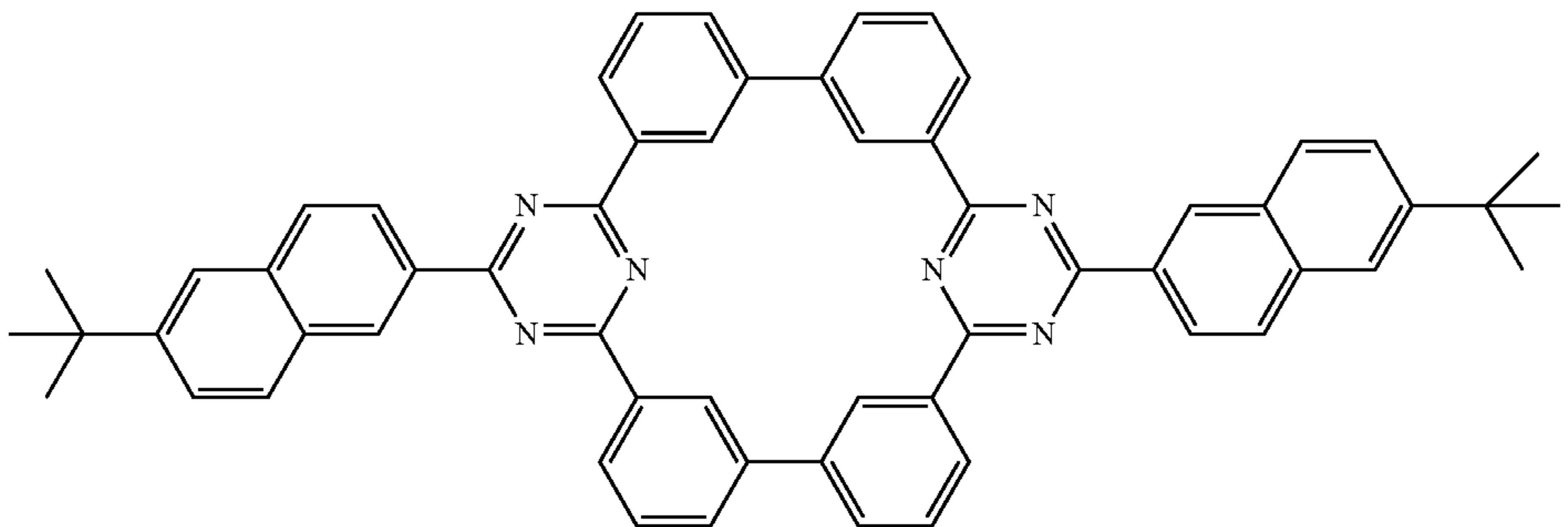
Compound 41
