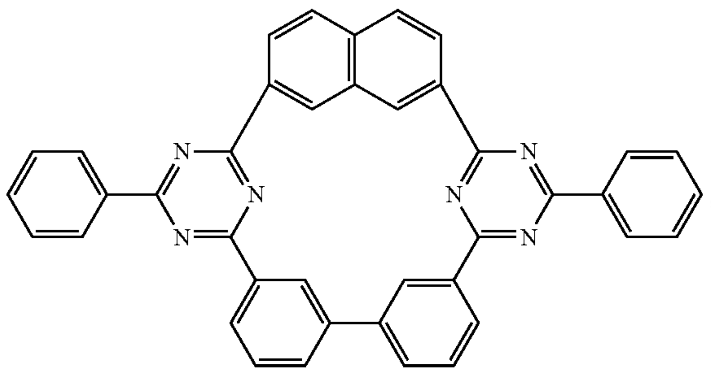
Compound 63
