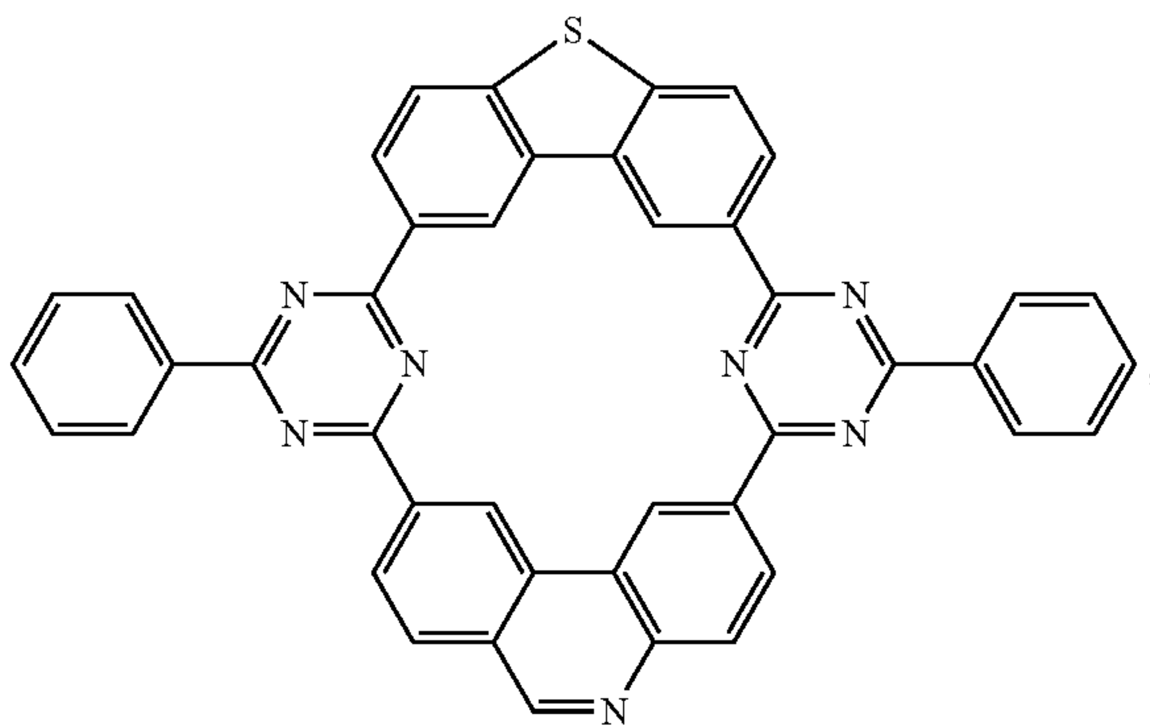
Compound 53
