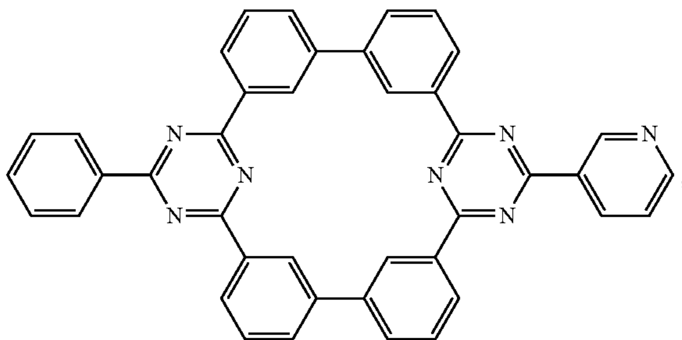
Compound 18
