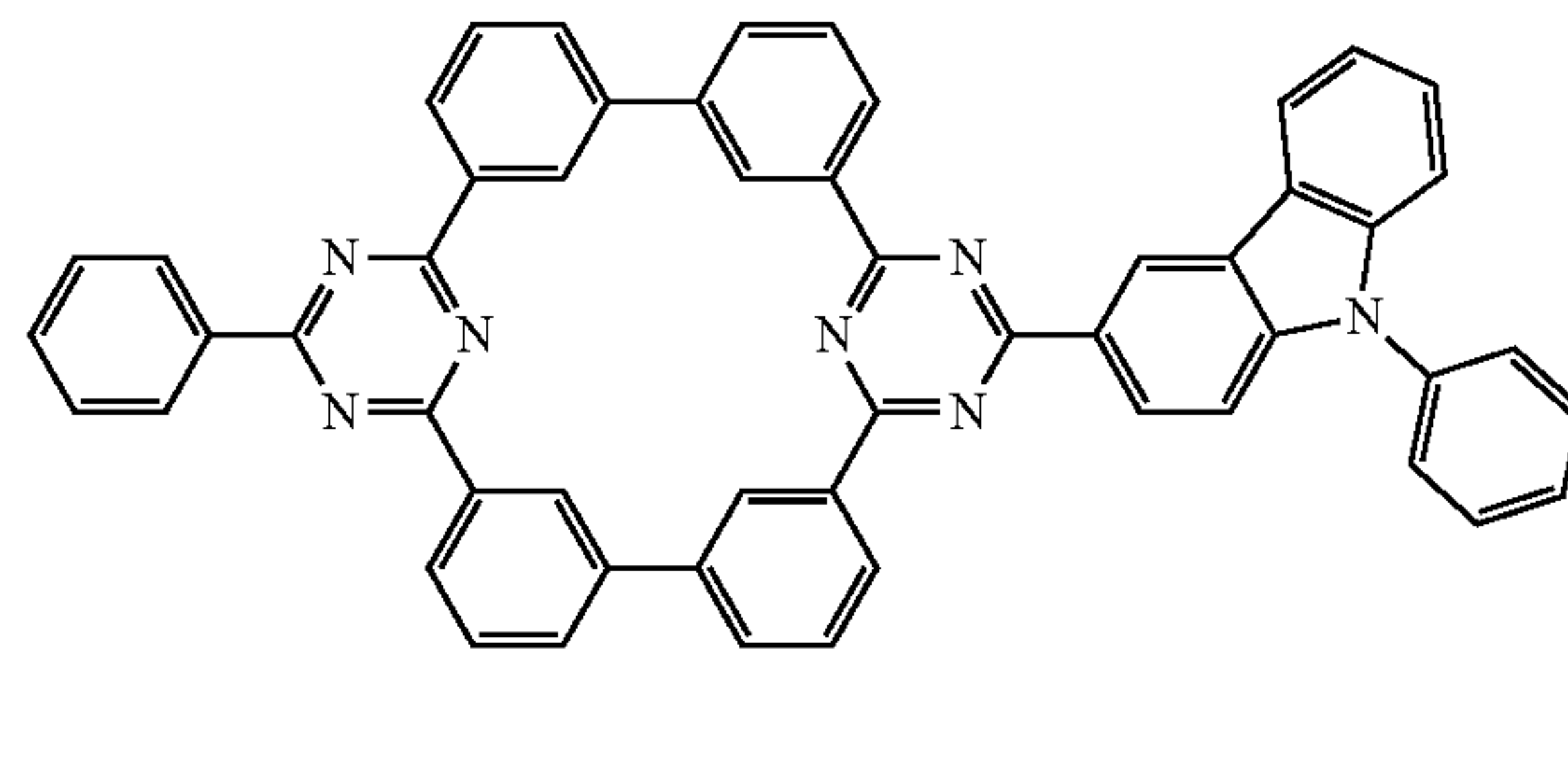
Compound 19
