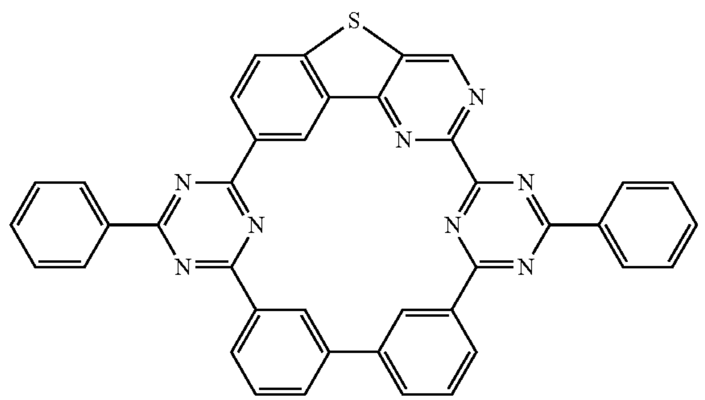
Compound 58
