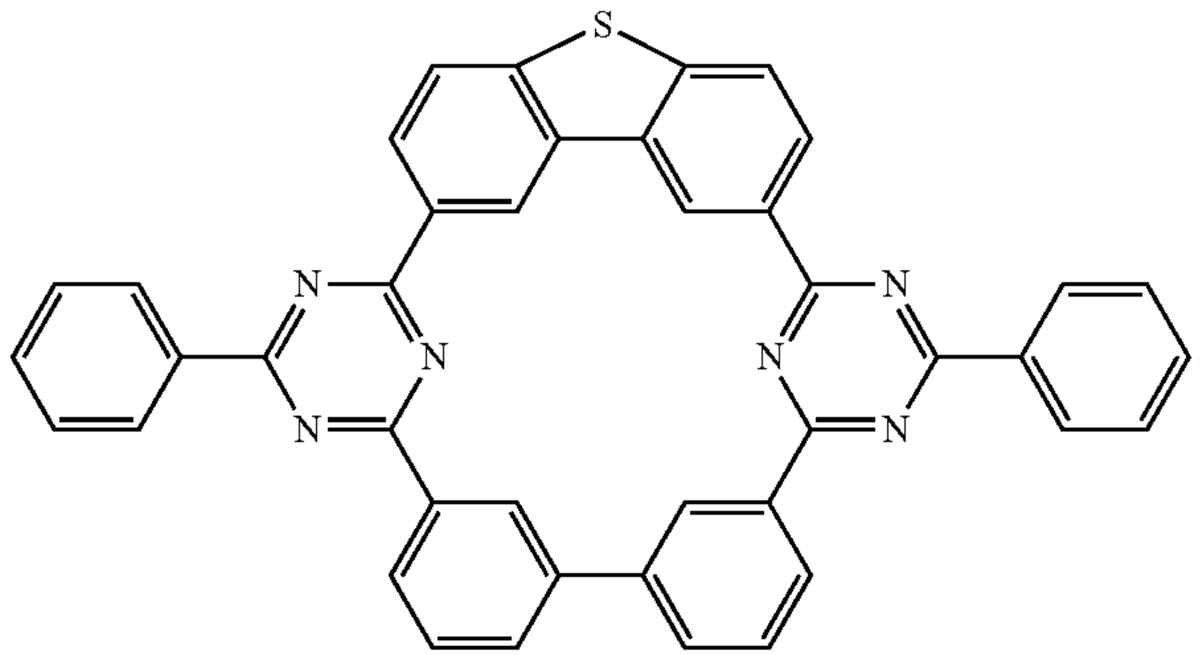
Compound 8
