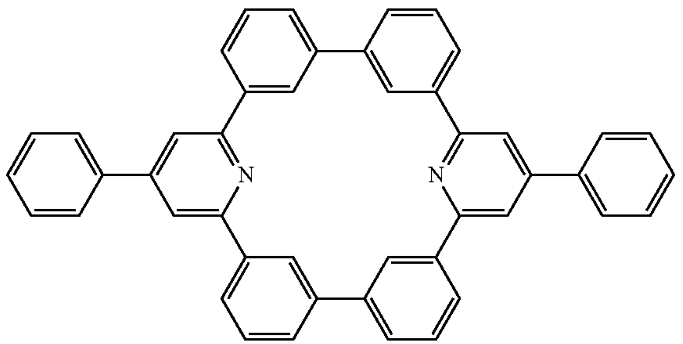
Compound 51
