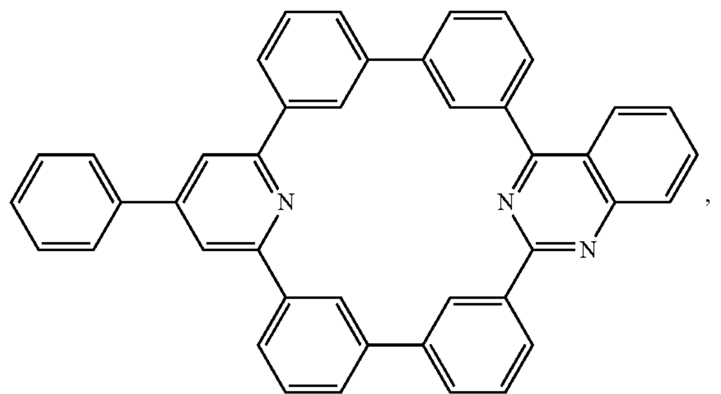
Compound 50
