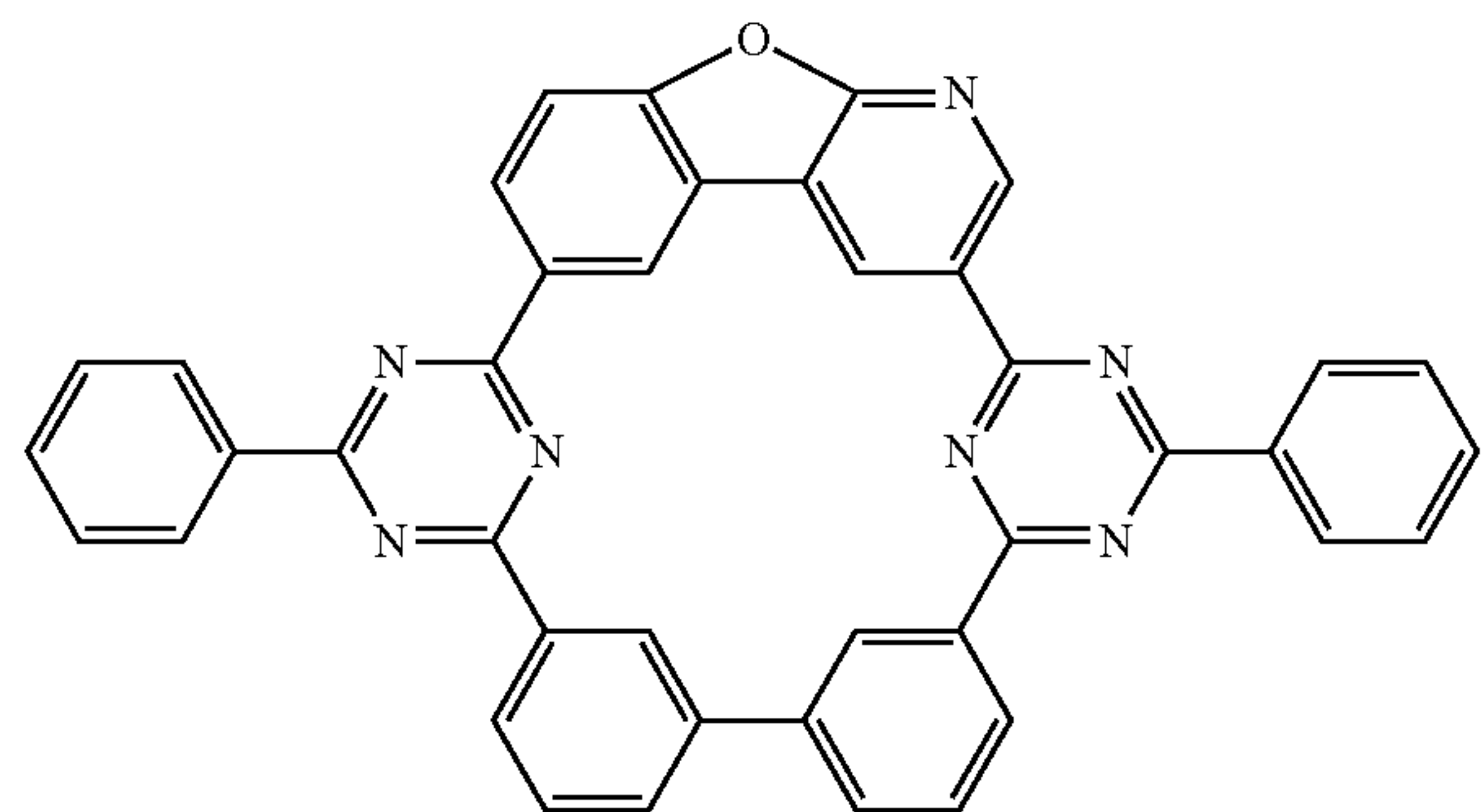
Compound 58
