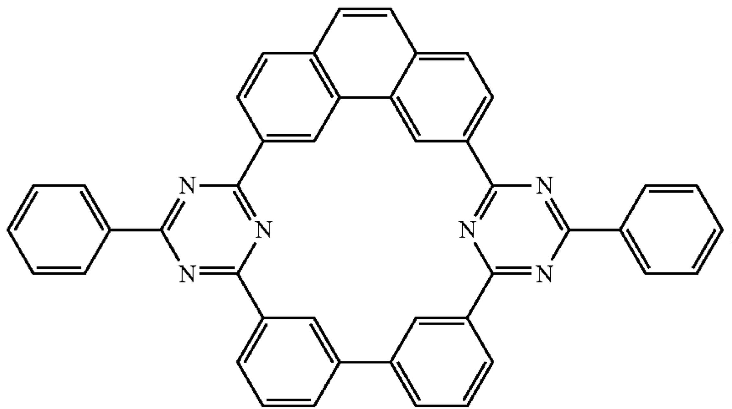
Compound 14
