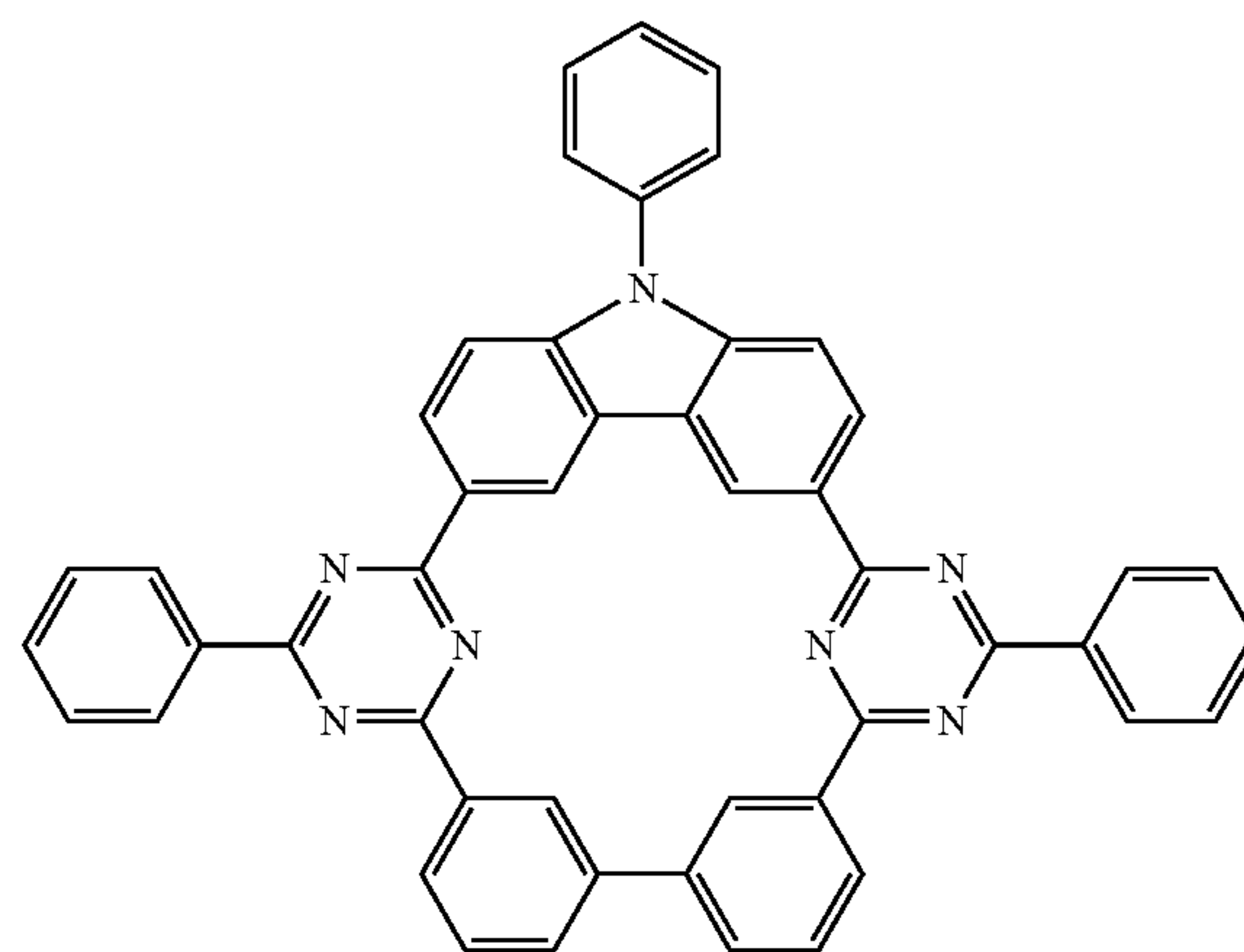
Compound 11
