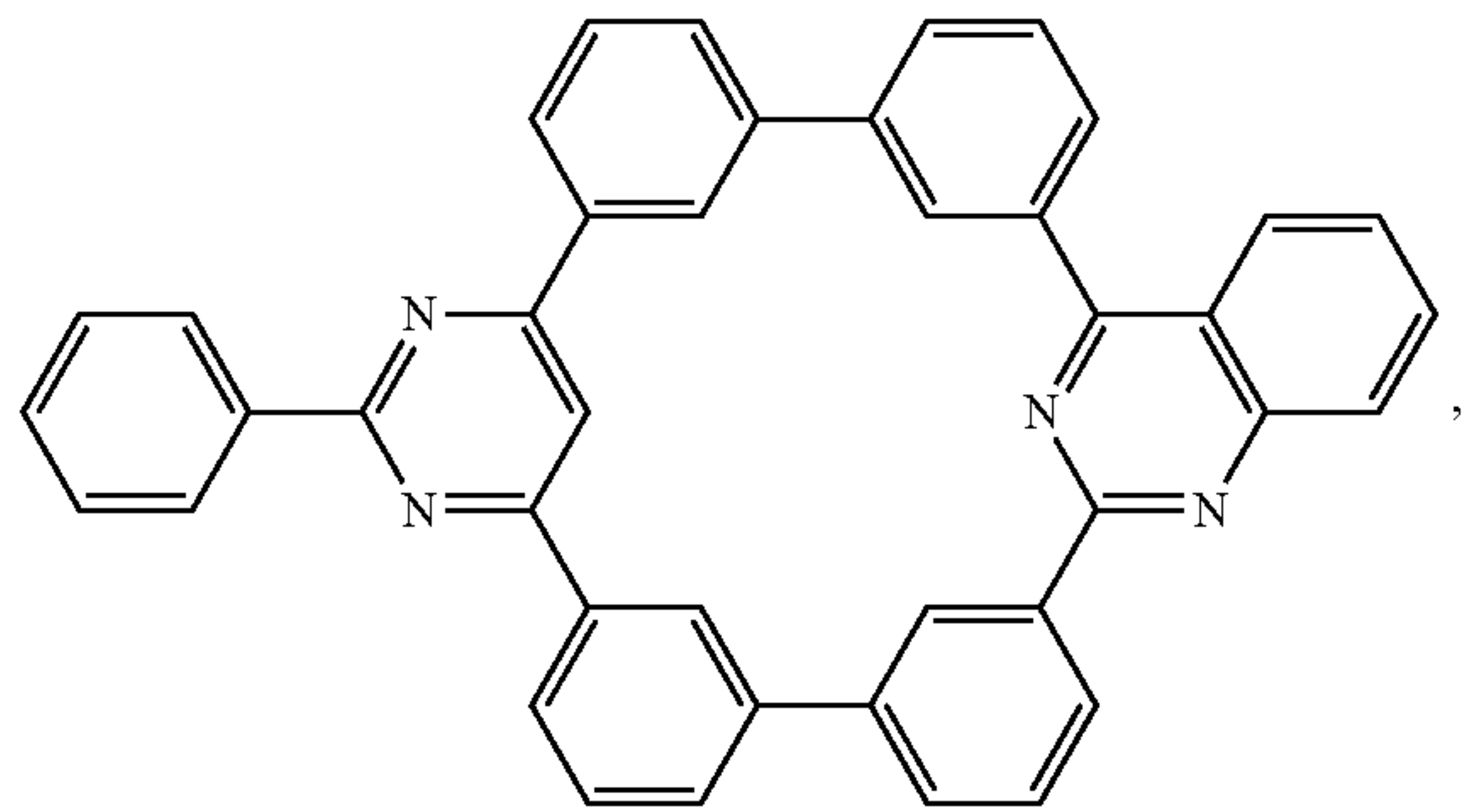
Compound 48
