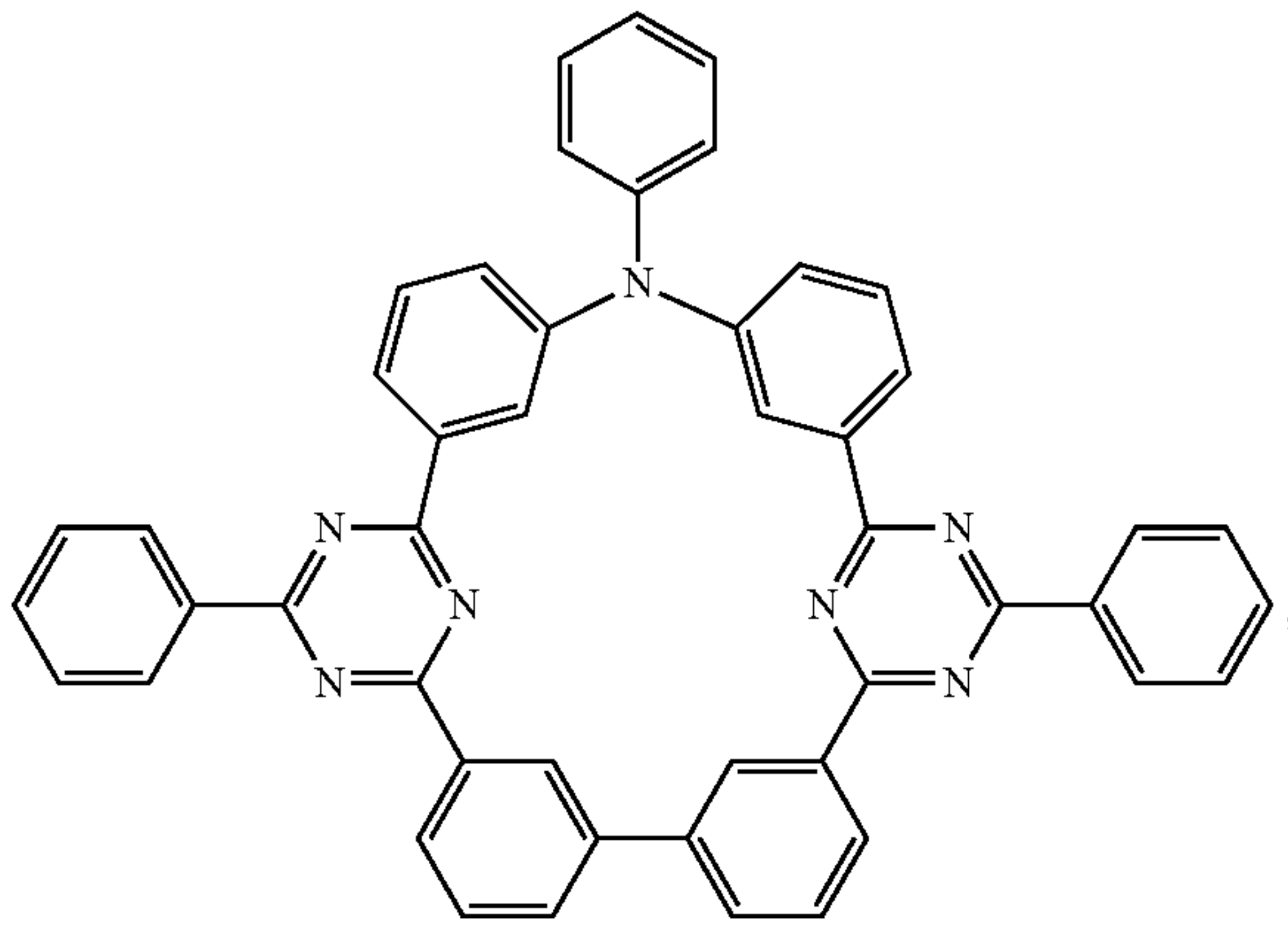
Compound 22
