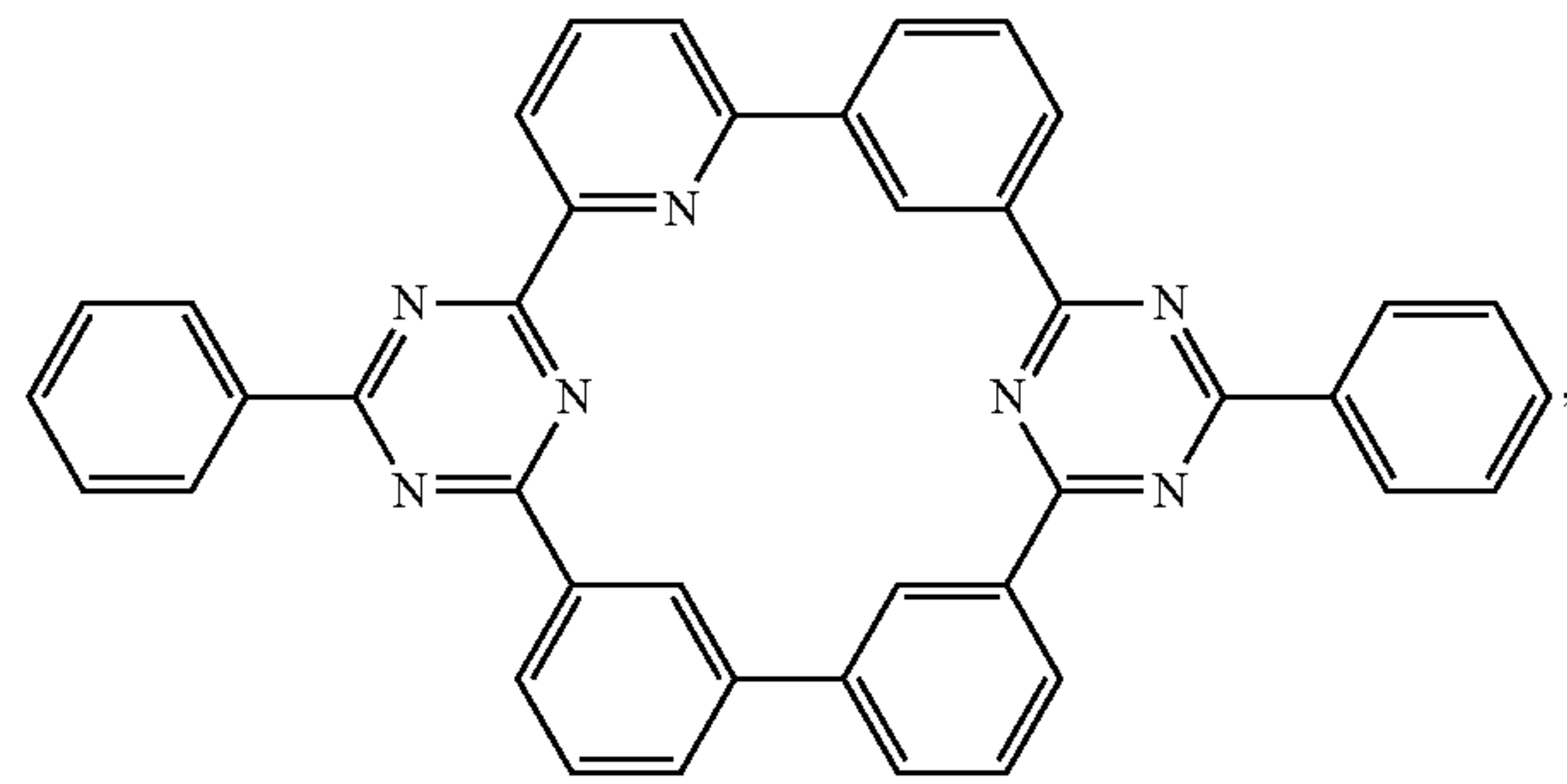
Compound 11
