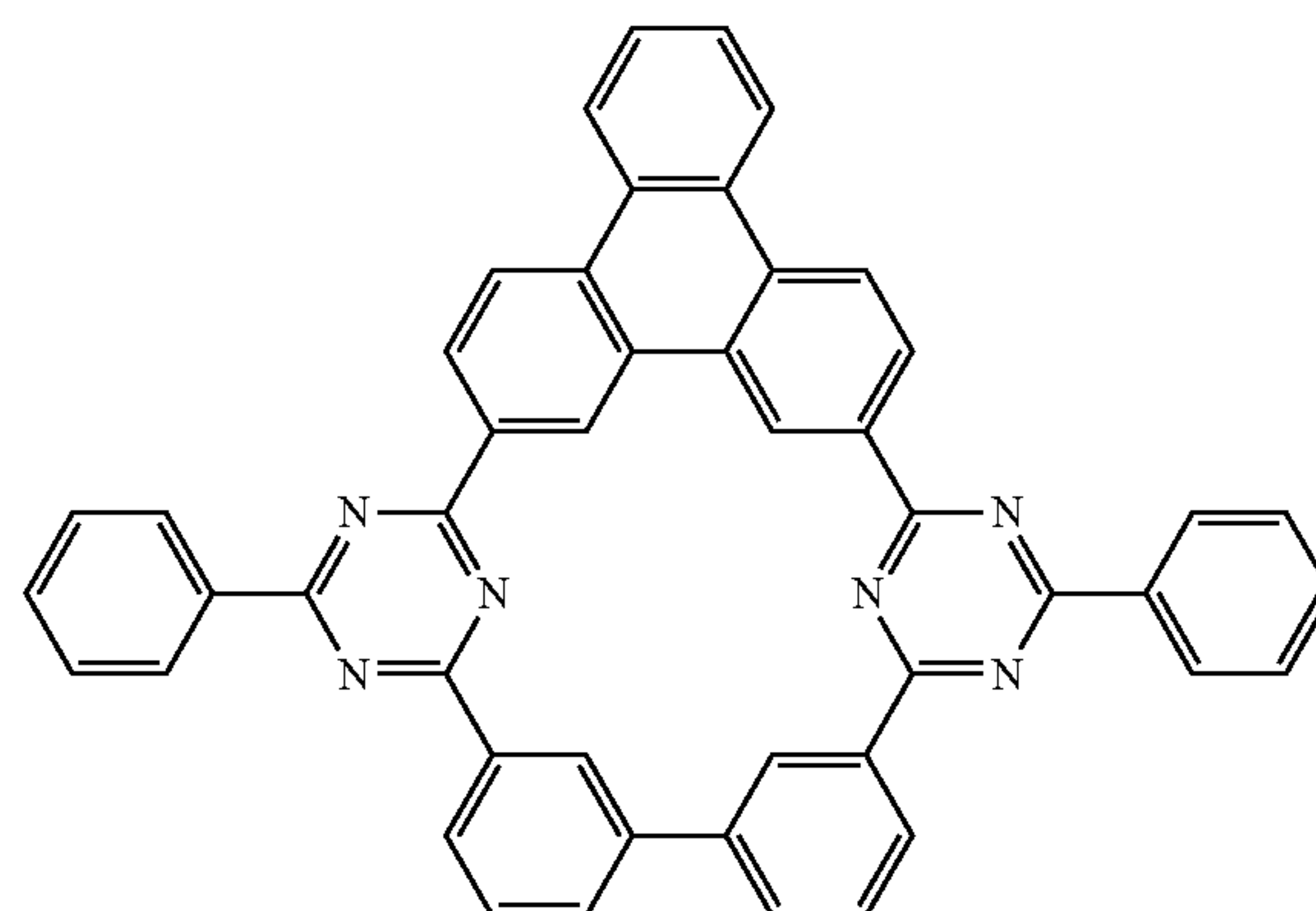
Compound 13
