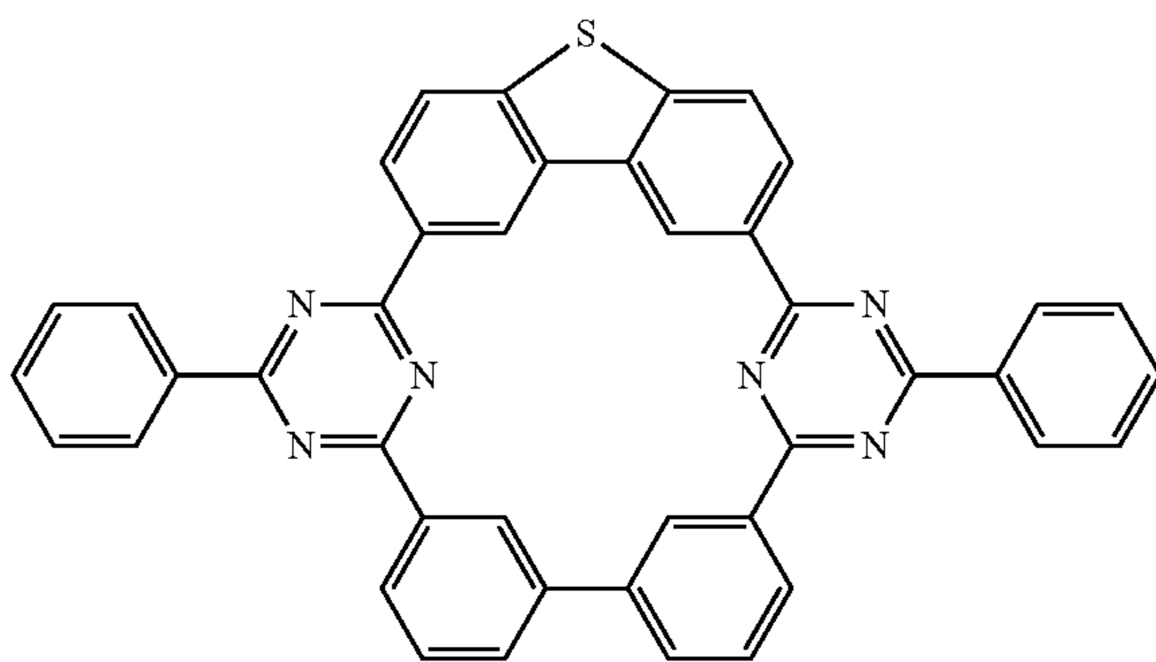
Compound 8
