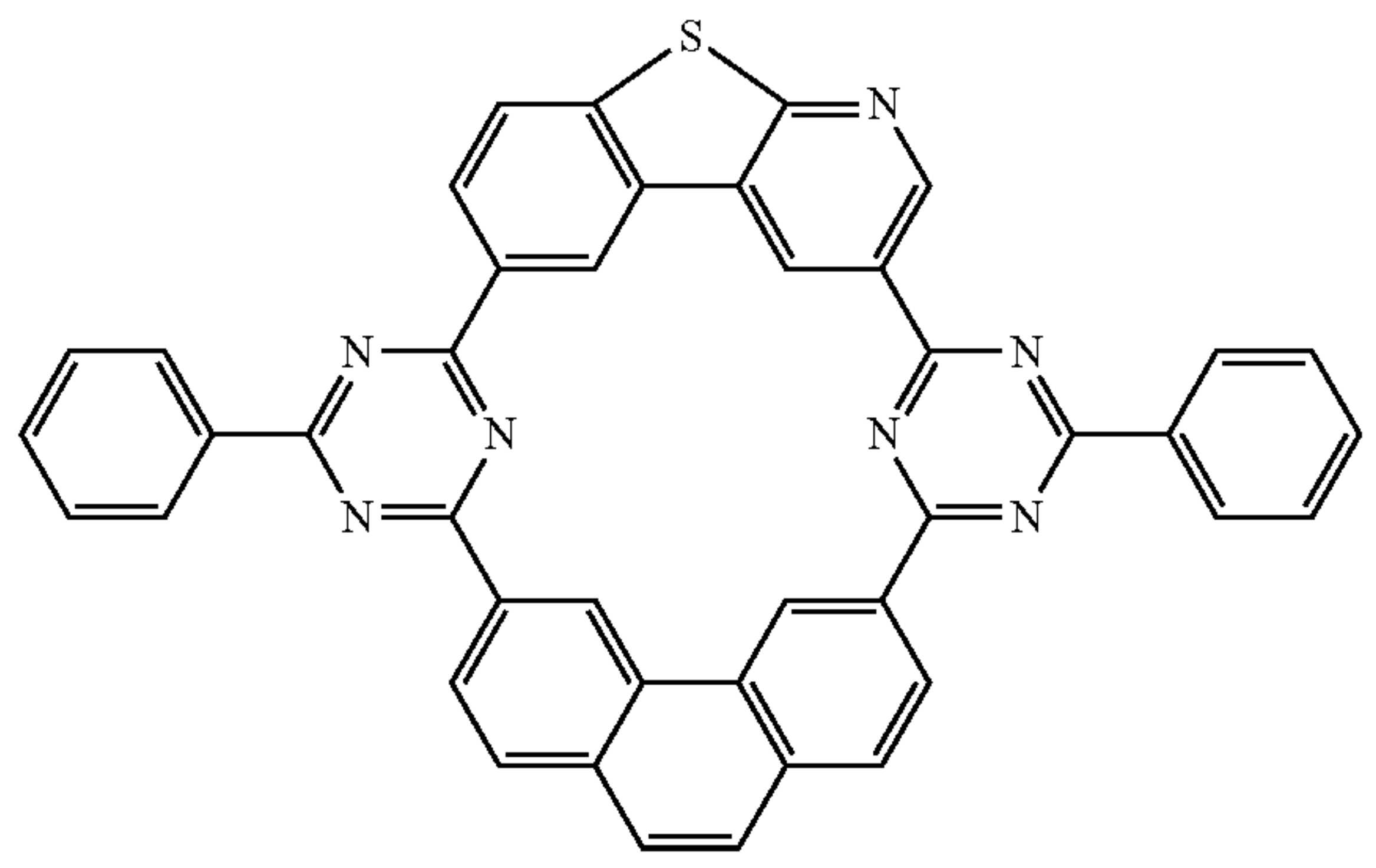
Compound 54
