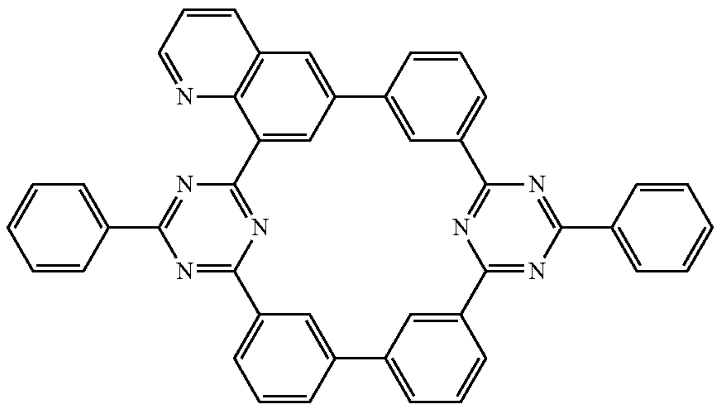
Compound 61
