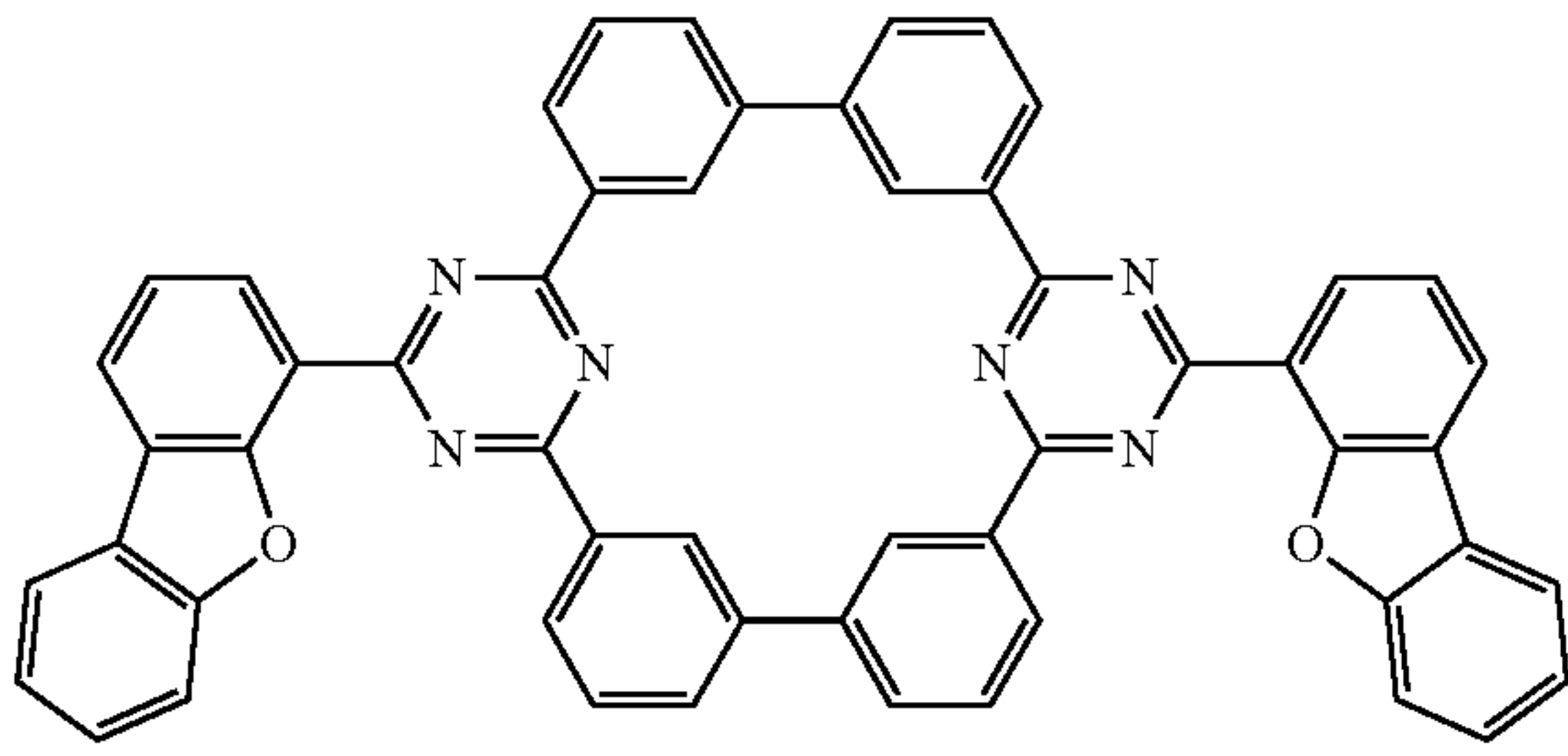
Compound 6
