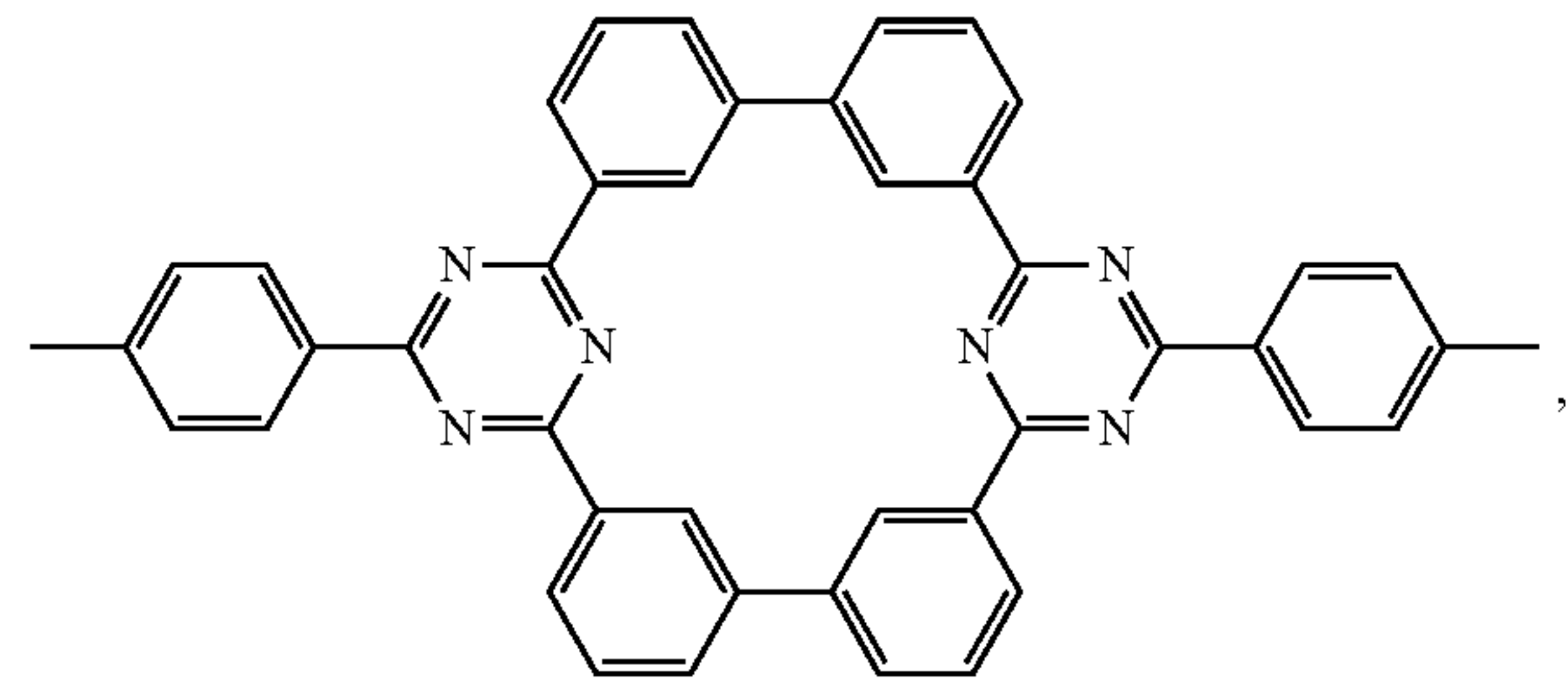
Compound 36
