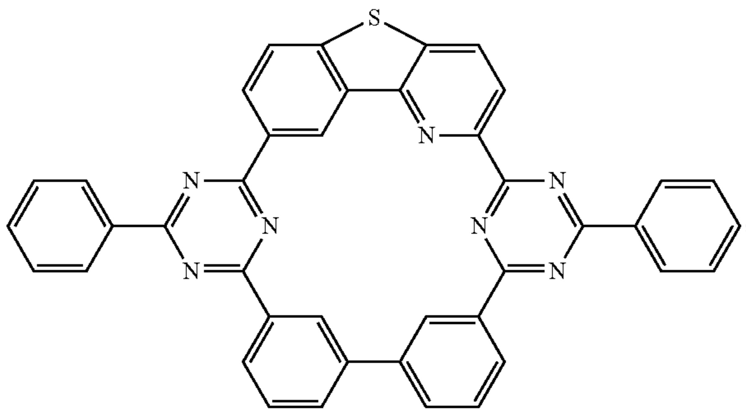
Compound 55
