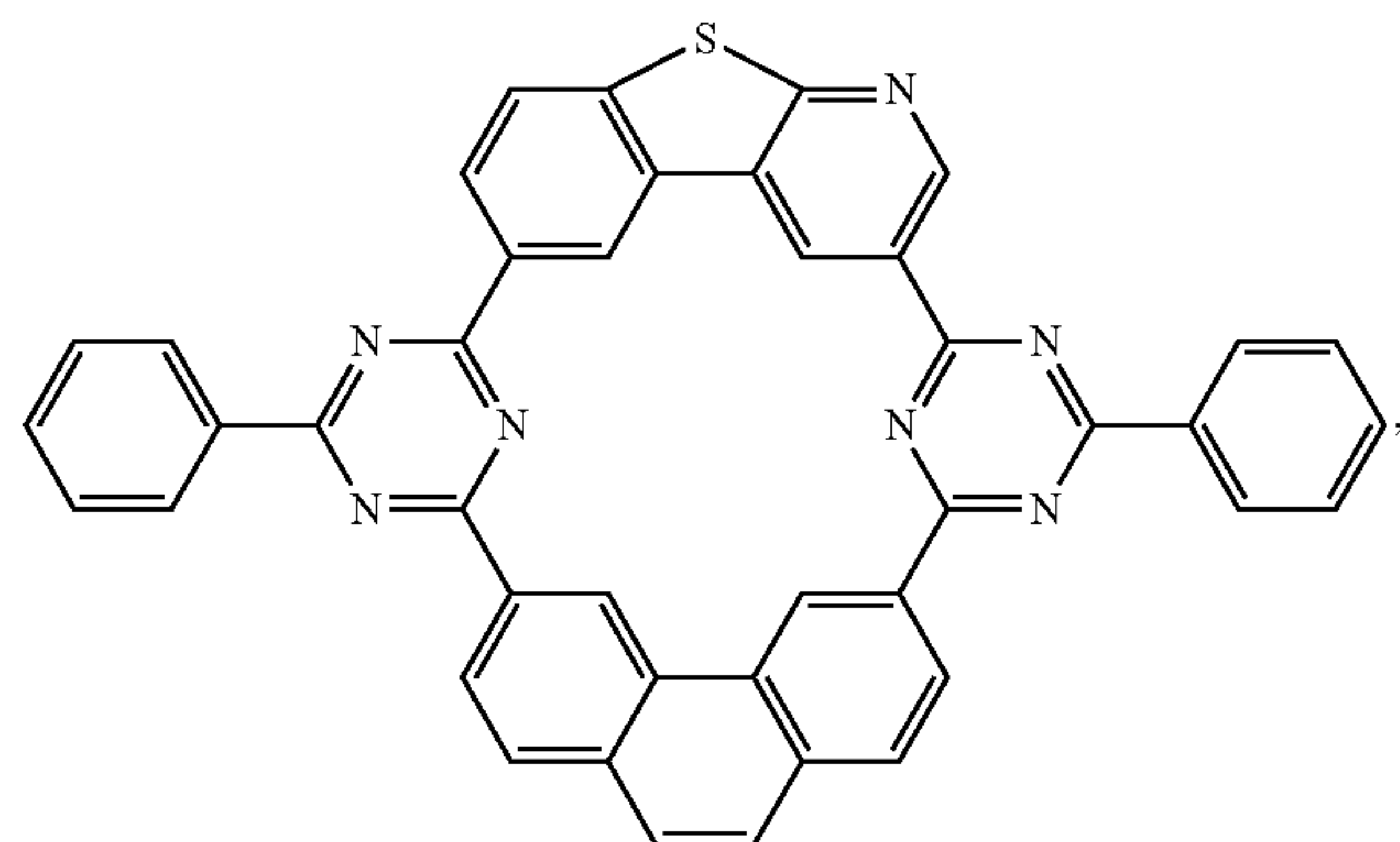
Compound 54
