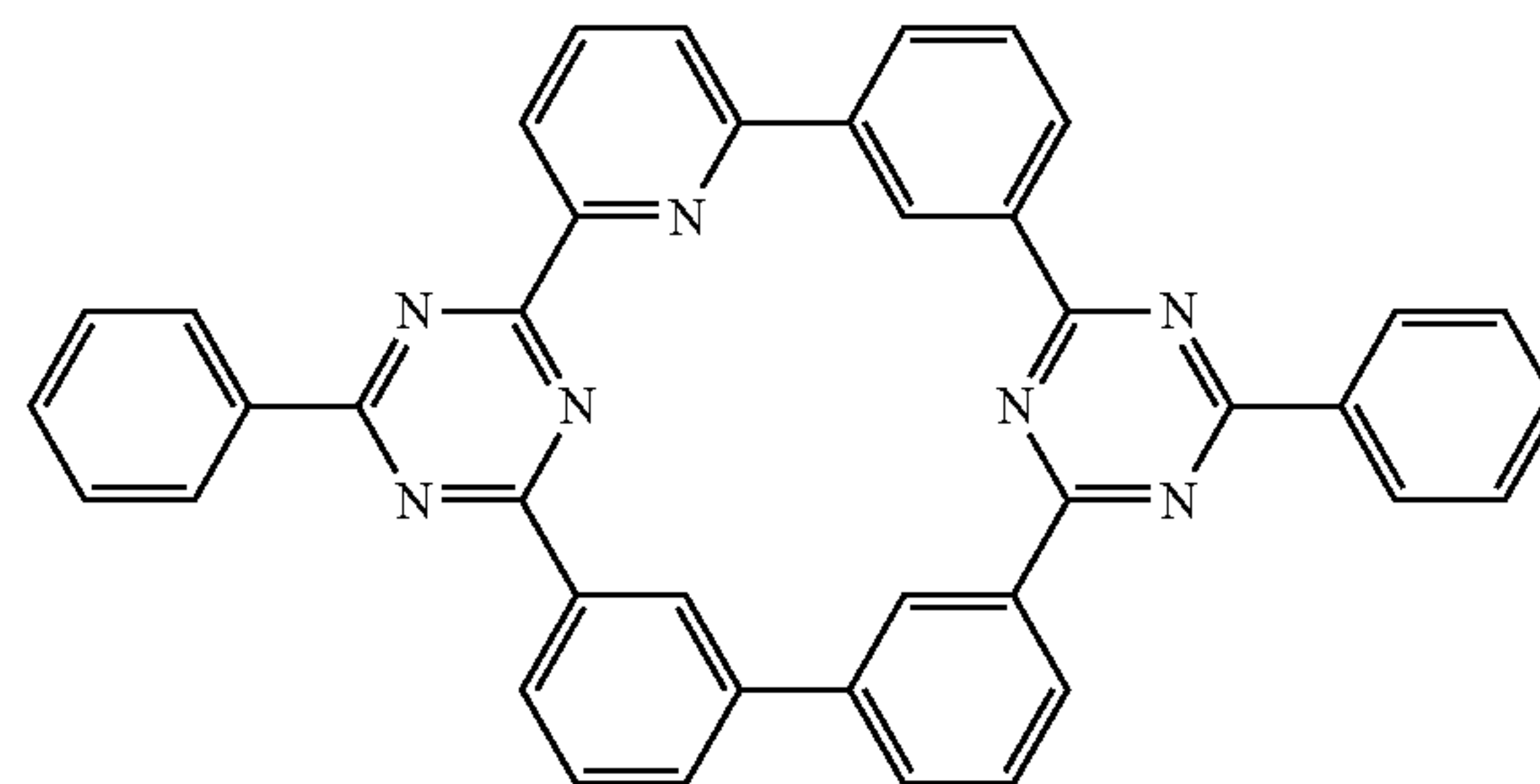
Compound 11
