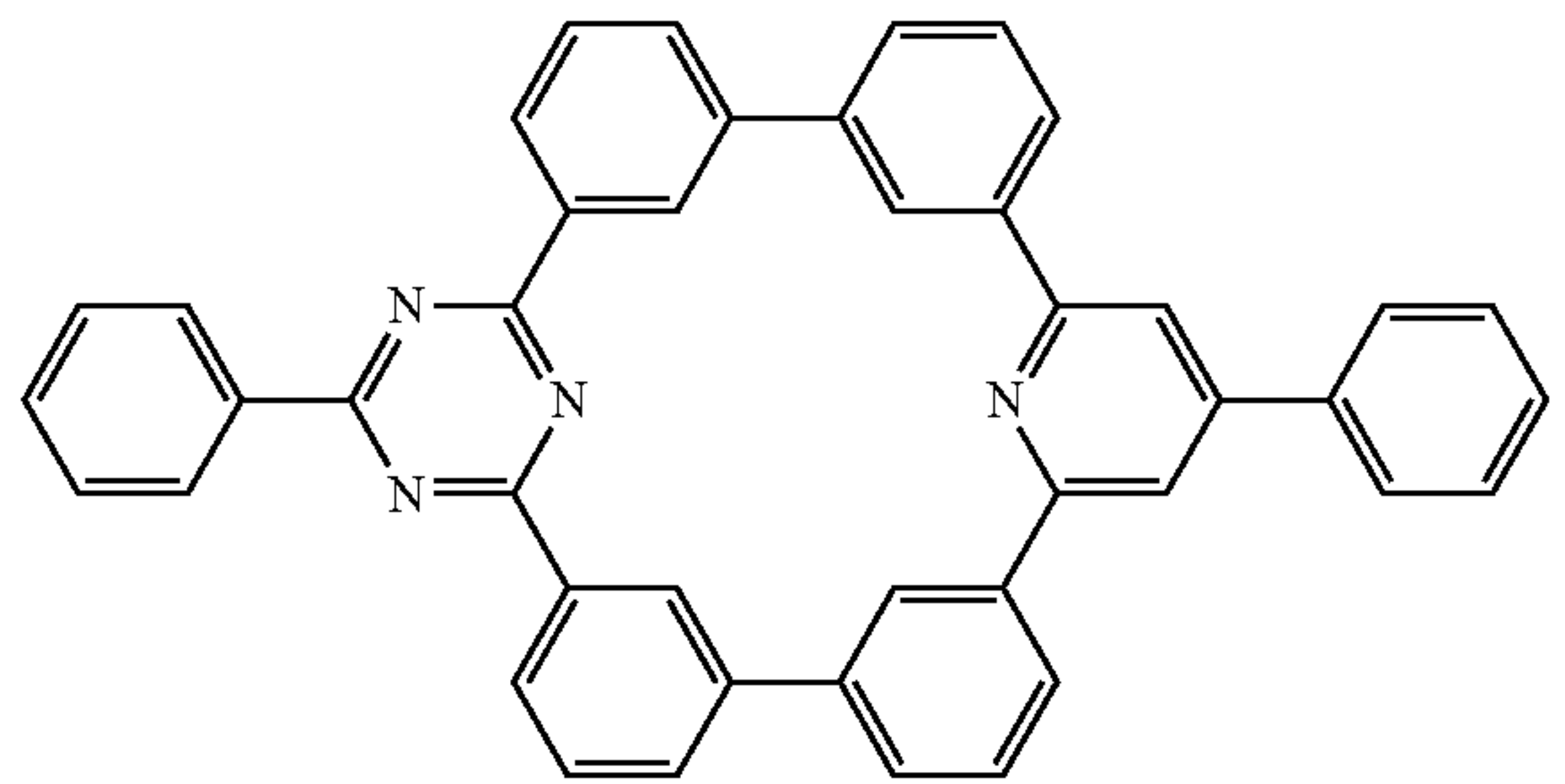
Compound 46
