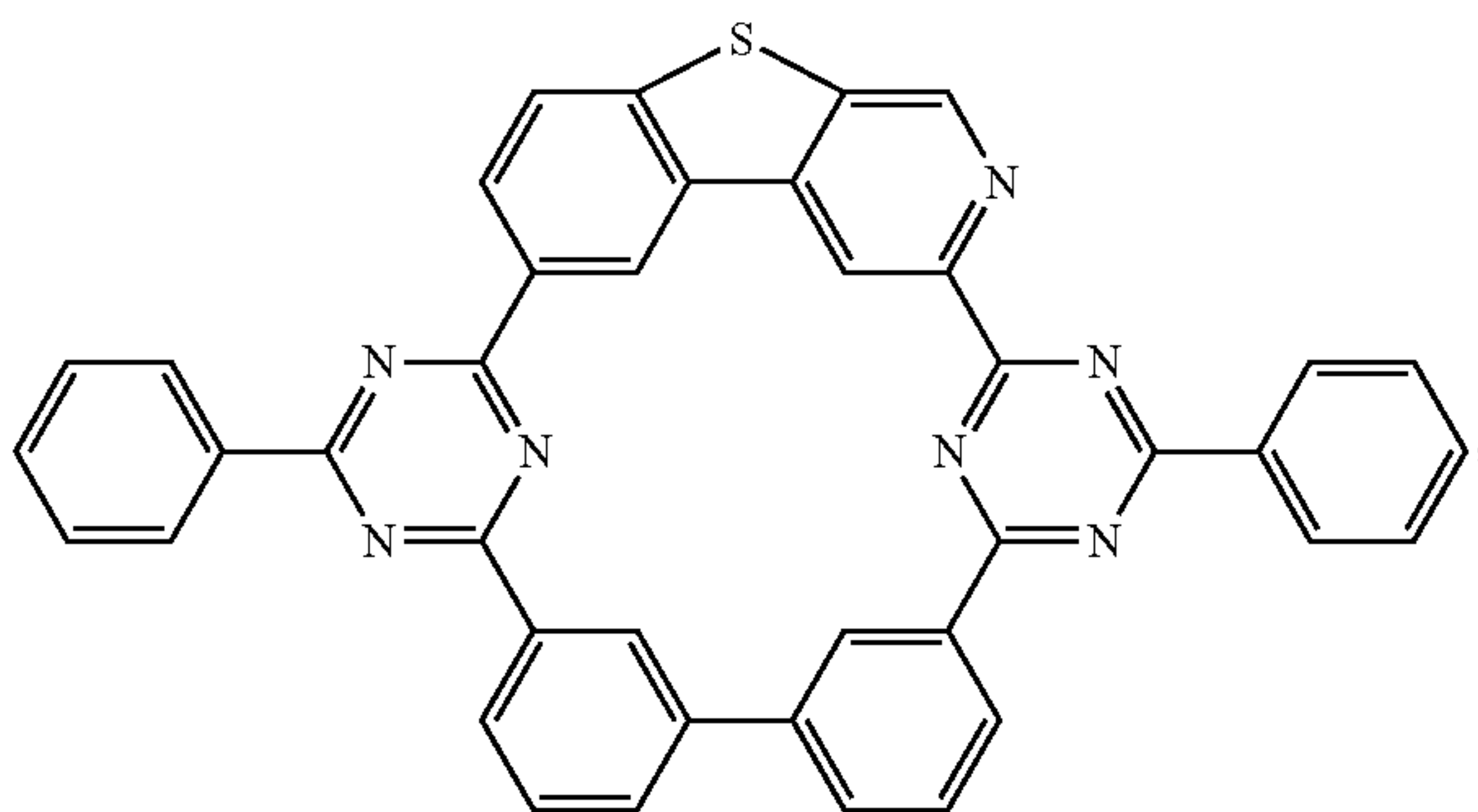
Compound 57
