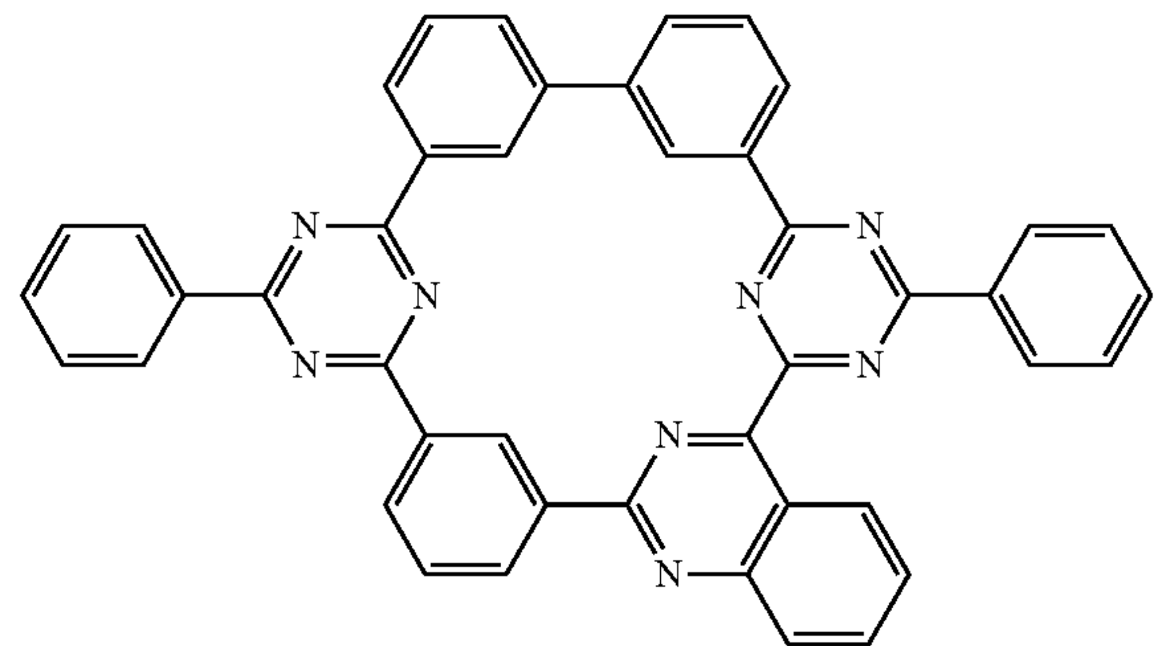
Compound 17
