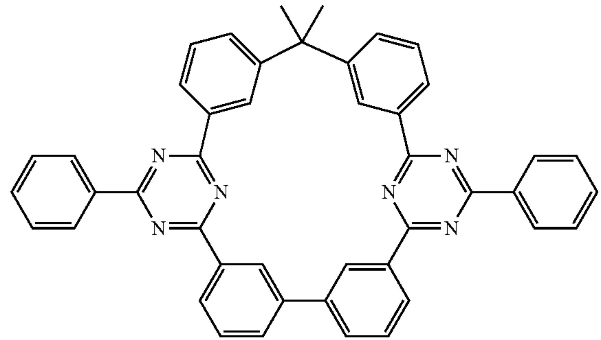
Compound 23
