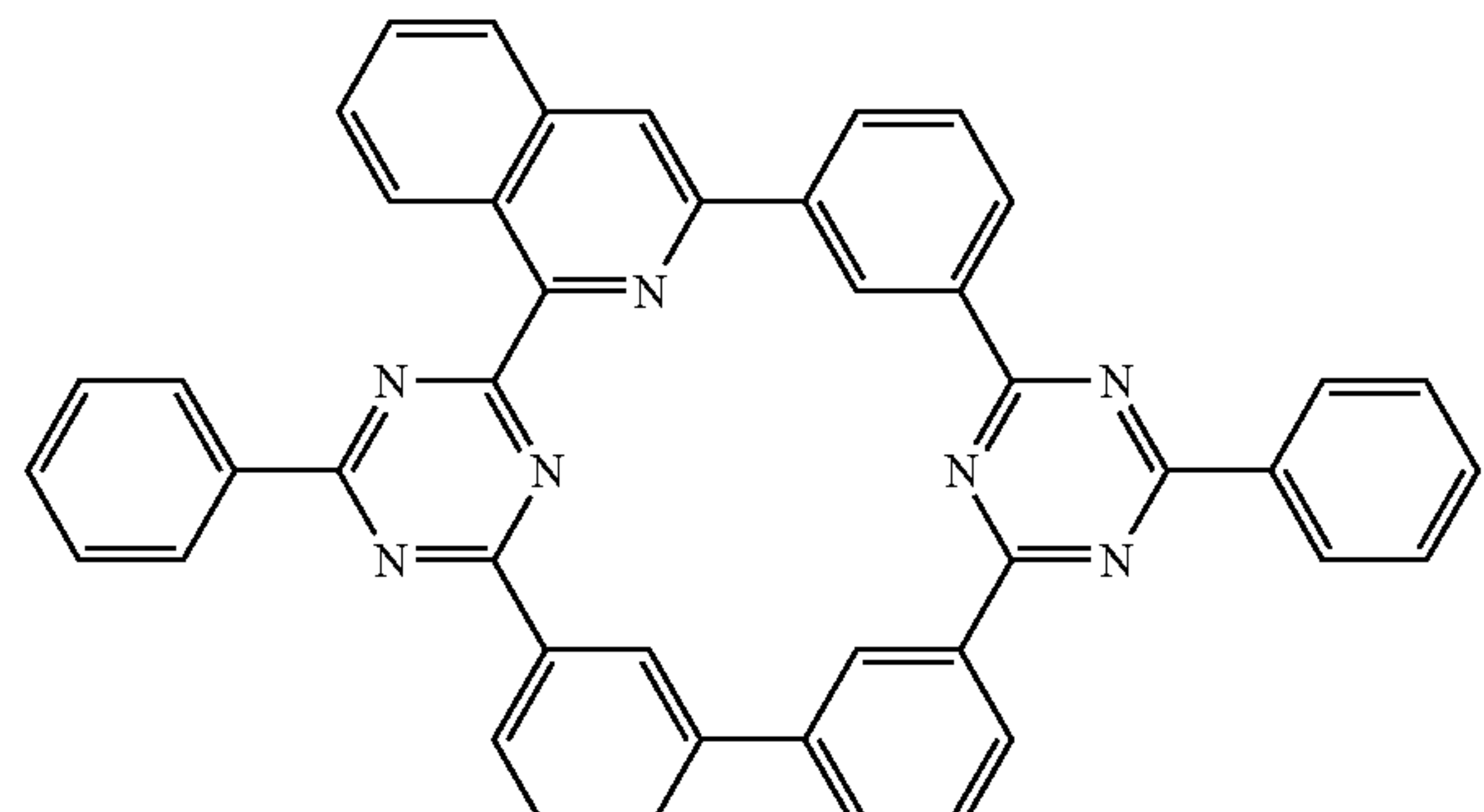
Compound 60
