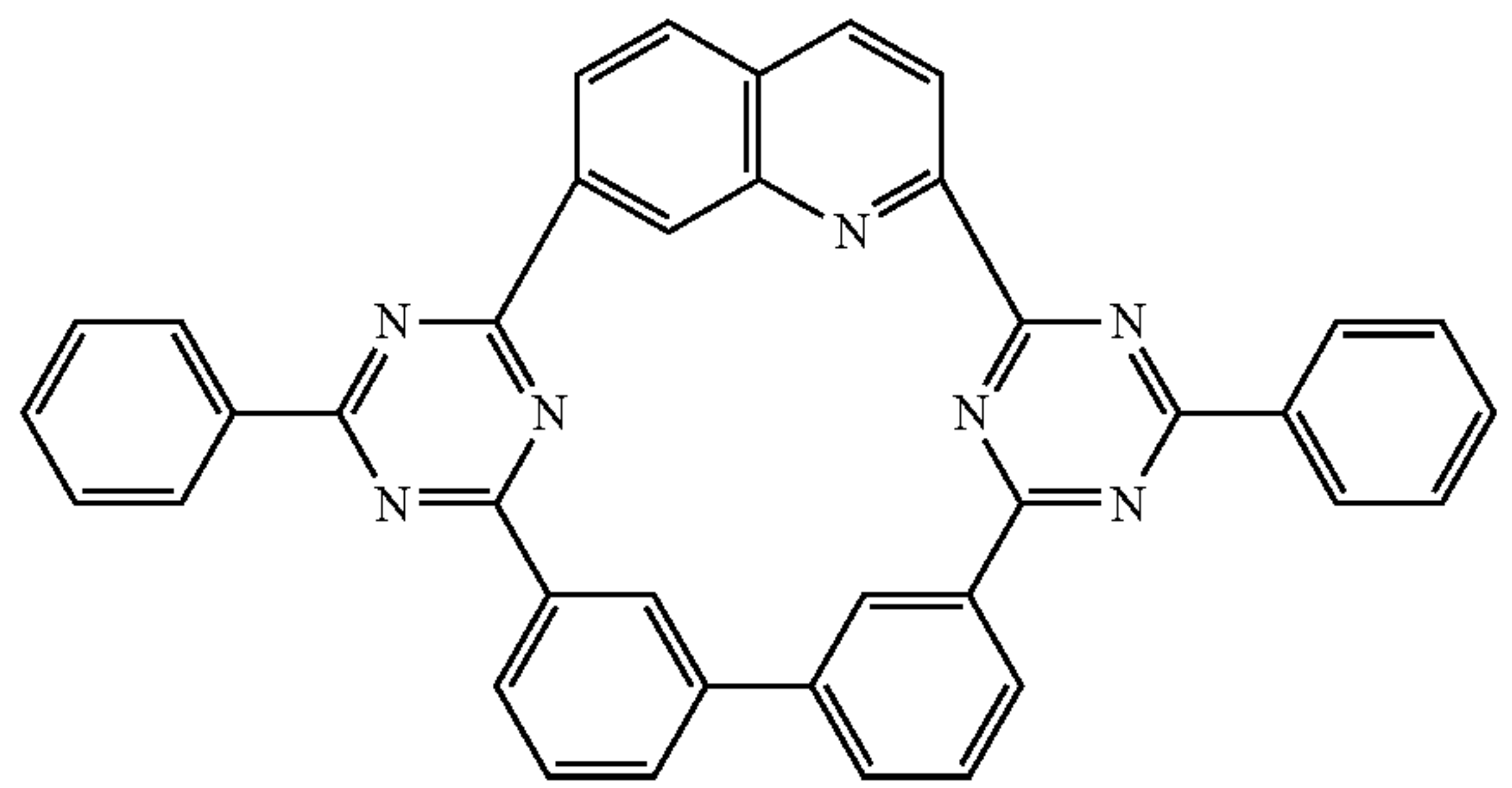
Compound 64
