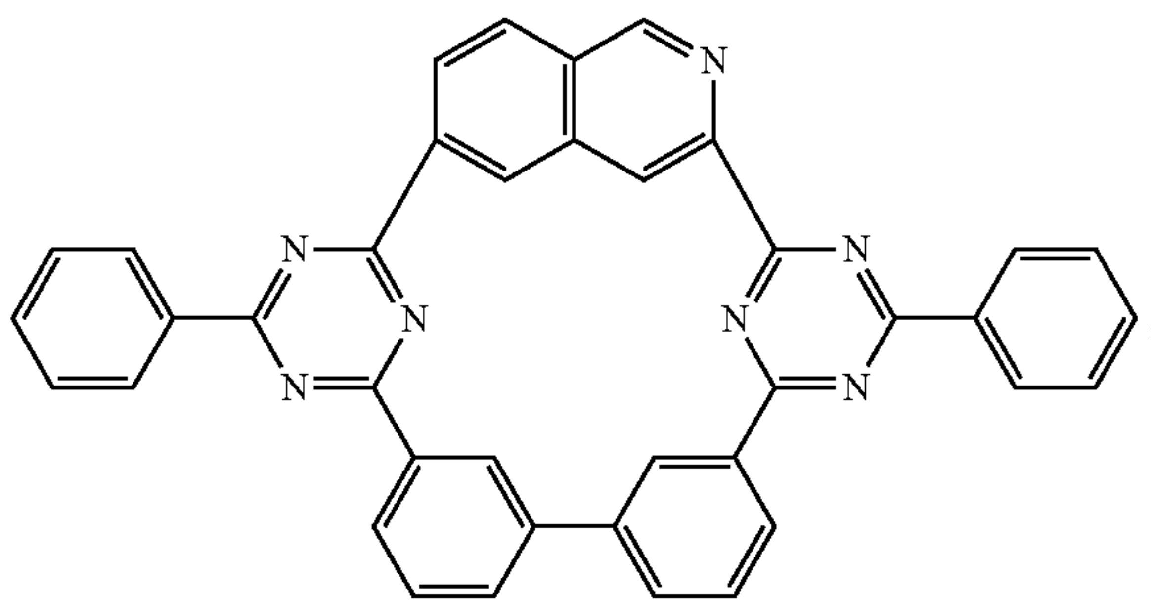
Compound 65
