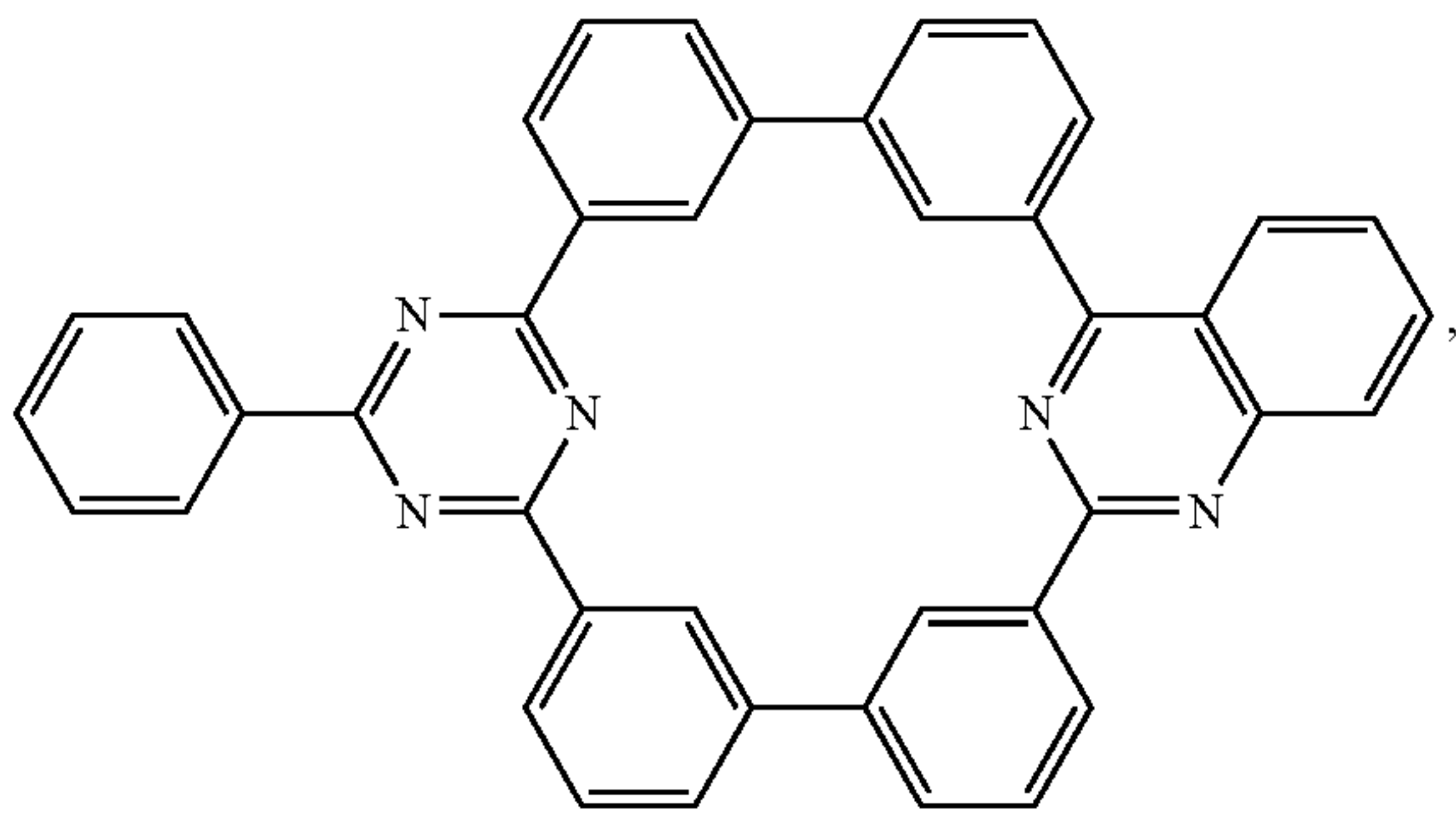
Compound 43
