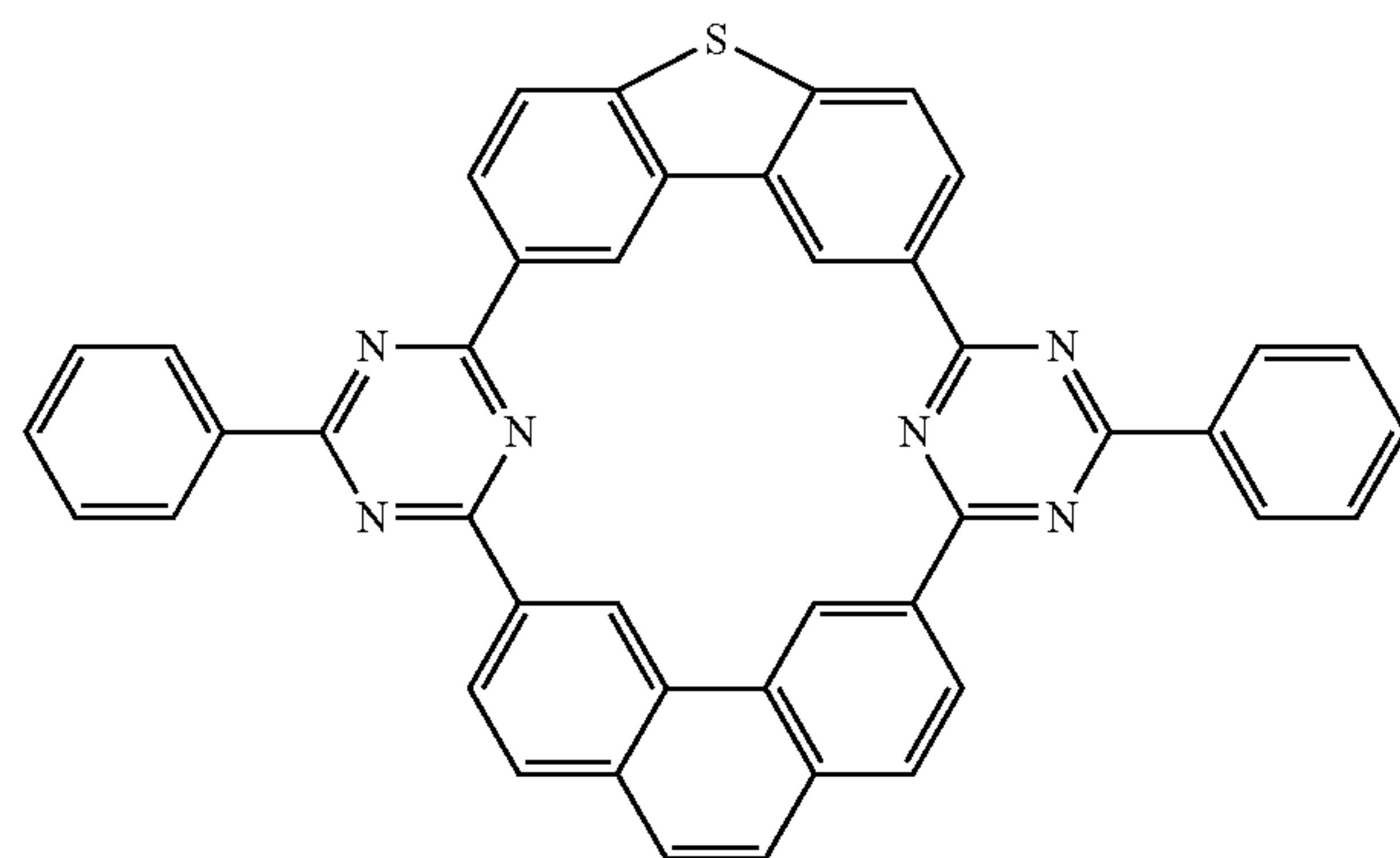
Compound 52
