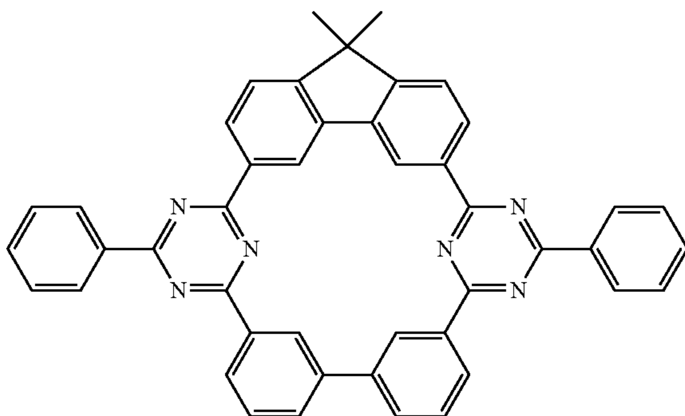
Compound 10
