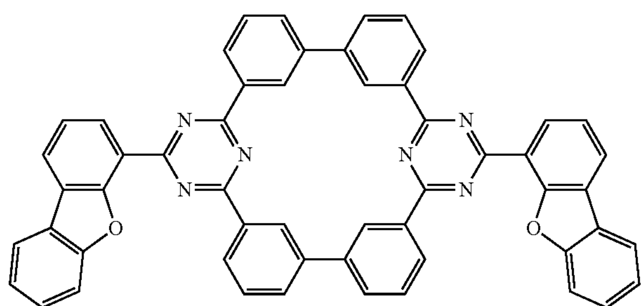
Compound 6
