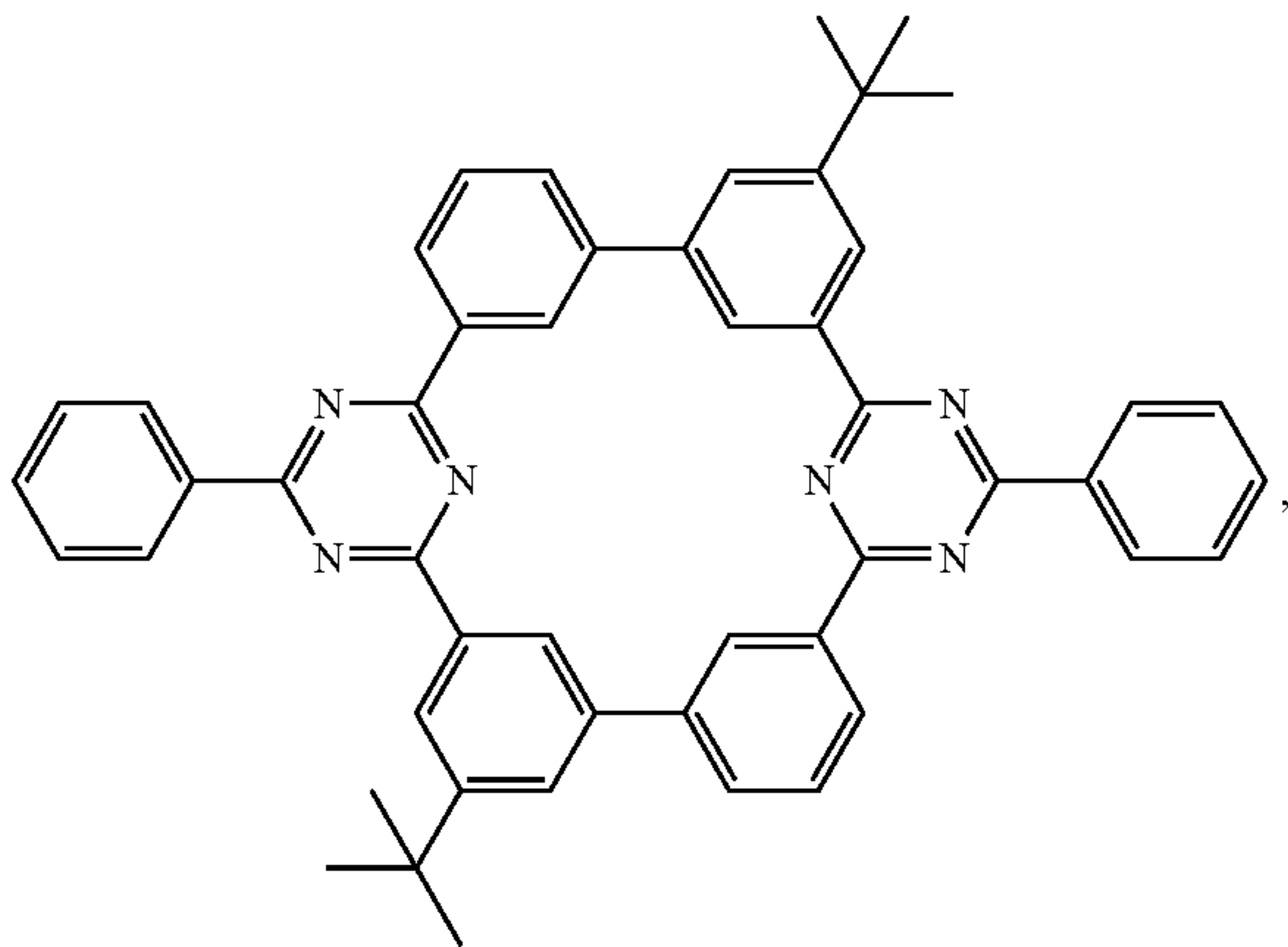
Compound 30
