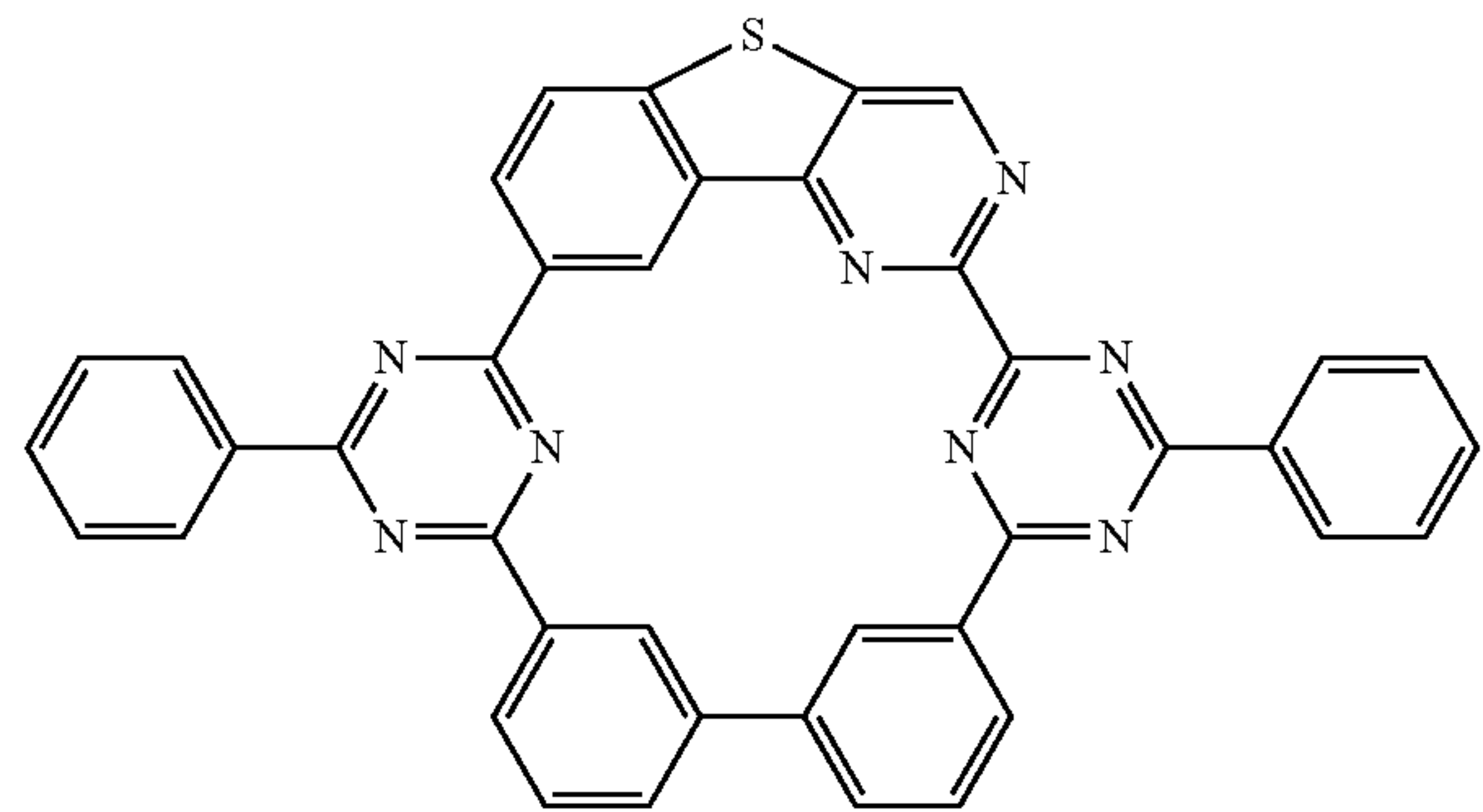
Compound 56
