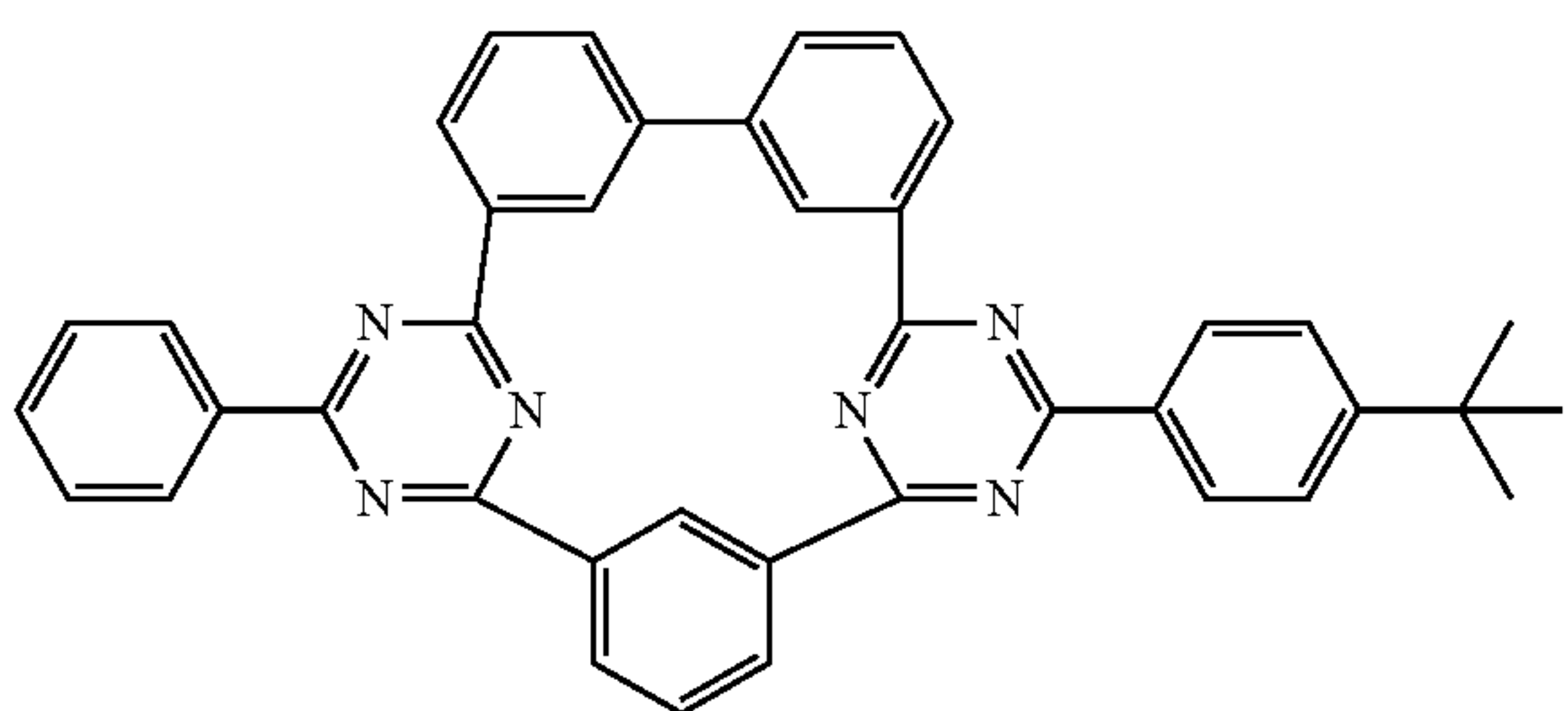
Compound 28
