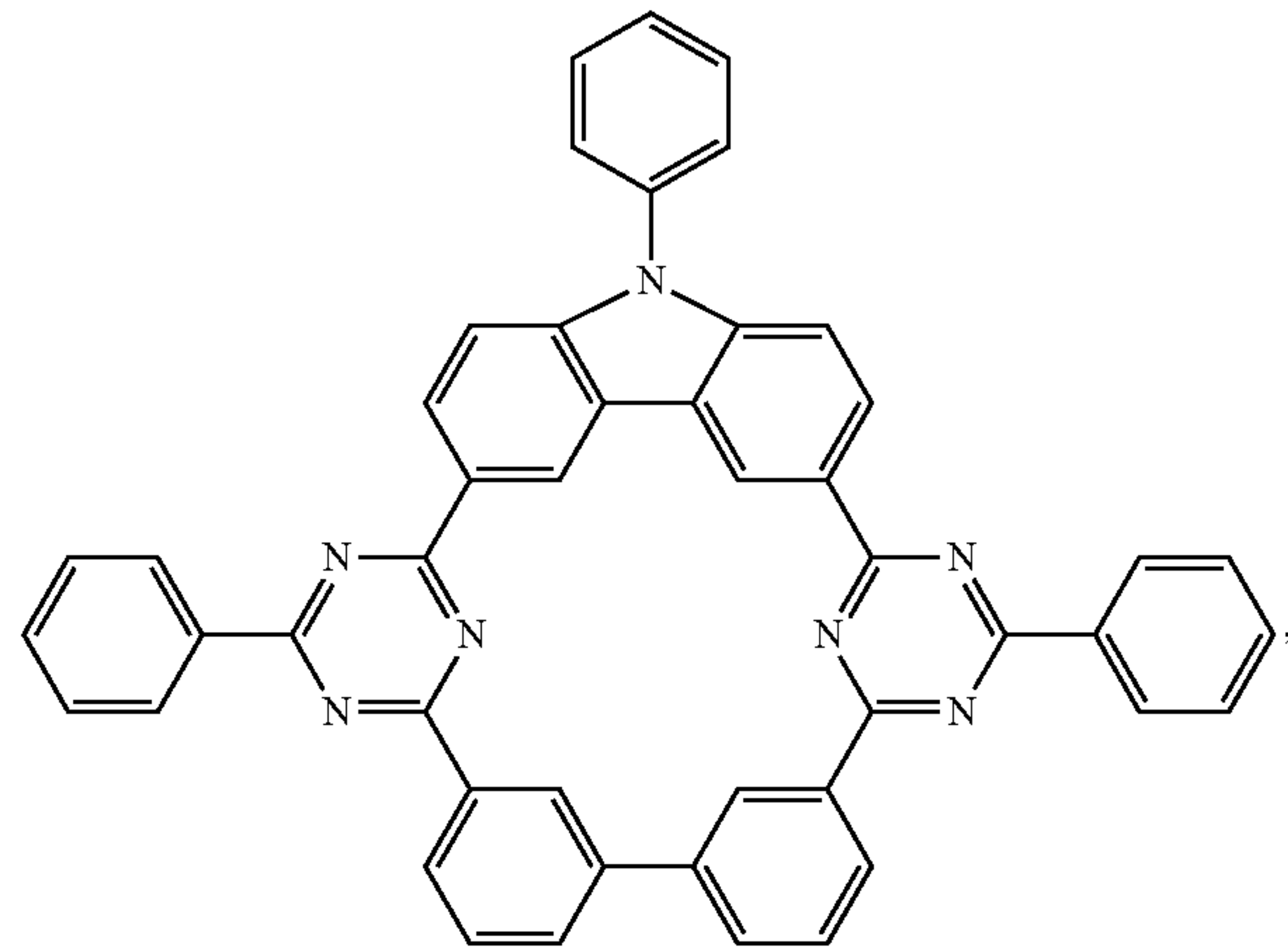
Compound 11
