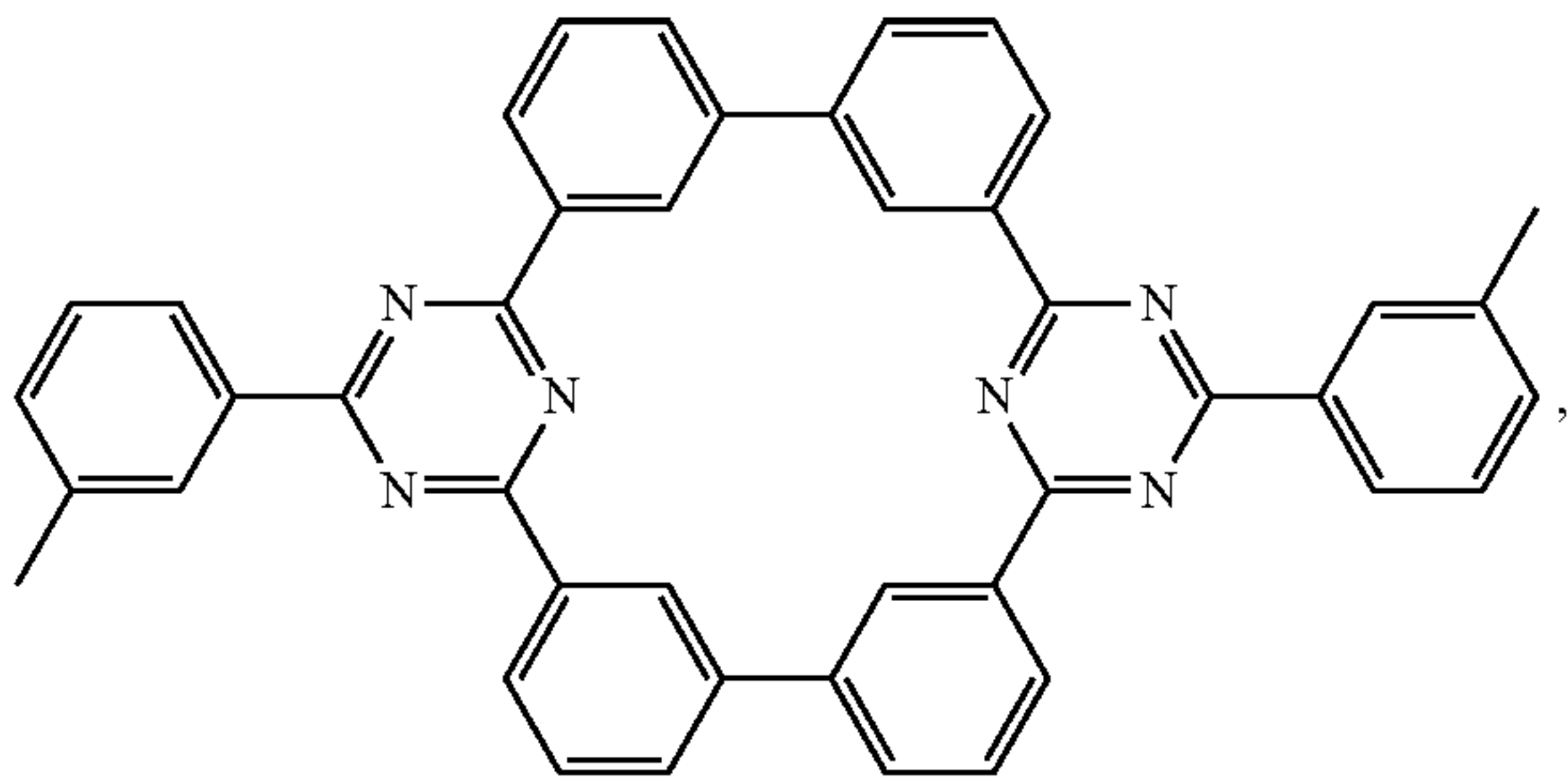
Compound 37
