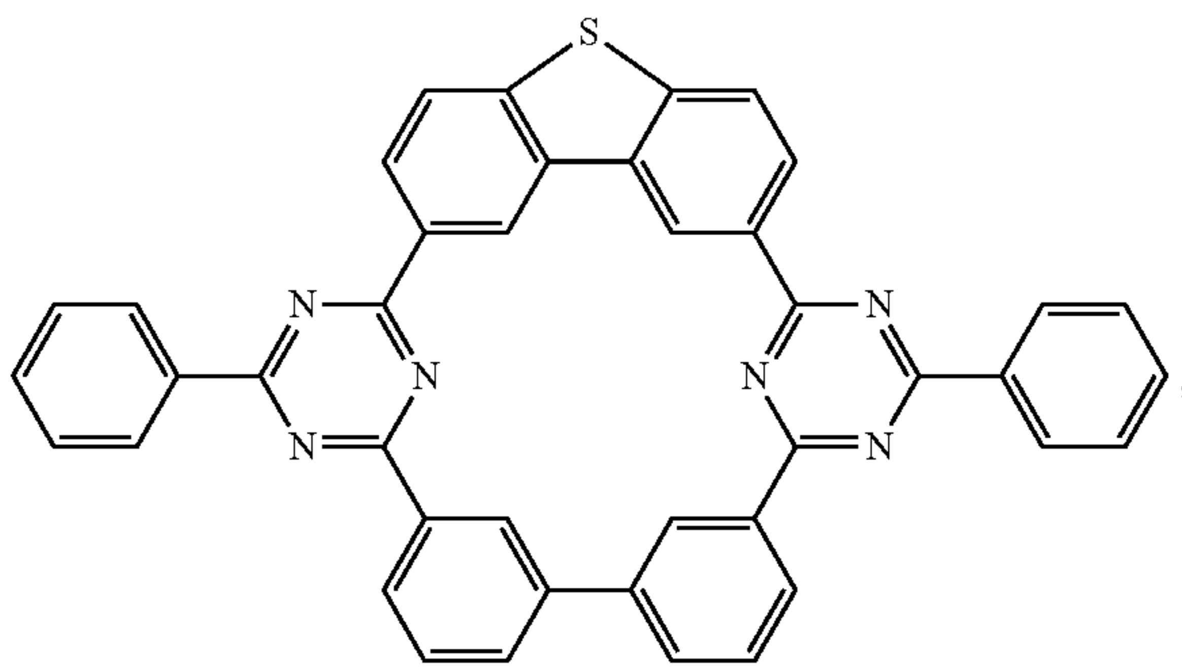
Compound 57
