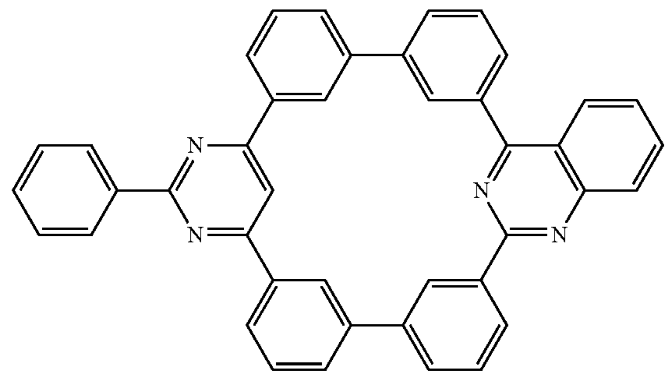
Compound 48
