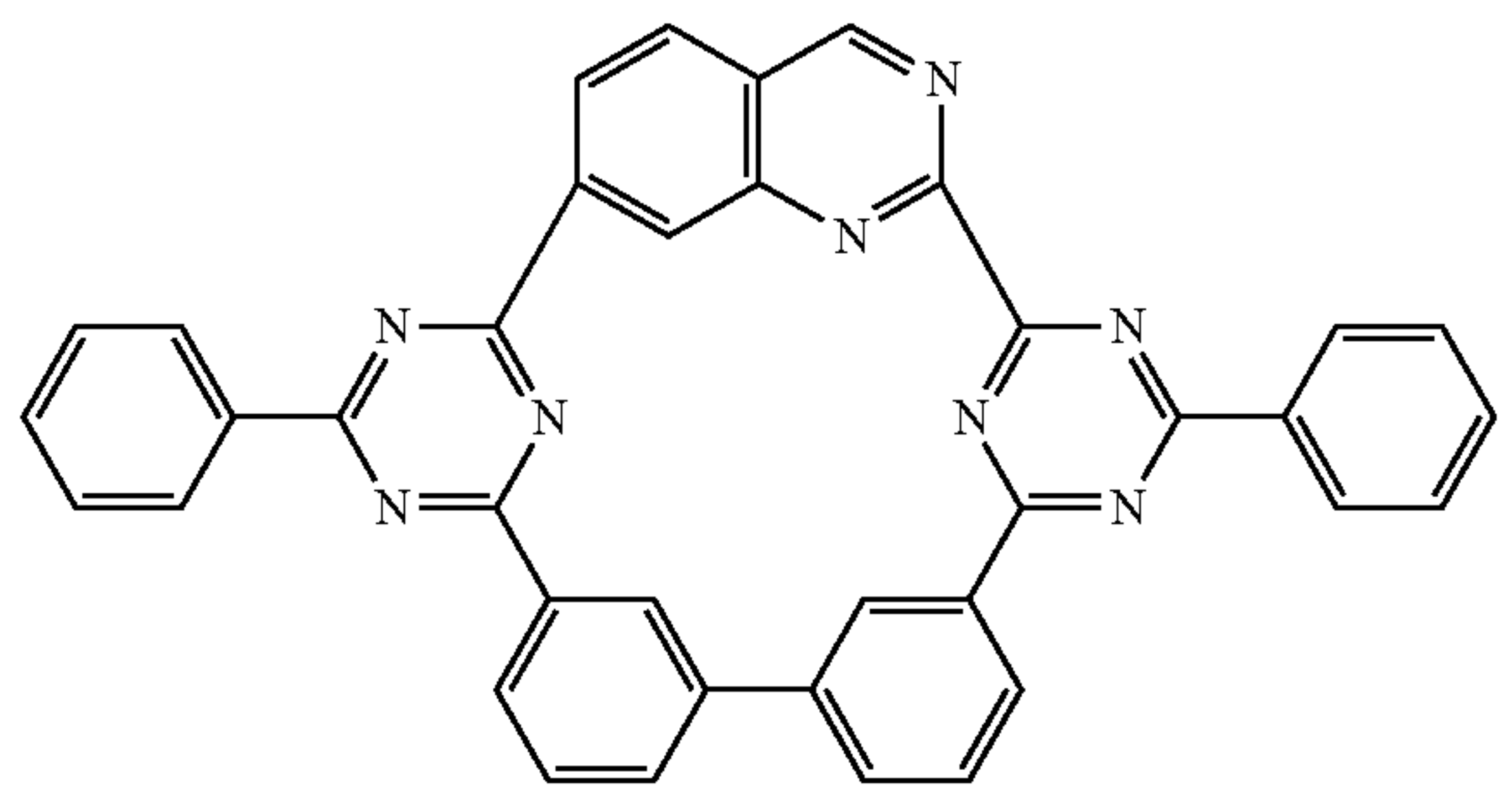
Compound 66
