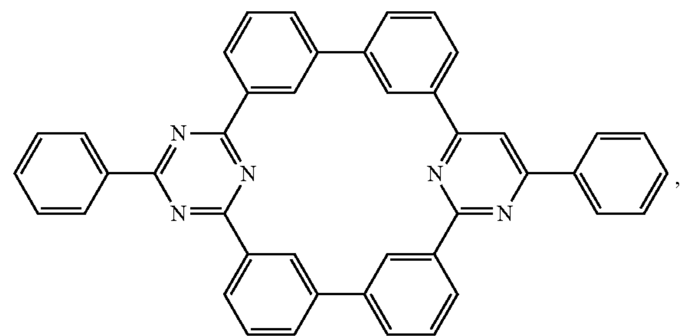
Compound 42
