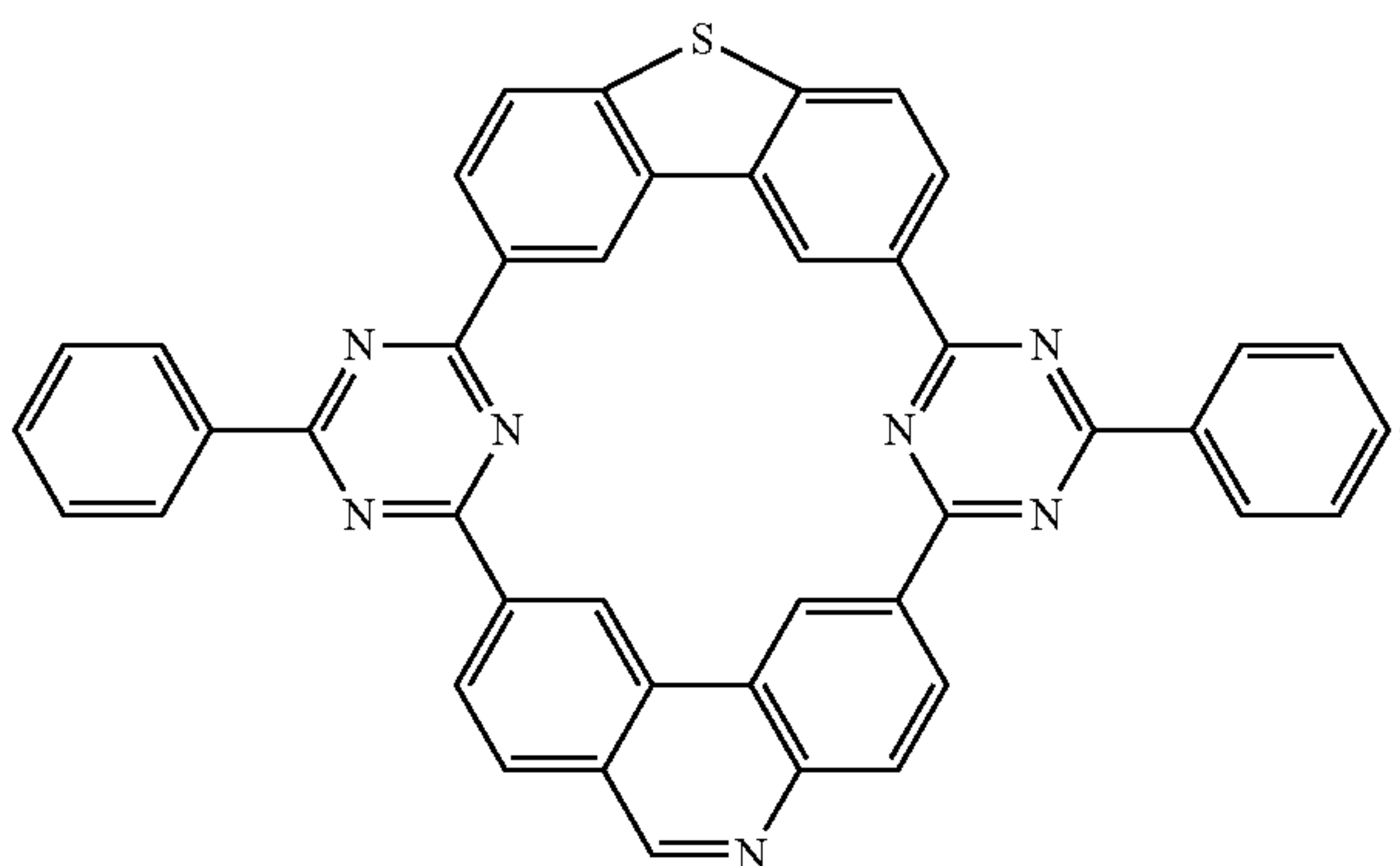
Compound 53
