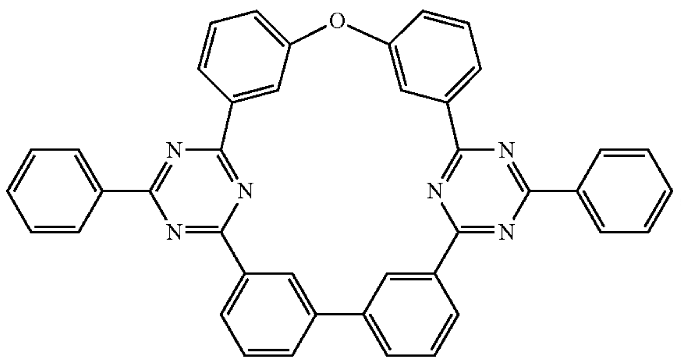
Compound 24
