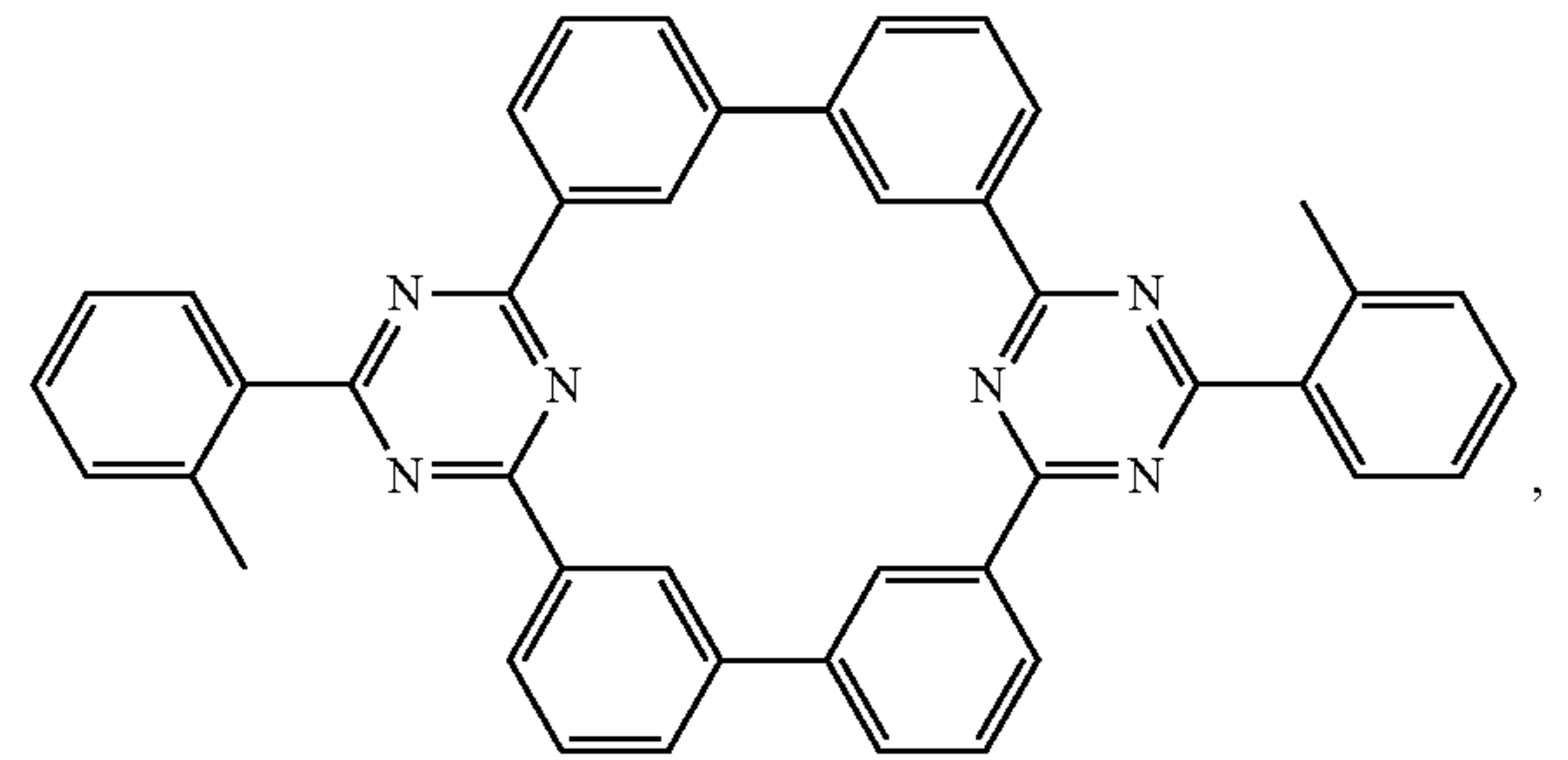
Compound 38
