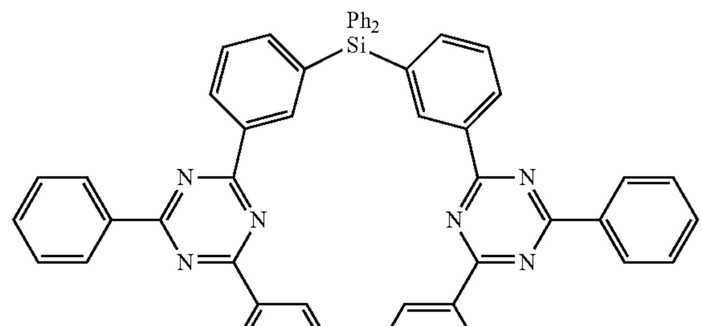
Compound 21
