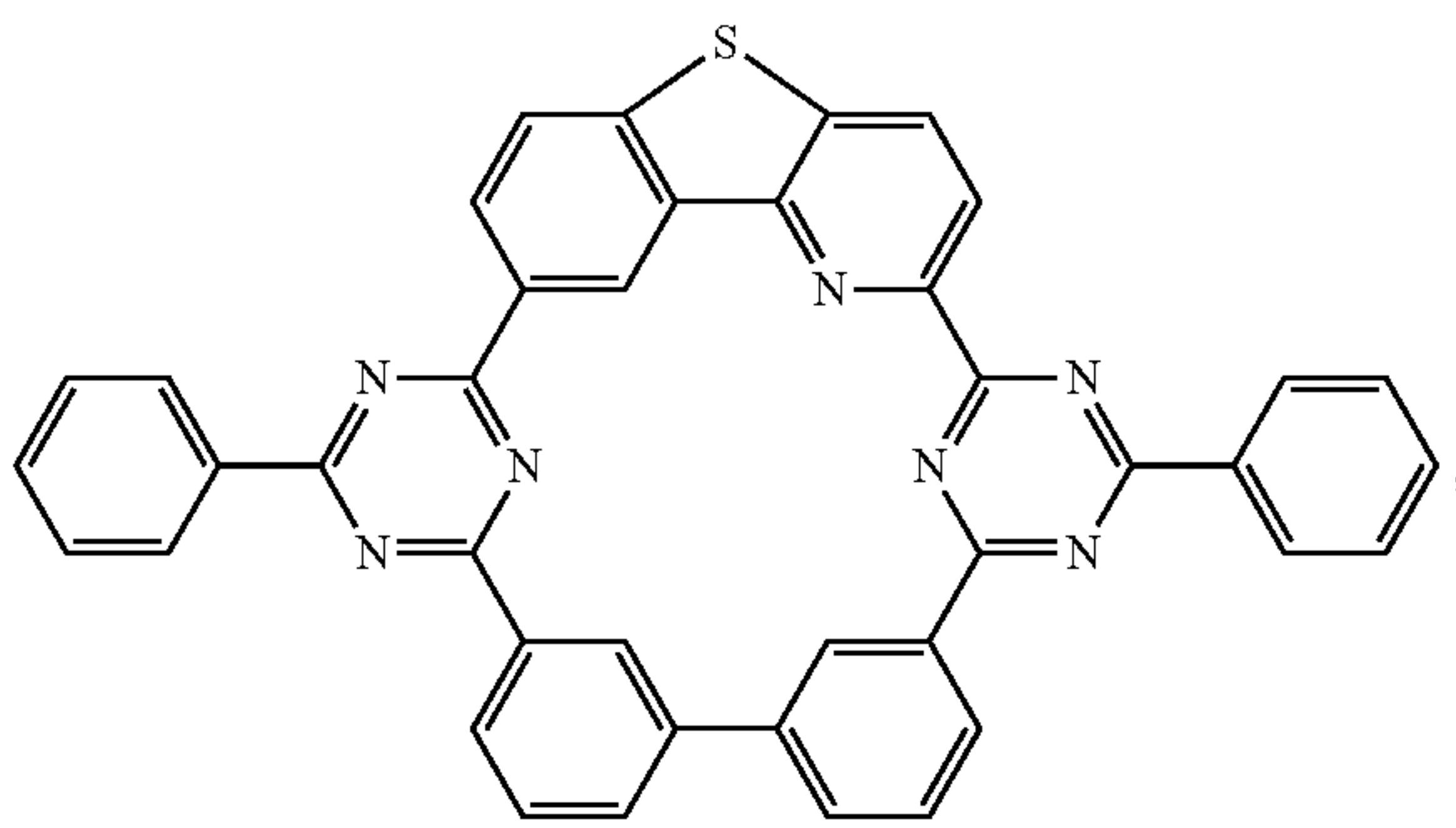
Compound 57
