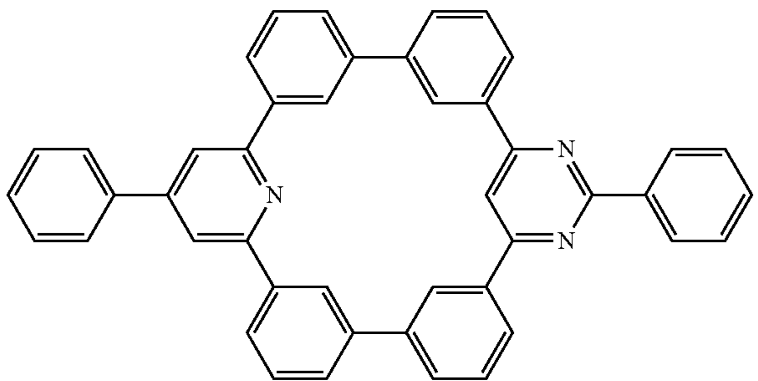
Compound 47
