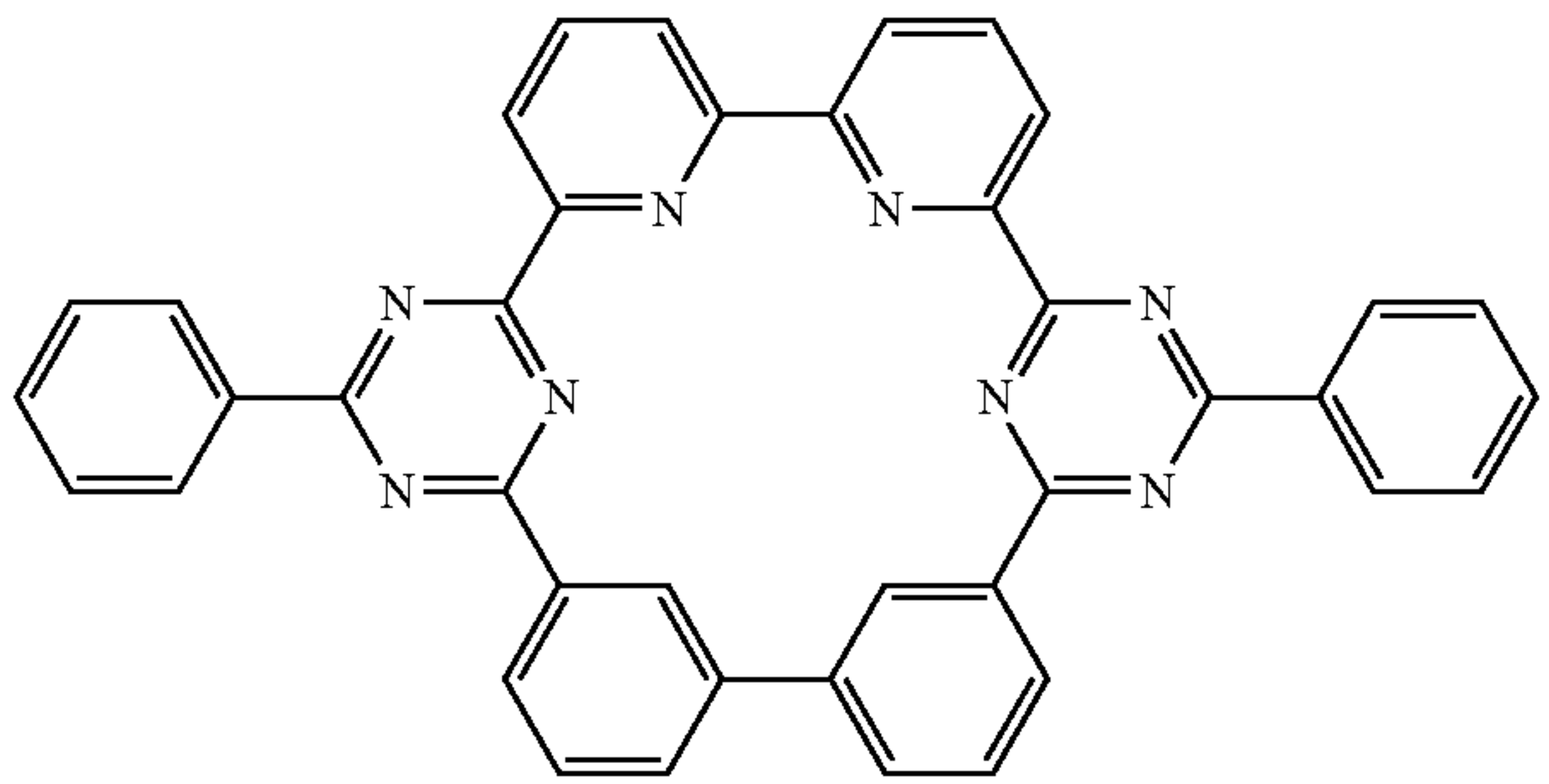
Compound 12
