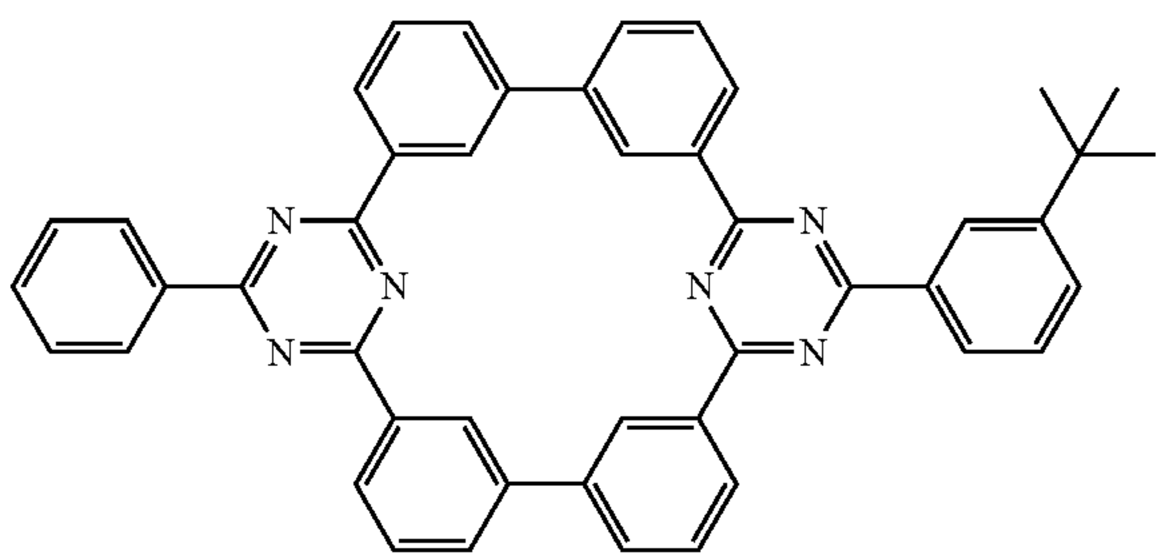
Compound 26
