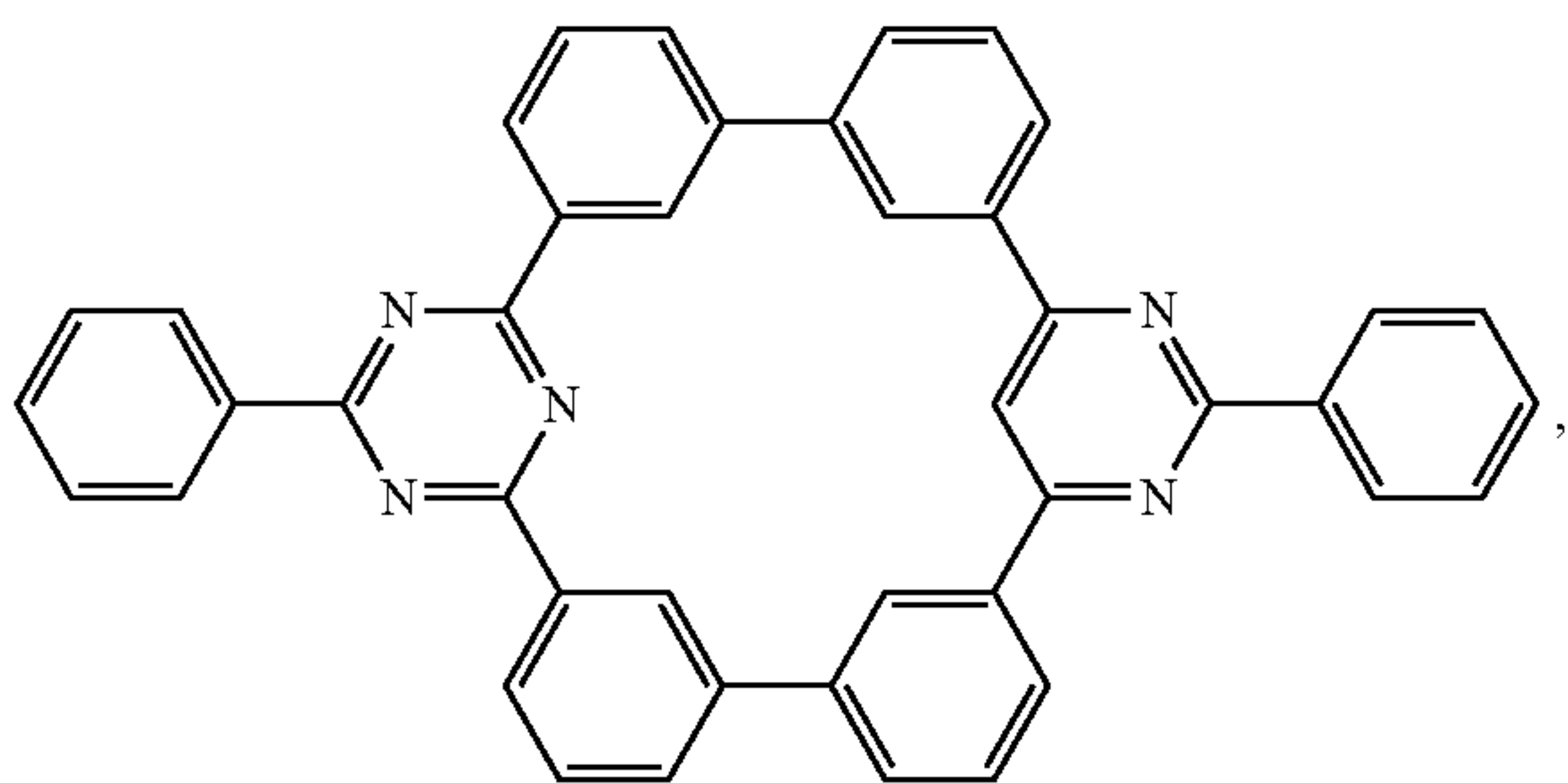
Compound 41
