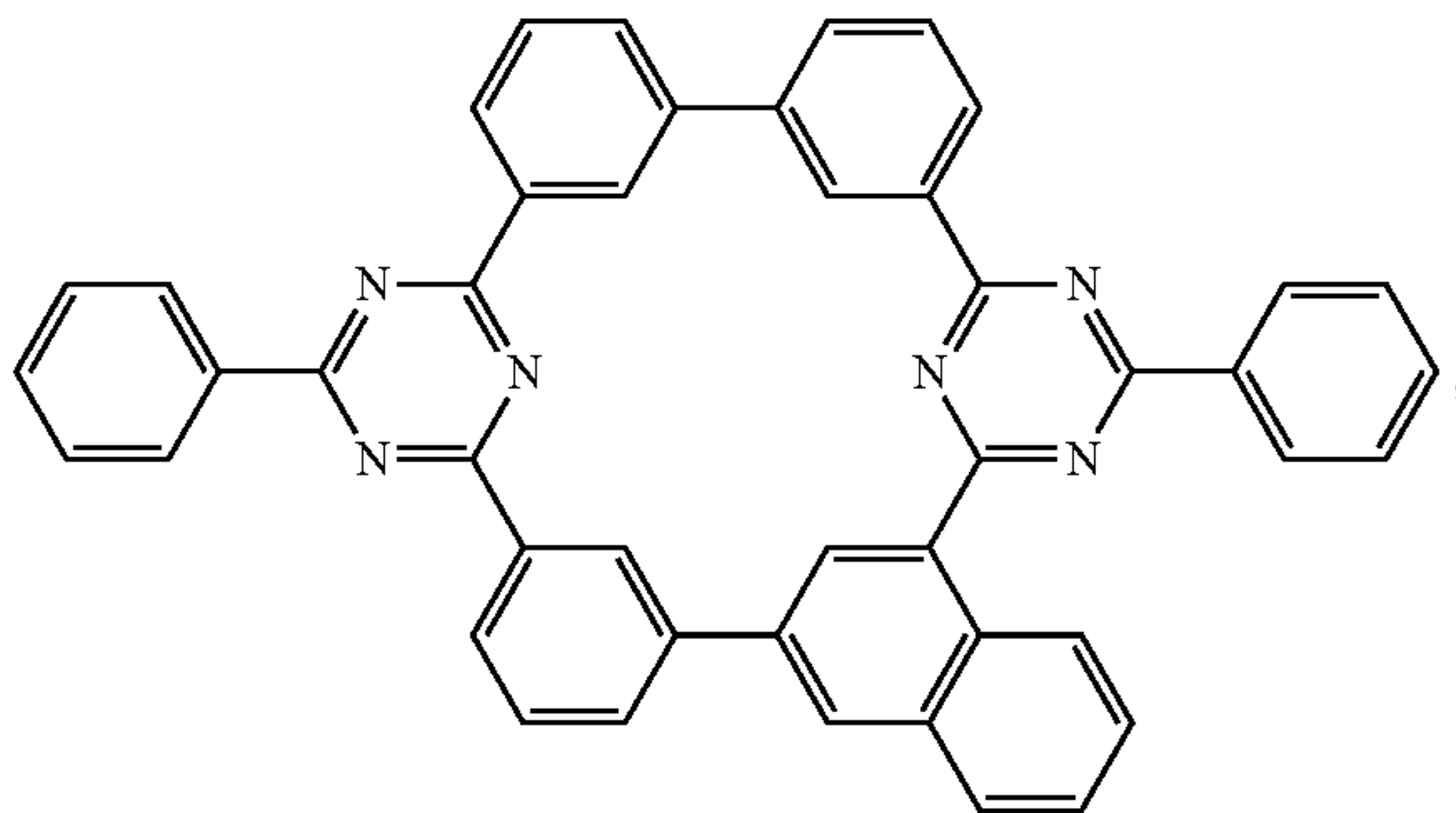
Compound 16
