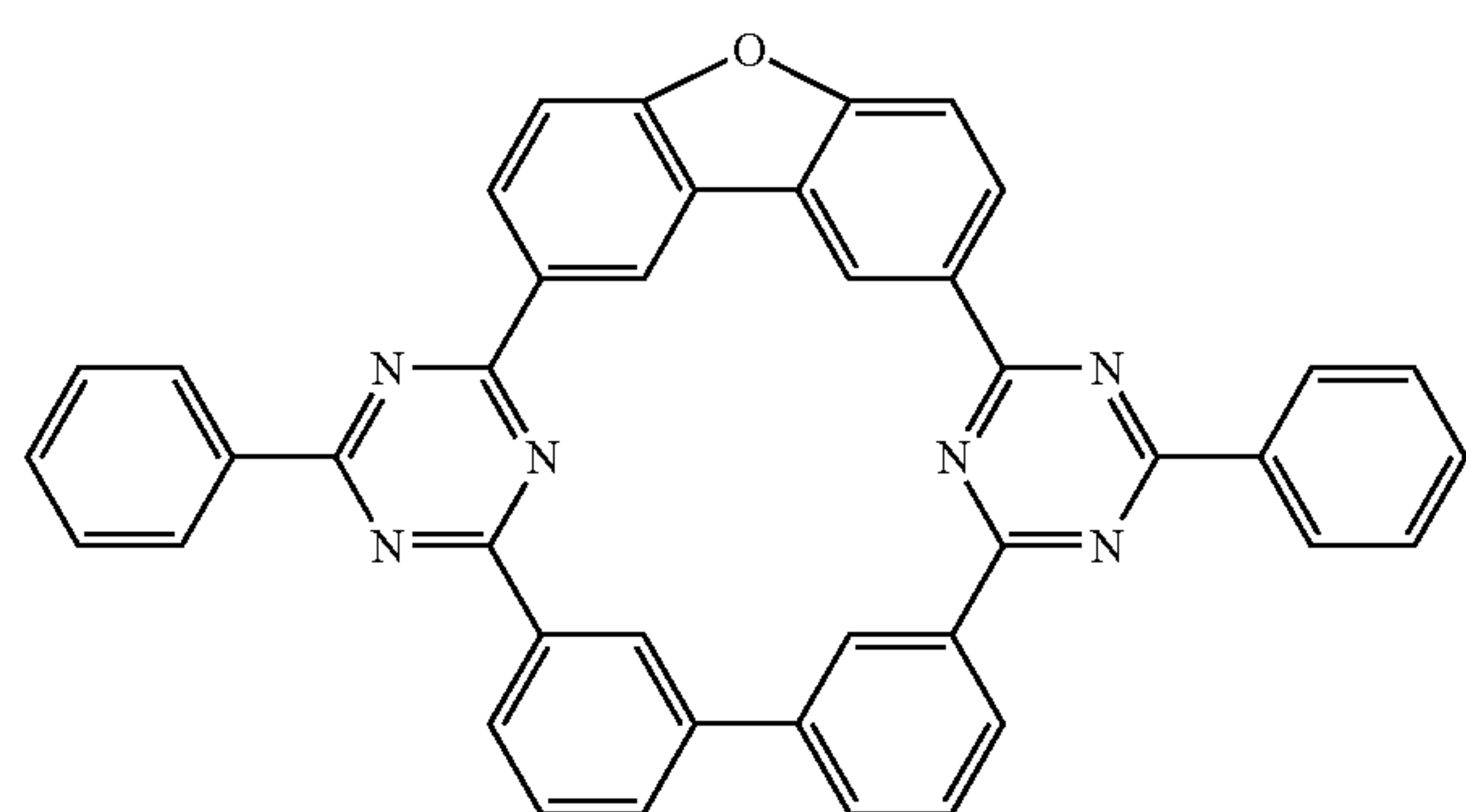
Compound 7
