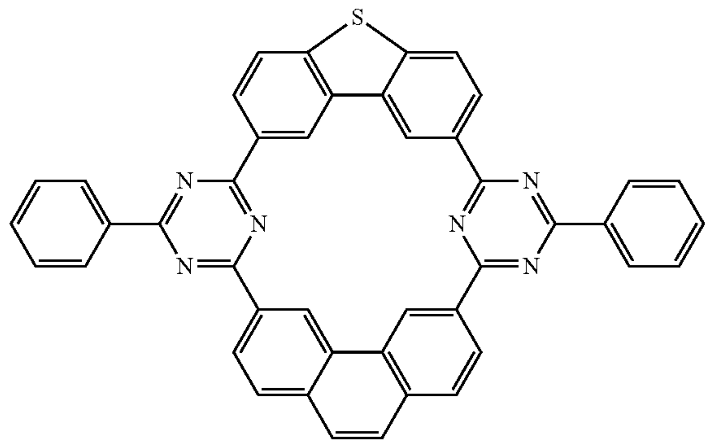
Compound 52
