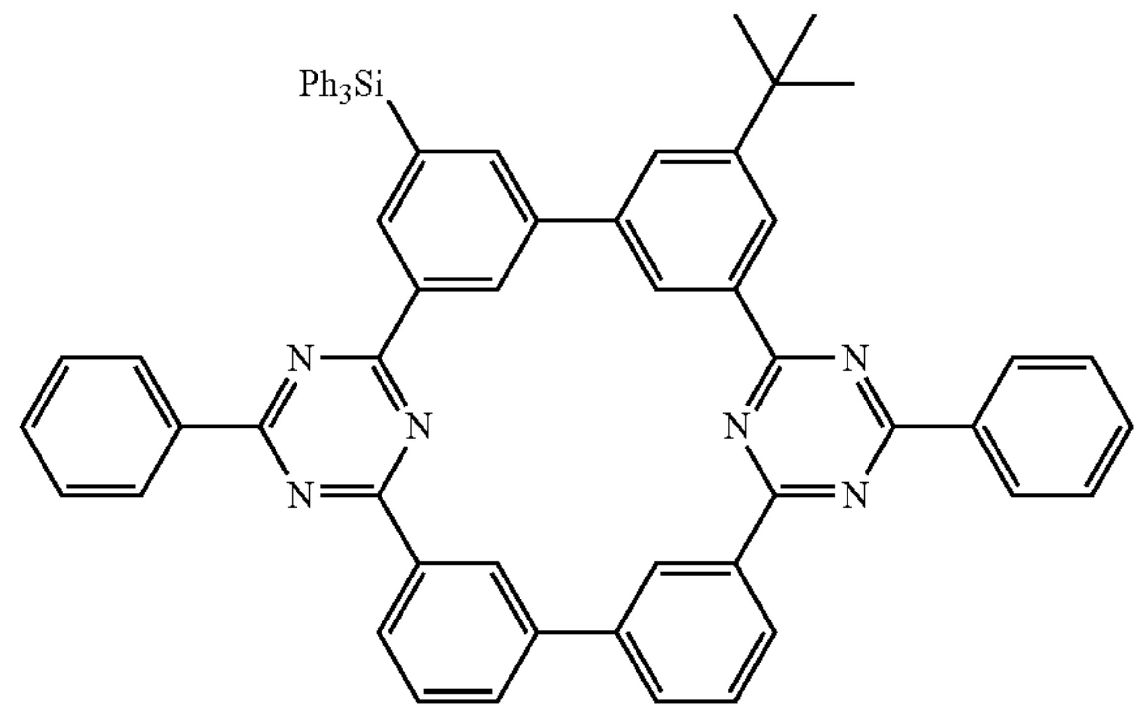
Compound 31
