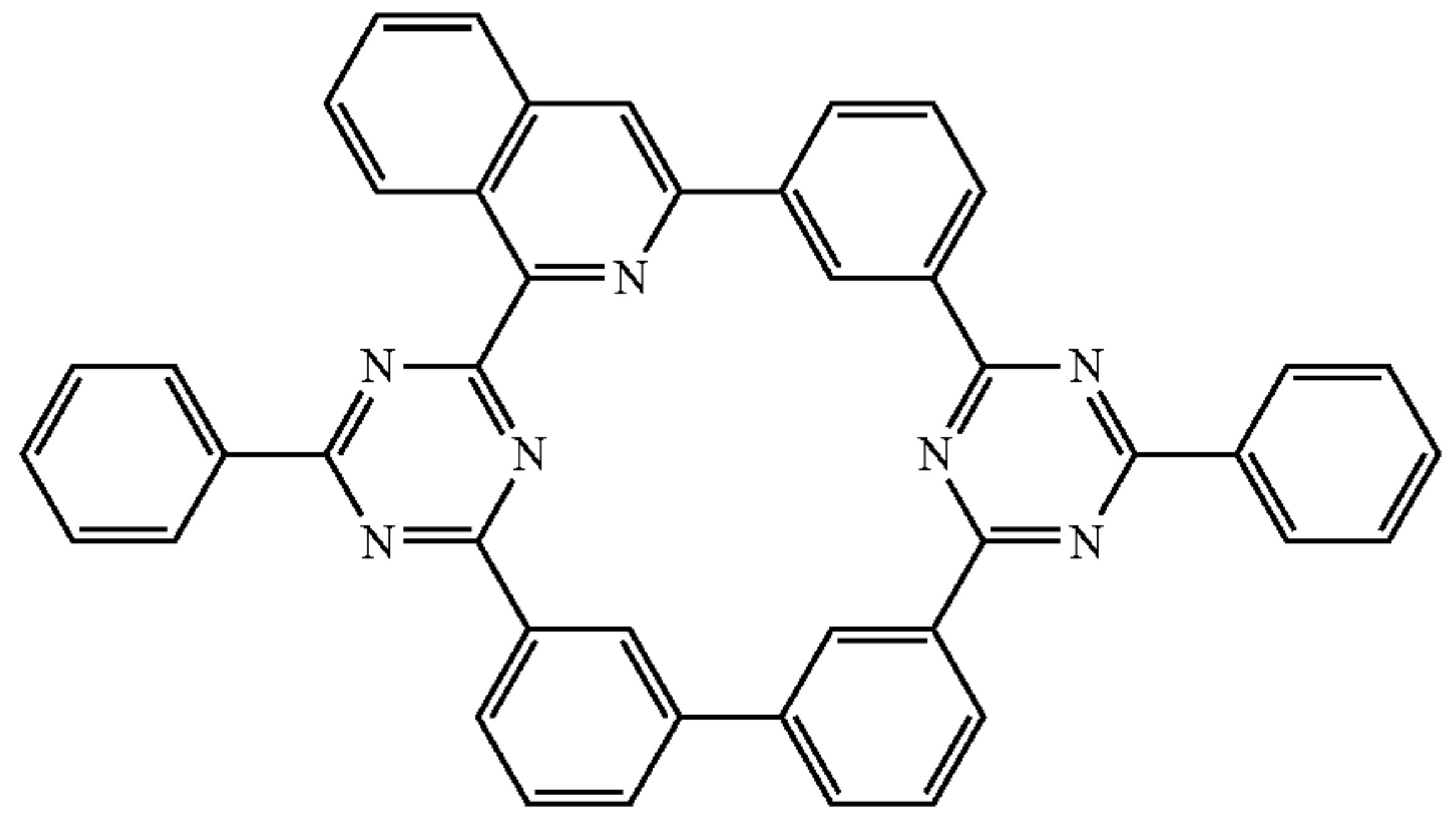
Compound 60
