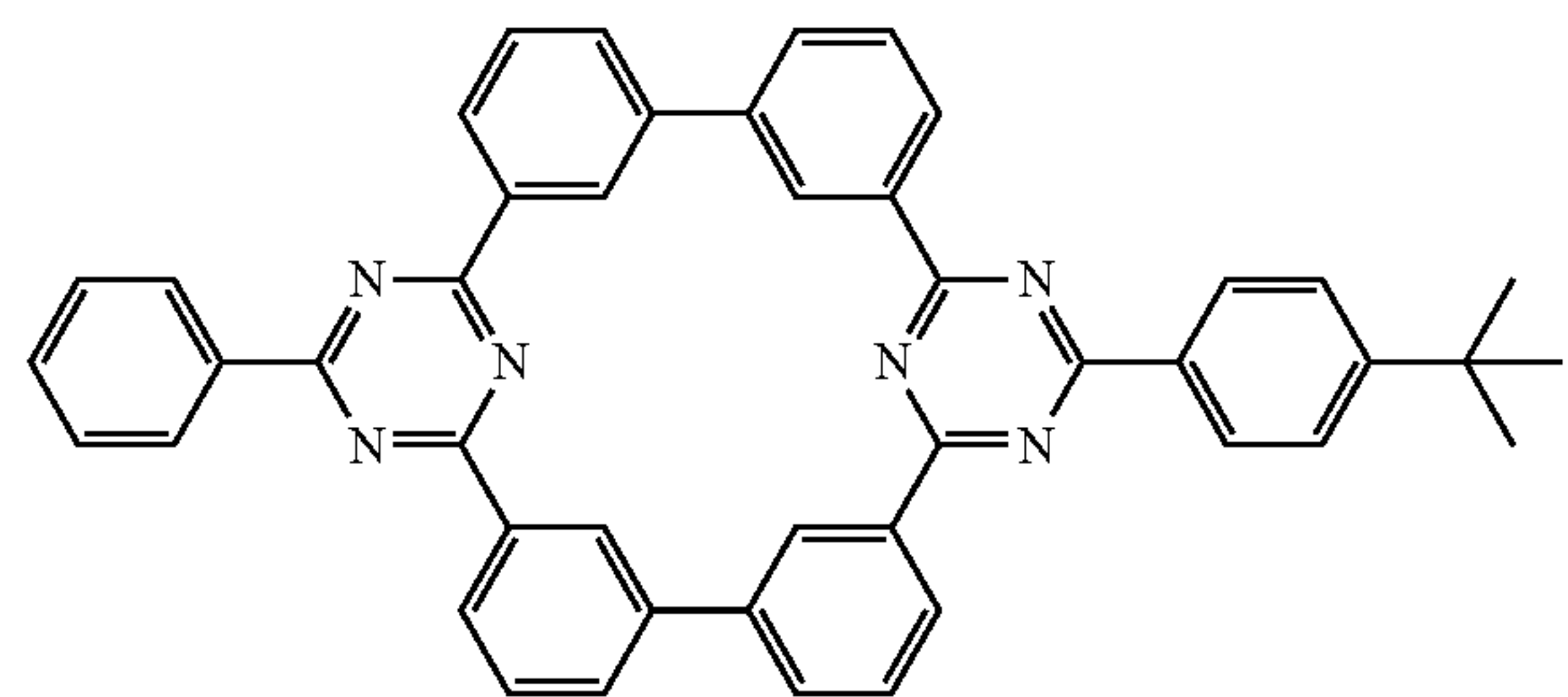
Compound 27
