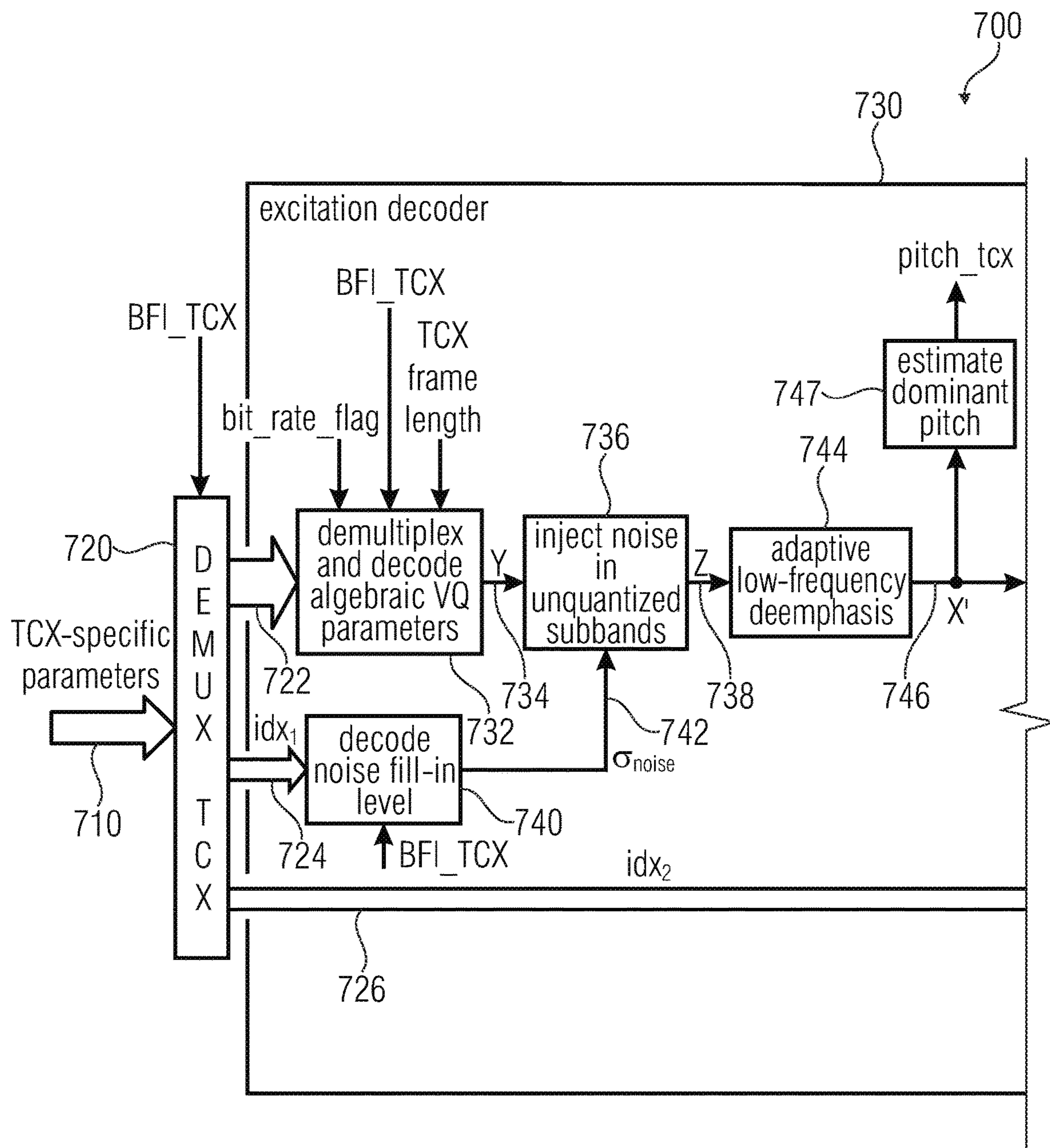
Block diagram of the TCX decoder
