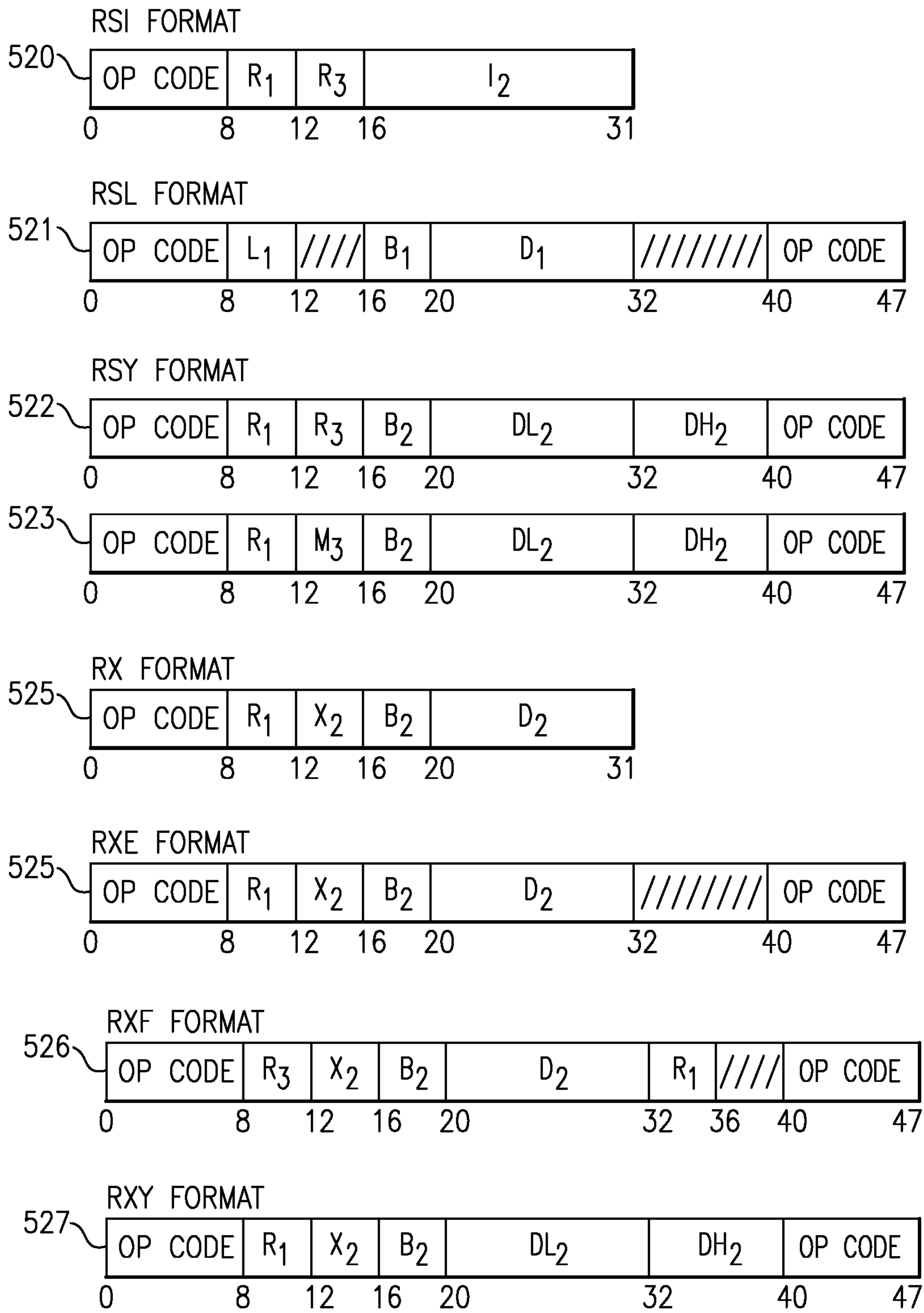
FIG.5C
