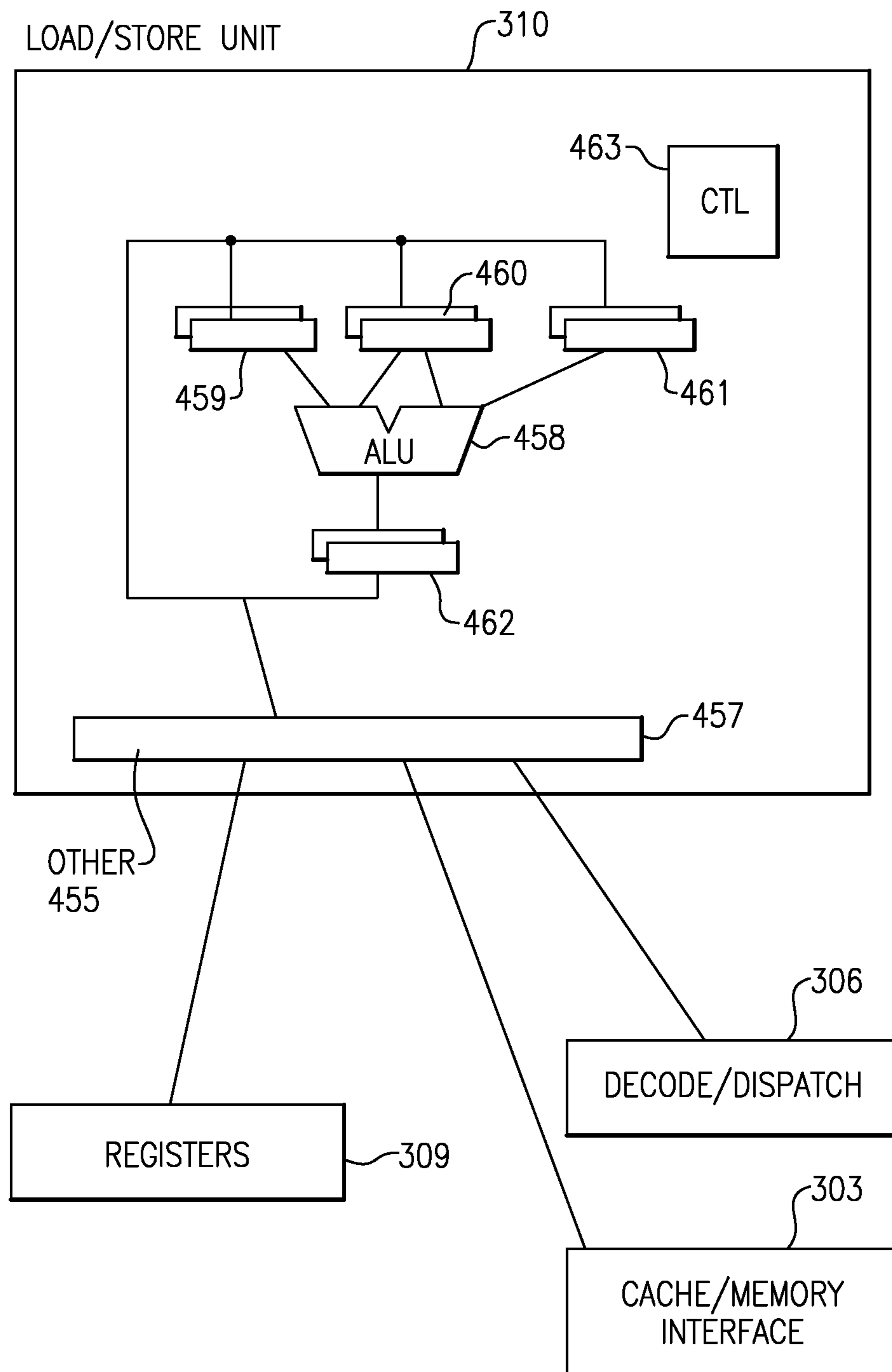
FIG.4C Prior Art
