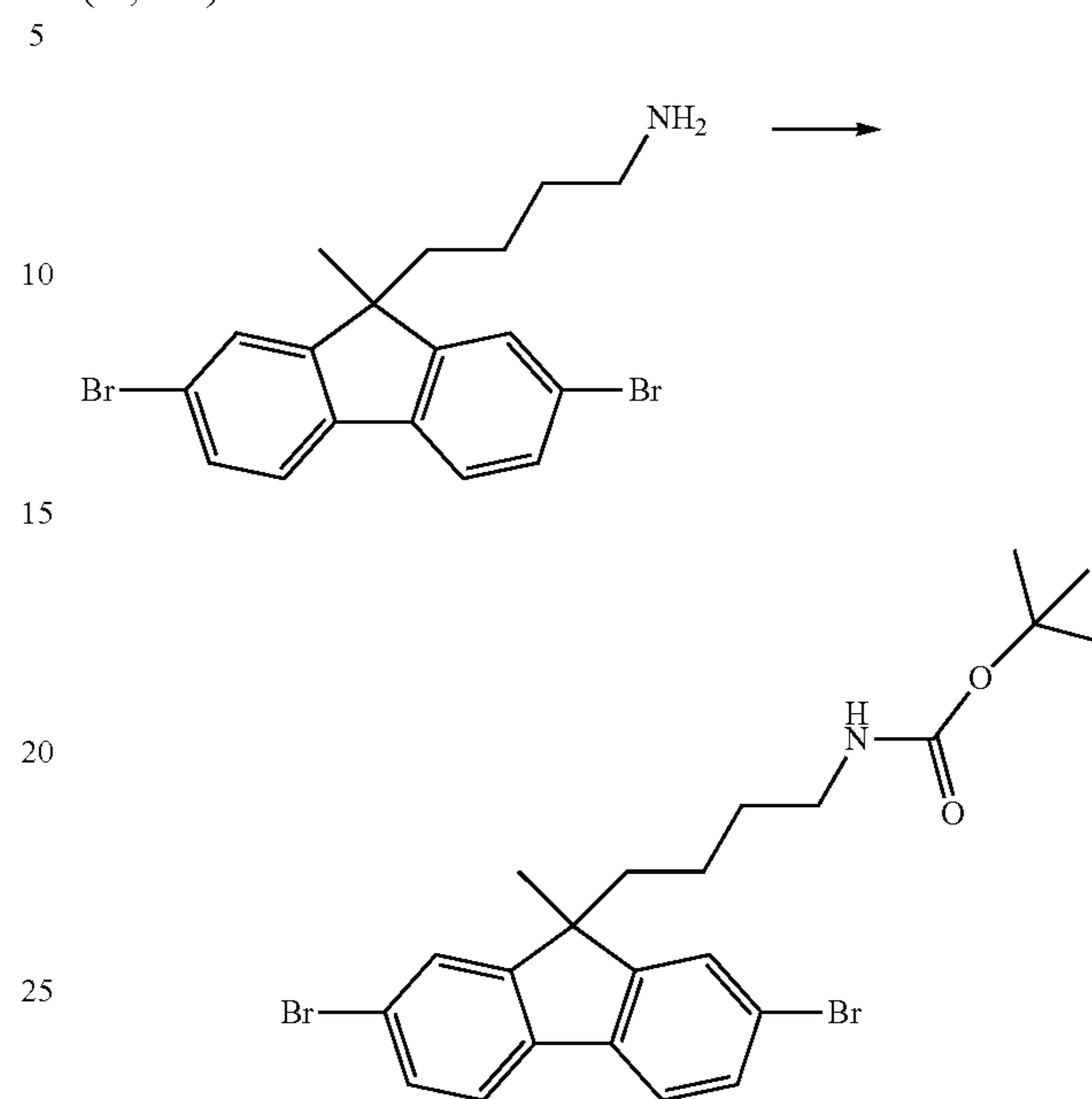
Step 4: tert-butyl-4-(2,7-dibromo-9-methyl-9H-fluoren-9-yl)butylcarbamate
