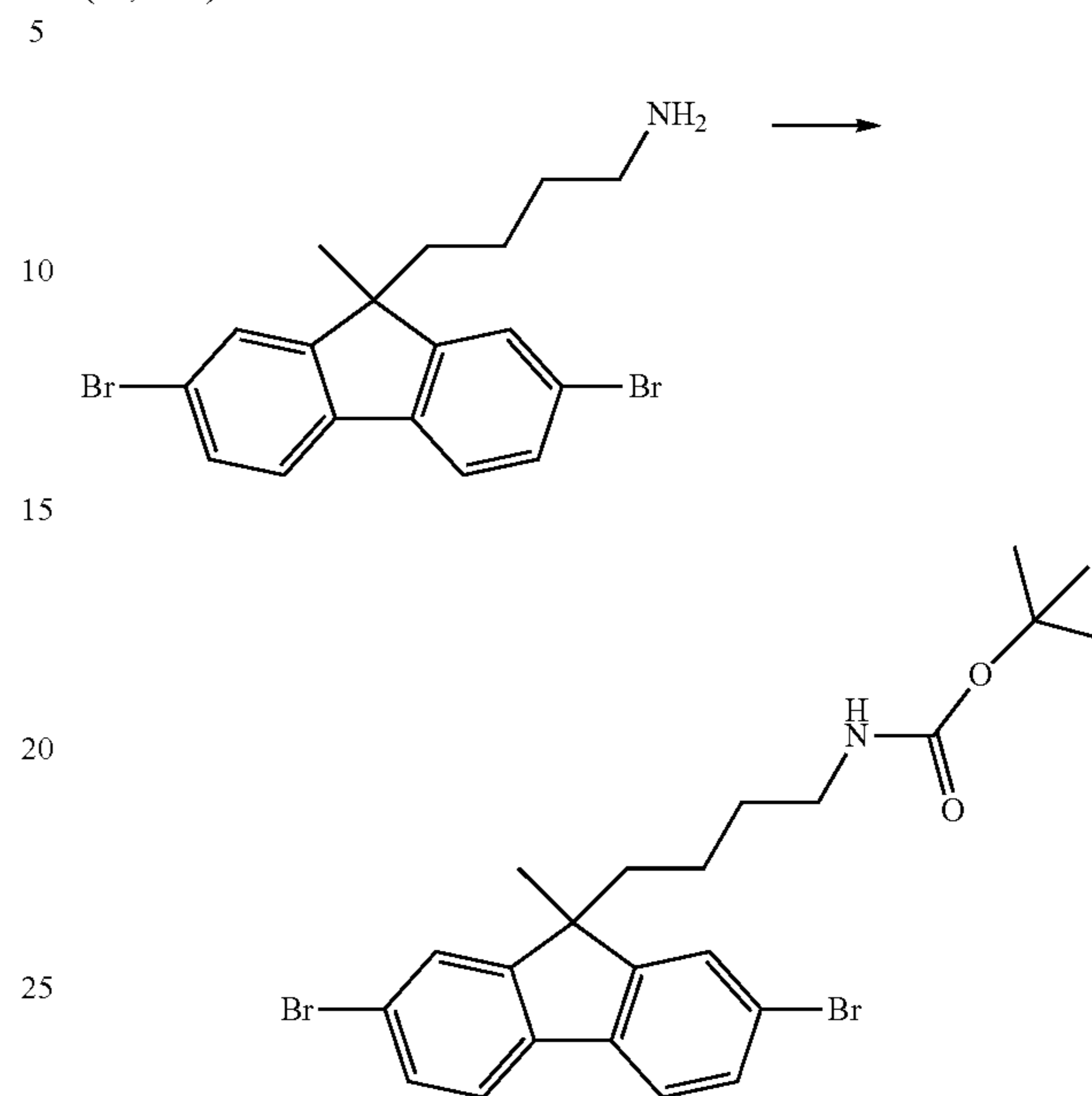
Step 4: tert-butyl-4-(2,7-dibromo-9-methyl-9H-fluoren-9-yl)butylcarbamate
