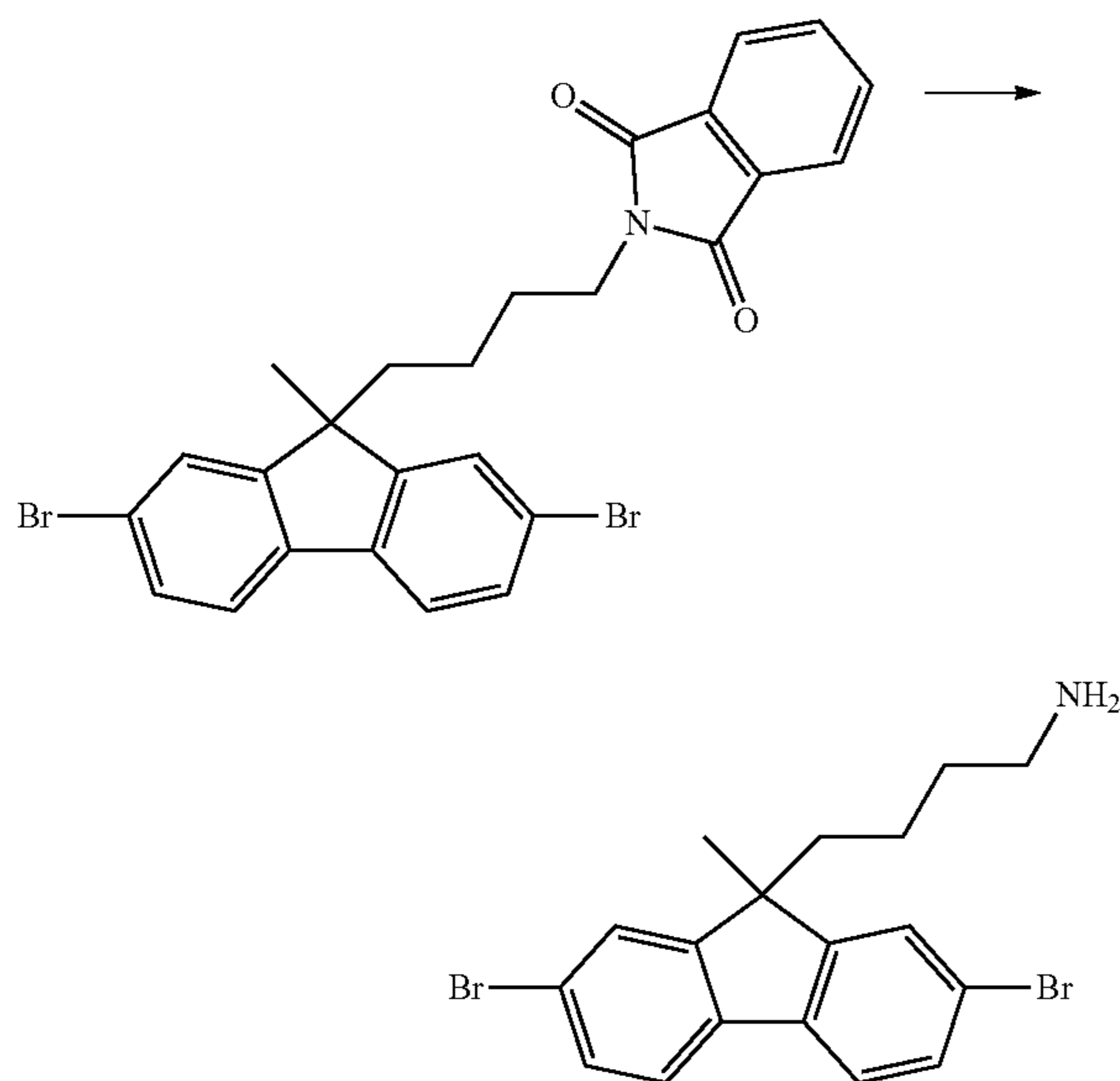
Step 3: 4-(2,7-dibromo-9-methyl-9H-fluoren-9-yl)butan-1-amine
