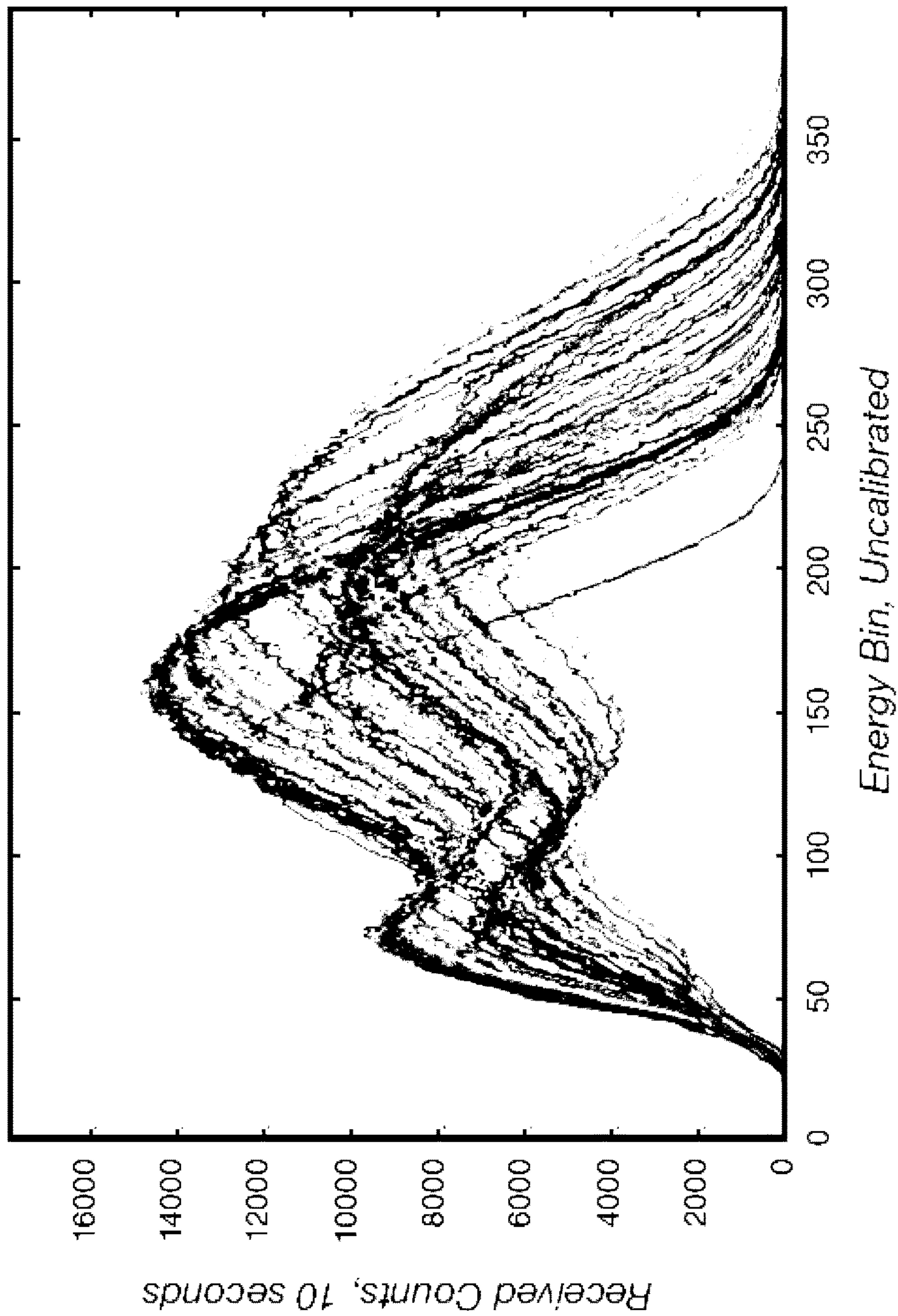
Uncalibrated Energy Spectra, 108 Detectors
