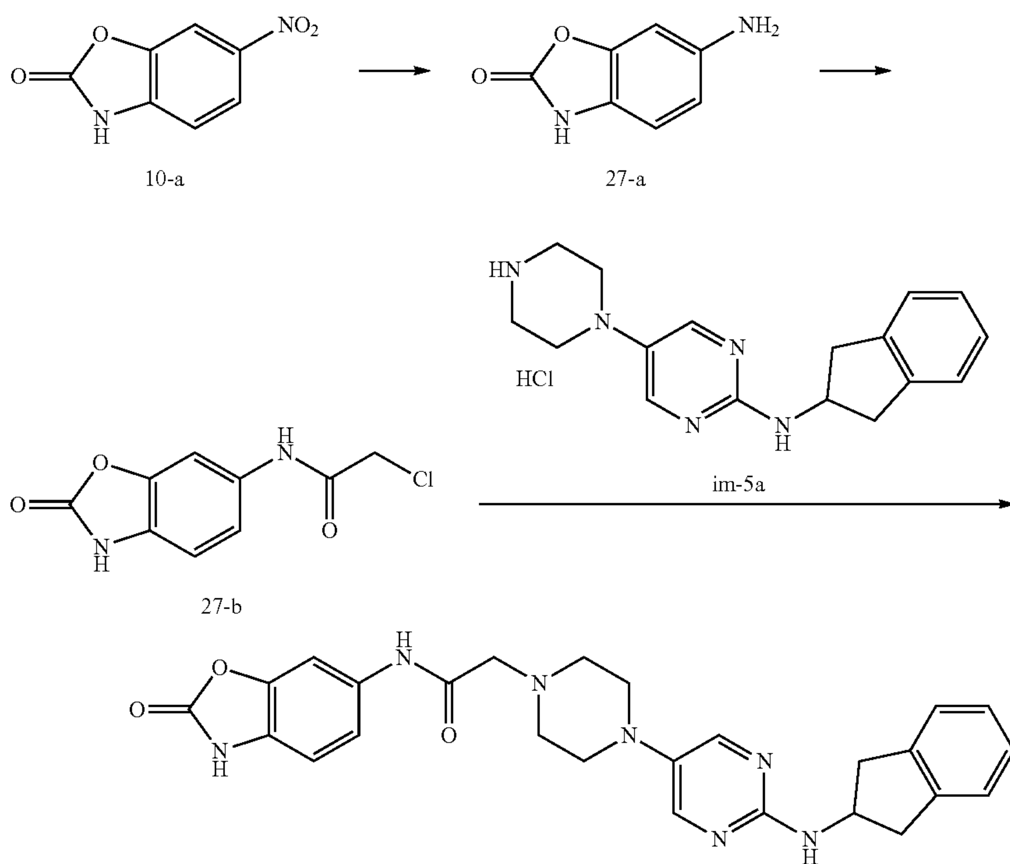
[Reaction scheme 4]
