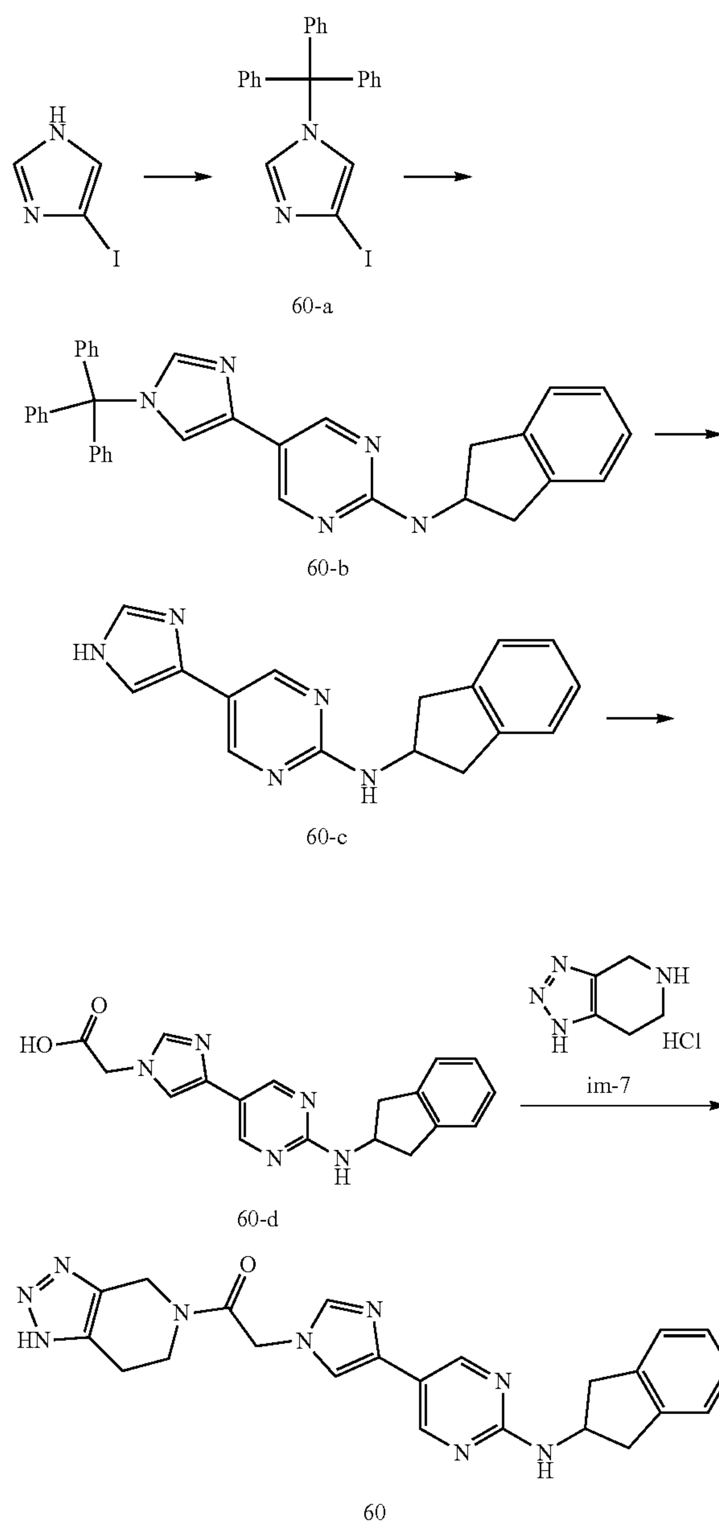
[Reaction scheme 10]
