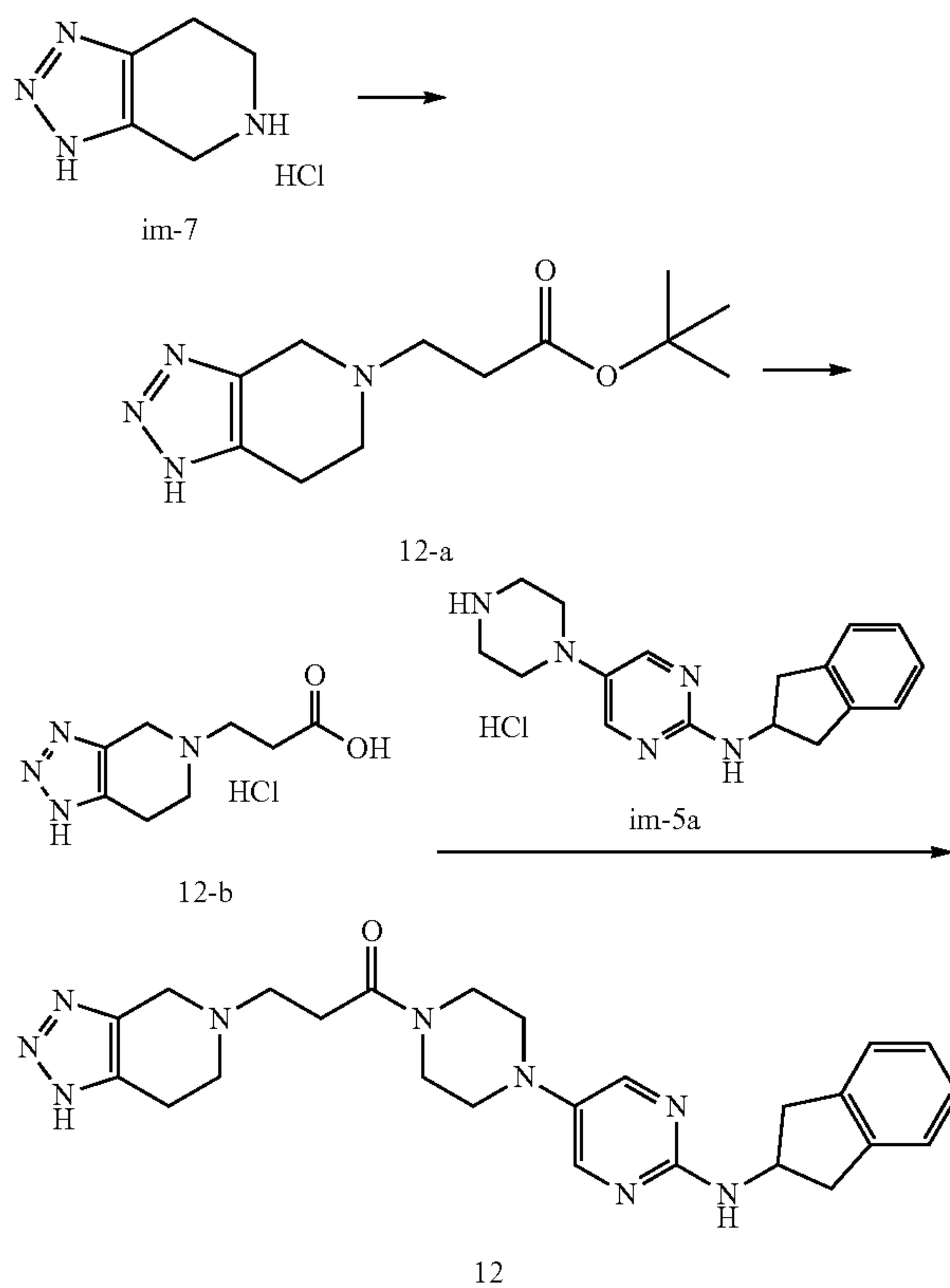
[Reaction scheme 3]
