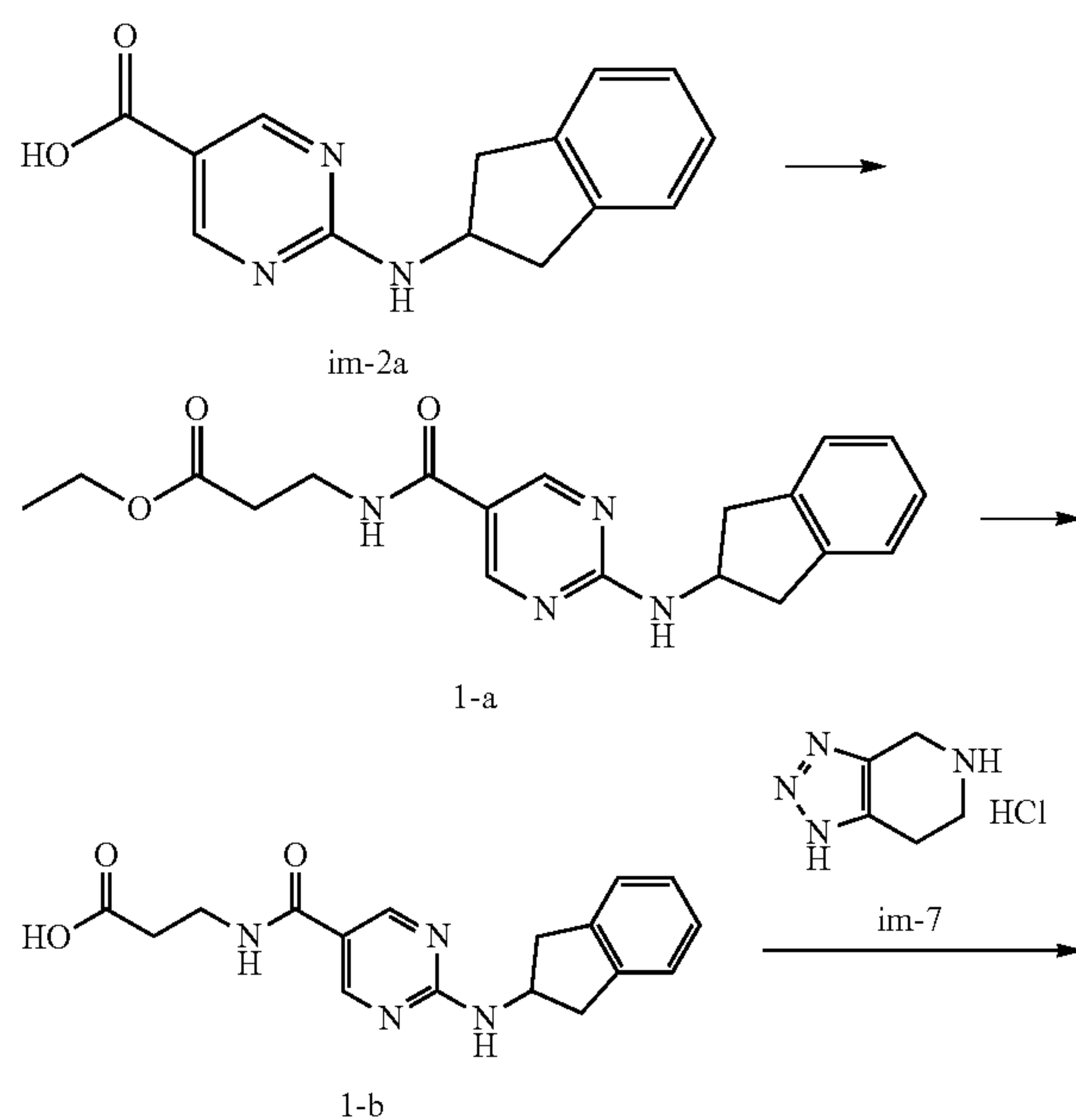
[Reaction scheme 1]
