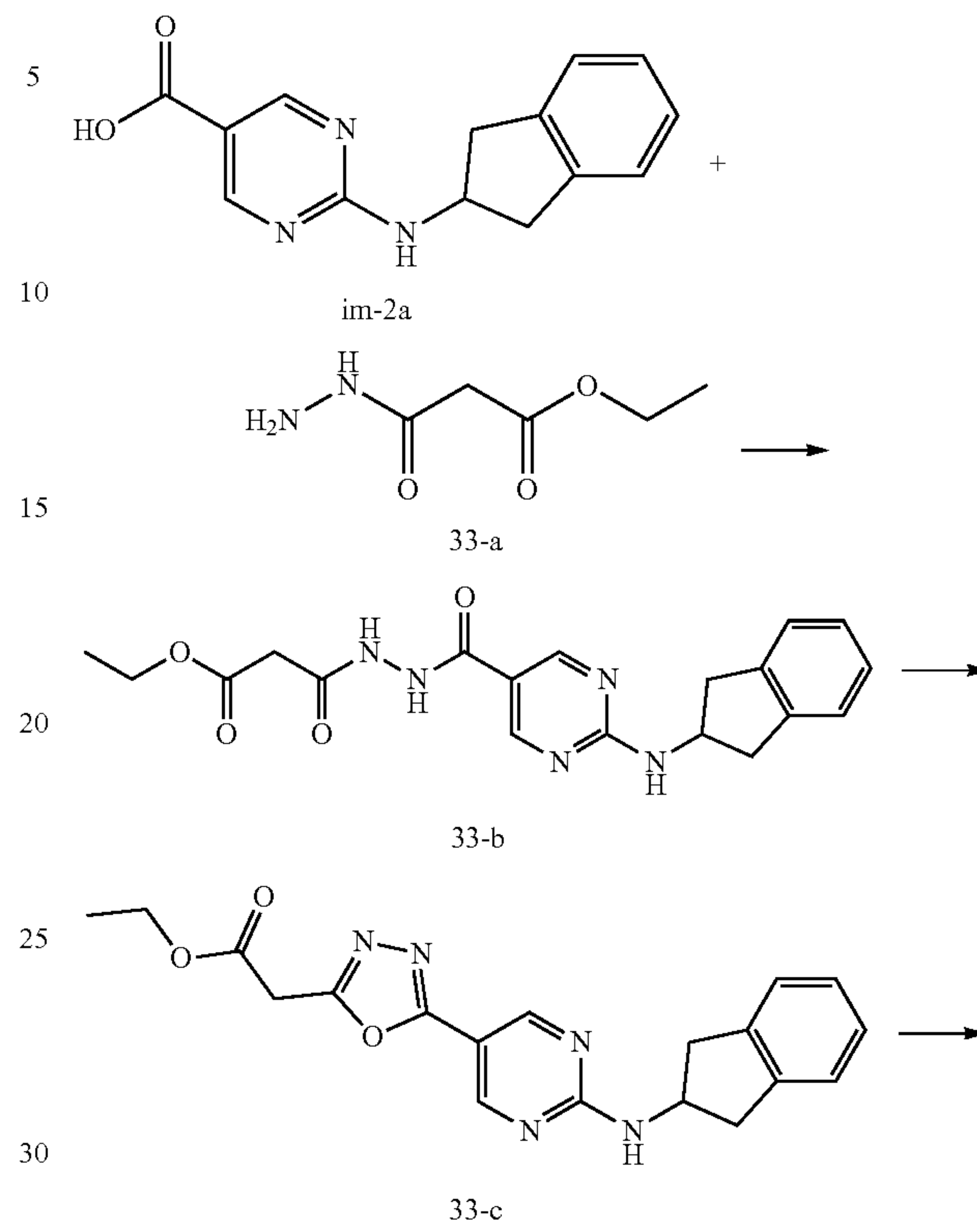
[Reaction scheme 5]
