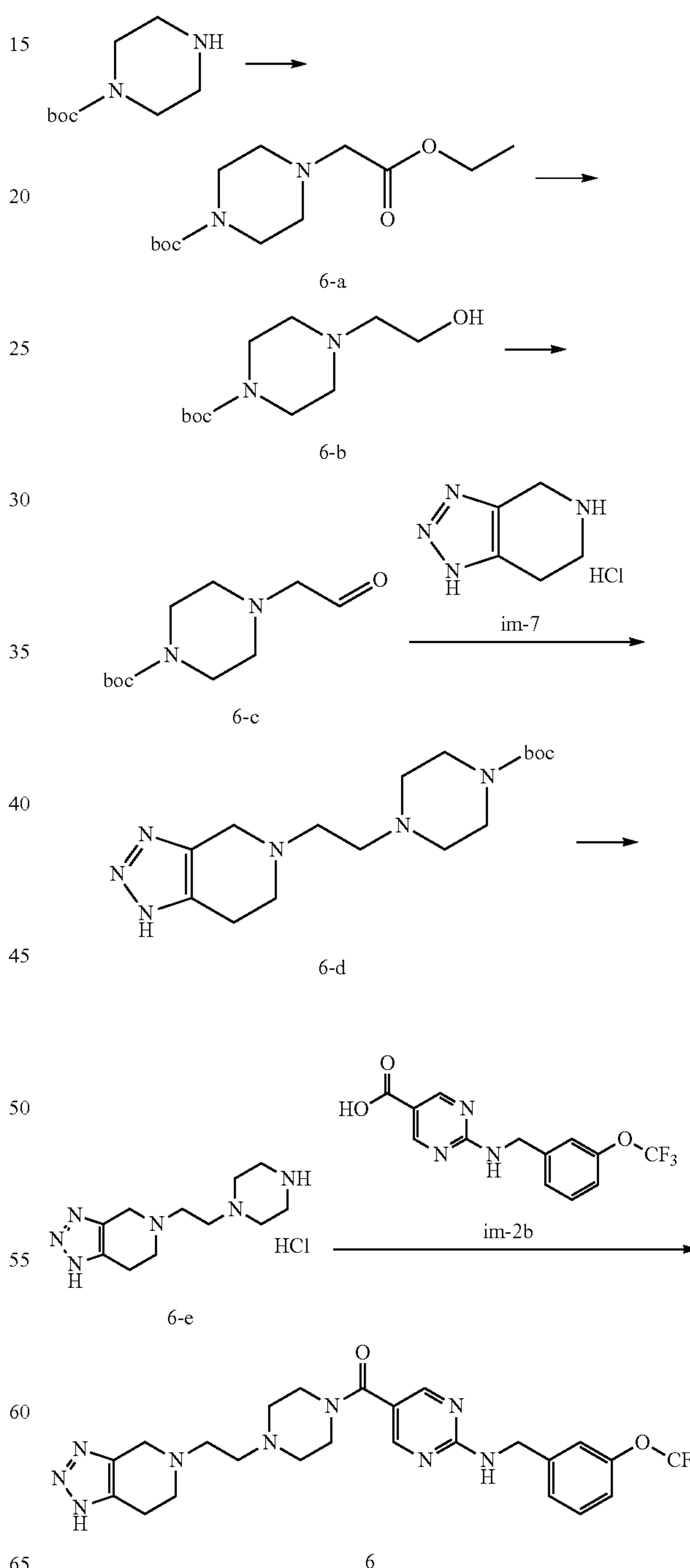
[Reaction scheme 2]
