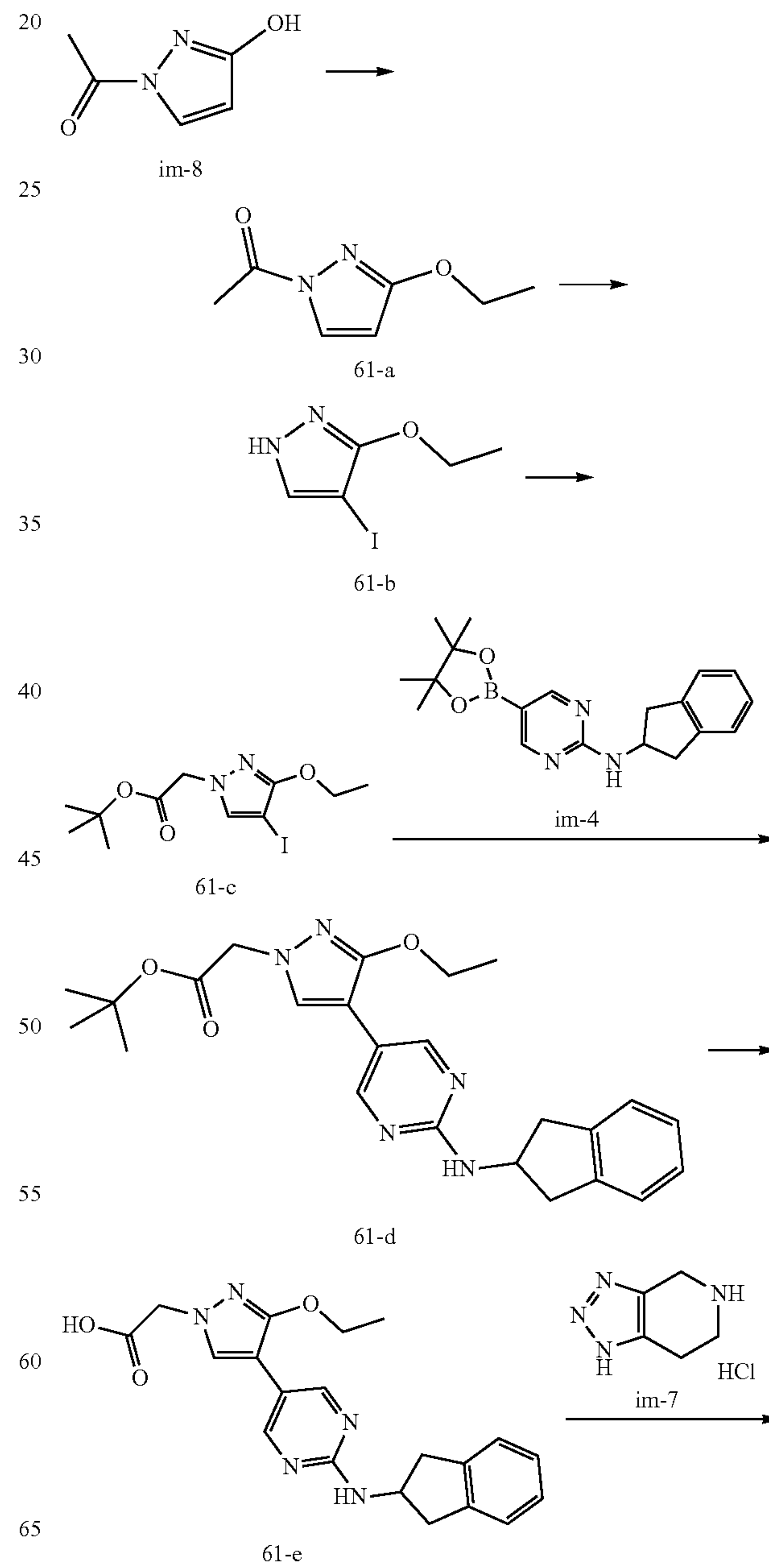
[Reaction scheme 11]
