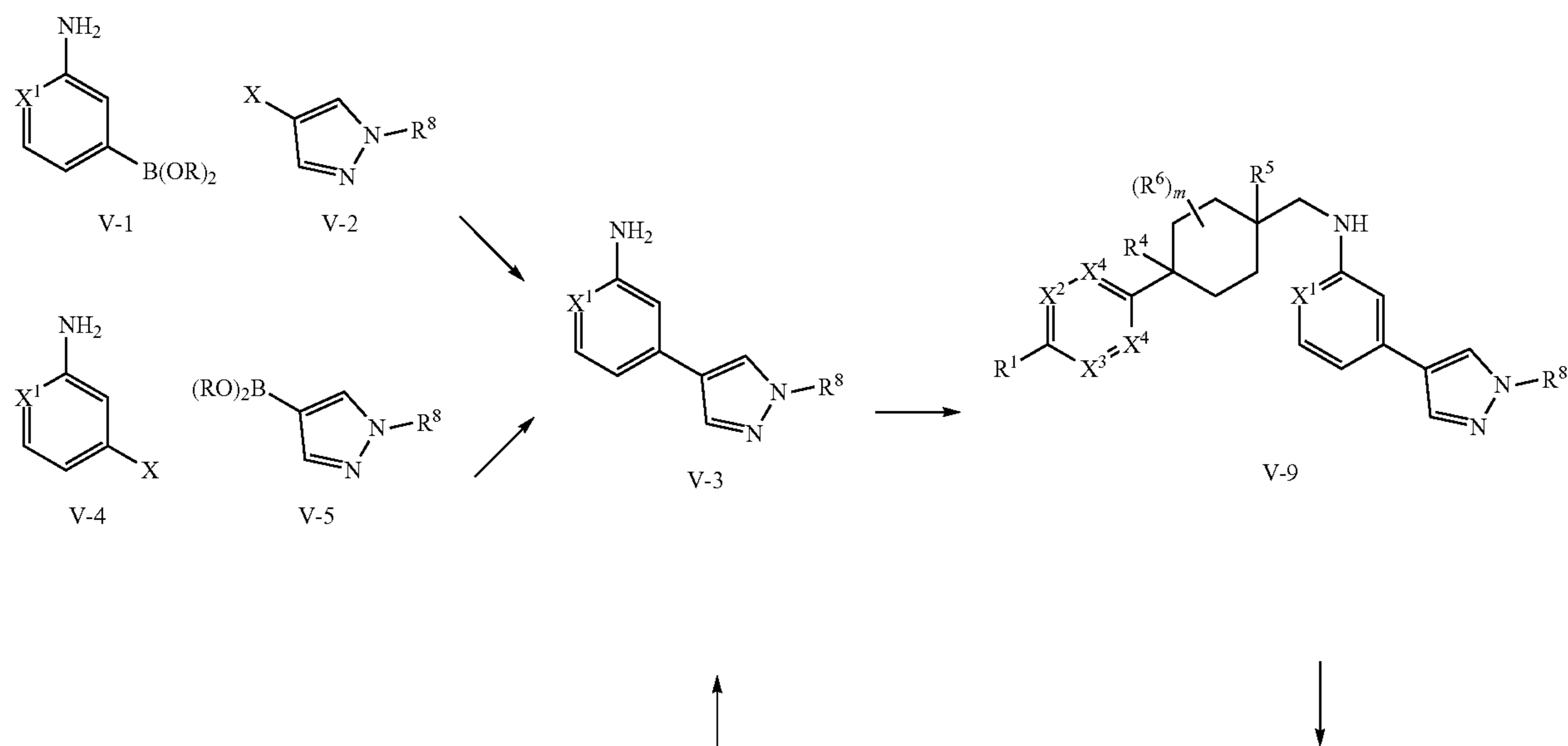
Scheme 5
