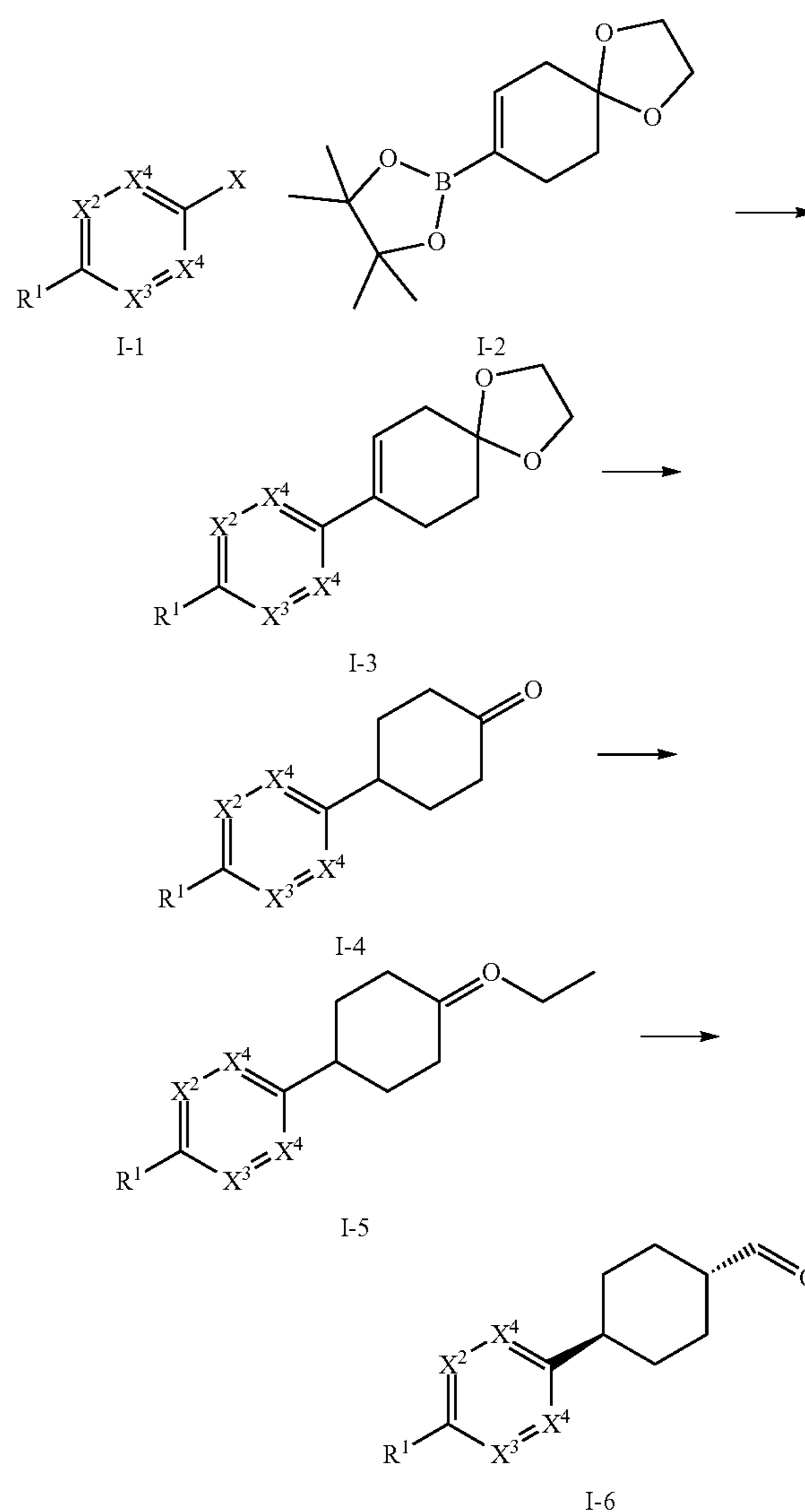
Scheme 1
