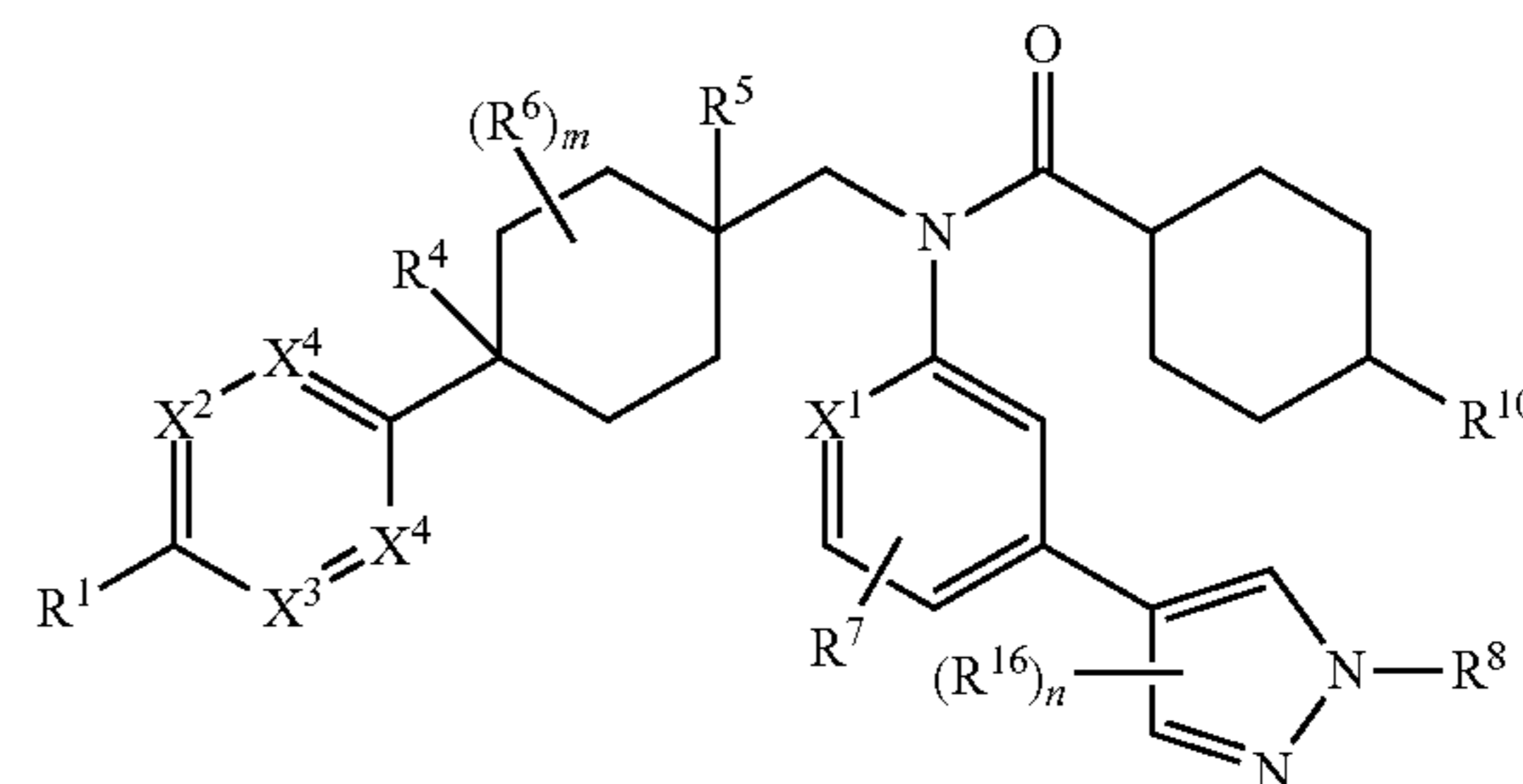
Formula (III)
