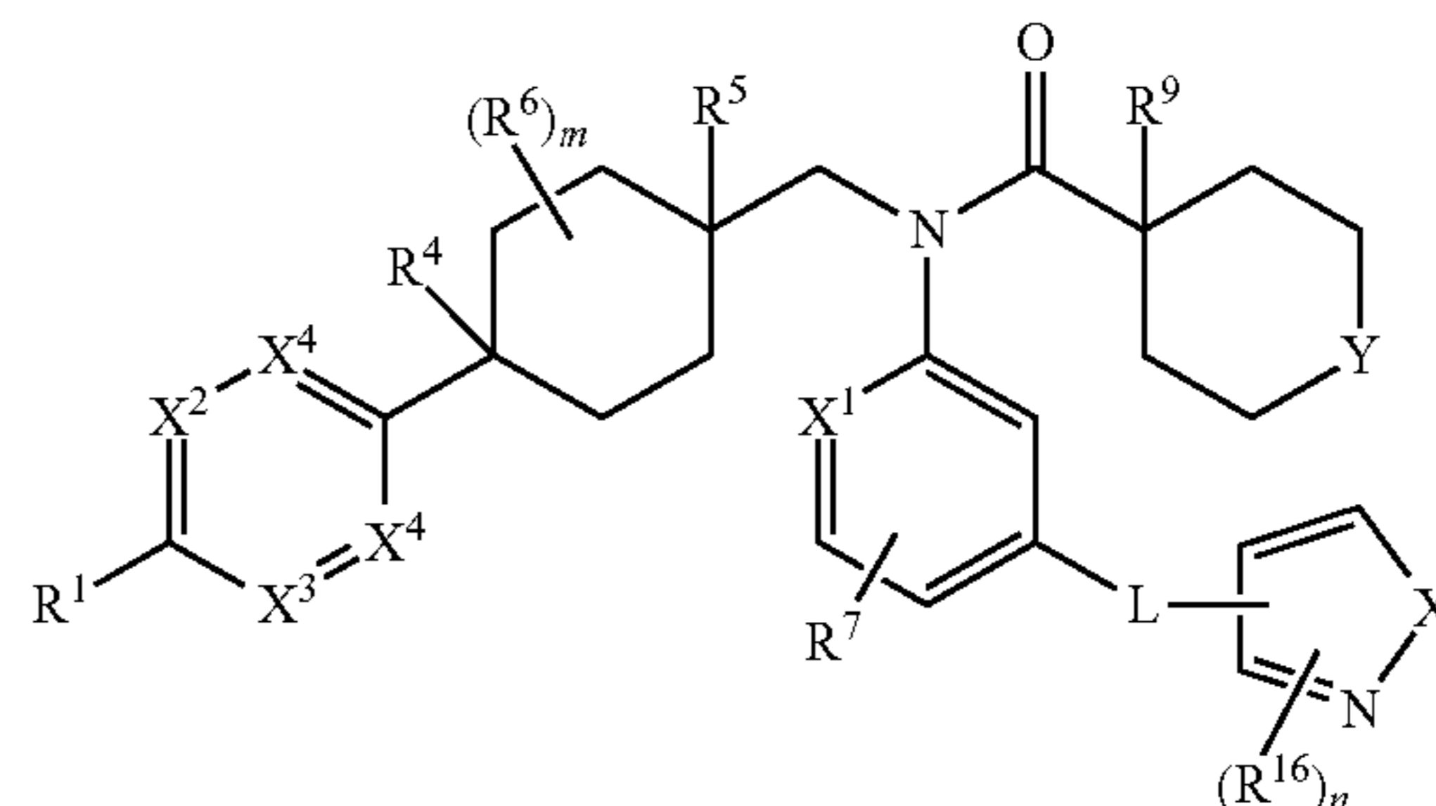
Formula (I)
