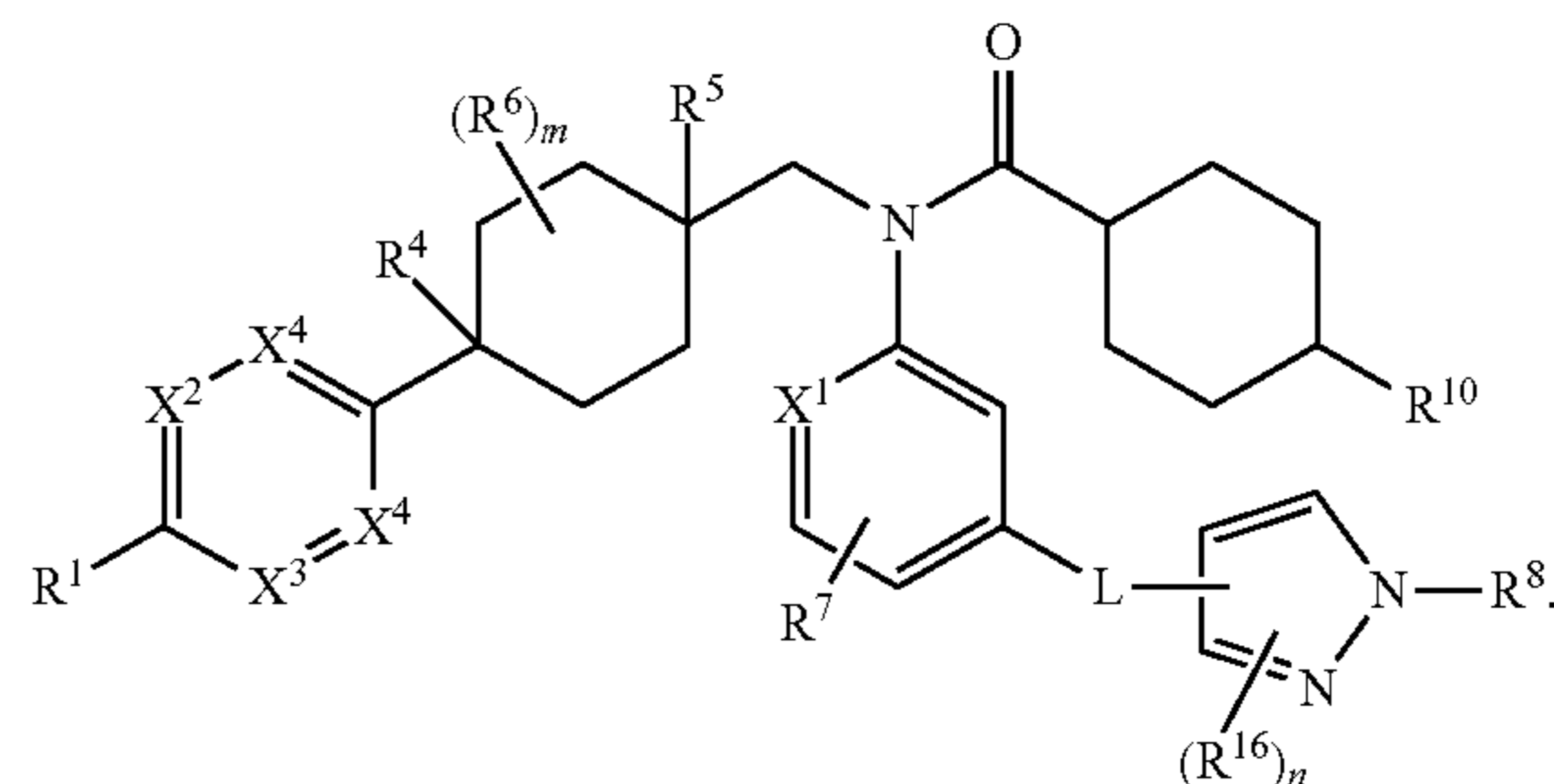
Formula (II)
