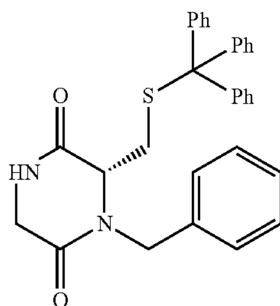
(6R)-1-benzyl-6-[(triphenylmethyl)sulfanyl]piperazine-2,5-dione
