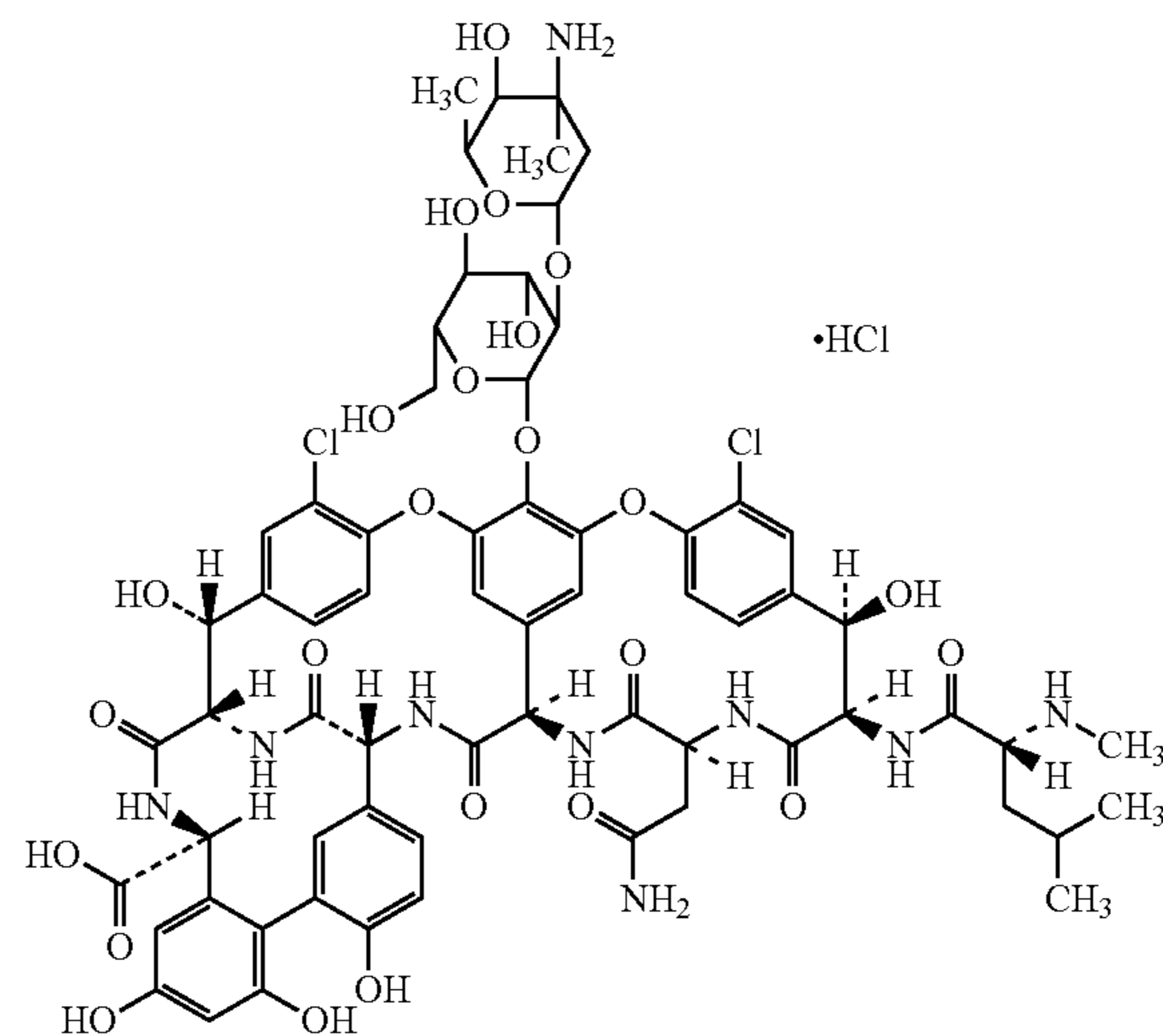
Vancomycin hydrochloride
