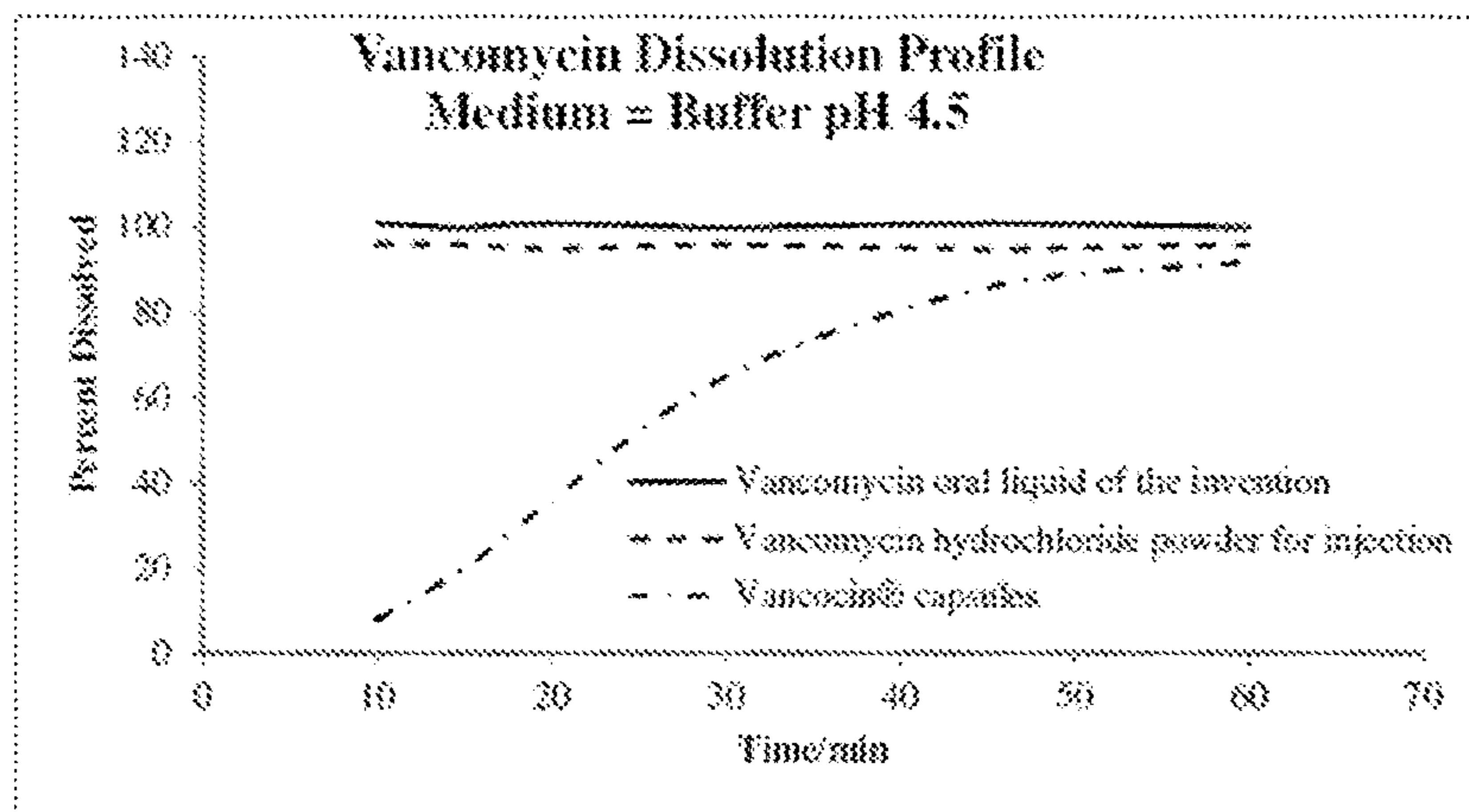
FIG. 4 Vancomycin Dissolution Profile in Buffer pH 4.5
