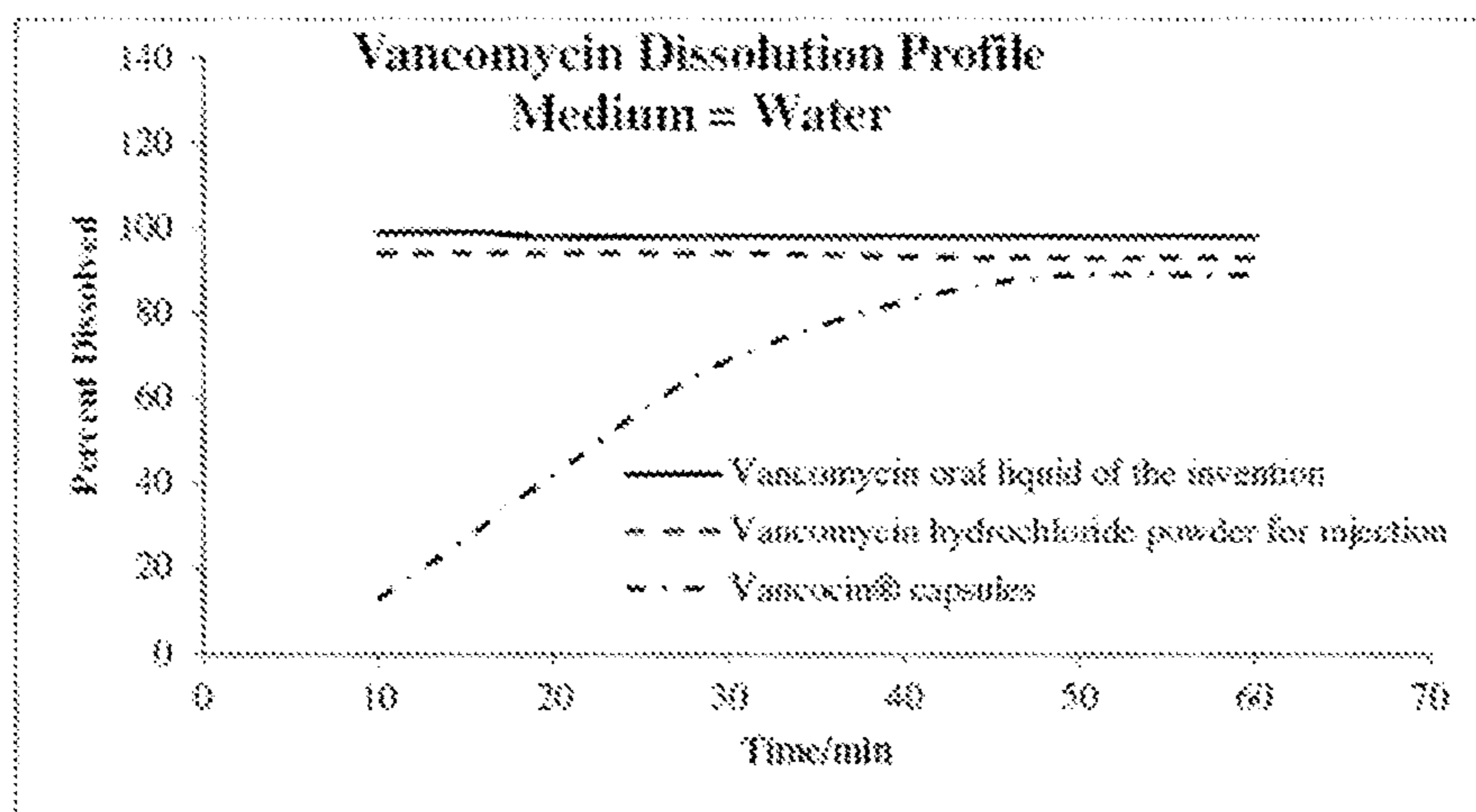
FIG. 3 Vancomycin Dissolution Profile in Water
