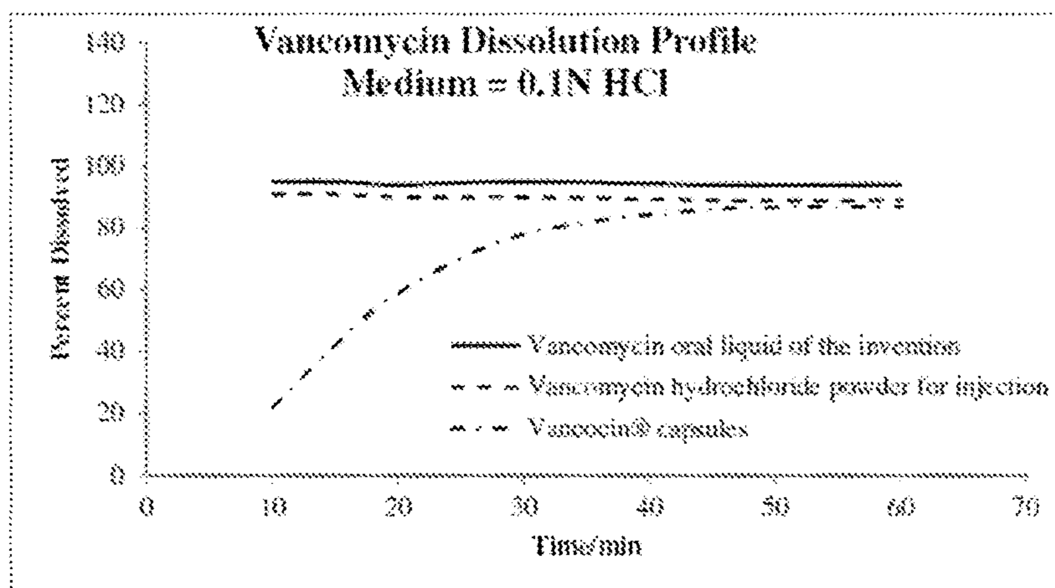
FIG. 6 Vancomycin Dissolution Profile in 0.1N HCl
