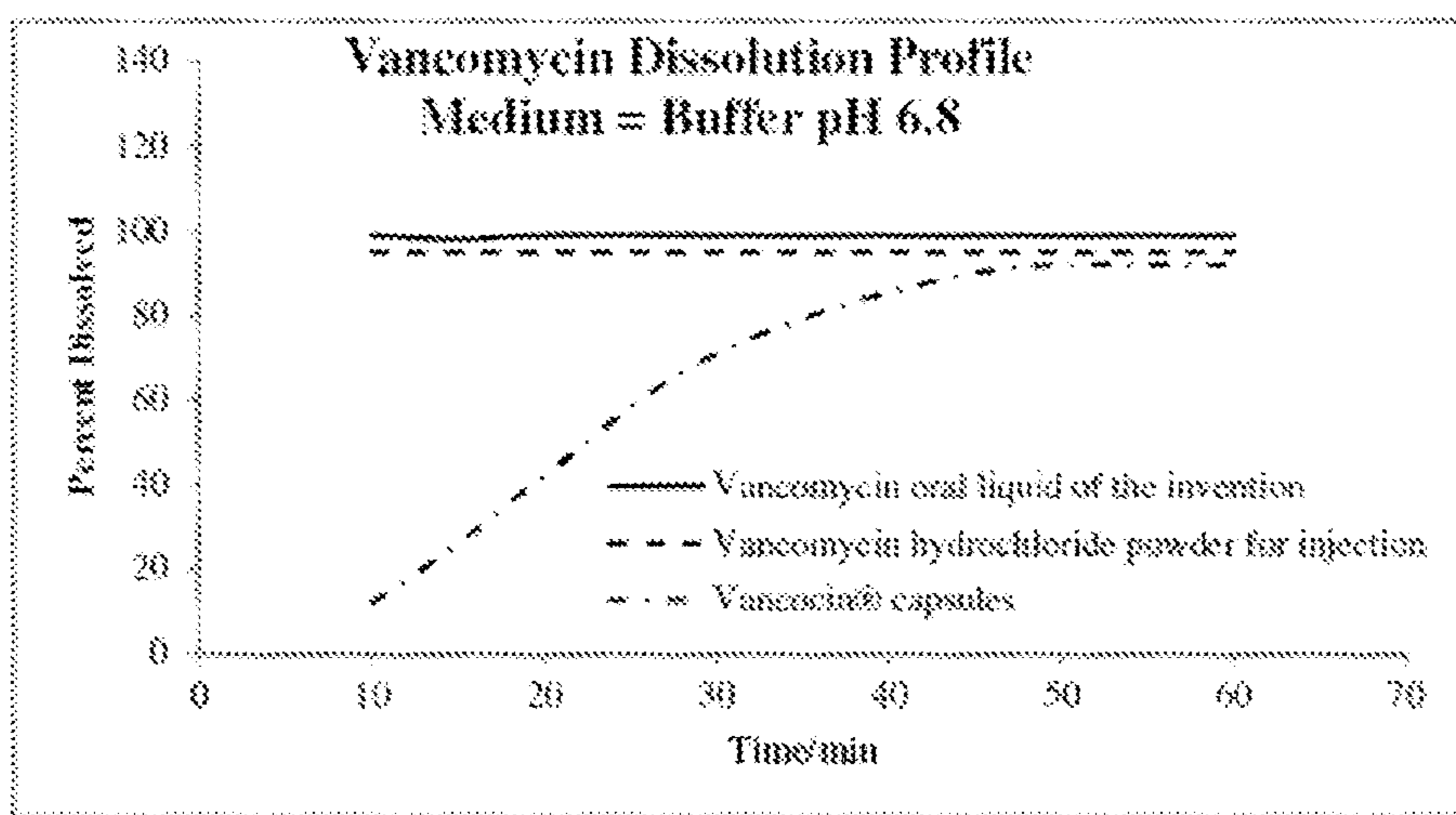
FIG. 5 Vancomycin Dissolution Profile in Buffer pH 6.8
