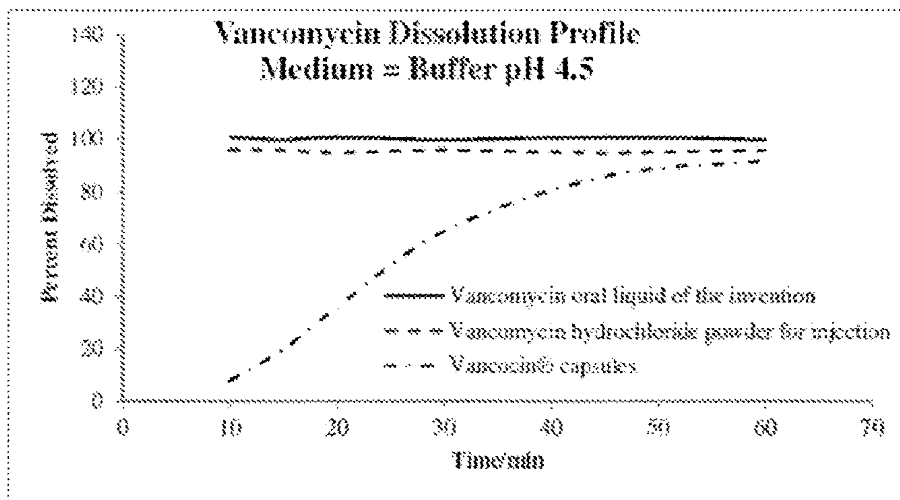
Vancomycin Dissolution Profile in Buffer pH 4.5
