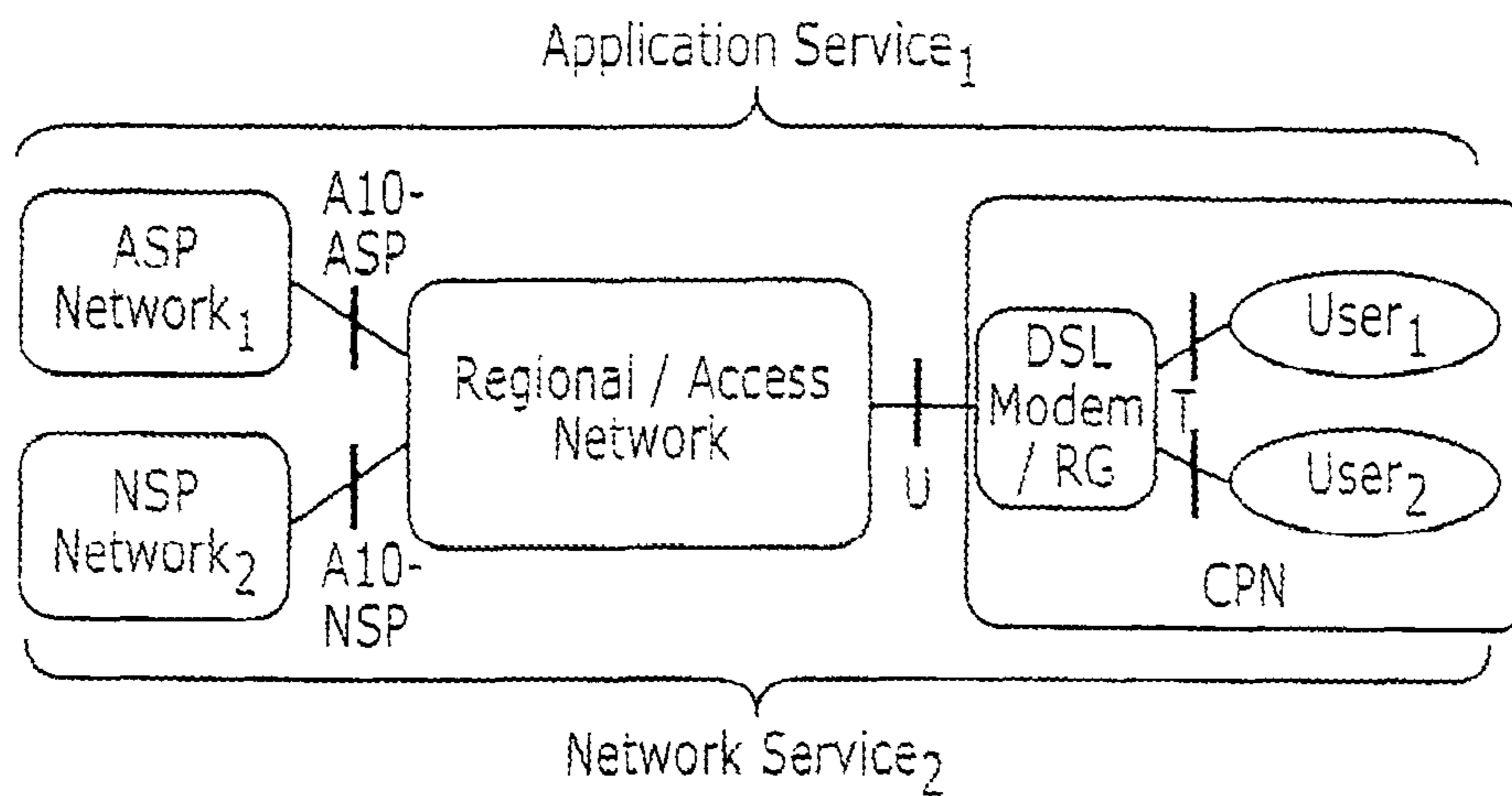
FIGURE 2 (PRIOR ART)
