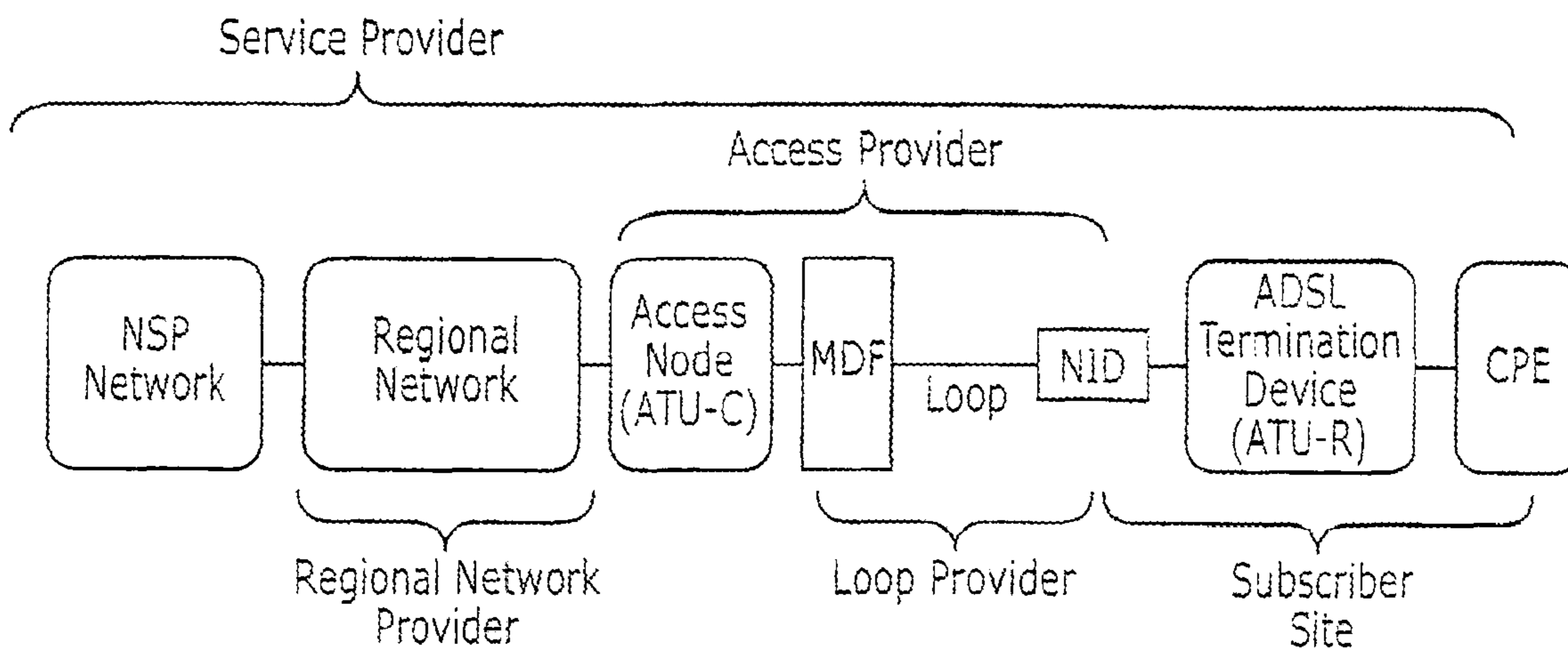
FIGURE 1 (PRIOR ART)
