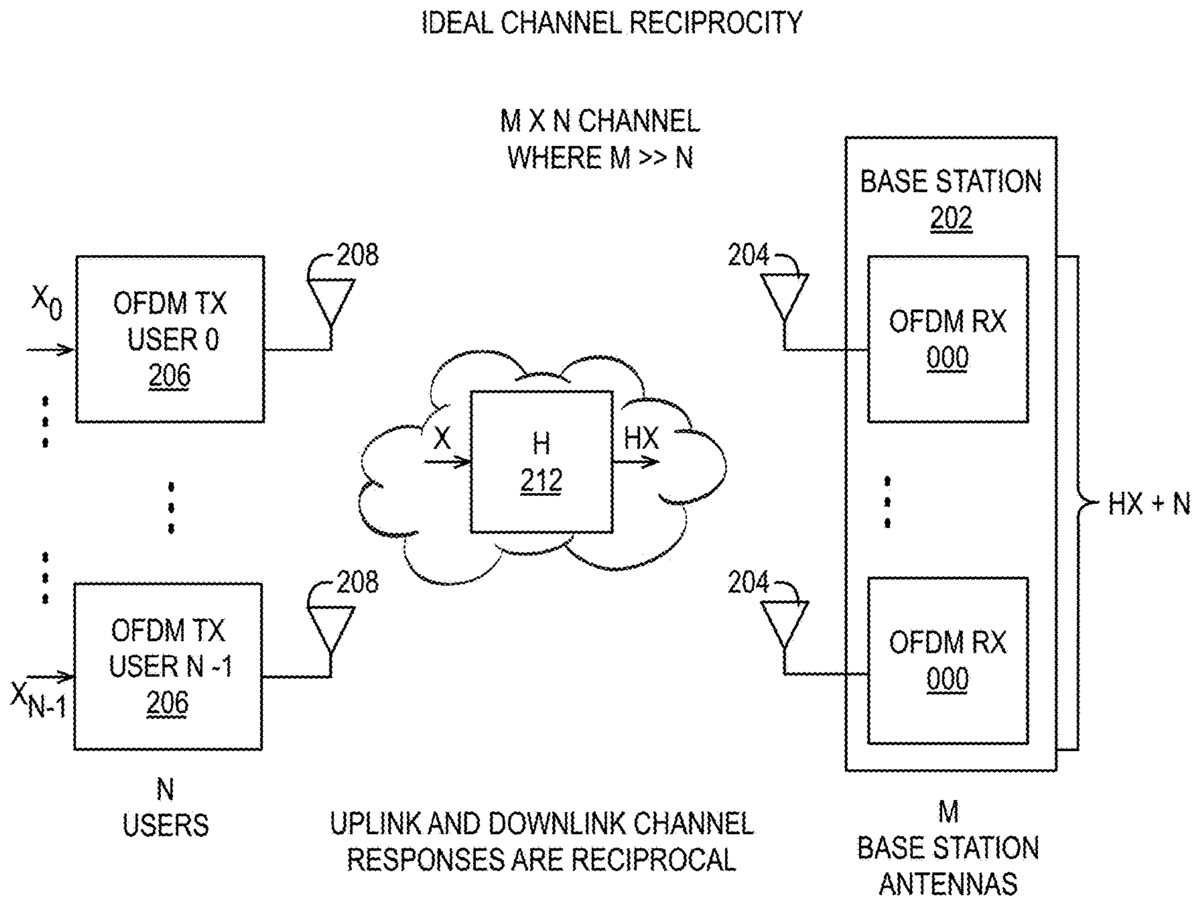
FIG. 2 (Prior Art)
