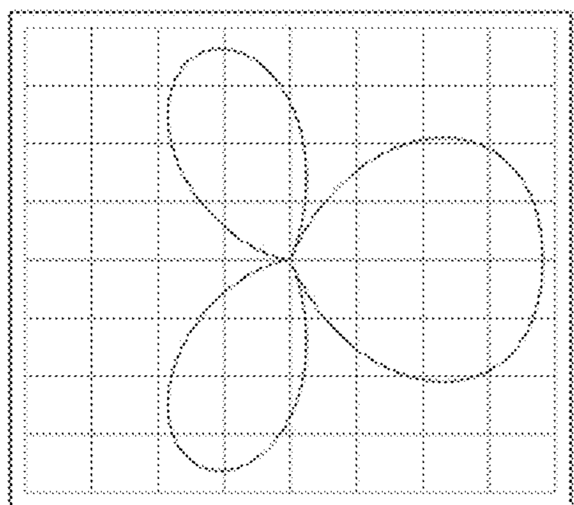
d = 3\lambda/4 \quad \Delta\phi = +90^\circ
