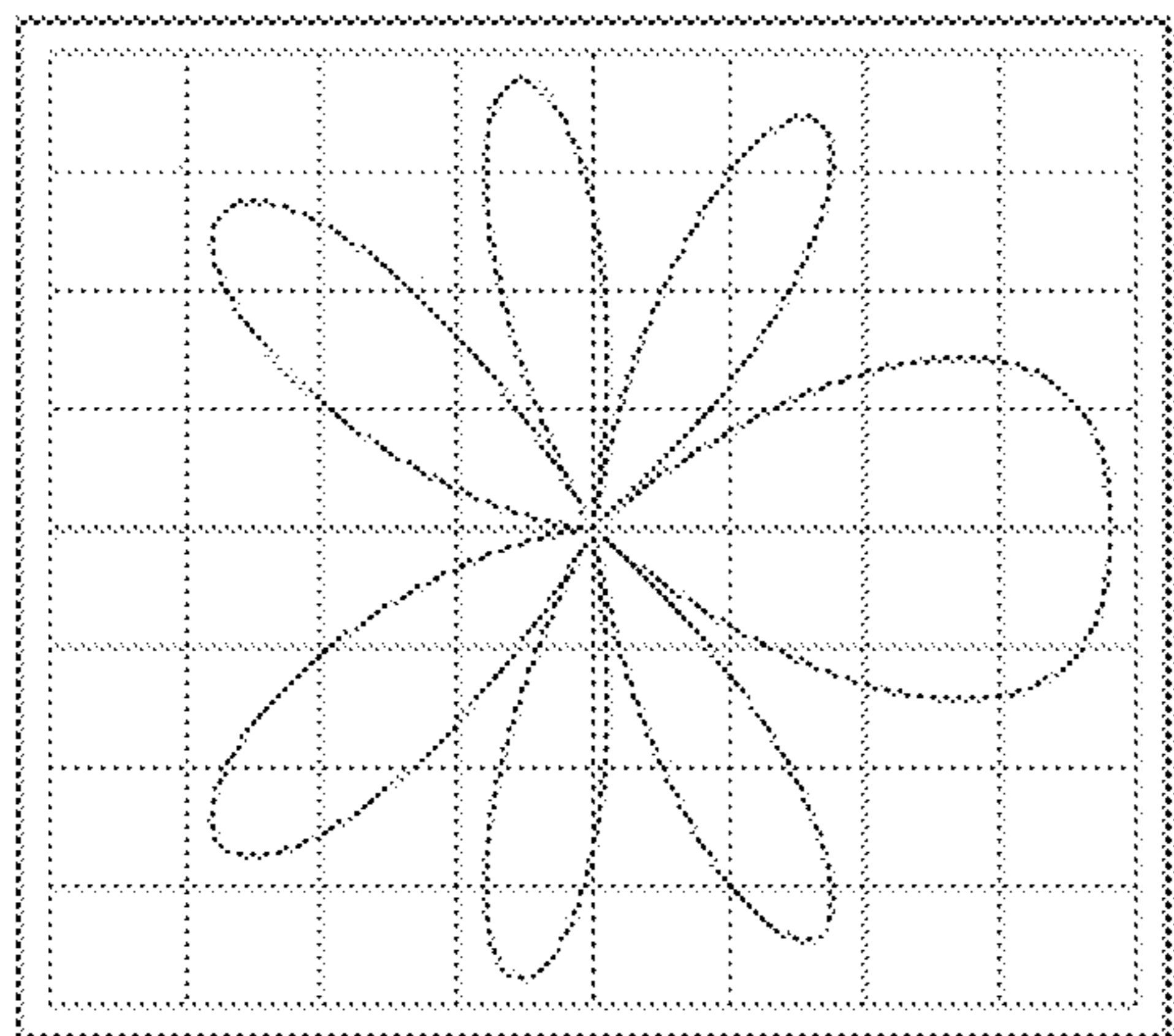
d = 7\lambda/4 \quad \Delta\phi = +90^\circ
