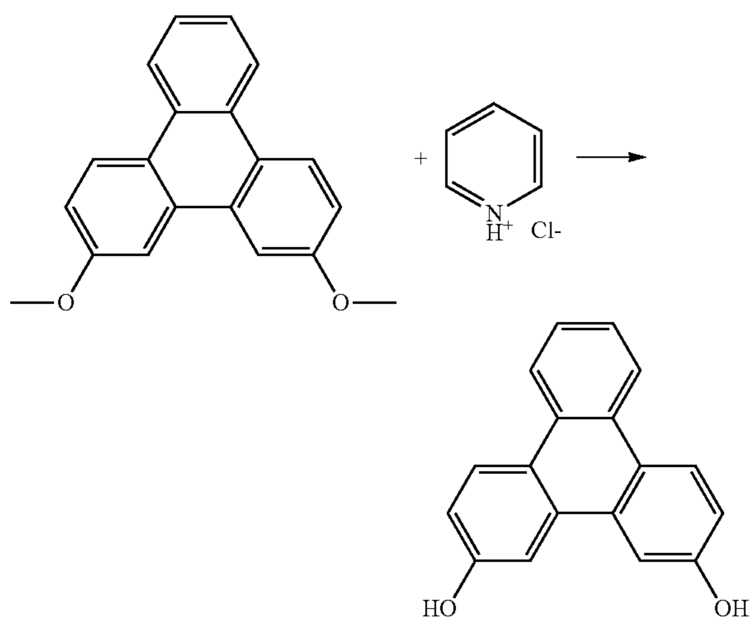
Triphenylene-2,11-diol
