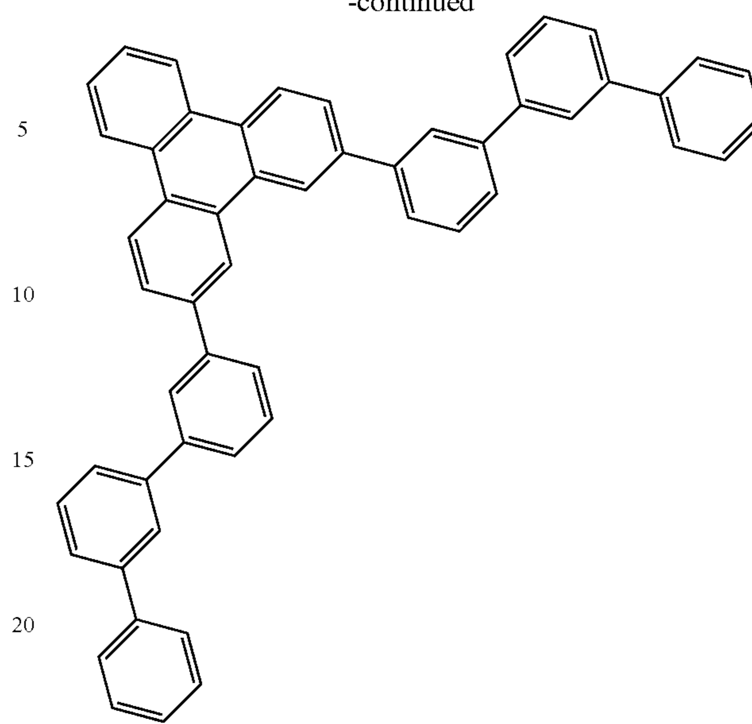
Compound 8
