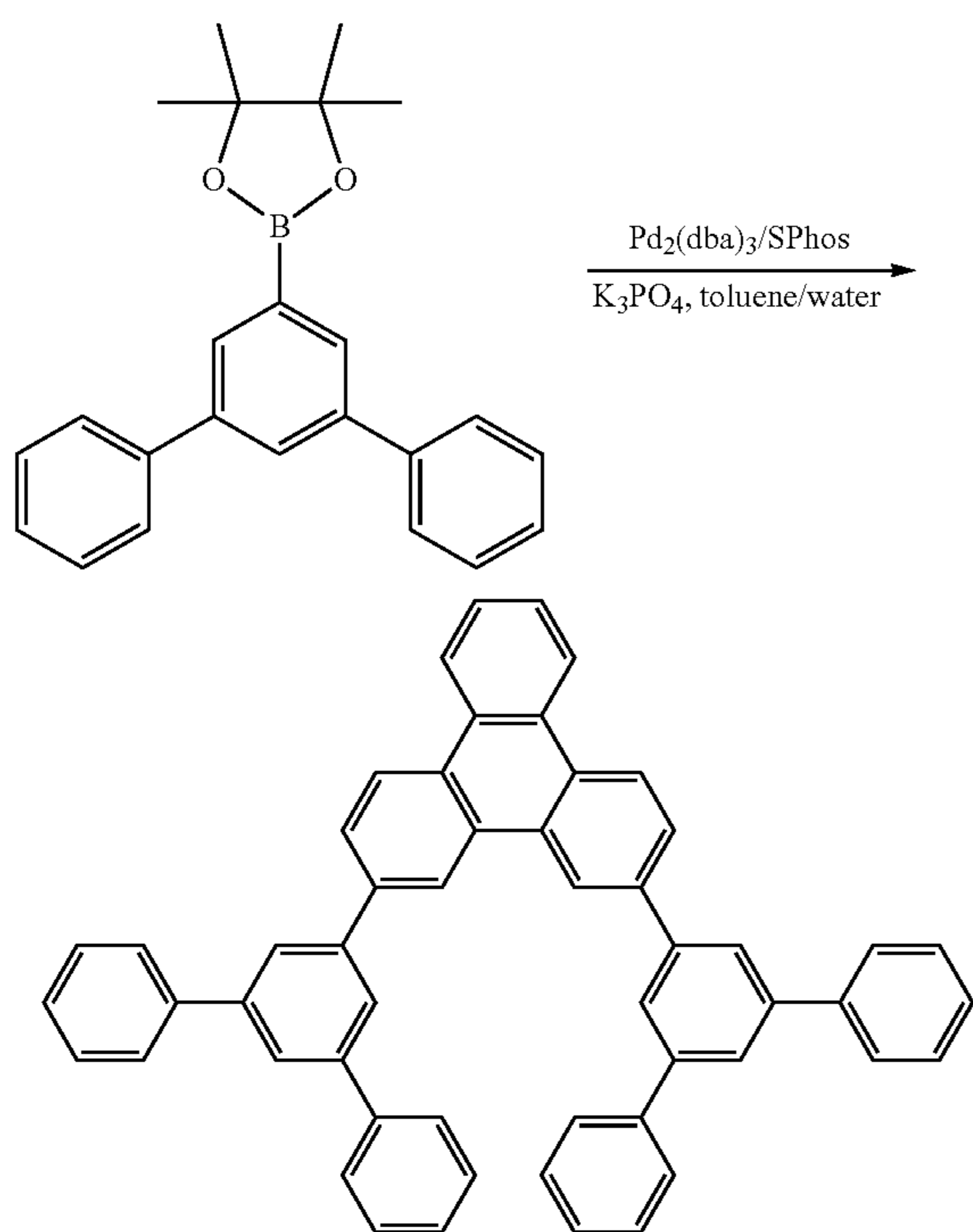
Compound 7
