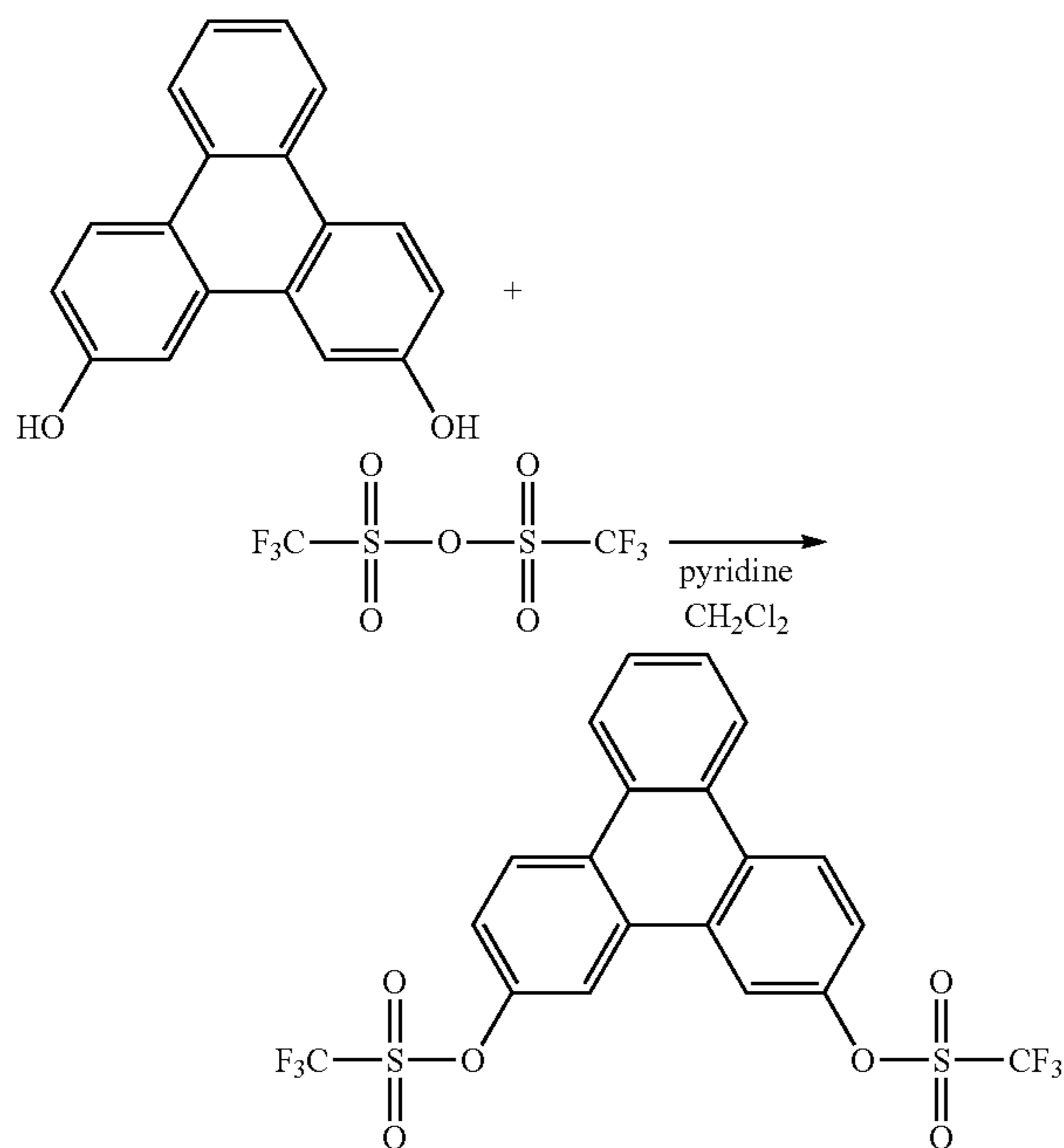
Triphenylene-2,11-dilyl bis(trifluoromethanesulfonate)
