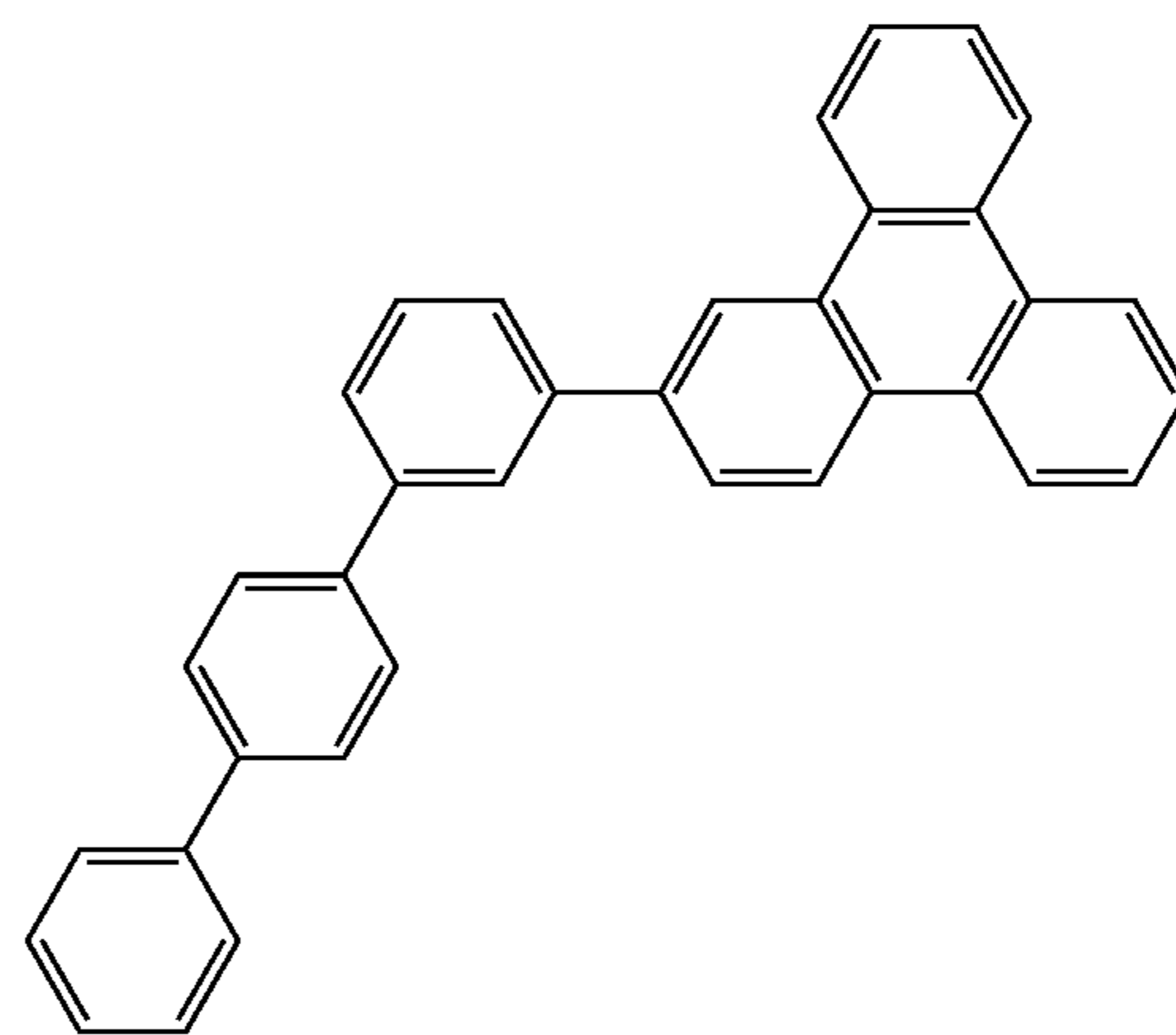
Compound 6
