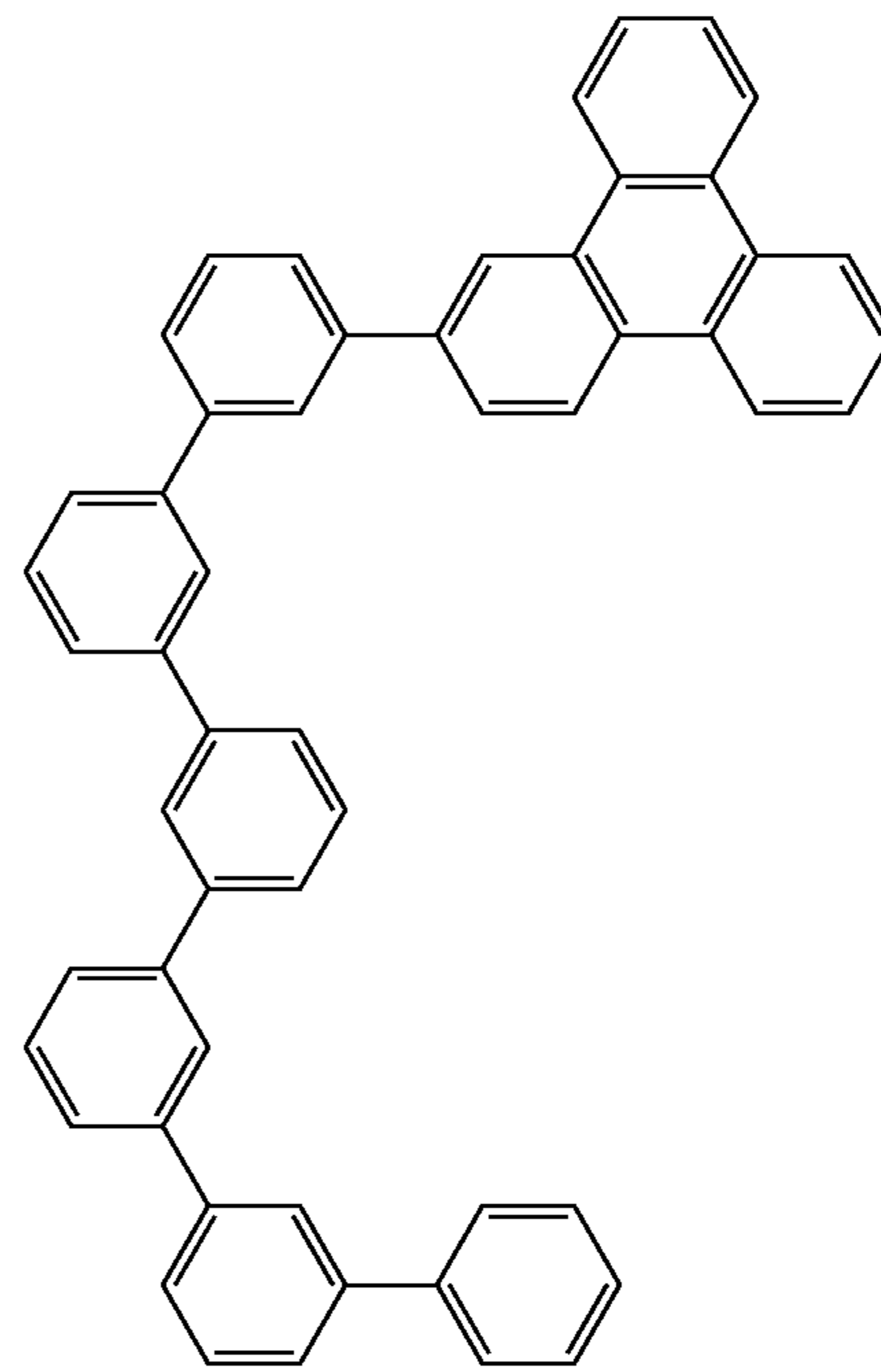
Compound 5
