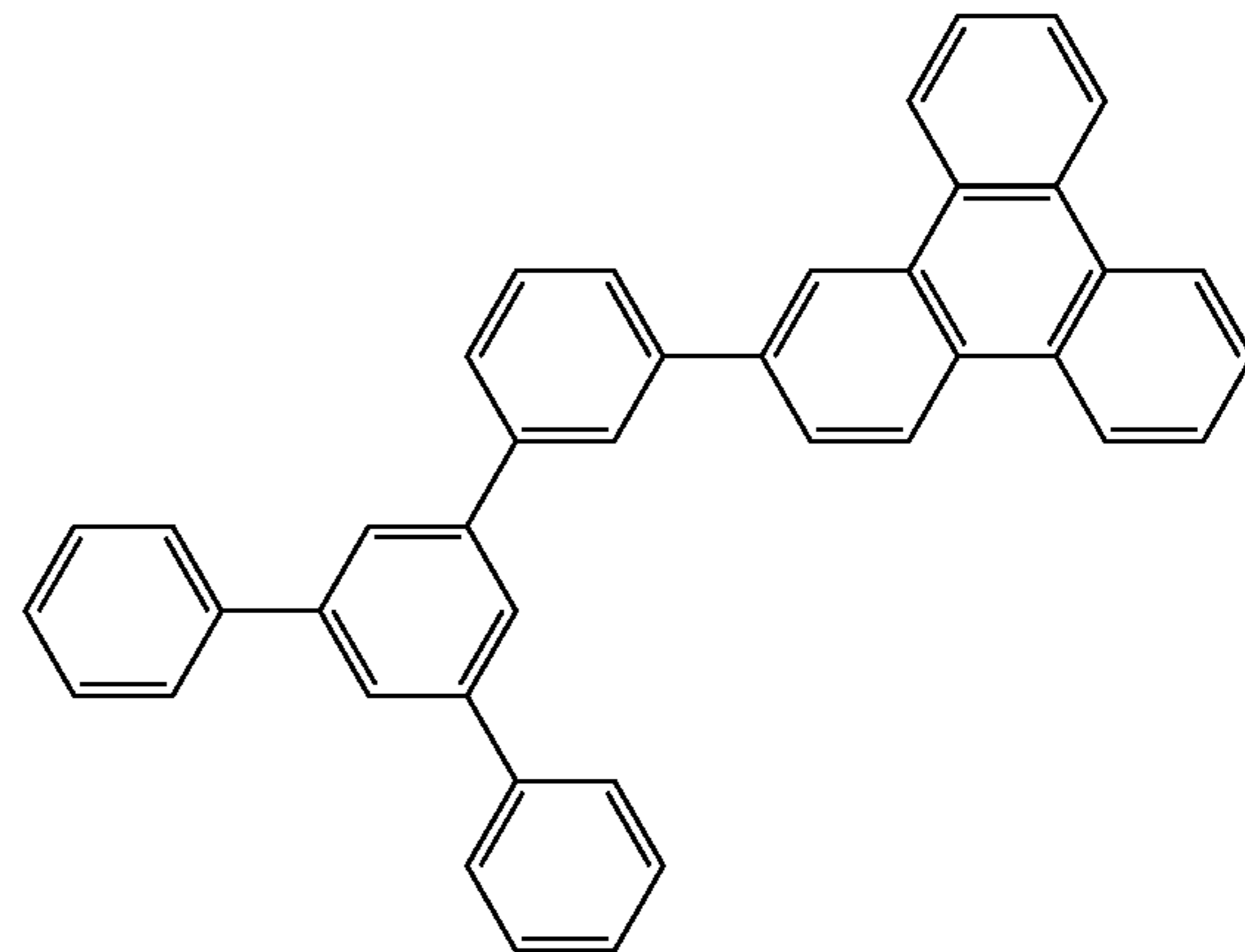
Compound 5
