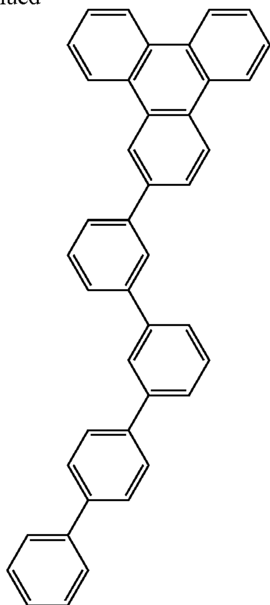
Compound 11
