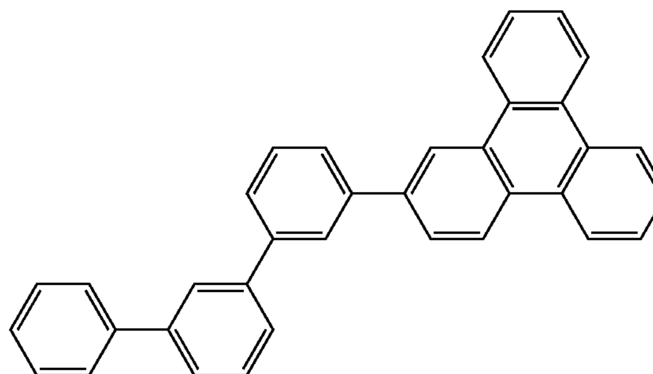
Compound 2
