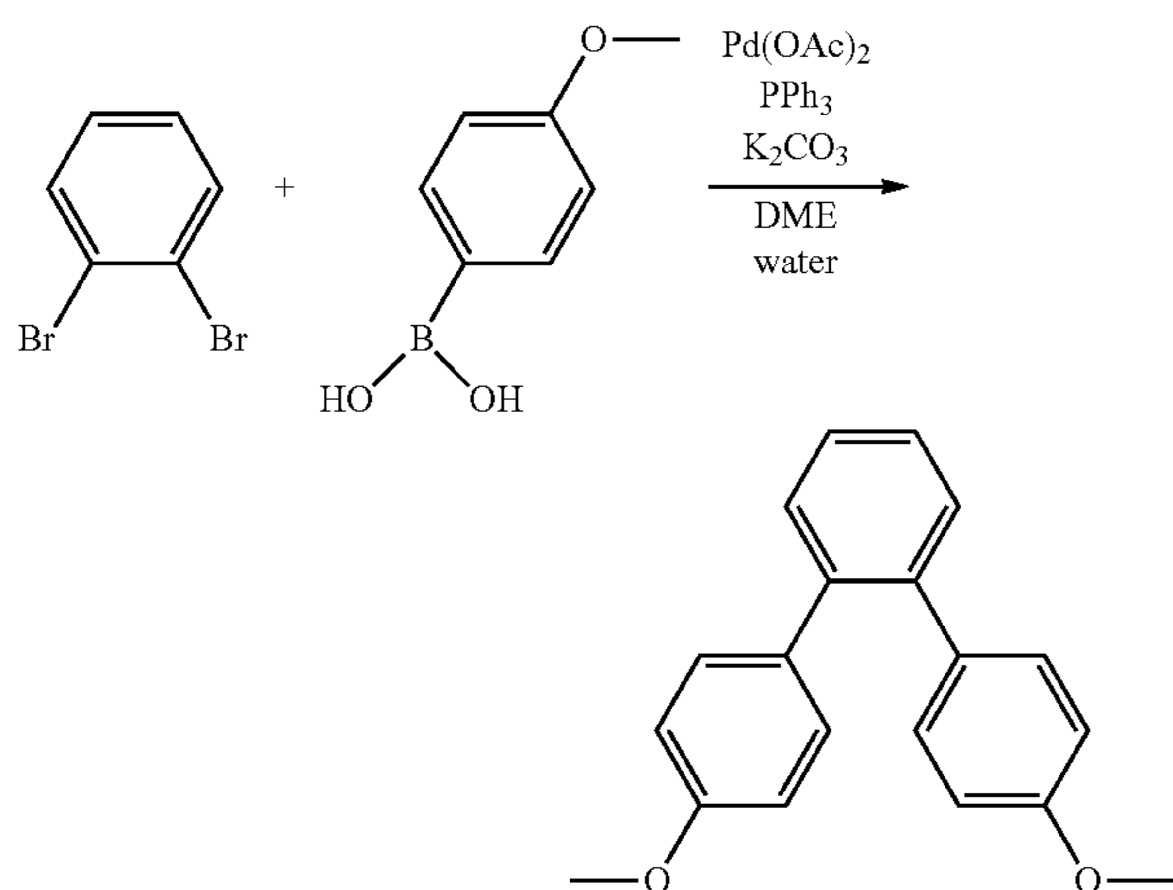
4,4'-Dimethoxy-o-terphenyl
