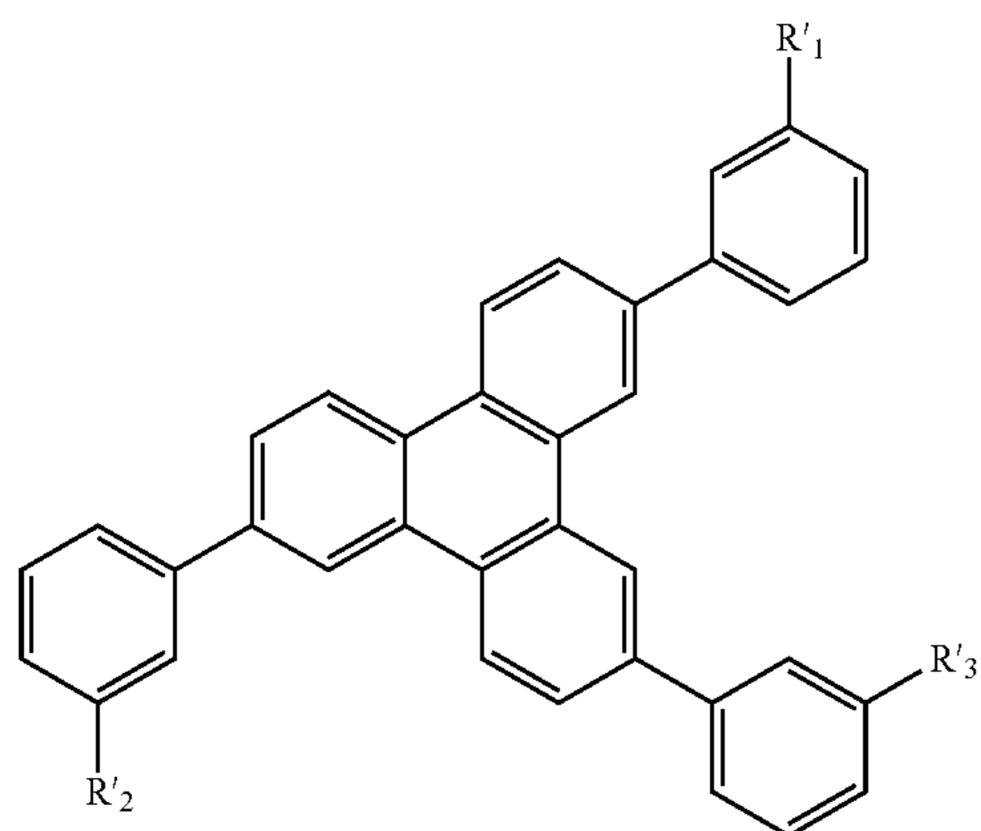
Substructure L
