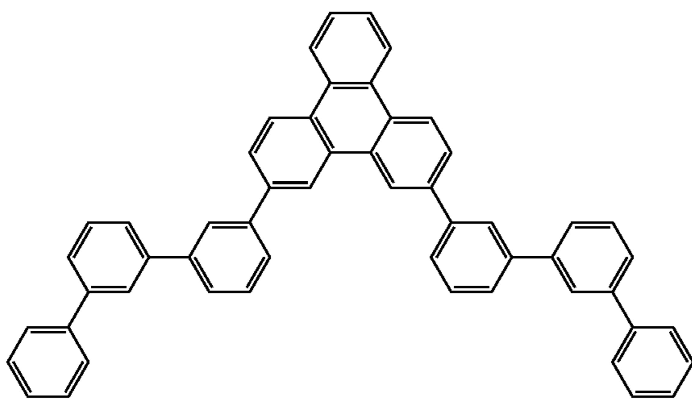
Compound 8
