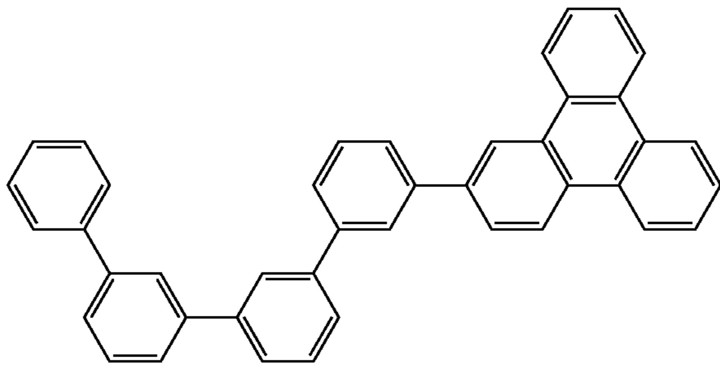
Compound 3
