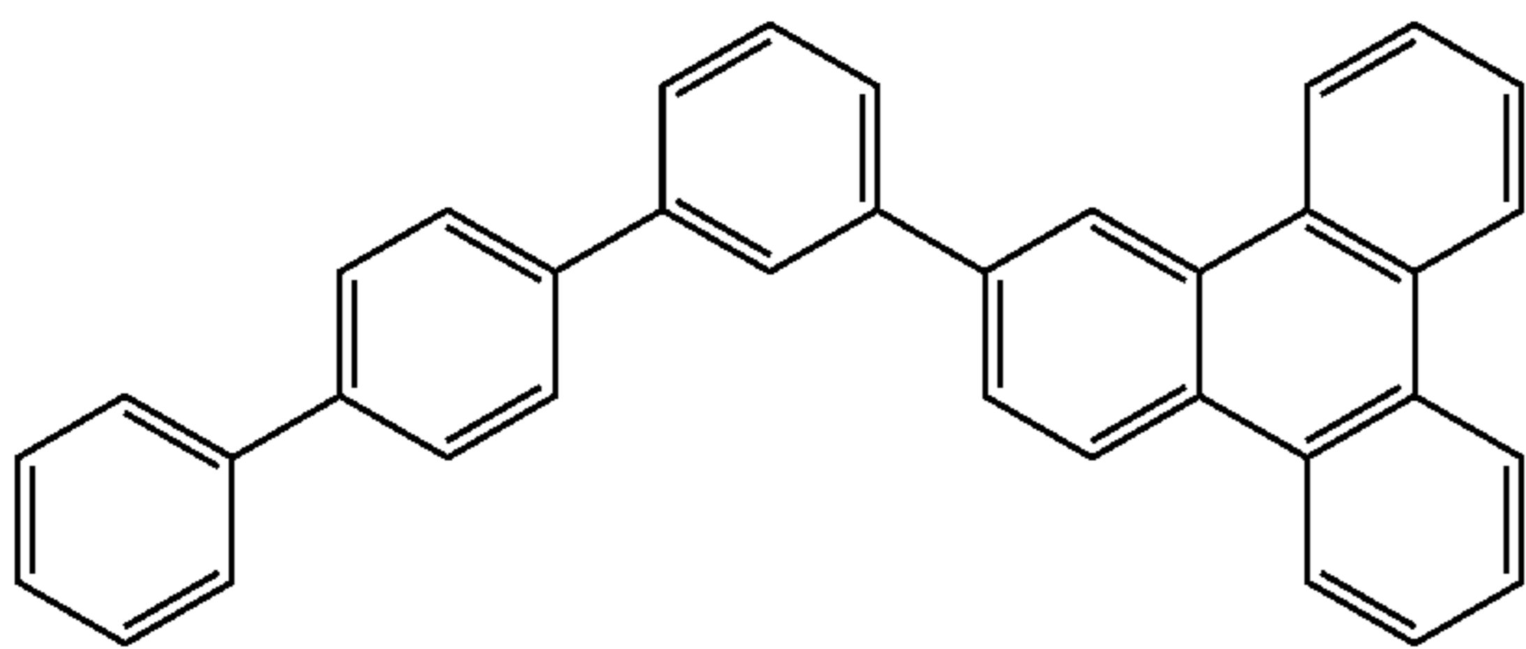
Compound 6
