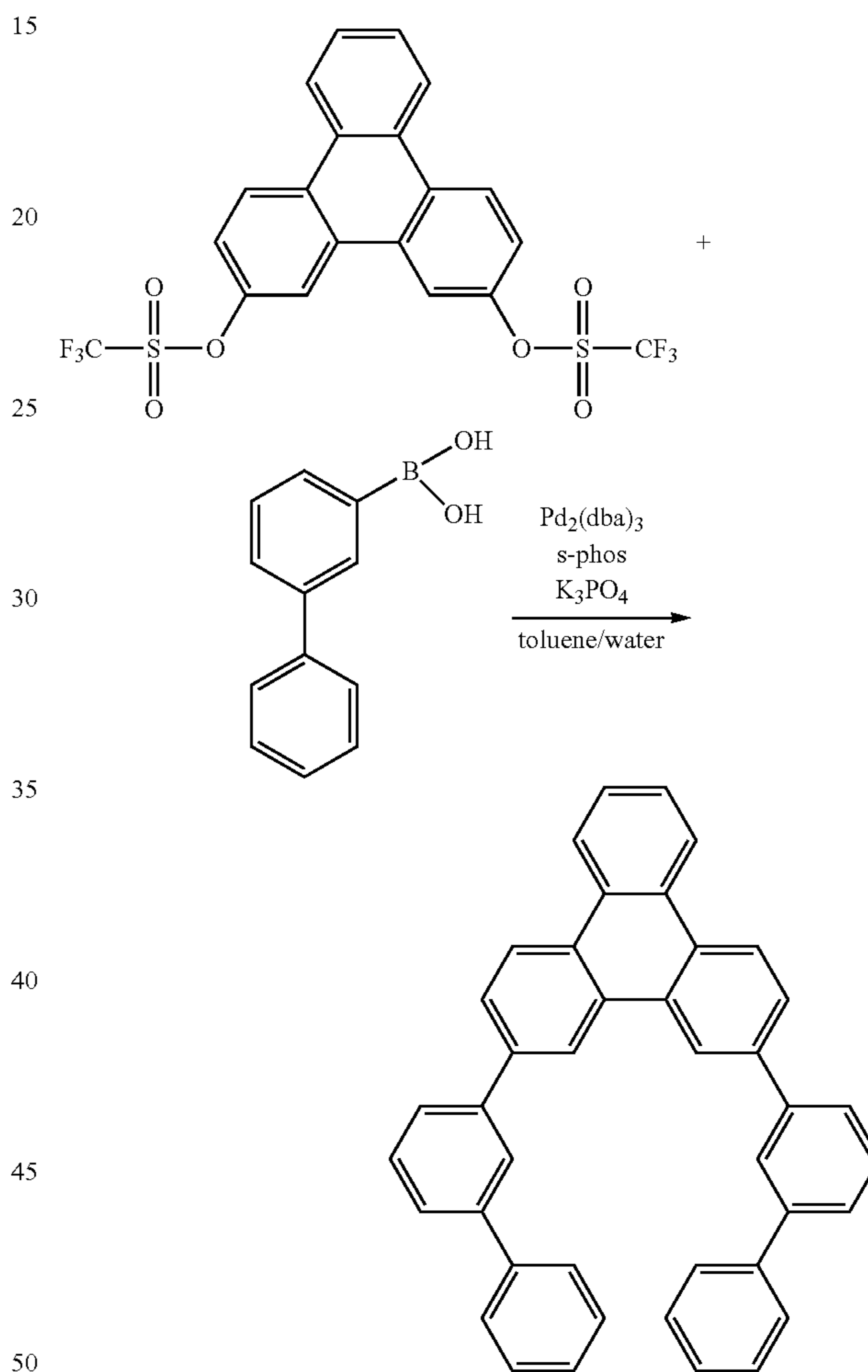
Compound 12
