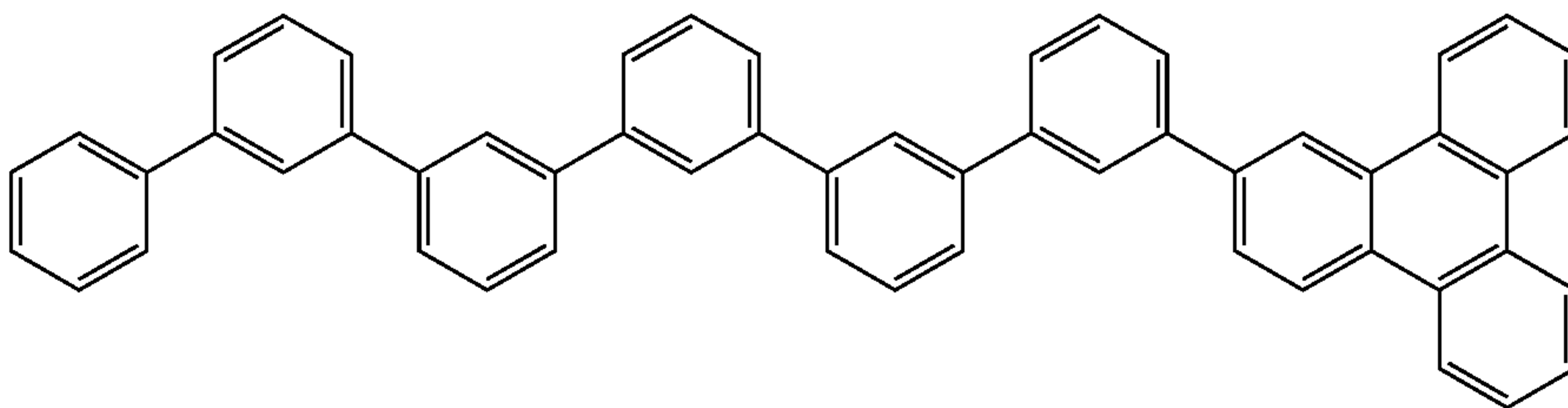
Compound 6
