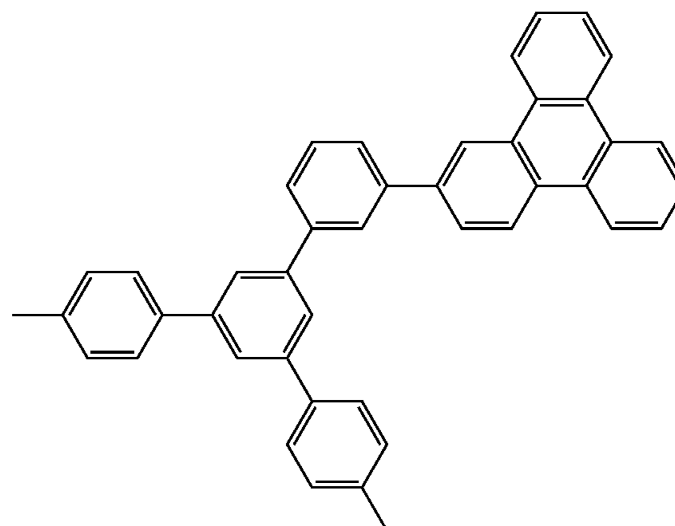
Compound 9
