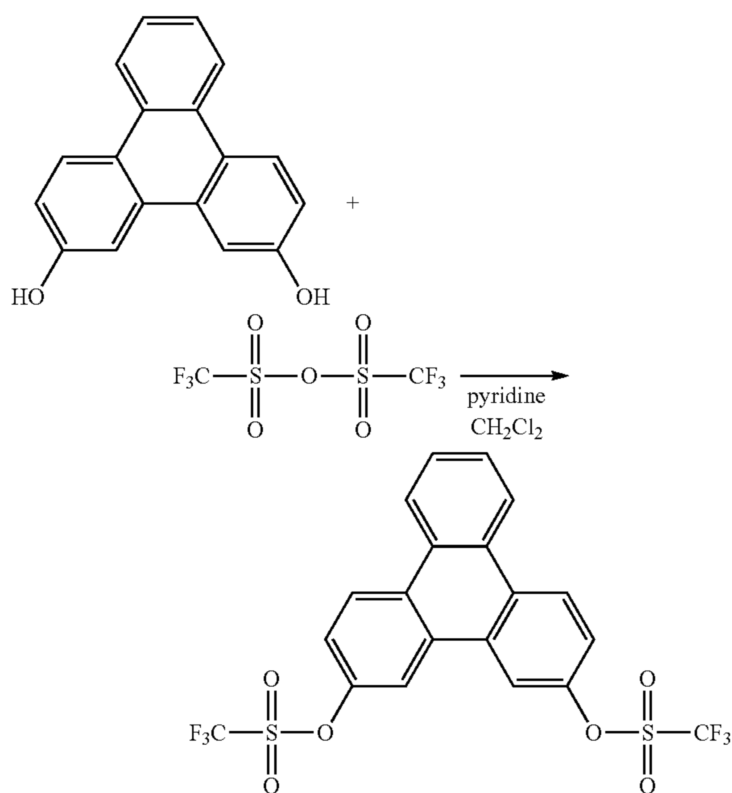
Triphenylene-2,11-dilyl bis(trifluoromethanesulfonate)
