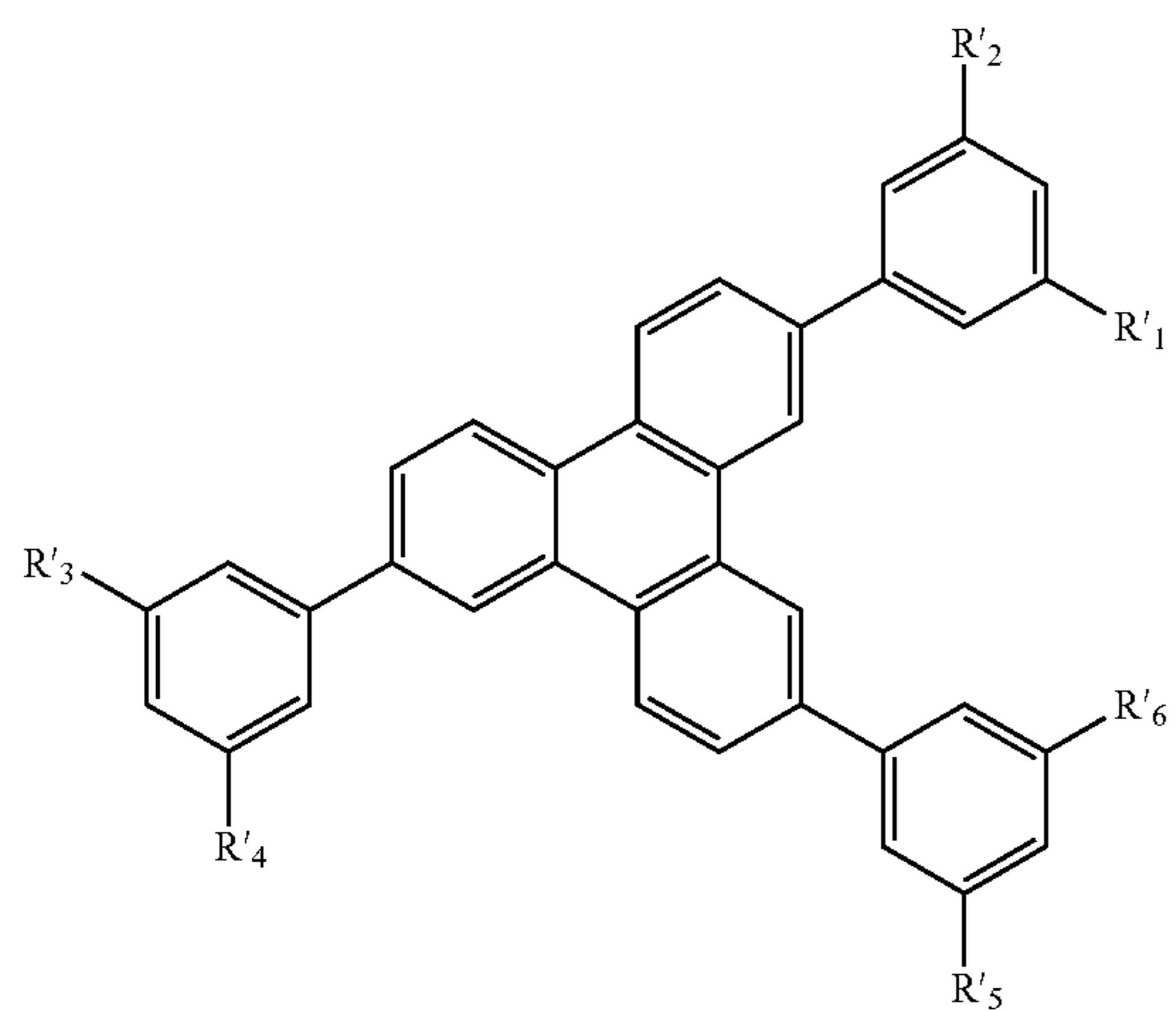
Substructure M
