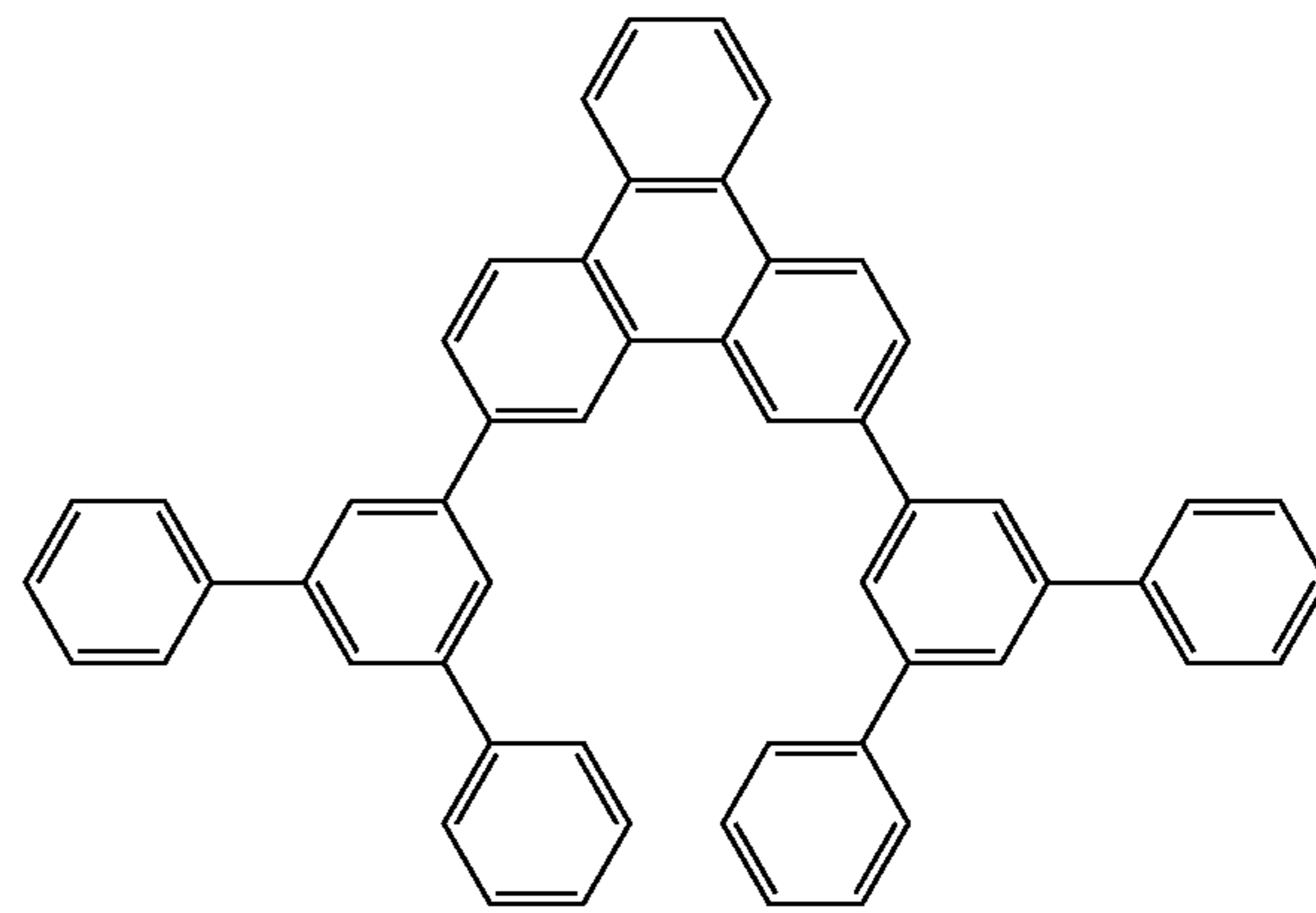
Compound 7
