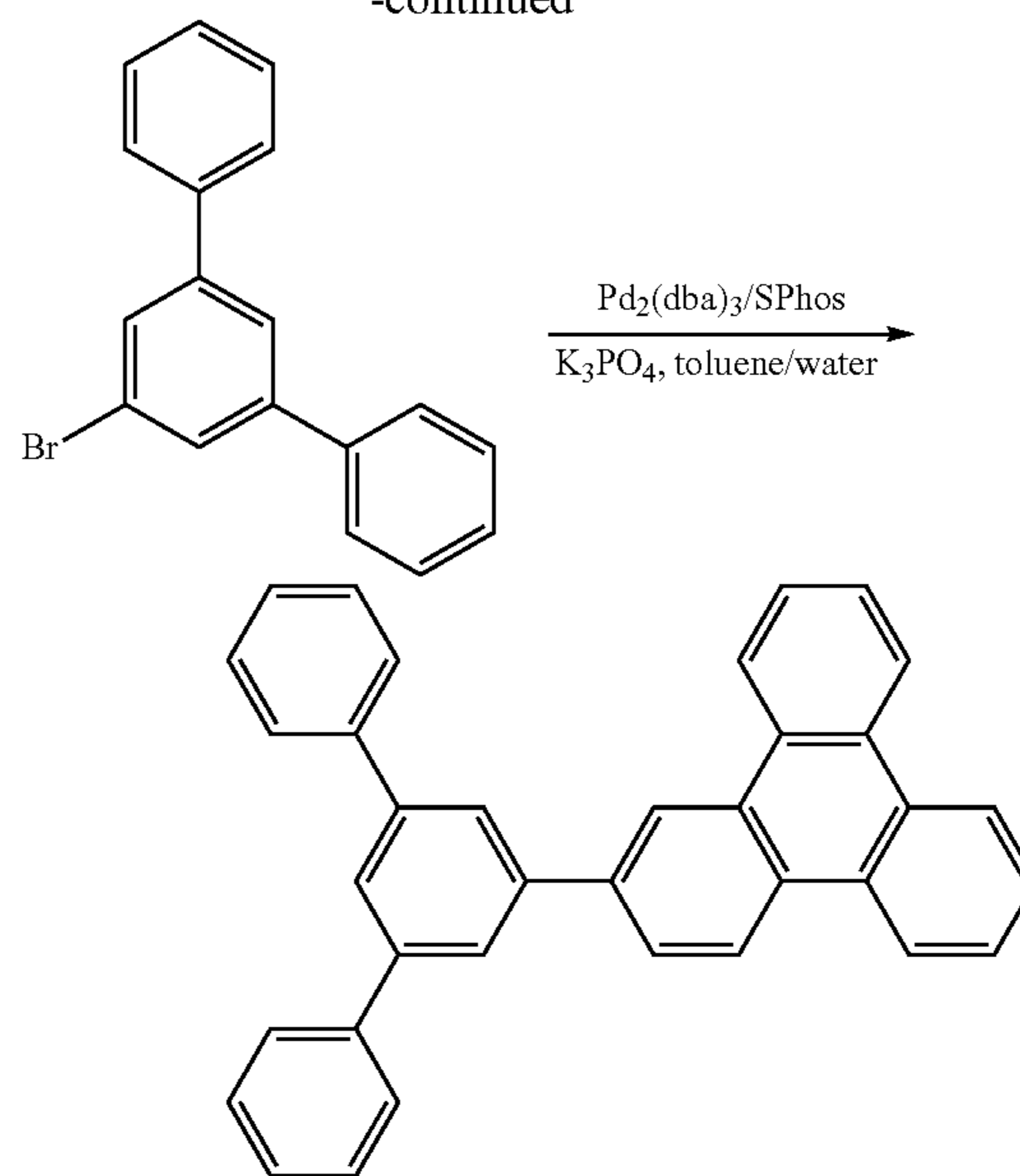
Compound 1
