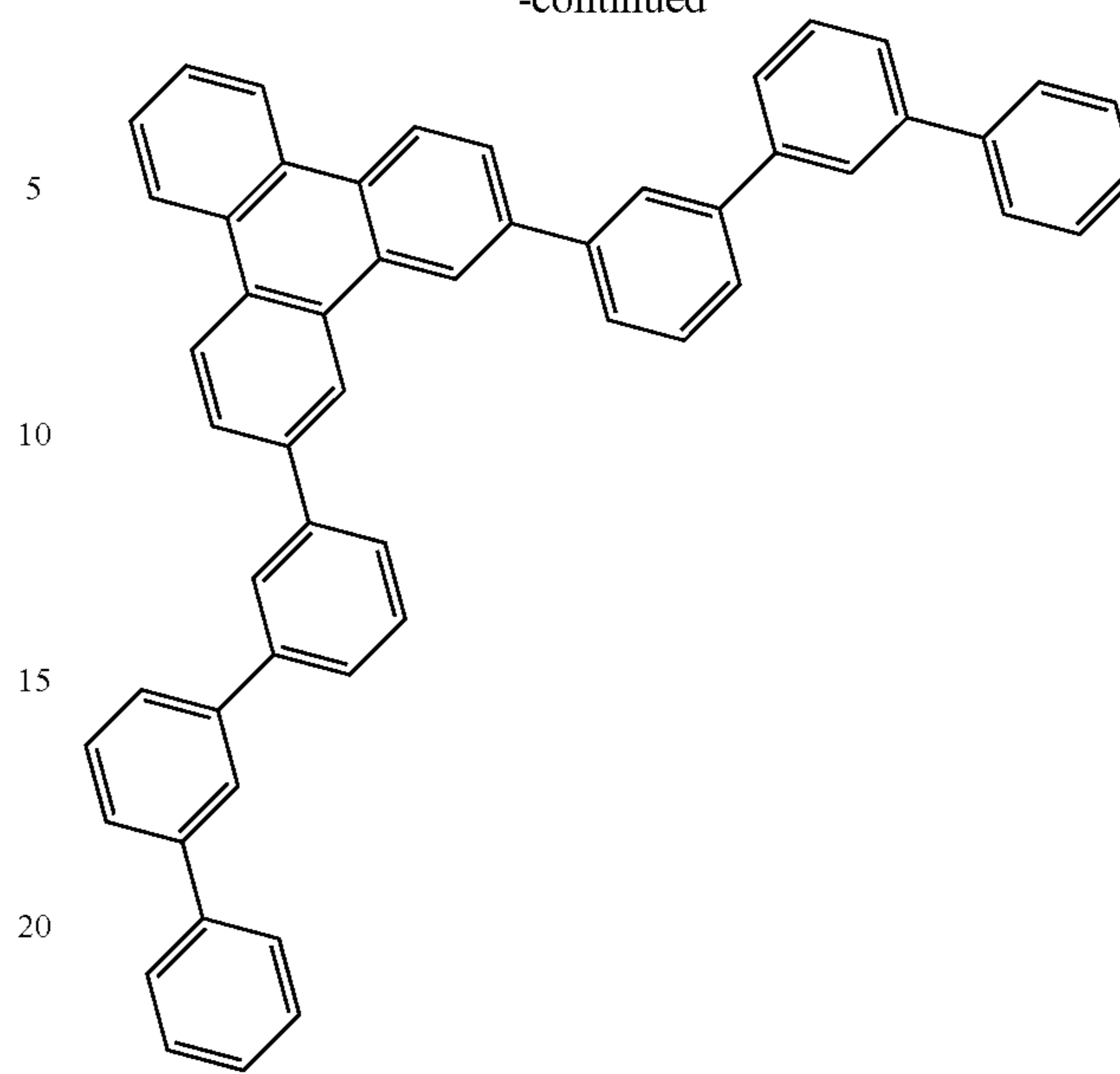
Compound 8
