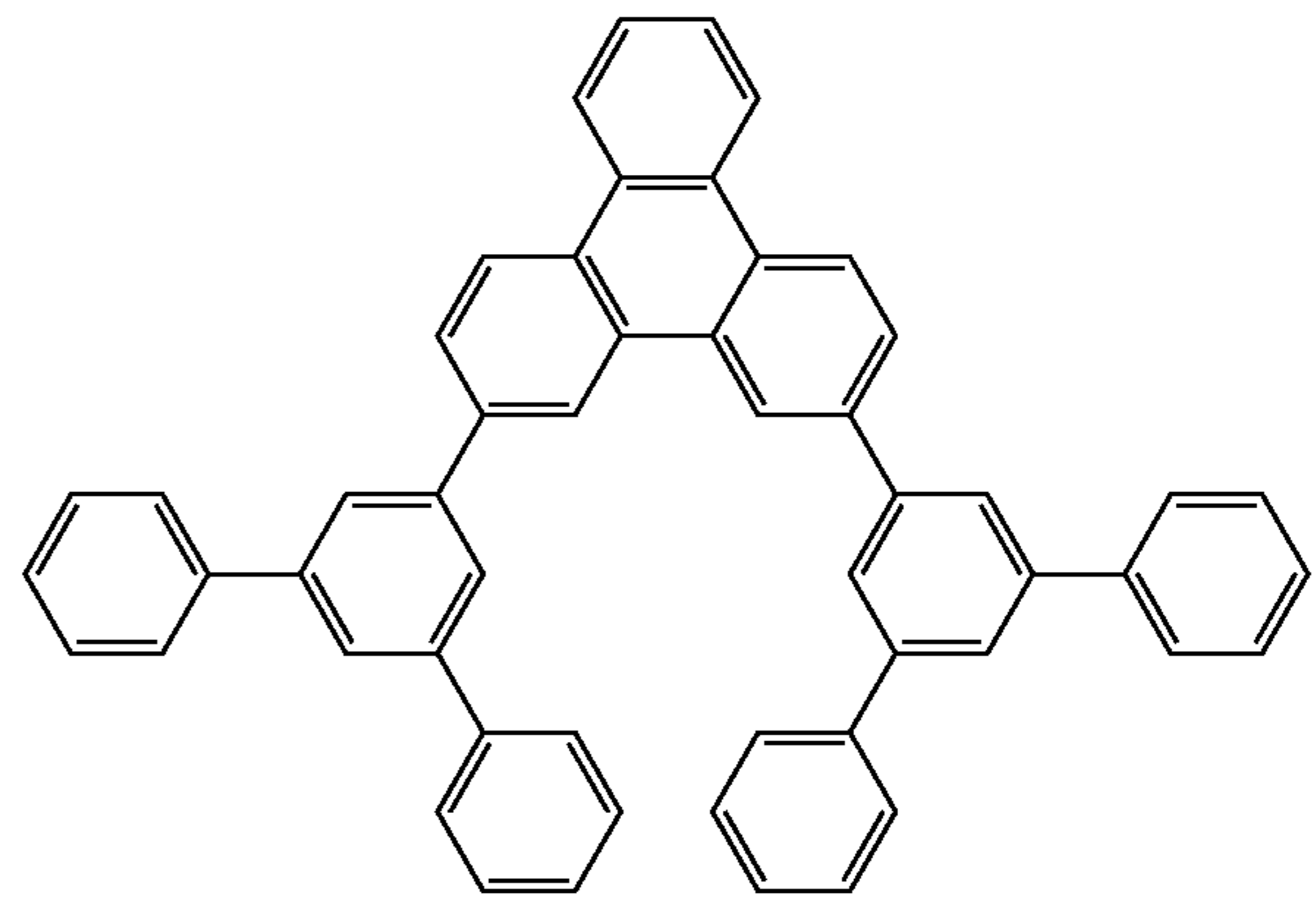
Compound 7
