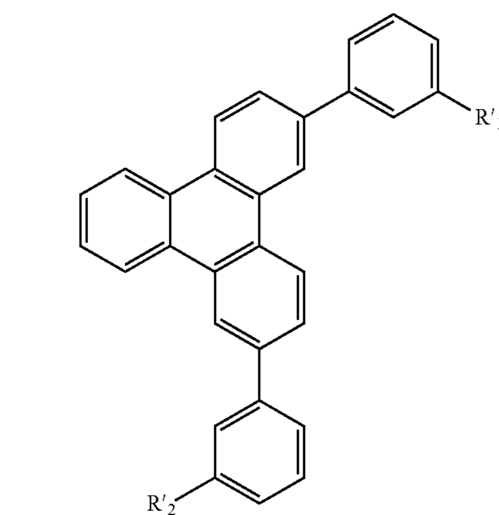
Substructure M
