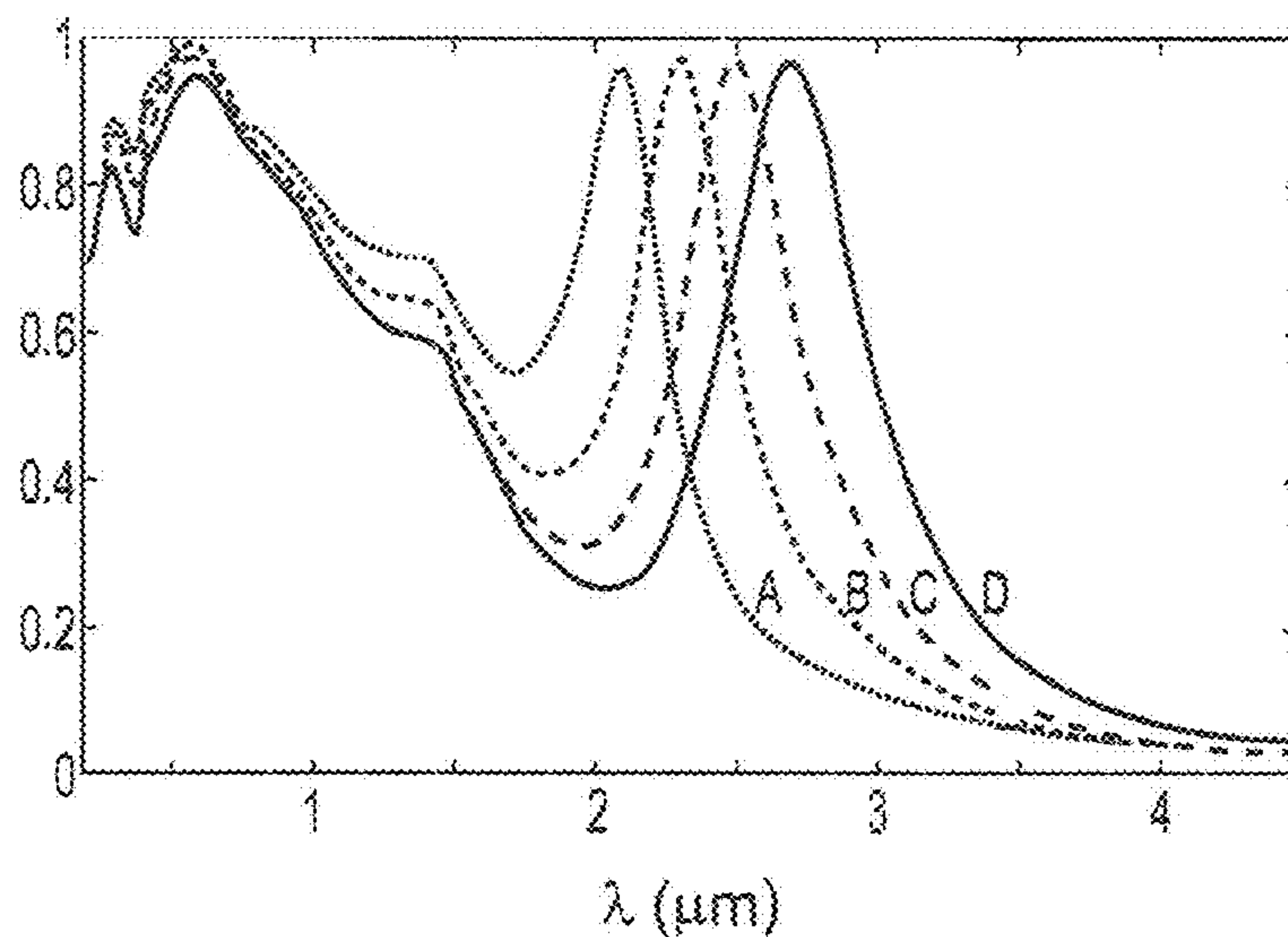
CALCULATED ABSORBANCE SPECTRA OF THE PREFERRED EMBODIMENT A OF FIGURE 9A, FOR SEVERAL SETS OF GEOMETRIC DIMENSIONS:
