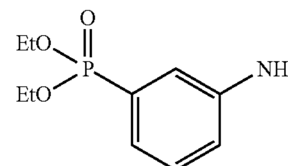
Diethyl 3-aminophenylphosphonate (13b)
