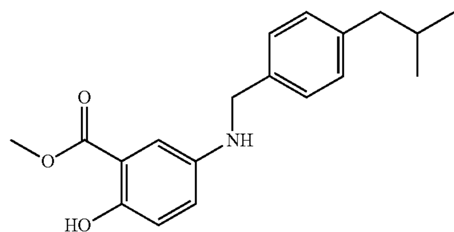
Methyl 2-hydroxy-5-(4-isobutylbenzylamino)benzoate (6g)
