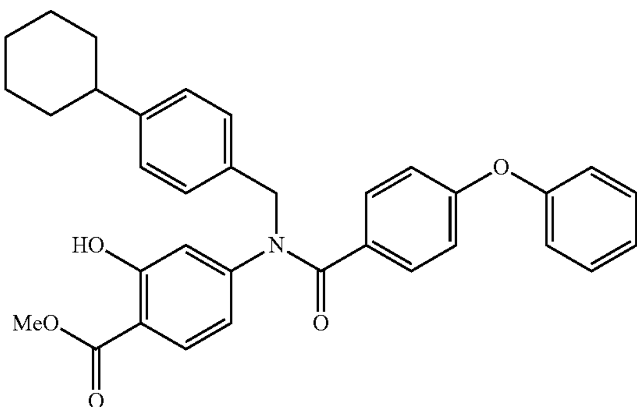
Methyl 4-(N-(4-cyclohexylbenzyl)-4-phenoxybenzamido)-2-hydroxybenzoate (32)
