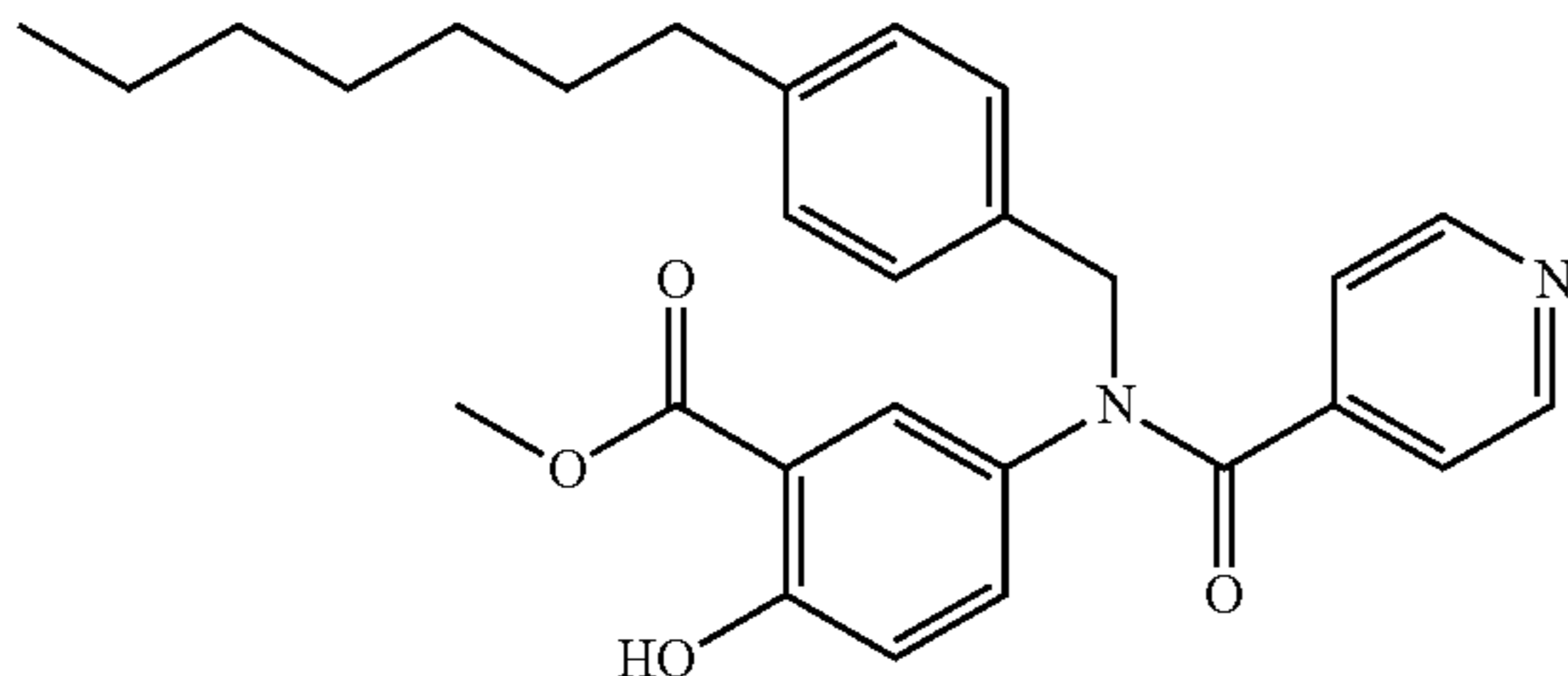
Methyl 5-(N-(4-heptylbenzyl)isonicotinamido)-2-hydroxybenzoate (19j)
