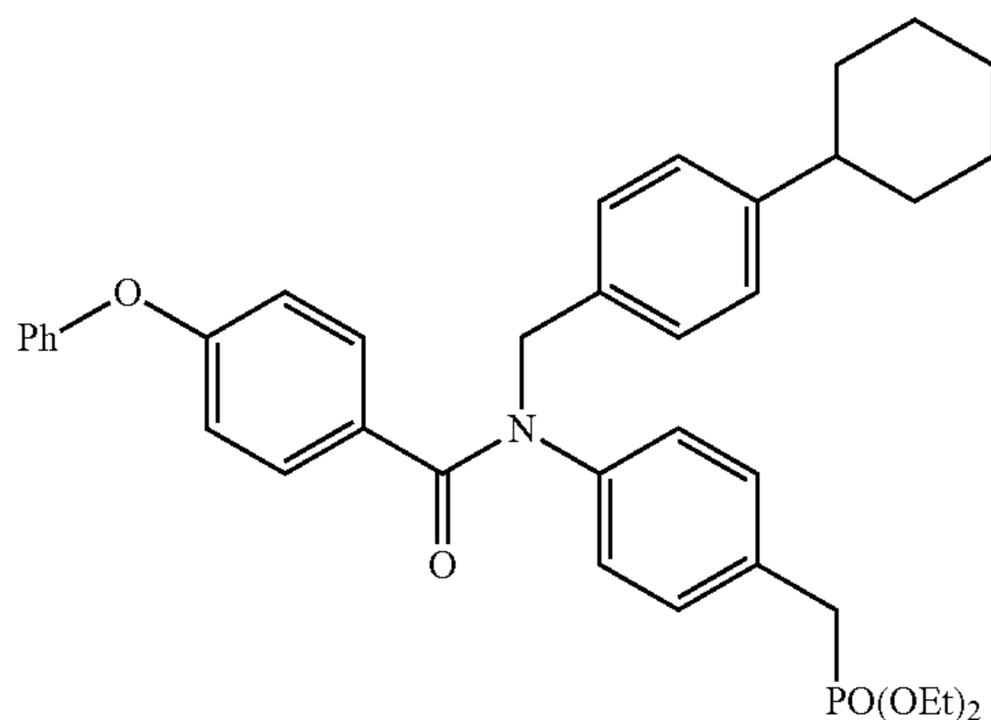
Diethyl 4-(N-(4-cyclohexylbenzyl)-4-phenoxybenzamido)benzylphosphonate (16d)
