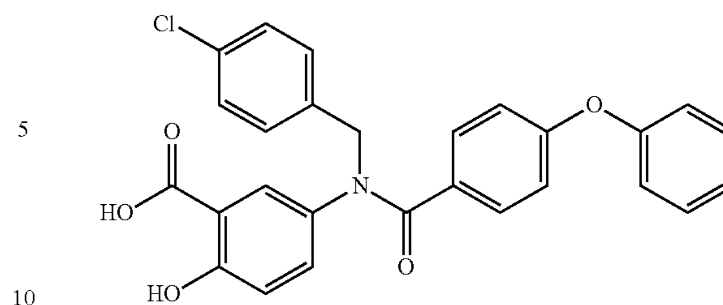
5-(N-(4-Chlorobenzyl)-4-phenoxybenzamido)-2-hydroxybenzoic acid (20d)
