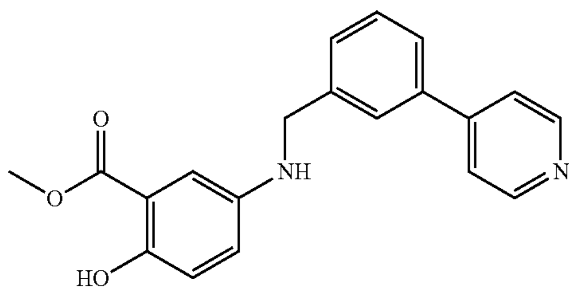
Methyl 2-hydroxy-5-(3-(pyridin-4-yl)benzylamino) benzoate (6f)
