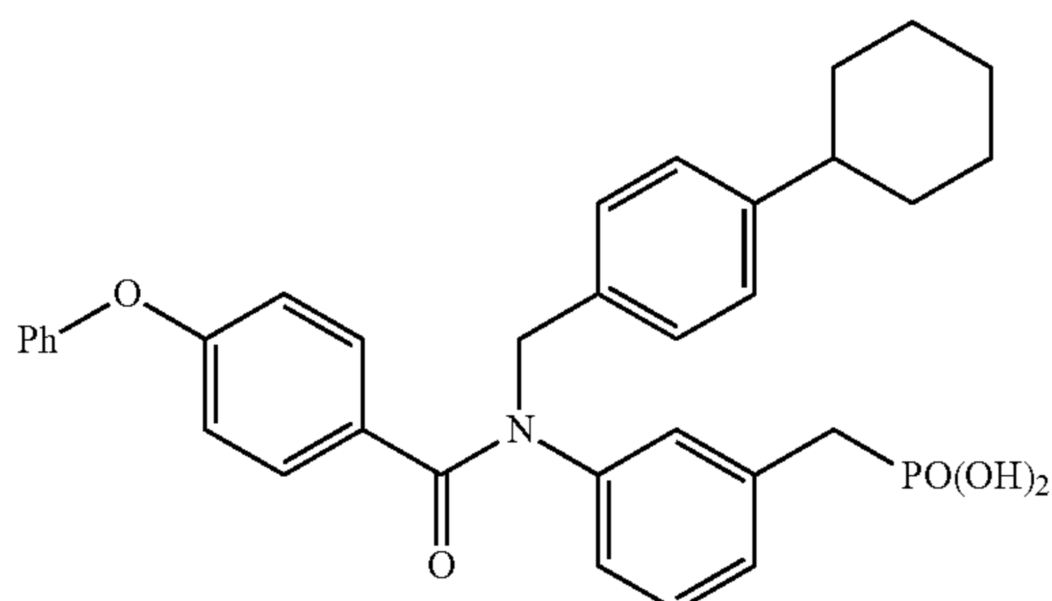
3-(N-(4-Cyclohexylbenzyl)-4-phenoxybenzamido)benzylphosphonic acid (17d)
