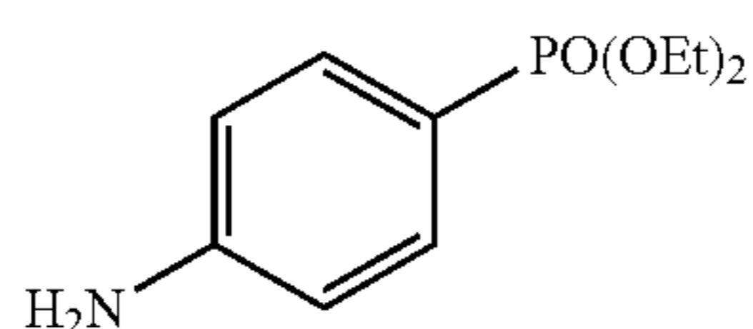
Diethyl 4-aminophenylphosphonate (13a)
