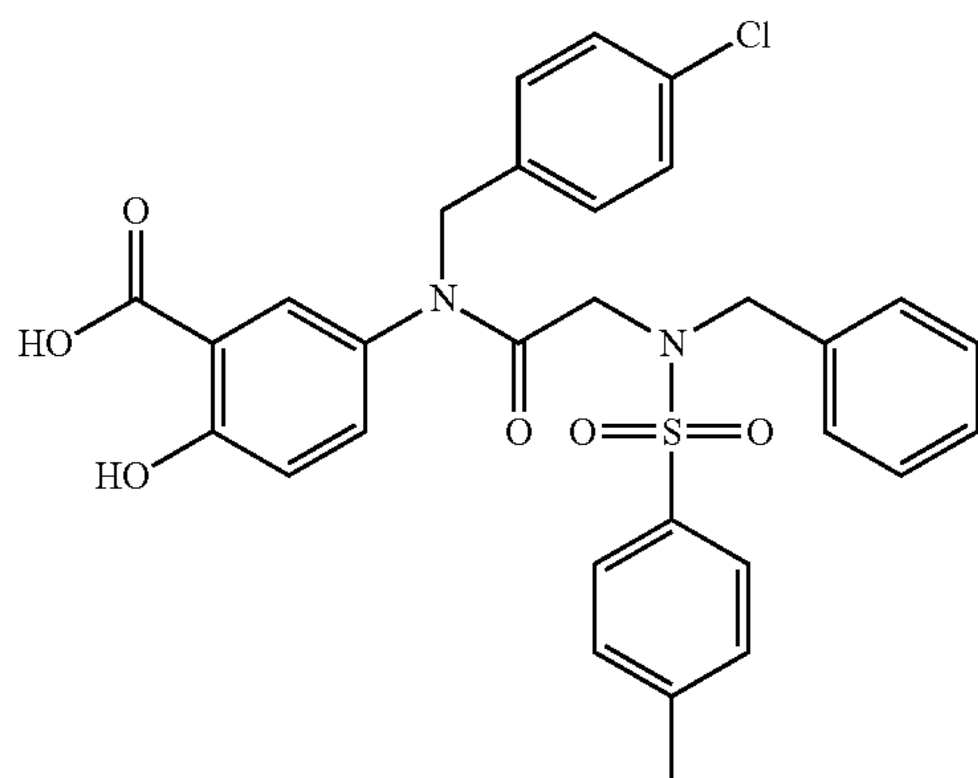
5-(2-(N-Benzyl-4-methylphenylsulfonamido)-N-(4-chlorobenzyl)acetamido)-2-hydroxybenzoic acid (9c)
