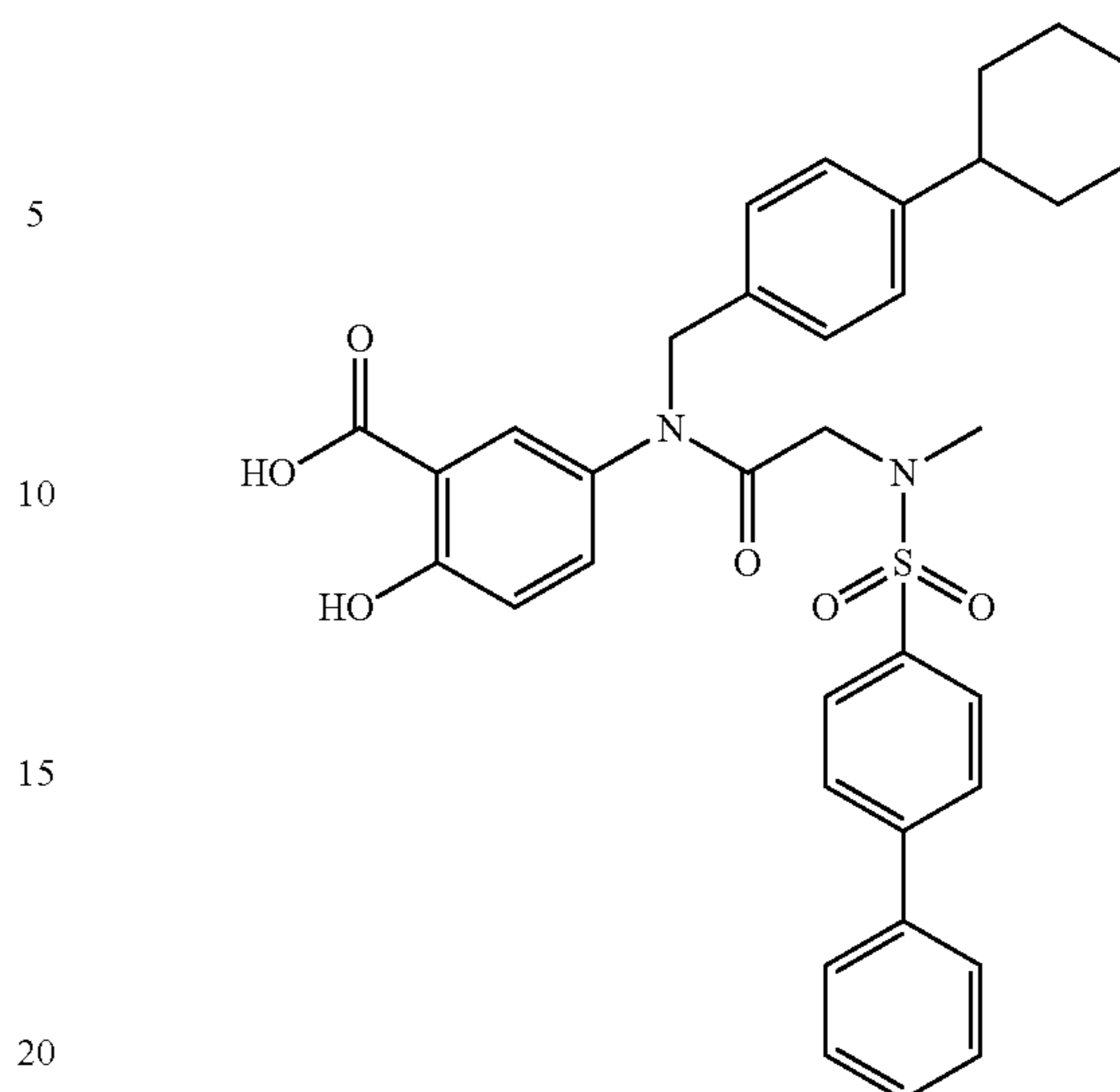
5-(N-(4-Cyclohexylbenzyl)-2-(N-methylbiphenyl-4-ylsulfonamido)acetamido)-2-hydroxybenzoic acid (9n)
