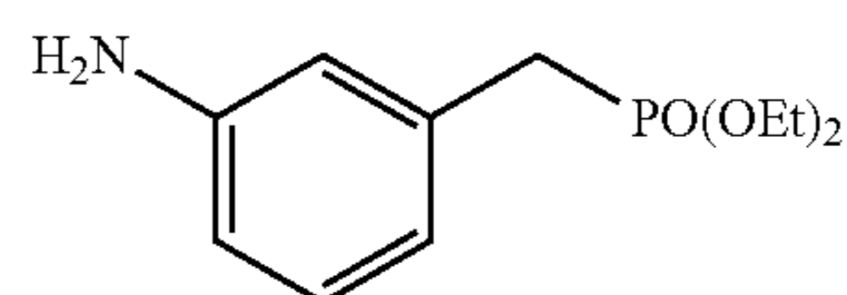
Diethyl 3-aminobenzylphosphonate (13d)
