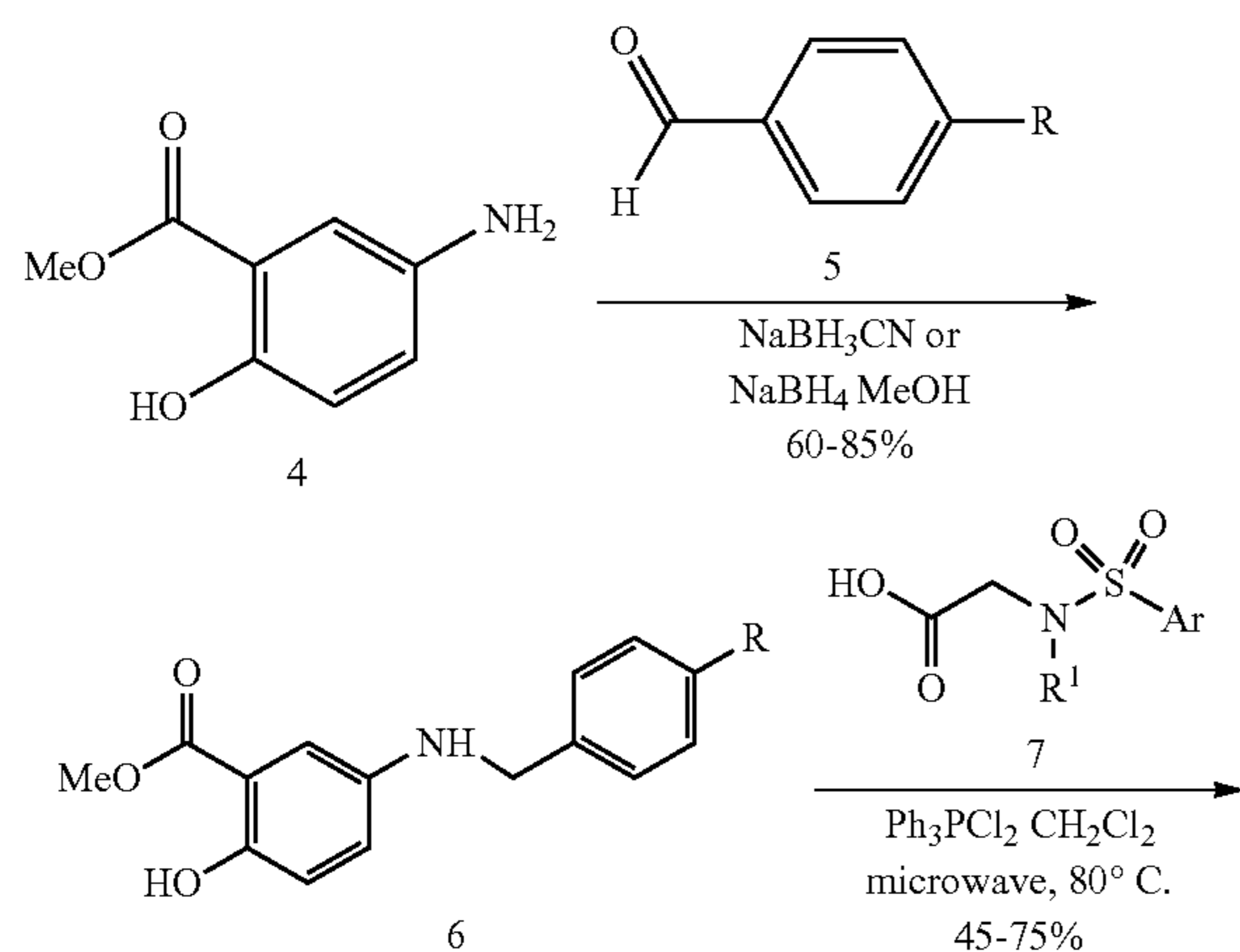
Scheme 1. Synthetic route to library 9
