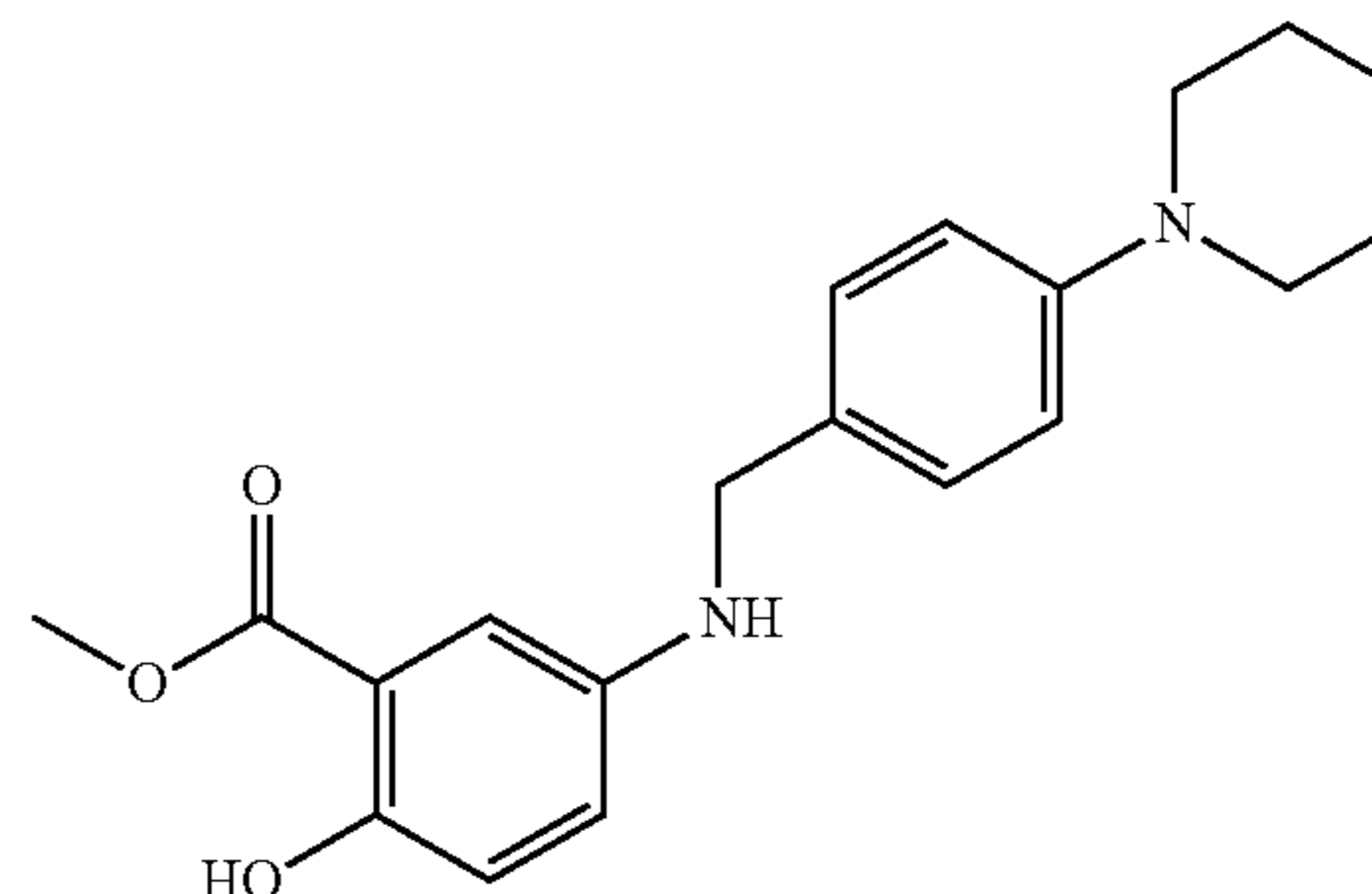
Methyl 2-hydroxy-5-(4-(piperidin-1-yl)benzyl- amino)benzoate (6h)
