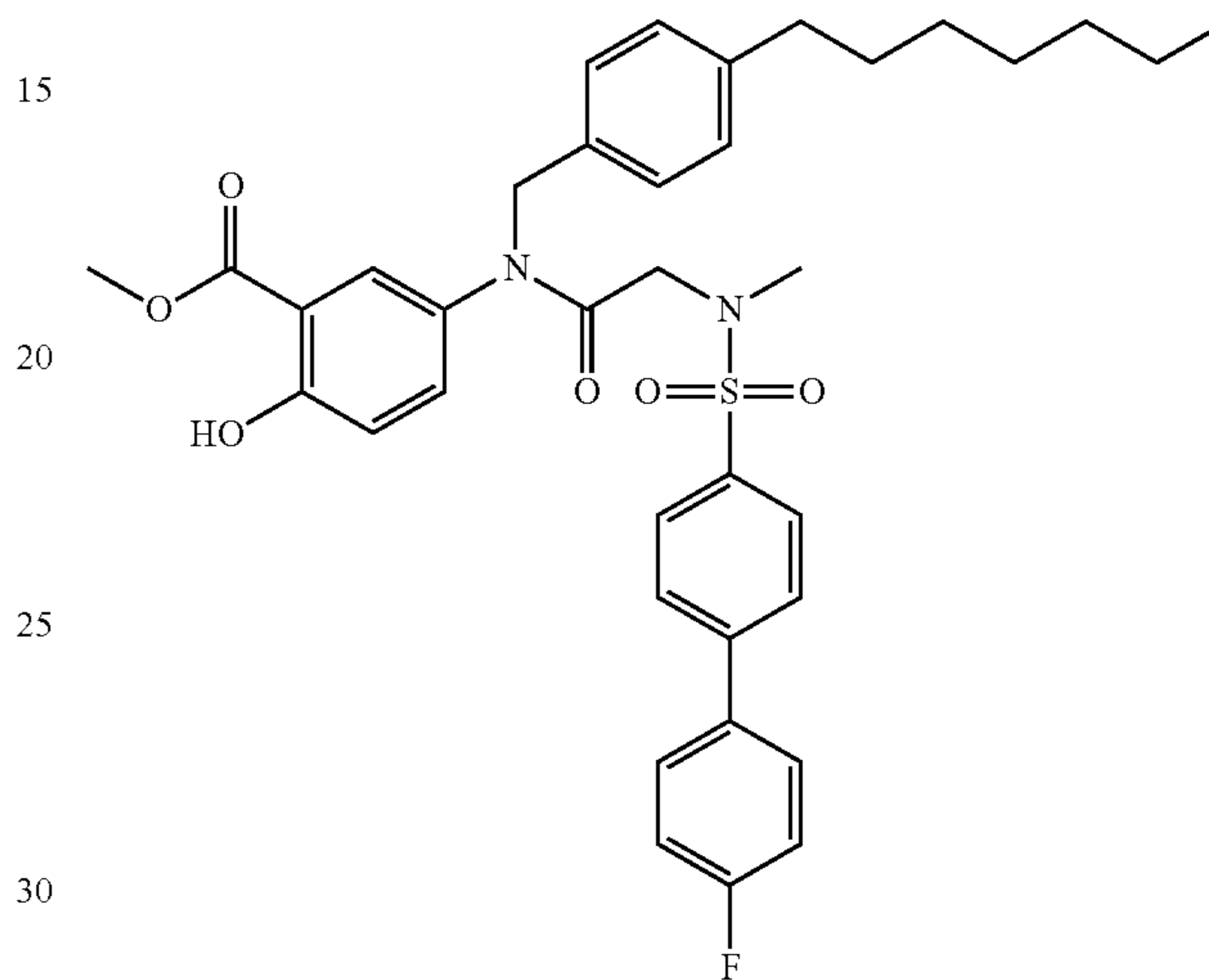
Methyl 5-(2-(4'-fluoro-N-methylbiphenyl-4-yl)sulfonamido)-N-(4-heptylbenzyl)acetamido)-2-hydroxybenzoate (8s)
