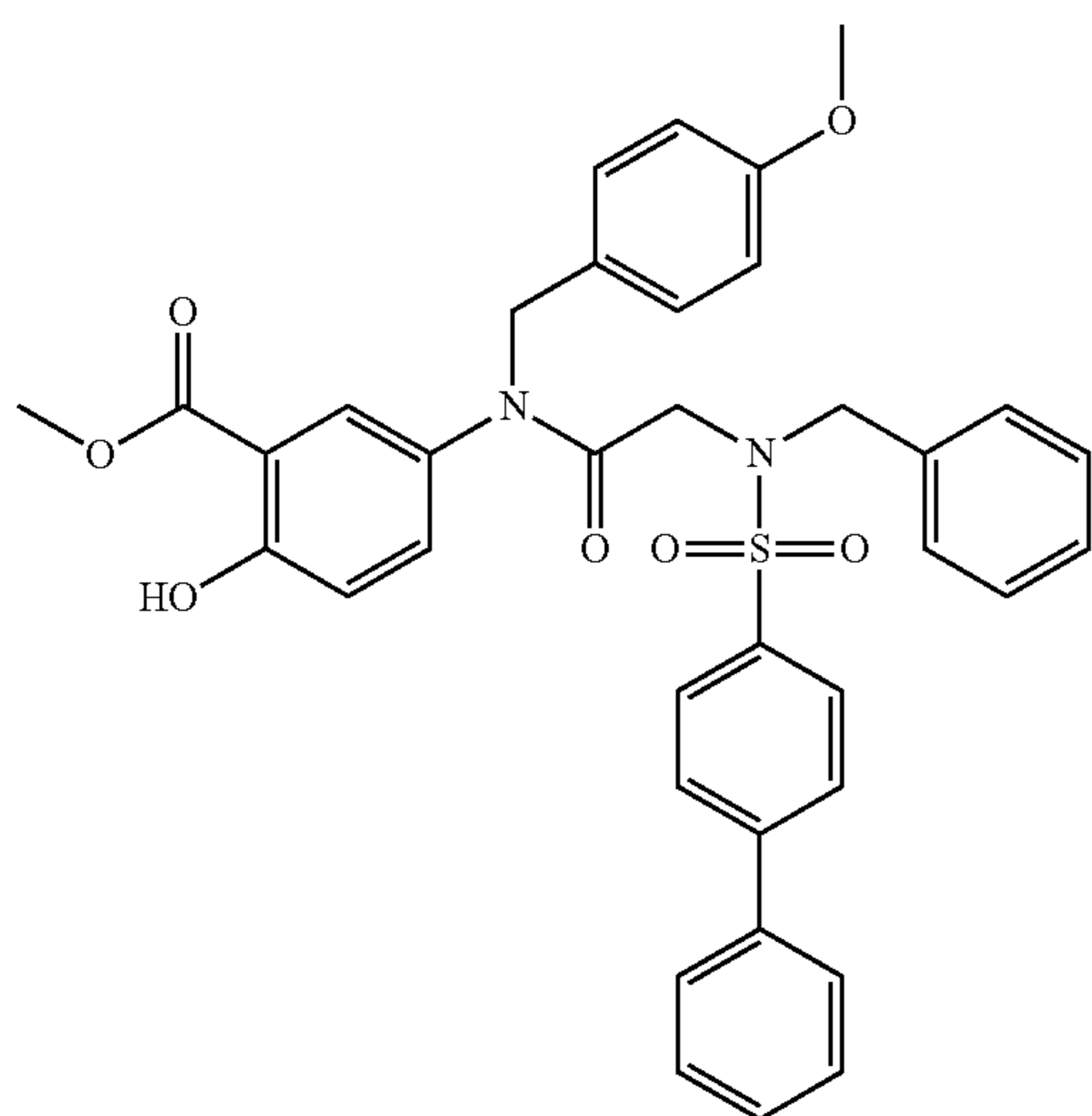
Methyl 5-(2-(N-benzylbiphenyl-4-ylsulfonamido)-N-(4-methoxybenzyl)acetamido)-2-hydroxybenzoate (8f)
