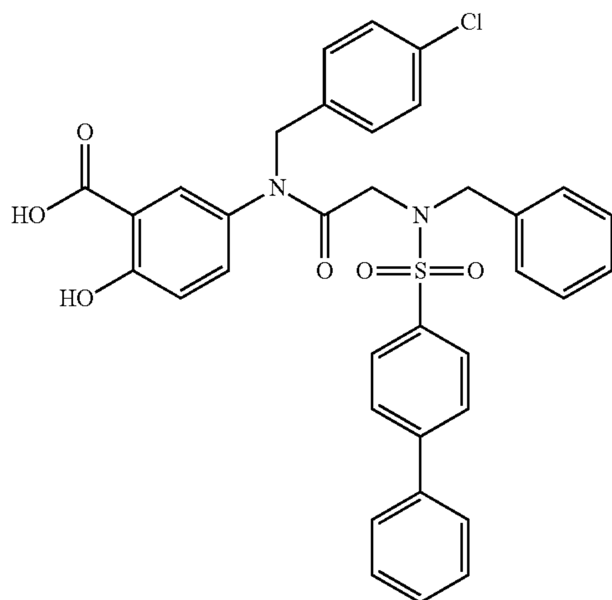
5-(2-(N-Benzylbiphenyl-4-ylsulfonamido)-N-(4-chlorobenzyl)acetamido)-2-hydroxybenzoic acid (9d)
