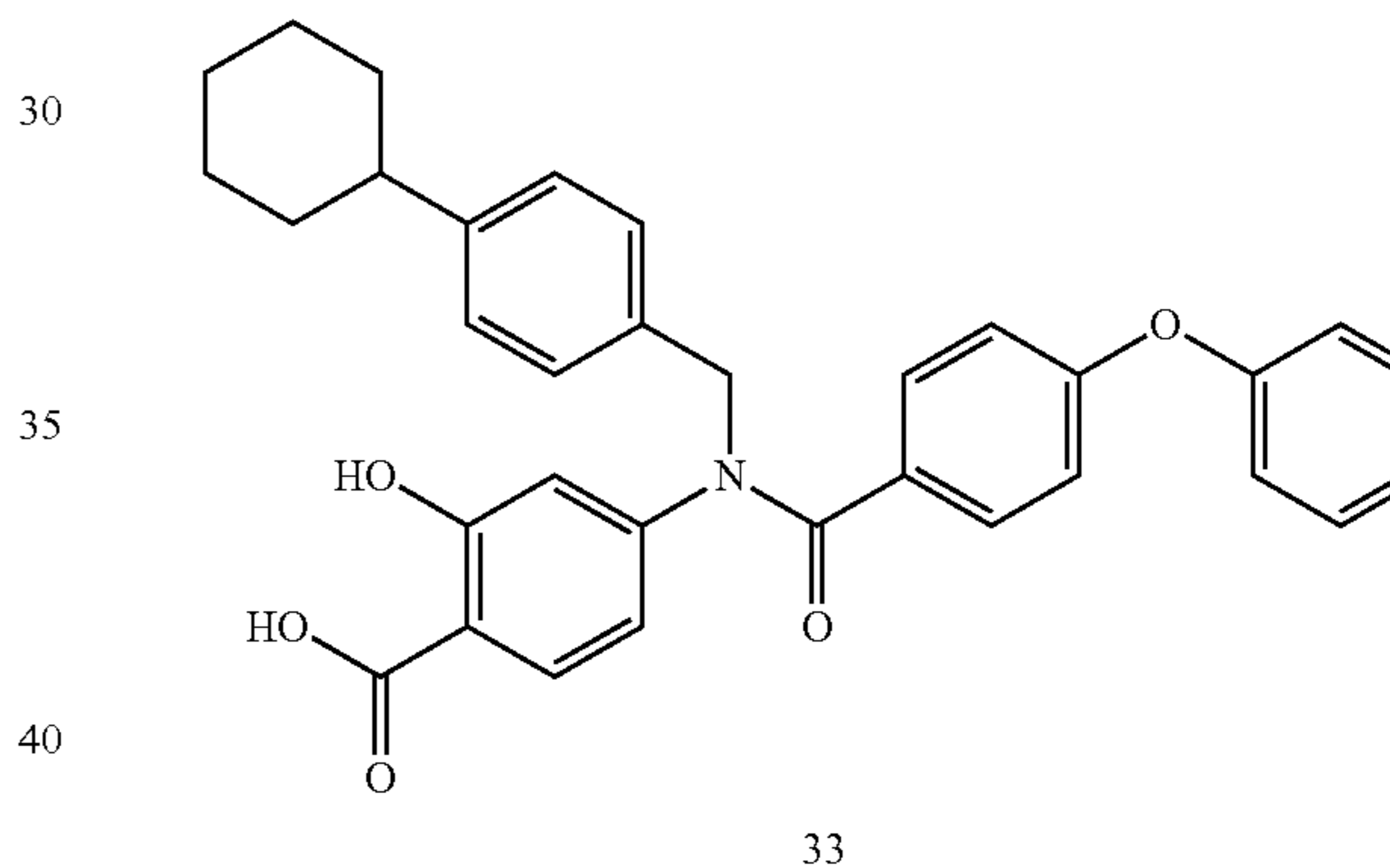
Synthesis of Carboxylic Acid 33
