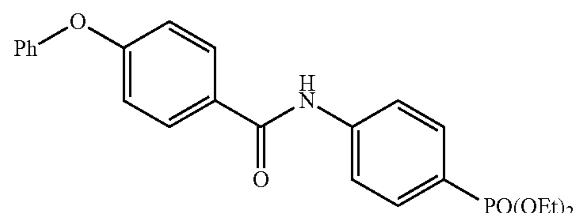
Diethyl 4-(4-phenoxybenzamido)phenylphosphonate (18a)
