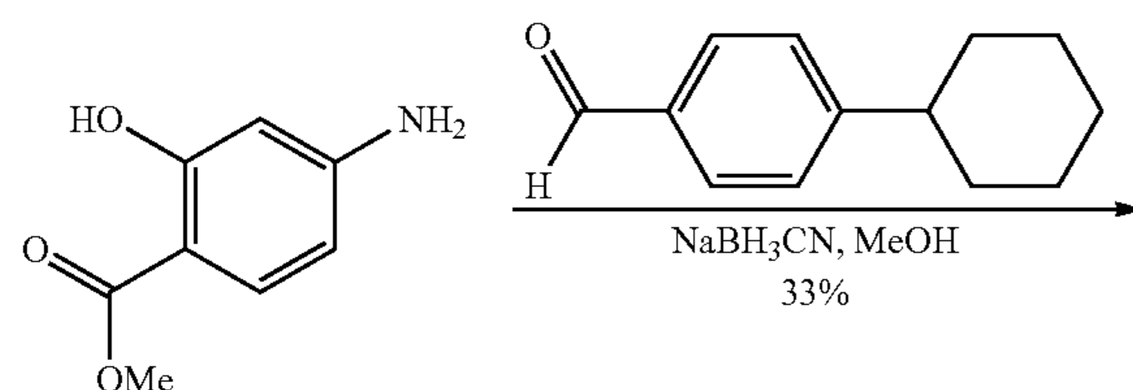
Scheme 5. Synthesis of the benzamide 33 derived from methyl 4-amino-2-hydroxybenzoate.
