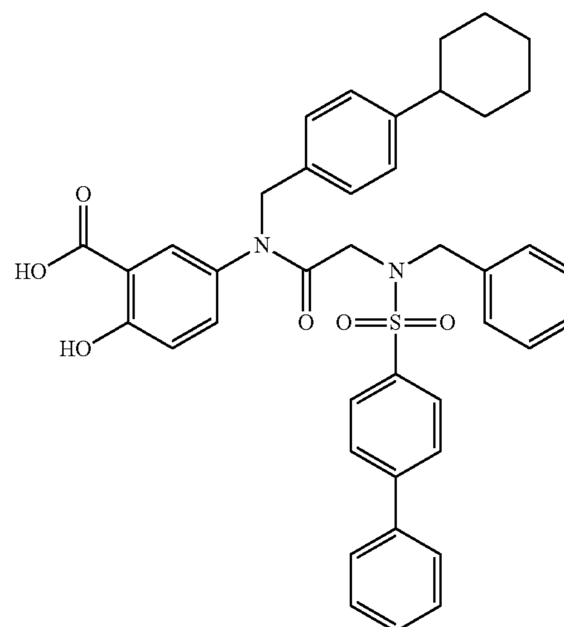
5-(2-(N-Benzylbiphenyl-4-ylsulfonamido)-N-(4-cyclohexylbenzyl)acetamido)-2-hydroxybenzoic acid (9g)
