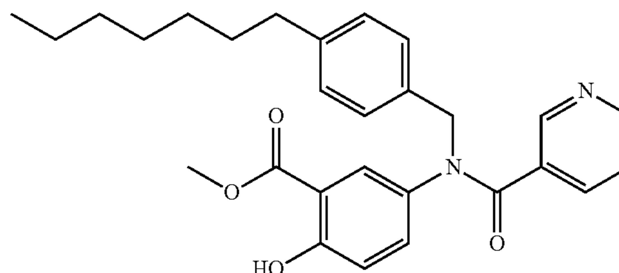
Methyl 5-(N-(4-heptylbenzyl)nicotinamido)-2-hydroxybenzoate (19l)
