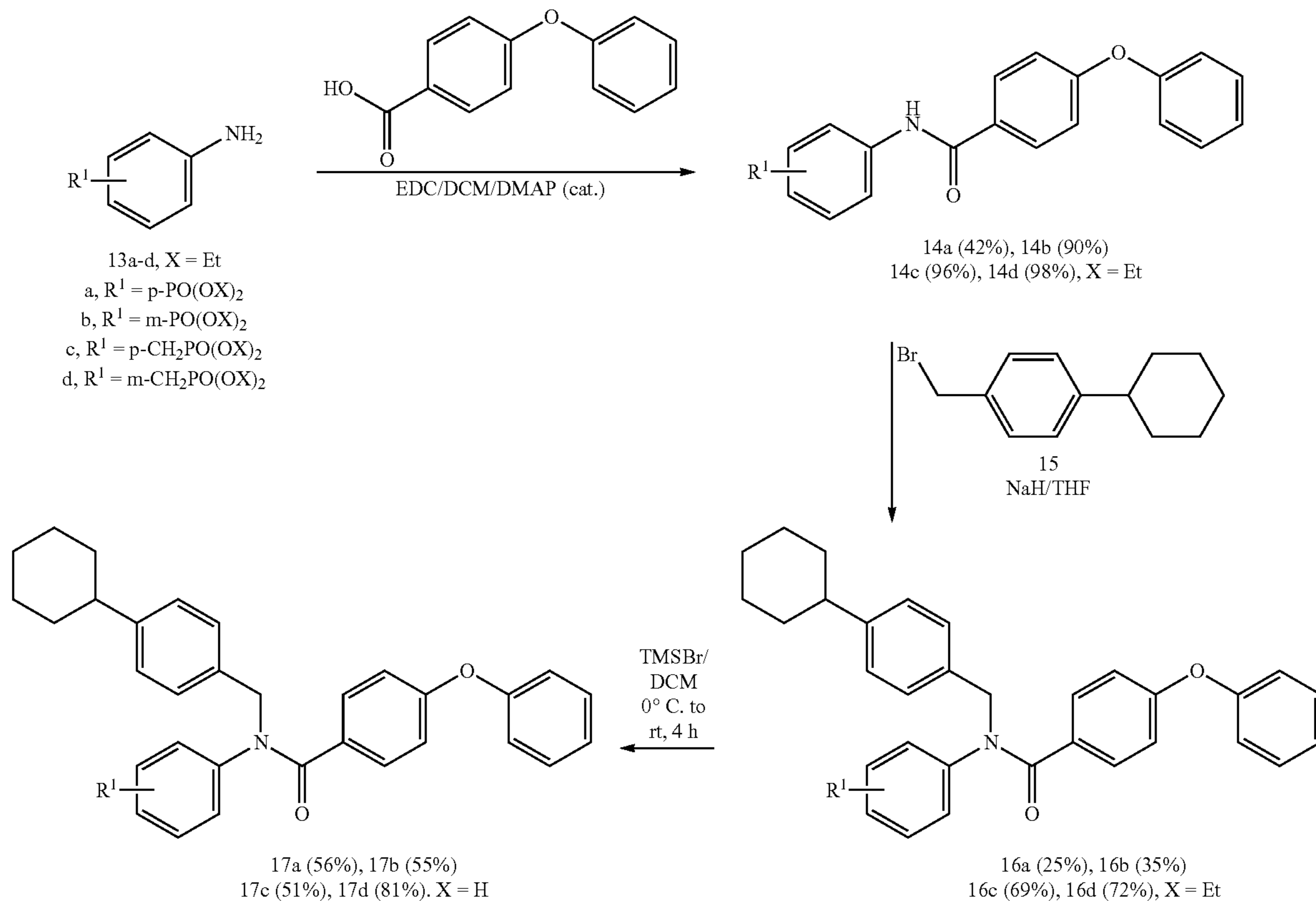
Scheme 2. Synthetic route to phosphonate containing benzamide analogs 17a-d
