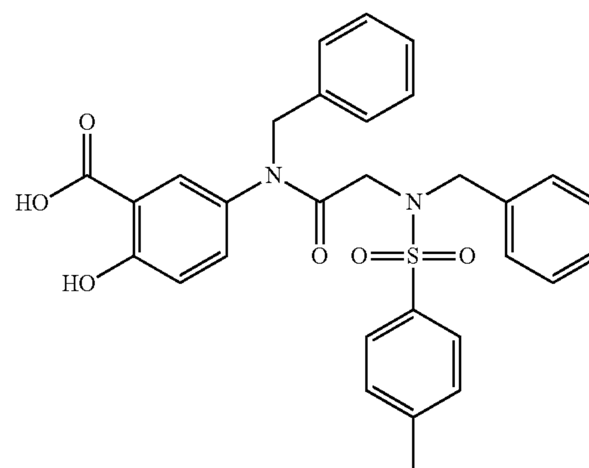
5-(N-Benzyl-2-(N-benzyl-4-methylphenylsulfonamido)acetamido)-2-hydroxybenzoic acid (9a)
