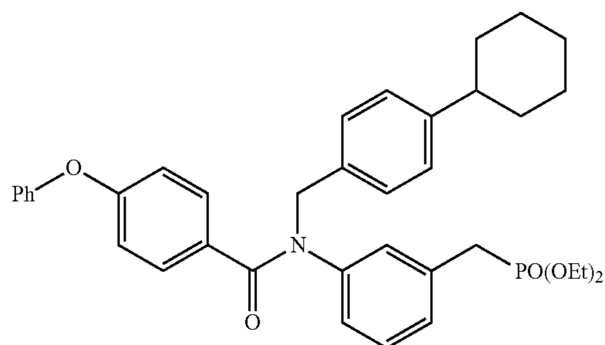
Diethyl 3-(N-(4-cyclohexylbenzyl)-4-phenoxybenzamido)benzylphosphonate (16c)
