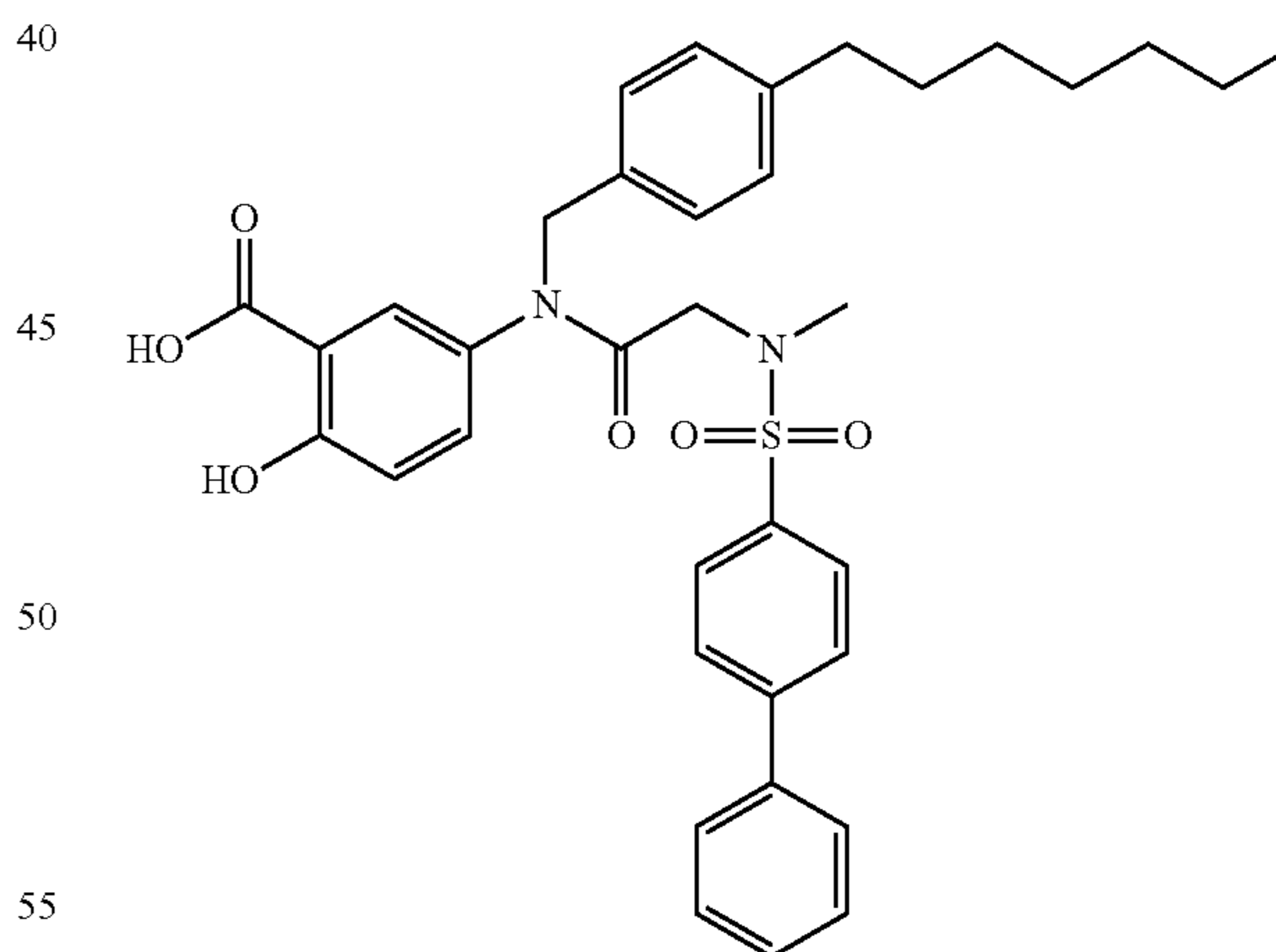
5-(N-(4-Heptylbenzyl)-2-(N-methylbiphenyl-4-ylsulfonamido)acetamido)-2-hydroxybenzoic acid (9o)
