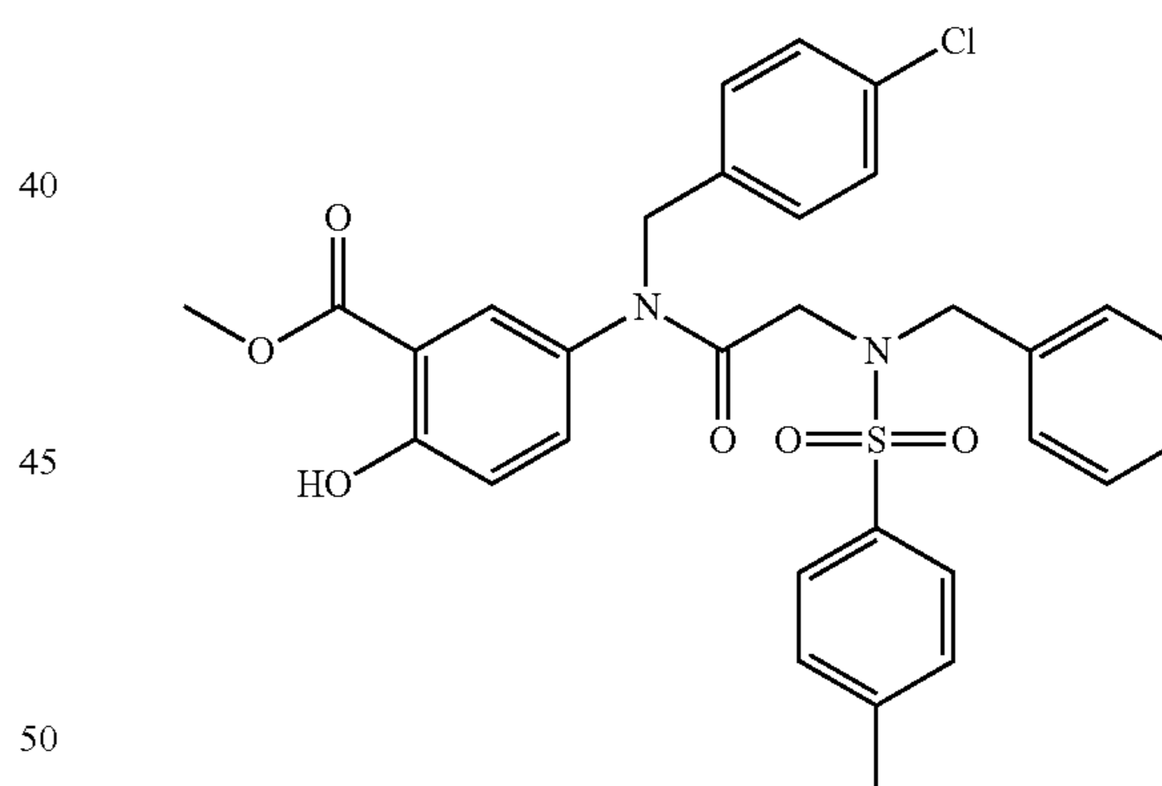
Methyl 5-(N-benzyl-2-(N-benzyl-4-methylphenylsulfonamido)acetamido)-2-hydroxybenzoate (8a)
