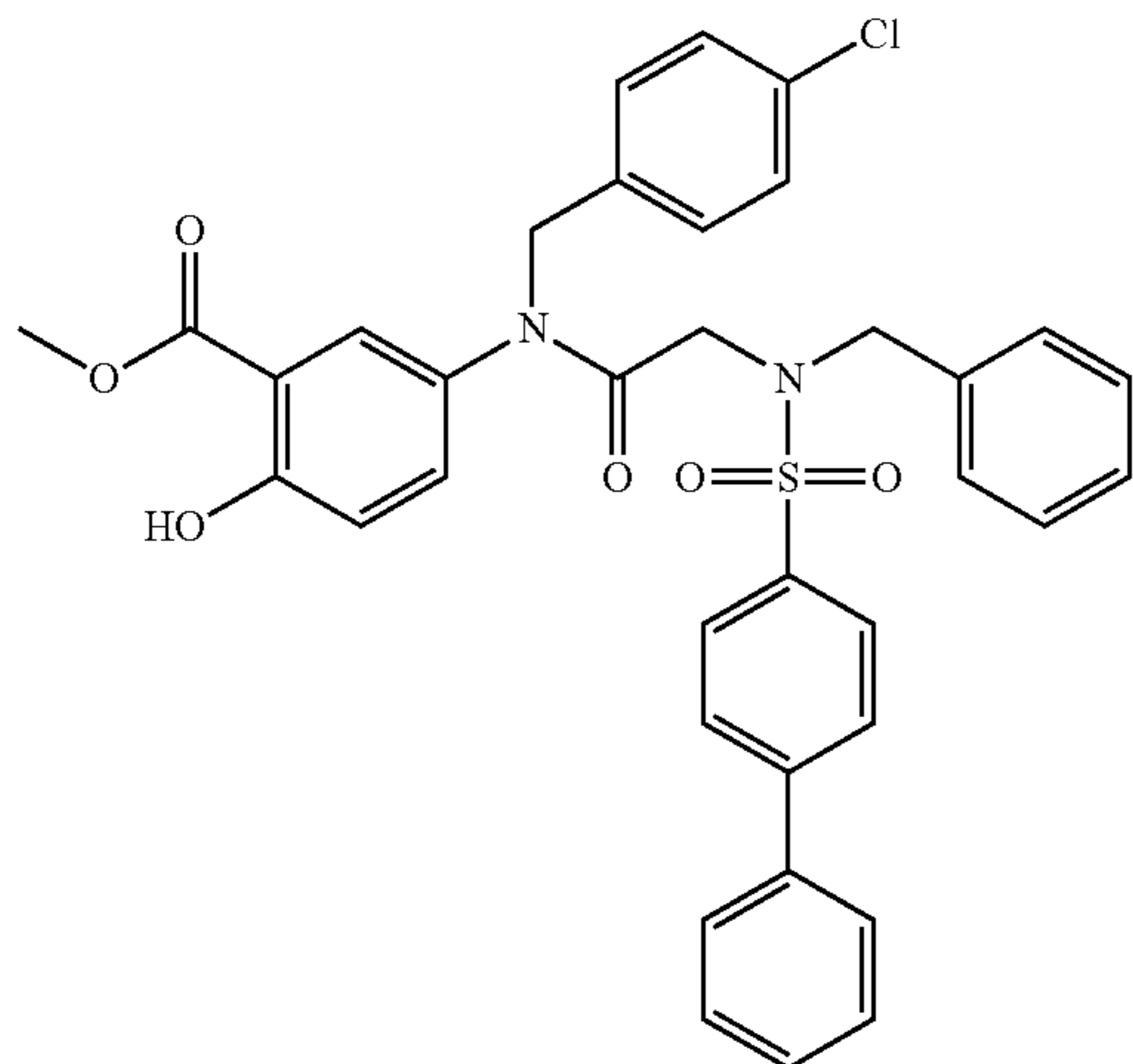
Methyl 5-(2-(N-benzylbiphenyl-4-ylsulfonamido)-N-(4-chlorobenzyl)acetamido)-2-hydroxybenzoate (8d)
