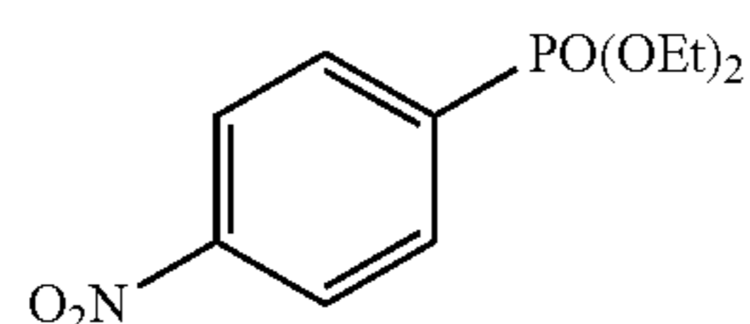
Diethyl 4-nitrophenylphosphonate
