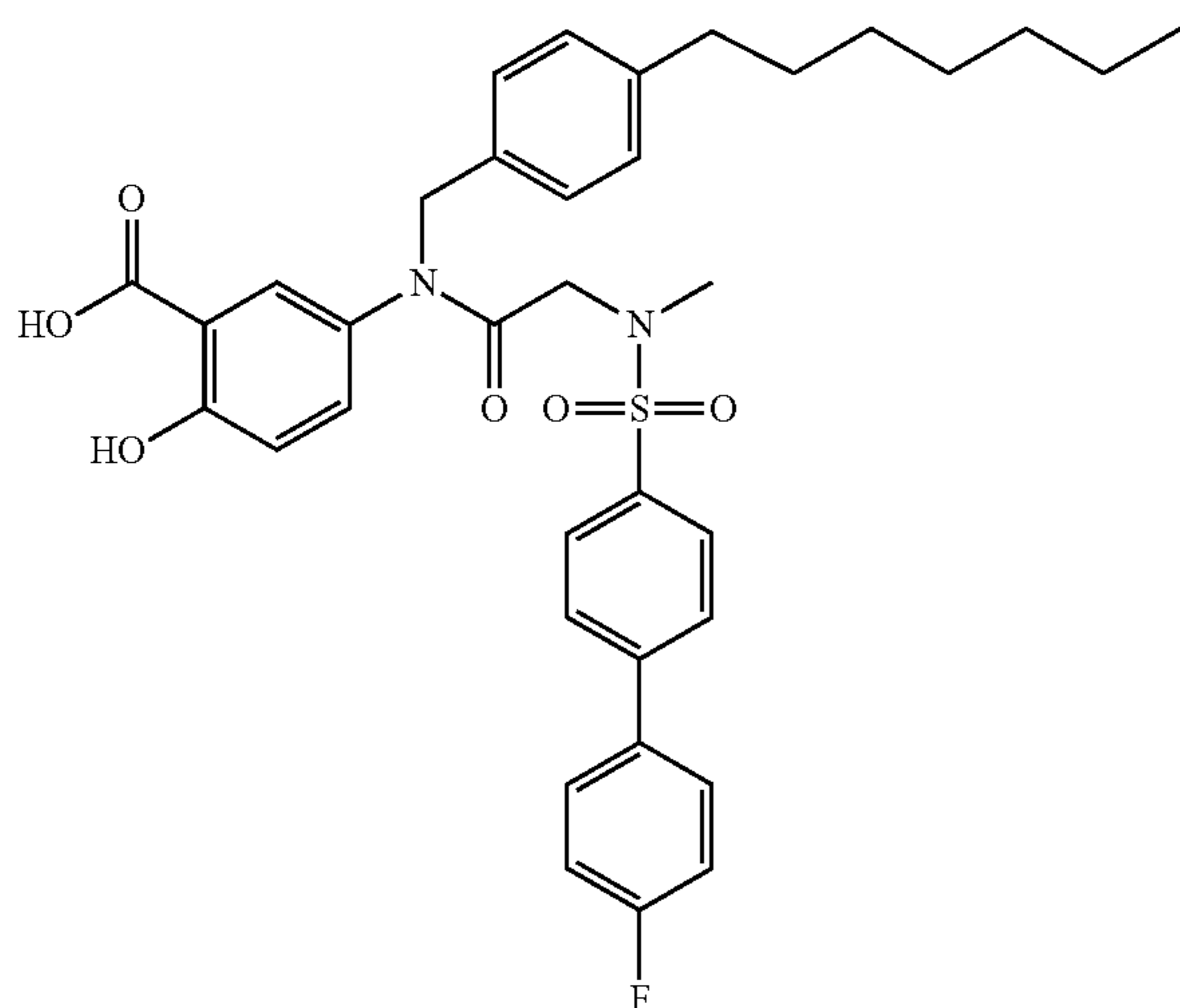
5-(2-(4'-Fluoro-N-methylbiphenyl-4-ylsulfonamido)-N-(4-heptylbenzyl)acetamido)-2-hydroxybenzoic acid (9s)
