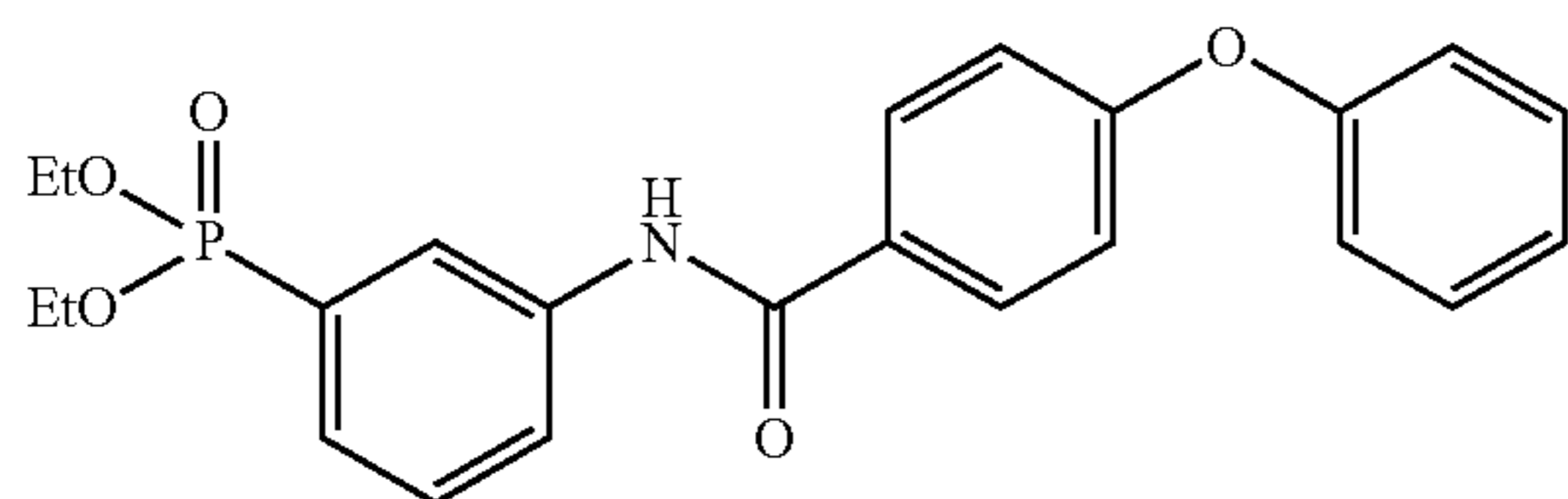
Diethyl 3-(4-phenoxybenzamido)phenylphosphonate (14b)
