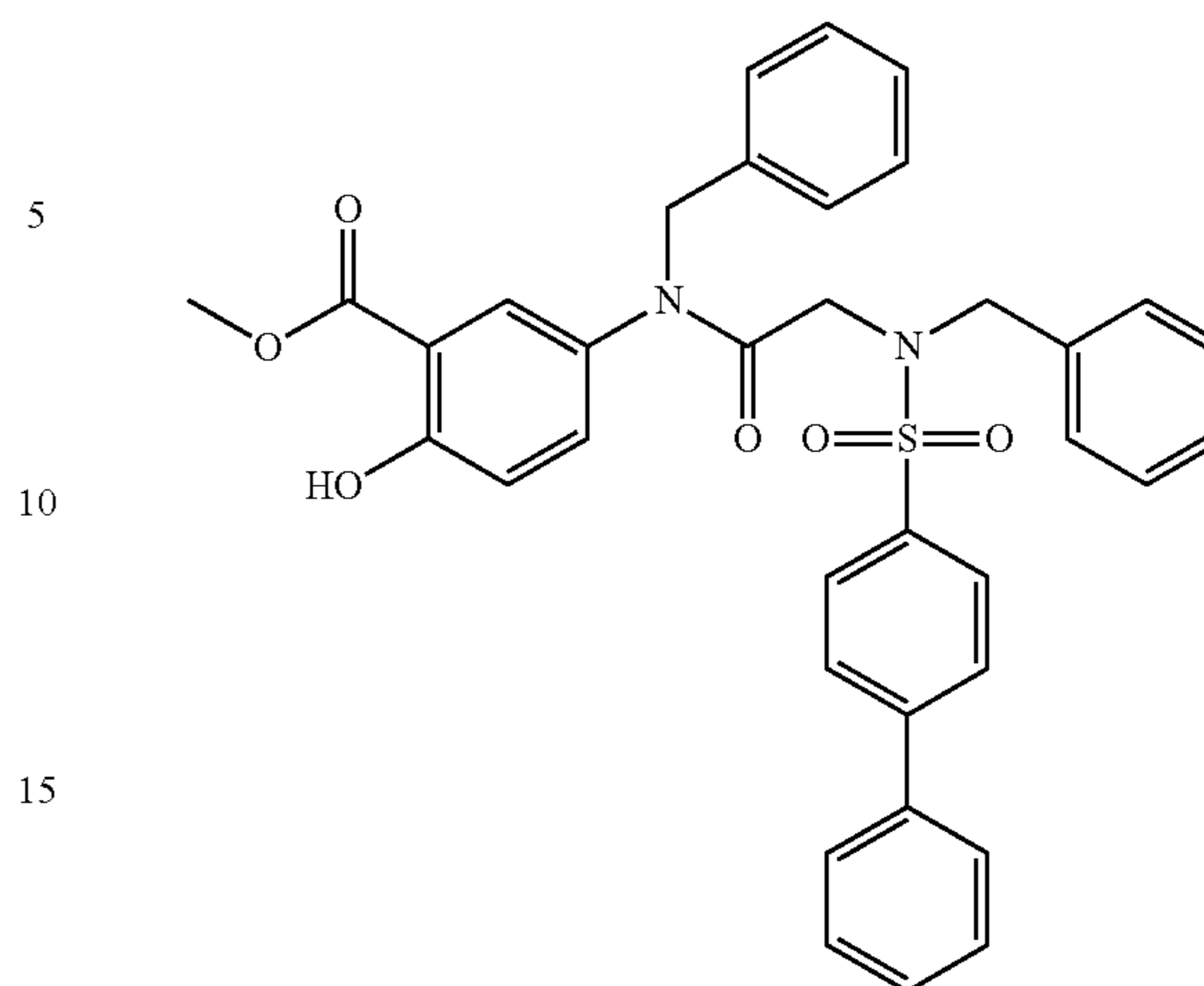
2-(N-Benzylbiphenyl-4-ylsulfonamido)acetic acid (7f)
