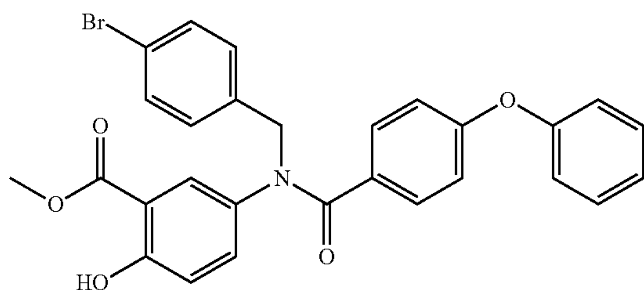
Methyl 5-(N-(4-bromobenzyl)-4-phenoxybenzamido)-2-hydroxybenzoate (19e)
