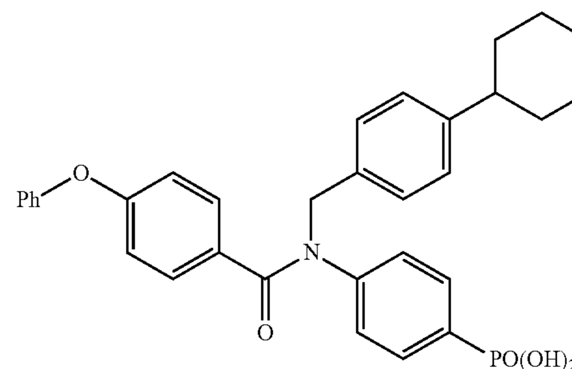
4-(N-(4-Cyclohexylbenzyl)-4-phenoxybenzamido)phenylphosphonic acid (17a)
