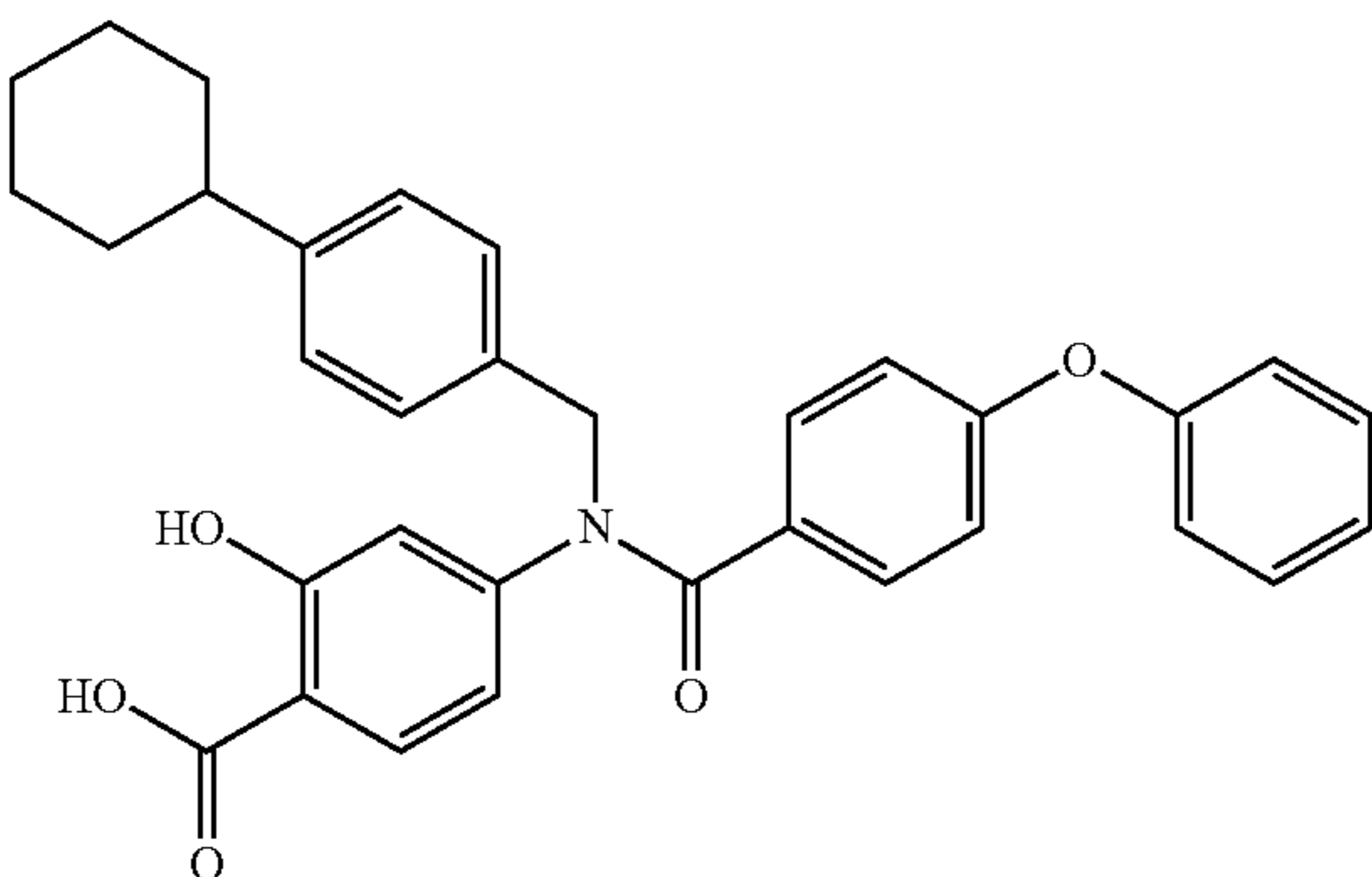
4-(N-(4-Cyclohexylbenzyl)-4-phenoxybenzamido)-2-hydroxybenzoate (33)
