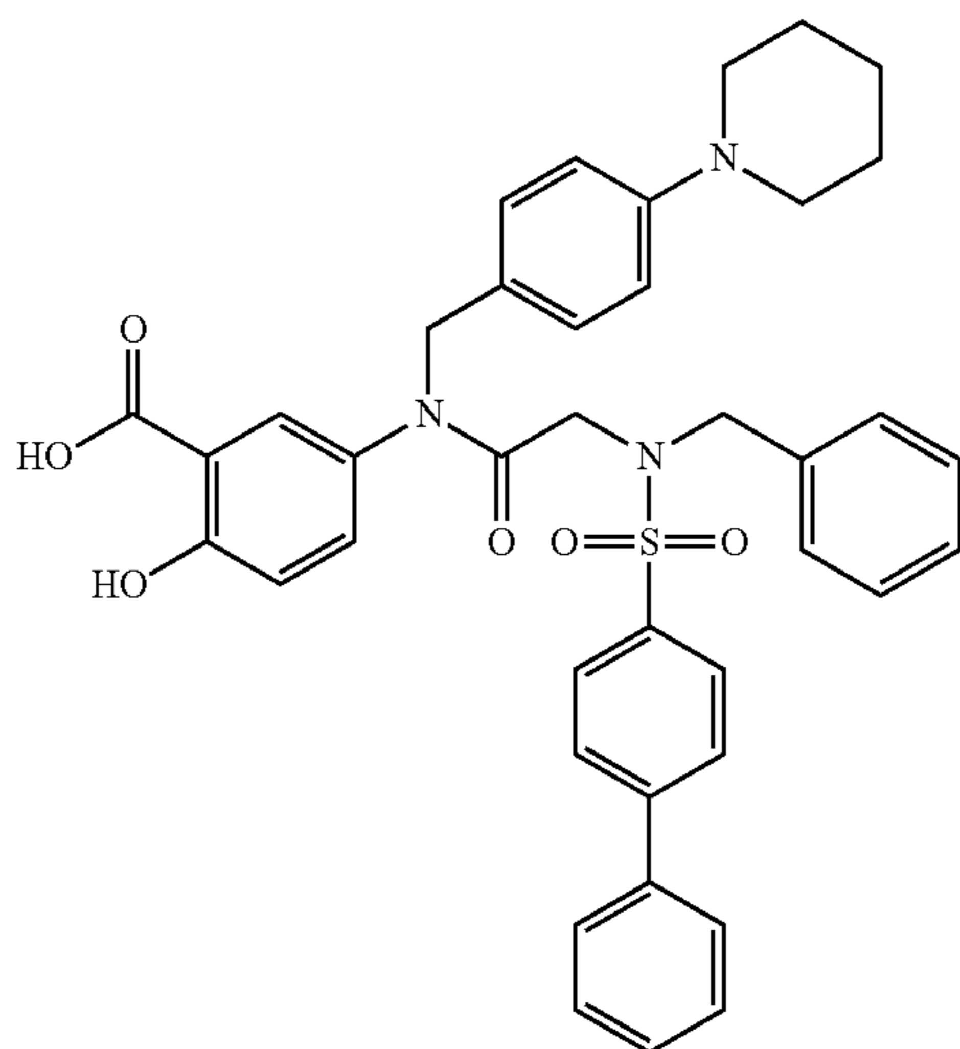
5-(2-(N-Benzylbiphenyl-4-ylsulfonamido)-N-(4-piperidin-1-yl)benzyl)acetamido)-2-hydroxybenzoic acid (9t)
