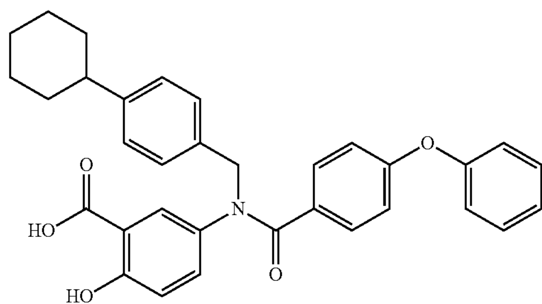
5-(N-(4-Cyclohexylbenzyl)-4-phenoxybenzamido)-2-hydroxybenzoic acid (20g)
