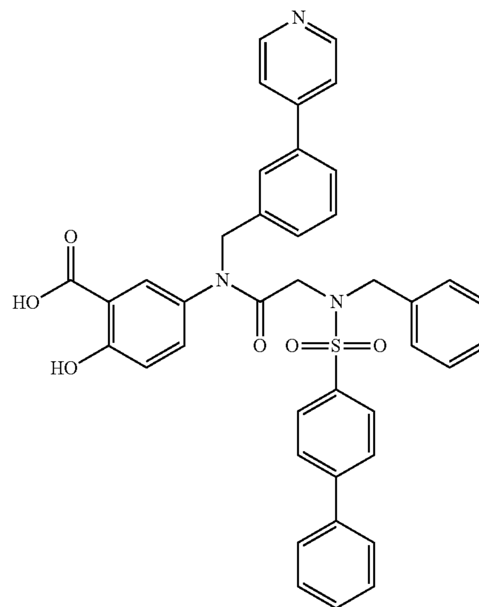
5-(2-(N-Benzylbiphenyl-4-ylsulfonamido)-N-(3-(pyridin-4-yl)benzyl)acetamido)-2-hydroxybenzoic acid (9u)
