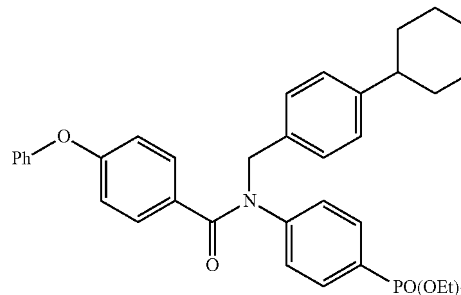
Diethyl 4-(N-(4-cyclohexylbenzyl)-4-phenoxybenzamido)phenylphosphonate (16a)
