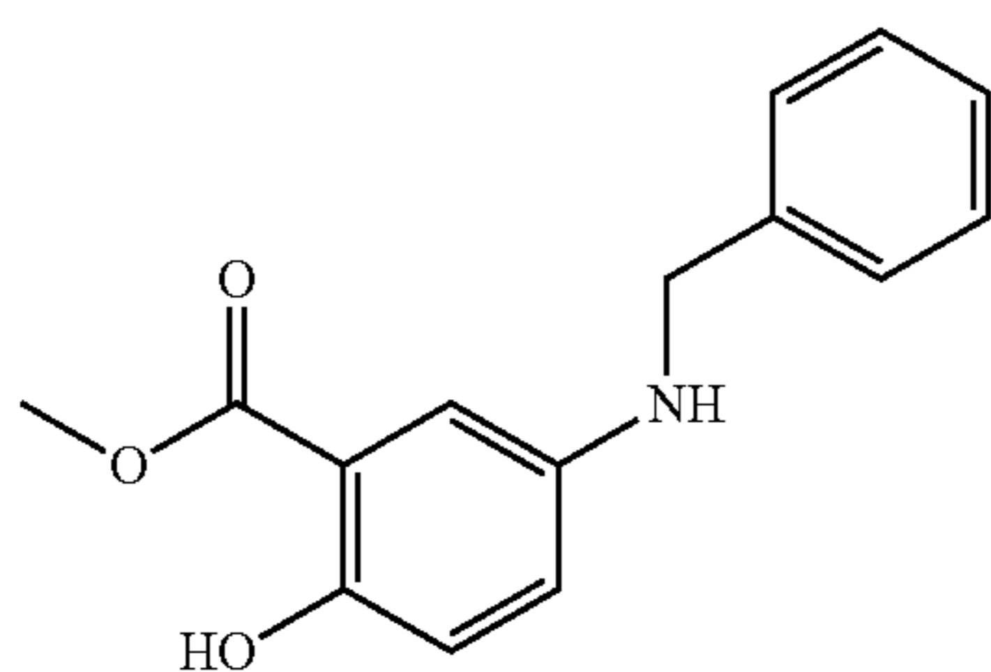
Methyl 5-(benzylamino)-2-hydroxybenzoate (6a)
