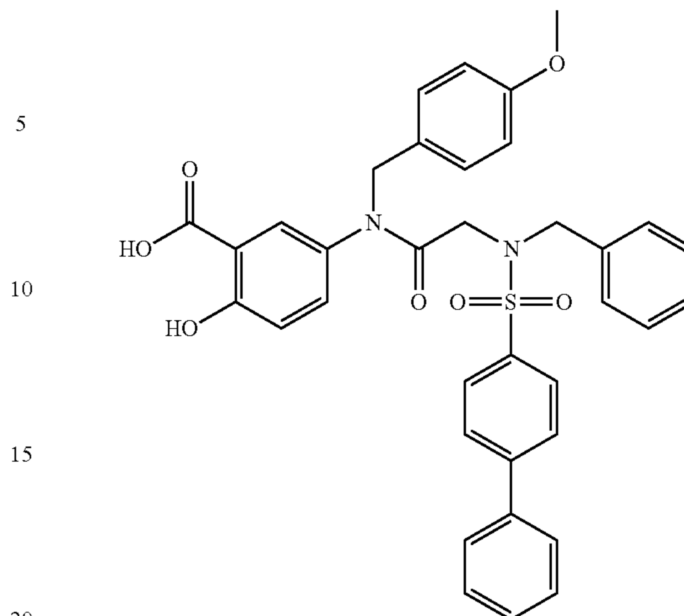
5-(2-(N-Benzylbiphenyl-4-ylsulfonamido)-N-(4-methoxybenzyl)acetamido)-2-hydroxybenzoic acid (9f)
