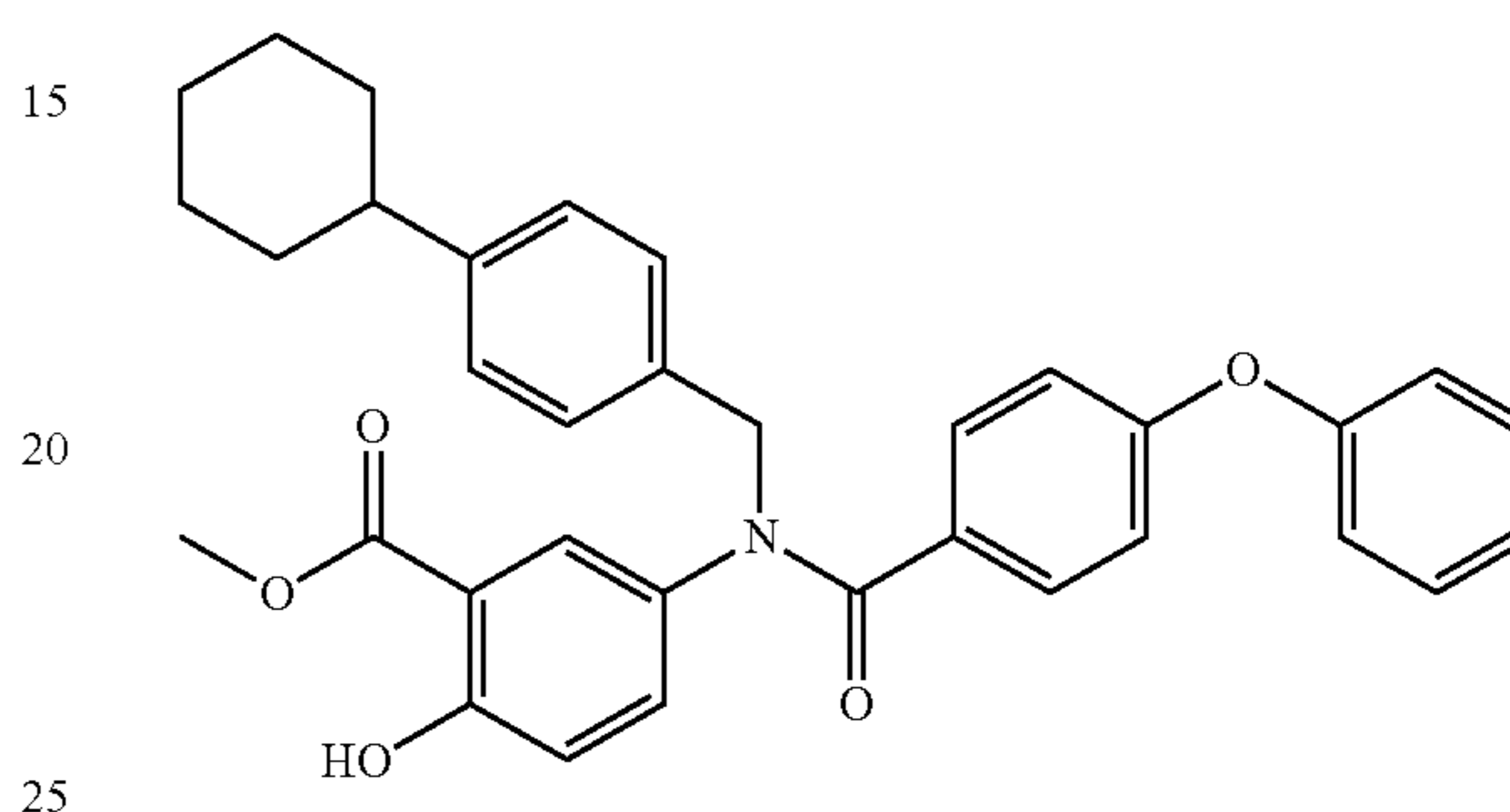
Methyl 5-(N-(4-cyclohexylbenzyl)-4-phenoxybenzamido)-2-hydroxybenzoate (19g)
