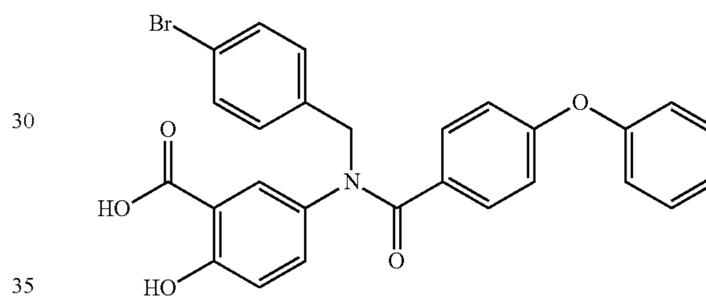
5-(N-(4-Bromobenzyl)-4-phenoxybenzamido)-2-hydroxybenzoic acid (20e)
