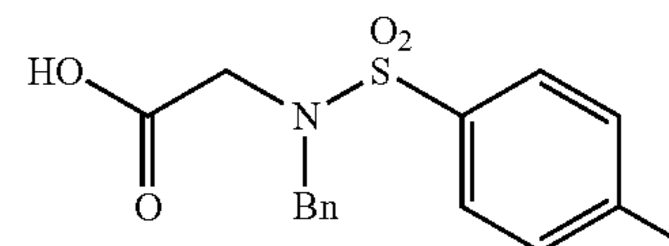
2-(N-Benzyl-4-methylphenylsulfonamido)acetic acid (7e)
