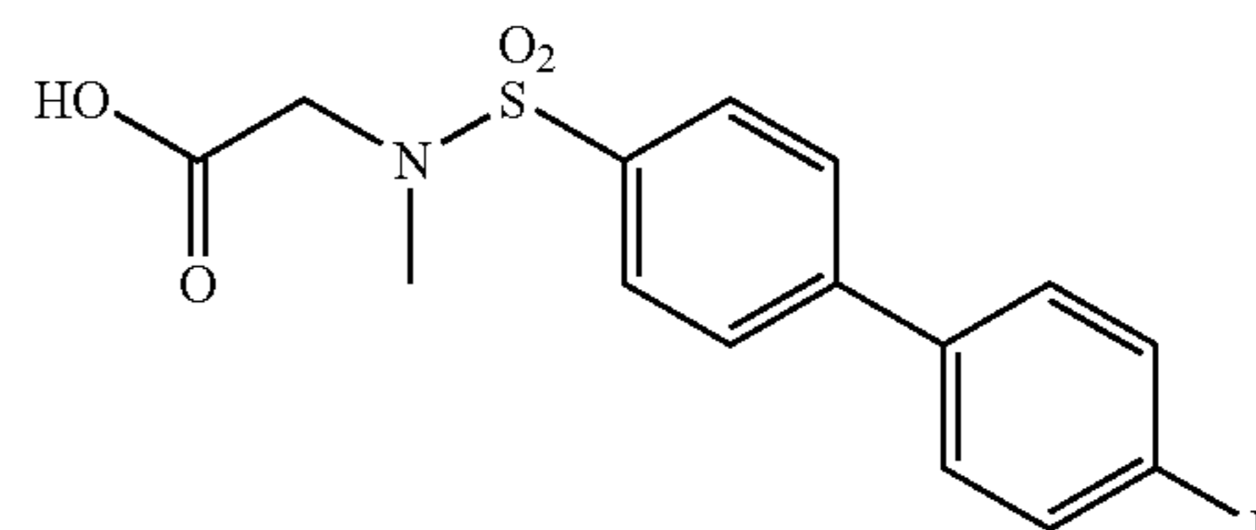
2-(4'-Fluoro-N-methylbiphenyl-4-ylsulfonamido)acetic acid (7d)
