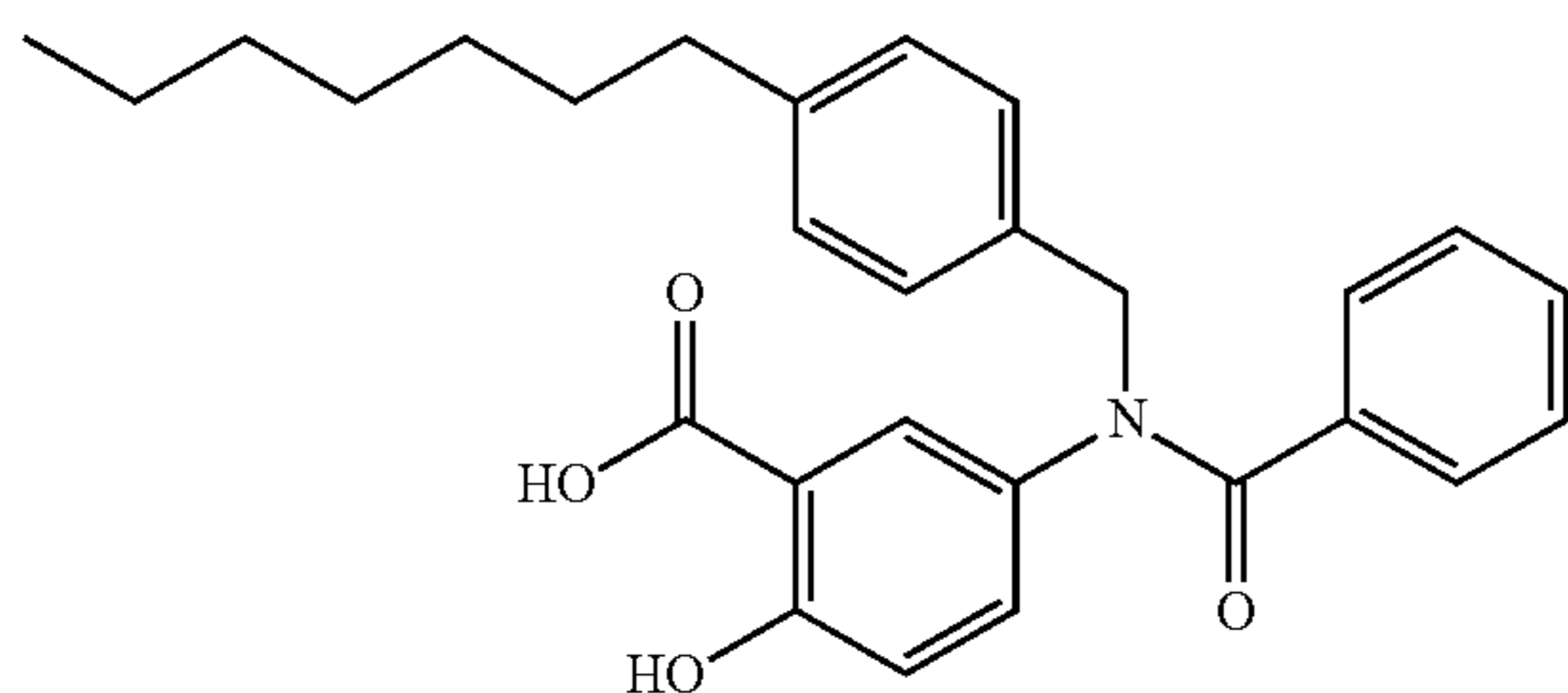
5-(N-(4-Heptylbenzyl)benzamido)-2-hydroxybenzoic acid (20h)
