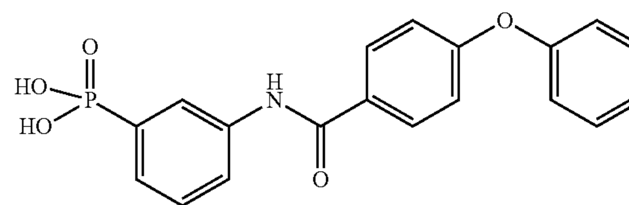
3-(4-Phenoxybenzamido)phenylphosphonic acid (18b)
