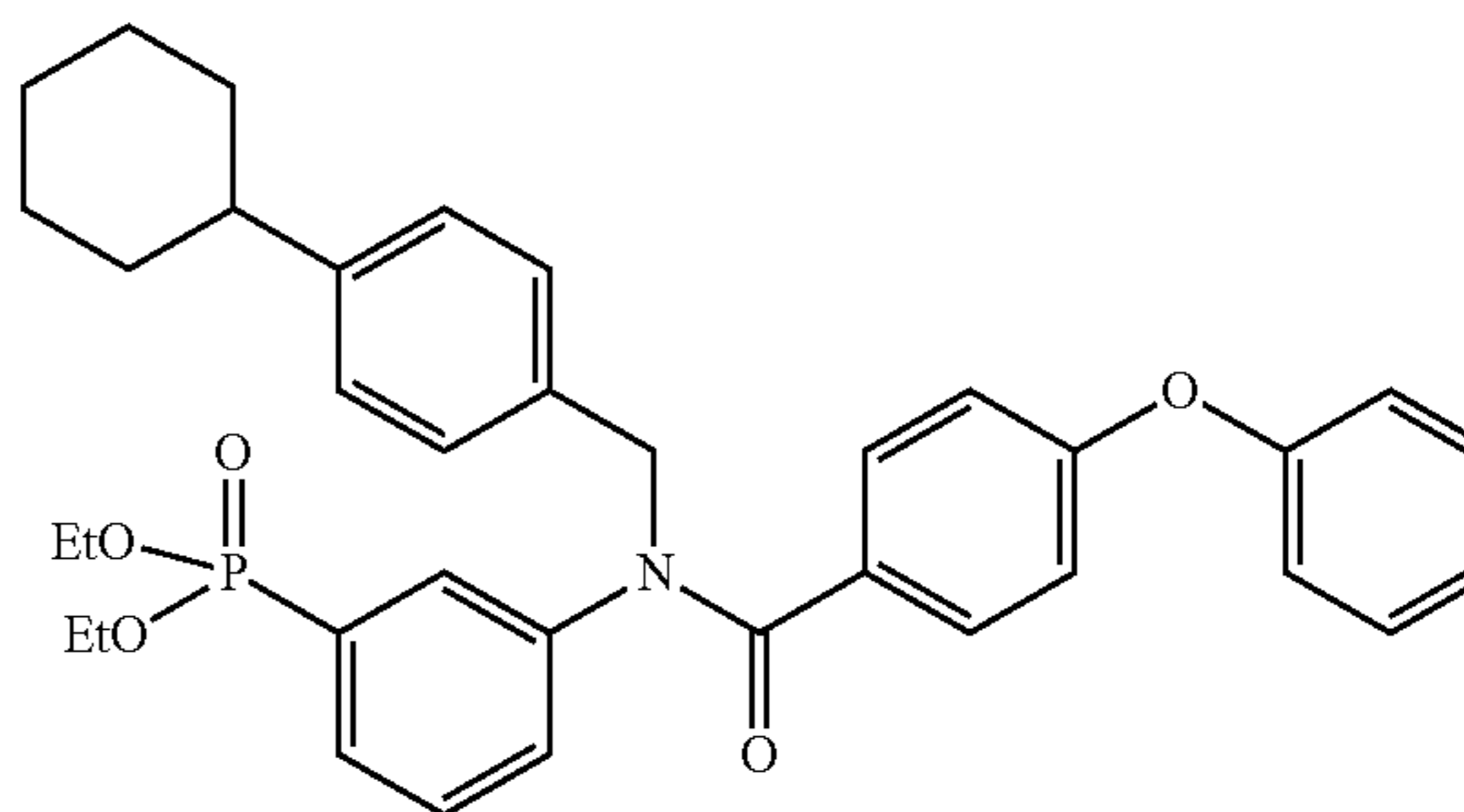
Diethyl 3-(N-(4-cyclohexylbenzyl)-4-phenoxybenzamido)phenylphosphonate (16b)
