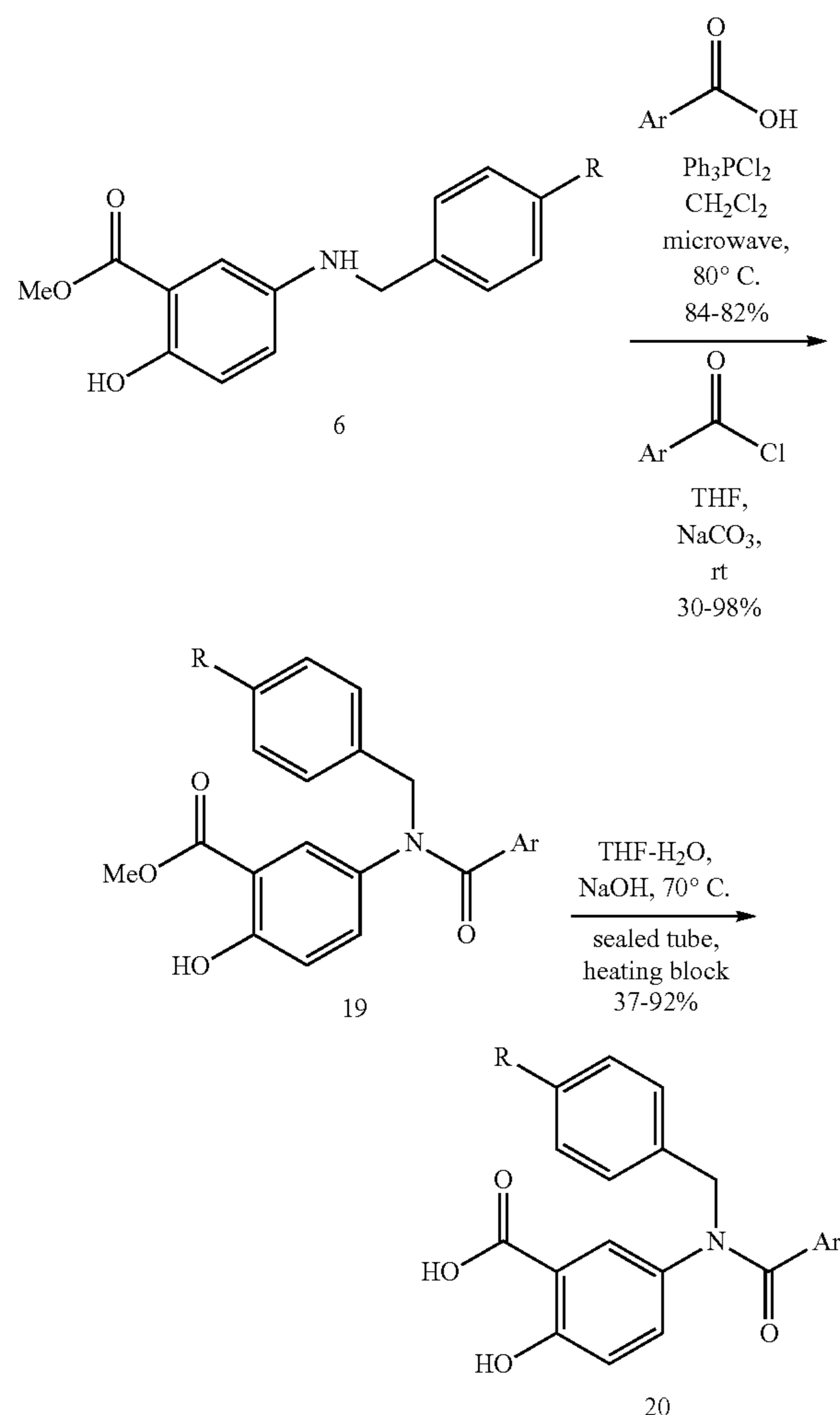
Scheme 3. Synthetic route to N-benzamide library 20
