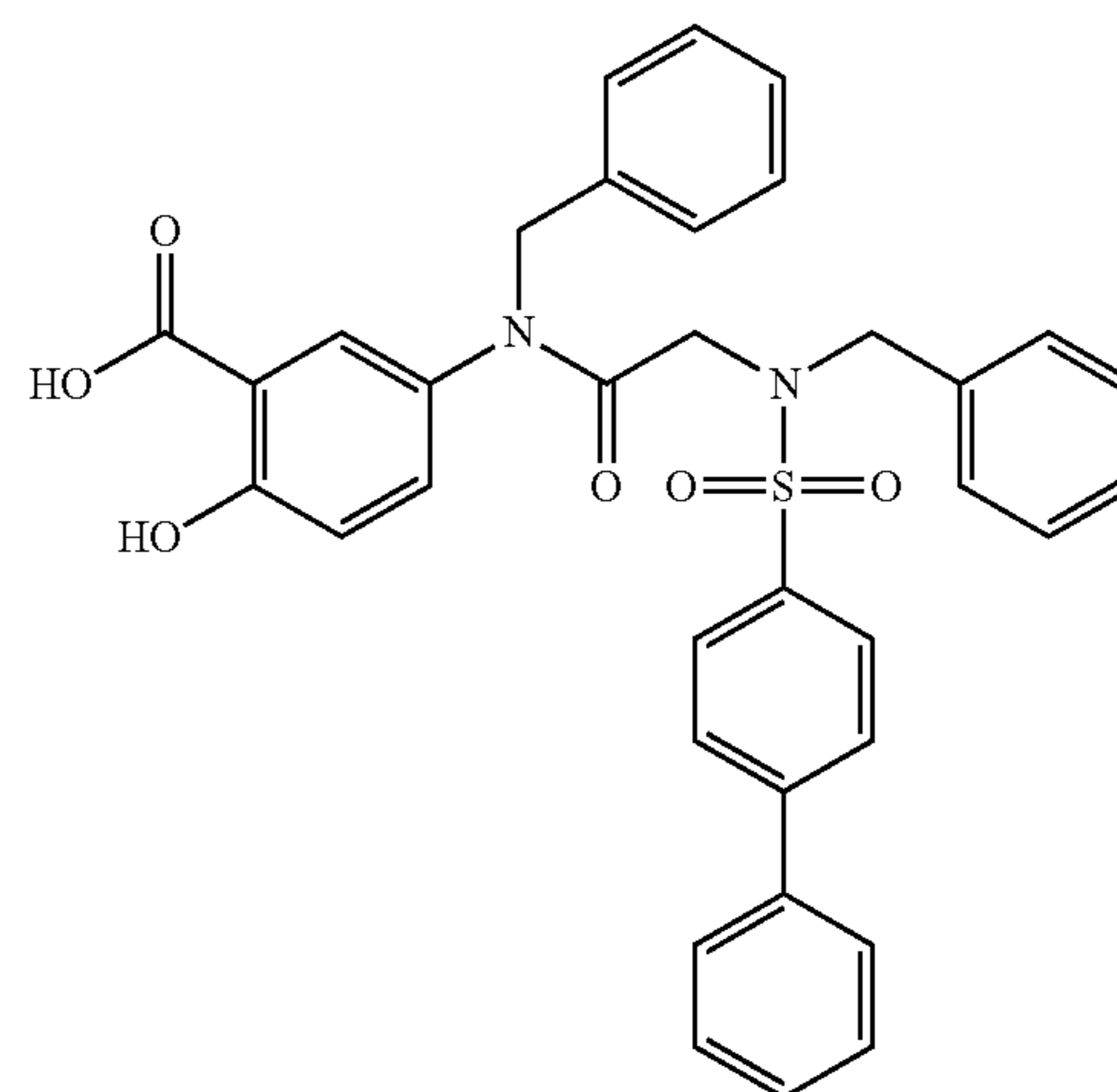
5-(N-Benzyl-2-(N-benzylbiphenyl-4-ylsulfonamido)acetamido)-2-hydroxybenzoic acid (9b)
