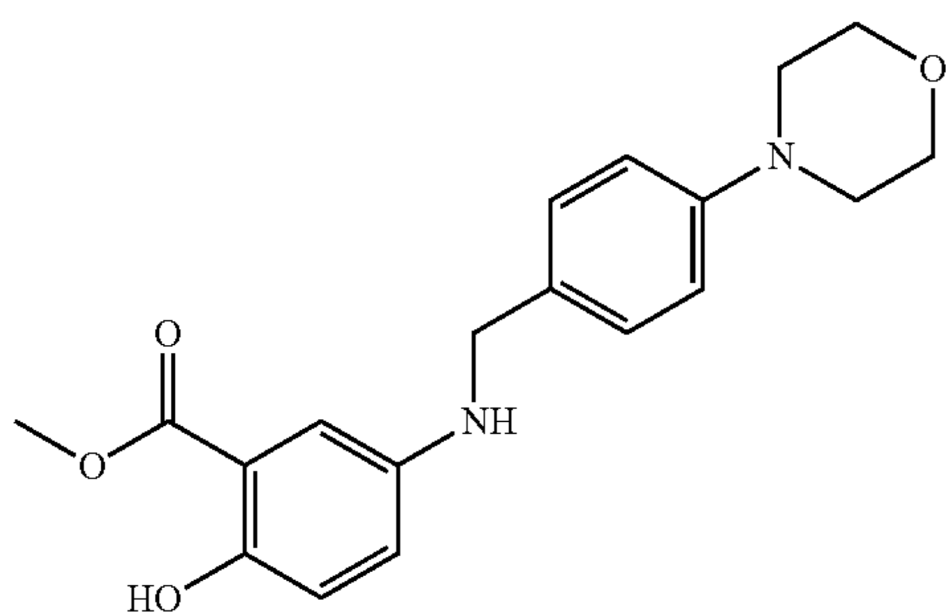
Methyl 2-hydroxy-5-(4-morpholinobenzylamino)benzoate (6e)
