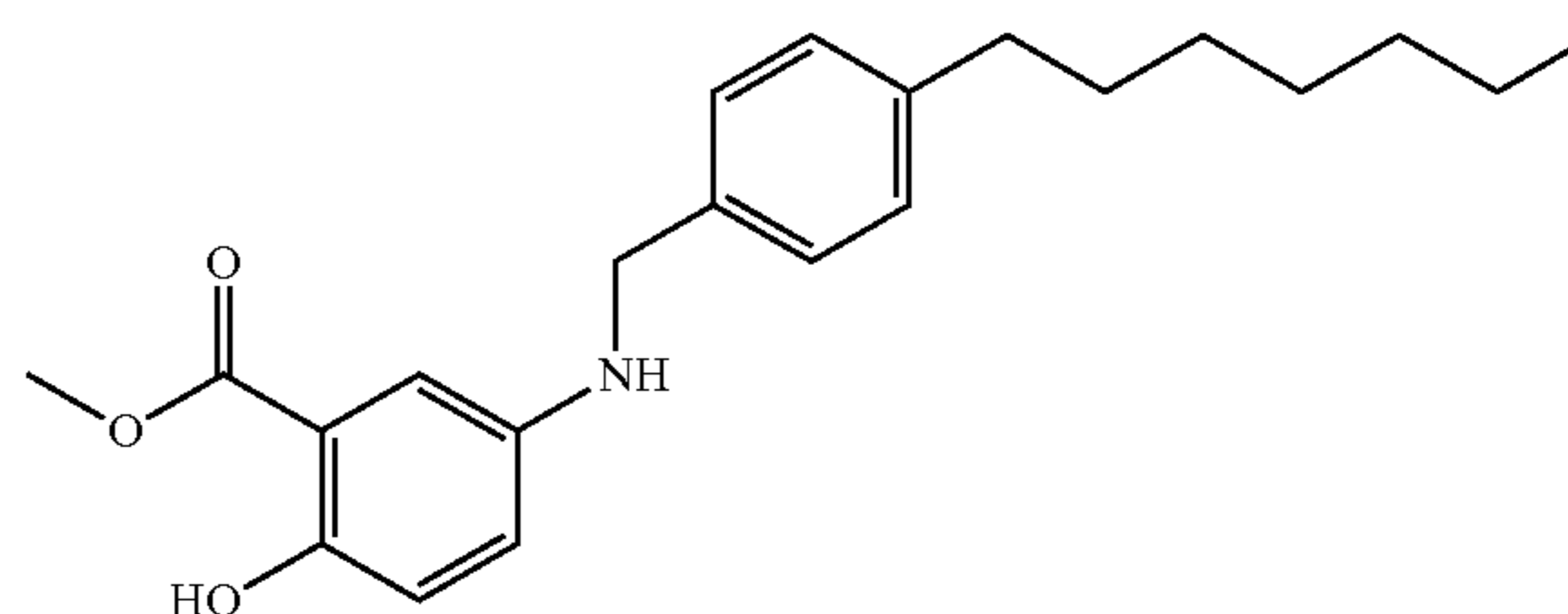
Methyl 5-(4-heptylbenzylamino)-2-hydroxybenzoate (6i)
