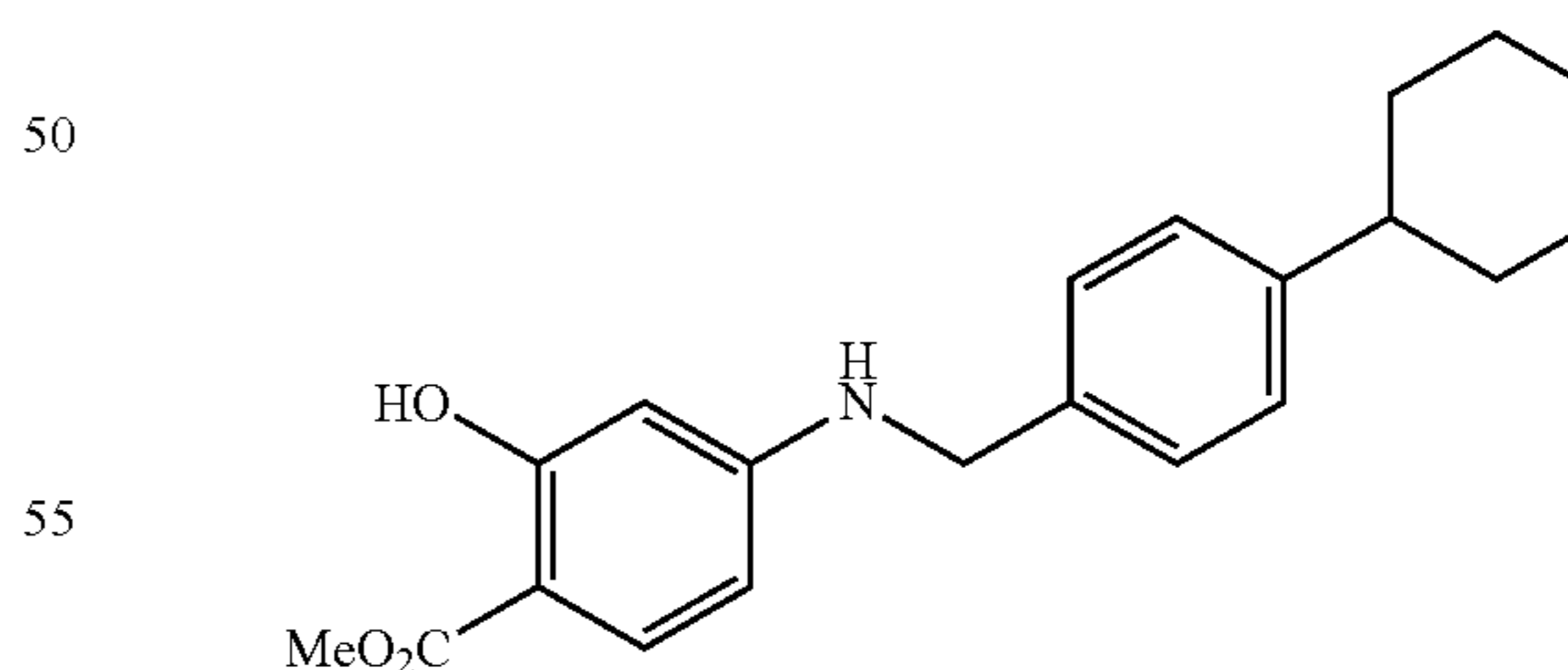
Methyl 4-(4-cyclohexylbenzylamino)-2-hydroxybenzoate (31)
