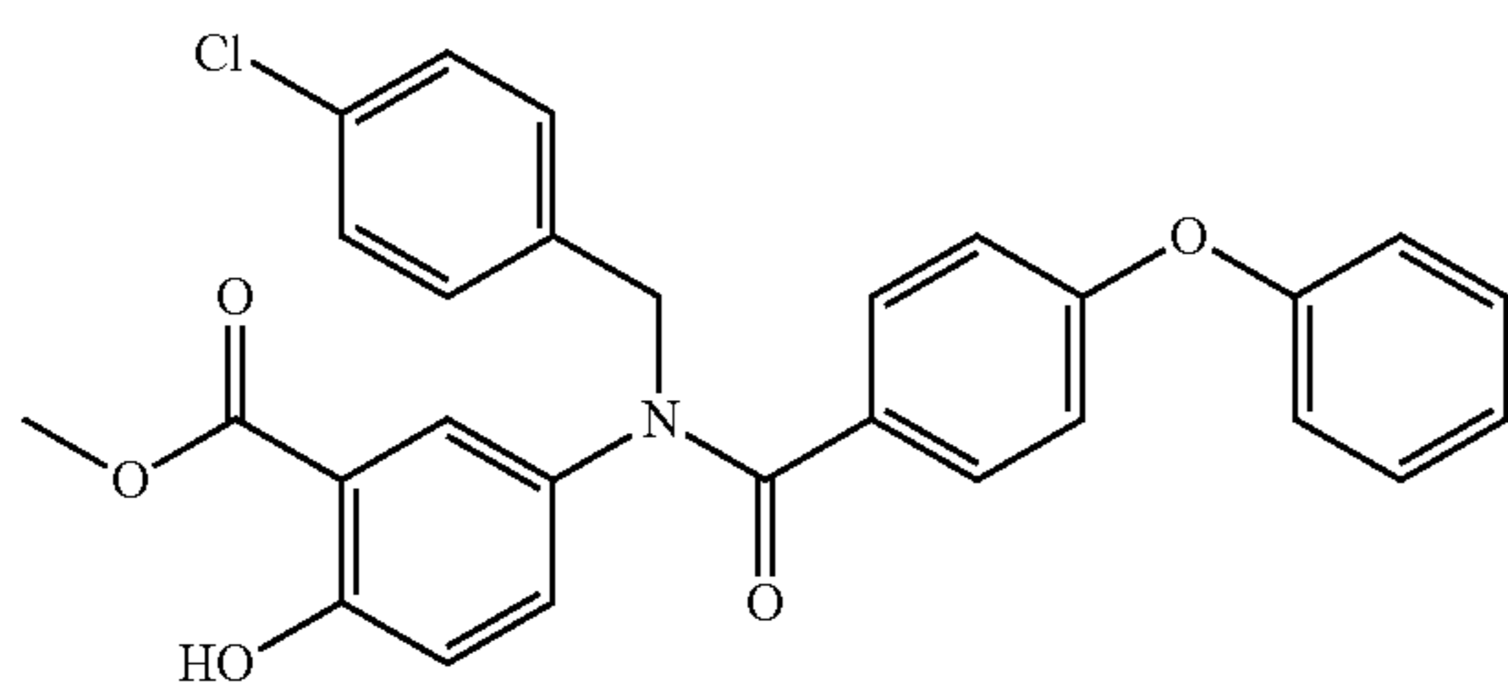
Methyl 5-(N-(4-chlorobenzyl)-4-phenoxybenzamido)-2-hydroxybenzoate (19d)
