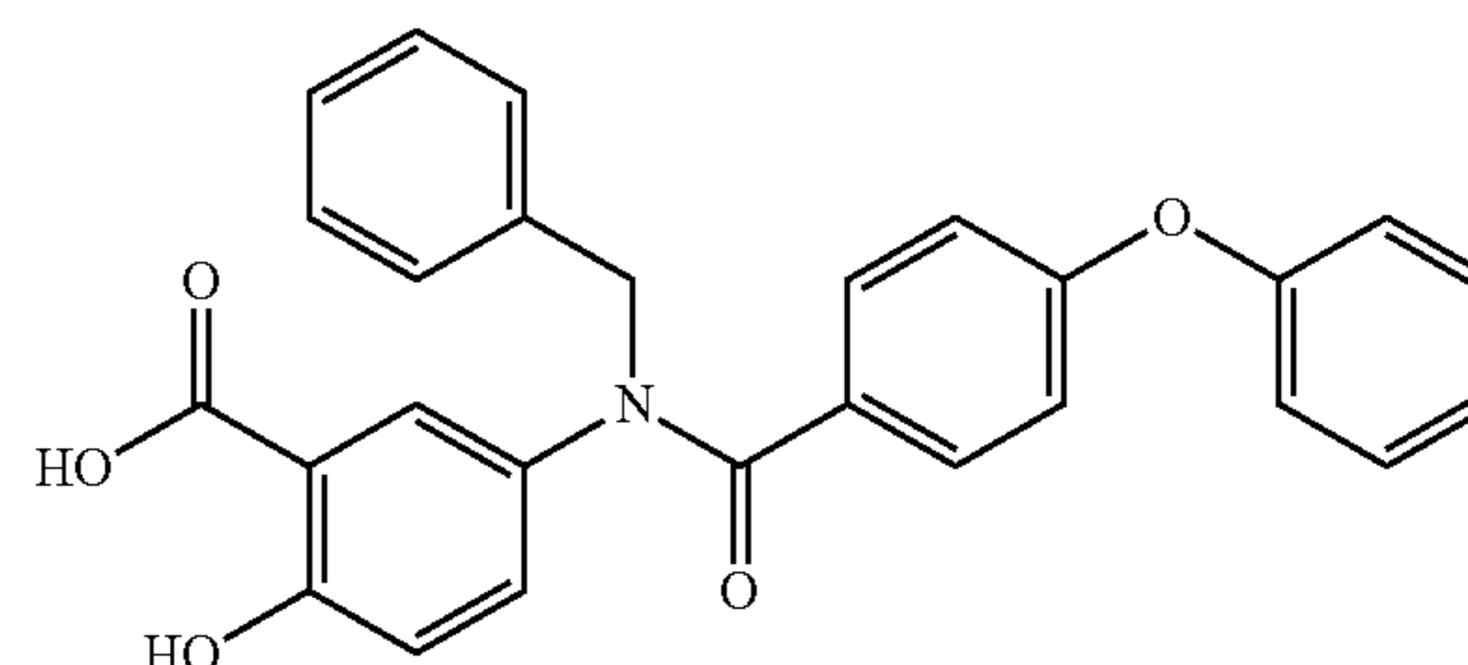
5-(N-Benzyl-4-phenoxybenzamido)-2-hydroxybenzoic acid (20a)
