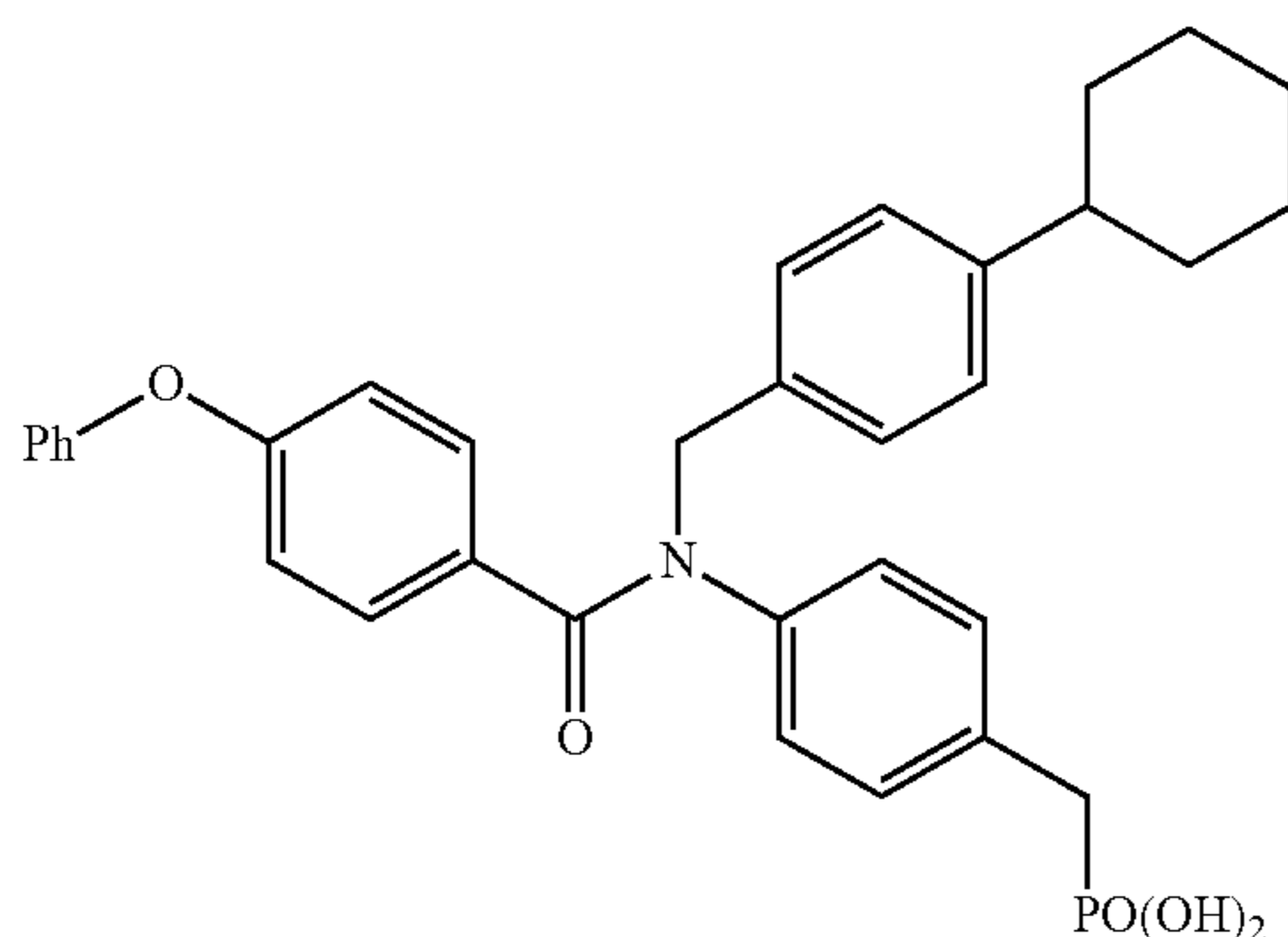
4-(N-(4-Cyclohexylbenzyl)-4-phenoxybenzamido)benzylphosphonic acid (17c)
