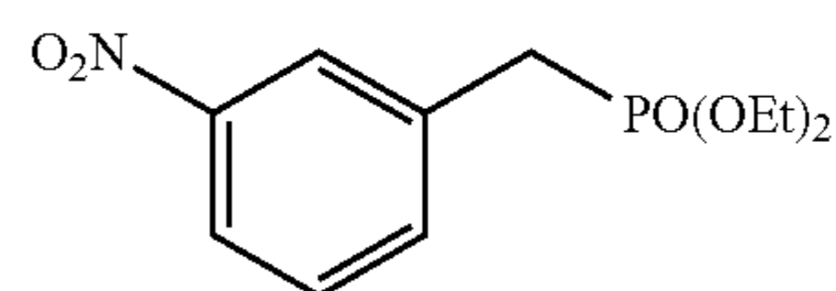
Diethyl 3-nitrobenzylphosphonate
