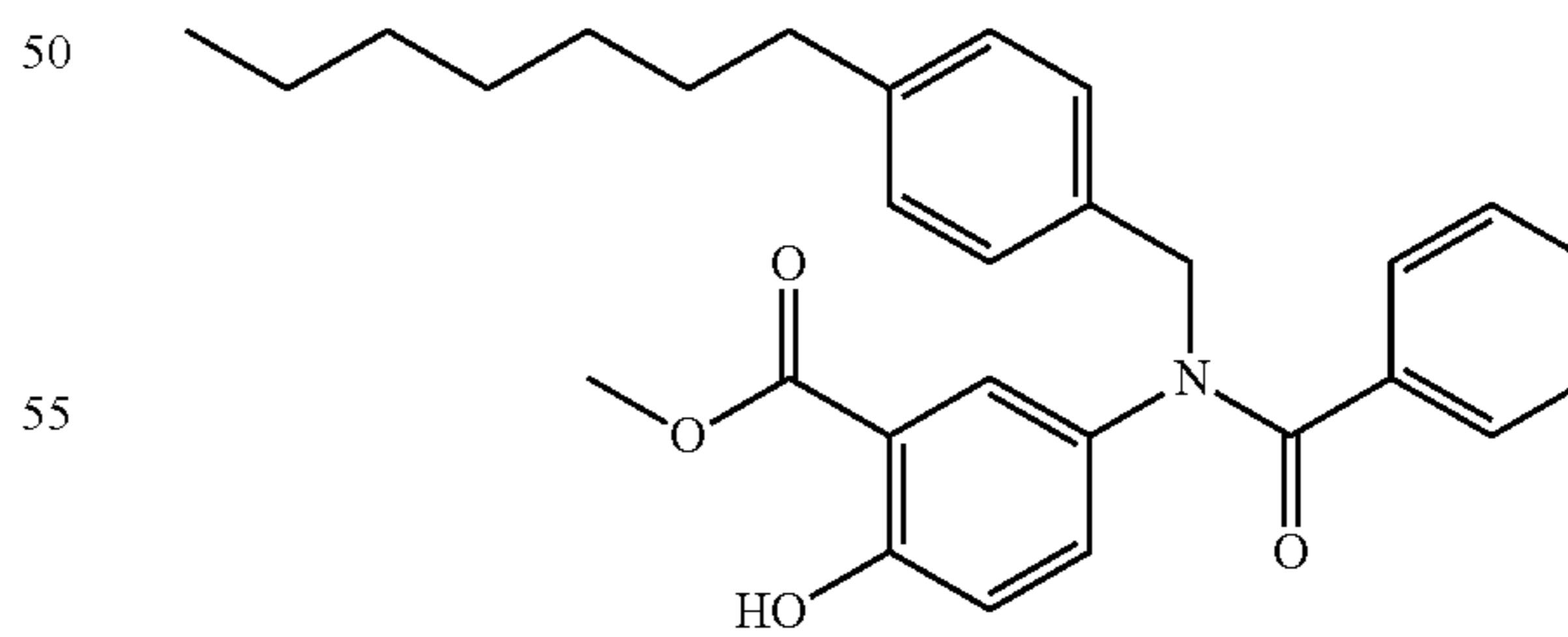
Methyl 5-(N-(4-heptylbenzyl)benzamido)-2-hydroxybenzoate (19h)
