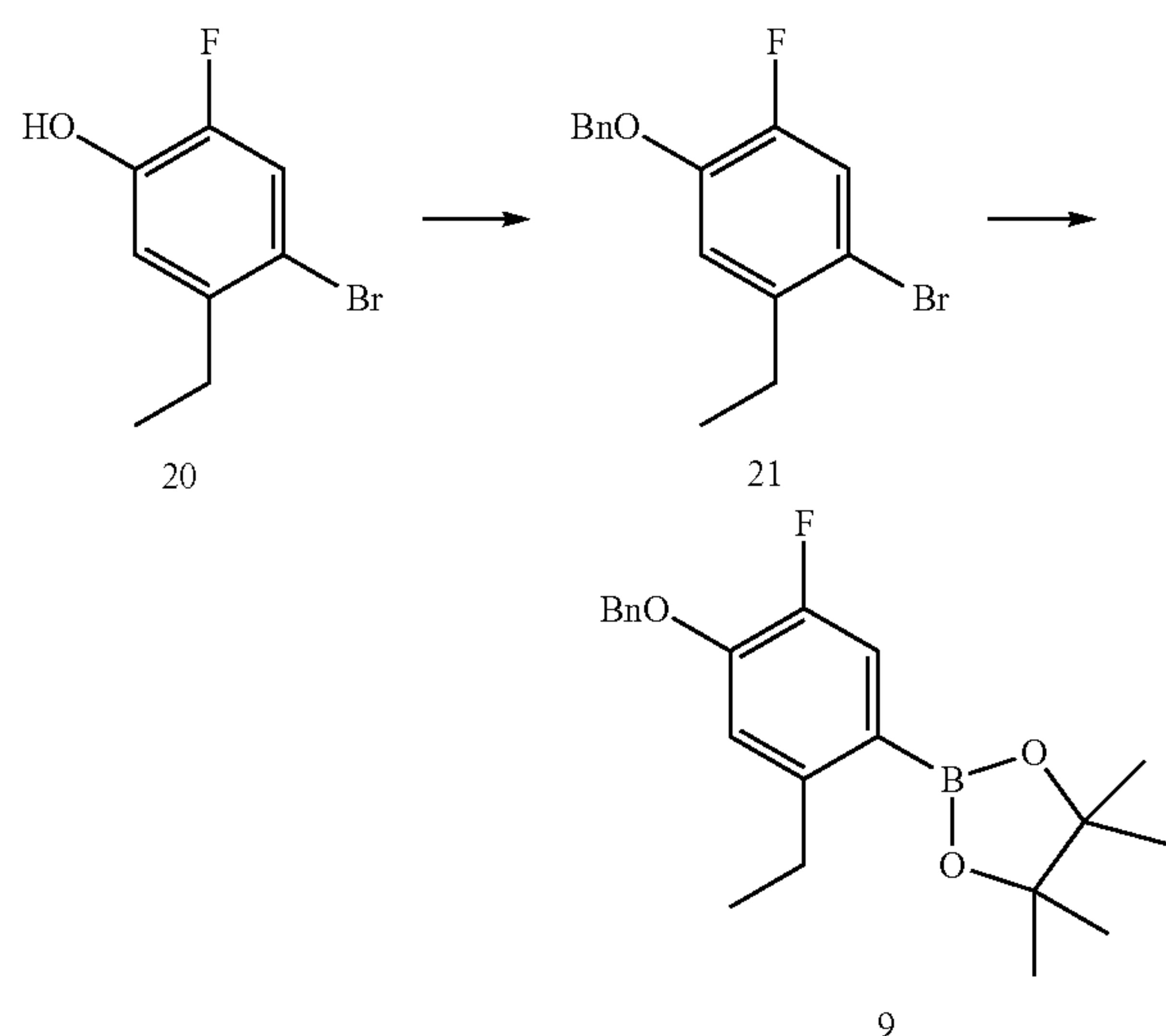
(a) 1-(Benzyloxy)-4-bromo-5-ethyl-2-fluorobenzene (21)
