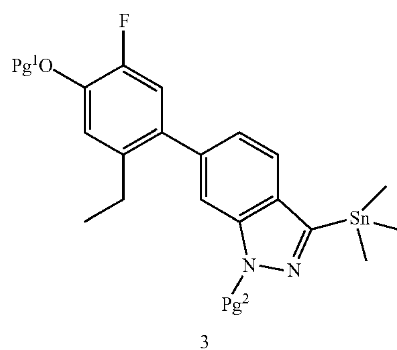
Scheme 2
