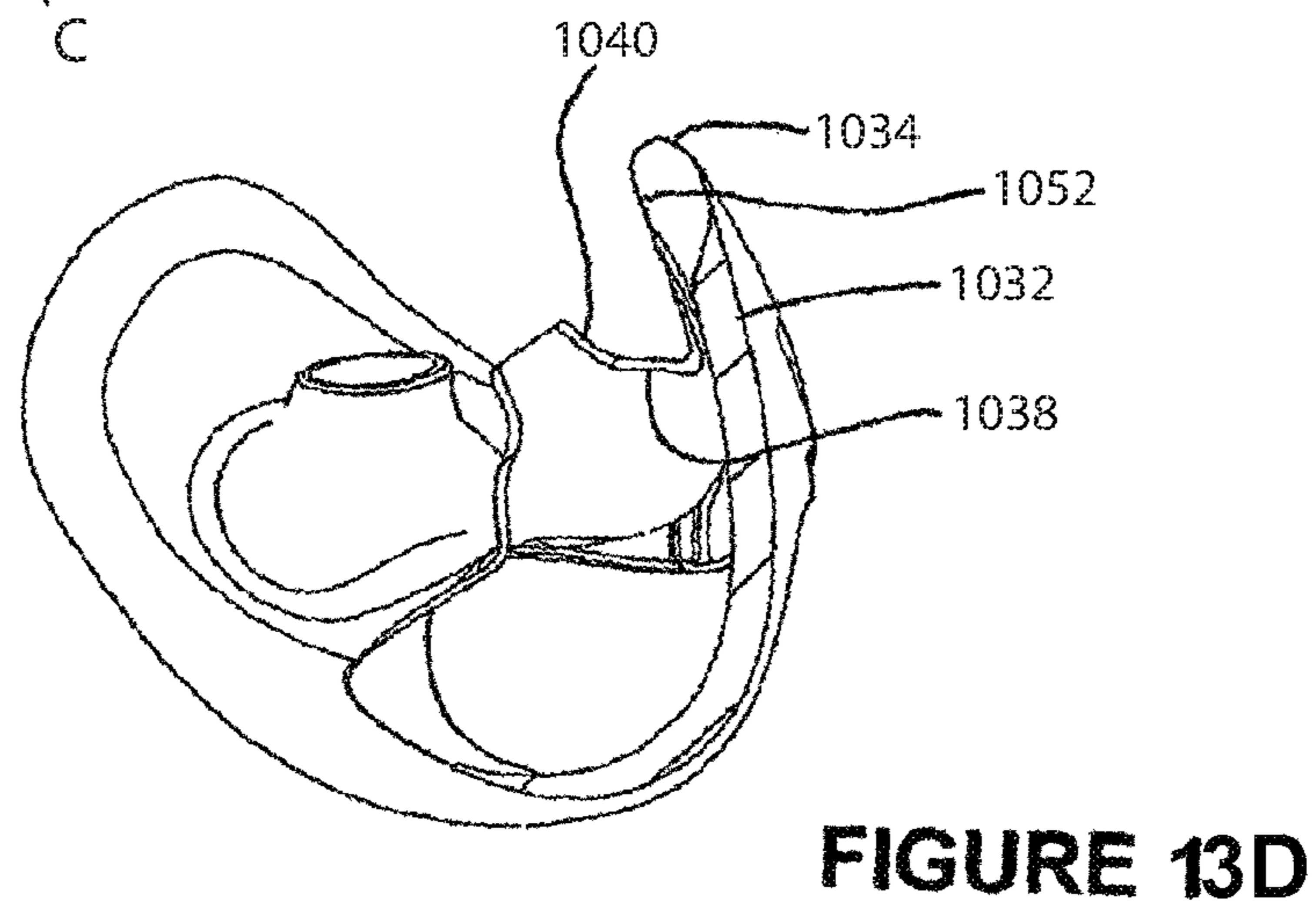
SECTION C-C
