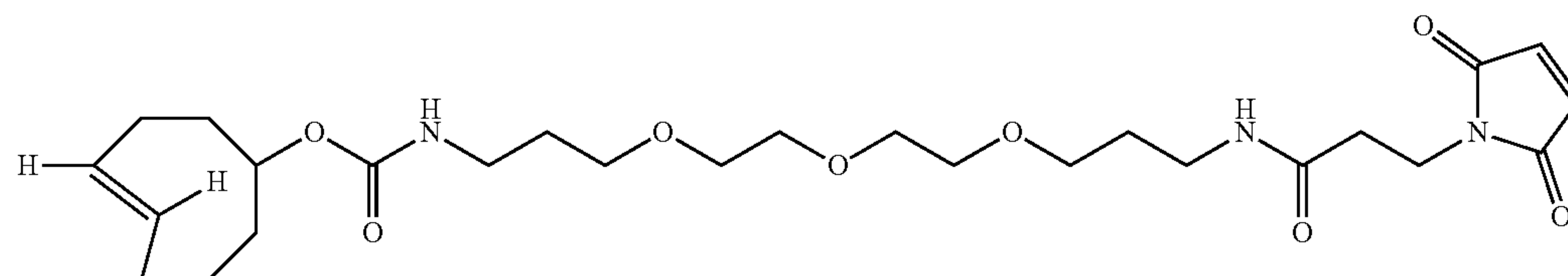
TCO-PEG3-Maleimide III
