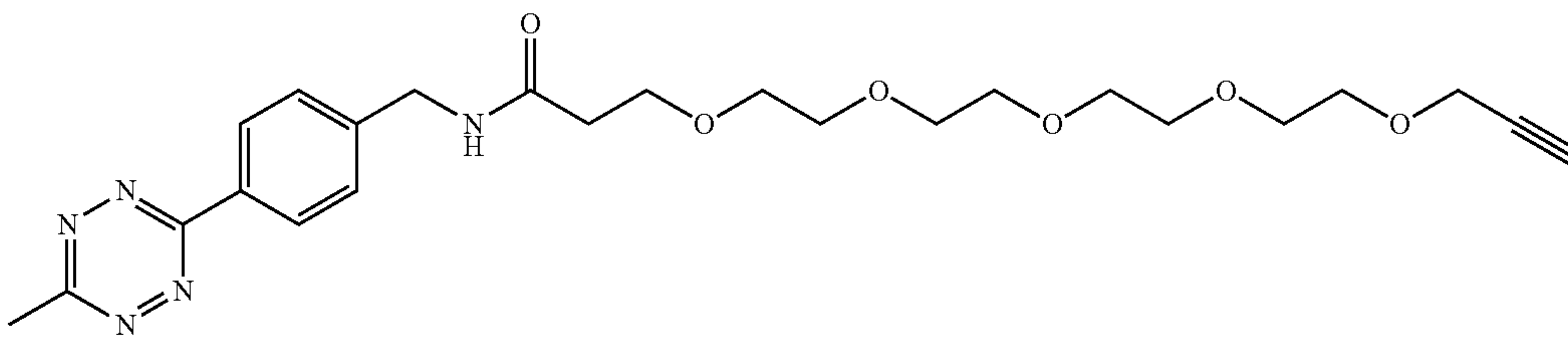
Tetrazine-PEG4-Alkyne XII
