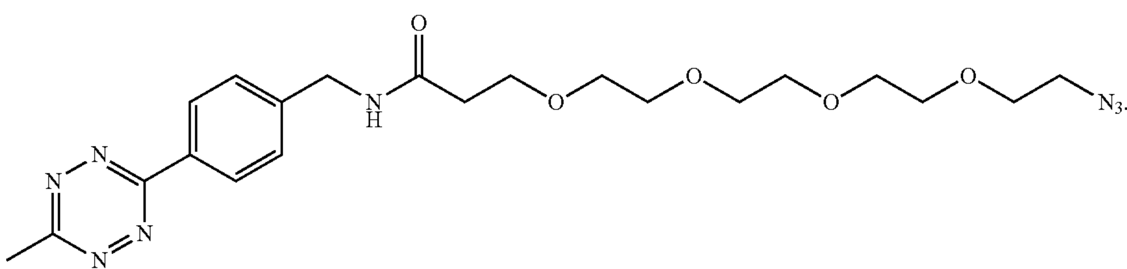
Tetrazine-PEG4-Azide XIV
