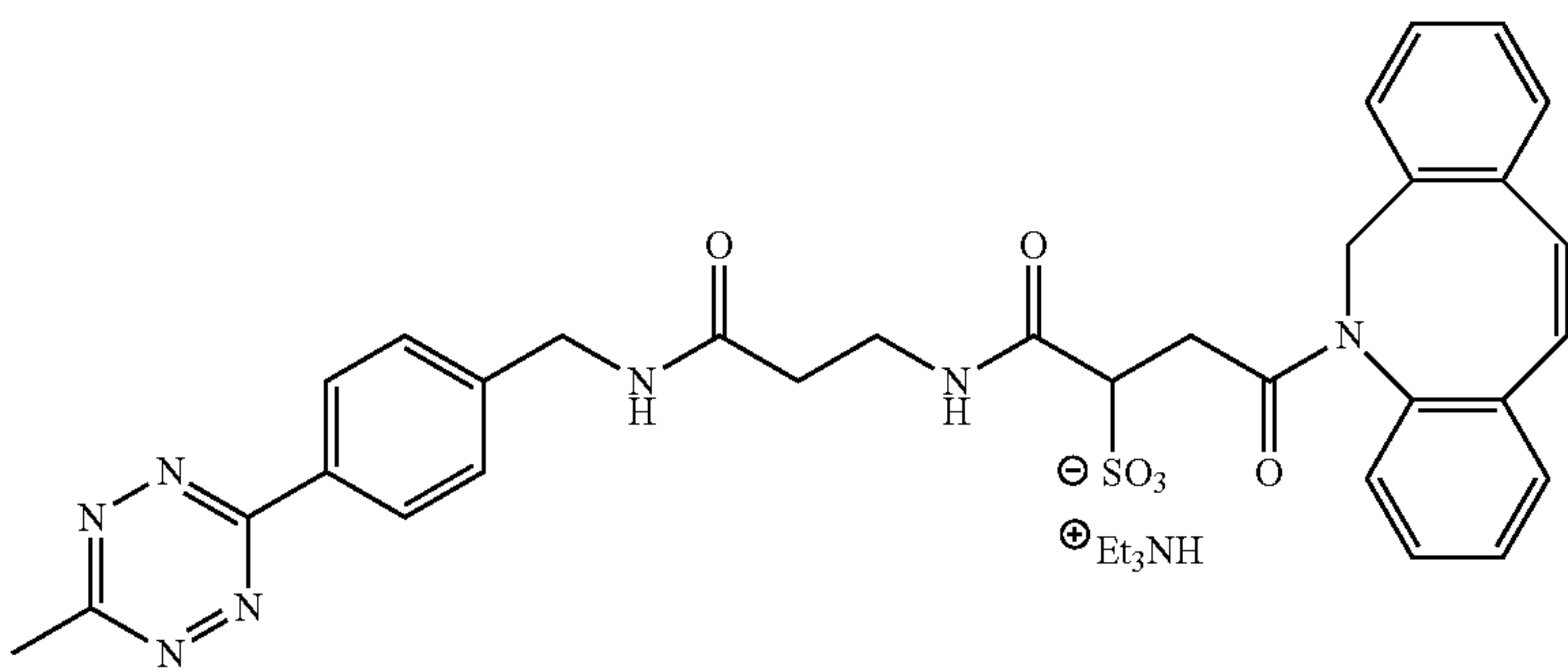
Tetrazine-DBCO XIII
