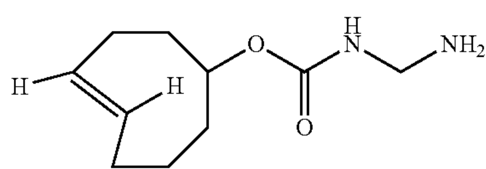
TCO-Amine IV
