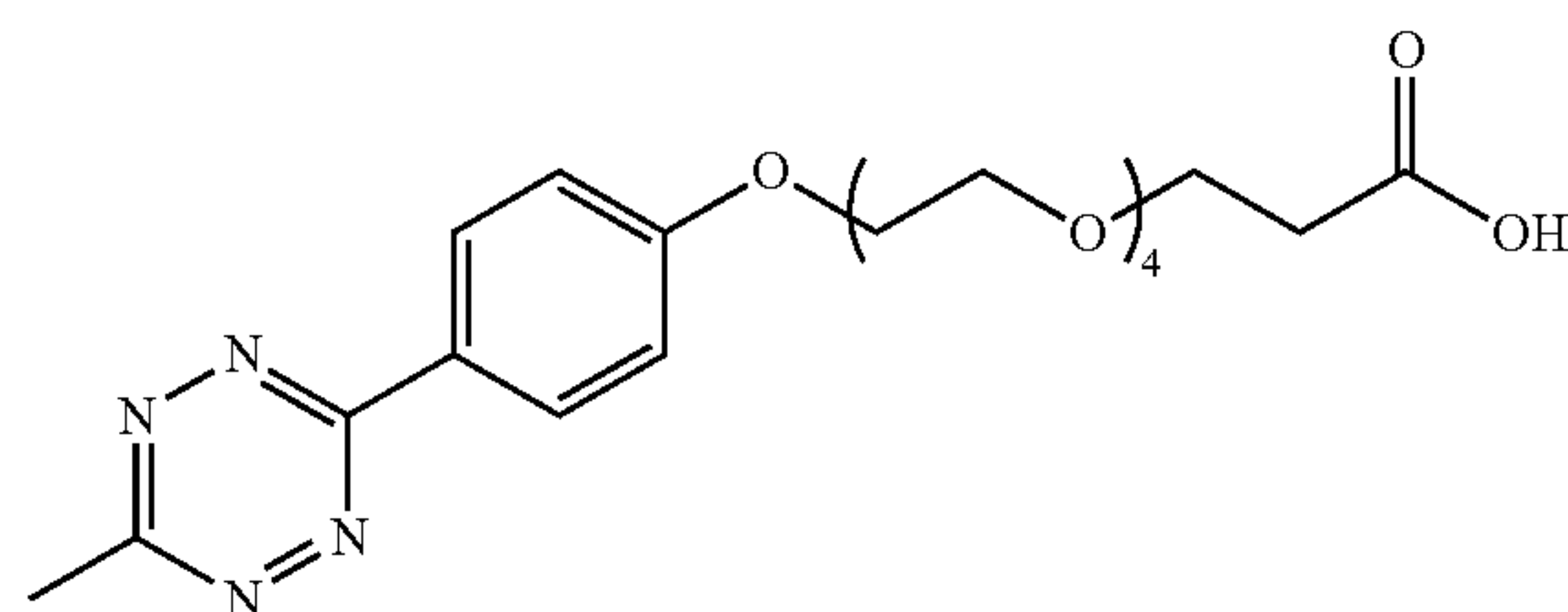
Tetrazine-PEG4-Acid IX
