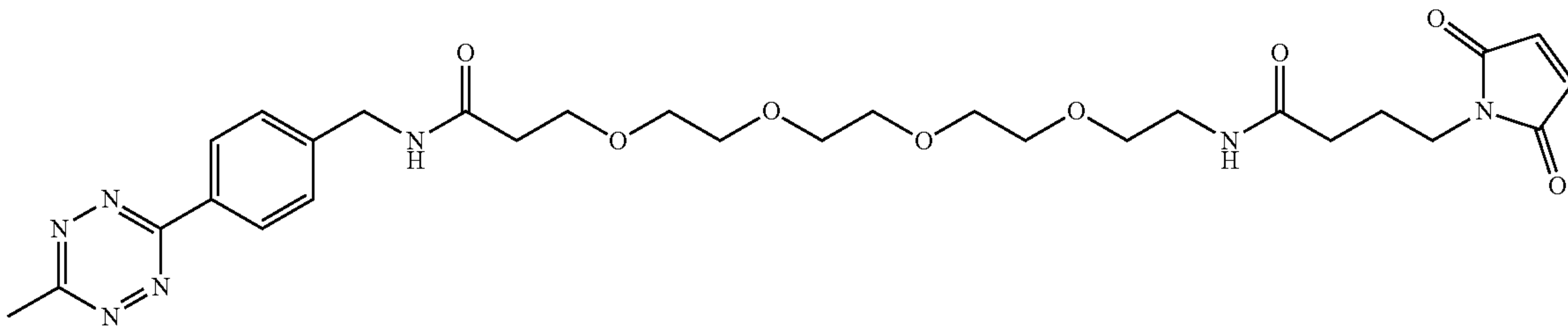
Tetrazine-PEG4-Maleimide XI
