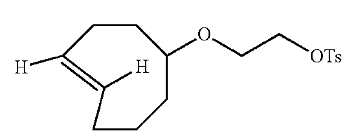
TCO-Tosyl VI
