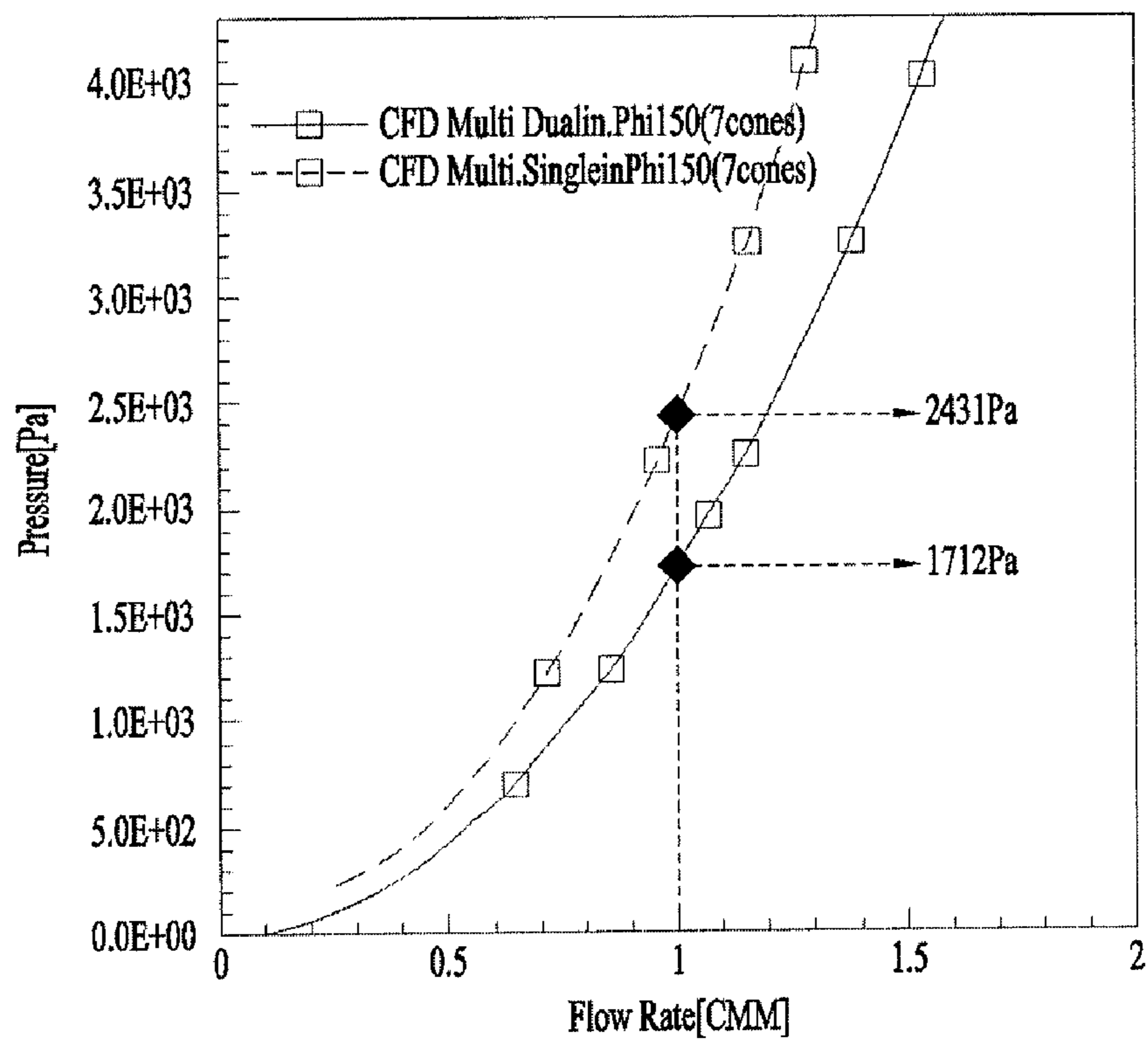
Figure 1. Comparison Pressure Loss between 2-in-1 & Multi
