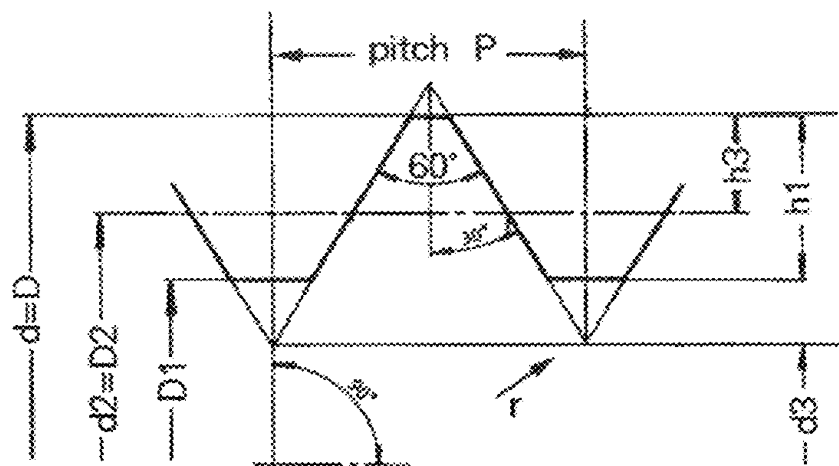
METRIC THREAD 60° PROFILE
