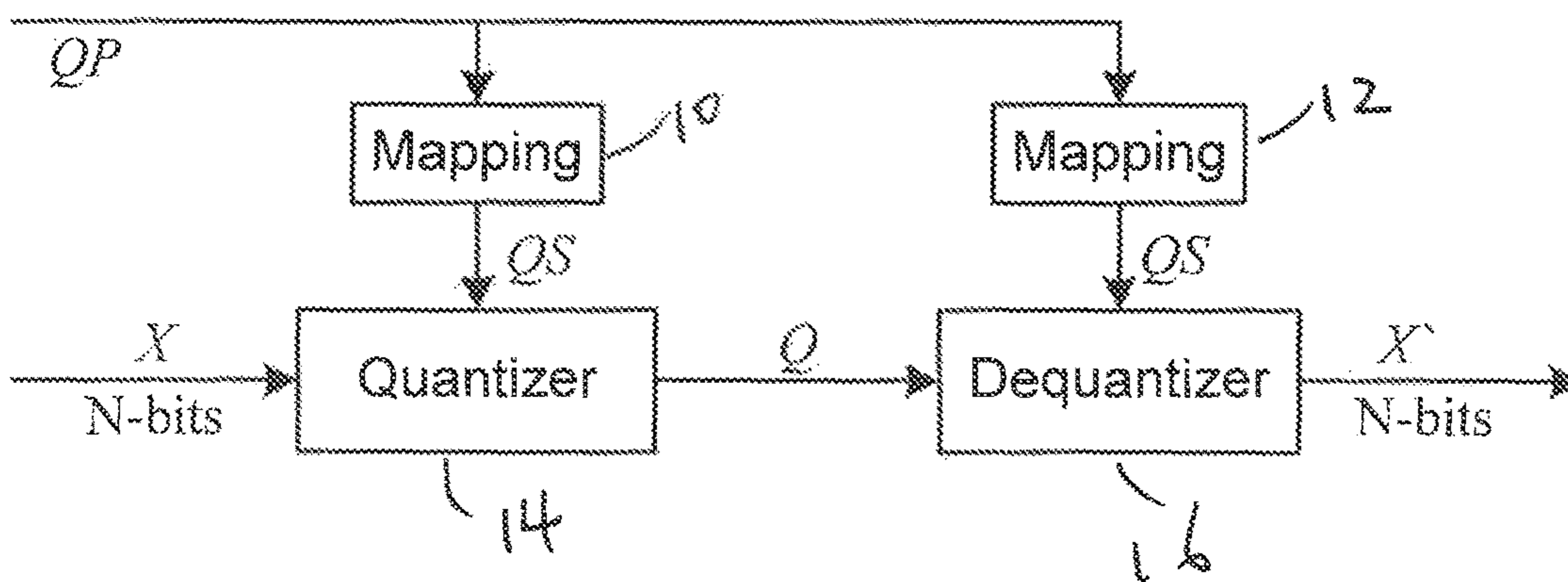
FIG. 4 Prior Art
