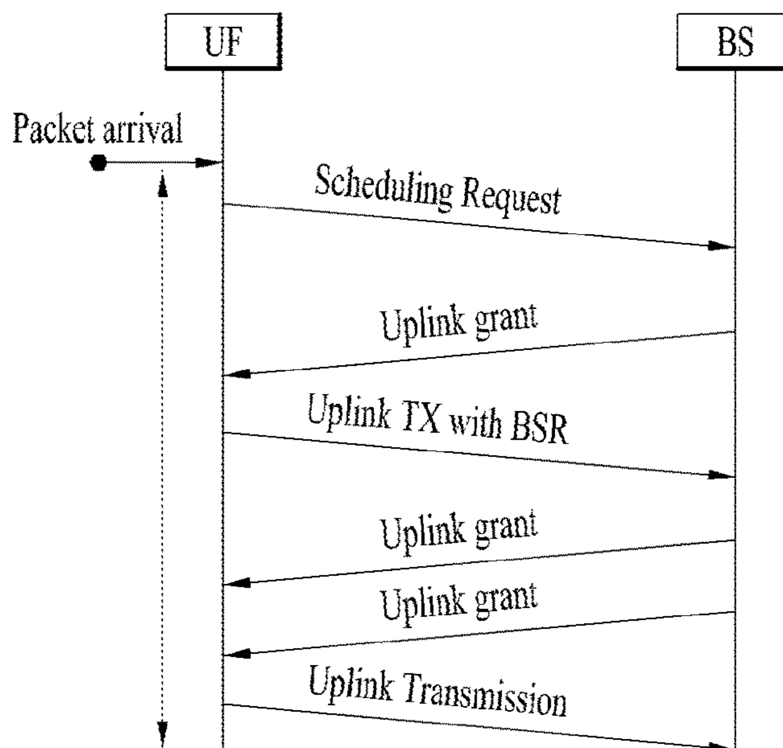
Fig. Uplink TX procedure with grant (a)
