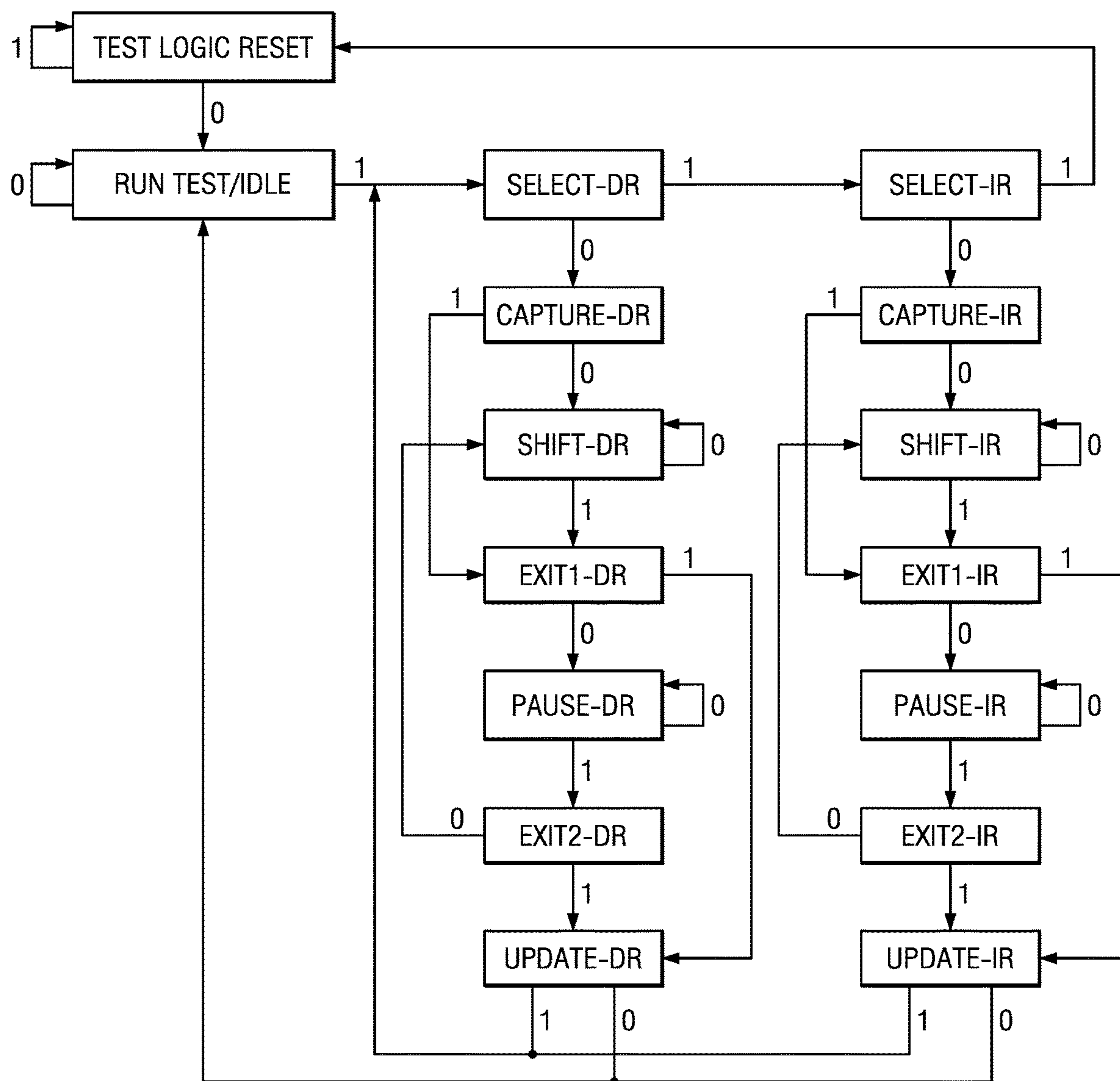
FIG. 4 (PRIOR ART)
