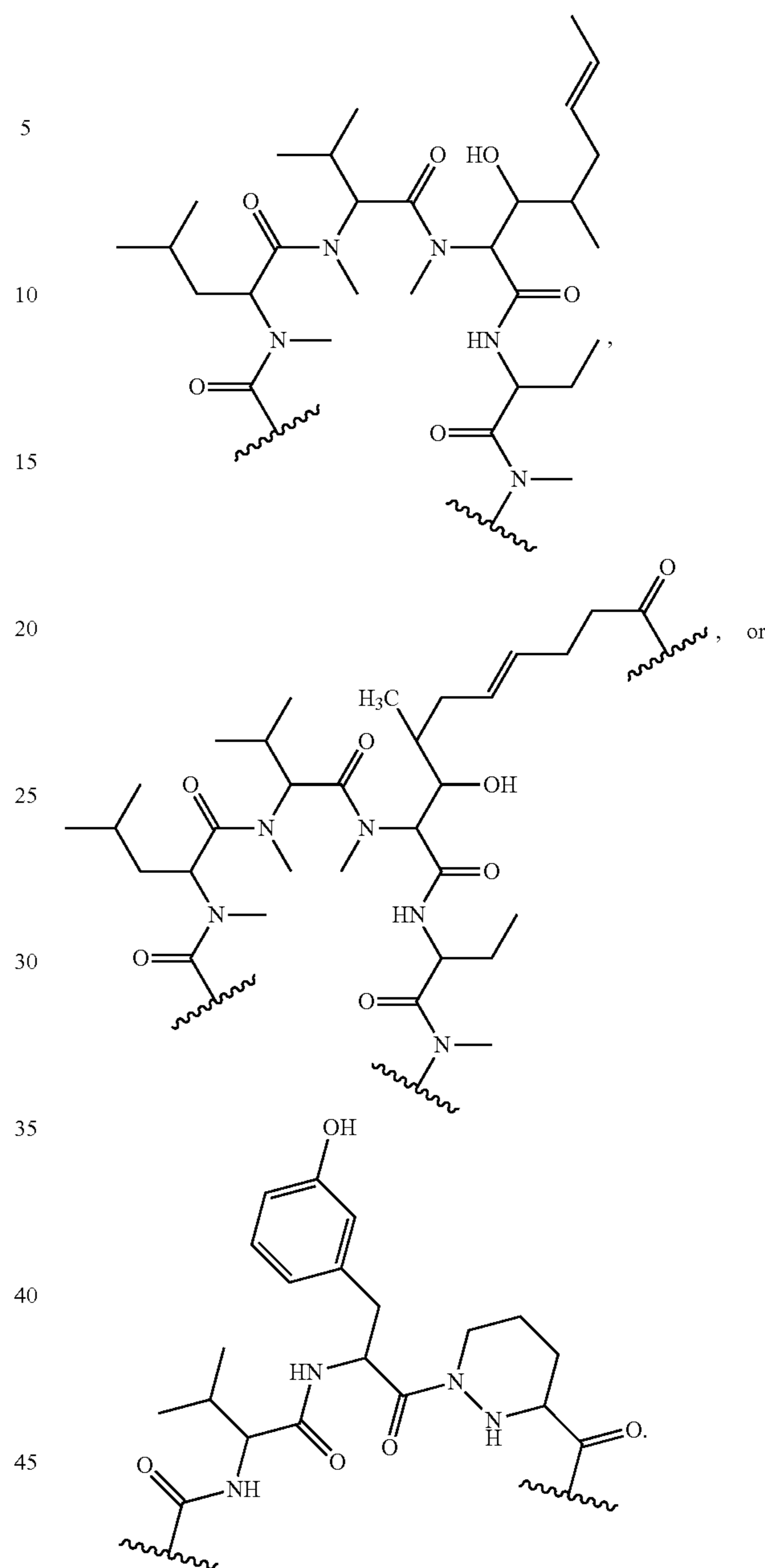
Formula IV
