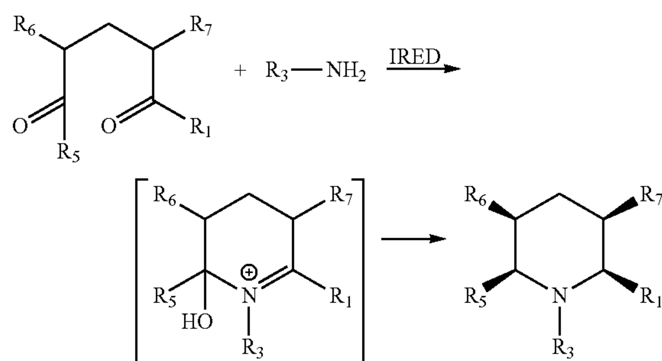
Scheme 6
