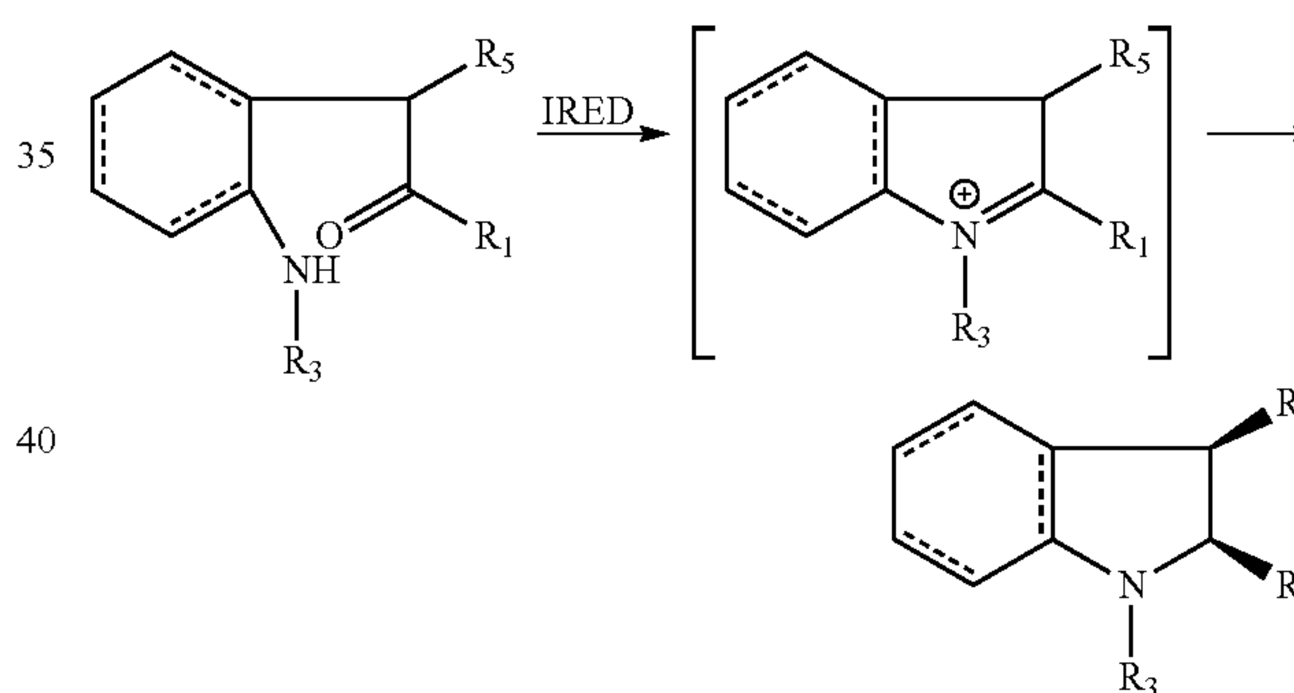
Scheme 5
