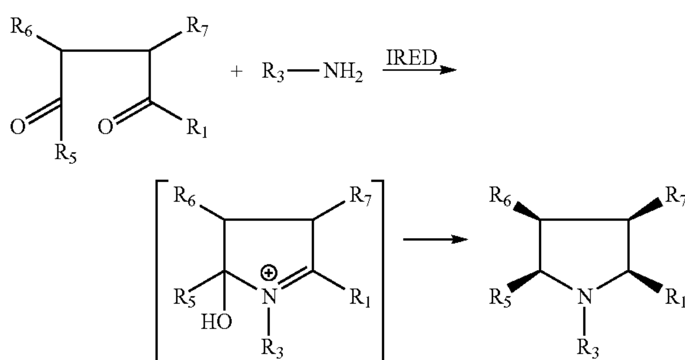
Scheme 8
