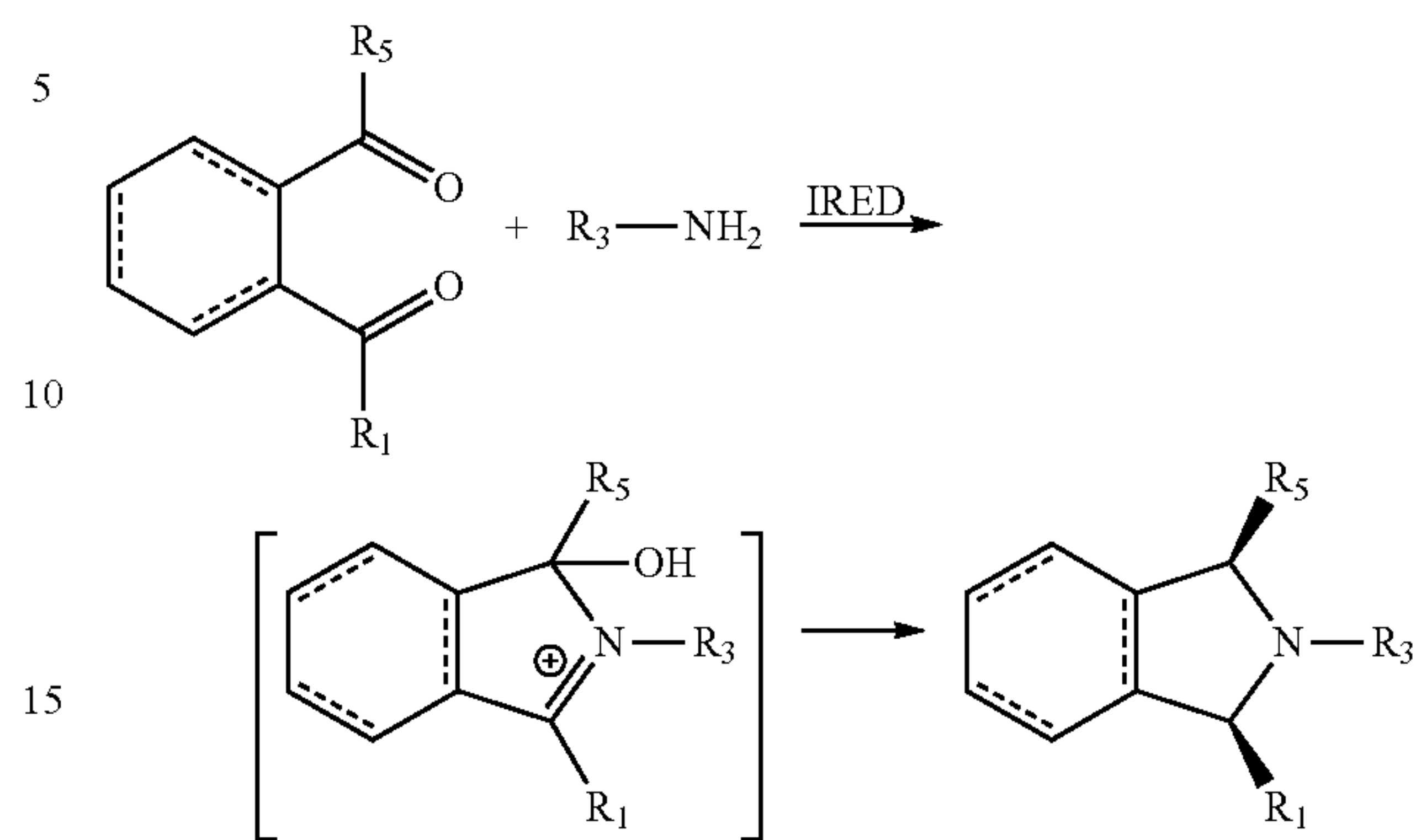
Scheme 9
