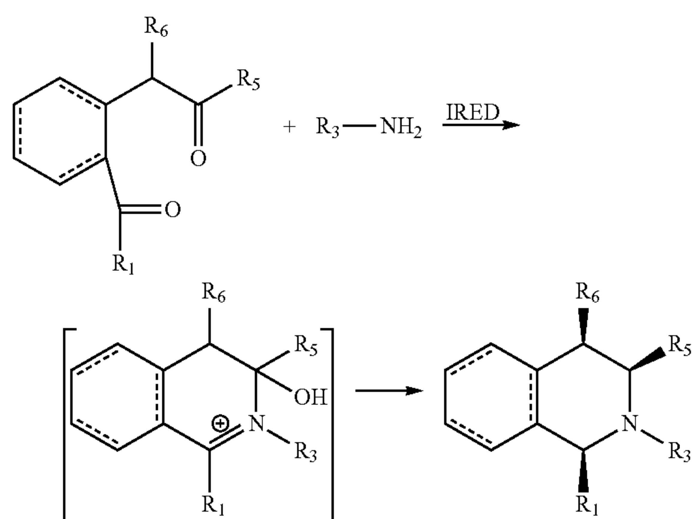
Scheme 8
