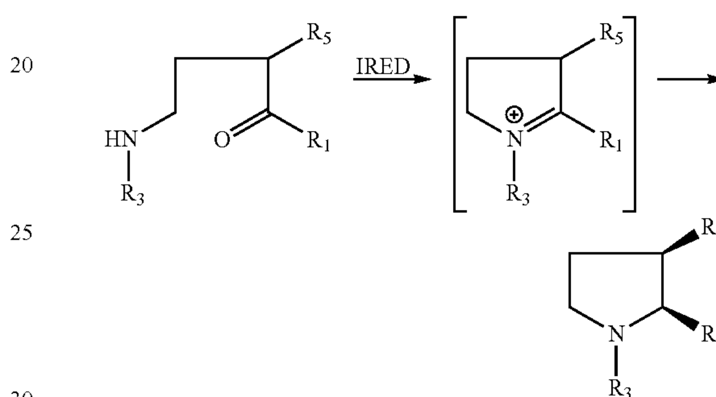
Scheme 5
