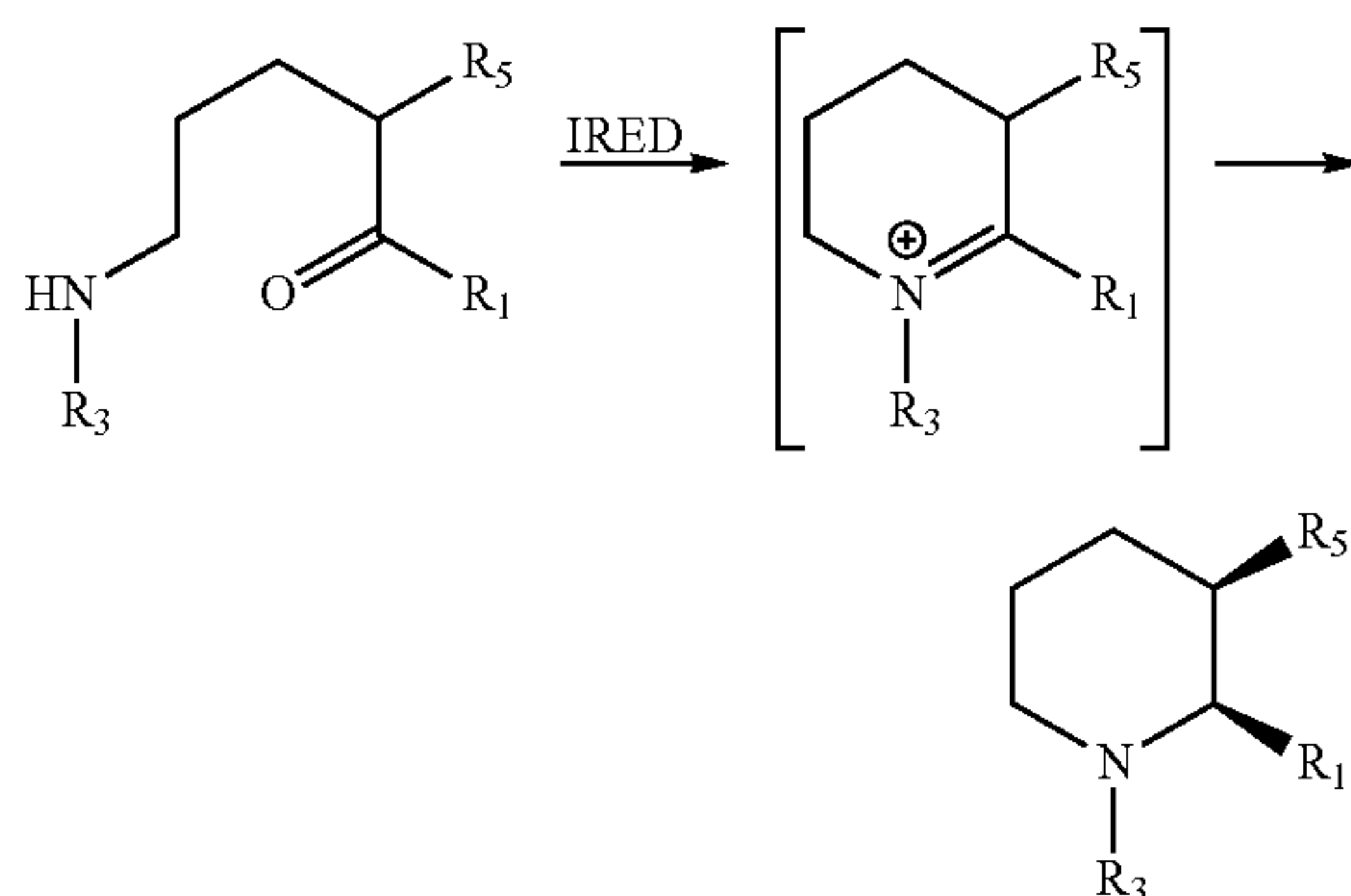
Scheme 2
